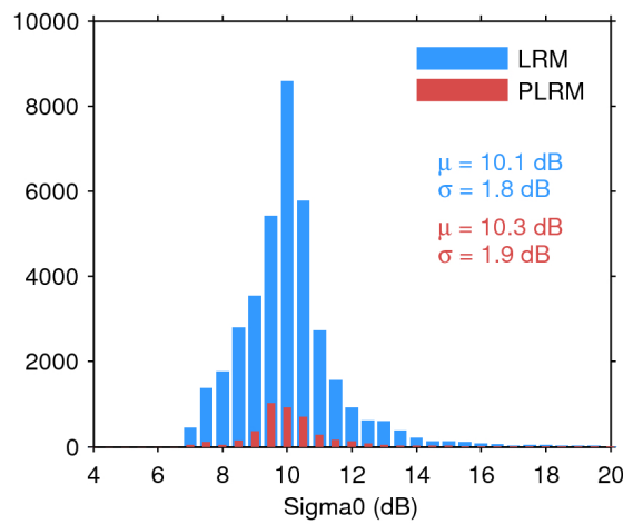
Figure 28. Histogram of science-valid sigma0 over oceans and lakes for LRM (blue) and PLRM (red) for 11/07/2017. The mean ( \mu ) and standard deviation ( \sigma ) are also shown. Note that values outside [4 20] dB are excluded from the histogram for the sake of readability but not from the computation of \mu and \sigma .
