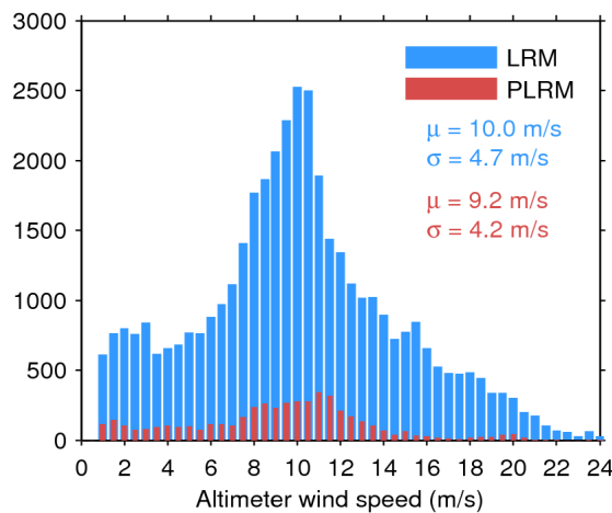
Figure 35. Histogram of science-valid wind over oceans and lakes for LRM (blue) and PLRM (red) for 11/07/2017. The mean ( \mu ) and standard deviation ( \sigma ) are also shown. Note that values larger than 24 m/s are excluded from the histogram for the sake of readability but not from the computation of \mu and \sigma .
