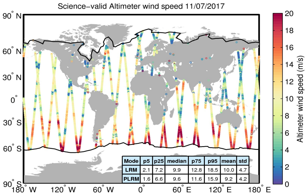
Figure 34. Geographical distribution of science-valid wind data over oceans and lakes for 11/07/2017. The statistical values shown in the table refer to the wind in m/s and are calculated separately for LRM and PLRM regions. The black lines mark the outer limit of the Arctic and Antarctic polar polygons. Gray circles denote records that have been rejected based on the editing criteria described in Table 5.
