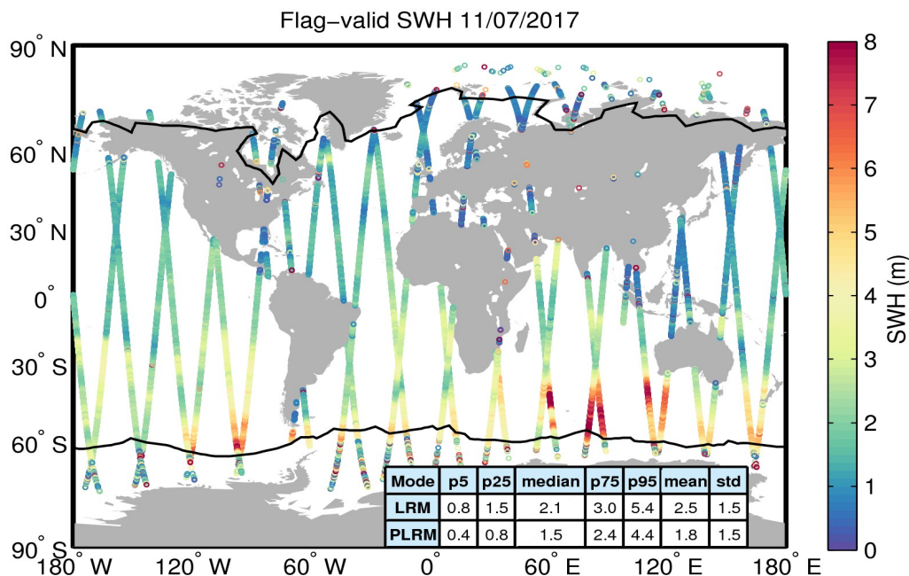
Figure 15. Geographical distribution of flag-valid SWH data over oceans and lakes for 11/07/2017. The statistical values shown in the table refer to the SWH in m and are calculated separately for LRM and PLRM regions. Measurements taken over polar polygons have been excluded from the computation of the statistical values. The black lines mark the outer limit of the Arctic and Antarctic polar polygons.
