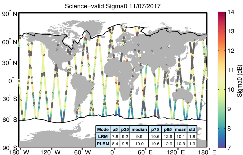
Figure 27. Geographical distribution of science-valid sigma0 data over oceans and lakes for 11/07/2017. The statistical values shown in the table refer to the sigma0 in dB and are calculated separately for LRM and PLRM regions. The black lines mark the outer limit of the Arctic and Antarctic polar polygons. Gray circles denote records that have been rejected based on the editing criteria described in Table 4.
