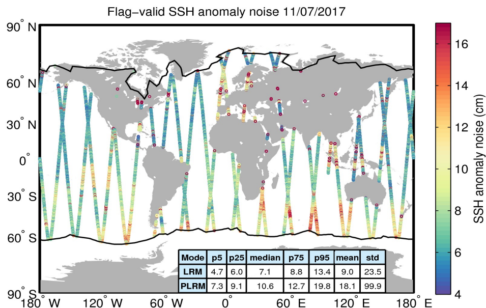
Figure 8. Geographical distribution of flag-valid 20-Hz SSH anomaly measurement noise over oceans and lakes for 11/07/2017. The statistical values shown in the table refer to the SSH anomaly noise and are calculated separately for LRM and PLRM regions. Measurements taken over polar polygons have been excluded from the computation of the statistical values. The black lines mark the outer limit of the Arctic and Antarctic polar polygons.
