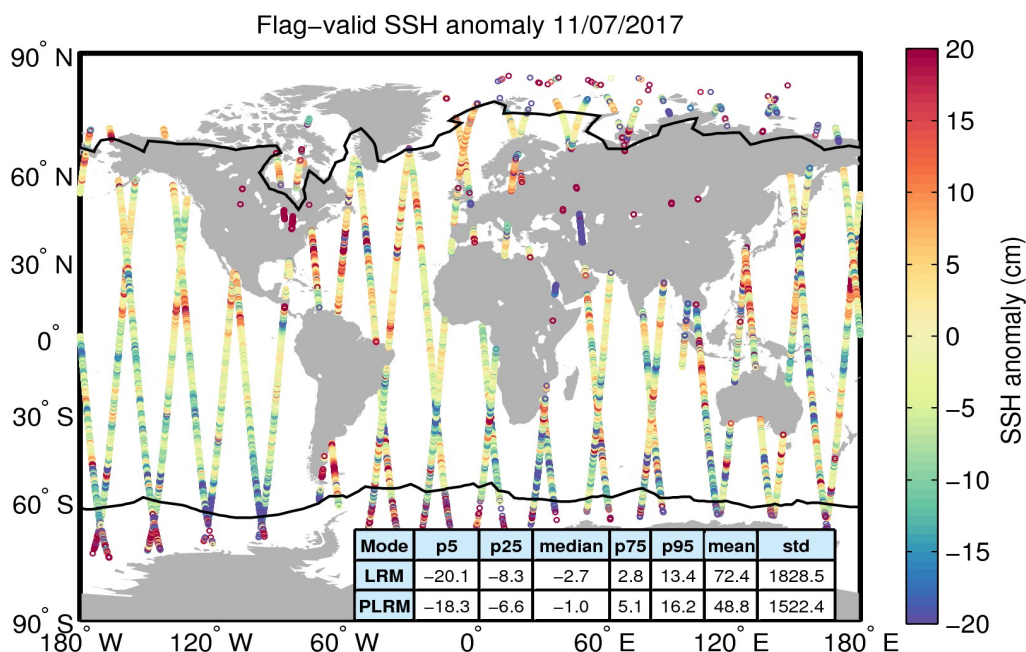
Figure 5. Geographical distribution of flag-valid 1-Hz SSH anomaly data over oceans and lakes for 11/07/2017. The statistical values shown in the table refer to the SSH anomaly in cm and are calculated separately for LRM and PLRM regions. Measurements taken over polar polygons have been excluded from the computation of the statistical values. The black lines mark the outer limit of the Arctic and Antarctic polar polygons.
