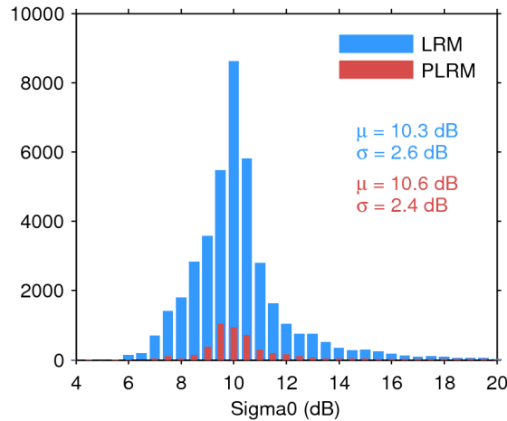
Figure 25. Histogram of flag-valid sigma0 over oceans and lakes for LRM (blue) and PLRM (red) for 11/07/2017. The mean ( \mu ) and standard deviation ( \sigma ) are also shown. Note that values outside [4 20] dB are excluded from the histogram for the sake of readability but not from the computation of \mu and \sigma .
