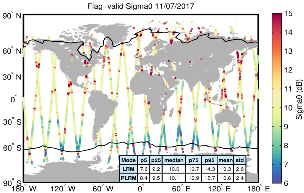
Figure 23. Geographical distribution of flag-valid sigma0 data over oceans and lakes for 11/07/2017. The statistical values shown in the table refer to the sigma0 in dB and are calculated separately for LRM and PLRM regions. Measurements taken over polar polygons have been excluded from the computation of the statistical values. The black lines mark the outer limit of the Arctic and Antarctic polar polygons.
