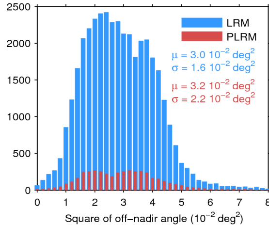
Figure 39. Histogram of flag-valid mispointing over oceans and lakes for LRM (blue) and PLRM (red) for 11/07/2017. Only positive values have been considered. The mean ( \mu ) and standard deviation ( \sigma ) are also shown. Note that values larger than 8 \cdot 10^{-2} \text{ deg}^2 are excluded from the histogram for the sake of readability but not from the computation of \mu and \sigma .
