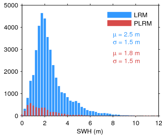
Figure 17. Histogram of flag-valid SWH over oceans and lakes for LRM (blue) and PLRM (red) for 11/07/2017. The mean ( \mu ) and standard deviation ( \sigma ) are also shown. Note that values larger than 12 m are excluded from the histogram for the sake of readability but not from the computation of \mu and \sigma .
