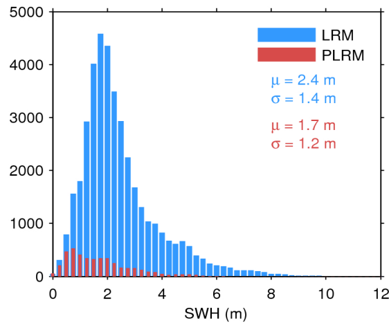
Figure 20. Histogram of science-valid SWH over oceans and lakes for LRM (blue) and PLRM (red) for 11/07/2017. The mean ( \mu ) and standard deviation ( \sigma ) are also shown. Note that values larger than 12 m are excluded from the histogram for the sake of readability but not from the computation of \mu and \sigma .
