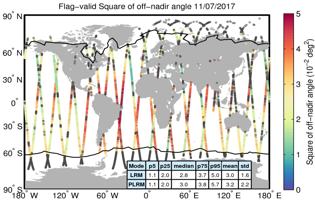
Figure 37. Geographical distribution of flag-valid mispointing data over oceans and lakes for 11/07/2017. The statistical values shown in the table refer to the mispointing in 10^{-2} deg 2 and are calculated separately for LRM and PLRM regions. Measurements taken over polar polygons have been excluded from the computation of the statistical values. The black lines mark the outer limit of the Arctic and Antarctic polar polygons. Gray circles denote negative values.
