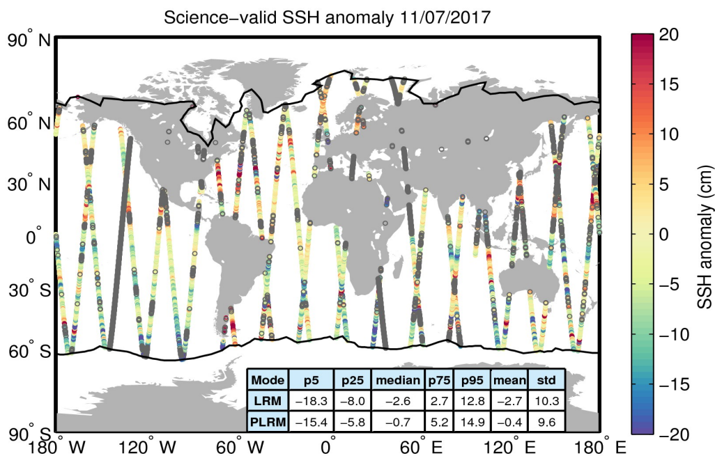
Figure 10. Geographical distribution of science-valid SSH anomaly data over oceans and lakes for 11/07/2017. The statistical values shown in the table refer to the SSH anomaly in cm and are calculated separately for LRM and PLRM regions. The black lines mark the outer limit of the Arctic and Antarctic polar polygons. Gray circles denote records that have been rejected based on the editing criteria described in Table 2.
