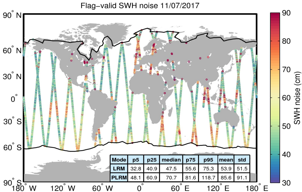
Figure 18. Geographical distribution of flag-valid 20-Hz SWH measurement noise over oceans and lakes for 11/07/2017. The statistical values shown in the table refer to the SWH noise and are calculated separately for LRM and PLRM regions. Measurements taken over polar polygons have been excluded from the computation of the statistical values. The black lines mark the outer limit of the Arctic and Antarctic polar polygons.
