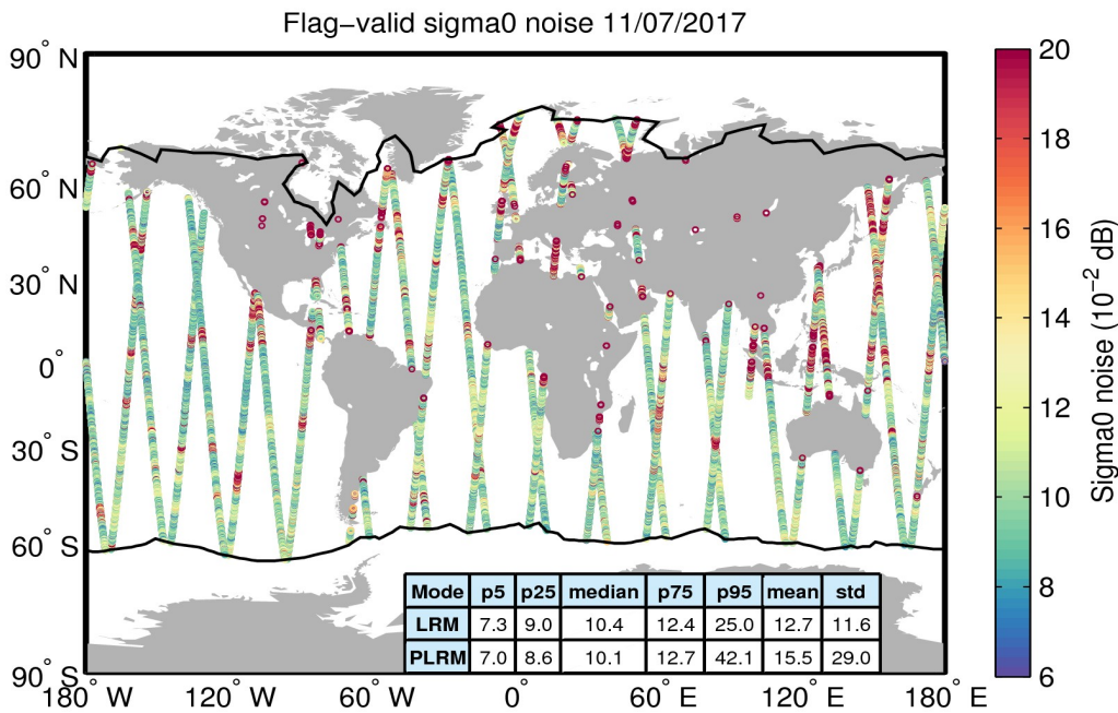
Figure 26. Geographical distribution of flag-valid 20-Hz sigma0 measurement noise over oceans and lakes for 11/07/2017. The statistical values shown in the table refer to the sigma0 noise and are calculated separately for LRM and PLRM regions. Measurements taken over polar polygons have been excluded from the computation of the statistical values. The black lines mark the outer limit of the Arctic and Antarctic polar polygons.
