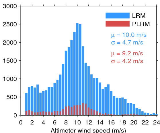
Figure 33. Histogram of flag-valid wind over oceans and lakes for LRM (blue) and PLRM (red) for 11/07/2017. The mean ( \mu ) and standard deviation ( \sigma ) are also shown. Note that values larger than 24 m/s are excluded from the histogram for the sake of readability but not from the computation of \mu and \sigma .
