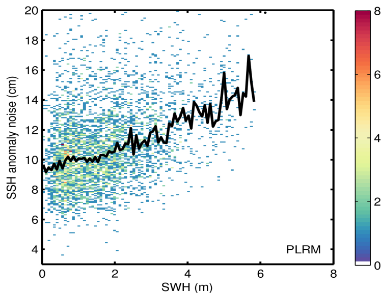
Figure 9. 2D histogram showing flag-valid SSH anomaly noise as a function of SWH for LRM (top) and PLRM (bottom) for 11/07/2017. The black line denotes the median SSH anomaly noise as a function of SWH.
