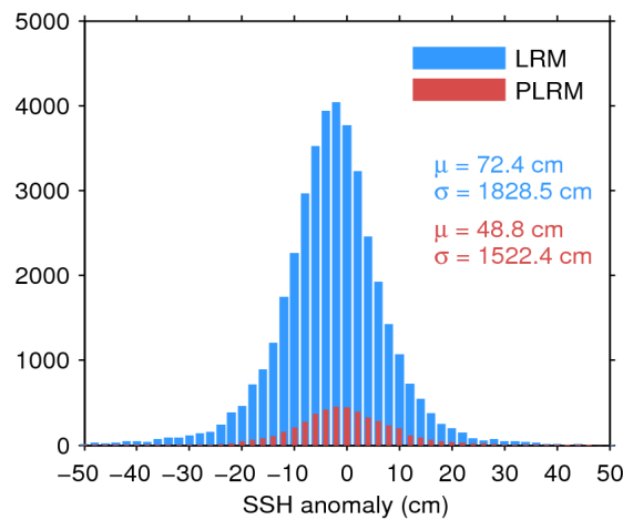
Figure 7. Histogram of flag-valid SSH anomaly over oceans and lakes for LRM (blue) and PLRM (red) for 11/07/2017. The mean ( \mu ) and standard deviation ( \sigma ) are also shown. Note that values outside [-50 50] cm are excluded from the histogram for the sake of readability but not from the computation of \mu and \sigma .
