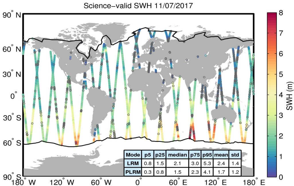
Figure 19. Geographical distribution of science-valid SWH data over oceans and lakes for 11/07/2017. The statistical values shown in the table refer to the SWH in m and are calculated separately for LRM and PLRM regions. The black lines mark the outer limit of the Arctic and Antarctic polar polygons. Gray circles denote records that have been rejected based on the editing criteria described in Table 3.
