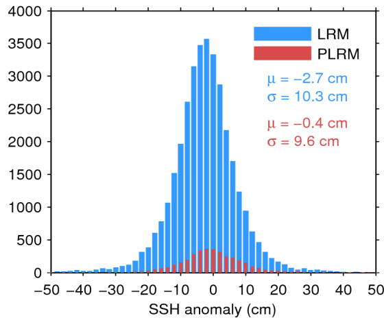
Figure 11. Histogram of science-valid SSH anomaly over oceans and lakes for LRM (blue) and PLRM (red) for 11/07/2017. The mean ( \mu ) and standard deviation ( \sigma ) are also shown. Note that values outside [-50\ 50] cm are excluded from the histogram for the sake of readability but not from the computation of \mu and \sigma .
