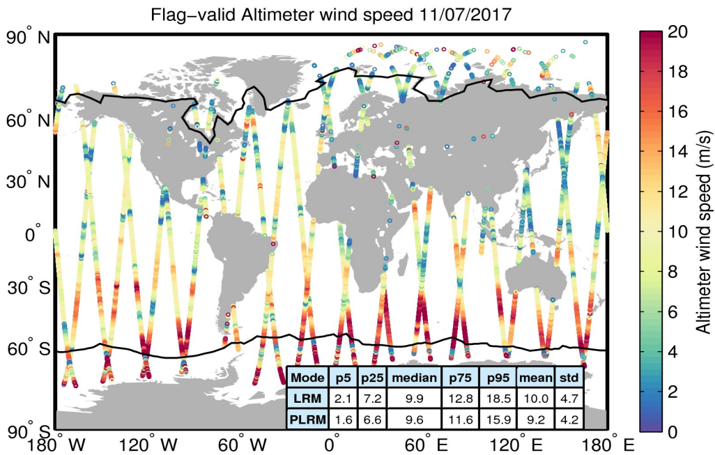
Figure 31. Geographical distribution of flag-valid wind data over oceans and lakes for 11/07/2017. The statistical values shown in the table refer to the wind in m/s and are calculated separately for LRM and PLRM regions. Measurements taken over polar polygons have been excluded from the computation of the statistical values. The black lines mark the outer limit of the Arctic and Antarctic polar polygons.
