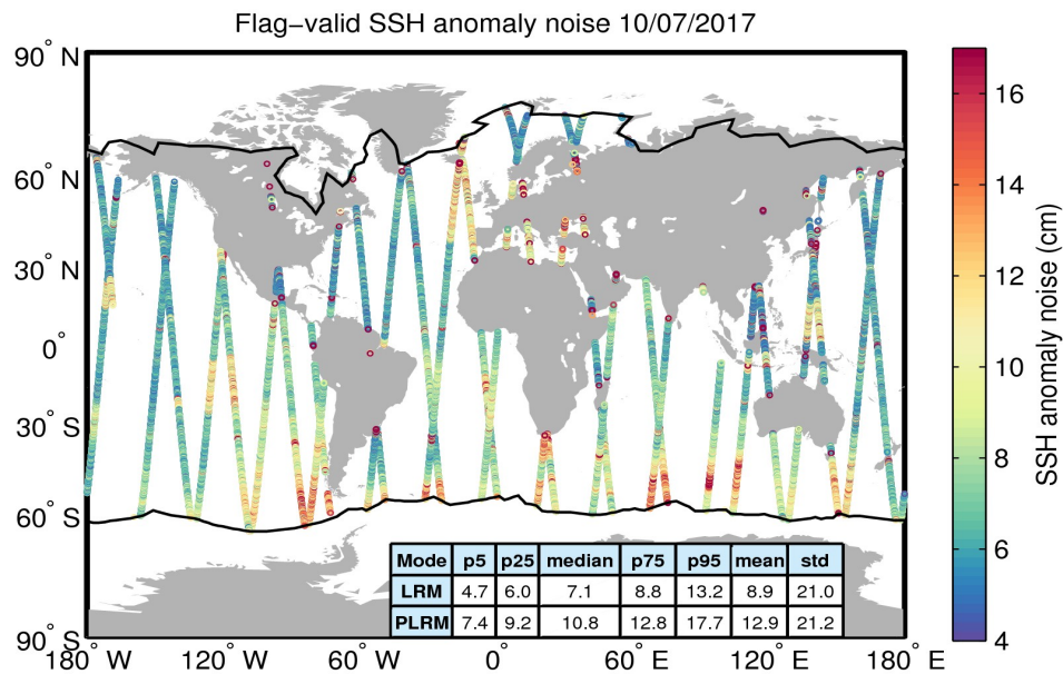
Figure 8. Geographical distribution of flag-valid 20-Hz SSH anomaly measurement noise over oceans and lakes for 10/07/2017. The statistical values shown in the table refer to the SSH anomaly noise and are calculated separately for LRM and PLRM regions. Measurements taken over polar polygons have been excluded from the computation of the statistical values. The black lines mark the outer limit of the Arctic and Antarctic polar polygons.
