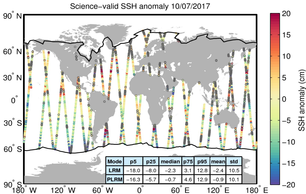
Figure 10. Geographical distribution of science-valid SSH anomaly data over oceans and lakes for 10/07/2017. The statistical values shown in the table refer to the SSH anomaly in cm and are calculated separately for LRM and PLRM regions. The black lines mark the outer limit of the Arctic and Antarctic polar polygons. Gray circles denote records that have been rejected based on the editing criteria described in Table 2.
