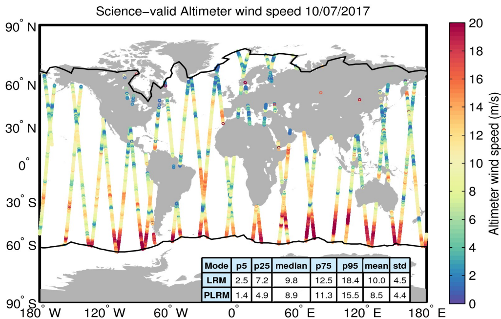
Figure 34. Geographical distribution of science-valid wind data over oceans and lakes for 10/07/2017. The statistical values shown in the table refer to the wind in m/s and are calculated separately for LRM and PLRM regions. The black lines mark the outer limit of the Arctic and Antarctic polar polygons. Gray circles denote records that have been rejected based on the editing criteria described in Table 5.
