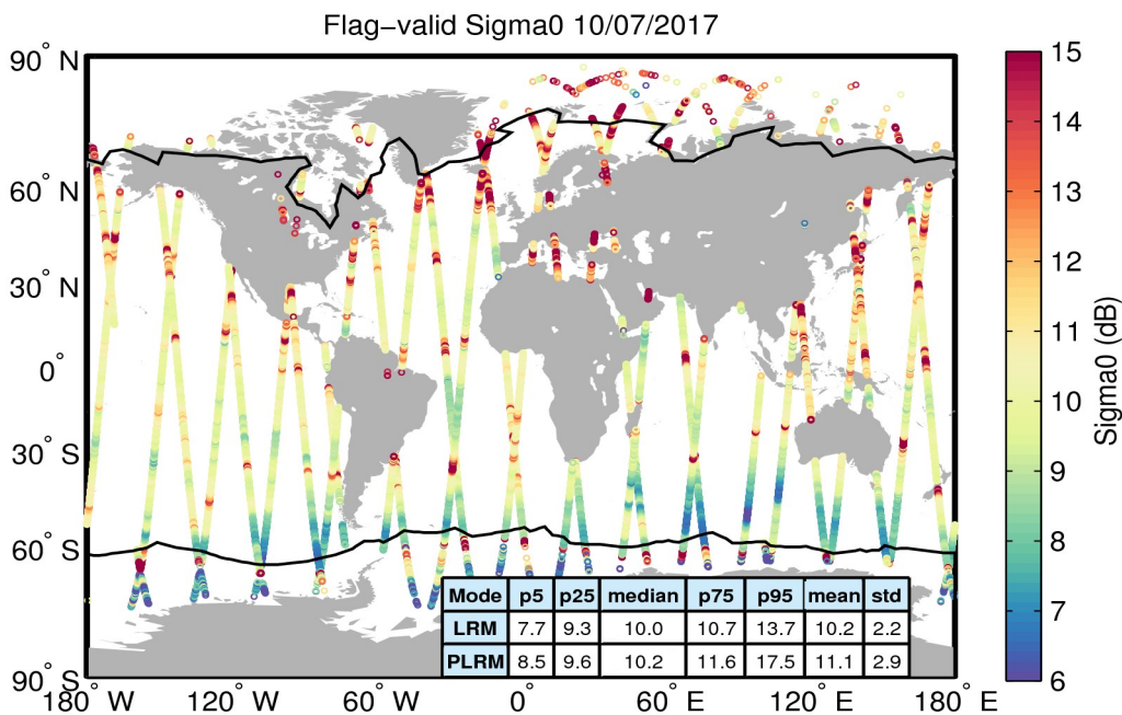
Figure 23. Geographical distribution of flag-valid sigma0 data over oceans and lakes for 10/07/2017. The statistical values shown in the table refer to the sigma0 in dB and are calculated separately for LRM and PLRM regions. Measurements taken over polar polygons have been excluded from the computation of the statistical values. The black lines mark the outer limit of the Arctic and Antarctic polar polygons.
