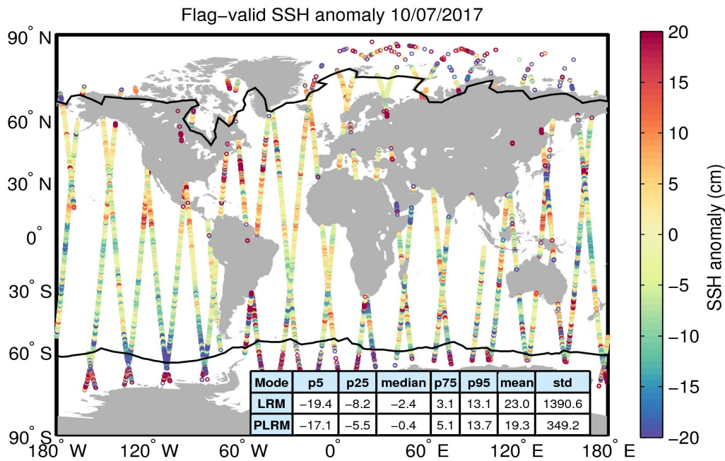
Figure 5. Geographical distribution of flag-valid 1-Hz SSH anomaly data over oceans and lakes for 10/07/2017. The statistical values shown in the table refer to the SSH anomaly in cm and are calculated separately for LRM and PLRM regions. Measurements taken over polar polygons have been excluded from the computation of the statistical values. The black lines mark the outer limit of the Arctic and Antarctic polar polygons.
