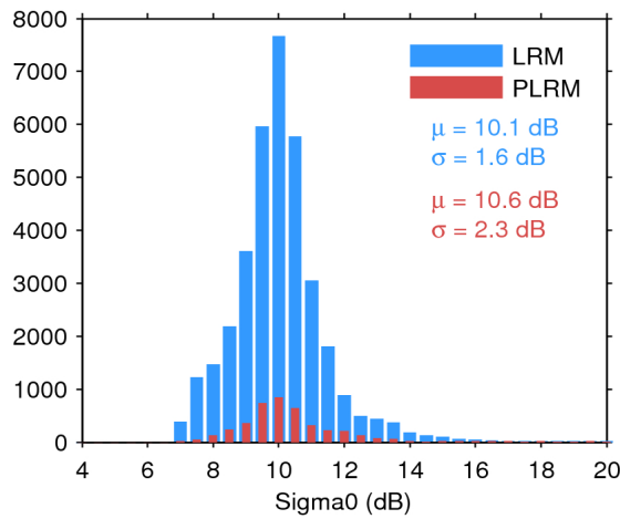
Figure 28. Histogram of science-valid sigma0 over oceans and lakes for LRM (blue) and PLRM (red) for 10/07/2017. The mean ( \mu ) and standard deviation ( \sigma ) are also shown. Note that values outside [4 20] dB are excluded from the histogram for the sake of readability but not from the computation of \mu and \sigma .
