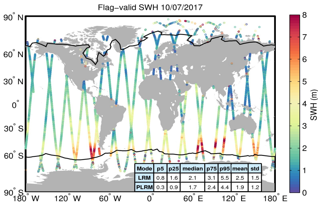
Figure 15. Geographical distribution of flag-valid SWH data over oceans and lakes for 10/07/2017. The statistical values shown in the table refer to the SWH in m and are calculated separately for LRM and PLRM regions. Measurements taken over polar polygons have been excluded from the computation of the statistical values. The black lines mark the outer limit of the Arctic and Antarctic polar polygons.
