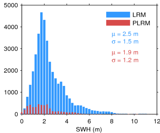
Figure 17. Histogram of flag-valid SWH over oceans and lakes for LRM (blue) and PLRM (red) for 10/07/2017. The mean ( \mu ) and standard deviation ( \sigma ) are also shown. Note that values larger than 12 m are excluded from the histogram for the sake of readability but not from the computation of \mu and \sigma .
