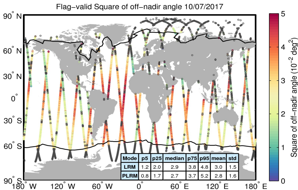
Figure 37. Geographical distribution of flag-valid mispointing data over oceans and lakes for 10/07/2017. The statistical values shown in the table refer to the mispointing in 10^{-2} deg 2 and are calculated separately for LRM and PLRM regions. Measurements taken over polar polygons have been excluded from the computation of the statistical values. The black lines mark the outer limit of the Arctic and Antarctic polar polygons. Gray circles denote negative values.
