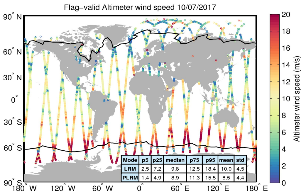
Figure 31. Geographical distribution of flag-valid wind data over oceans and lakes for 10/07/2017. The statistical values shown in the table refer to the wind in m/s and are calculated separately for LRM and PLRM regions. Measurements taken over polar polygons have been excluded from the computation of the statistical values. The black lines mark the outer limit of the Arctic and Antarctic polar polygons.
