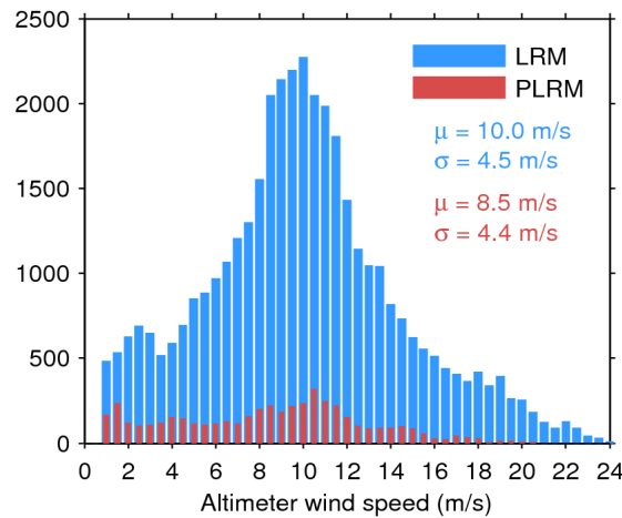
Figure 33. Histogram of flag-valid wind over oceans and lakes for LRM (blue) and PLRM (red) for 10/07/2017. The mean ( \mu ) and standard deviation ( \sigma ) are also shown. Note that values larger than 24 m/s are excluded from the histogram for the sake of readability but not from the computation of \mu and \sigma .
