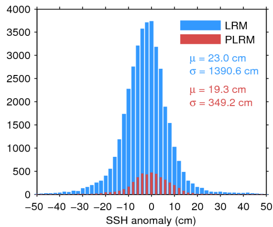
Figure 7. Histogram of flag-valid SSH anomaly over oceans and lakes for LRM (blue) and PLRM (red) for 10/07/2017. The mean ( \mu ) and standard deviation ( \sigma ) are also shown. Note that values outside [-50\ 50] cm are excluded from the histogram for the sake of readability but not from the computation of \mu and \sigma .
