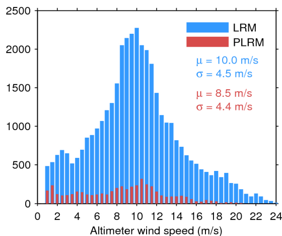
Figure 35. Histogram of science-valid wind over oceans and lakes for LRM (blue) and PLRM (red) for 10/07/2017. The mean ( \mu ) and standard deviation ( \sigma ) are also shown. Note that values larger than 24 m/s are excluded from the histogram for the sake of readability but not from the computation of \mu and \sigma .
