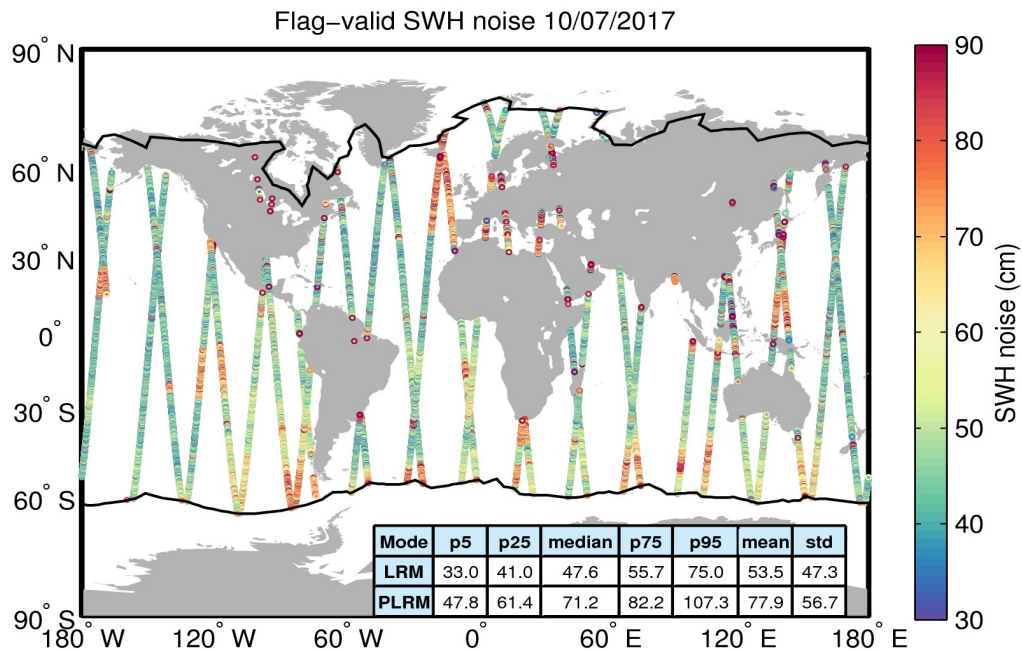
Figure 18. Geographical distribution of flag-valid 20-Hz SWH measurement noise over oceans and lakes for 10/07/2017. The statistical values shown in the table refer to the SWH noise and are calculated separately for LRM and PLRM regions. Measurements taken over polar polygons have been excluded from the computation of the statistical values. The black lines mark the outer limit of the Arctic and Antarctic polar polygons.
