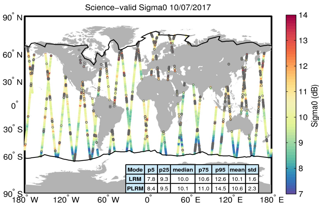
Figure 27. Geographical distribution of science-valid sigma0 data over oceans and lakes for 10/07/2017. The statistical values shown in the table refer to the sigma0 in dB and are calculated separately for LRM and PLRM regions. The black lines mark the outer limit of the Arctic and Antarctic polar polygons. Gray circles denote records that have been rejected based on the editing criteria described in Table 4.
