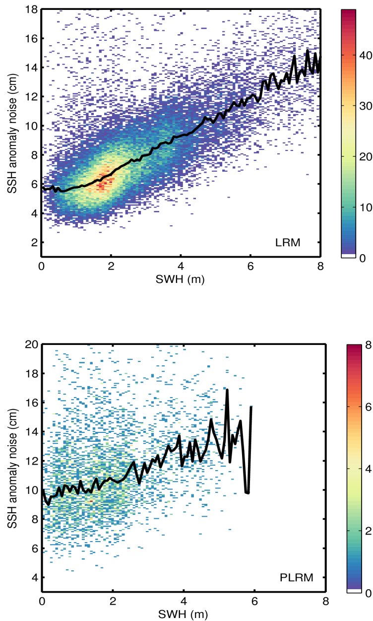
Figure 9. 2D histogram showing flag-valid SSH anomaly noise as a function of SWH for LRM (top) and PLRM (bottom) for 10/07/2017. The black line denotes the median SSH anomaly noise as a function of SWH.
