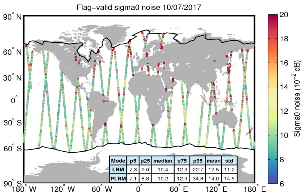
Figure 26. Geographical distribution of flag-valid 20-Hz sigma0 measurement noise over oceans and lakes for 10/07/2017. The statistical values shown in the table refer to the sigma0 noise and are calculated separately for LRM and PLRM regions. Measurements taken over polar polygons have been excluded from the computation of the statistical values. The black lines mark the outer limit of the Arctic and Antarctic polar polygons.
