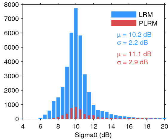
Figure 25. Histogram of flag-valid sigma0 over oceans and lakes for LRM (blue) and PLRM (red) for 10/07/2017. The mean ( \mu ) and standard deviation ( \sigma ) are also shown. Note that values outside [4 20] dB are excluded from the histogram for the sake of readability but not from the computation of \mu and \sigma .
