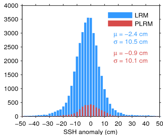
Figure 11. Histogram of science-valid SSH anomaly over oceans and lakes for LRM (blue) and PLRM (red) for 10/07/2017. The mean ( \mu ) and standard deviation ( \sigma ) are also shown. Note that values outside [-50 50] cm are excluded from the histogram for the sake of readability but not from the computation of \mu and \sigma .
