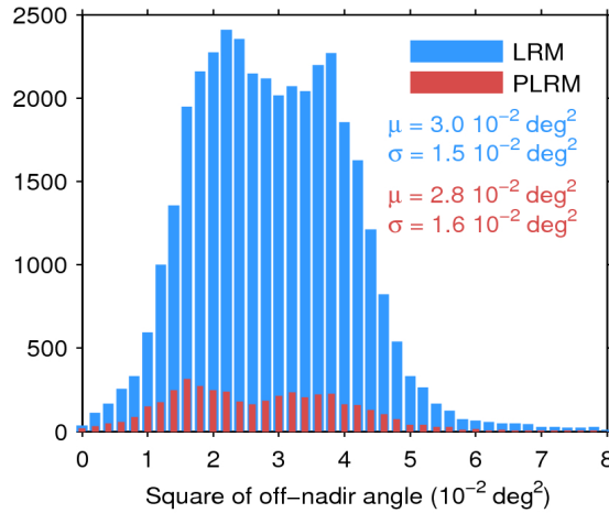
Figure 39. Histogram of flag-valid mispointing over oceans and lakes for LRM (blue) and PLRM (red) for 10/07/2017. Only positive values have been considered. The mean ( \mu ) and standard deviation ( \sigma ) are also shown. Note that values larger than 8 \cdot 10^{-2} \text{ deg}^2 are excluded from the histogram for the sake of readability but not from the computation of \mu and \sigma .
