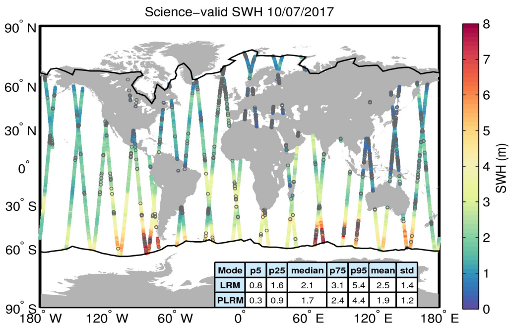
Figure 19. Geographical distribution of science-valid SWH data over oceans and lakes for 10/07/2017. The statistical values shown in the table refer to the SWH in m and are calculated separately for LRM and PLRM regions. The black lines mark the outer limit of the Arctic and Antarctic polar polygons. Gray circles denote records that have been rejected based on the editing criteria described in Table 3.
