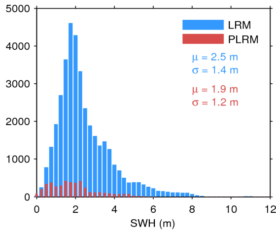
Figure 20. Histogram of science-valid SWH over oceans and lakes for LRM (blue) and PLRM (red) for 10/07/2017. The mean ( \mu ) and standard deviation ( \sigma ) are also shown. Note that values larger than 12 m are excluded from the histogram for the sake of readability but not from the computation of \mu and \sigma .
