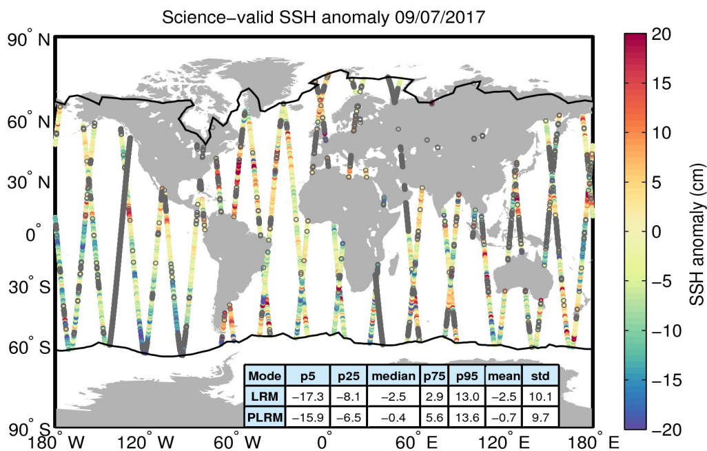
Figure 10. Geographical distribution of science-valid SSH anomaly data over oceans and lakes for 09/07/2017. The statistical values shown in the table refer to the SSH anomaly in cm and are calculated separately for LRM and PLRM regions. The black lines mark the outer limit of the Arctic and Antarctic polar polygons. Gray circles denote records that have been rejected based on the editing criteria described in Table 2.
