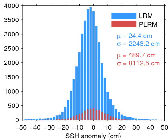
Figure 7. Histogram of flag-valid SSH anomaly over oceans and lakes for LRM (blue) and PLRM (red) for 09/07/2017. The mean ( \mu ) and standard deviation ( \sigma ) are also shown. Note that values outside [-50 \ 50] cm are excluded from the histogram for the sake of readability but not from the computation of \mu and \sigma .
