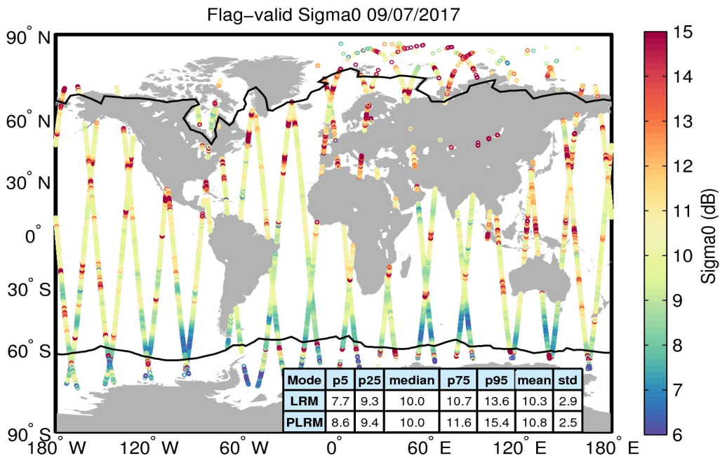
Figure 23. Geographical distribution of flag-valid sigma0 data over oceans and lakes for 09/07/2017. The statistical values shown in the table refer to the sigma0 in dB and are calculated separately for LRM and PLRM regions. Measurements taken over polar polygons have been excluded from the computation of the statistical values. The black lines mark the outer limit of the Arctic and Antarctic polar polygons.
