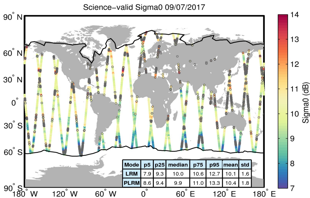
Figure 27. Geographical distribution of science-valid sigma0 data over oceans and lakes for 09/07/2017. The statistical values shown in the table refer to the sigma0 in dB and are calculated separately for LRM and PLRM regions. The black lines mark the outer limit of the Arctic and Antarctic polar polygons. Gray circles denote records that have been rejected based on the editing criteria described in Table 4.
