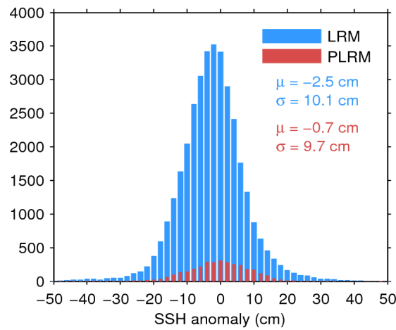
Figure 11. Histogram of science-valid SSH anomaly over oceans and lakes for LRM (blue) and PLRM (red) for 09/07/2017. The mean ( \mu ) and standard deviation ( \sigma ) are also shown. Note that values outside [-50\ 50] cm are excluded from the histogram for the sake of readability but not from the computation of \mu and \sigma .
