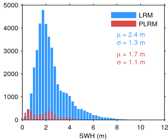
Figure 20. Histogram of science-valid SWH over oceans and lakes for LRM (blue) and PLRM (red) for 09/07/2017. The mean ( \mu ) and standard deviation ( \sigma ) are also shown. Note that values larger than 12 m are excluded from the histogram for the sake of readability but not from the computation of \mu and \sigma .
