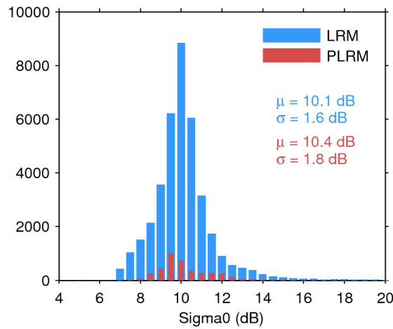
Figure 28. Histogram of science-valid sigma0 over oceans and lakes for LRM (blue) and PLRM (red) for 09/07/2017. The mean ( \mu ) and standard deviation ( \sigma ) are also shown. Note that values outside [4 20] dB are excluded from the histogram for the sake of readability but not from the computation of \mu and \sigma .
