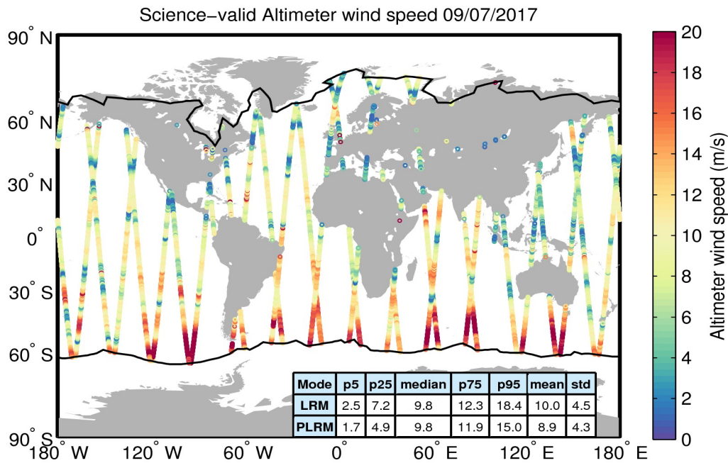
Figure 34. Geographical distribution of science-valid wind data over oceans and lakes for 09/07/2017. The statistical values shown in the table refer to the wind in m/s and are calculated separately for LRM and PLRM regions. The black lines mark the outer limit of the Arctic and Antarctic polar polygons. Gray circles denote records that have been rejected based on the editing criteria described in Table 5.
