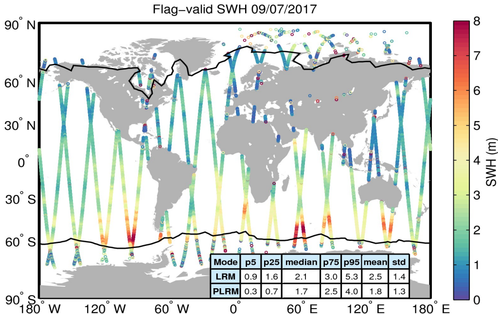
Figure 15. Geographical distribution of flag-valid SWH data over oceans and lakes for 09/07/2017. The statistical values shown in the table refer to the SWH in m and are calculated separately for LRM and PLRM regions. Measurements taken over polar polygons have been excluded from the computation of the statistical values. The black lines mark the outer limit of the Arctic and Antarctic polar polygons.
