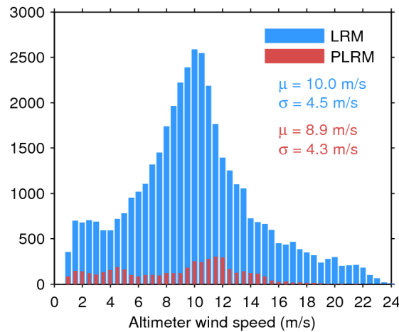
Figure 33. Histogram of flag-valid wind over oceans and lakes for LRM (blue) and PLRM (red) for 09/07/2017. The mean ( \mu ) and standard deviation ( \sigma ) are also shown. Note that values larger than 24 m/s are excluded from the histogram for the sake of readability but not from the computation of \mu and \sigma .
