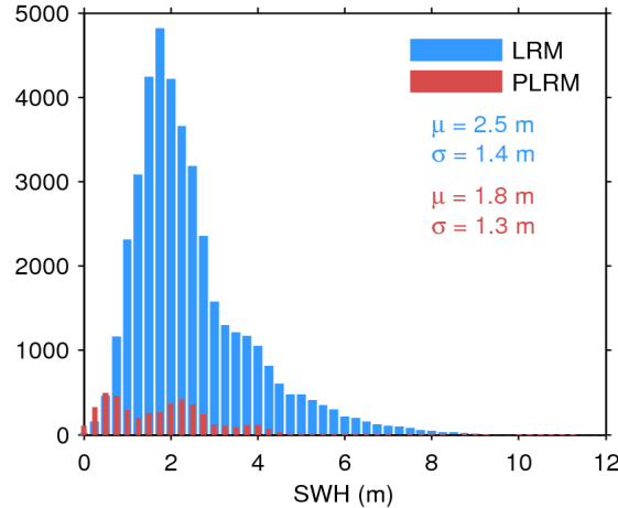
Figure 17. Histogram of flag-valid SWH over oceans and lakes for LRM (blue) and PLRM (red) for 09/07/2017. The mean ( \mu ) and standard deviation ( \sigma ) are also shown. Note that values larger than 12 m are excluded from the histogram for the sake of readability but not from the computation of \mu and \sigma .
