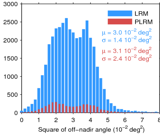
Figure 39. Histogram of flag-valid mispointing over oceans and lakes for LRM (blue) and PLRM (red) for 09/07/2017. Only positive values have been considered. The mean ( \mu ) and standard deviation ( \sigma ) are also shown. Note that values larger than 8 \cdot 10^{-2} \text{ deg}^2 are excluded from the histogram for the sake of readability but not from the computation of \mu and \sigma .
