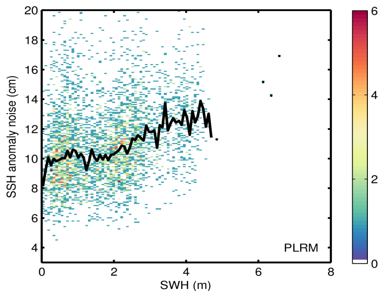
Figure 9. 2D histogram showing flag-valid SSH anomaly noise as a function of SWH for LRM (top) and PLRM (bottom) for 09/07/2017. The black line denotes the median SSH anomaly noise as a function of SWH.
