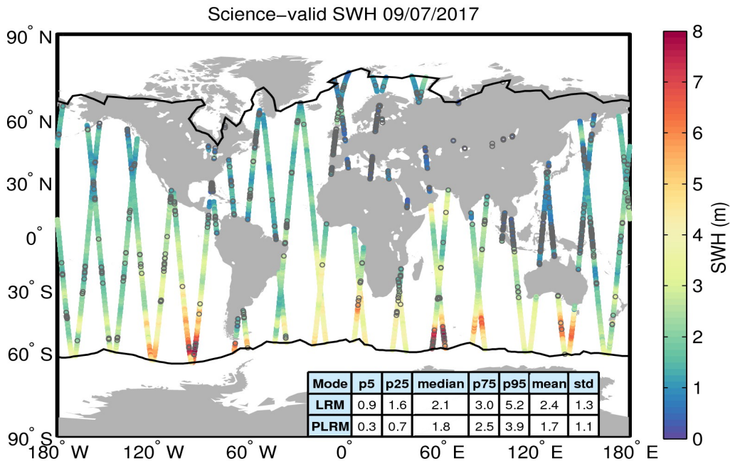
Figure 19. Geographical distribution of science-valid SWH data over oceans and lakes for 09/07/2017. The statistical values shown in the table refer to the SWH in m and are calculated separately for LRM and PLRM regions. The black lines mark the outer limit of the Arctic and Antarctic polar polygons. Gray circles denote records that have been rejected based on the editing criteria described in Table 3.
