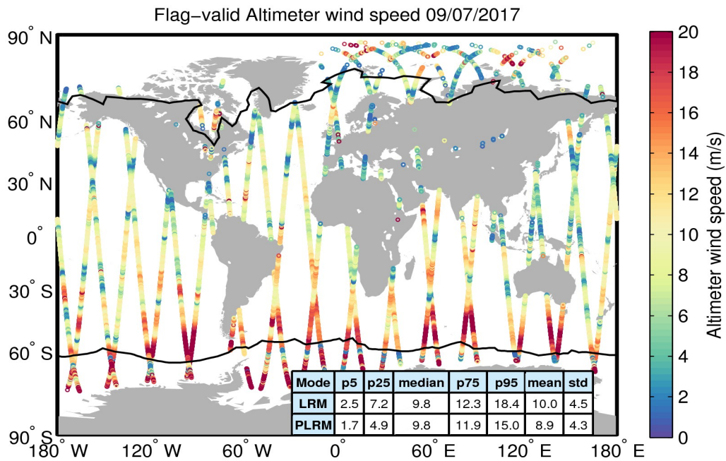
Figure 31. Geographical distribution of flag-valid wind data over oceans and lakes for 09/07/2017. The statistical values shown in the table refer to the wind in m/s and are calculated separately for LRM and PLRM regions. Measurements taken over polar polygons have been excluded from the computation of the statistical values. The black lines mark the outer limit of the Arctic and Antarctic polar polygons.
