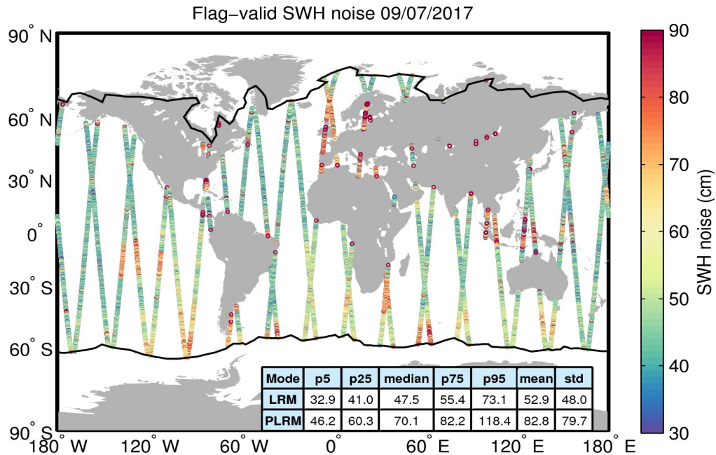
Figure 18. Geographical distribution of flag-valid 20-Hz SWH measurement noise over oceans and lakes for 09/07/2017. The statistical values shown in the table refer to the SWH noise and are calculated separately for LRM and PLRM regions. Measurements taken over polar polygons have been excluded from the computation of the statistical values. The black lines mark the outer limit of the Arctic and Antarctic polar polygons.
