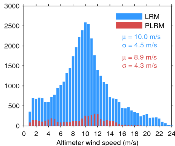
Figure 35. Histogram of science-valid wind over oceans and lakes for LRM (blue) and PLRM (red) for 09/07/2017. The mean ( \mu ) and standard deviation ( \sigma ) are also shown. Note that values larger than 24 m/s are excluded from the histogram for the sake of readability but not from the computation of \mu and \sigma .
