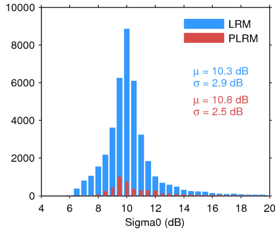
Figure 25. Histogram of flag-valid sigma0 over oceans and lakes for LRM (blue) and PLRM (red) for 09/07/2017. The mean ( \mu ) and standard deviation ( \sigma ) are also shown. Note that values outside [4 20] dB are excluded from the histogram for the sake of readability but not from the computation of \mu and \sigma .
