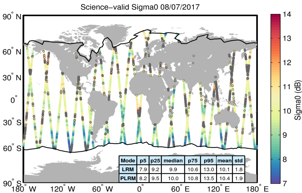
Figure 27. Geographical distribution of science-valid sigma0 data over oceans and lakes for 08/07/2017. The statistical values shown in the table refer to the sigma0 in dB and are calculated separately for LRM and PLRM regions. The black lines mark the outer limit of the Arctic and Antarctic polar polygons. Gray circles denote records that have been rejected based on the editing criteria described in Table 4.
