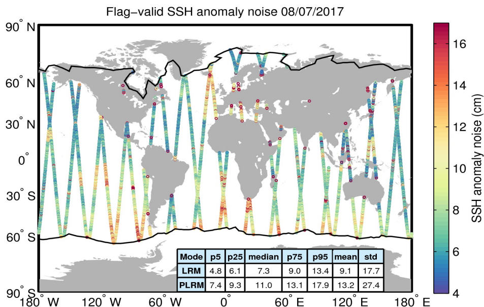
Figure 8. Geographical distribution of flag-valid 20-Hz SSH anomaly measurement noise over oceans and lakes for 08/07/2017. The statistical values shown in the table refer to the SSH anomaly noise and are calculated separately for LRM and PLRM regions. Measurements taken over polar polygons have been excluded from the computation of the statistical values. The black lines mark the outer limit of the Arctic and Antarctic polar polygons.
