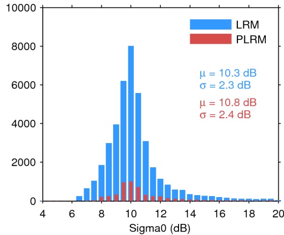
Figure 25. Histogram of flag-valid sigma0 over oceans and lakes for LRM (blue) and PLRM (red) for 08/07/2017. The mean ( \mu ) and standard deviation ( \sigma ) are also shown. Note that values outside [4 20] dB are excluded from the histogram for the sake of readability but not from the computation of \mu and \sigma .
