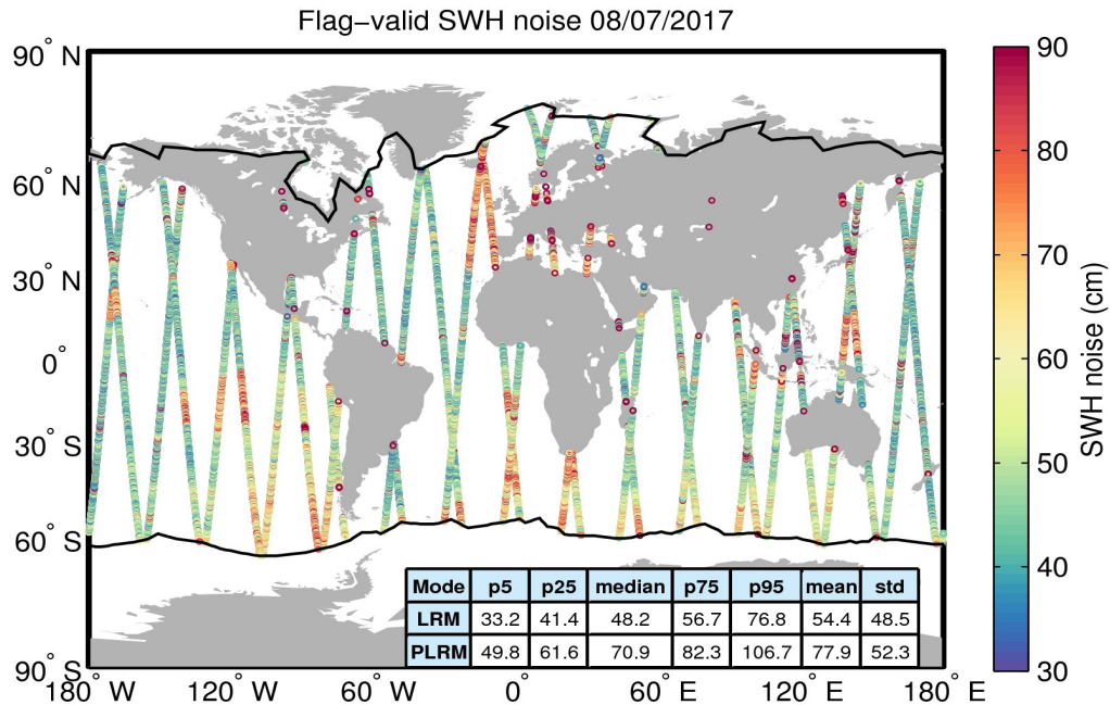
Figure 18. Geographical distribution of flag-valid 20-Hz SWH measurement noise over oceans and lakes for 08/07/2017. The statistical values shown in the table refer to the SWH noise and are calculated separately for LRM and PLRM regions. Measurements taken over polar polygons have been excluded from the computation of the statistical values. The black lines mark the outer limit of the Arctic and Antarctic polar polygons.
