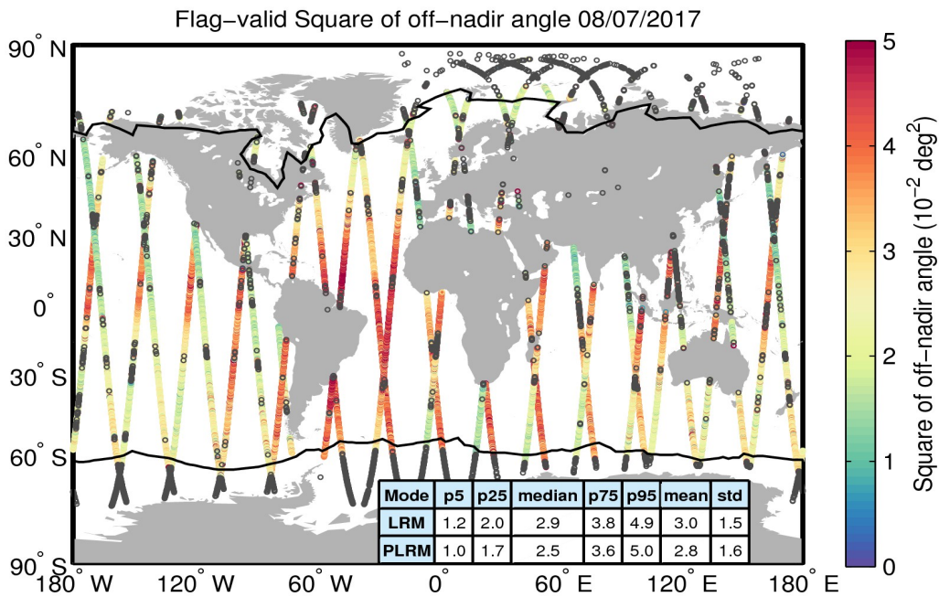
Figure 37. Geographical distribution of flag-valid mispointing data over oceans and lakes for 08/07/2017. The statistical values shown in the table refer to the mispointing in 10^{-2} deg 2 and are calculated separately for LRM and PLRM regions. Measurements taken over polar polygons have been excluded from the computation of the statistical values. The black lines mark the outer limit of the Arctic and Antarctic polar polygons. Gray circles denote negative values.
