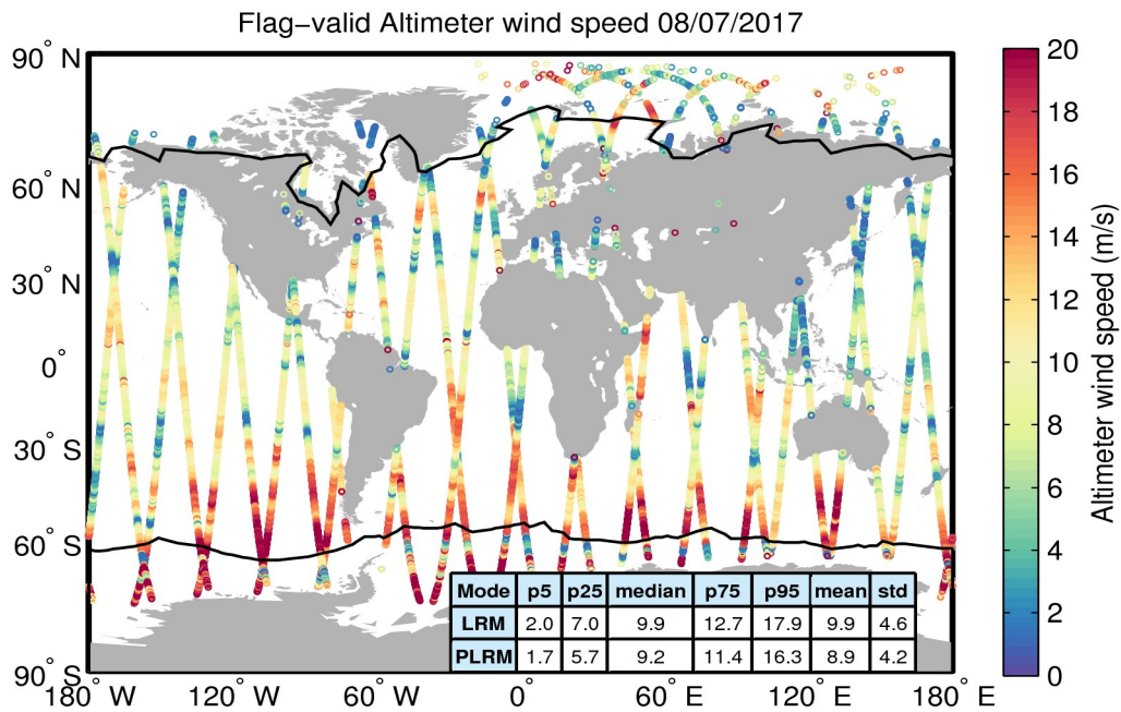
Figure 31. Geographical distribution of flag-valid wind data over oceans and lakes for 08/07/2017. The statistical values shown in the table refer to the wind in m/s and are calculated separately for LRM and PLRM regions. Measurements taken over polar polygons have been excluded from the computation of the statistical values. The black lines mark the outer limit of the Arctic and Antarctic polar polygons.
