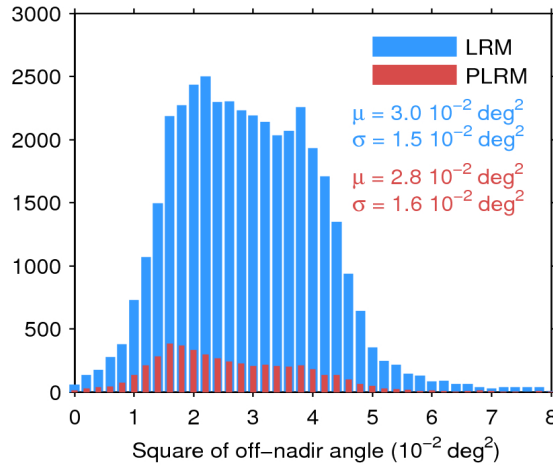
Figure 39. Histogram of flag-valid mispointing over oceans and lakes for LRM (blue) and PLRM (red) for 08/07/2017. Only positive values have been considered. The mean ( \mu ) and standard deviation ( \sigma ) are also shown. Note that values larger than 8 \cdot 10^{-2} \text{ deg}^2 are excluded from the histogram for the sake of readability but not from the computation of \mu and \sigma .
