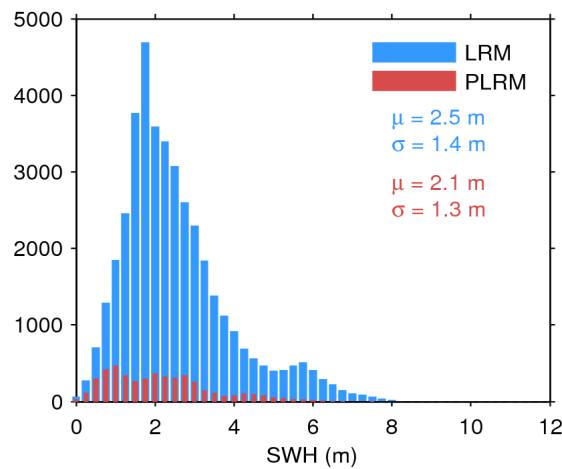
Figure 20. Histogram of science-valid SWH over oceans and lakes for LRM (blue) and PLRM (red) for 08/07/2017. The mean ( \mu ) and standard deviation ( \sigma ) are also shown. Note that values larger than 12 m are excluded from the histogram for the sake of readability but not from the computation of \mu and \sigma .
