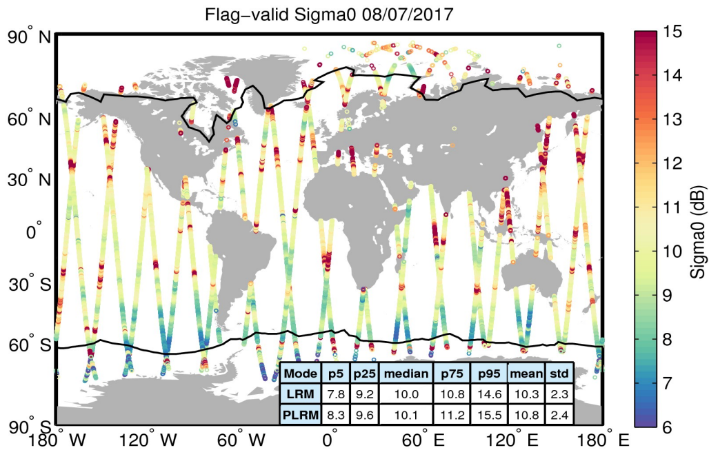
Figure 23. Geographical distribution of flag-valid sigma0 data over oceans and lakes for 08/07/2017. The statistical values shown in the table refer to the sigma0 in dB and are calculated separately for LRM and PLRM regions. Measurements taken over polar polygons have been excluded from the computation of the statistical values. The black lines mark the outer limit of the Arctic and Antarctic polar polygons.
