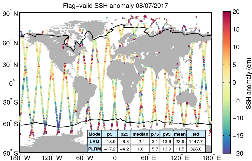
Figure 5. Geographical distribution of flag-valid 1-Hz SSH anomaly data over oceans and lakes for 08/07/2017. The statistical values shown in the table refer to the SSH anomaly in cm and are calculated separately for LRM and PLRM regions. Measurements taken over polar polygons have been excluded from the computation of the statistical values. The black lines mark the outer limit of the Arctic and Antarctic polar polygons.
