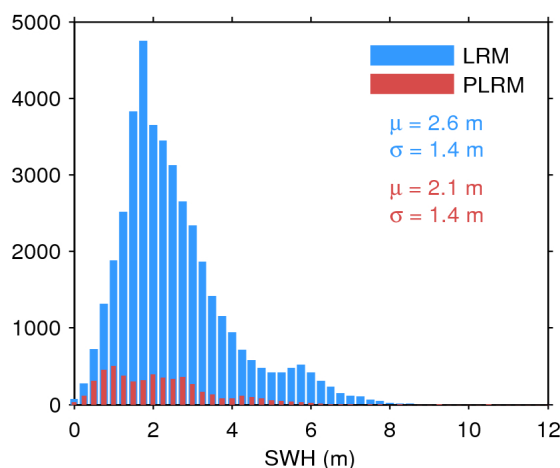
Figure 17. Histogram of flag-valid SWH over oceans and lakes for LRM (blue) and PLRM (red) for 08/07/2017. The mean ( \mu ) and standard deviation ( \sigma ) are also shown. Note that values larger than 12 m are excluded from the histogram for the sake of readability but not from the computation of \mu and \sigma .
