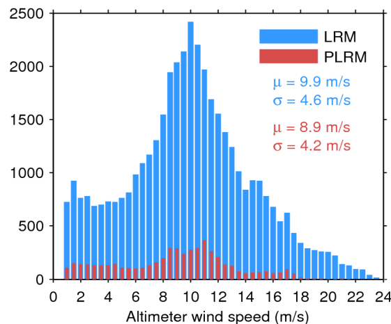
Figure 35. Histogram of science-valid wind over oceans and lakes for LRM (blue) and PLRM (red) for 08/07/2017. The mean ( \mu ) and standard deviation ( \sigma ) are also shown. Note that values larger than 24 m/s are excluded from the histogram for the sake of readability but not from the computation of \mu and \sigma .
