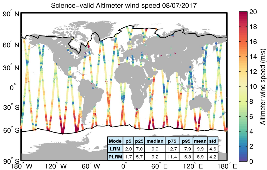
Figure 34. Geographical distribution of science-valid wind data over oceans and lakes for 08/07/2017. The statistical values shown in the table refer to the wind in m/s and are calculated separately for LRM and PLRM regions. The black lines mark the outer limit of the Arctic and Antarctic polar polygons. Gray circles denote records that have been rejected based on the editing criteria described in Table 5.
