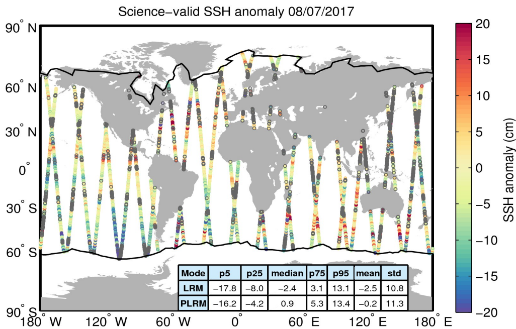
Figure 10. Geographical distribution of science-valid SSH anomaly data over oceans and lakes for 08/07/2017. The statistical values shown in the table refer to the SSH anomaly in cm and are calculated separately for LRM and PLRM regions. The black lines mark the outer limit of the Arctic and Antarctic polar polygons. Gray circles denote records that have been rejected based on the editing criteria described in Table 2.
