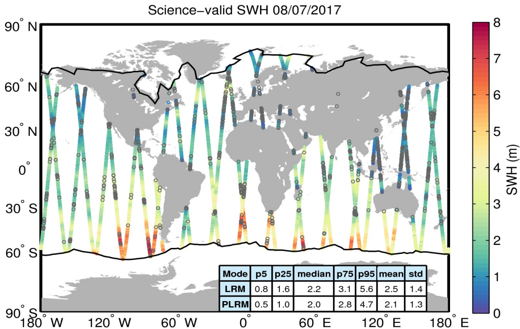
Figure 19. Geographical distribution of science-valid SWH data over oceans and lakes for 08/07/2017. The statistical values shown in the table refer to the SWH in m and are calculated separately for LRM and PLRM regions. The black lines mark the outer limit of the Arctic and Antarctic polar polygons. Gray circles denote records that have been rejected based on the editing criteria described in Table 3.
