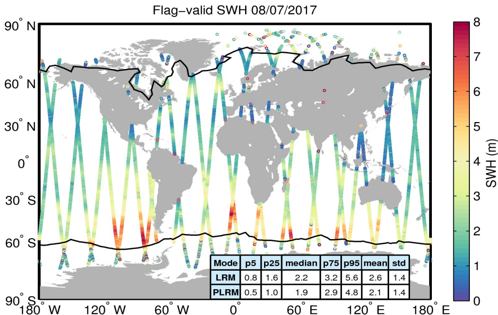
Figure 15. Geographical distribution of flag-valid SWH data over oceans and lakes for 08/07/2017. The statistical values shown in the table refer to the SWH in m and are calculated separately for LRM and PLRM regions. Measurements taken over polar polygons have been excluded from the computation of the statistical values. The black lines mark the outer limit of the Arctic and Antarctic polar polygons.
