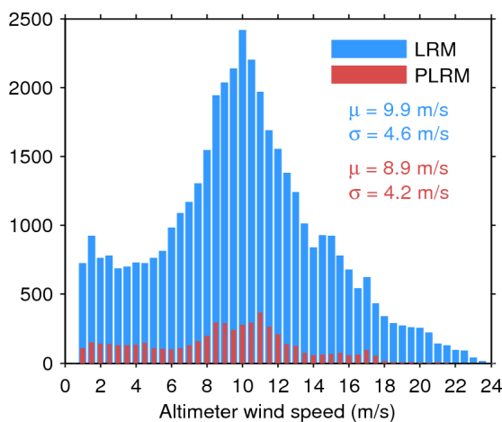
Figure 33. Histogram of flag-valid wind over oceans and lakes for LRM (blue) and PLRM (red) for 08/07/2017. The mean ( \mu ) and standard deviation ( \sigma ) are also shown. Note that values larger than 24 m/s are excluded from the histogram for the sake of readability but not from the computation of \mu and \sigma .
