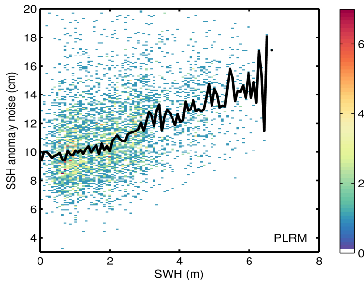
Figure 9. 2D histogram showing flag-valid SSH anomaly noise as a function of SWH for LRM (top) and PLRM (bottom) for 08/07/2017. The black line denotes the median SSH anomaly noise as a function of SWH.
