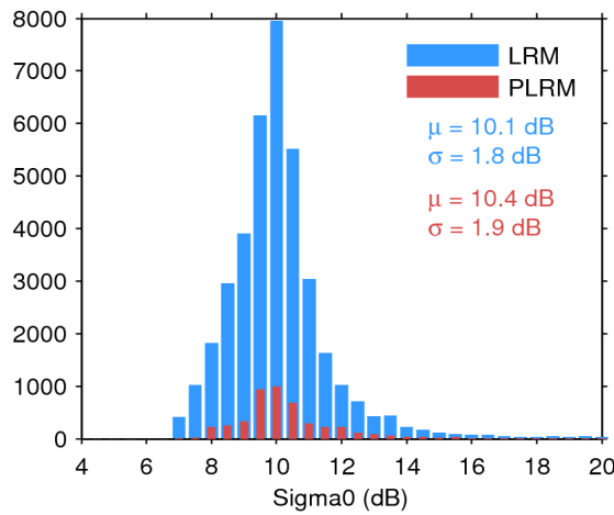
Figure 28. Histogram of science-valid sigma0 over oceans and lakes for LRM (blue) and PLRM (red) for 08/07/2017. The mean ( \mu ) and standard deviation ( \sigma ) are also shown. Note that values outside [4 20] dB are excluded from the histogram for the sake of readability but not from the computation of \mu and \sigma .
