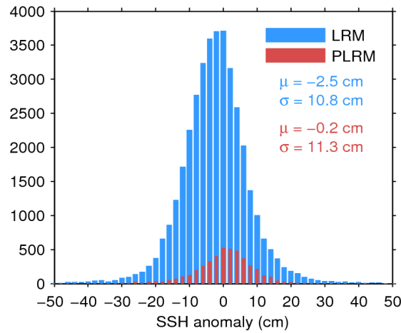
Figure 11. Histogram of science-valid SSH anomaly over oceans and lakes for LRM (blue) and PLRM (red) for 08/07/2017. The mean ( \mu ) and standard deviation ( \sigma ) are also shown. Note that values outside [-50\ 50] cm are excluded from the histogram for the sake of readability but not from the computation of \mu and \sigma .
