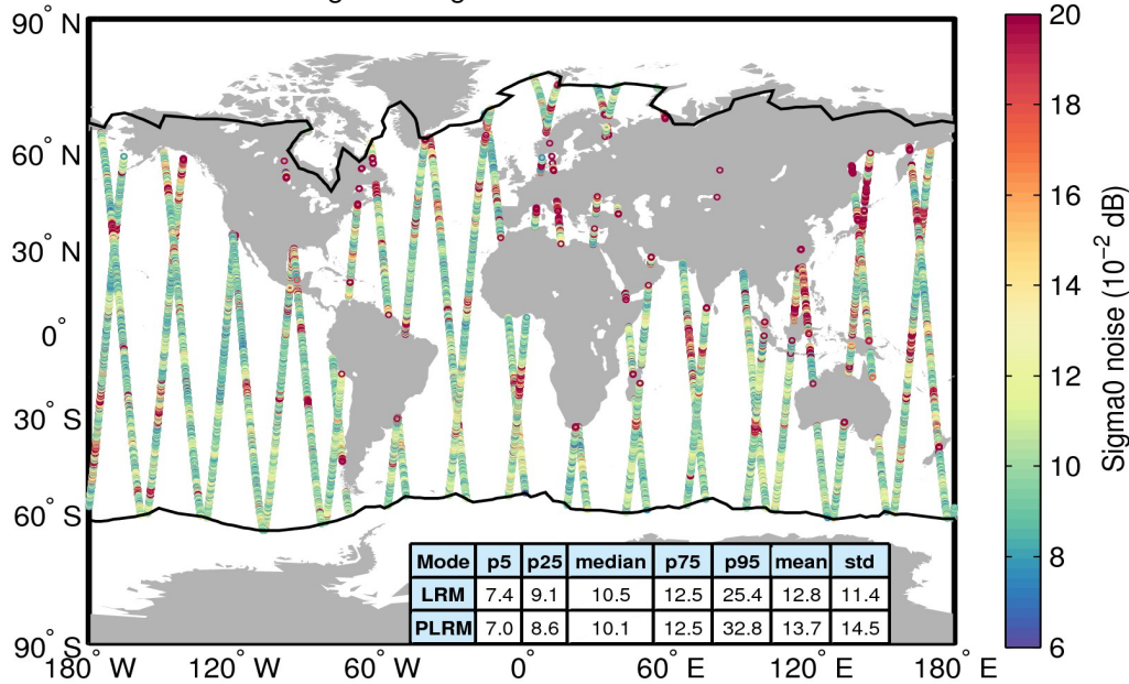
Flag-valid sigma0 noise 08/07/2017
