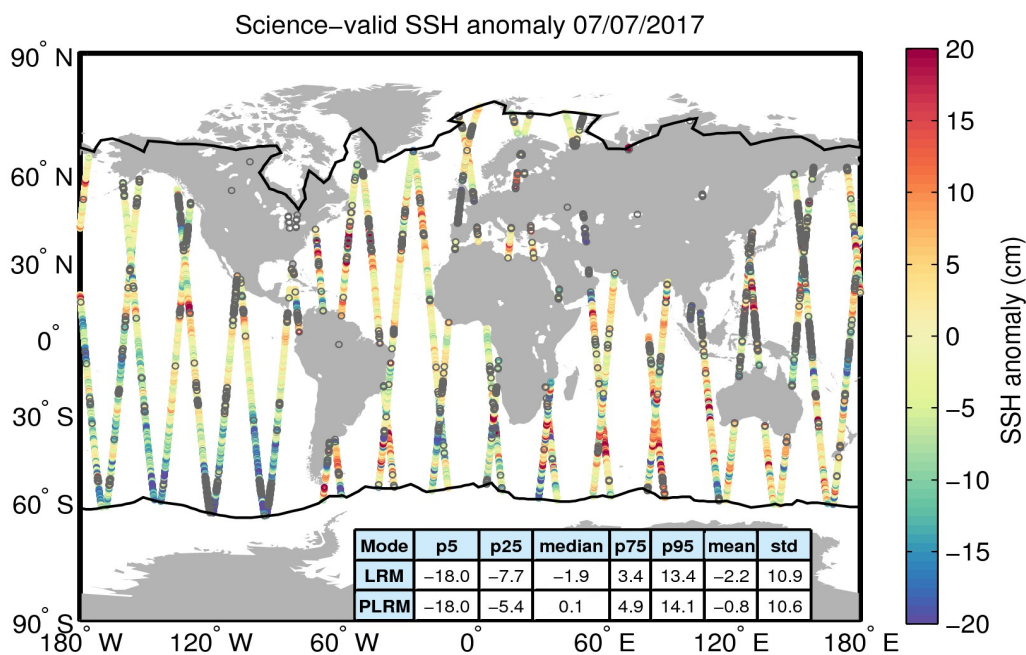
Figure 10. Geographical distribution of science-valid SSH anomaly data over oceans and lakes for 07/07/2017. The statistical values shown in the table refer to the SSH anomaly in cm and are calculated separately for LRM and PLRM regions. The black lines mark the outer limit of the Arctic and Antarctic polar polygons. Gray circles denote records that have been rejected based on the editing criteria described in Table 2.
