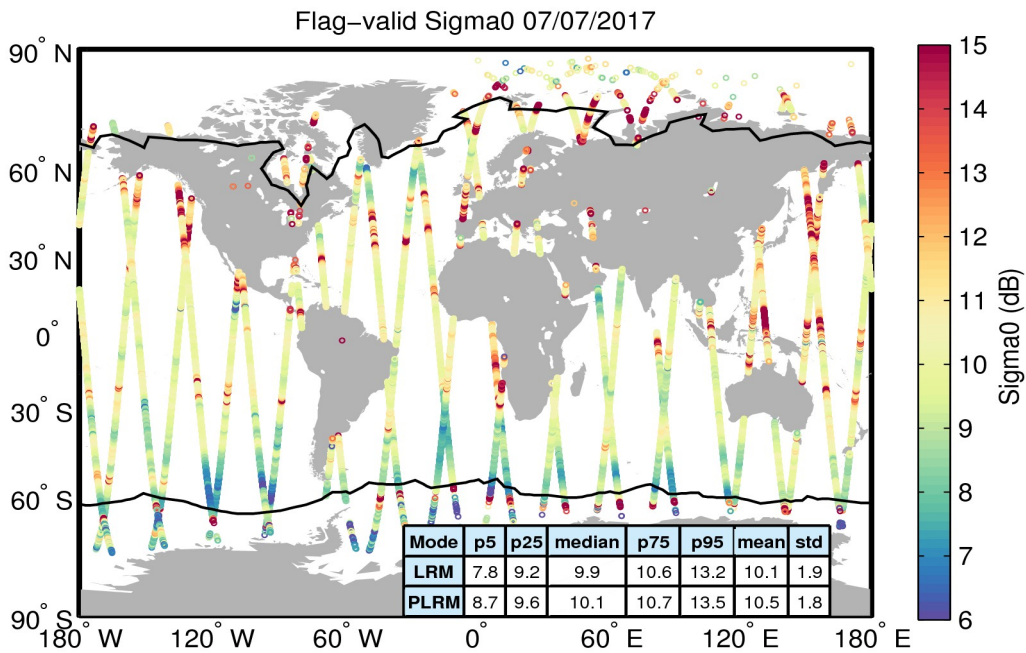
Figure 23. Geographical distribution of flag-valid sigma0 data over oceans and lakes for 07/07/2017. The statistical values shown in the table refer to the sigma0 in dB and are calculated separately for LRM and PLRM regions. Measurements taken over polar polygons have been excluded from the computation of the statistical values. The black lines mark the outer limit of the Arctic and Antarctic polar polygons.
