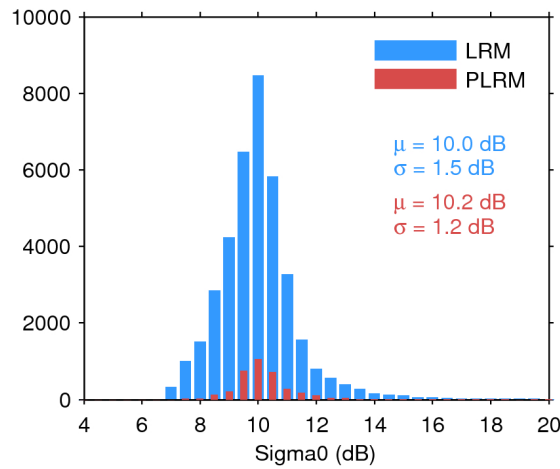
Figure 28. Histogram of science-valid sigma0 over oceans and lakes for LRM (blue) and PLRM (red) for 07/07/2017. The mean ( \mu ) and standard deviation ( \sigma ) are also shown. Note that values outside [4 20] dB are excluded from the histogram for the sake of readability but not from the computation of \mu and \sigma .
