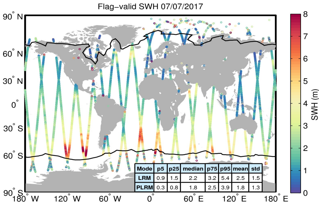
Figure 15. Geographical distribution of flag-valid SWH data over oceans and lakes for 07/07/2017. The statistical values shown in the table refer to the SWH in m and are calculated separately for LRM and PLRM regions. Measurements taken over polar polygons have been excluded from the computation of the statistical values. The black lines mark the outer limit of the Arctic and Antarctic polar polygons.
