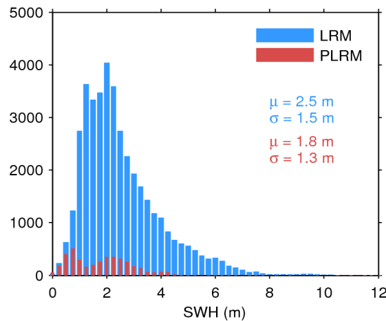
Figure 17. Histogram of flag-valid SWH over oceans and lakes for LRM (blue) and PLRM (red) for 07/07/2017. The mean ( \mu ) and standard deviation ( \sigma ) are also shown. Note that values larger than 12 m are excluded from the histogram for the sake of readability but not from the computation of \mu and \sigma .
