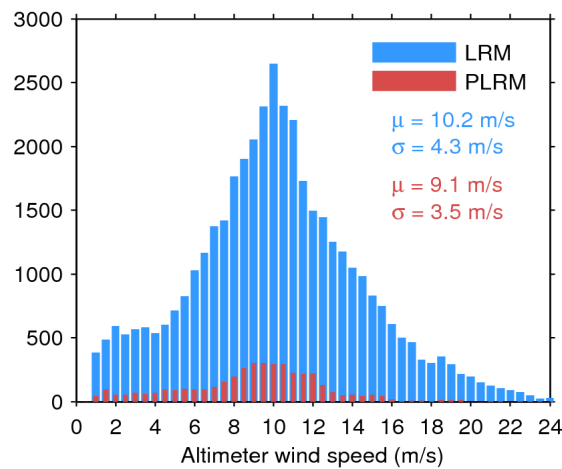
Figure 33. Histogram of flag-valid wind over oceans and lakes for LRM (blue) and PLRM (red) for 07/07/2017. The mean ( \mu ) and standard deviation ( \sigma ) are also shown. Note that values larger than 24 m/s are excluded from the histogram for the sake of readability but not from the computation of \mu and \sigma .
