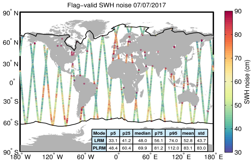
Figure 18. Geographical distribution of flag-valid 20-Hz SWH measurement noise over oceans and lakes for 07/07/2017. The statistical values shown in the table refer to the SWH noise and are calculated separately for LRM and PLRM regions. Measurements taken over polar polygons have been excluded from the computation of the statistical values. The black lines mark the outer limit of the Arctic and Antarctic polar polygons.
