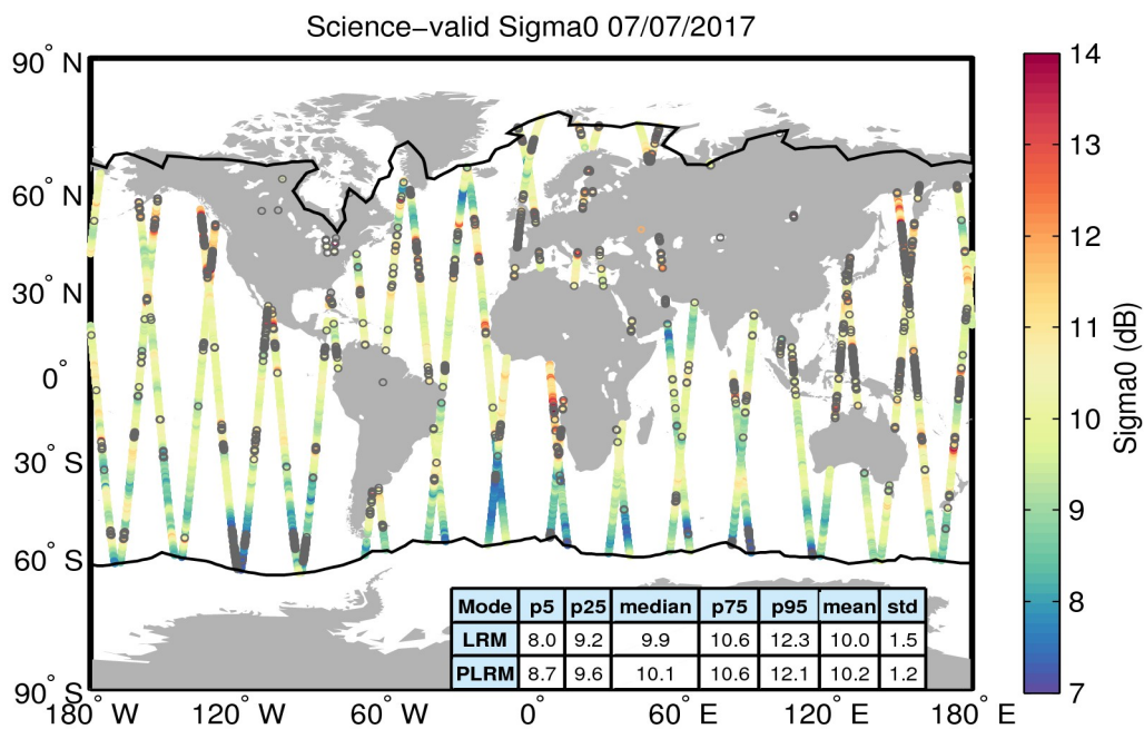
Figure 27. Geographical distribution of science-valid sigma0 data over oceans and lakes for 07/07/2017. The statistical values shown in the table refer to the sigma0 in dB and are calculated separately for LRM and PLRM regions. The black lines mark the outer limit of the Arctic and Antarctic polar polygons. Gray circles denote records that have been rejected based on the editing criteria described in Table 4.
