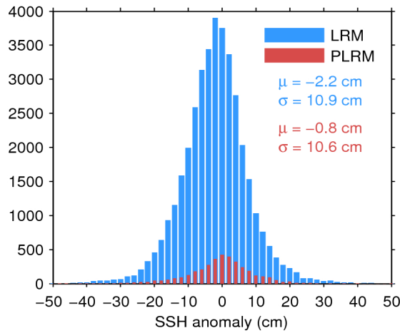
Figure 11. Histogram of science-valid SSH anomaly over oceans and lakes for LRM (blue) and PLRM (red) for 07/07/2017. The mean ( \mu ) and standard deviation ( \sigma ) are also shown. Note that values outside [-50\ 50] cm are excluded from the histogram for the sake of readability but not from the computation of \mu and \sigma .
