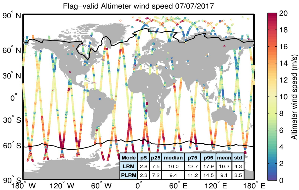
Figure 31. Geographical distribution of flag-valid wind data over oceans and lakes for 07/07/2017. The statistical values shown in the table refer to the wind in m/s and are calculated separately for LRM and PLRM regions. Measurements taken over polar polygons have been excluded from the computation of the statistical values. The black lines mark the outer limit of the Arctic and Antarctic polar polygons.
