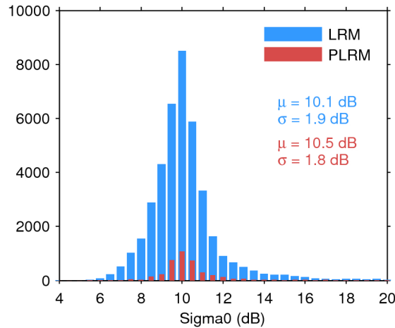
Figure 25. Histogram of flag-valid sigma0 over oceans and lakes for LRM (blue) and PLRM (red) for 07/07/2017. The mean ( \mu ) and standard deviation ( \sigma ) are also shown. Note that values outside [4 20] dB are excluded from the histogram for the sake of readability but not from the computation of \mu and \sigma .
