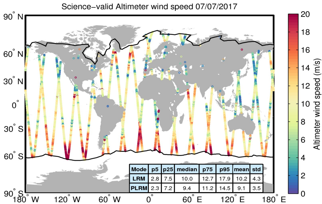
Figure 34. Geographical distribution of science-valid wind data over oceans and lakes for 07/07/2017. The statistical values shown in the table refer to the wind in m/s and are calculated separately for LRM and PLRM regions. The black lines mark the outer limit of the Arctic and Antarctic polar polygons. Gray circles denote records that have been rejected based on the editing criteria described in Table 5.
