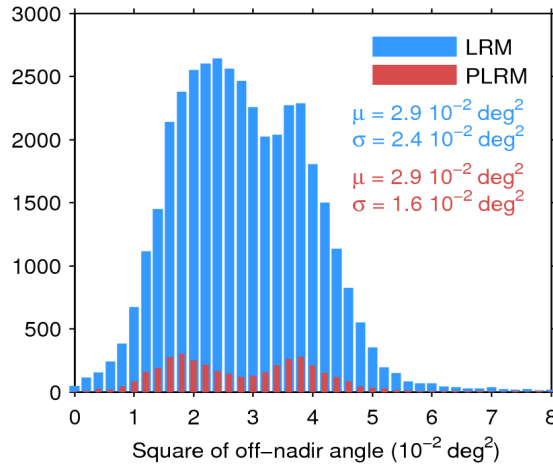
Figure 39. Histogram of flag-valid mispointing over oceans and lakes for LRM (blue) and PLRM (red) for 07/07/2017. Only positive values have been considered. The mean ( \mu ) and standard deviation ( \sigma ) are also shown. Note that values larger than 8 \cdot 10^{-2} \text{ deg}^2 are excluded from the histogram for the sake of readability but not from the computation of \mu and \sigma .
