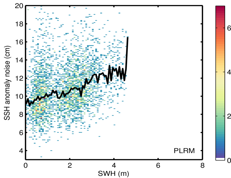
Figure 9. 2D histogram showing flag-valid SSH anomaly noise as a function of SWH for LRM (top) and PLRM (bottom) for 07/07/2017. The black line denotes the median SSH anomaly noise as a function of SWH.
