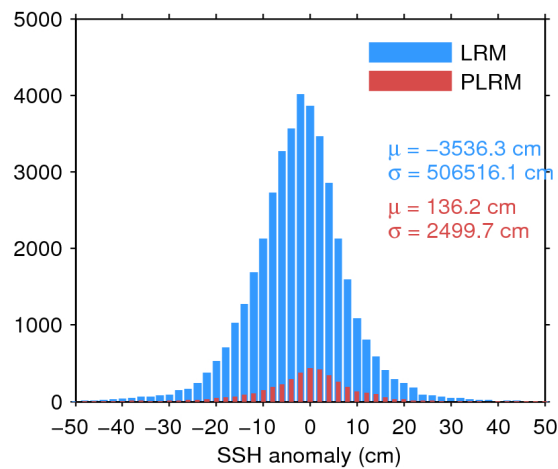
Figure 7. Histogram of flag-valid SSH anomaly over oceans and lakes for LRM (blue) and PLRM (red) for 07/07/2017. The mean ( \mu ) and standard deviation ( \sigma ) are also shown. Note that values outside [-50\ 50] cm are excluded from the histogram for the sake of readability but not from the computation of \mu and \sigma .
