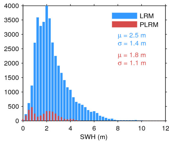
Figure 20. Histogram of science-valid SWH over oceans and lakes for LRM (blue) and PLRM (red) for 07/07/2017. The mean ( \mu ) and standard deviation ( \sigma ) are also shown. Note that values larger than 12 m are excluded from the histogram for the sake of readability but not from the computation of \mu and \sigma .
