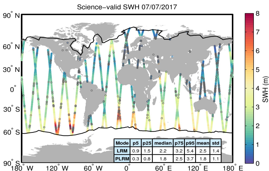
Figure 19. Geographical distribution of science-valid SWH data over oceans and lakes for 07/07/2017. The statistical values shown in the table refer to the SWH in m and are calculated separately for LRM and PLRM regions. The black lines mark the outer limit of the Arctic and Antarctic polar polygons. Gray circles denote records that have been rejected based on the editing criteria described in Table 3.
