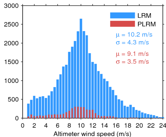
Figure 35. Histogram of science-valid wind over oceans and lakes for LRM (blue) and PLRM (red) for 07/07/2017. The mean ( \mu ) and standard deviation ( \sigma ) are also shown. Note that values larger than 24 m/s are excluded from the histogram for the sake of readability but not from the computation of \mu and \sigma .
