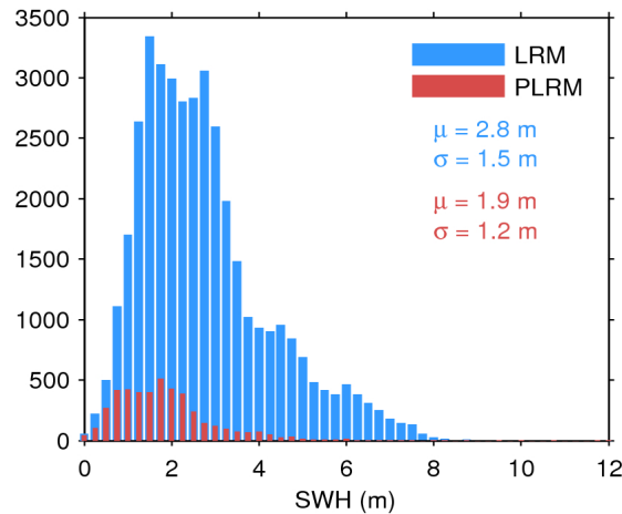
Figure 17. Histogram of flag-valid SWH over oceans and lakes for LRM (blue) and PLRM (red) for 06/07/2017. The mean ( \mu ) and standard deviation ( \sigma ) are also shown. Note that values larger than 12 m are excluded from the histogram for the sake of readability but not from the computation of \mu and \sigma .
