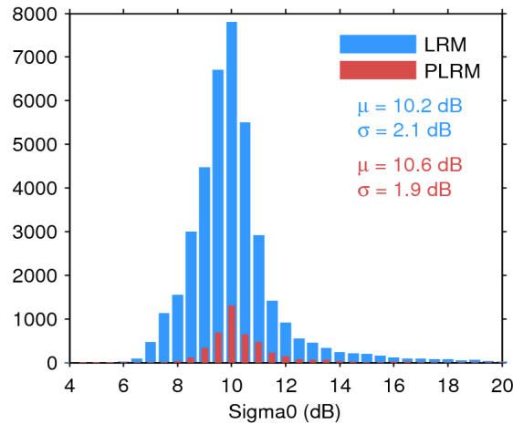
Figure 25. Histogram of flag-valid sigma0 over oceans and lakes for LRM (blue) and PLRM (red) for 06/07/2017. The mean ( \mu ) and standard deviation ( \sigma ) are also shown. Note that values outside [4 20] dB are excluded from the histogram for the sake of readability but not from the computation of \mu and \sigma .
