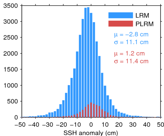
Figure 11. Histogram of science-valid SSH anomaly over oceans and lakes for LRM (blue) and PLRM (red) for 06/07/2017. The mean ( \mu ) and standard deviation ( \sigma ) are also shown. Note that values outside [-50 50] cm are excluded from the histogram for the sake of readability but not from the computation of \mu and \sigma .
