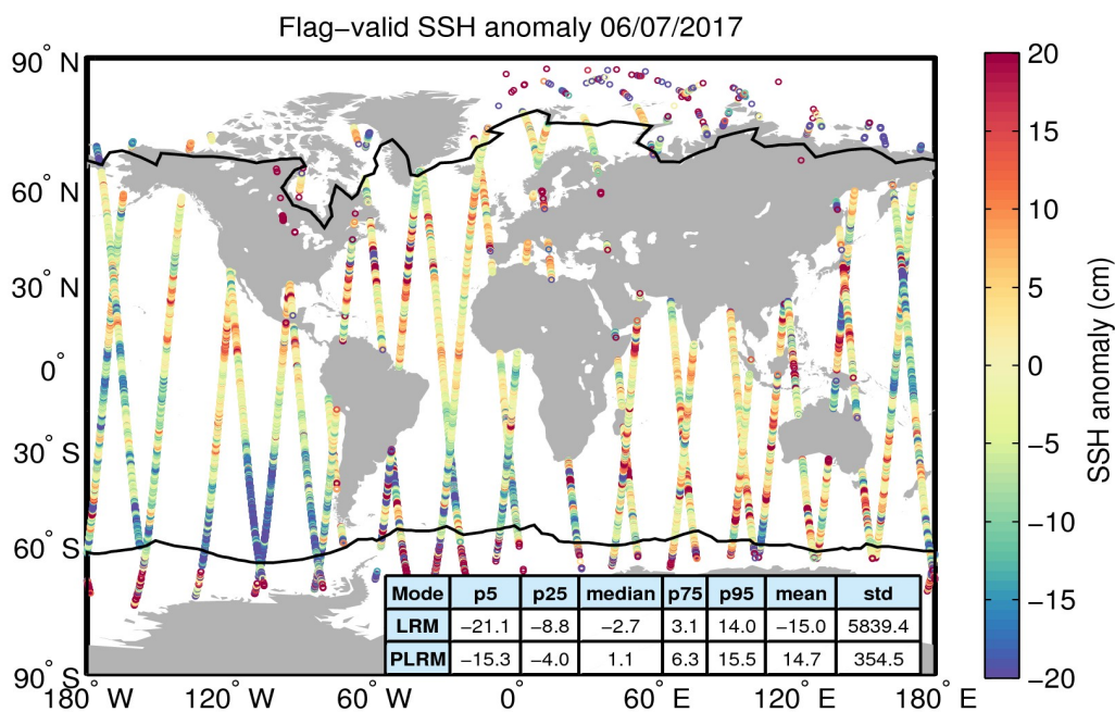
Figure 5. Geographical distribution of flag-valid 1-Hz SSH anomaly data over oceans and lakes for 06/07/2017. The statistical values shown in the table refer to the SSH anomaly in cm and are calculated separately for LRM and PLRM regions. Measurements taken over polar polygons have been excluded from the computation of the statistical values. The black lines mark the outer limit of the Arctic and Antarctic polar polygons.
