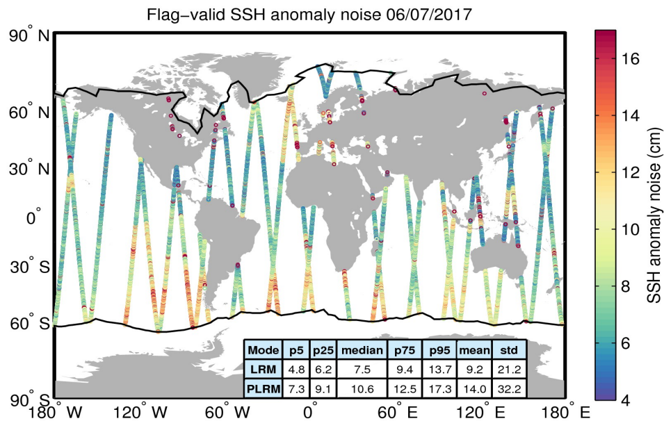
Figure 8. Geographical distribution of flag-valid 20-Hz SSH anomaly measurement noise over oceans and lakes for 06/07/2017. The statistical values shown in the table refer to the SSH anomaly noise and are calculated separately for LRM and PLRM regions. Measurements taken over polar polygons have been excluded from the computation of the statistical values. The black lines mark the outer limit of the Arctic and Antarctic polar polygons.
