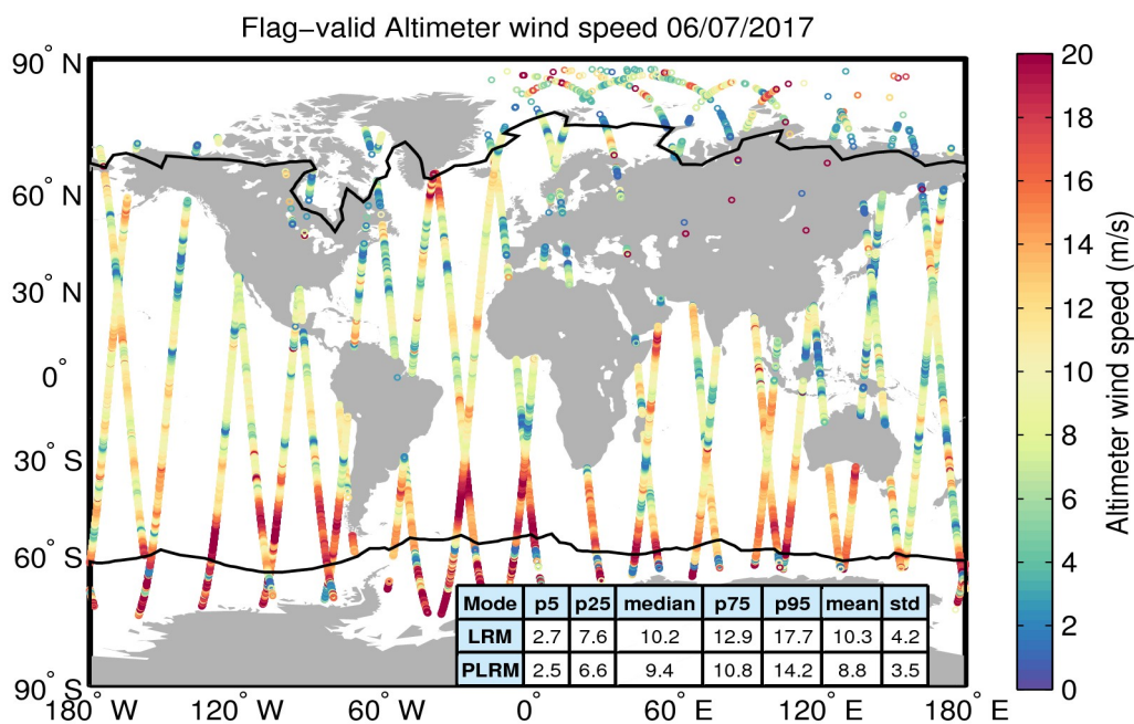
Figure 31. Geographical distribution of flag-valid wind data over oceans and lakes for 06/07/2017. The statistical values shown in the table refer to the wind in m/s and are calculated separately for LRM and PLRM regions. Measurements taken over polar polygons have been excluded from the computation of the statistical values. The black lines mark the outer limit of the Arctic and Antarctic polar polygons.
