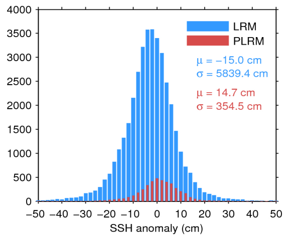
Figure 7. Histogram of flag-valid SSH anomaly over oceans and lakes for LRM (blue) and PLRM (red) for 06/07/2017. The mean ( \mu ) and standard deviation ( \sigma ) are also shown. Note that values outside [-50 \ 50] cm are excluded from the histogram for the sake of readability but not from the computation of \mu and \sigma .
