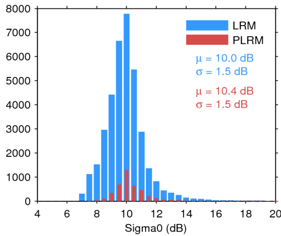
Figure 28. Histogram of science-valid sigma0 over oceans and lakes for LRM (blue) and PLRM (red) for 06/07/2017. The mean ( \mu ) and standard deviation ( \sigma ) are also shown. Note that values outside [4 20] dB are excluded from the histogram for the sake of readability but not from the computation of \mu and \sigma .
