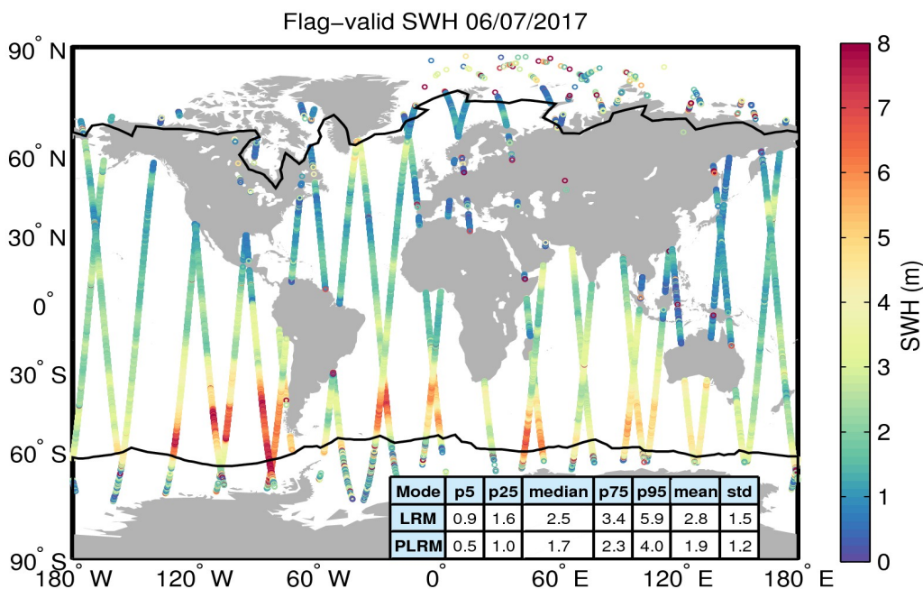
Figure 15. Geographical distribution of flag-valid SWH data over oceans and lakes for 06/07/2017. The statistical values shown in the table refer to the SWH in m and are calculated separately for LRM and PLRM regions. Measurements taken over polar polygons have been excluded from the computation of the statistical values. The black lines mark the outer limit of the Arctic and Antarctic polar polygons.
