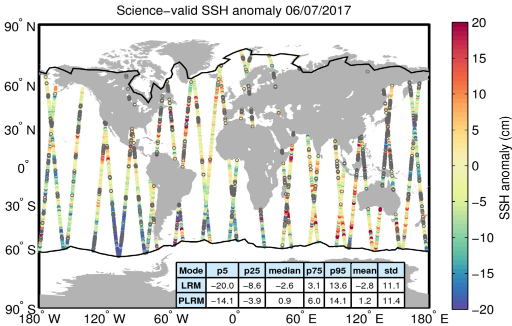
Figure 10. Geographical distribution of science-valid SSH anomaly data over oceans and lakes for 06/07/2017. The statistical values shown in the table refer to the SSH anomaly in cm and are calculated separately for LRM and PLRM regions. The black lines mark the outer limit of the Arctic and Antarctic polar polygons. Gray circles denote records that have been rejected based on the editing criteria described in Table 2.
