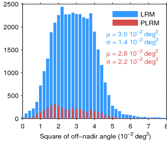
Figure 39. Histogram of flag-valid mispointing over oceans and lakes for LRM (blue) and PLRM (red) for 06/07/2017. Only positive values have been considered. The mean ( \mu ) and standard deviation ( \sigma ) are also shown. Note that values larger than 8 \cdot 10^{-2} \text{ deg}^2 are excluded from the histogram for the sake of readability but not from the computation of \mu and \sigma .
