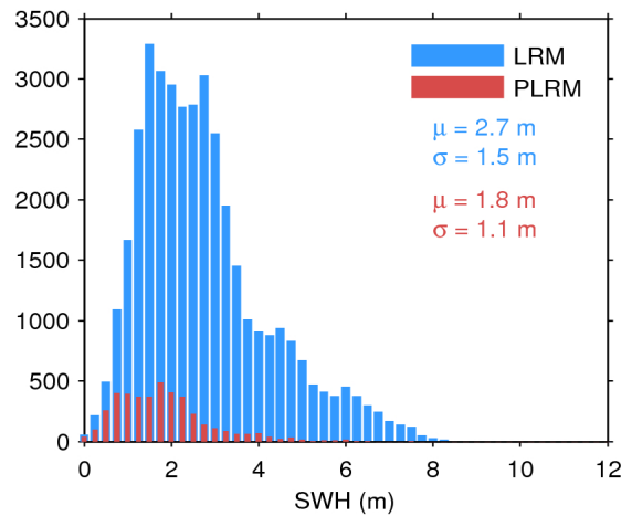
Figure 20. Histogram of science-valid SWH over oceans and lakes for LRM (blue) and PLRM (red) for 06/07/2017. The mean ( \mu ) and standard deviation ( \sigma ) are also shown. Note that values larger than 12 m are excluded from the histogram for the sake of readability but not from the computation of \mu and \sigma .
