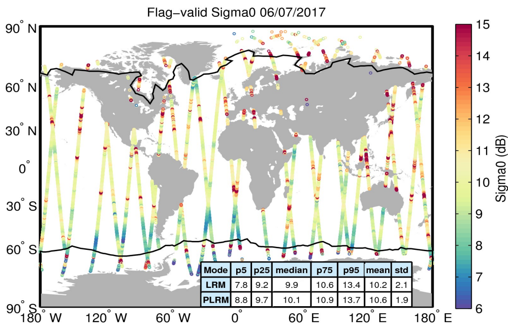
Figure 23. Geographical distribution of flag-valid sigma0 data over oceans and lakes for 06/07/2017. The statistical values shown in the table refer to the sigma0 in dB and are calculated separately for LRM and PLRM regions. Measurements taken over polar polygons have been excluded from the computation of the statistical values. The black lines mark the outer limit of the Arctic and Antarctic polar polygons.
