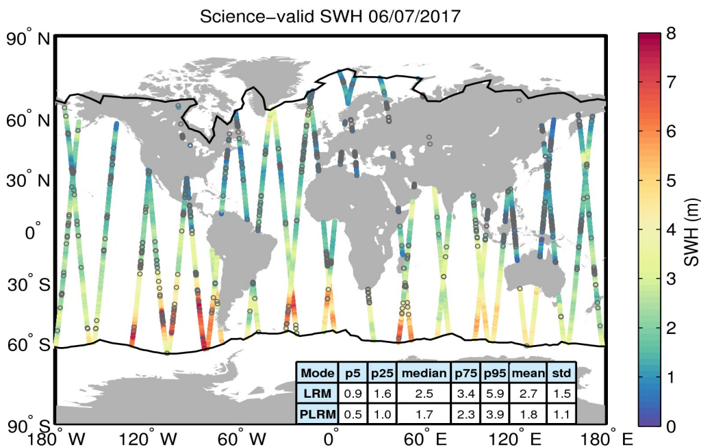
Figure 19. Geographical distribution of science-valid SWH data over oceans and lakes for 06/07/2017. The statistical values shown in the table refer to the SWH in m and are calculated separately for LRM and PLRM regions. The black lines mark the outer limit of the Arctic and Antarctic polar polygons. Gray circles denote records that have been rejected based on the editing criteria described in Table 3.
