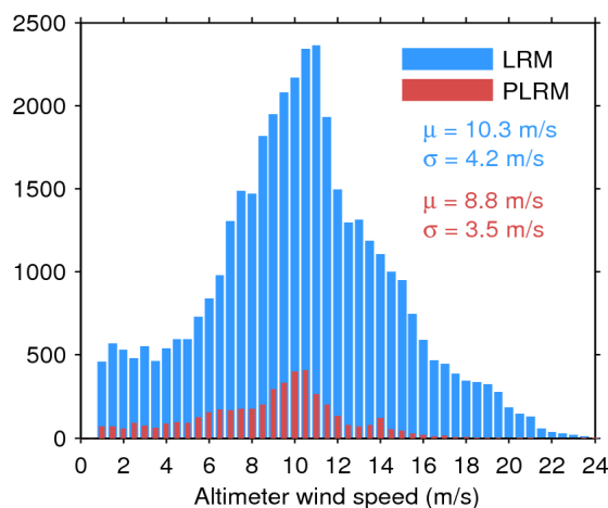
Figure 35. Histogram of science-valid wind over oceans and lakes for LRM (blue) and PLRM (red) for 06/07/2017. The mean ( \mu ) and standard deviation ( \sigma ) are also shown. Note that values larger than 24 m/s are excluded from the histogram for the sake of readability but not from the computation of \mu and \sigma .
