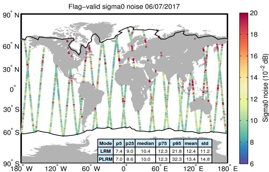
Figure 26. Geographical distribution of flag-valid 20-Hz sigma0 measurement noise over oceans and lakes for 06/07/2017. The statistical values shown in the table refer to the sigma0 noise and are calculated separately for LRM and PLRM regions. Measurements taken over polar polygons have been excluded from the computation of the statistical values. The black lines mark the outer limit of the Arctic and Antarctic polar polygons.
