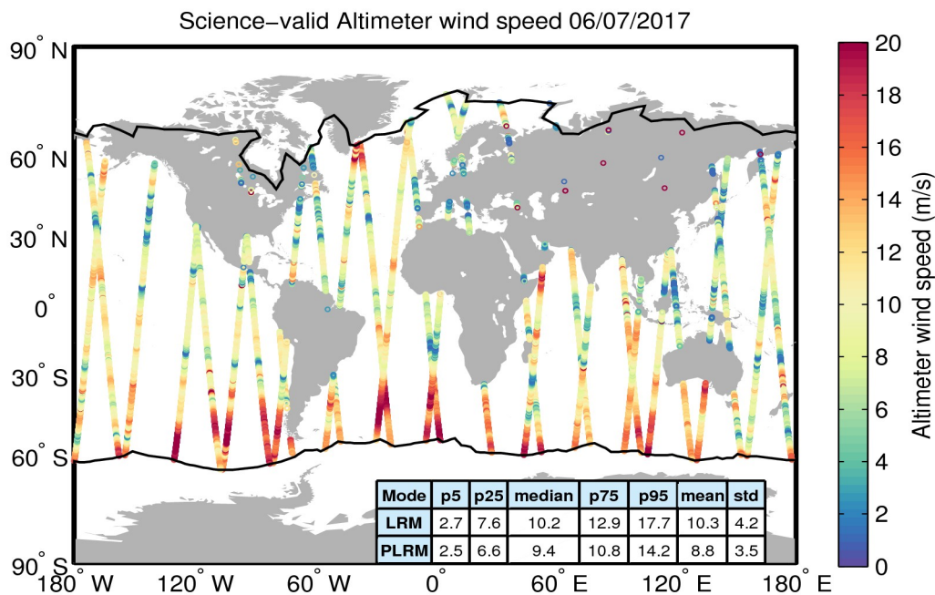
Figure 34. Geographical distribution of science-valid wind data over oceans and lakes for 06/07/2017. The statistical values shown in the table refer to the wind in m/s and are calculated separately for LRM and PLRM regions. The black lines mark the outer limit of the Arctic and Antarctic polar polygons. Gray circles denote records that have been rejected based on the editing criteria described in Table 5.
