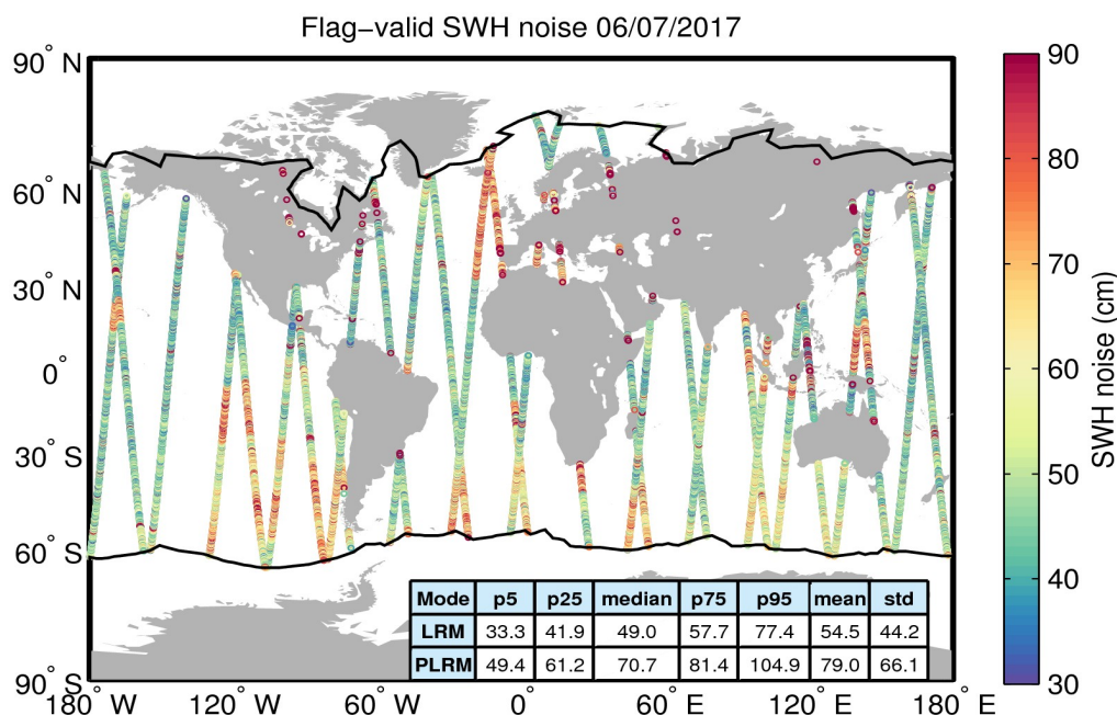
Figure 18. Geographical distribution of flag-valid 20-Hz SWH measurement noise over oceans and lakes for 06/07/2017. The statistical values shown in the table refer to the SWH noise and are calculated separately for LRM and PLRM regions. Measurements taken over polar polygons have been excluded from the computation of the statistical values. The black lines mark the outer limit of the Arctic and Antarctic polar polygons.
