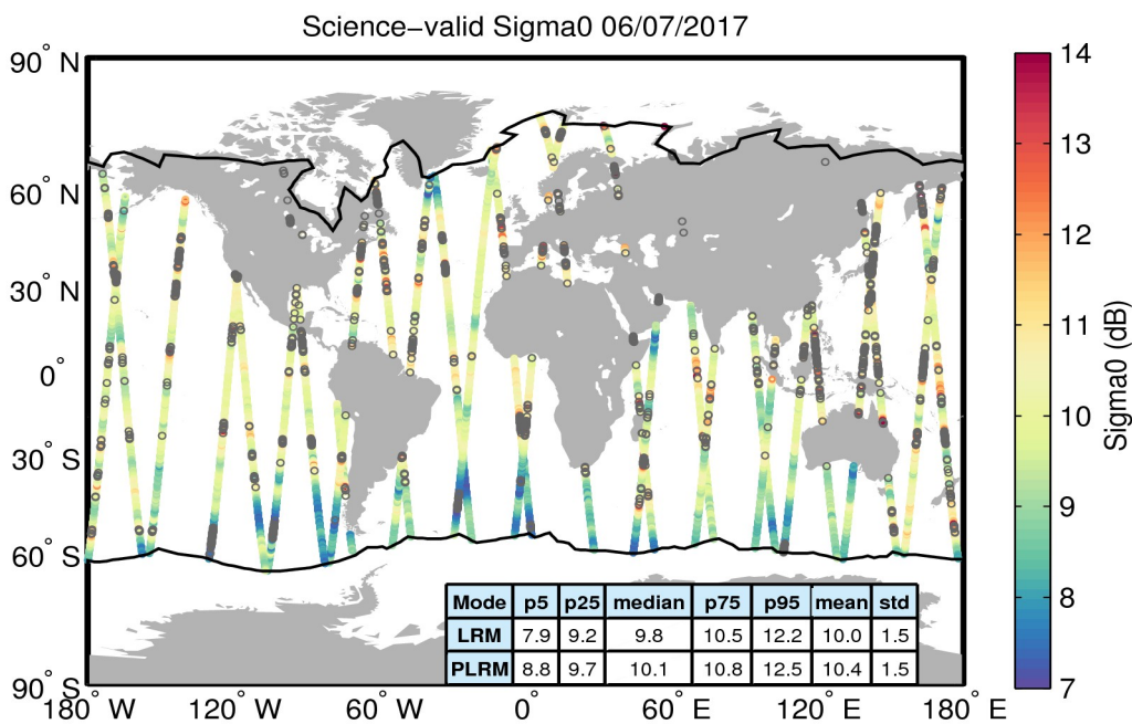
Figure 27. Geographical distribution of science-valid sigma0 data over oceans and lakes for 06/07/2017. The statistical values shown in the table refer to the sigma0 in dB and are calculated separately for LRM and PLRM regions. The black lines mark the outer limit of the Arctic and Antarctic polar polygons. Gray circles denote records that have been rejected based on the editing criteria described in Table 4.
