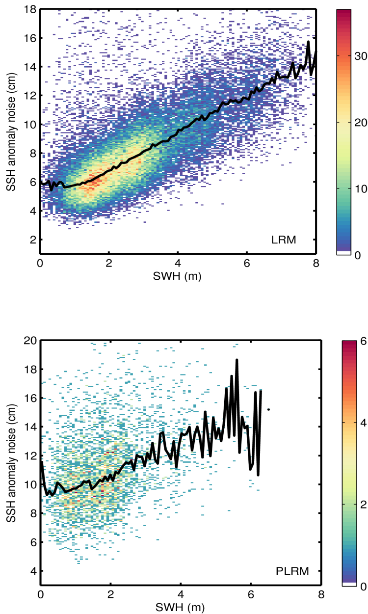
Figure 9. 2D histogram showing flag-valid SSH anomaly noise as a function of SWH for LRM (top) and PLRM (bottom) for 06/07/2017. The black line denotes the median SSH anomaly noise as a function of SWH.
