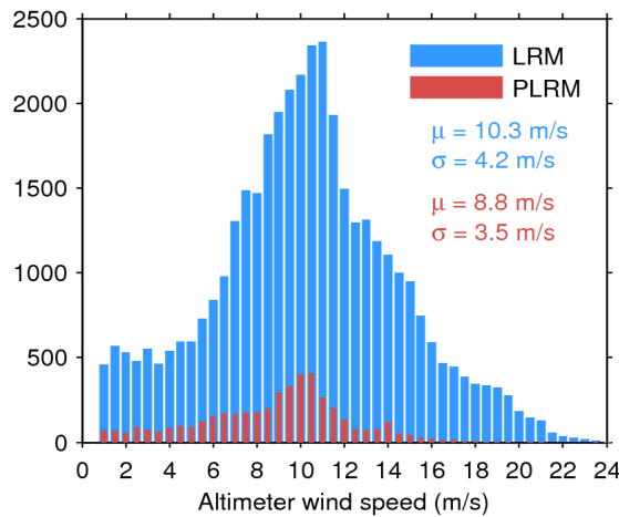
Figure 33. Histogram of flag-valid wind over oceans and lakes for LRM (blue) and PLRM (red) for 06/07/2017. The mean ( \mu ) and standard deviation ( \sigma ) are also shown. Note that values larger than 24 m/s are excluded from the histogram for the sake of readability but not from the computation of \mu and \sigma .
