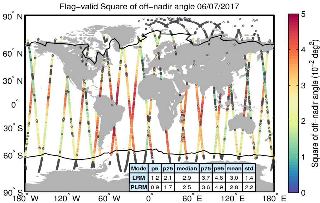
Figure 37. Geographical distribution of flag-valid mispointing data over oceans and lakes for 06/07/2017. The statistical values shown in the table refer to the mispointing in 10^{-2} deg 2 and are calculated separately for LRM and PLRM regions. Measurements taken over polar polygons have been excluded from the computation of the statistical values. The black lines mark the outer limit of the Arctic and Antarctic polar polygons. Gray circles denote negative values.
