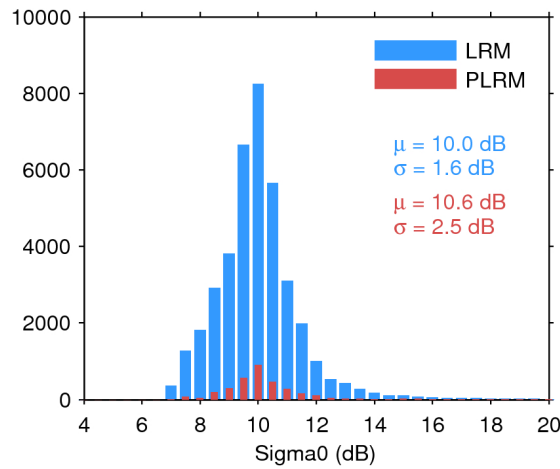
Figure 28. Histogram of science-valid sigma0 over oceans and lakes for LRM (blue) and PLRM (red) for 05/07/2017. The mean ( \mu ) and standard deviation ( \sigma ) are also shown. Note that values outside [4 20] dB are excluded from the histogram for the sake of readability but not from the computation of \mu and \sigma .
