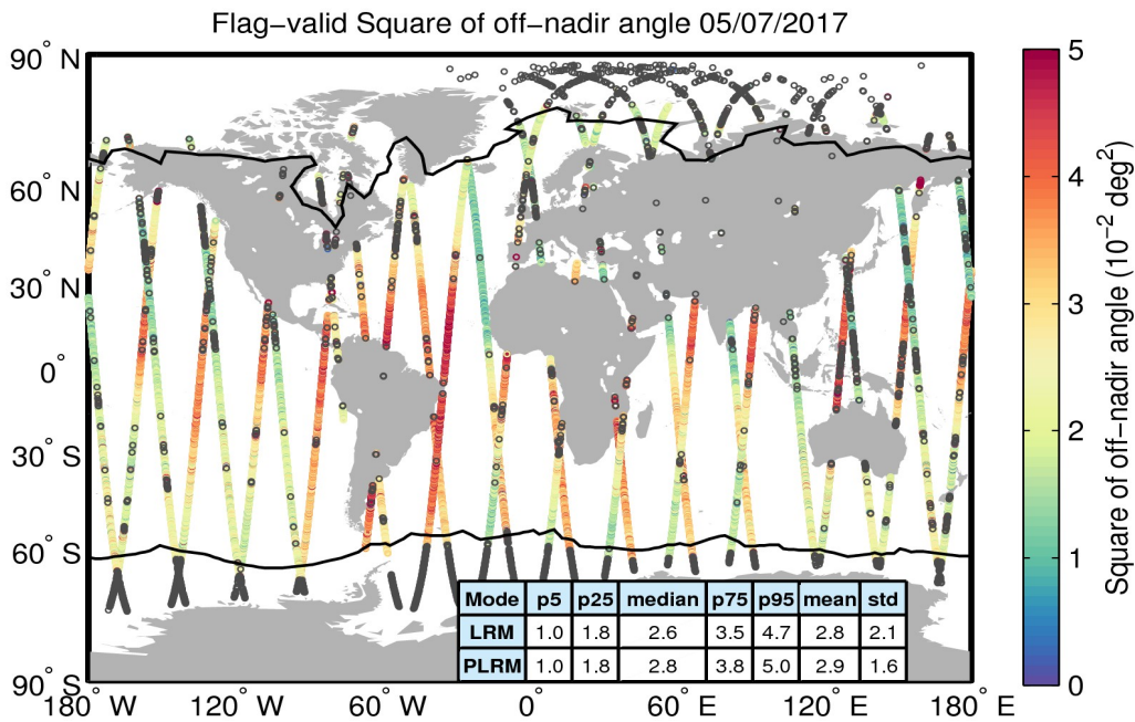
Figure 37. Geographical distribution of flag-valid mispointing data over oceans and lakes for 05/07/2017. The statistical values shown in the table refer to the mispointing in 10^{-2} \text{ deg}^2 and are calculated separately for LRM and PLRM regions. Measurements taken over polar polygons have been excluded from the computation of the statistical values. The black lines mark the outer limit of the Arctic and Antarctic polar polygons. Gray circles denote negative values.
