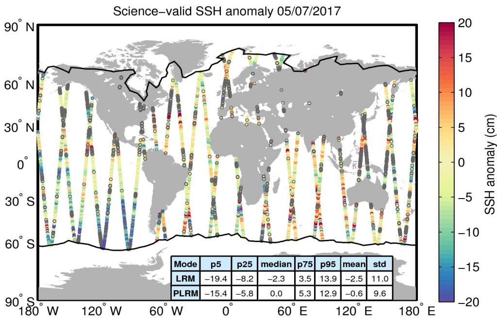
Figure 10. Geographical distribution of science-valid SSH anomaly data over oceans and lakes for 05/07/2017. The statistical values shown in the table refer to the SSH anomaly in cm and are calculated separately for LRM and PLRM regions. The black lines mark the outer limit of the Arctic and Antarctic polar polygons. Gray circles denote records that have been rejected based on the editing criteria described in Table 2.
