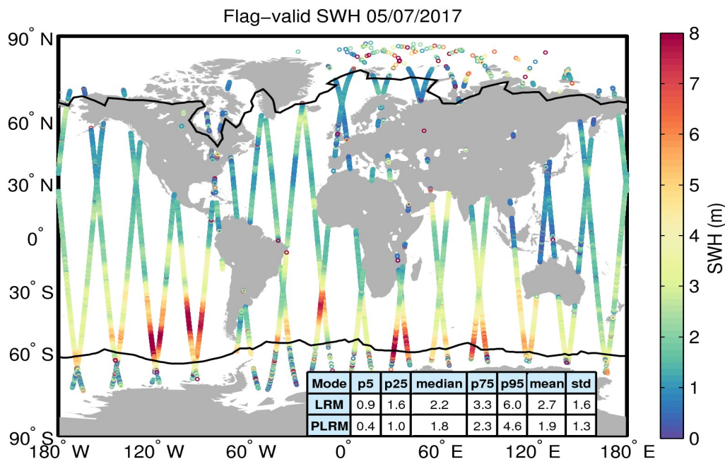
Figure 15. Geographical distribution of flag-valid SWH data over oceans and lakes for 05/07/2017. The statistical values shown in the table refer to the SWH in m and are calculated separately for LRM and PLRM regions. Measurements taken over polar polygons have been excluded from the computation of the statistical values. The black lines mark the outer limit of the Arctic and Antarctic polar polygons.
