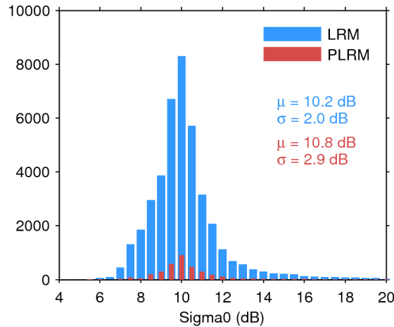
Figure 25. Histogram of flag-valid sigma0 over oceans and lakes for LRM (blue) and PLRM (red) for 05/07/2017. The mean ( \mu ) and standard deviation ( \sigma ) are also shown. Note that values outside [4 20] dB are excluded from the histogram for the sake of readability but not from the computation of \mu and \sigma .
