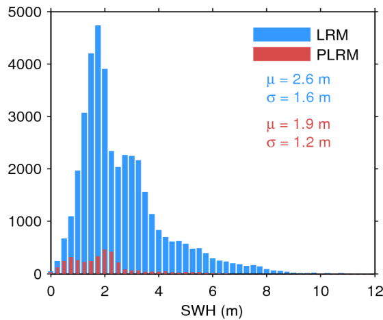
Figure 20. Histogram of science-valid SWH over oceans and lakes for LRM (blue) and PLRM (red) for 05/07/2017. The mean ( \mu ) and standard deviation ( \sigma ) are also shown. Note that values larger than 12 m are excluded from the histogram for the sake of readability but not from the computation of \mu and \sigma .
