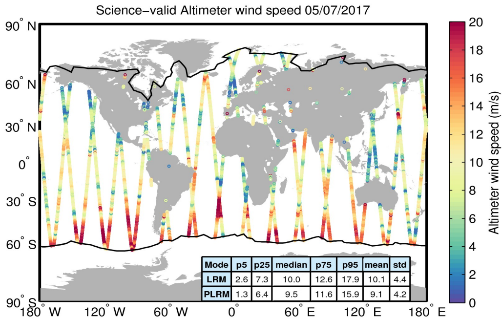
Figure 34. Geographical distribution of science-valid wind data over oceans and lakes for 05/07/2017. The statistical values shown in the table refer to the wind in m/s and are calculated separately for LRM and PLRM regions. The black lines mark the outer limit of the Arctic and Antarctic polar polygons. Gray circles denote records that have been rejected based on the editing criteria described in Table 5.
