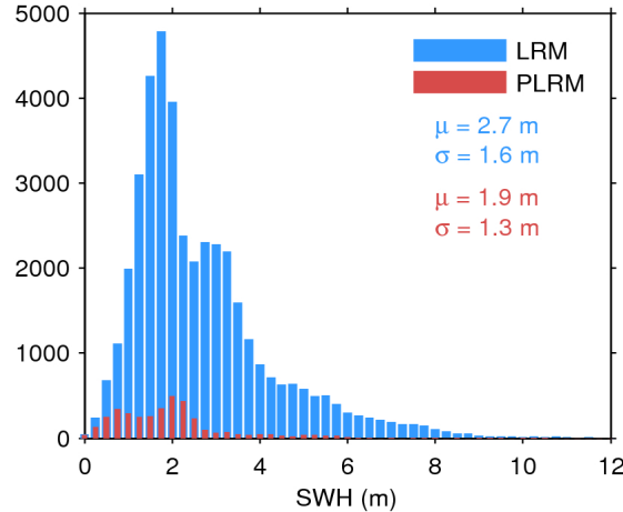
Figure 17. Histogram of flag-valid SWH over oceans and lakes for LRM (blue) and PLRM (red) for 05/07/2017. The mean ( \mu ) and standard deviation ( \sigma ) are also shown. Note that values larger than 12 m are excluded from the histogram for the sake of readability but not from the computation of \mu and \sigma .
