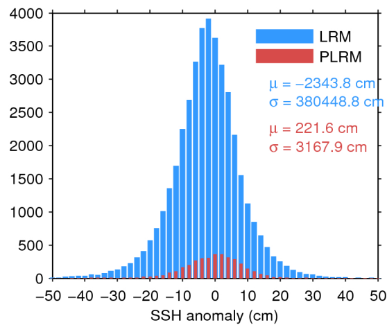
Figure 7. Histogram of flag-valid SSH anomaly over oceans and lakes for LRM (blue) and PLRM (red) for 05/07/2017. The mean ( \mu ) and standard deviation ( \sigma ) are also shown. Note that values outside [-50 \ 50] cm are excluded from the histogram for the sake of readability but not from the computation of \mu and \sigma .
