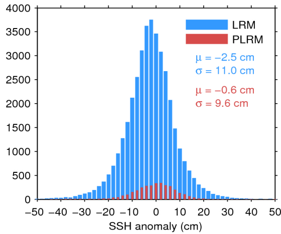
Figure 11. Histogram of science-valid SSH anomaly over oceans and lakes for LRM (blue) and PLRM (red) for 05/07/2017. The mean ( \mu ) and standard deviation ( \sigma ) are also shown. Note that values outside [-50 50] cm are excluded from the histogram for the sake of readability but not from the computation of \mu and \sigma .
