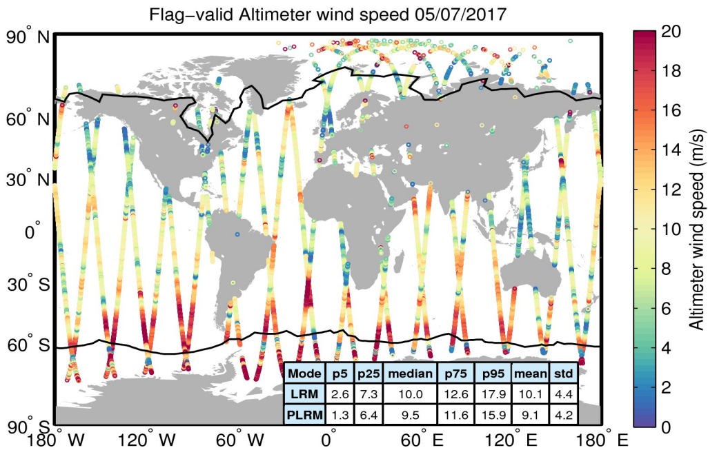
Figure 31. Geographical distribution of flag-valid wind data over oceans and lakes for 05/07/2017. The statistical values shown in the table refer to the wind in m/s and are calculated separately for LRM and PLRM regions. Measurements taken over polar polygons have been excluded from the computation of the statistical values. The black lines mark the outer limit of the Arctic and Antarctic polar polygons.
