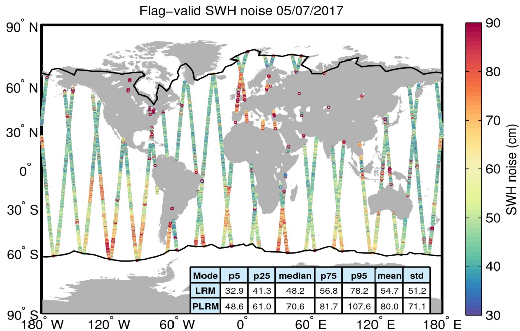
Figure 18. Geographical distribution of flag-valid 20-Hz SWH measurement noise over oceans and lakes for 05/07/2017. The statistical values shown in the table refer to the SWH noise and are calculated separately for LRM and PLRM regions. Measurements taken over polar polygons have been excluded from the computation of the statistical values. The black lines mark the outer limit of the Arctic and Antarctic polar polygons.
