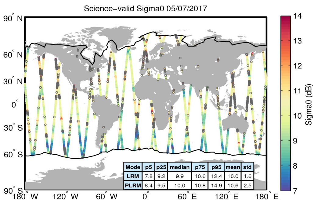
Figure 27. Geographical distribution of science-valid sigma0 data over oceans and lakes for 05/07/2017. The statistical values shown in the table refer to the sigma0 in dB and are calculated separately for LRM and PLRM regions. The black lines mark the outer limit of the Arctic and Antarctic polar polygons. Gray circles denote records that have been rejected based on the editing criteria described in Table 4.
