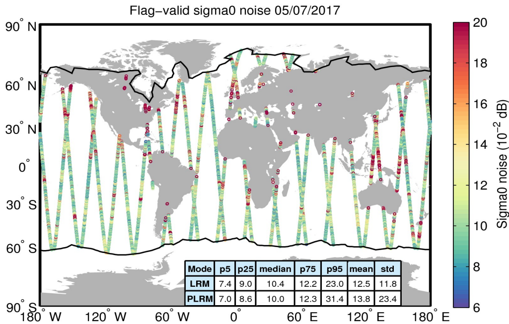
Figure 26. Geographical distribution of flag-valid 20-Hz sigma0 measurement noise over oceans and lakes for 05/07/2017. The statistical values shown in the table refer to the sigma0 noise and are calculated separately for LRM and PLRM regions. Measurements taken over polar polygons have been excluded from the computation of the statistical values. The black lines mark the outer limit of the Arctic and Antarctic polar polygons.
