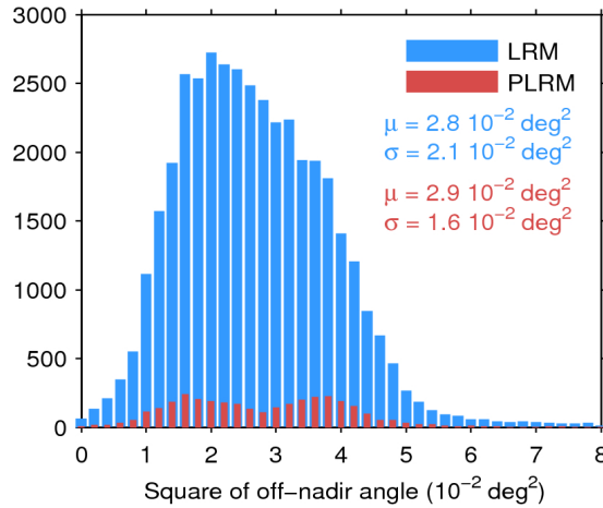
Figure 39. Histogram of flag-valid mispointing over oceans and lakes for LRM (blue) and PLRM (red) for 05/07/2017. Only positive values have been considered. The mean ( \mu ) and standard deviation ( \sigma ) are also shown. Note that values larger than 8 \cdot 10^{-2} \text{ deg}^2 are excluded from the histogram for the sake of readability but not from the computation of \mu and \sigma .
