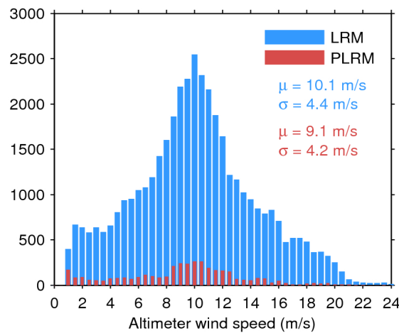
Figure 33. Histogram of flag-valid wind over oceans and lakes for LRM (blue) and PLRM (red) for 05/07/2017. The mean ( \mu ) and standard deviation ( \sigma ) are also shown. Note that values larger than 24 m/s are excluded from the histogram for the sake of readability but not from the computation of \mu and \sigma .
