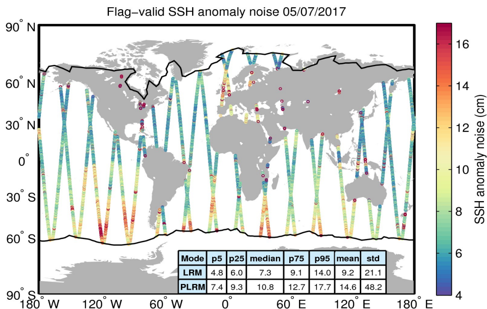
Figure 8. Geographical distribution of flag-valid 20-Hz SSH anomaly measurement noise over oceans and lakes for 05/07/2017. The statistical values shown in the table refer to the SSH anomaly noise and are calculated separately for LRM and PLRM regions. Measurements taken over polar polygons have been excluded from the computation of the statistical values. The black lines mark the outer limit of the Arctic and Antarctic polar polygons.
