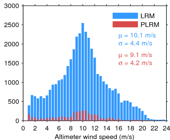
Figure 35. Histogram of science-valid wind over oceans and lakes for LRM (blue) and PLRM (red) for 05/07/2017. The mean ( \mu ) and standard deviation ( \sigma ) are also shown. Note that values larger than 24 m/s are excluded from the histogram for the sake of readability but not from the computation of \mu and \sigma .
