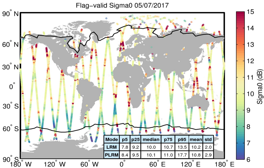
Figure 23. Geographical distribution of flag-valid sigma0 data over oceans and lakes for 05/07/2017. The statistical values shown in the table refer to the sigma0 in dB and are calculated separately for LRM and PLRM regions. Measurements taken over polar polygons have been excluded from the computation of the statistical values. The black lines mark the outer limit of the Arctic and Antarctic polar polygons.
