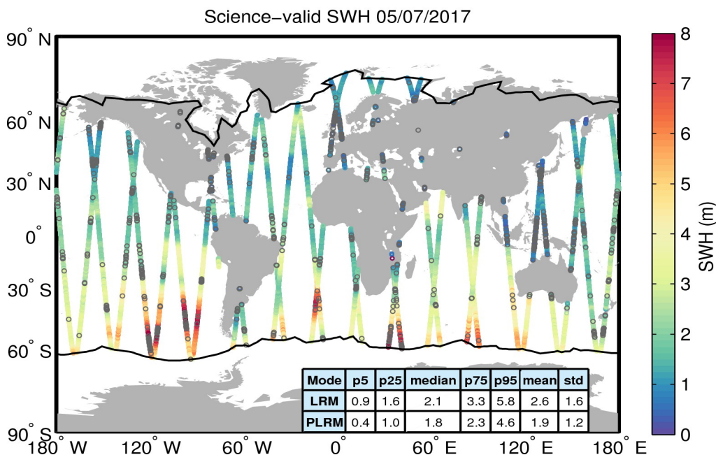
Figure 19. Geographical distribution of science-valid SWH data over oceans and lakes for 05/07/2017. The statistical values shown in the table refer to the SWH in m and are calculated separately for LRM and PLRM regions. The black lines mark the outer limit of the Arctic and Antarctic polar polygons. Gray circles denote records that have been rejected based on the editing criteria described in Table 3.
