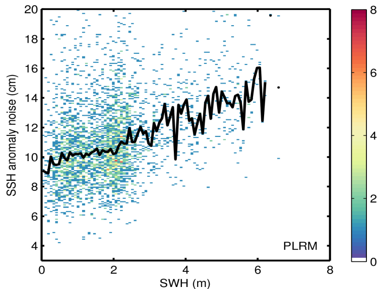
Figure 9. 2D histogram showing flag-valid SSH anomaly noise as a function of SWH for LRM (top) and PLRM (bottom) for 05/07/2017. The black line denotes the median SSH anomaly noise as a function of SWH.
