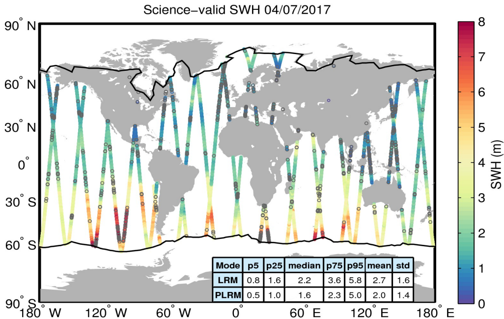
Figure 19. Geographical distribution of science-valid SWH data over oceans and lakes for 04/07/2017. The statistical values shown in the table refer to the SWH in m and are calculated separately for LRM and PLRM regions. The black lines mark the outer limit of the Arctic and Antarctic polar polygons. Gray circles denote records that have been rejected based on the editing criteria described in Table 3.
