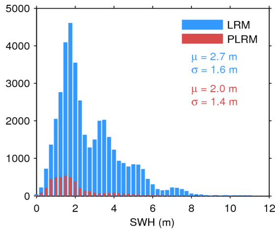
Figure 20. Histogram of science-valid SWH over oceans and lakes for LRM (blue) and PLRM (red) for 04/07/2017. The mean ( \mu ) and standard deviation ( \sigma ) are also shown. Note that values larger than 12 m are excluded from the histogram for the sake of readability but not from the computation of \mu and \sigma .
