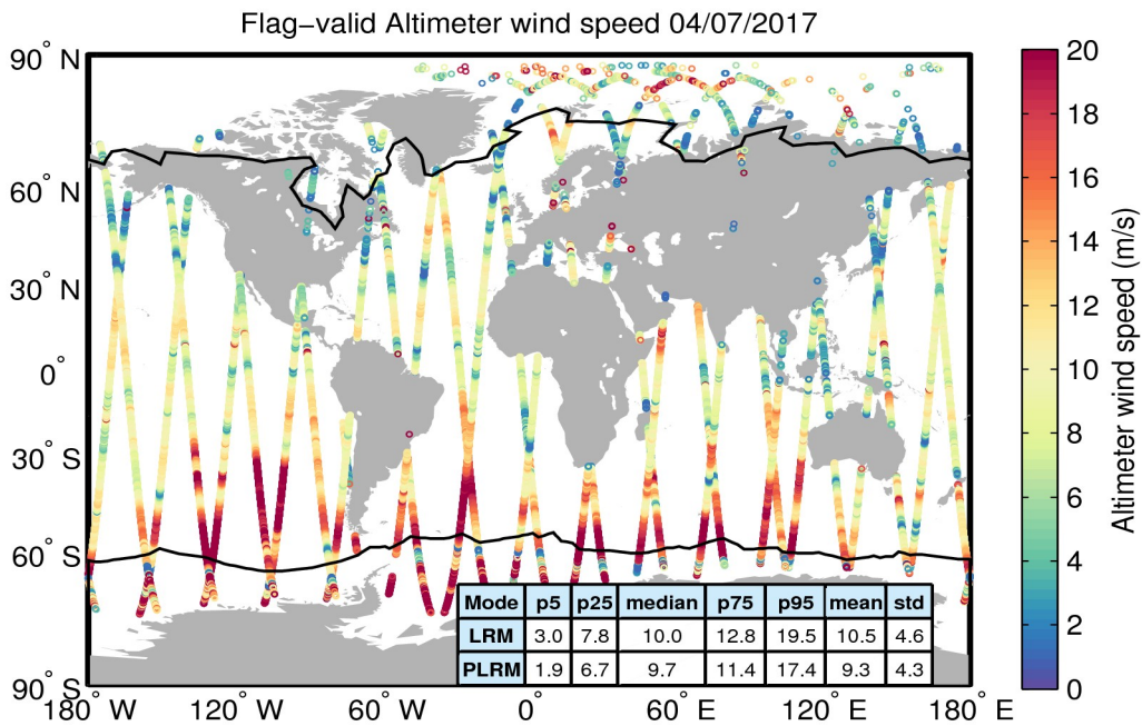
Figure 31. Geographical distribution of flag-valid wind data over oceans and lakes for 04/07/2017. The statistical values shown in the table refer to the wind in m/s and are calculated separately for LRM and PLRM regions. Measurements taken over polar polygons have been excluded from the computation of the statistical values. The black lines mark the outer limit of the Arctic and Antarctic polar polygons.
