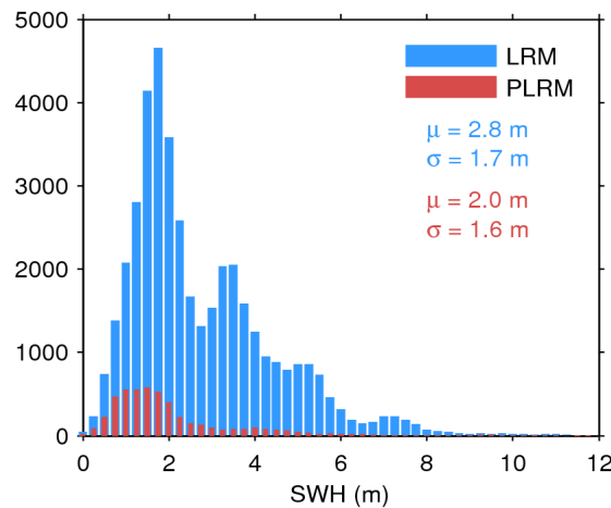
Figure 17. Histogram of flag-valid SWH over oceans and lakes for LRM (blue) and PLRM (red) for 04/07/2017. The mean ( \mu ) and standard deviation ( \sigma ) are also shown. Note that values larger than 12 m are excluded from the histogram for the sake of readability but not from the computation of \mu and \sigma .
