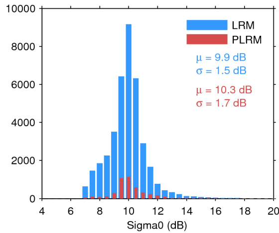
Figure 28. Histogram of science-valid sigma0 over oceans and lakes for LRM (blue) and PLRM (red) for 04/07/2017. The mean ( \mu ) and standard deviation ( \sigma ) are also shown. Note that values outside [4 20] dB are excluded from the histogram for the sake of readability but not from the computation of \mu and \sigma .
