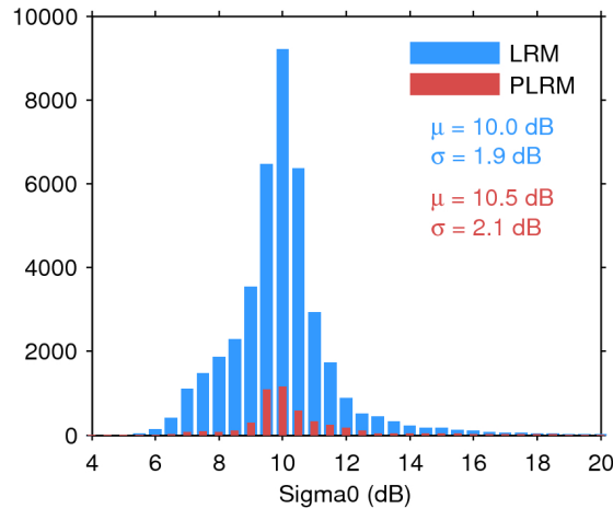
Figure 25. Histogram of flag-valid sigma0 over oceans and lakes for LRM (blue) and PLRM (red) for 04/07/2017. The mean ( \mu ) and standard deviation ( \sigma ) are also shown. Note that values outside [4 20] dB are excluded from the histogram for the sake of readability but not from the computation of \mu and \sigma .
