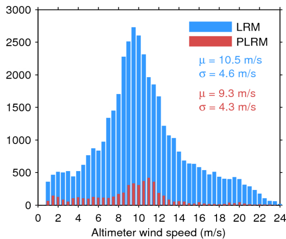
Figure 35. Histogram of science-valid wind over oceans and lakes for LRM (blue) and PLRM (red) for 04/07/2017. The mean ( \mu ) and standard deviation ( \sigma ) are also shown. Note that values larger than 24 m/s are excluded from the histogram for the sake of readability but not from the computation of \mu and \sigma .
