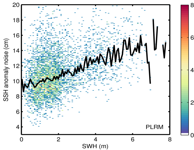
Figure 9. 2D histogram showing flag-valid SSH anomaly noise as a function of SWH for LRM (top) and PLRM (bottom) for 04/07/2017. The black line denotes the median SSH anomaly noise as a function of SWH.
