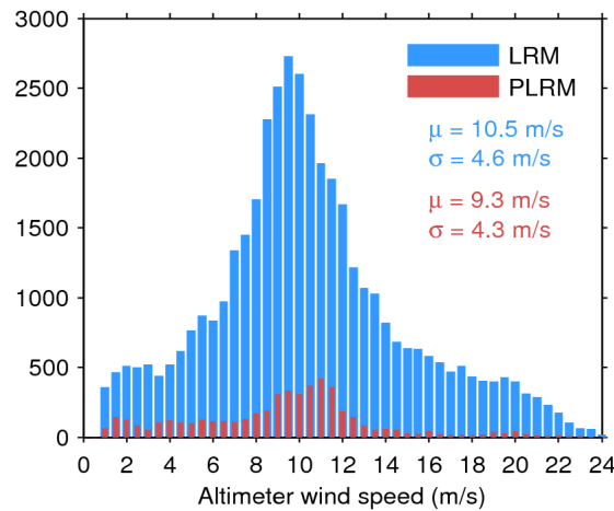
Figure 33. Histogram of flag-valid wind over oceans and lakes for LRM (blue) and PLRM (red) for 04/07/2017. The mean ( \mu ) and standard deviation ( \sigma ) are also shown. Note that values larger than 24 m/s are excluded from the histogram for the sake of readability but not from the computation of \mu and \sigma .
