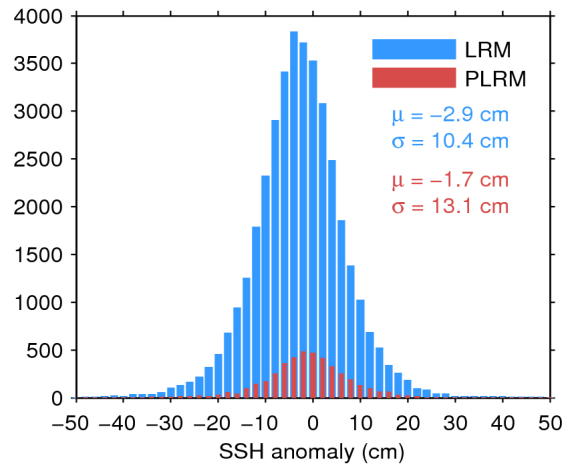
Figure 11. Histogram of science-valid SSH anomaly over oceans and lakes for LRM (blue) and PLRM (red) for 04/07/2017. The mean ( \mu ) and standard deviation ( \sigma ) are also shown. Note that values outside [-50\ 50] cm are excluded from the histogram for the sake of readability but not from the computation of \mu and \sigma .
