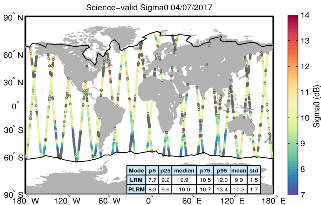
Figure 27. Geographical distribution of science-valid sigma0 data over oceans and lakes for 04/07/2017. The statistical values shown in the table refer to the sigma0 in dB and are calculated separately for LRM and PLRM regions. The black lines mark the outer limit of the Arctic and Antarctic polar polygons. Gray circles denote records that have been rejected based on the editing criteria described in Table 4.
