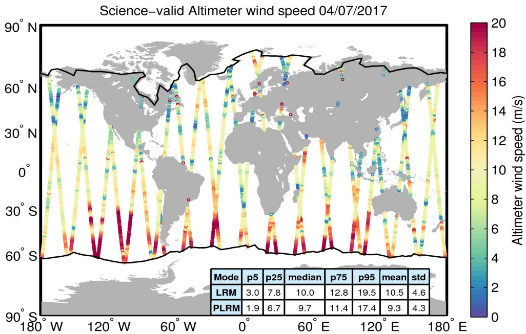
Figure 34. Geographical distribution of science-valid wind data over oceans and lakes for 04/07/2017. The statistical values shown in the table refer to the wind in m/s and are calculated separately for LRM and PLRM regions. The black lines mark the outer limit of the Arctic and Antarctic polar polygons. Gray circles denote records that have been rejected based on the editing criteria described in Table 5.
