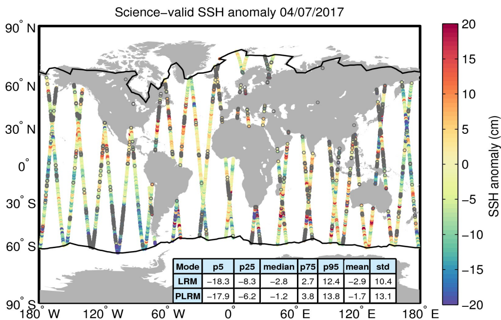
Figure 10. Geographical distribution of science-valid SSH anomaly data over oceans and lakes for 04/07/2017. The statistical values shown in the table refer to the SSH anomaly in cm and are calculated separately for LRM and PLRM regions. The black lines mark the outer limit of the Arctic and Antarctic polar polygons. Gray circles denote records that have been rejected based on the editing criteria described in Table 2.
