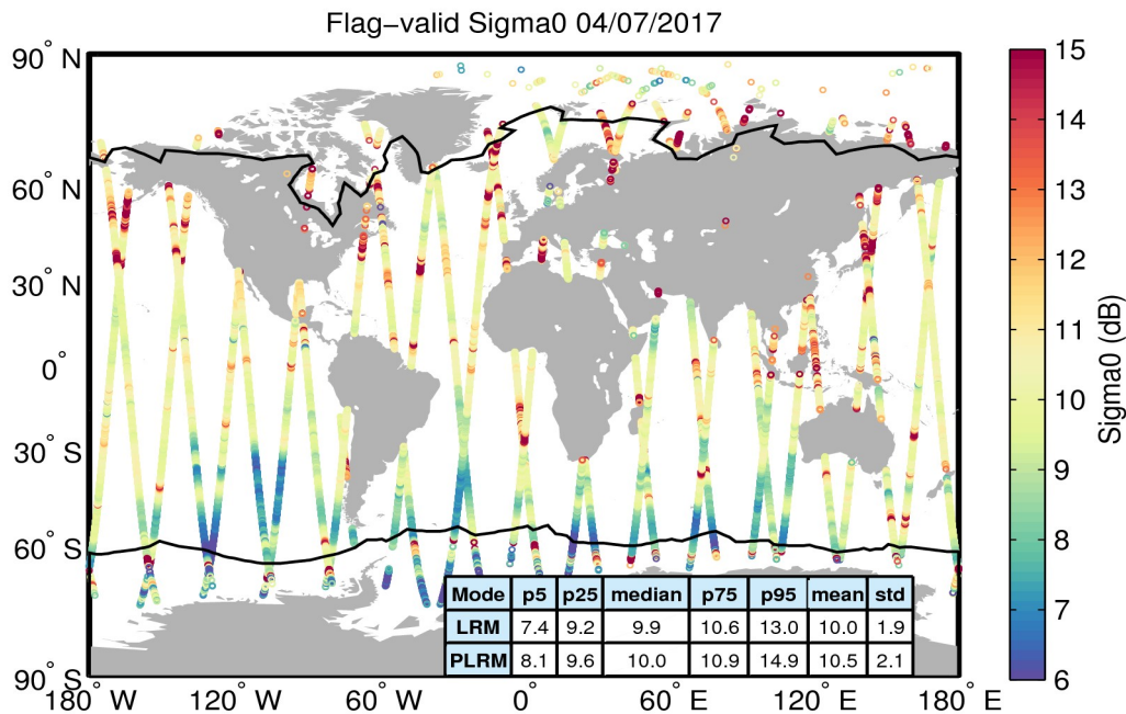
Figure 23. Geographical distribution of flag-valid sigma0 data over oceans and lakes for 04/07/2017. The statistical values shown in the table refer to the sigma0 in dB and are calculated separately for LRM and PLRM regions. Measurements taken over polar polygons have been excluded from the computation of the statistical values. The black lines mark the outer limit of the Arctic and Antarctic polar polygons.
