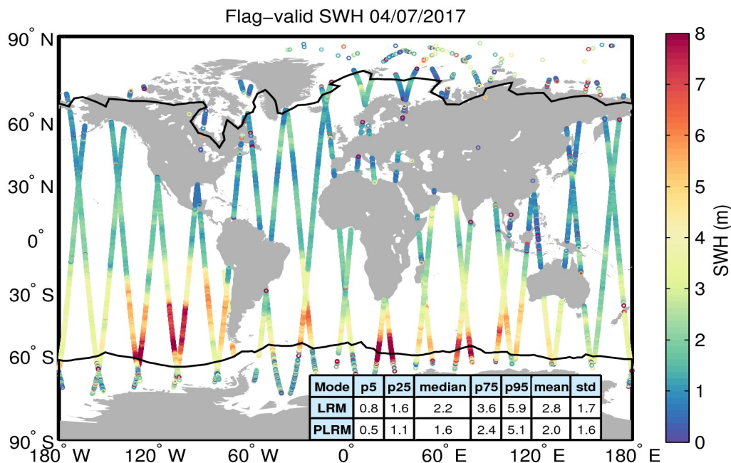
Figure 15. Geographical distribution of flag-valid SWH data over oceans and lakes for 04/07/2017. The statistical values shown in the table refer to the SWH in m and are calculated separately for LRM and PLRM regions. Measurements taken over polar polygons have been excluded from the computation of the statistical values. The black lines mark the outer limit of the Arctic and Antarctic polar polygons.
