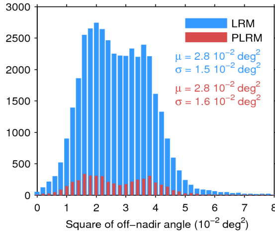
Figure 39. Histogram of flag-valid mispointing over oceans and lakes for LRM (blue) and PLRM (red) for 04/07/2017. Only positive values have been considered. The mean ( \mu ) and standard deviation ( \sigma ) are also shown. Note that values larger than 8 \cdot 10^{-2} \text{ deg}^2 are excluded from the histogram for the sake of readability but not from the computation of \mu and \sigma .
