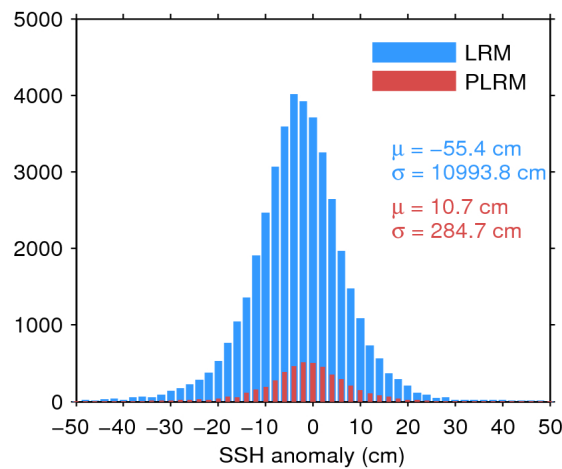
Figure 7. Histogram of flag-valid SSH anomaly over oceans and lakes for LRM (blue) and PLRM (red) for 04/07/2017. The mean ( \mu ) and standard deviation ( \sigma ) are also shown. Note that values outside [-50 50] cm are excluded from the histogram for the sake of readability but not from the computation of \mu and \sigma .
