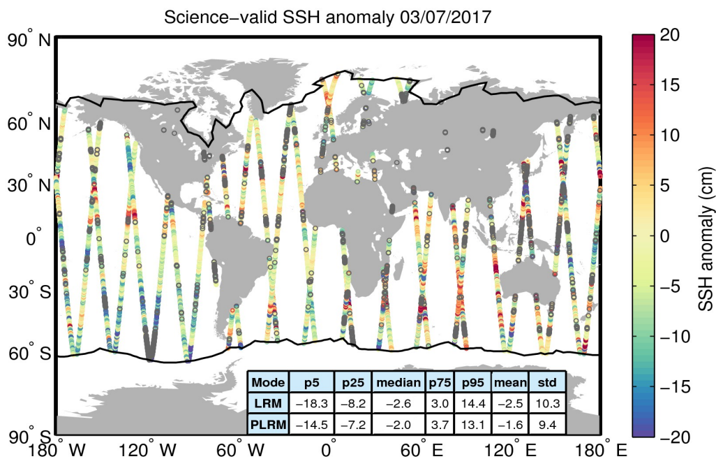
Figure 10. Geographical distribution of science-valid SSH anomaly data over oceans and lakes for 03/07/2017. The statistical values shown in the table refer to the SSH anomaly in cm and are calculated separately for LRM and PLRM regions. The black lines mark the outer limit of the Arctic and Antarctic polar polygons. Gray circles denote records that have been rejected based on the editing criteria described in Table 2.
