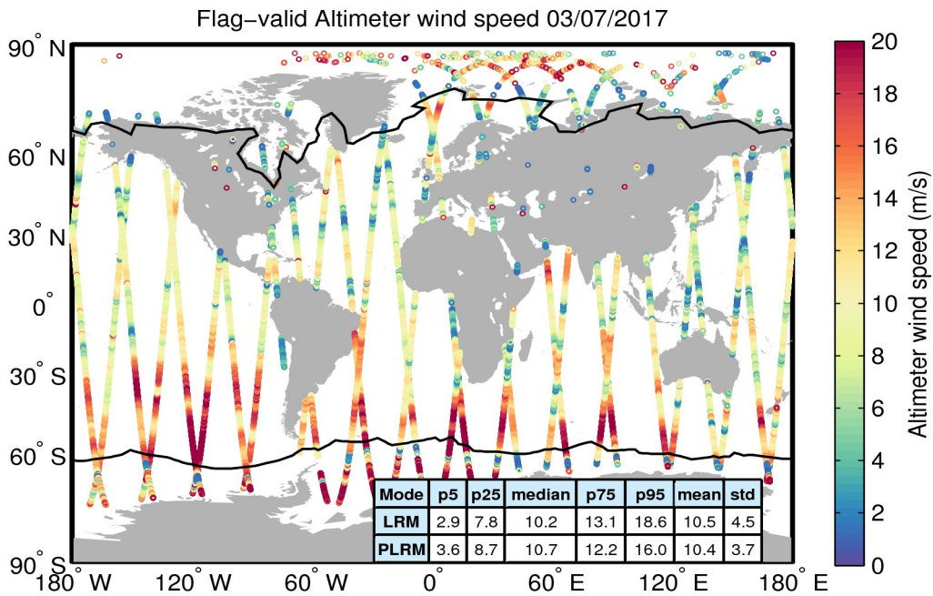
Figure 31. Geographical distribution of flag-valid wind data over oceans and lakes for 03/07/2017. The statistical values shown in the table refer to the wind in m/s and are calculated separately for LRM and PLRM regions. Measurements taken over polar polygons have been excluded from the computation of the statistical values. The black lines mark the outer limit of the Arctic and Antarctic polar polygons.
