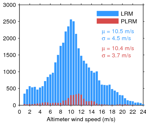
Figure 33. Histogram of flag-valid wind over oceans and lakes for LRM (blue) and PLRM (red) for 03/07/2017. The mean ( \mu ) and standard deviation ( \sigma ) are also shown. Note that values larger than 24 m/s are excluded from the histogram for the sake of readability but not from the computation of \mu and \sigma .
