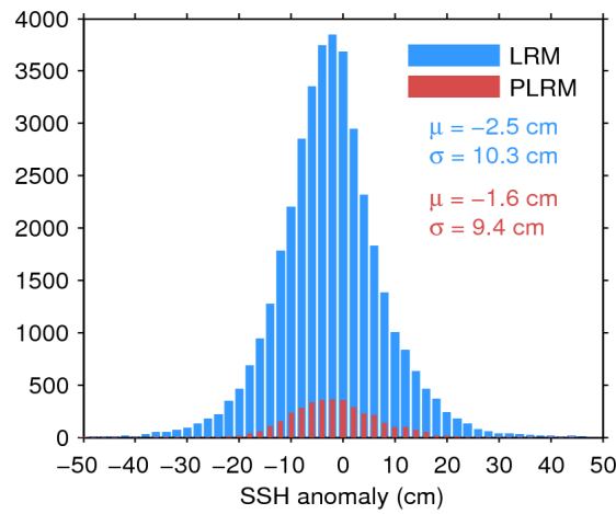
Figure 11. Histogram of science-valid SSH anomaly over oceans and lakes for LRM (blue) and PLRM (red) for 03/07/2017. The mean ( \mu ) and standard deviation ( \sigma ) are also shown. Note that values outside [-50 50] cm are excluded from the histogram for the sake of readability but not from the computation of \mu and \sigma .
