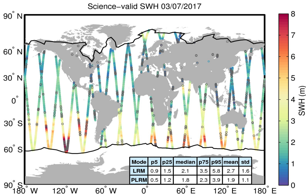
Figure 19. Geographical distribution of science-valid SWH data over oceans and lakes for 03/07/2017. The statistical values shown in the table refer to the SWH in m and are calculated separately for LRM and PLRM regions. The black lines mark the outer limit of the Arctic and Antarctic polar polygons. Gray circles denote records that have been rejected based on the editing criteria described in Table 3.
