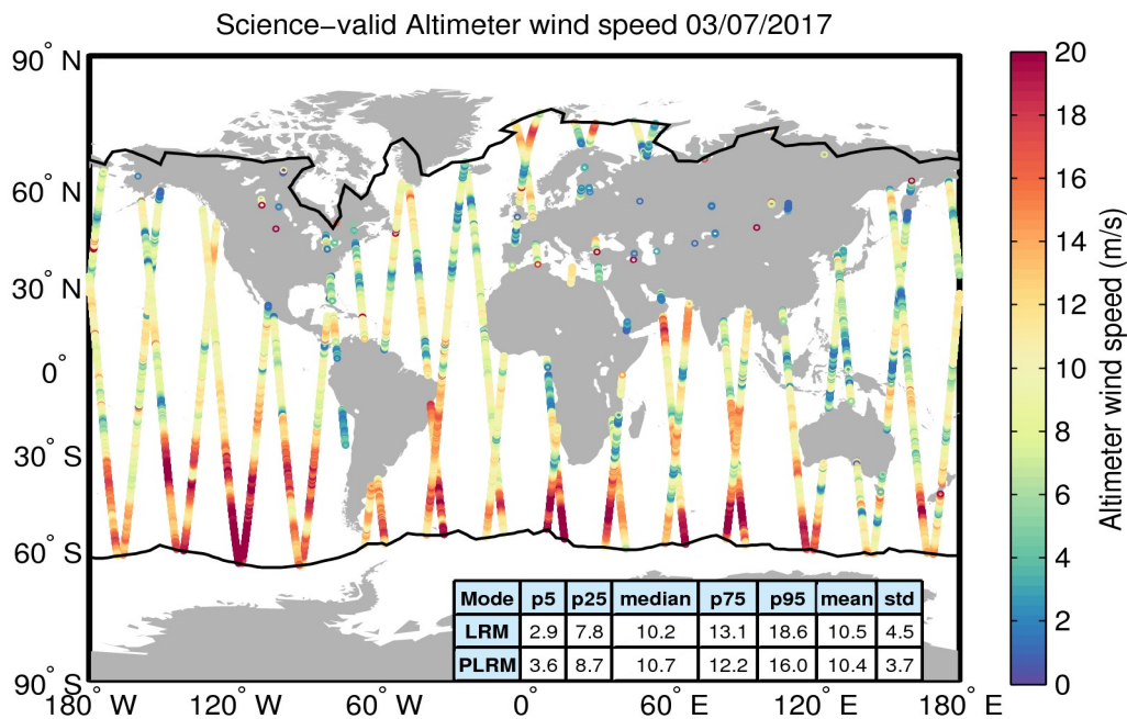
Figure 34. Geographical distribution of science-valid wind data over oceans and lakes for 03/07/2017. The statistical values shown in the table refer to the wind in m/s and are calculated separately for LRM and PLRM regions. The black lines mark the outer limit of the Arctic and Antarctic polar polygons. Gray circles denote records that have been rejected based on the editing criteria described in Table 5.
