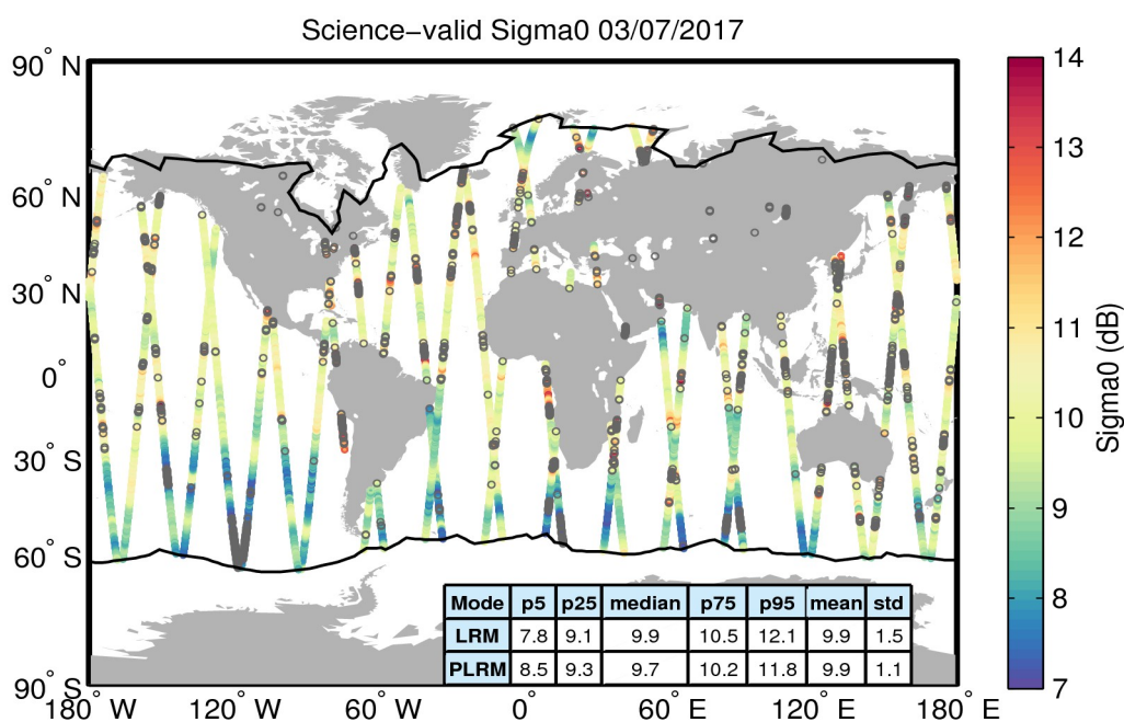
Figure 27. Geographical distribution of science-valid sigma0 data over oceans and lakes for 03/07/2017. The statistical values shown in the table refer to the sigma0 in dB and are calculated separately for LRM and PLRM regions. The black lines mark the outer limit of the Arctic and Antarctic polar polygons. Gray circles denote records that have been rejected based on the editing criteria described in Table 4.
