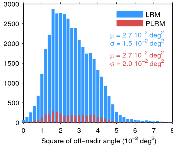
Figure 39. Histogram of flag-valid mispointing over oceans and lakes for LRM (blue) and PLRM (red) for 03/07/2017. Only positive values have been considered. The mean ( \mu ) and standard deviation ( \sigma ) are also shown. Note that values larger than 8 \cdot 10^{-2} \text{ deg}^2 are excluded from the histogram for the sake of readability but not from the computation of \mu and \sigma .
