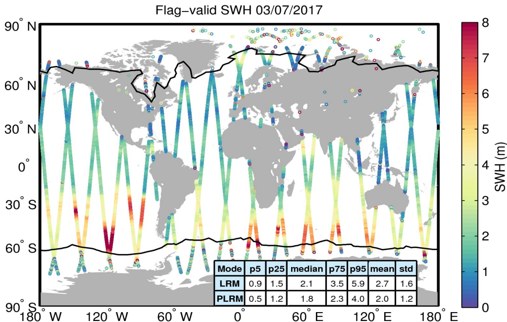
Figure 15. Geographical distribution of flag-valid SWH data over oceans and lakes for 03/07/2017. The statistical values shown in the table refer to the SWH in m and are calculated separately for LRM and PLRM regions. Measurements taken over polar polygons have been excluded from the computation of the statistical values. The black lines mark the outer limit of the Arctic and Antarctic polar polygons.
