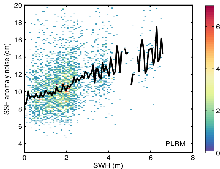
Figure 9. 2D histogram showing flag-valid SSH anomaly noise as a function of SWH for LRM (top) and PLRM (bottom) for 03/07/2017. The black line denotes the median SSH anomaly noise as a function of SWH.
