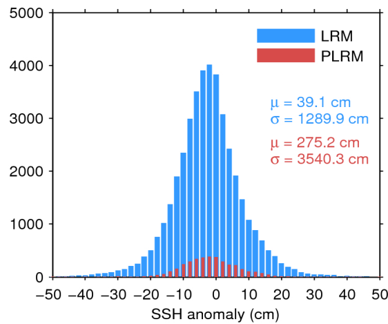
Figure 7. Histogram of flag-valid SSH anomaly over oceans and lakes for LRM (blue) and PLRM (red) for 03/07/2017. The mean ( \mu ) and standard deviation ( \sigma ) are also shown. Note that values outside [-50 50] cm are excluded from the histogram for the sake of readability but not from the computation of \mu and \sigma .
