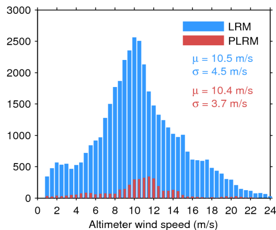
Figure 35. Histogram of science-valid wind over oceans and lakes for LRM (blue) and PLRM (red) for 03/07/2017. The mean ( \mu ) and standard deviation ( \sigma ) are also shown. Note that values larger than 24 m/s are excluded from the histogram for the sake of readability but not from the computation of \mu and \sigma .
