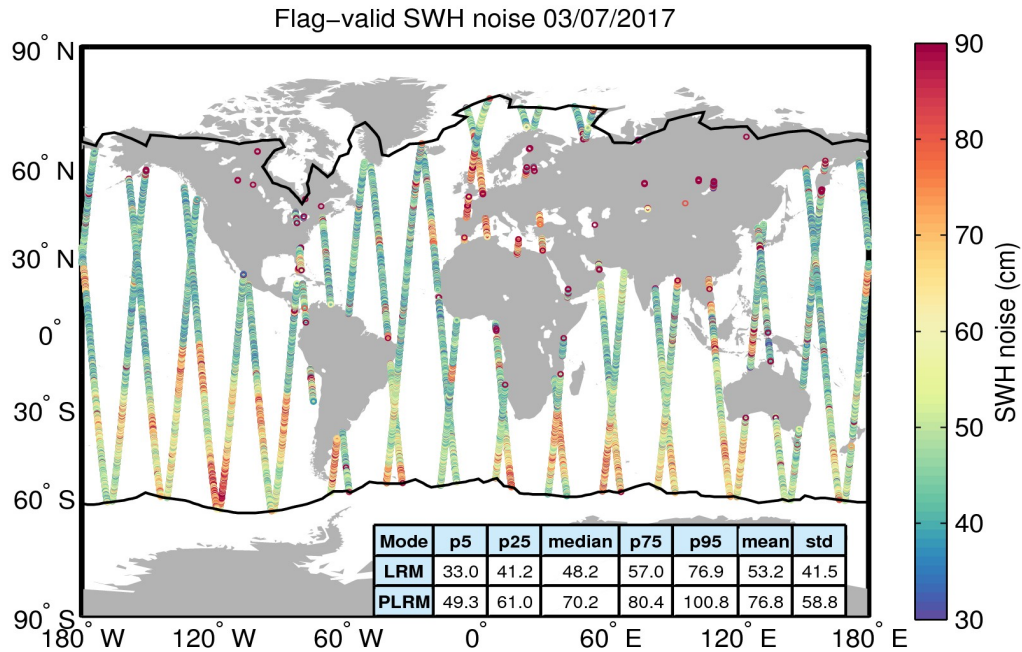
Figure 18. Geographical distribution of flag-valid 20-Hz SWH measurement noise over oceans and lakes for 03/07/2017. The statistical values shown in the table refer to the SWH noise and are calculated separately for LRM and PLRM regions. Measurements taken over polar polygons have been excluded from the computation of the statistical values. The black lines mark the outer limit of the Arctic and Antarctic polar polygons.
