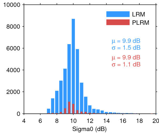
Figure 28. Histogram of science-valid sigma0 over oceans and lakes for LRM (blue) and PLRM (red) for 03/07/2017. The mean ( \mu ) and standard deviation ( \sigma ) are also shown. Note that values outside [4 20] dB are excluded from the histogram for the sake of readability but not from the computation of \mu and \sigma .
