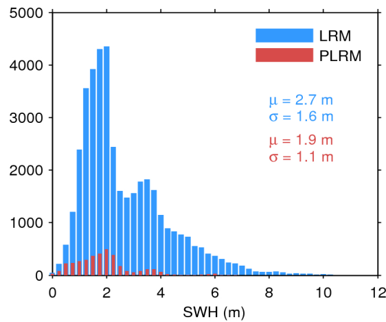
Figure 20. Histogram of science-valid SWH over oceans and lakes for LRM (blue) and PLRM (red) for 03/07/2017. The mean ( \mu ) and standard deviation ( \sigma ) are also shown. Note that values larger than 12 m are excluded from the histogram for the sake of readability but not from the computation of \mu and \sigma .
