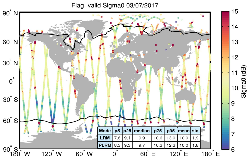
Figure 23. Geographical distribution of flag-valid sigma0 data over oceans and lakes for 03/07/2017. The statistical values shown in the table refer to the sigma0 in dB and are calculated separately for LRM and PLRM regions. Measurements taken over polar polygons have been excluded from the computation of the statistical values. The black lines mark the outer limit of the Arctic and Antarctic polar polygons.
