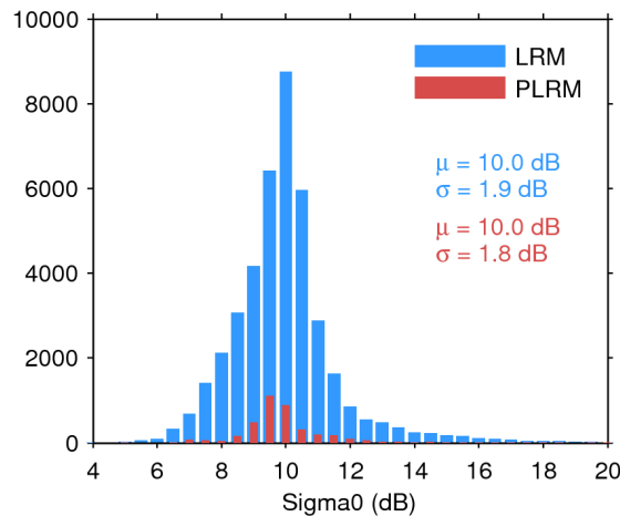
Figure 25. Histogram of flag-valid sigma0 over oceans and lakes for LRM (blue) and PLRM (red) for 03/07/2017. The mean ( \mu ) and standard deviation ( \sigma ) are also shown. Note that values outside [4 20] dB are excluded from the histogram for the sake of readability but not from the computation of \mu and \sigma .
