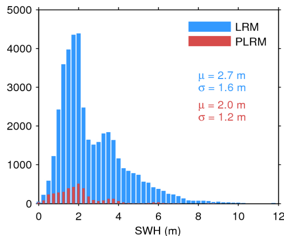
Figure 17. Histogram of flag-valid SWH over oceans and lakes for LRM (blue) and PLRM (red) for 03/07/2017. The mean ( \mu ) and standard deviation ( \sigma ) are also shown. Note that values larger than 12 m are excluded from the histogram for the sake of readability but not from the computation of \mu and \sigma .
