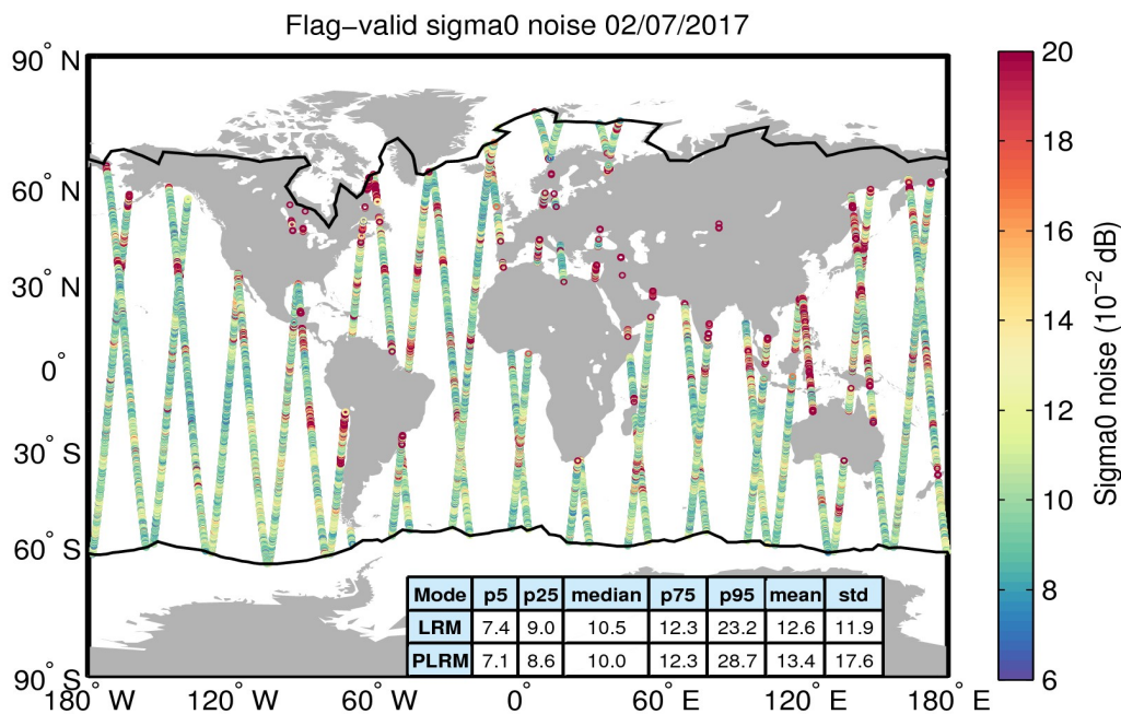
Figure 26. Geographical distribution of flag-valid 20-Hz sigma0 measurement noise over oceans and lakes for 02/07/2017. The statistical values shown in the table refer to the sigma0 noise and are calculated separately for LRM and PLRM regions. Measurements taken over polar polygons have been excluded from the computation of the statistical values. The black lines mark the outer limit of the Arctic and Antarctic polar polygons.
