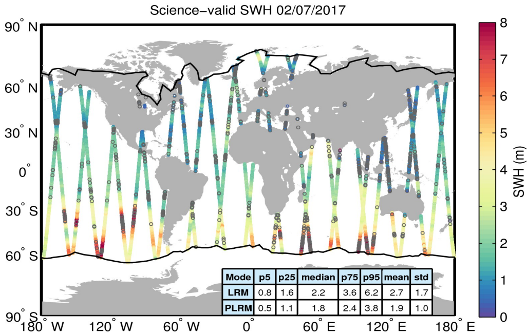
Figure 19. Geographical distribution of science-valid SWH data over oceans and lakes for 02/07/2017. The statistical values shown in the table refer to the SWH in m and are calculated separately for LRM and PLRM regions. The black lines mark the outer limit of the Arctic and Antarctic polar polygons. Gray circles denote records that have been rejected based on the editing criteria described in Table 3.
