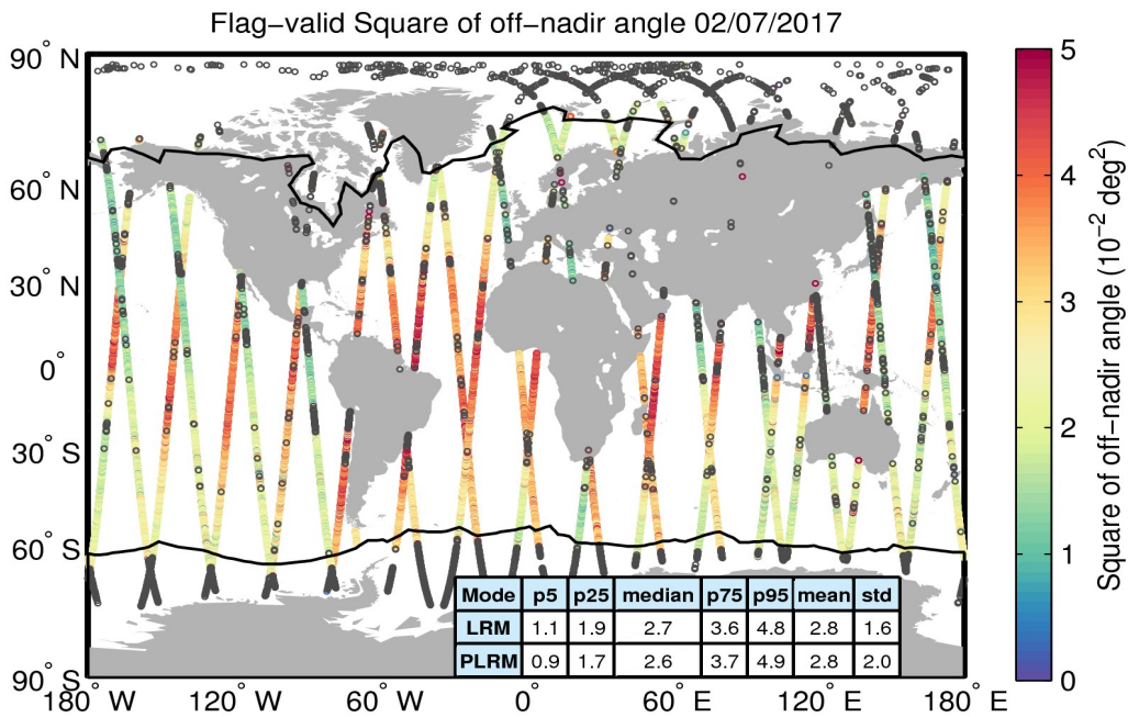
Figure 37. Geographical distribution of flag-valid mispointing data over oceans and lakes for 02/07/2017. The statistical values shown in the table refer to the mispointing in 10^{-2} deg 2 and are calculated separately for LRM and PLRM regions. Measurements taken over polar polygons have been excluded from the computation of the statistical values. The black lines mark the outer limit of the Arctic and Antarctic polar polygons. Gray circles denote negative values.
