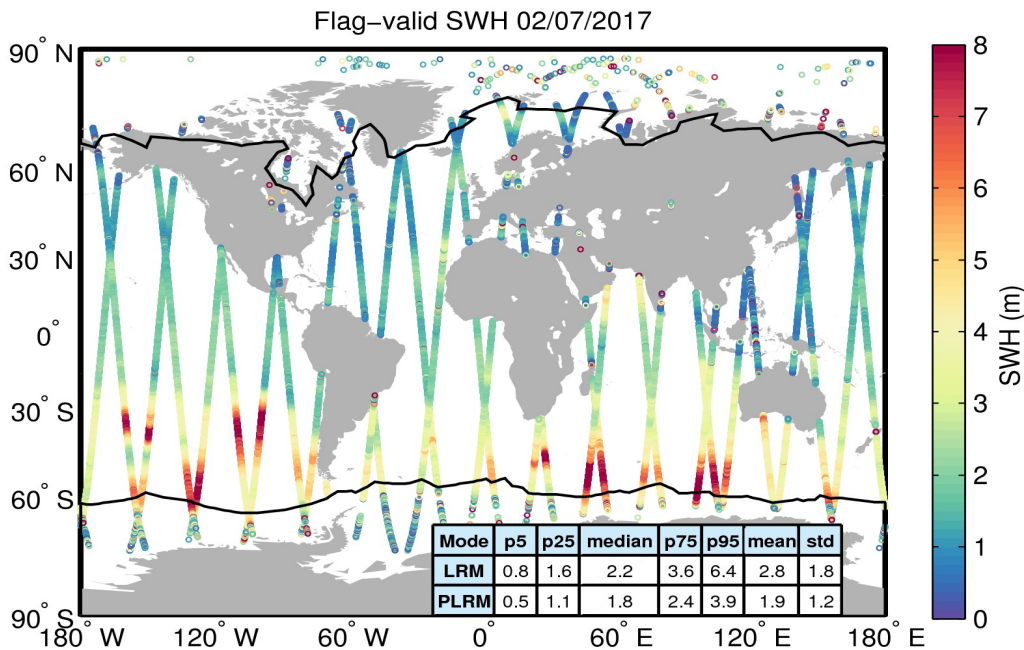
Figure 15. Geographical distribution of flag-valid SWH data over oceans and lakes for 02/07/2017. The statistical values shown in the table refer to the SWH in m and are calculated separately for LRM and PLRM regions. Measurements taken over polar polygons have been excluded from the computation of the statistical values. The black lines mark the outer limit of the Arctic and Antarctic polar polygons.
