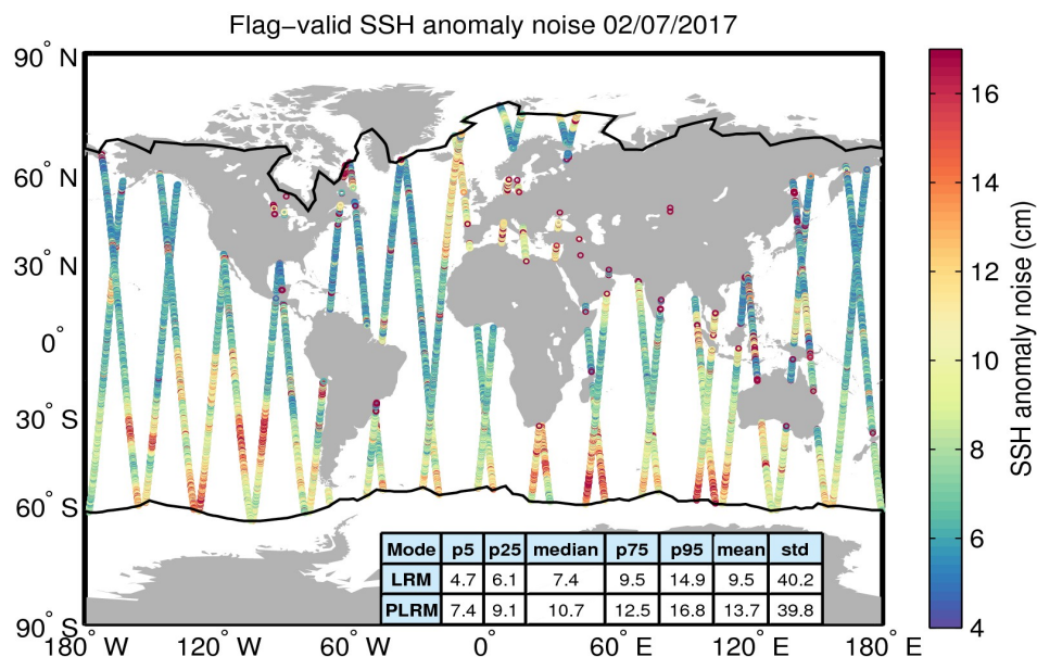
Figure 8. Geographical distribution of flag-valid 20-Hz SSH anomaly measurement noise over oceans and lakes for 02/07/2017. The statistical values shown in the table refer to the SSH anomaly noise and are calculated separately for LRM and PLRM regions. Measurements taken over polar polygons have been excluded from the computation of the statistical values. The black lines mark the outer limit of the Arctic and Antarctic polar polygons.
