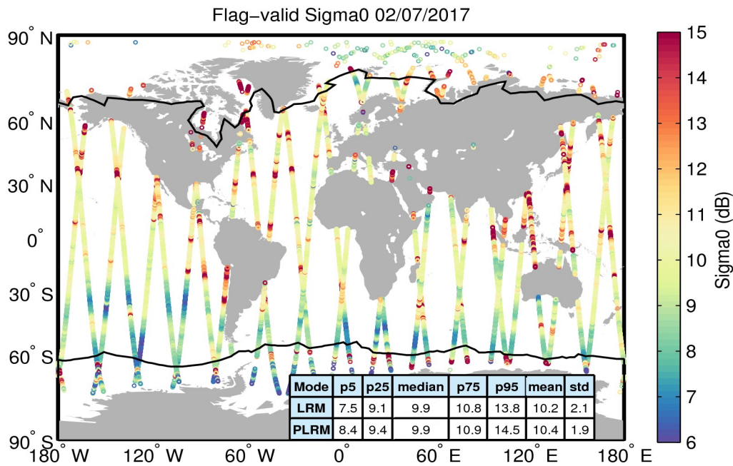
Figure 23. Geographical distribution of flag-valid sigma0 data over oceans and lakes for 02/07/2017. The statistical values shown in the table refer to the sigma0 in dB and are calculated separately for LRM and PLRM regions. Measurements taken over polar polygons have been excluded from the computation of the statistical values. The black lines mark the outer limit of the Arctic and Antarctic polar polygons.
