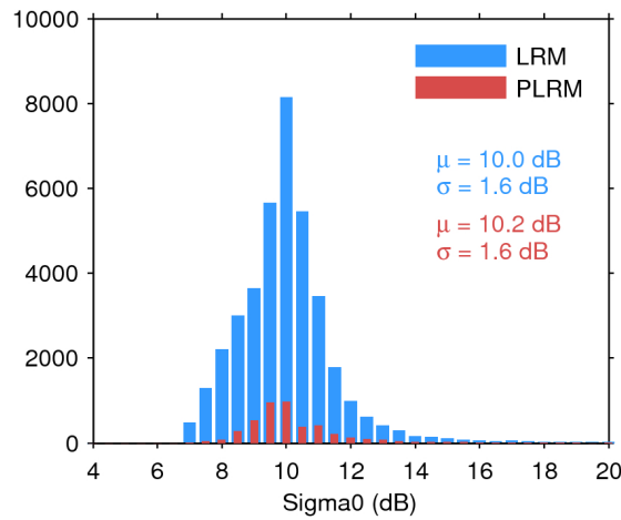
Figure 28. Histogram of science-valid sigma0 over oceans and lakes for LRM (blue) and PLRM (red) for 02/07/2017. The mean ( \mu ) and standard deviation ( \sigma ) are also shown. Note that values outside [4 20] dB are excluded from the histogram for the sake of readability but not from the computation of \mu and \sigma .
