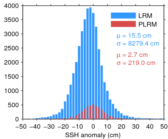
Figure 7. Histogram of flag-valid SSH anomaly over oceans and lakes for LRM (blue) and PLRM (red) for 02/07/2017. The mean ( \mu ) and standard deviation ( \sigma ) are also shown. Note that values outside [-50\ 50] cm are excluded from the histogram for the sake of readability but not from the computation of \mu and \sigma .
