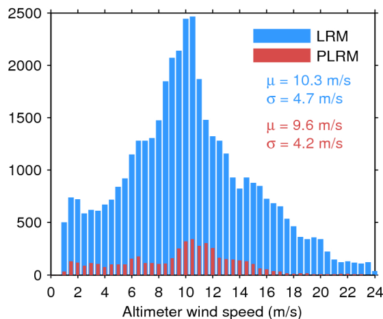
Figure 35. Histogram of science-valid wind over oceans and lakes for LRM (blue) and PLRM (red) for 02/07/2017. The mean ( \mu ) and standard deviation ( \sigma ) are also shown. Note that values larger than 24 m/s are excluded from the histogram for the sake of readability but not from the computation of \mu and \sigma .
