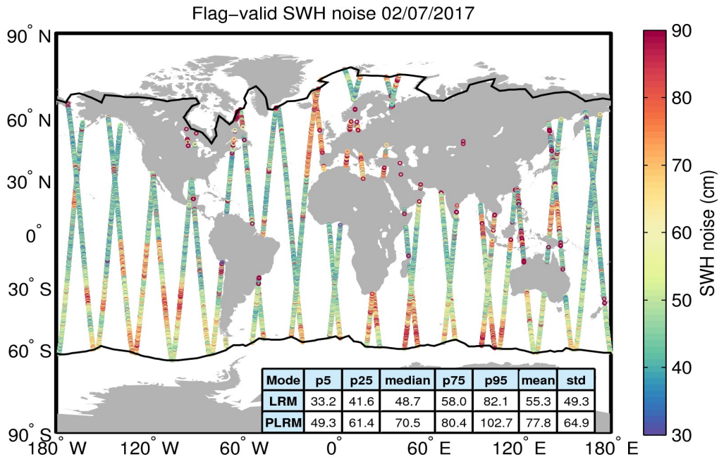
Figure 18. Geographical distribution of flag-valid 20-Hz SWH measurement noise over oceans and lakes for 02/07/2017. The statistical values shown in the table refer to the SWH noise and are calculated separately for LRM and PLRM regions. Measurements taken over polar polygons have been excluded from the computation of the statistical values. The black lines mark the outer limit of the Arctic and Antarctic polar polygons.
