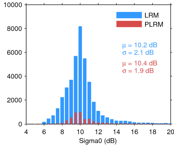
Figure 25. Histogram of flag-valid sigma0 over oceans and lakes for LRM (blue) and PLRM (red) for 02/07/2017. The mean ( \mu ) and standard deviation ( \sigma ) are also shown. Note that values outside [4 20] dB are excluded from the histogram for the sake of readability but not from the computation of \mu and \sigma .
