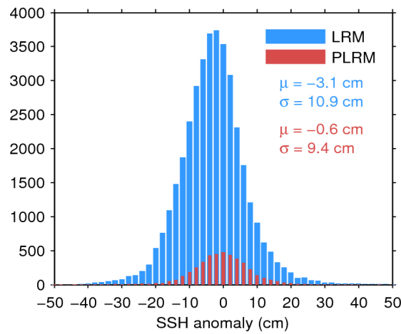
Figure 11. Histogram of science-valid SSH anomaly over oceans and lakes for LRM (blue) and PLRM (red) for 02/07/2017. The mean ( \mu ) and standard deviation ( \sigma ) are also shown. Note that values outside [-50 50] cm are excluded from the histogram for the sake of readability but not from the computation of \mu and \sigma .
