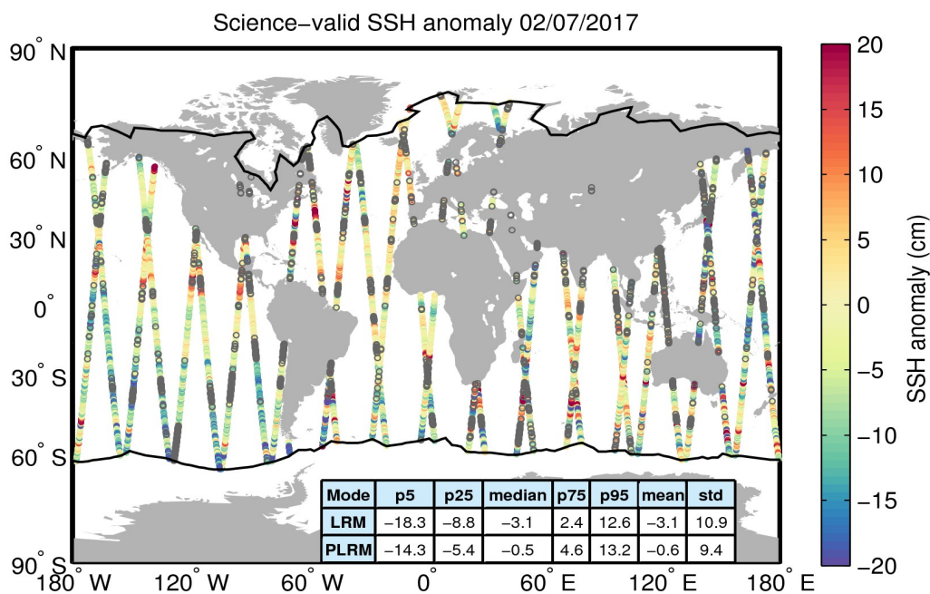
Figure 10. Geographical distribution of science-valid SSH anomaly data over oceans and lakes for 02/07/2017. The statistical values shown in the table refer to the SSH anomaly in cm and are calculated separately for LRM and PLRM regions. The black lines mark the outer limit of the Arctic and Antarctic polar polygons. Gray circles denote records that have been rejected based on the editing criteria described in Table 2.
