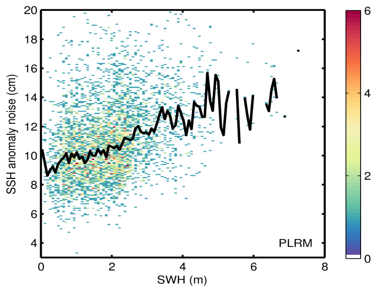
Figure 9. 2D histogram showing flag-valid SSH anomaly noise as a function of SWH for LRM (top) and PLRM (bottom) for 02/07/2017. The black line denotes the median SSH anomaly noise as a function of SWH.
