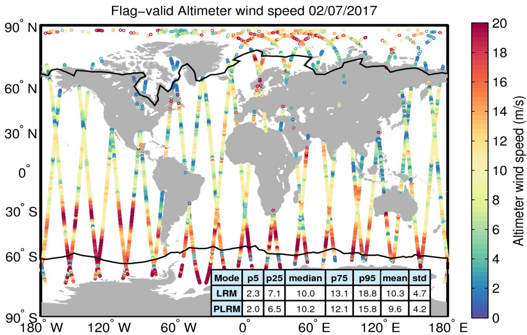
Figure 31. Geographical distribution of flag-valid wind data over oceans and lakes for 02/07/2017. The statistical values shown in the table refer to the wind in m/s and are calculated separately for LRM and PLRM regions. Measurements taken over polar polygons have been excluded from the computation of the statistical values. The black lines mark the outer limit of the Arctic and Antarctic polar polygons.
