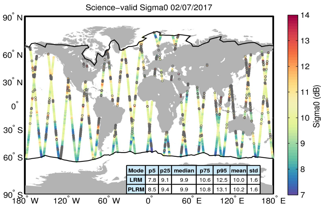
Figure 27. Geographical distribution of science-valid sigma0 data over oceans and lakes for 02/07/2017. The statistical values shown in the table refer to the sigma0 in dB and are calculated separately for LRM and PLRM regions. The black lines mark the outer limit of the Arctic and Antarctic polar polygons. Gray circles denote records that have been rejected based on the editing criteria described in Table 4.
