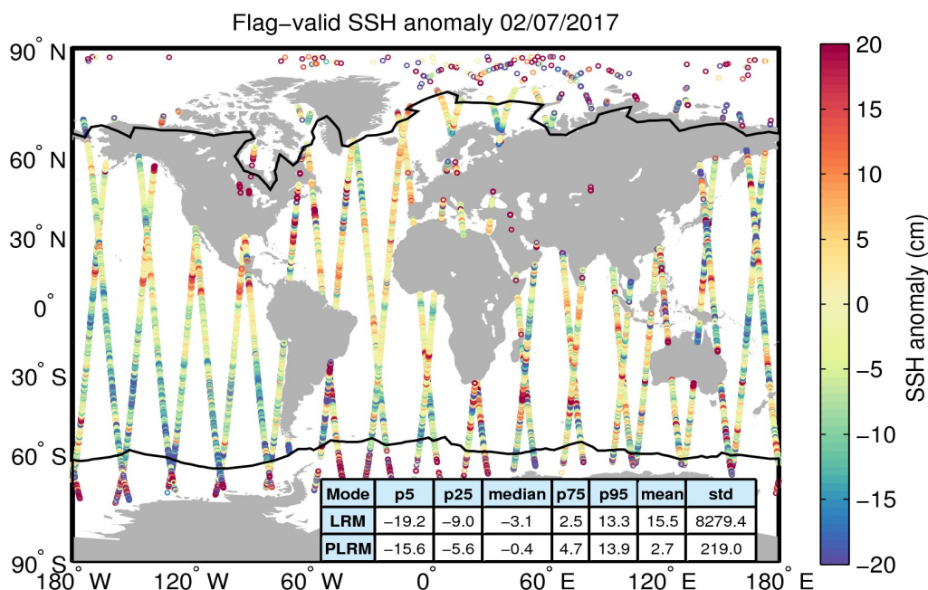
Figure 5. Geographical distribution of flag-valid 1-Hz SSH anomaly data over oceans and lakes for 02/07/2017. The statistical values shown in the table refer to the SSH anomaly in cm and are calculated separately for LRM and PLRM regions. Measurements taken over polar polygons have been excluded from the computation of the statistical values. The black lines mark the outer limit of the Arctic and Antarctic polar polygons.
