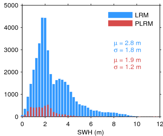
Figure 17. Histogram of flag-valid SWH over oceans and lakes for LRM (blue) and PLRM (red) for 02/07/2017. The mean ( \mu ) and standard deviation ( \sigma ) are also shown. Note that values larger than 12 m are excluded from the histogram for the sake of readability but not from the computation of \mu and \sigma .
