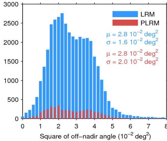
Figure 39. Histogram of flag-valid mispointing over oceans and lakes for LRM (blue) and PLRM (red) for 02/07/2017. Only positive values have been considered. The mean ( \mu ) and standard deviation ( \sigma ) are also shown. Note that values larger than 8 \cdot 10^{-2} \text{ deg}^2 are excluded from the histogram for the sake of readability but not from the computation of \mu and \sigma .
