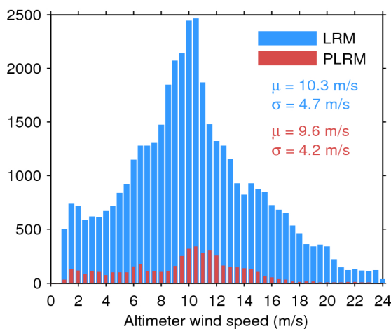
Figure 33. Histogram of flag-valid wind over oceans and lakes for LRM (blue) and PLRM (red) for 02/07/2017. The mean ( \mu ) and standard deviation ( \sigma ) are also shown. Note that values larger than 24 m/s are excluded from the histogram for the sake of readability but not from the computation of \mu and \sigma .
