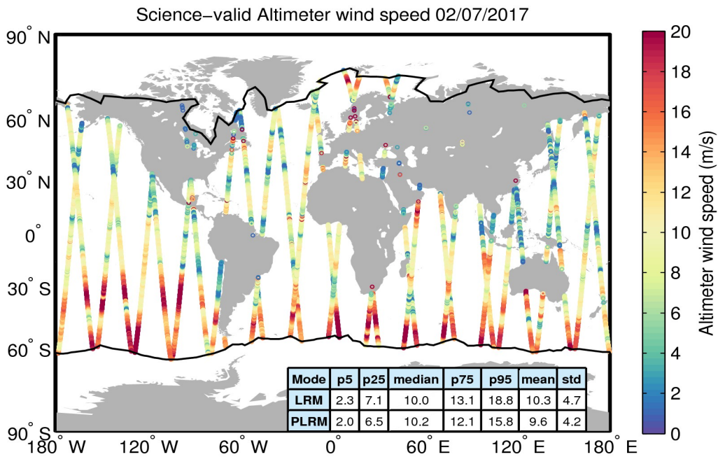
Figure 34. Geographical distribution of science-valid wind data over oceans and lakes for 02/07/2017. The statistical values shown in the table refer to the wind in m/s and are calculated separately for LRM and PLRM regions. The black lines mark the outer limit of the Arctic and Antarctic polar polygons. Gray circles denote records that have been rejected based on the editing criteria described in Table 5.
