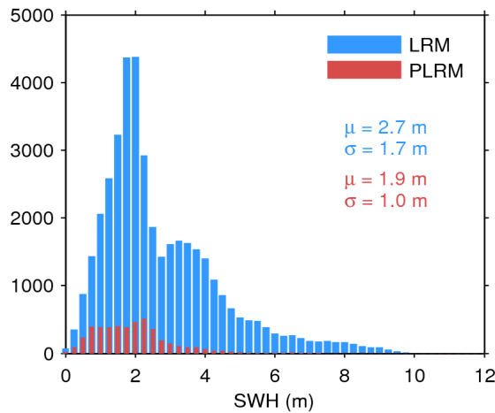
Figure 20. Histogram of science-valid SWH over oceans and lakes for LRM (blue) and PLRM (red) for 02/07/2017. The mean ( \mu ) and standard deviation ( \sigma ) are also shown. Note that values larger than 12 m are excluded from the histogram for the sake of readability but not from the computation of \mu and \sigma .
