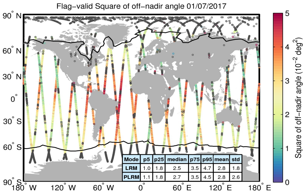
Figure 37. Geographical distribution of flag-valid mispointing data over oceans and lakes for 01/07/2017. The statistical values shown in the table refer to the mispointing in 10^{-2} deg 2 and are calculated separately for LRM and PLRM regions. Measurements taken over polar polygons have been excluded from the computation of the statistical values. The black lines mark the outer limit of the Arctic and Antarctic polar polygons. Gray circles denote negative values.
