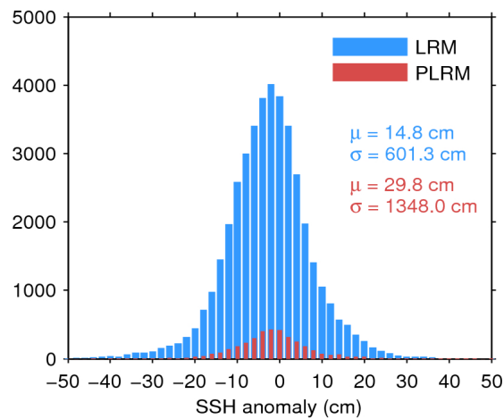
Figure 7. Histogram of flag-valid SSH anomaly over oceans and lakes for LRM (blue) and PLRM (red) for 01/07/2017. The mean ( \mu ) and standard deviation ( \sigma ) are also shown. Note that values outside [-50\ 50] cm are excluded from the histogram for the sake of readability but not from the computation of \mu and \sigma .
