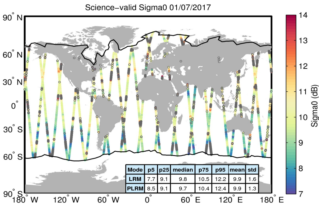
Figure 27. Geographical distribution of science-valid sigma0 data over oceans and lakes for 01/07/2017. The statistical values shown in the table refer to the sigma0 in dB and are calculated separately for LRM and PLRM regions. The black lines mark the outer limit of the Arctic and Antarctic polar polygons. Gray circles denote records that have been rejected based on the editing criteria described in Table 4.
