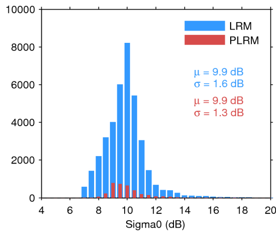
Figure 28. Histogram of science-valid sigma0 over oceans and lakes for LRM (blue) and PLRM (red) for 01/07/2017. The mean ( \mu ) and standard deviation ( \sigma ) are also shown. Note that values outside [4 20] dB are excluded from the histogram for the sake of readability but not from the computation of \mu and \sigma .
