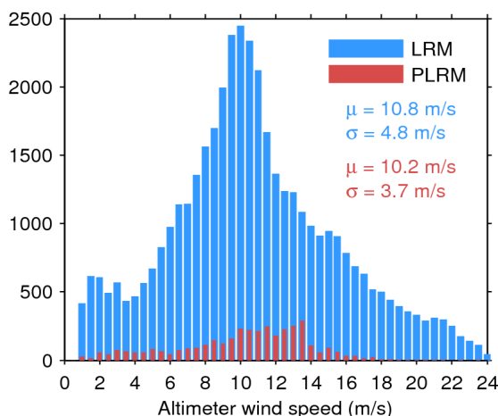
Figure 33. Histogram of flag-valid wind over oceans and lakes for LRM (blue) and PLRM (red) for 01/07/2017. The mean ( \mu ) and standard deviation ( \sigma ) are also shown. Note that values larger than 24 m/s are excluded from the histogram for the sake of readability but not from the computation of \mu and \sigma .
