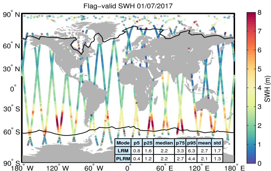
Figure 15. Geographical distribution of flag-valid SWH data over oceans and lakes for 01/07/2017. The statistical values shown in the table refer to the SWH in m and are calculated separately for LRM and PLRM regions. Measurements taken over polar polygons have been excluded from the computation of the statistical values. The black lines mark the outer limit of the Arctic and Antarctic polar polygons.
