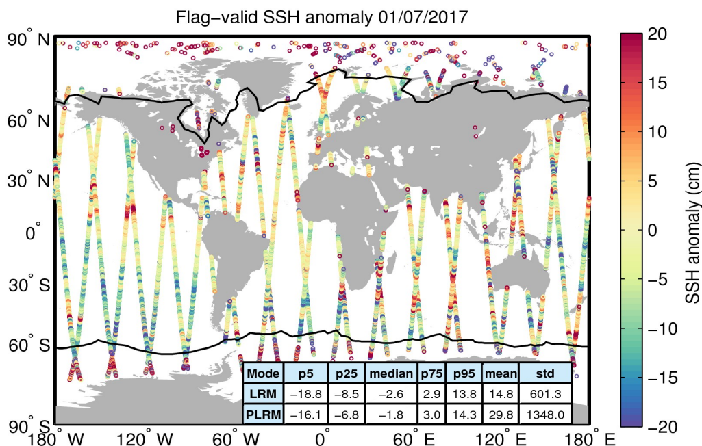
Figure 5. Geographical distribution of flag-valid 1-Hz SSH anomaly data over oceans and lakes for 01/07/2017. The statistical values shown in the table refer to the SSH anomaly in cm and are calculated separately for LRM and PLRM regions. Measurements taken over polar polygons have been excluded from the computation of the statistical values. The black lines mark the outer limit of the Arctic and Antarctic polar polygons.
