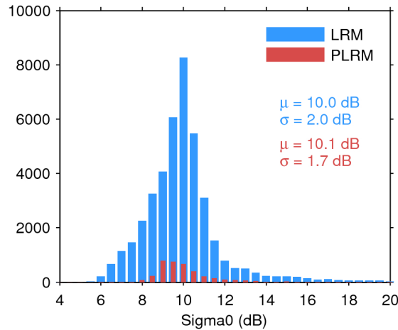
Figure 25. Histogram of flag-valid sigma0 over oceans and lakes for LRM (blue) and PLRM (red) for 01/07/2017. The mean ( \mu ) and standard deviation ( \sigma ) are also shown. Note that values outside [4 20] dB are excluded from the histogram for the sake of readability but not from the computation of \mu and \sigma .
