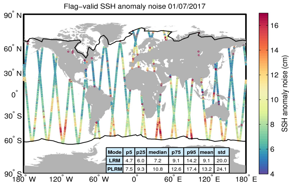
Figure 8. Geographical distribution of flag-valid 20-Hz SSH anomaly measurement noise over oceans and lakes for 01/07/2017. The statistical values shown in the table refer to the SSH anomaly noise and are calculated separately for LRM and PLRM regions. Measurements taken over polar polygons have been excluded from the computation of the statistical values. The black lines mark the outer limit of the Arctic and Antarctic polar polygons.
