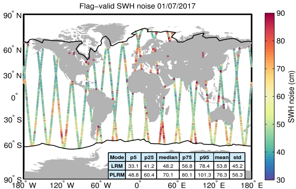
Figure 18. Geographical distribution of flag-valid 20-Hz SWH measurement noise over oceans and lakes for 01/07/2017. The statistical values shown in the table refer to the SWH noise and are calculated separately for LRM and PLRM regions. Measurements taken over polar polygons have been excluded from the computation of the statistical values. The black lines mark the outer limit of the Arctic and Antarctic polar polygons.
