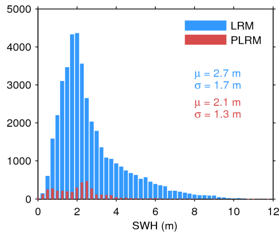
Figure 17. Histogram of flag-valid SWH over oceans and lakes for LRM (blue) and PLRM (red) for 01/07/2017. The mean ( \mu ) and standard deviation ( \sigma ) are also shown. Note that values larger than 12 m are excluded from the histogram for the sake of readability but not from the computation of \mu and \sigma .
