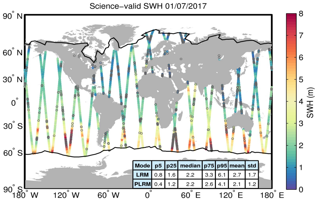
Figure 19. Geographical distribution of science-valid SWH data over oceans and lakes for 01/07/2017. The statistical values shown in the table refer to the SWH in m and are calculated separately for LRM and PLRM regions. The black lines mark the outer limit of the Arctic and Antarctic polar polygons. Gray circles denote records that have been rejected based on the editing criteria described in Table 3.
