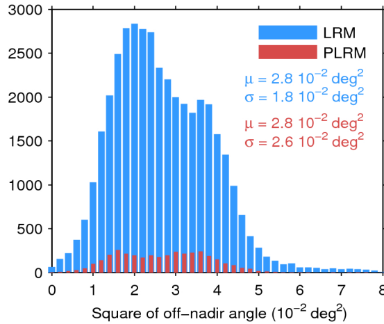
Figure 39. Histogram of flag-valid mispointing over oceans and lakes for LRM (blue) and PLRM (red) for 01/07/2017. Only positive values have been considered. The mean ( \mu ) and standard deviation ( \sigma ) are also shown. Note that values larger than 8 \cdot 10^{-2} \text{ deg}^2 are excluded from the histogram for the sake of readability but not from the computation of \mu and \sigma .
