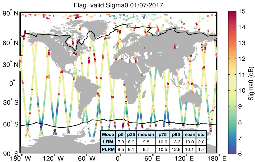
Figure 23. Geographical distribution of flag-valid sigma0 data over oceans and lakes for 01/07/2017. The statistical values shown in the table refer to the sigma0 in dB and are calculated separately for LRM and PLRM regions. Measurements taken over polar polygons have been excluded from the computation of the statistical values. The black lines mark the outer limit of the Arctic and Antarctic polar polygons.
