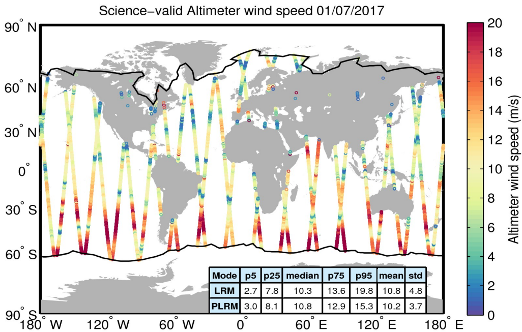
Figure 34. Geographical distribution of science-valid wind data over oceans and lakes for 01/07/2017. The statistical values shown in the table refer to the wind in m/s and are calculated separately for LRM and PLRM regions. The black lines mark the outer limit of the Arctic and Antarctic polar polygons. Gray circles denote records that have been rejected based on the editing criteria described in Table 5.
