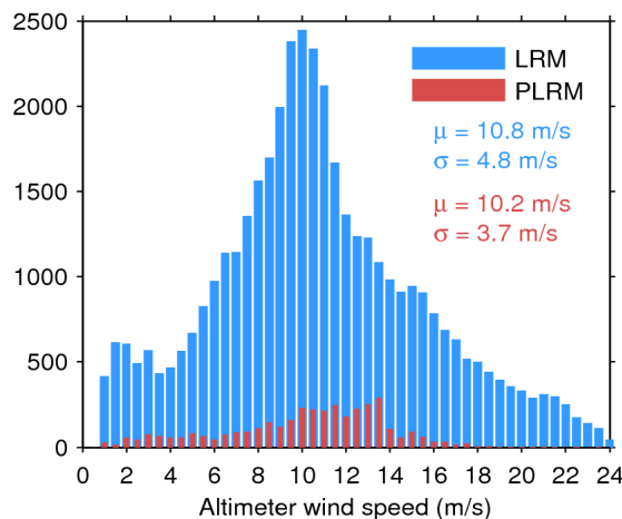
Figure 35. Histogram of science-valid wind over oceans and lakes for LRM (blue) and PLRM (red) for 01/07/2017. The mean ( \mu ) and standard deviation ( \sigma ) are also shown. Note that values larger than 24 m/s are excluded from the histogram for the sake of readability but not from the computation of \mu and \sigma .
