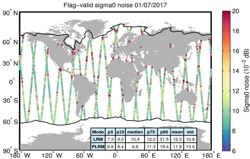
Figure 26. Geographical distribution of flag-valid 20-Hz sigma0 measurement noise over oceans and lakes for 01/07/2017. The statistical values shown in the table refer to the sigma0 noise and are calculated separately for LRM and PLRM regions. Measurements taken over polar polygons have been excluded from the computation of the statistical values. The black lines mark the outer limit of the Arctic and Antarctic polar polygons.
