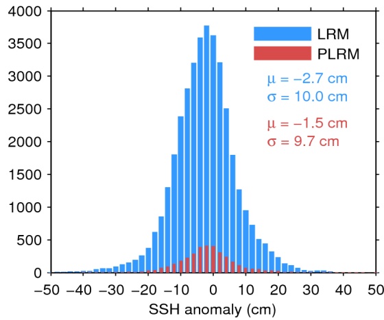
Figure 11. Histogram of science-valid SSH anomaly over oceans and lakes for LRM (blue) and PLRM (red) for 01/07/2017. The mean ( \mu ) and standard deviation ( \sigma ) are also shown. Note that values outside [-50\ 50] cm are excluded from the histogram for the sake of readability but not from the computation of \mu and \sigma .
