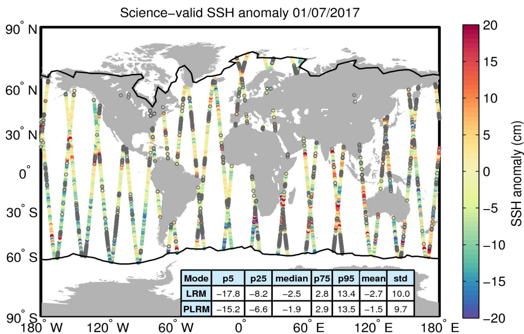
Figure 10. Geographical distribution of science-valid SSH anomaly data over oceans and lakes for 01/07/2017. The statistical values shown in the table refer to the SSH anomaly in cm and are calculated separately for LRM and PLRM regions. The black lines mark the outer limit of the Arctic and Antarctic polar polygons. Gray circles denote records that have been rejected based on the editing criteria described in Table 2.
