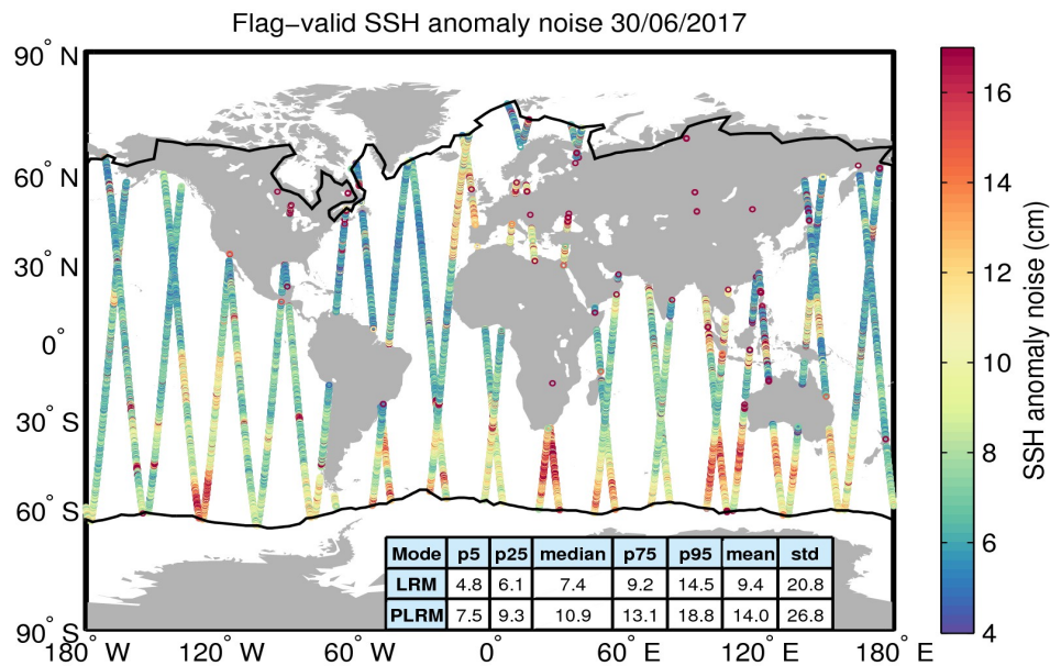
Figure 8. Geographical distribution of flag-valid 20-Hz SSH anomaly measurement noise over oceans and lakes for 30/06/2017. The statistical values shown in the table refer to the SSH anomaly noise and are calculated separately for LRM and PLRM regions. Measurements taken over polar polygons have been excluded from the computation of the statistical values. The black lines mark the outer limit of the Arctic and Antarctic polar polygons.
