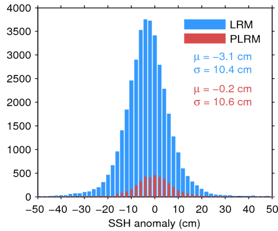
Figure 11. Histogram of science-valid SSH anomaly over oceans and lakes for LRM (blue) and PLRM (red) for 30/06/2017. The mean ( \mu ) and standard deviation ( \sigma ) are also shown. Note that values outside [-50 50] cm are excluded from the histogram for the sake of readability but not from the computation of \mu and \sigma .
