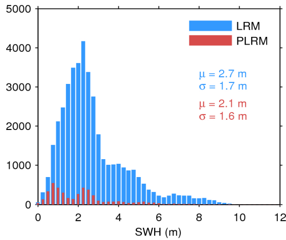
Figure 20. Histogram of science-valid SWH over oceans and lakes for LRM (blue) and PLRM (red) for 30/06/2017. The mean ( \mu ) and standard deviation ( \sigma ) are also shown. Note that values larger than 12 m are excluded from the histogram for the sake of readability but not from the computation of \mu and \sigma .
