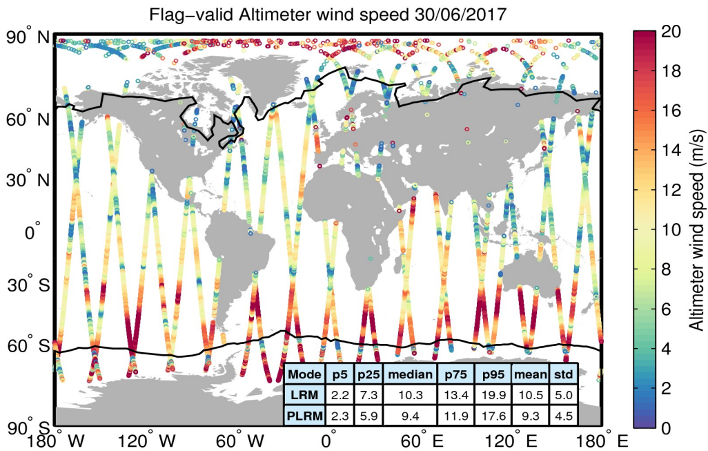
Figure 31. Geographical distribution of flag-valid wind data over oceans and lakes for 30/06/2017. The statistical values shown in the table refer to the wind in m/s and are calculated separately for LRM and PLRM regions. Measurements taken over polar polygons have been excluded from the computation of the statistical values. The black lines mark the outer limit of the Arctic and Antarctic polar polygons.
