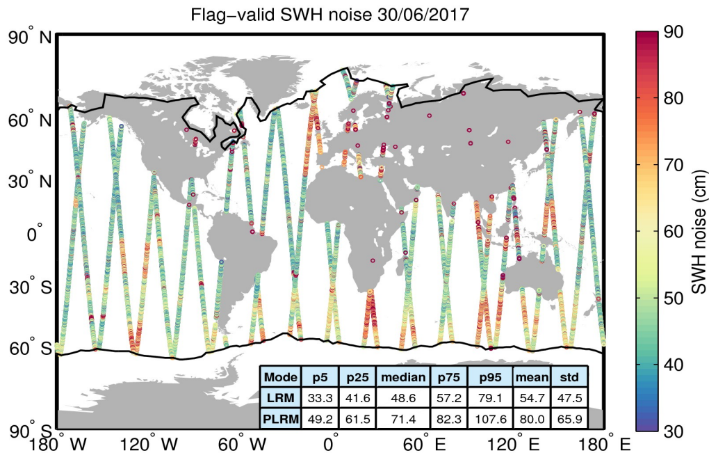
Figure 18. Geographical distribution of flag-valid 20-Hz SWH measurement noise over oceans and lakes for 30/06/2017. The statistical values shown in the table refer to the SWH noise and are calculated separately for LRM and PLRM regions. Measurements taken over polar polygons have been excluded from the computation of the statistical values. The black lines mark the outer limit of the Arctic and Antarctic polar polygons.
