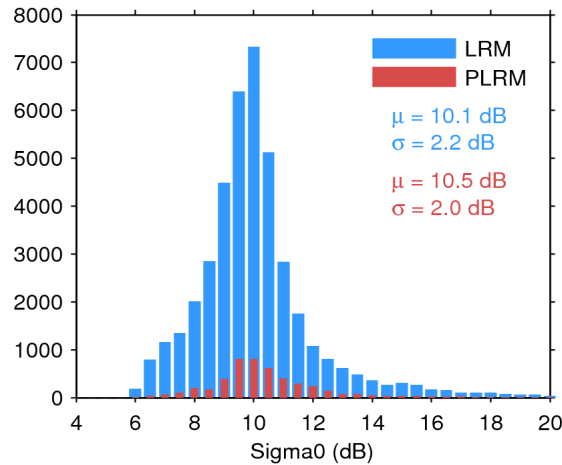
Figure 25. Histogram of flag-valid sigma0 over oceans and lakes for LRM (blue) and PLRM (red) for 30/06/2017. The mean ( \mu ) and standard deviation ( \sigma ) are also shown. Note that values outside [4 20] dB are excluded from the histogram for the sake of readability but not from the computation of \mu and \sigma .
