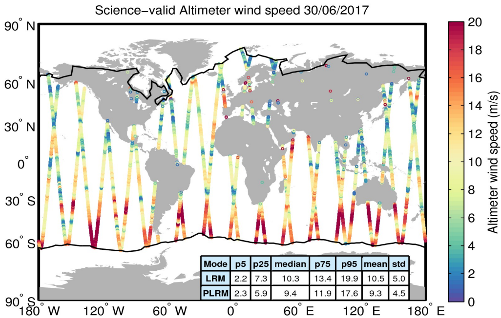
Figure 34. Geographical distribution of science-valid wind data over oceans and lakes for 30/06/2017. The statistical values shown in the table refer to the wind in m/s and are calculated separately for LRM and PLRM regions. The black lines mark the outer limit of the Arctic and Antarctic polar polygons. Gray circles denote records that have been rejected based on the editing criteria described in Table 5.
