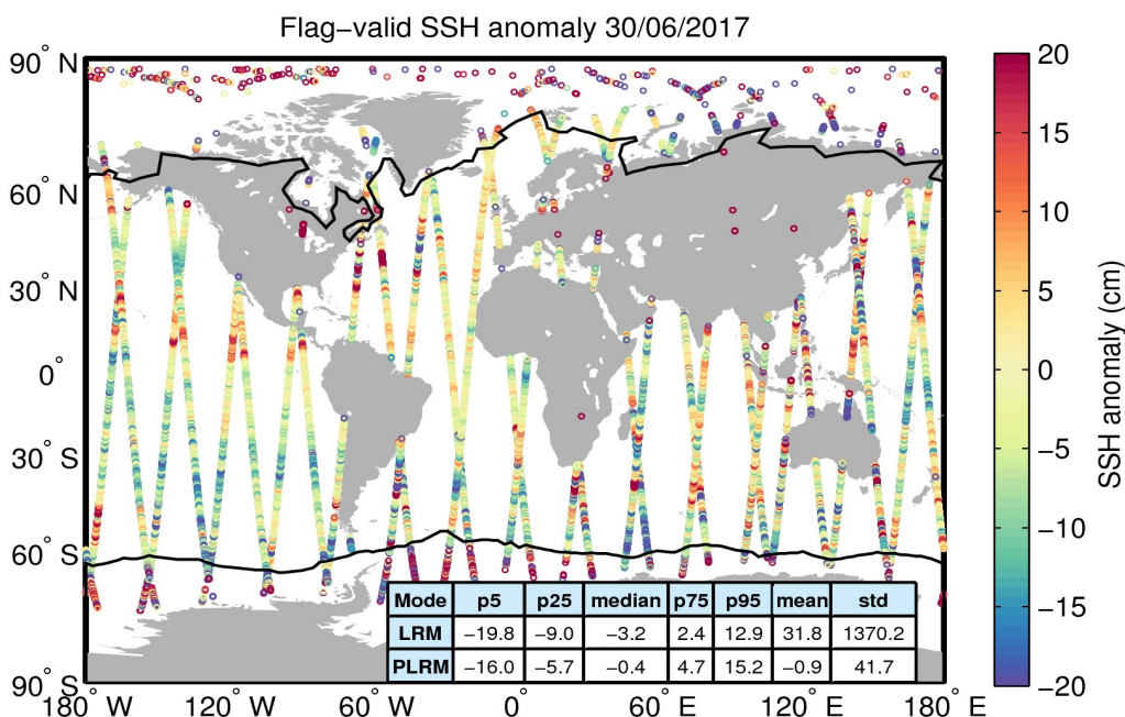
Figure 5. Geographical distribution of flag-valid 1-Hz SSH anomaly data over oceans and lakes for 30/06/2017. The statistical values shown in the table refer to the SSH anomaly in cm and are calculated separately for LRM and PLRM regions. Measurements taken over polar polygons have been excluded from the computation of the statistical values. The black lines mark the outer limit of the Arctic and Antarctic polar polygons.
