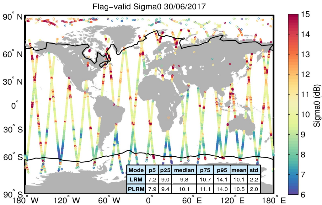
Figure 23. Geographical distribution of flag-valid sigma0 data over oceans and lakes for 30/06/2017. The statistical values shown in the table refer to the sigma0 in dB and are calculated separately for LRM and PLRM regions. Measurements taken over polar polygons have been excluded from the computation of the statistical values. The black lines mark the outer limit of the Arctic and Antarctic polar polygons.
