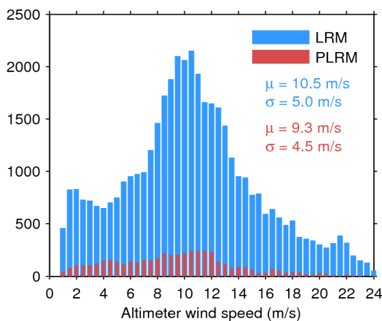
Figure 33. Histogram of flag-valid wind over oceans and lakes for LRM (blue) and PLRM (red) for 30/06/2017. The mean ( \mu ) and standard deviation ( \sigma ) are also shown. Note that values larger than 24 m/s are excluded from the histogram for the sake of readability but not from the computation of \mu and \sigma .
