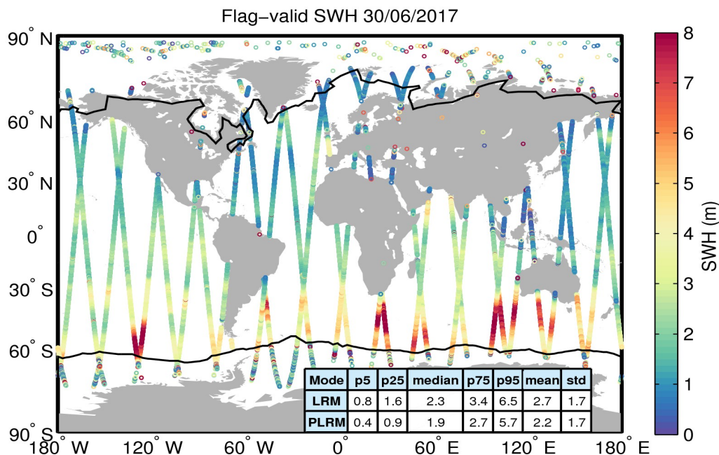
Figure 15. Geographical distribution of flag-valid SWH data over oceans and lakes for 30/06/2017. The statistical values shown in the table refer to the SWH in m and are calculated separately for LRM and PLRM regions. Measurements taken over polar polygons have been excluded from the computation of the statistical values. The black lines mark the outer limit of the Arctic and Antarctic polar polygons.
