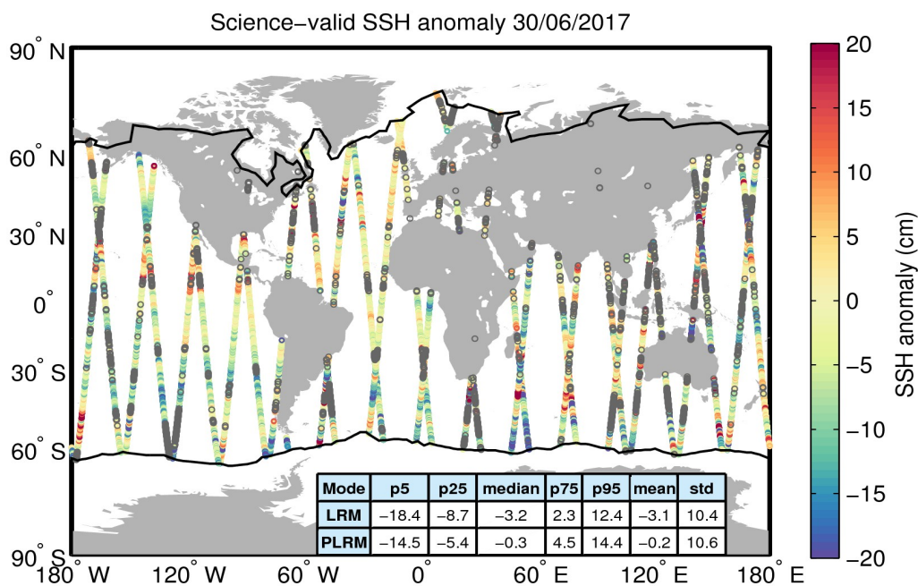
Figure 10. Geographical distribution of science-valid SSH anomaly data over oceans and lakes for 30/06/2017. The statistical values shown in the table refer to the SSH anomaly in cm and are calculated separately for LRM and PLRM regions. The black lines mark the outer limit of the Arctic and Antarctic polar polygons. Gray circles denote records that have been rejected based on the editing criteria described in Table 2.
