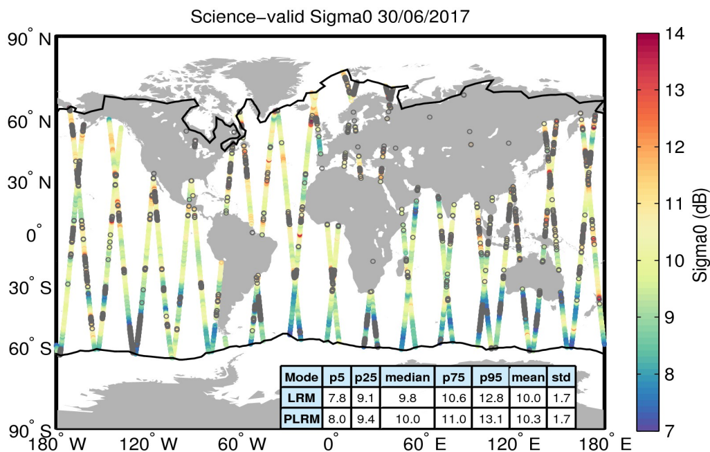
Figure 27. Geographical distribution of science-valid sigma0 data over oceans and lakes for 30/06/2017. The statistical values shown in the table refer to the sigma0 in dB and are calculated separately for LRM and PLRM regions. The black lines mark the outer limit of the Arctic and Antarctic polar polygons. Gray circles denote records that have been rejected based on the editing criteria described in Table 4.
