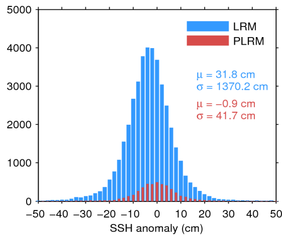
Figure 7. Histogram of flag-valid SSH anomaly over oceans and lakes for LRM (blue) and PLRM (red) for 30/06/2017. The mean ( \mu ) and standard deviation ( \sigma ) are also shown. Note that values outside [-50 50] cm are excluded from the histogram for the sake of readability but not from the computation of \mu and \sigma .
