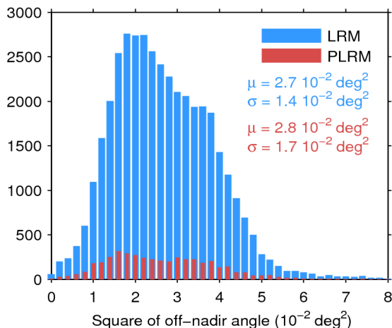
Figure 39. Histogram of flag-valid mispointing over oceans and lakes for LRM (blue) and PLRM (red) for 30/06/2017. Only positive values have been considered. The mean ( \mu ) and standard deviation ( \sigma ) are also shown. Note that values larger than 8 \cdot 10^{-2} \text{ deg}^2 are excluded from the histogram for the sake of readability but not from the computation of \mu and \sigma .
