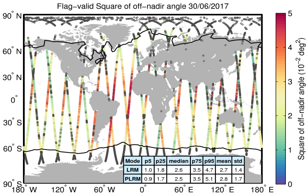
Figure 37. Geographical distribution of flag-valid mispointing data over oceans and lakes for 30/06/2017. The statistical values shown in the table refer to the mispointing in 10^{-2} deg 2 and are calculated separately for LRM and PLRM regions. Measurements taken over polar polygons have been excluded from the computation of the statistical values. The black lines mark the outer limit of the Arctic and Antarctic polar polygons. Gray circles denote negative values.
