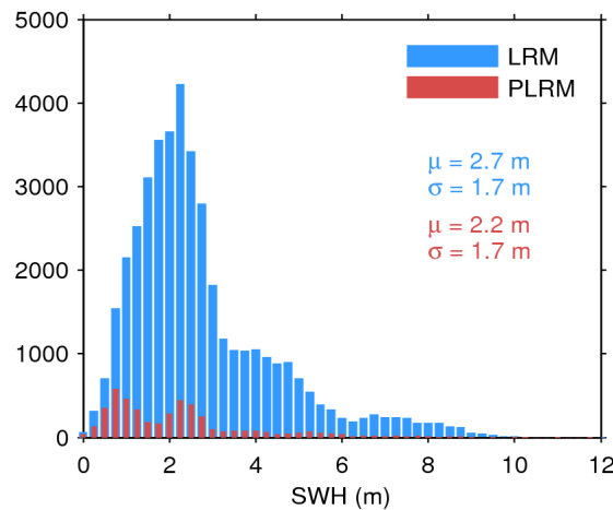
Figure 17. Histogram of flag-valid SWH over oceans and lakes for LRM (blue) and PLRM (red) for 30/06/2017. The mean ( \mu ) and standard deviation ( \sigma ) are also shown. Note that values larger than 12 m are excluded from the histogram for the sake of readability but not from the computation of \mu and \sigma .
