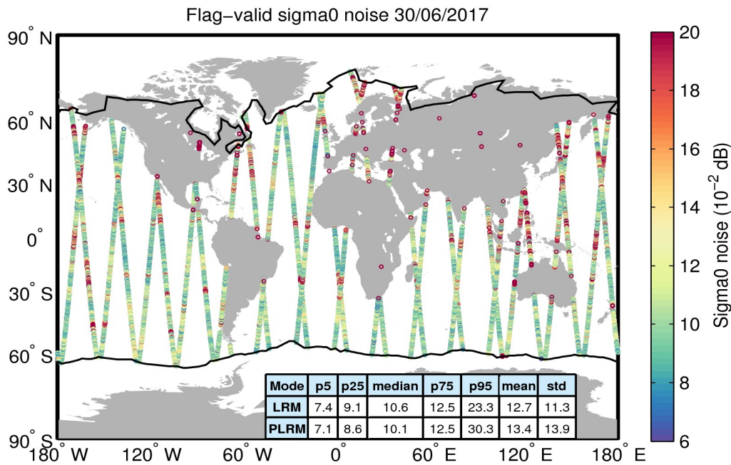
Figure 26. Geographical distribution of flag-valid 20-Hz sigma0 measurement noise over oceans and lakes for 30/06/2017. The statistical values shown in the table refer to the sigma0 noise and are calculated separately for LRM and PLRM regions. Measurements taken over polar polygons have been excluded from the computation of the statistical values. The black lines mark the outer limit of the Arctic and Antarctic polar polygons.
