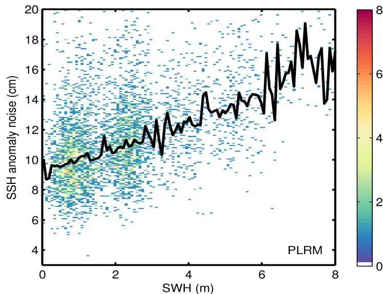
Figure 9. 2D histogram showing flag-valid SSH anomaly noise as a function of SWH for LRM (top) and PLRM (bottom) for 30/06/2017. The black line denotes the median SSH anomaly noise as a function of SWH.
