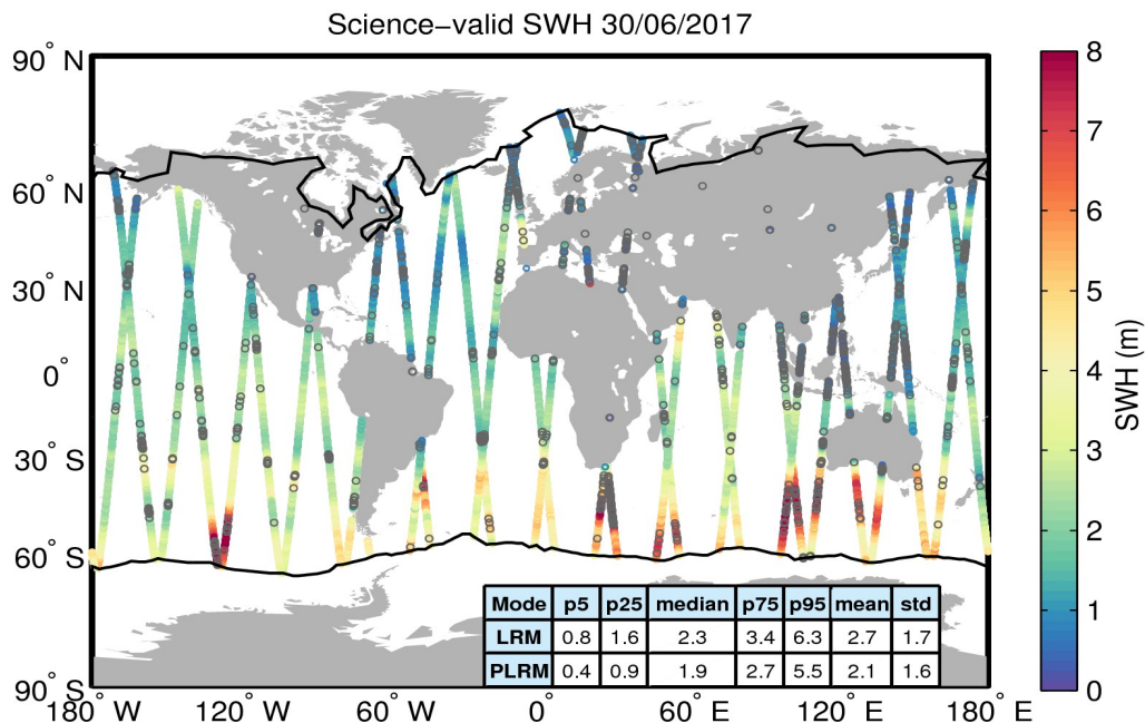
Figure 19. Geographical distribution of science-valid SWH data over oceans and lakes for 30/06/2017. The statistical values shown in the table refer to the SWH in m and are calculated separately for LRM and PLRM regions. The black lines mark the outer limit of the Arctic and Antarctic polar polygons. Gray circles denote records that have been rejected based on the editing criteria described in Table 3.
