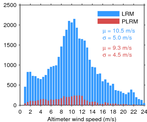
Figure 35. Histogram of science-valid wind over oceans and lakes for LRM (blue) and PLRM (red) for 30/06/2017. The mean ( \mu ) and standard deviation ( \sigma ) are also shown. Note that values larger than 24 m/s are excluded from the histogram for the sake of readability but not from the computation of \mu and \sigma .
