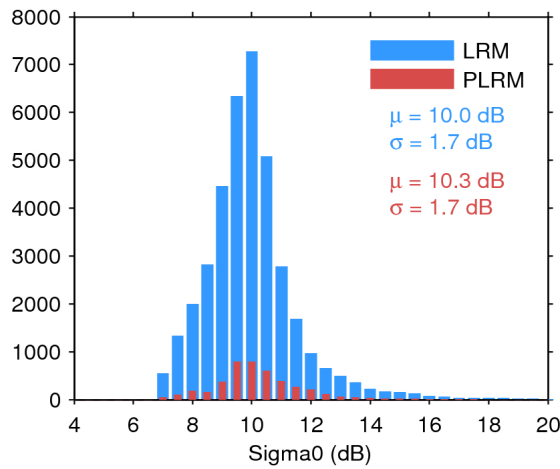
Figure 28. Histogram of science-valid sigma0 over oceans and lakes for LRM (blue) and PLRM (red) for 30/06/2017. The mean ( \mu ) and standard deviation ( \sigma ) are also shown. Note that values outside [4 20] dB are excluded from the histogram for the sake of readability but not from the computation of \mu and \sigma .
