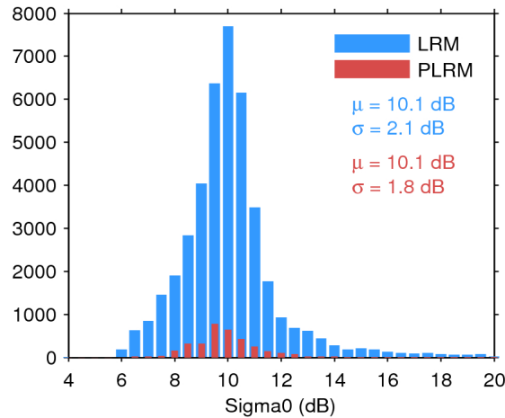
Figure 25. Histogram of flag-valid sigma0 over oceans and lakes for LRM (blue) and PLRM (red) for 29/06/2017. The mean ( \mu ) and standard deviation ( \sigma ) are also shown. Note that values outside [4 20] dB are excluded from the histogram for the sake of readability but not from the computation of \mu and \sigma .
