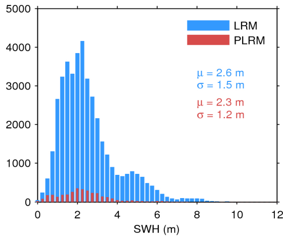
Figure 20. Histogram of science-valid SWH over oceans and lakes for LRM (blue) and PLRM (red) for 29/06/2017. The mean ( \mu ) and standard deviation ( \sigma ) are also shown. Note that values larger than 12 m are excluded from the histogram for the sake of readability but not from the computation of \mu and \sigma .
