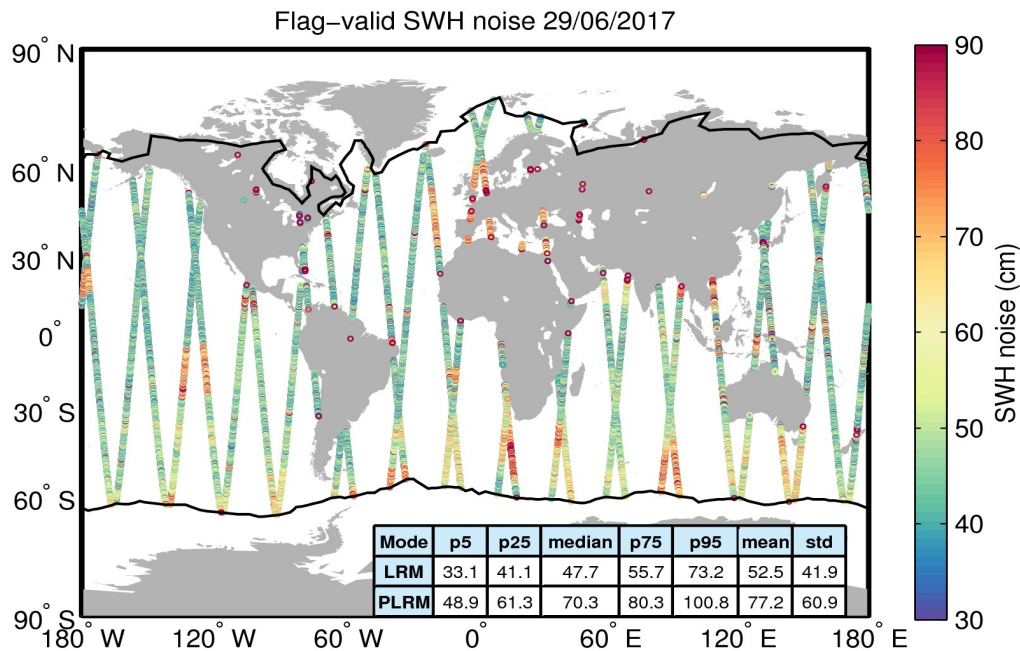
Figure 18. Geographical distribution of flag-valid 20-Hz SWH measurement noise over oceans and lakes for 29/06/2017. The statistical values shown in the table refer to the SWH noise and are calculated separately for LRM and PLRM regions. Measurements taken over polar polygons have been excluded from the computation of the statistical values. The black lines mark the outer limit of the Arctic and Antarctic polar polygons.
