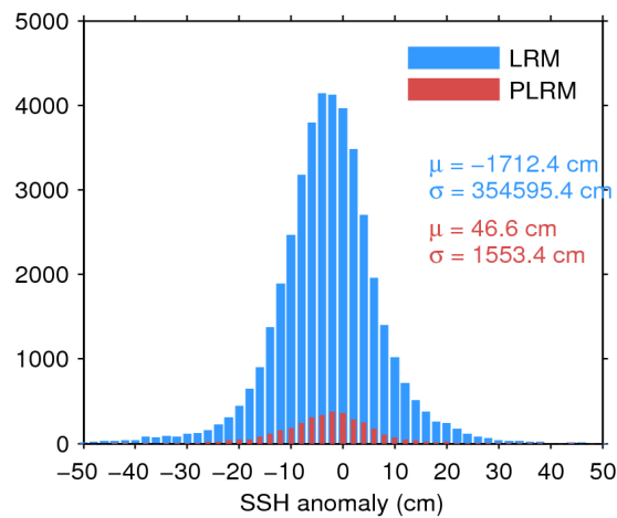
Figure 7. Histogram of flag-valid SSH anomaly over oceans and lakes for LRM (blue) and PLRM (red) for 29/06/2017. The mean ( \mu ) and standard deviation ( \sigma ) are also shown. Note that values outside [-50\ 50] cm are excluded from the histogram for the sake of readability but not from the computation of \mu and \sigma .
