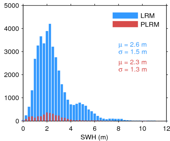
Figure 17. Histogram of flag-valid SWH over oceans and lakes for LRM (blue) and PLRM (red) for 29/06/2017. The mean ( \mu ) and standard deviation ( \sigma ) are also shown. Note that values larger than 12 m are excluded from the histogram for the sake of readability but not from the computation of \mu and \sigma .
