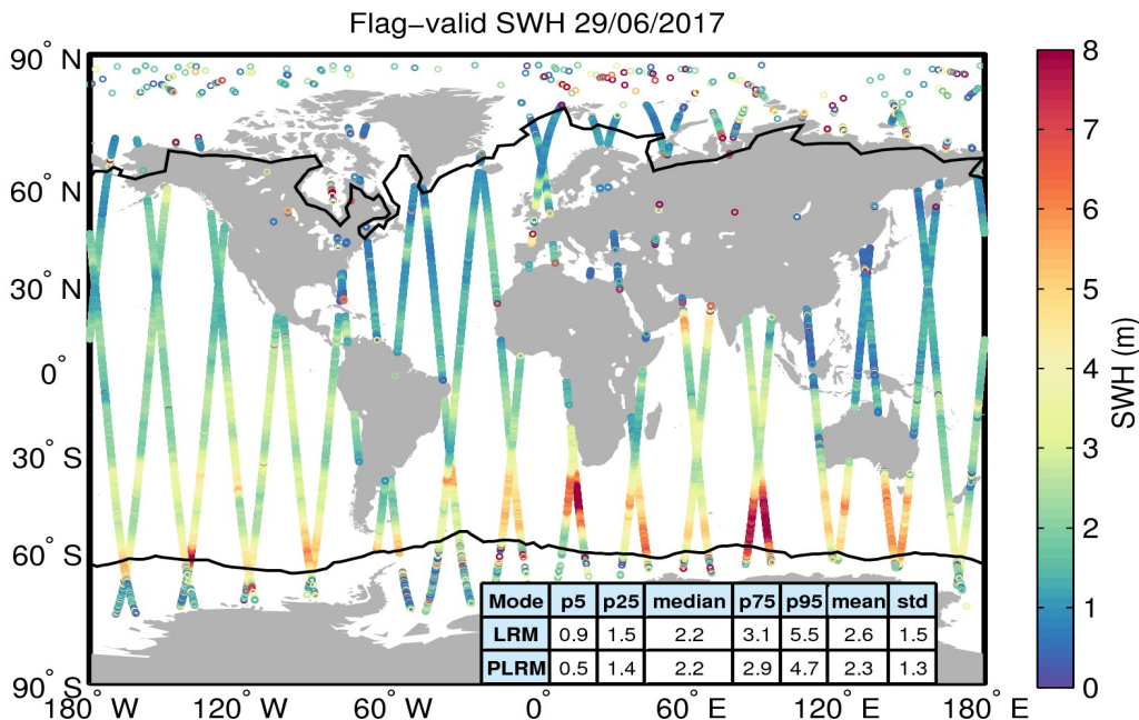
Figure 15. Geographical distribution of flag-valid SWH data over oceans and lakes for 29/06/2017. The statistical values shown in the table refer to the SWH in m and are calculated separately for LRM and PLRM regions. Measurements taken over polar polygons have been excluded from the computation of the statistical values. The black lines mark the outer limit of the Arctic and Antarctic polar polygons.
