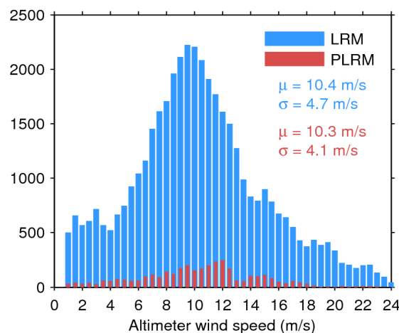
Figure 35. Histogram of science-valid wind over oceans and lakes for LRM (blue) and PLRM (red) for 29/06/2017. The mean ( \mu ) and standard deviation ( \sigma ) are also shown. Note that values larger than 24 m/s are excluded from the histogram for the sake of readability but not from the computation of \mu and \sigma .
