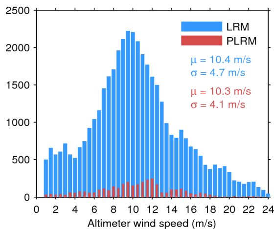
Figure 33. Histogram of flag-valid wind over oceans and lakes for LRM (blue) and PLRM (red) for 29/06/2017. The mean ( \mu ) and standard deviation ( \sigma ) are also shown. Note that values larger than 24 m/s are excluded from the histogram for the sake of readability but not from the computation of \mu and \sigma .
