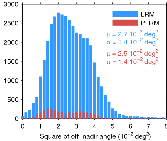
Figure 39. Histogram of flag-valid mispointing over oceans and lakes for LRM (blue) and PLRM (red) for 29/06/2017. Only positive values have been considered. The mean ( \mu ) and standard deviation ( \sigma ) are also shown. Note that values larger than 8 \cdot 10^{-2} \text{ deg}^2 are excluded from the histogram for the sake of readability but not from the computation of \mu and \sigma .
