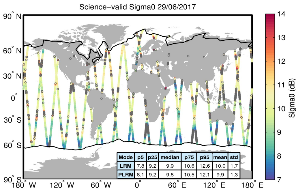
Figure 27. Geographical distribution of science-valid sigma0 data over oceans and lakes for 29/06/2017. The statistical values shown in the table refer to the sigma0 in dB and are calculated separately for LRM and PLRM regions. The black lines mark the outer limit of the Arctic and Antarctic polar polygons. Gray circles denote records that have been rejected based on the editing criteria described in Table 4.
