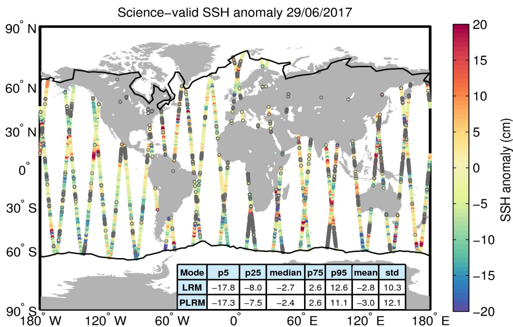
Figure 10. Geographical distribution of science-valid SSH anomaly data over oceans and lakes for 29/06/2017. The statistical values shown in the table refer to the SSH anomaly in cm and are calculated separately for LRM and PLRM regions. The black lines mark the outer limit of the Arctic and Antarctic polar polygons. Gray circles denote records that have been rejected based on the editing criteria described in Table 2.
