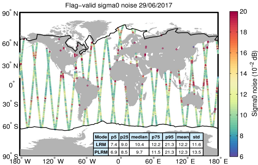
Figure 26. Geographical distribution of flag-valid 20-Hz sigma0 measurement noise over oceans and lakes for 29/06/2017. The statistical values shown in the table refer to the sigma0 noise and are calculated separately for LRM and PLRM regions. Measurements taken over polar polygons have been excluded from the computation of the statistical values. The black lines mark the outer limit of the Arctic and Antarctic polar polygons.
