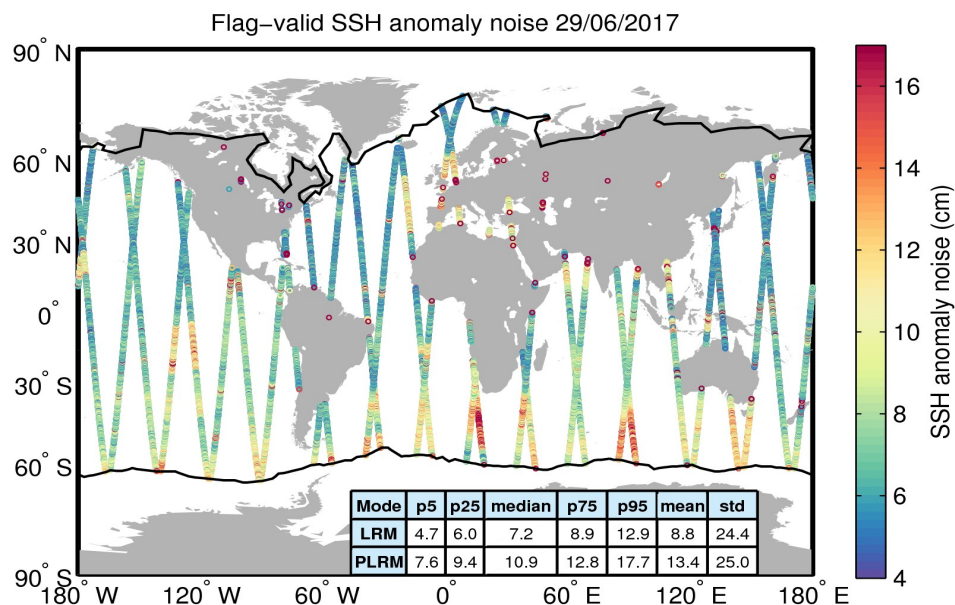
Figure 8. Geographical distribution of flag-valid 20-Hz SSH anomaly measurement noise over oceans and lakes for 29/06/2017. The statistical values shown in the table refer to the SSH anomaly noise and are calculated separately for LRM and PLRM regions. Measurements taken over polar polygons have been excluded from the computation of the statistical values. The black lines mark the outer limit of the Arctic and Antarctic polar polygons.
