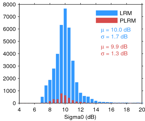
Figure 28. Histogram of science-valid sigma0 over oceans and lakes for LRM (blue) and PLRM (red) for 29/06/2017. The mean ( \mu ) and standard deviation ( \sigma ) are also shown. Note that values outside [4 20] dB are excluded from the histogram for the sake of readability but not from the computation of \mu and \sigma .
