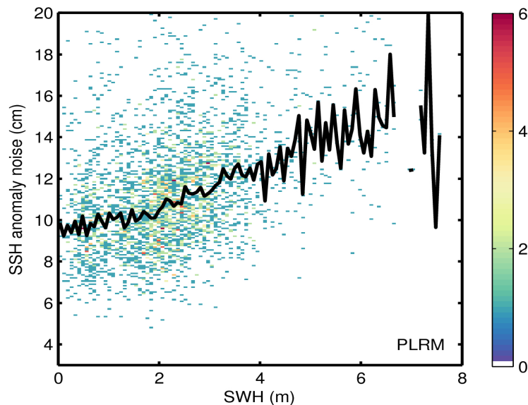
Figure 9. 2D histogram showing flag-valid SSH anomaly noise as a function of SWH for LRM (top) and PLRM (bottom) for 29/06/2017. The black line denotes the median SSH anomaly noise as a function of SWH.
