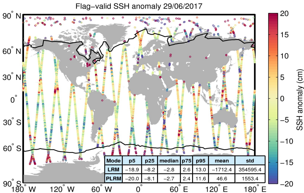
Figure 5. Geographical distribution of flag-valid 1-Hz SSH anomaly data over oceans and lakes for 29/06/2017. The statistical values shown in the table refer to the SSH anomaly in cm and are calculated separately for LRM and PLRM regions. Measurements taken over polar polygons have been excluded from the computation of the statistical values. The black lines mark the outer limit of the Arctic and Antarctic polar polygons.
