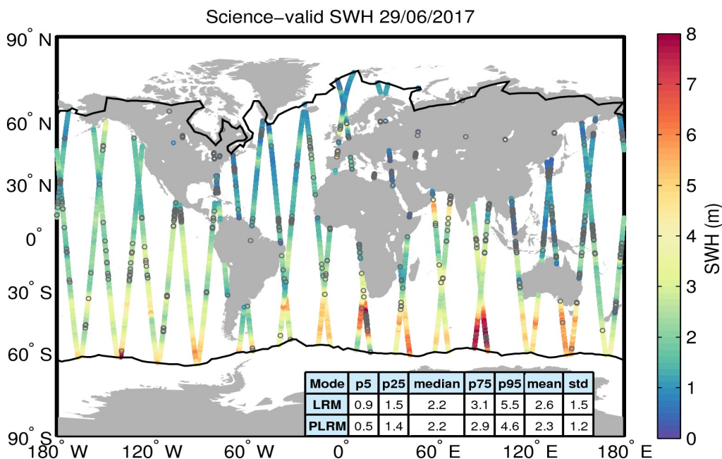
Figure 19. Geographical distribution of science-valid SWH data over oceans and lakes for 29/06/2017. The statistical values shown in the table refer to the SWH in m and are calculated separately for LRM and PLRM regions. The black lines mark the outer limit of the Arctic and Antarctic polar polygons. Gray circles denote records that have been rejected based on the editing criteria described in Table 3.
