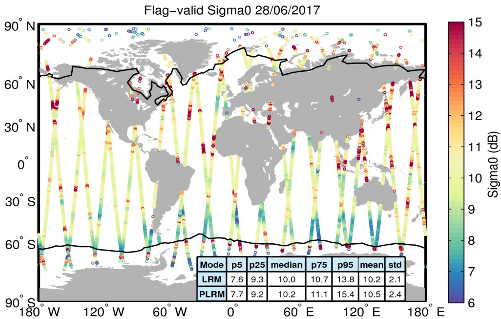
Figure 23. Geographical distribution of flag-valid sigma0 data over oceans and lakes for 28/06/2017. The statistical values shown in the table refer to the sigma0 in dB and are calculated separately for LRM and PLRM regions. Measurements taken over polar polygons have been excluded from the computation of the statistical values. The black lines mark the outer limit of the Arctic and Antarctic polar polygons.
