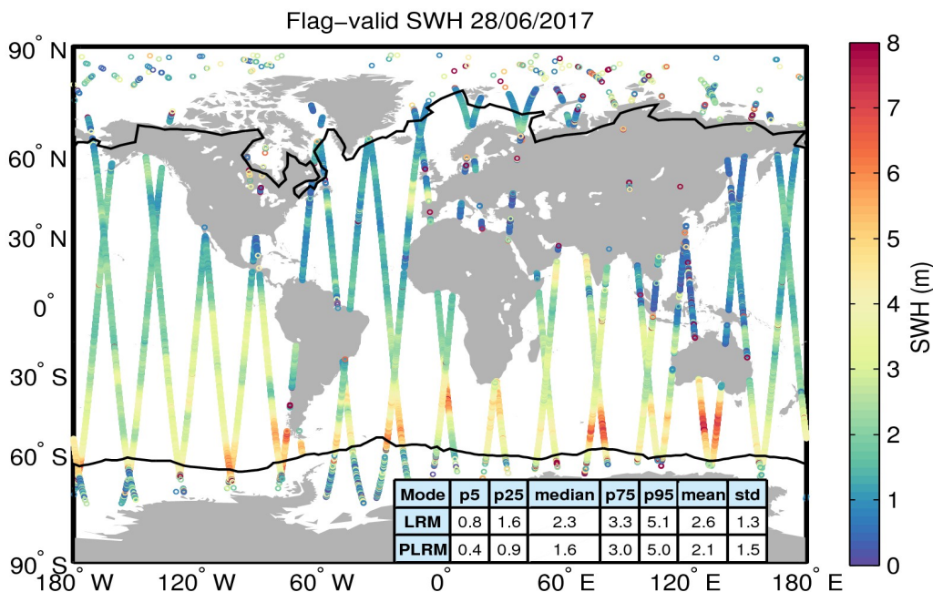
Figure 15. Geographical distribution of flag-valid SWH data over oceans and lakes for 28/06/2017. The statistical values shown in the table refer to the SWH in m and are calculated separately for LRM and PLRM regions. Measurements taken over polar polygons have been excluded from the computation of the statistical values. The black lines mark the outer limit of the Arctic and Antarctic polar polygons.
