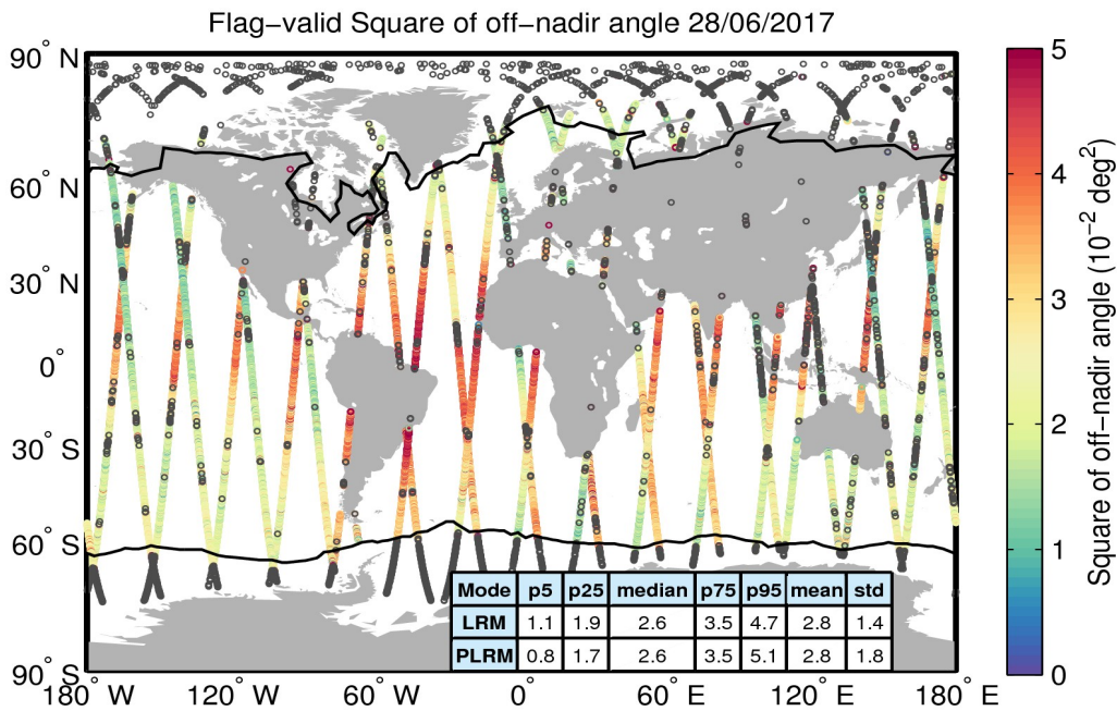
Figure 37. Geographical distribution of flag-valid mispointing data over oceans and lakes for 28/06/2017. The statistical values shown in the table refer to the mispointing in 10^{-2} deg 2 and are calculated separately for LRM and PLRM regions. Measurements taken over polar polygons have been excluded from the computation of the statistical values. The black lines mark the outer limit of the Arctic and Antarctic polar polygons. Gray circles denote negative values.
