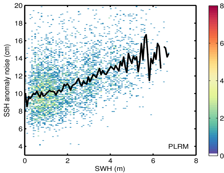
Figure 9. 2D histogram showing flag-valid SSH anomaly noise as a function of SWH for LRM (top) and PLRM (bottom) for 28/06/2017. The black line denotes the median SSH anomaly noise as a function of SWH.
