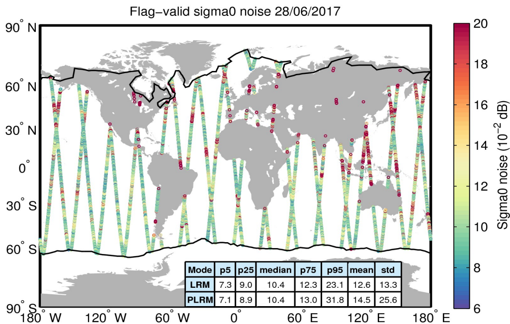
Figure 26. Geographical distribution of flag-valid 20-Hz sigma0 measurement noise over oceans and lakes for 28/06/2017. The statistical values shown in the table refer to the sigma0 noise and are calculated separately for LRM and PLRM regions. Measurements taken over polar polygons have been excluded from the computation of the statistical values. The black lines mark the outer limit of the Arctic and Antarctic polar polygons.
