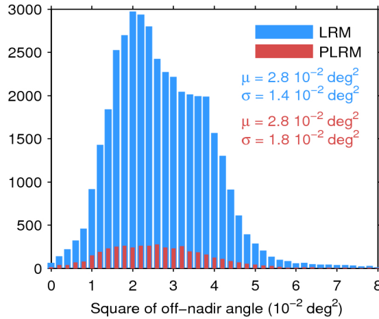
Figure 39. Histogram of flag-valid mispointing over oceans and lakes for LRM (blue) and PLRM (red) for 28/06/2017. Only positive values have been considered. The mean ( \mu ) and standard deviation ( \sigma ) are also shown. Note that values larger than 8 \cdot 10^{-2} \text{ deg}^2 are excluded from the histogram for the sake of readability but not from the computation of \mu and \sigma .
