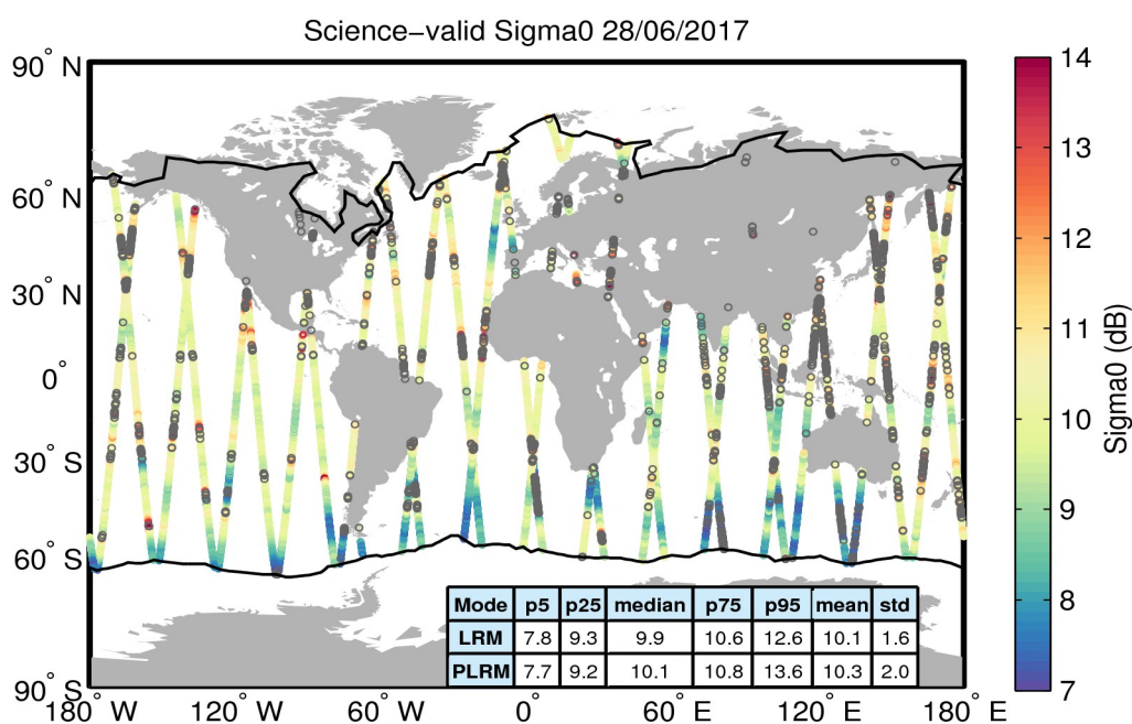
Figure 27. Geographical distribution of science-valid sigma0 data over oceans and lakes for 28/06/2017. The statistical values shown in the table refer to the sigma0 in dB and are calculated separately for LRM and PLRM regions. The black lines mark the outer limit of the Arctic and Antarctic polar polygons. Gray circles denote records that have been rejected based on the editing criteria described in Table 4.
