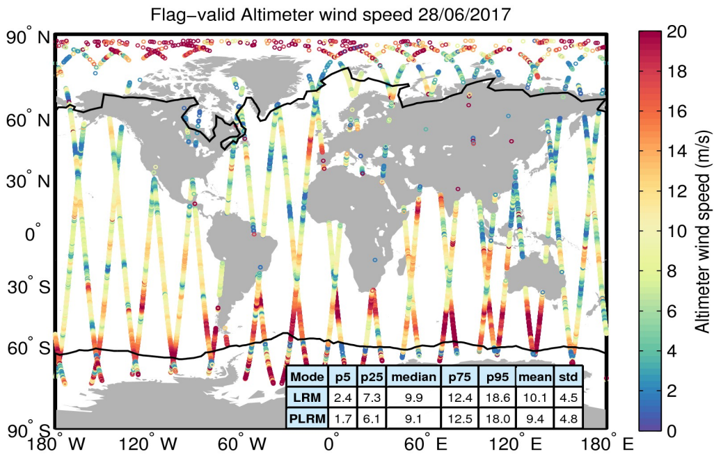
Figure 31. Geographical distribution of flag-valid wind data over oceans and lakes for 28/06/2017. The statistical values shown in the table refer to the wind in m/s and are calculated separately for LRM and PLRM regions. Measurements taken over polar polygons have been excluded from the computation of the statistical values. The black lines mark the outer limit of the Arctic and Antarctic polar polygons.
