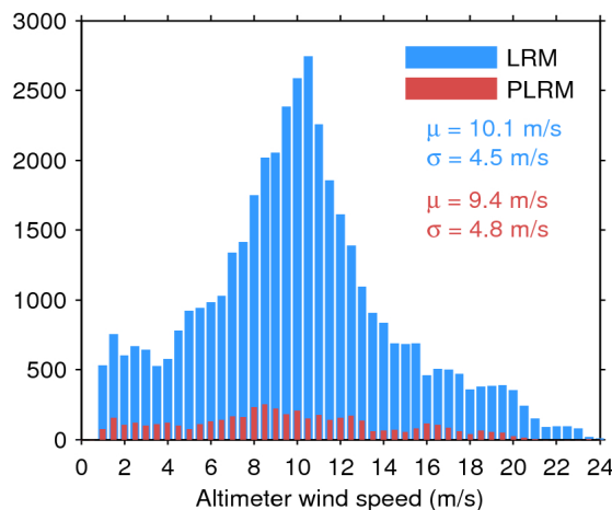
Figure 35. Histogram of science-valid wind over oceans and lakes for LRM (blue) and PLRM (red) for 28/06/2017. The mean ( \mu ) and standard deviation ( \sigma ) are also shown. Note that values larger than 24 m/s are excluded from the histogram for the sake of readability but not from the computation of \mu and \sigma .
