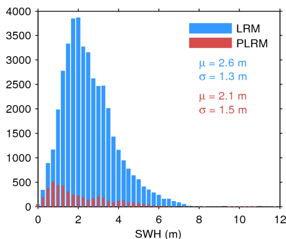
Figure 17. Histogram of flag-valid SWH over oceans and lakes for LRM (blue) and PLRM (red) for 28/06/2017. The mean ( \mu ) and standard deviation ( \sigma ) are also shown. Note that values larger than 12 m are excluded from the histogram for the sake of readability but not from the computation of \mu and \sigma .
