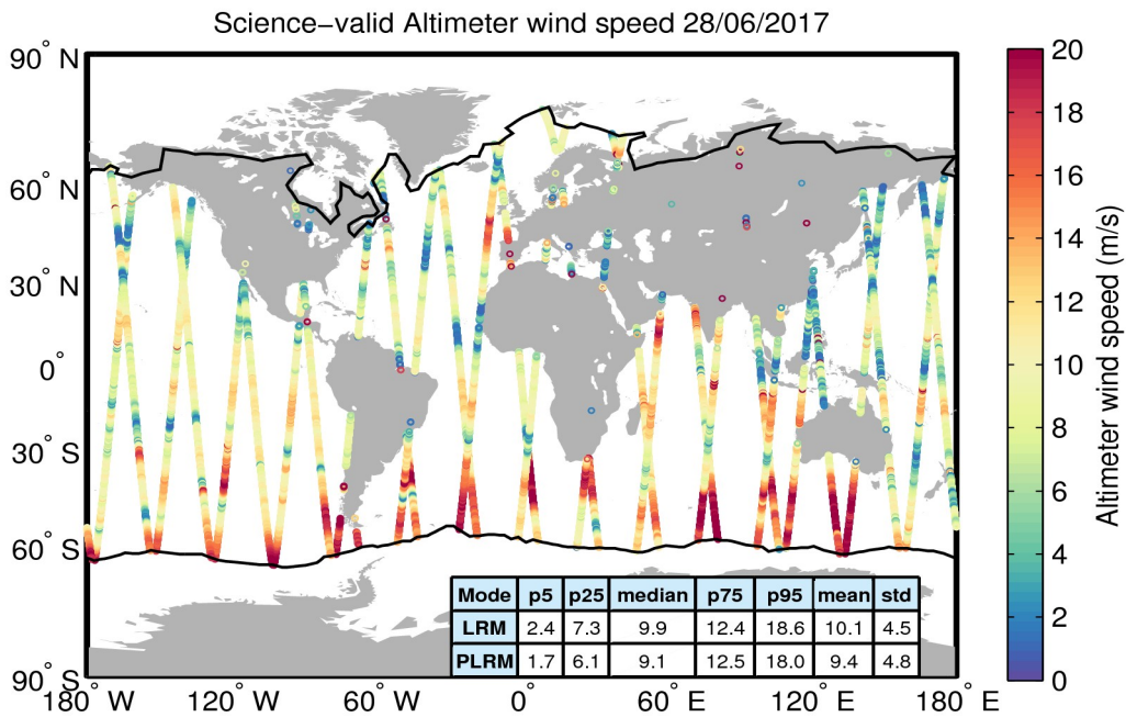
Figure 34. Geographical distribution of science-valid wind data over oceans and lakes for 28/06/2017. The statistical values shown in the table refer to the wind in m/s and are calculated separately for LRM and PLRM regions. The black lines mark the outer limit of the Arctic and Antarctic polar polygons. Gray circles denote records that have been rejected based on the editing criteria described in Table 5.
