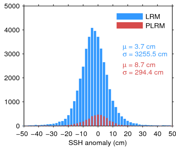
Figure 7. Histogram of flag-valid SSH anomaly over oceans and lakes for LRM (blue) and PLRM (red) for 28/06/2017. The mean ( \mu ) and standard deviation ( \sigma ) are also shown. Note that values outside [-50\ 50] cm are excluded from the histogram for the sake of readability but not from the computation of \mu and \sigma .
