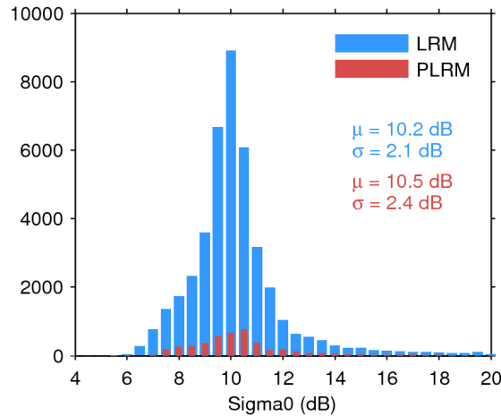
Figure 25. Histogram of flag-valid sigma0 over oceans and lakes for LRM (blue) and PLRM (red) for 28/06/2017. The mean ( \mu ) and standard deviation ( \sigma ) are also shown. Note that values outside [4 20] dB are excluded from the histogram for the sake of readability but not from the computation of \mu and \sigma .
