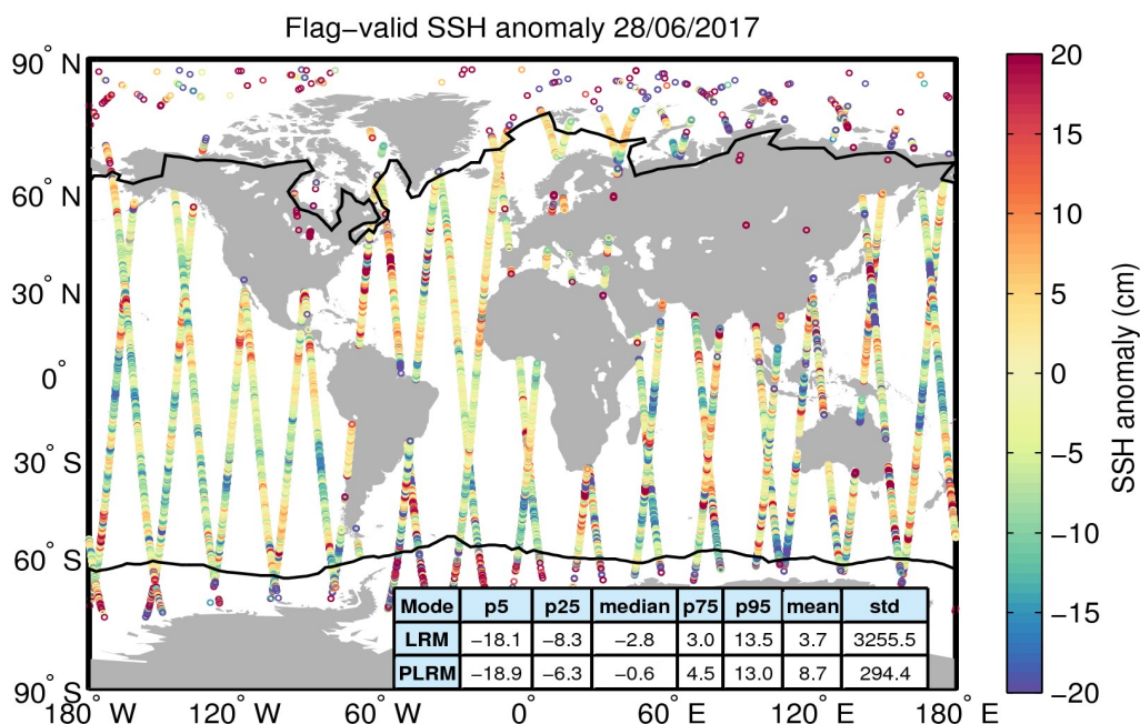
Figure 5. Geographical distribution of flag-valid 1-Hz SSH anomaly data over oceans and lakes for 28/06/2017. The statistical values shown in the table refer to the SSH anomaly in cm and are calculated separately for LRM and PLRM regions. Measurements taken over polar polygons have been excluded from the computation of the statistical values. The black lines mark the outer limit of the Arctic and Antarctic polar polygons.
