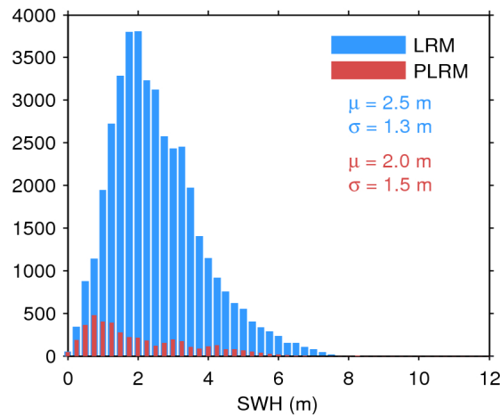
Figure 20. Histogram of science-valid SWH over oceans and lakes for LRM (blue) and PLRM (red) for 28/06/2017. The mean ( \mu ) and standard deviation ( \sigma ) are also shown. Note that values larger than 12 m are excluded from the histogram for the sake of readability but not from the computation of \mu and \sigma .
