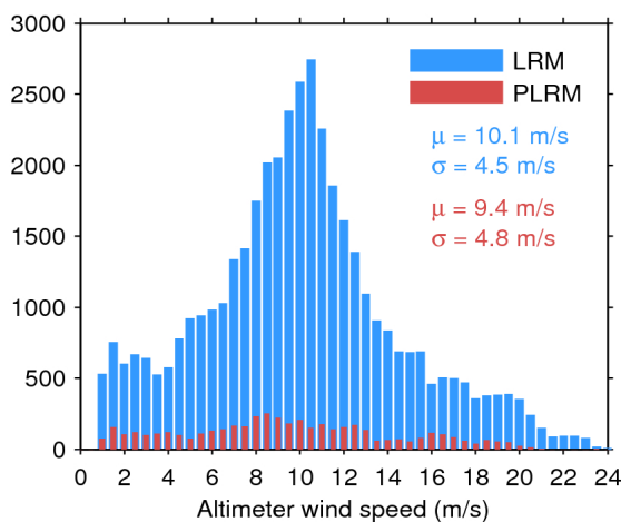
Figure 33. Histogram of flag-valid wind over oceans and lakes for LRM (blue) and PLRM (red) for 28/06/2017. The mean ( \mu ) and standard deviation ( \sigma ) are also shown. Note that values larger than 24 m/s are excluded from the histogram for the sake of readability but not from the computation of \mu and \sigma .
