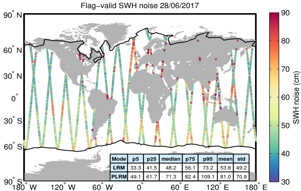
Figure 18. Geographical distribution of flag-valid 20-Hz SWH measurement noise over oceans and lakes for 28/06/2017. The statistical values shown in the table refer to the SWH noise and are calculated separately for LRM and PLRM regions. Measurements taken over polar polygons have been excluded from the computation of the statistical values. The black lines mark the outer limit of the Arctic and Antarctic polar polygons.
