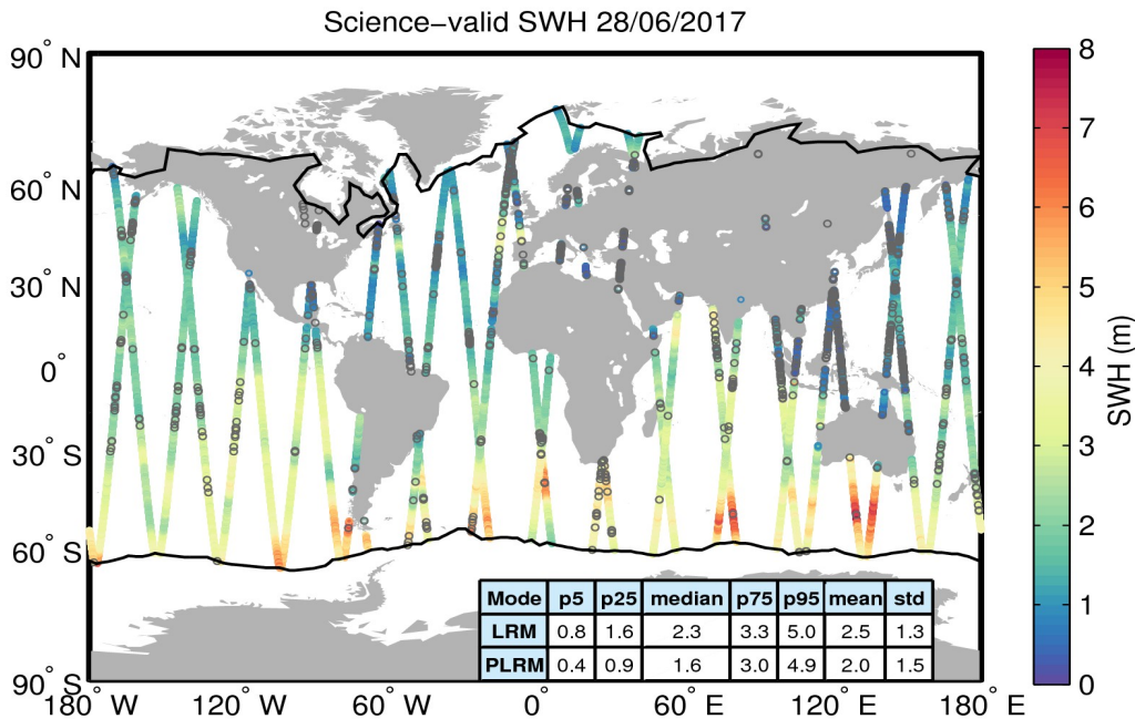
Figure 19. Geographical distribution of science-valid SWH data over oceans and lakes for 28/06/2017. The statistical values shown in the table refer to the SWH in m and are calculated separately for LRM and PLRM regions. The black lines mark the outer limit of the Arctic and Antarctic polar polygons. Gray circles denote records that have been rejected based on the editing criteria described in Table 3.
