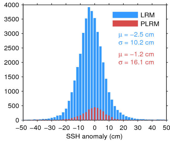
Figure 11. Histogram of science-valid SSH anomaly over oceans and lakes for LRM (blue) and PLRM (red) for 28/06/2017. The mean ( \mu ) and standard deviation ( \sigma ) are also shown. Note that values outside [-50 50] cm are excluded from the histogram for the sake of readability but not from the computation of \mu and \sigma .
