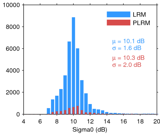
Figure 28. Histogram of science-valid sigma0 over oceans and lakes for LRM (blue) and PLRM (red) for 28/06/2017. The mean ( \mu ) and standard deviation ( \sigma ) are also shown. Note that values outside [4 20] dB are excluded from the histogram for the sake of readability but not from the computation of \mu and \sigma .
