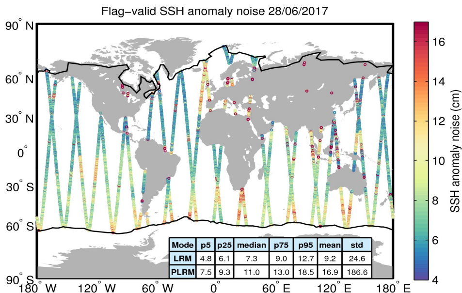
Figure 8. Geographical distribution of flag-valid 20-Hz SSH anomaly measurement noise over oceans and lakes for 28/06/2017. The statistical values shown in the table refer to the SSH anomaly noise and are calculated separately for LRM and PLRM regions. Measurements taken over polar polygons have been excluded from the computation of the statistical values. The black lines mark the outer limit of the Arctic and Antarctic polar polygons.
