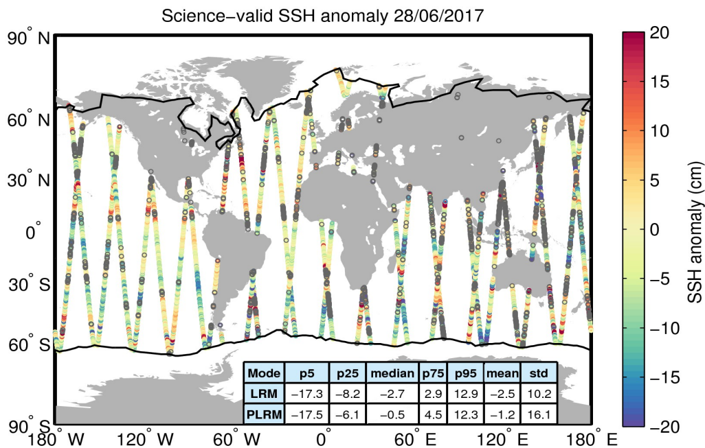
Figure 10. Geographical distribution of science-valid SSH anomaly data over oceans and lakes for 28/06/2017. The statistical values shown in the table refer to the SSH anomaly in cm and are calculated separately for LRM and PLRM regions. The black lines mark the outer limit of the Arctic and Antarctic polar polygons. Gray circles denote records that have been rejected based on the editing criteria described in Table 2.
