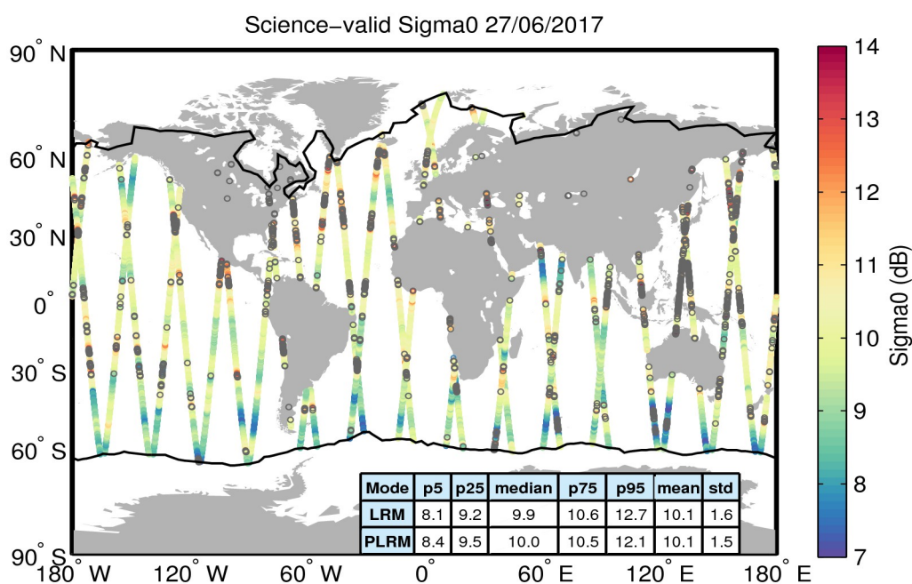
Figure 27. Geographical distribution of science-valid sigma0 data over oceans and lakes for 27/06/2017. The statistical values shown in the table refer to the sigma0 in dB and are calculated separately for LRM and PLRM regions. The black lines mark the outer limit of the Arctic and Antarctic polar polygons. Gray circles denote records that have been rejected based on the editing criteria described in Table 4.
