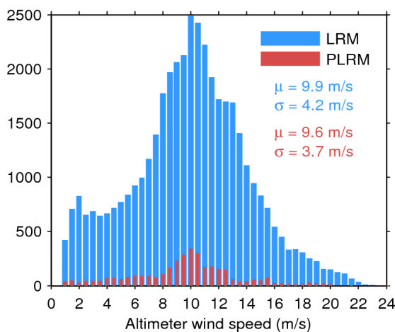
Figure 33. Histogram of flag-valid wind over oceans and lakes for LRM (blue) and PLRM (red) for 27/06/2017. The mean ( \mu ) and standard deviation ( \sigma ) are also shown. Note that values larger than 24 m/s are excluded from the histogram for the sake of readability but not from the computation of \mu and \sigma .
