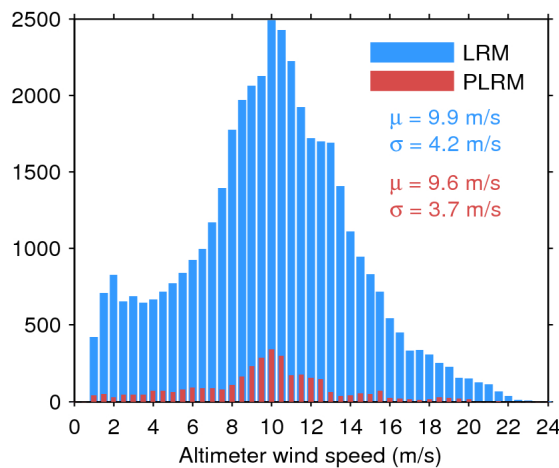
Figure 35. Histogram of science-valid wind over oceans and lakes for LRM (blue) and PLRM (red) for 27/06/2017. The mean ( \mu ) and standard deviation ( \sigma ) are also shown. Note that values larger than 24 m/s are excluded from the histogram for the sake of readability but not from the computation of \mu and \sigma .
