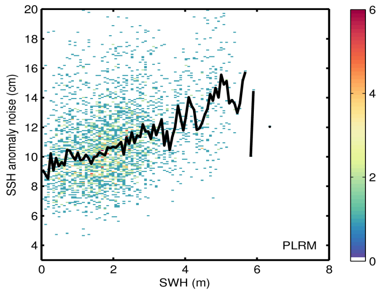
Figure 9. 2D histogram showing flag-valid SSH anomaly noise as a function of SWH for LRM (top) and PLRM (bottom) for 27/06/2017. The black line denotes the median SSH anomaly noise as a function of SWH.
