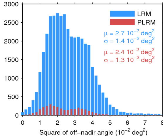
Figure 39. Histogram of flag-valid mispointing over oceans and lakes for LRM (blue) and PLRM (red) for 27/06/2017. Only positive values have been considered. The mean ( \mu ) and standard deviation ( \sigma ) are also shown. Note that values larger than 8 \cdot 10^{-2} \text{ deg}^2 are excluded from the histogram for the sake of readability but not from the computation of \mu and \sigma .
