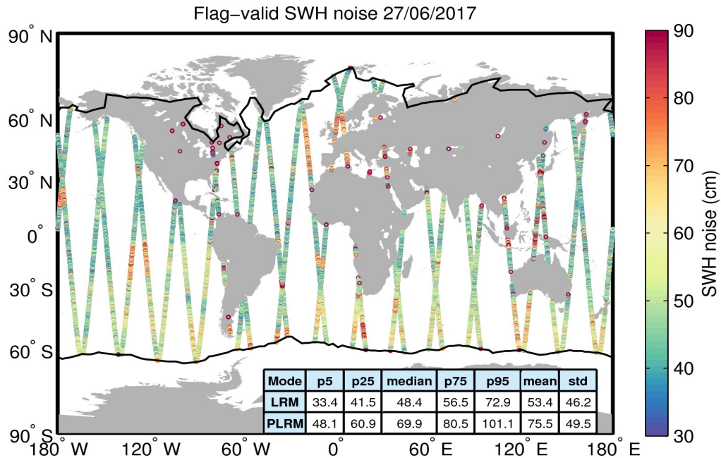
Figure 18. Geographical distribution of flag-valid 20-Hz SWH measurement noise over oceans and lakes for 27/06/2017. The statistical values shown in the table refer to the SWH noise and are calculated separately for LRM and PLRM regions. Measurements taken over polar polygons have been excluded from the computation of the statistical values. The black lines mark the outer limit of the Arctic and Antarctic polar polygons.
