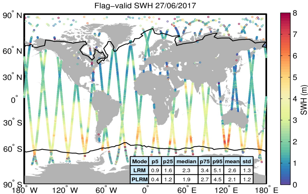
Figure 15. Geographical distribution of flag-valid SWH data over oceans and lakes for 27/06/2017. The statistical values shown in the table refer to the SWH in m and are calculated separately for LRM and PLRM regions. Measurements taken over polar polygons have been excluded from the computation of the statistical values. The black lines mark the outer limit of the Arctic and Antarctic polar polygons.
