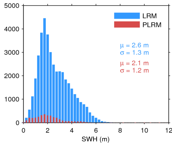
Figure 17. Histogram of flag-valid SWH over oceans and lakes for LRM (blue) and PLRM (red) for 27/06/2017. The mean ( \mu ) and standard deviation ( \sigma ) are also shown. Note that values larger than 12 m are excluded from the histogram for the sake of readability but not from the computation of \mu and \sigma .
