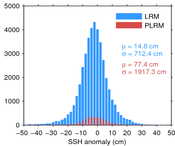
Figure 7. Histogram of flag-valid SSH anomaly over oceans and lakes for LRM (blue) and PLRM (red) for 27/06/2017. The mean ( \mu ) and standard deviation ( \sigma ) are also shown. Note that values outside [-50\ 50] cm are excluded from the histogram for the sake of readability but not from the computation of \mu and \sigma .
