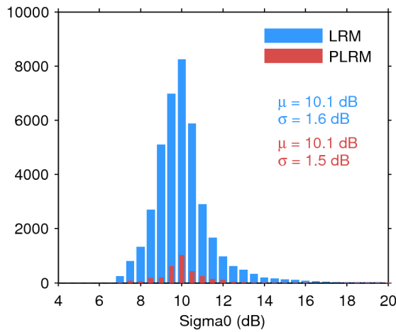
Figure 28. Histogram of science-valid sigma0 over oceans and lakes for LRM (blue) and PLRM (red) for 27/06/2017. The mean ( \mu ) and standard deviation ( \sigma ) are also shown. Note that values outside [4 20] dB are excluded from the histogram for the sake of readability but not from the computation of \mu and \sigma .
