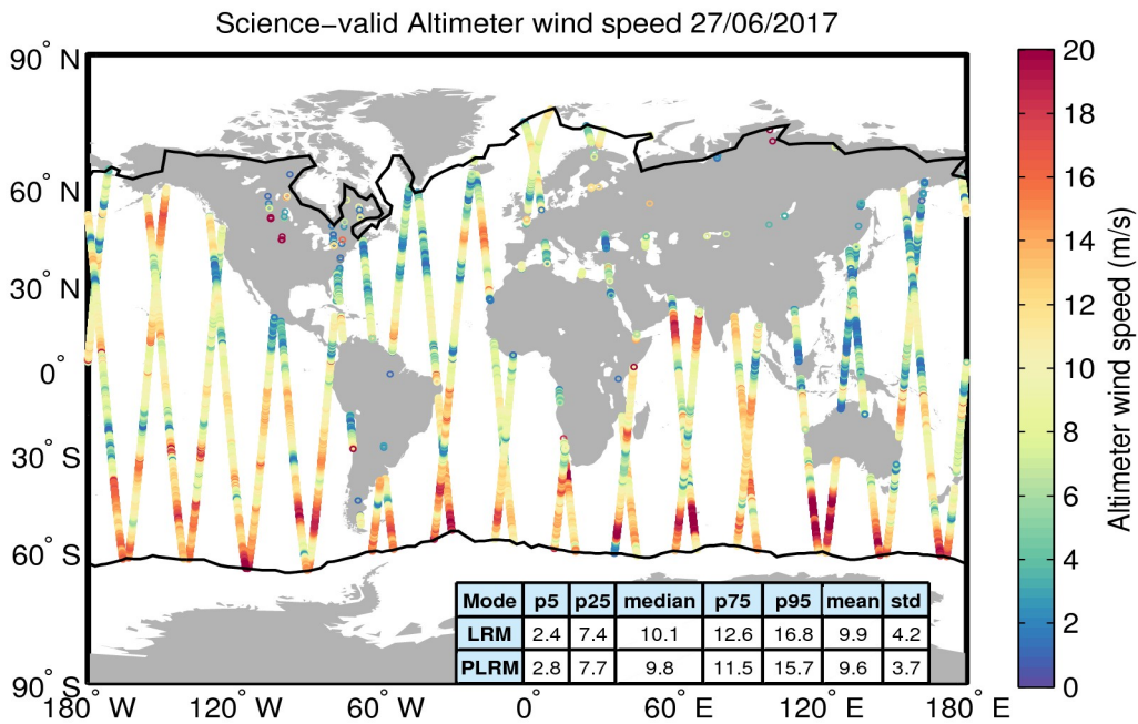
Figure 34. Geographical distribution of science-valid wind data over oceans and lakes for 27/06/2017. The statistical values shown in the table refer to the wind in m/s and are calculated separately for LRM and PLRM regions. The black lines mark the outer limit of the Arctic and Antarctic polar polygons. Gray circles denote records that have been rejected based on the editing criteria described in Table 5.
