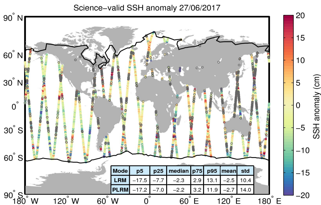
Figure 10. Geographical distribution of science-valid SSH anomaly data over oceans and lakes for 27/06/2017. The statistical values shown in the table refer to the SSH anomaly in cm and are calculated separately for LRM and PLRM regions. The black lines mark the outer limit of the Arctic and Antarctic polar polygons. Gray circles denote records that have been rejected based on the editing criteria described in Table 2.
