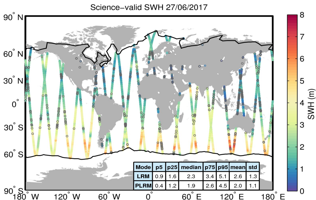
Figure 19. Geographical distribution of science-valid SWH data over oceans and lakes for 27/06/2017. The statistical values shown in the table refer to the SWH in m and are calculated separately for LRM and PLRM regions. The black lines mark the outer limit of the Arctic and Antarctic polar polygons. Gray circles denote records that have been rejected based on the editing criteria described in Table 3.
