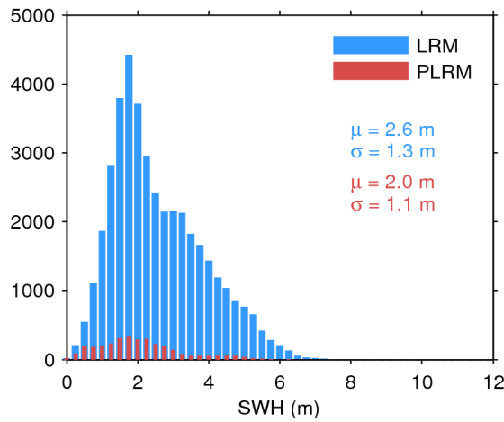
Figure 20. Histogram of science-valid SWH over oceans and lakes for LRM (blue) and PLRM (red) for 27/06/2017. The mean ( \mu ) and standard deviation ( \sigma ) are also shown. Note that values larger than 12 m are excluded from the histogram for the sake of readability but not from the computation of \mu and \sigma .
