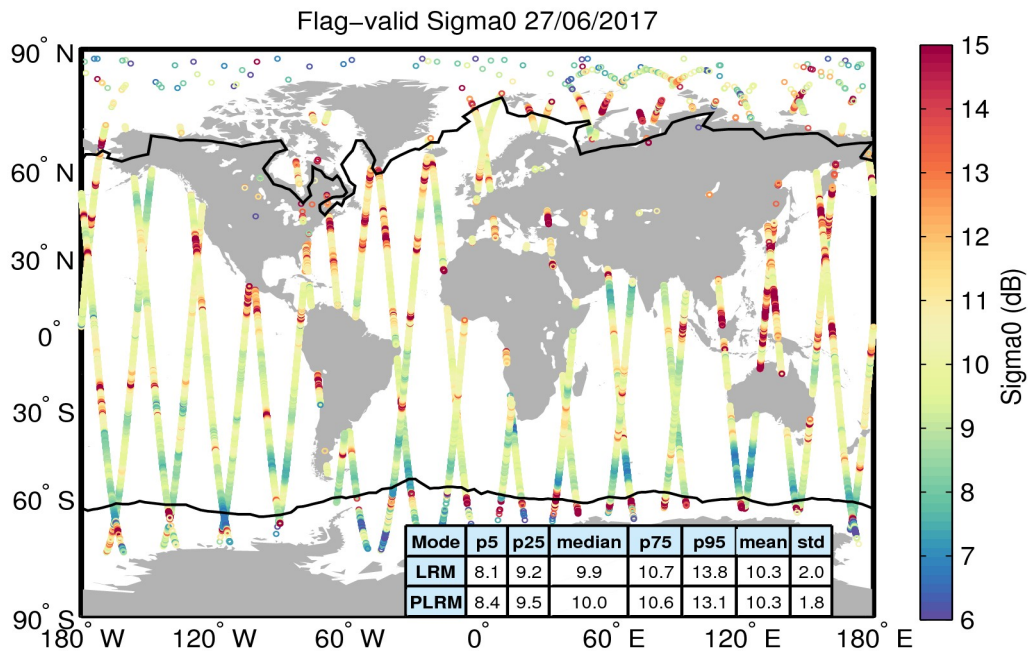
Figure 23. Geographical distribution of flag-valid sigma0 data over oceans and lakes for 27/06/2017. The statistical values shown in the table refer to the sigma0 in dB and are calculated separately for LRM and PLRM regions. Measurements taken over polar polygons have been excluded from the computation of the statistical values. The black lines mark the outer limit of the Arctic and Antarctic polar polygons.
