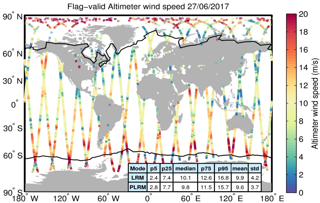
Figure 31. Geographical distribution of flag-valid wind data over oceans and lakes for 27/06/2017. The statistical values shown in the table refer to the wind in m/s and are calculated separately for LRM and PLRM regions. Measurements taken over polar polygons have been excluded from the computation of the statistical values. The black lines mark the outer limit of the Arctic and Antarctic polar polygons.
