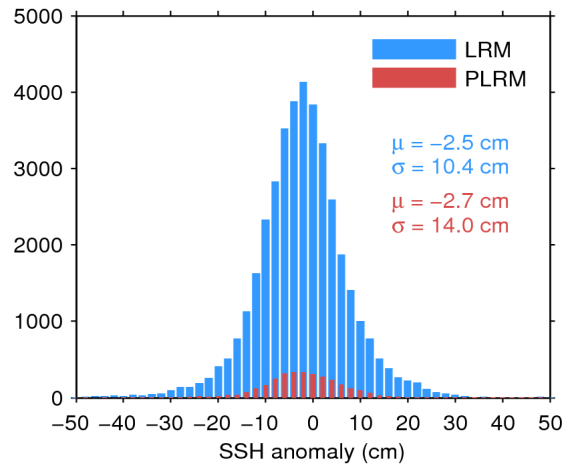
Figure 11. Histogram of science-valid SSH anomaly over oceans and lakes for LRM (blue) and PLRM (red) for 27/06/2017. The mean ( \mu ) and standard deviation ( \sigma ) are also shown. Note that values outside [-50\ 50] cm are excluded from the histogram for the sake of readability but not from the computation of \mu and \sigma .
