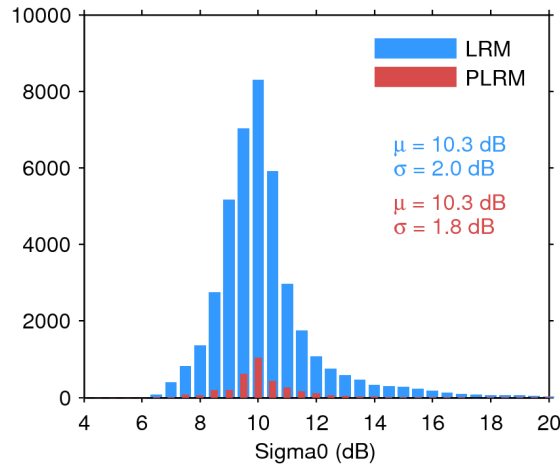
Figure 25. Histogram of flag-valid sigma0 over oceans and lakes for LRM (blue) and PLRM (red) for 27/06/2017. The mean ( \mu ) and standard deviation ( \sigma ) are also shown. Note that values outside [4 20] dB are excluded from the histogram for the sake of readability but not from the computation of \mu and \sigma .
