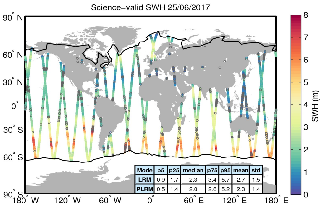
Figure 19. Geographical distribution of science-valid SWH data over oceans and lakes for 25/06/2017. The statistical values shown in the table refer to the SWH in m and are calculated separately for LRM and PLRM regions. The black lines mark the outer limit of the Arctic and Antarctic polar polygons. Gray circles denote records that have been rejected based on the editing criteria described in Table 3.
