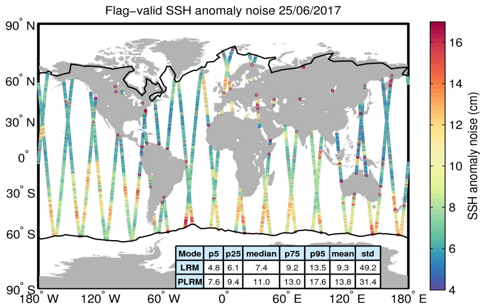
Figure 8. Geographical distribution of flag-valid 20-Hz SSH anomaly measurement noise over oceans and lakes for 25/06/2017. The statistical values shown in the table refer to the SSH anomaly noise and are calculated separately for LRM and PLRM regions. Measurements taken over polar polygons have been excluded from the computation of the statistical values. The black lines mark the outer limit of the Arctic and Antarctic polar polygons.
