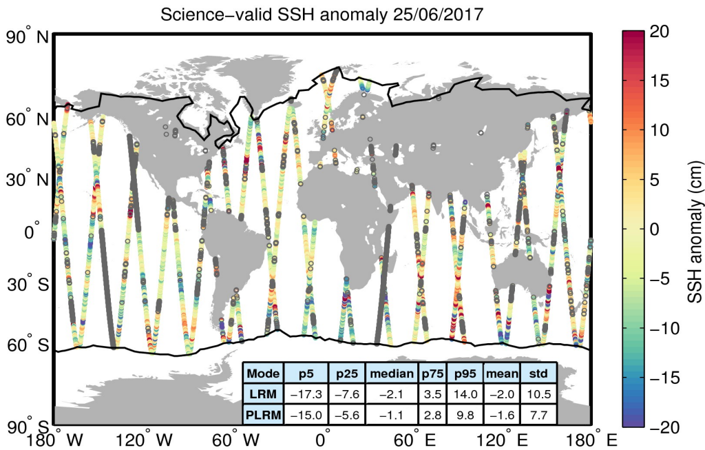
Figure 10. Geographical distribution of science-valid SSH anomaly data over oceans and lakes for 25/06/2017. The statistical values shown in the table refer to the SSH anomaly in cm and are calculated separately for LRM and PLRM regions. The black lines mark the outer limit of the Arctic and Antarctic polar polygons. Gray circles denote records that have been rejected based on the editing criteria described in Table 2.
