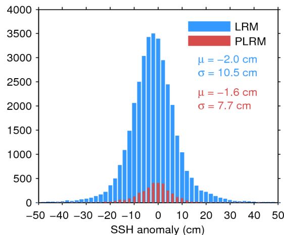
Figure 11. Histogram of science-valid SSH anomaly over oceans and lakes for LRM (blue) and PLRM (red) for 25/06/2017. The mean ( \mu ) and standard deviation ( \sigma ) are also shown. Note that values outside [-50 50] cm are excluded from the histogram for the sake of readability but not from the computation of \mu and \sigma .
