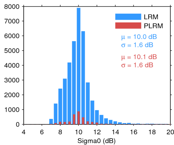
Figure 28. Histogram of science-valid sigma0 over oceans and lakes for LRM (blue) and PLRM (red) for 25/06/2017. The mean ( \mu ) and standard deviation ( \sigma ) are also shown. Note that values outside [4 20] dB are excluded from the histogram for the sake of readability but not from the computation of \mu and \sigma .
