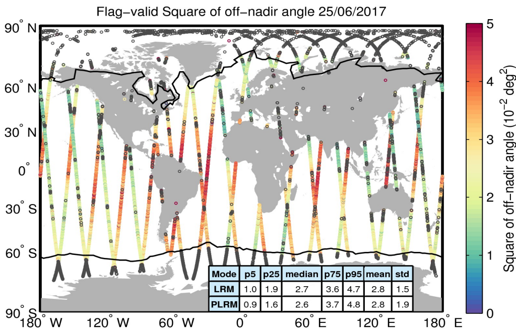
Figure 37. Geographical distribution of flag-valid mispointing data over oceans and lakes for 25/06/2017. The statistical values shown in the table refer to the mispointing in 10^{-2} deg 2 and are calculated separately for LRM and PLRM regions. Measurements taken over polar polygons have been excluded from the computation of the statistical values. The black lines mark the outer limit of the Arctic and Antarctic polar polygons. Gray circles denote negative values.
