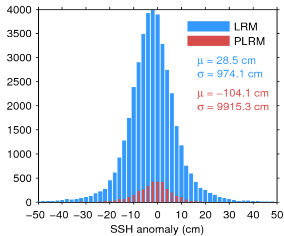
Figure 7. Histogram of flag-valid SSH anomaly over oceans and lakes for LRM (blue) and PLRM (red) for 25/06/2017. The mean ( \mu ) and standard deviation ( \sigma ) are also shown. Note that values outside [-50 50] cm are excluded from the histogram for the sake of readability but not from the computation of \mu and \sigma .
