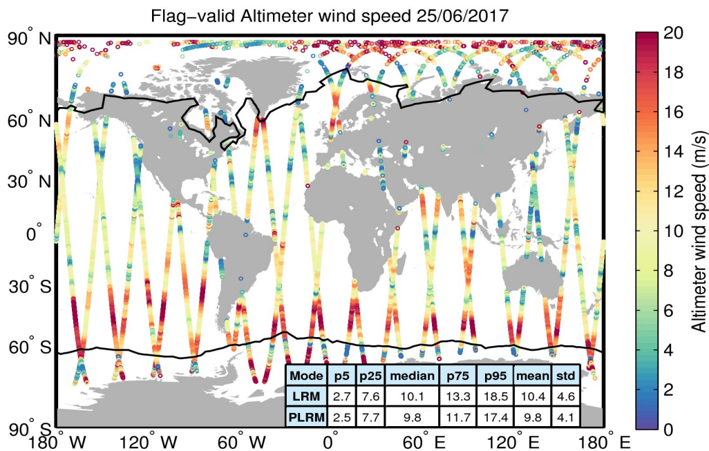
Figure 31. Geographical distribution of flag-valid wind data over oceans and lakes for 25/06/2017. The statistical values shown in the table refer to the wind in m/s and are calculated separately for LRM and PLRM regions. Measurements taken over polar polygons have been excluded from the computation of the statistical values. The black lines mark the outer limit of the Arctic and Antarctic polar polygons.
