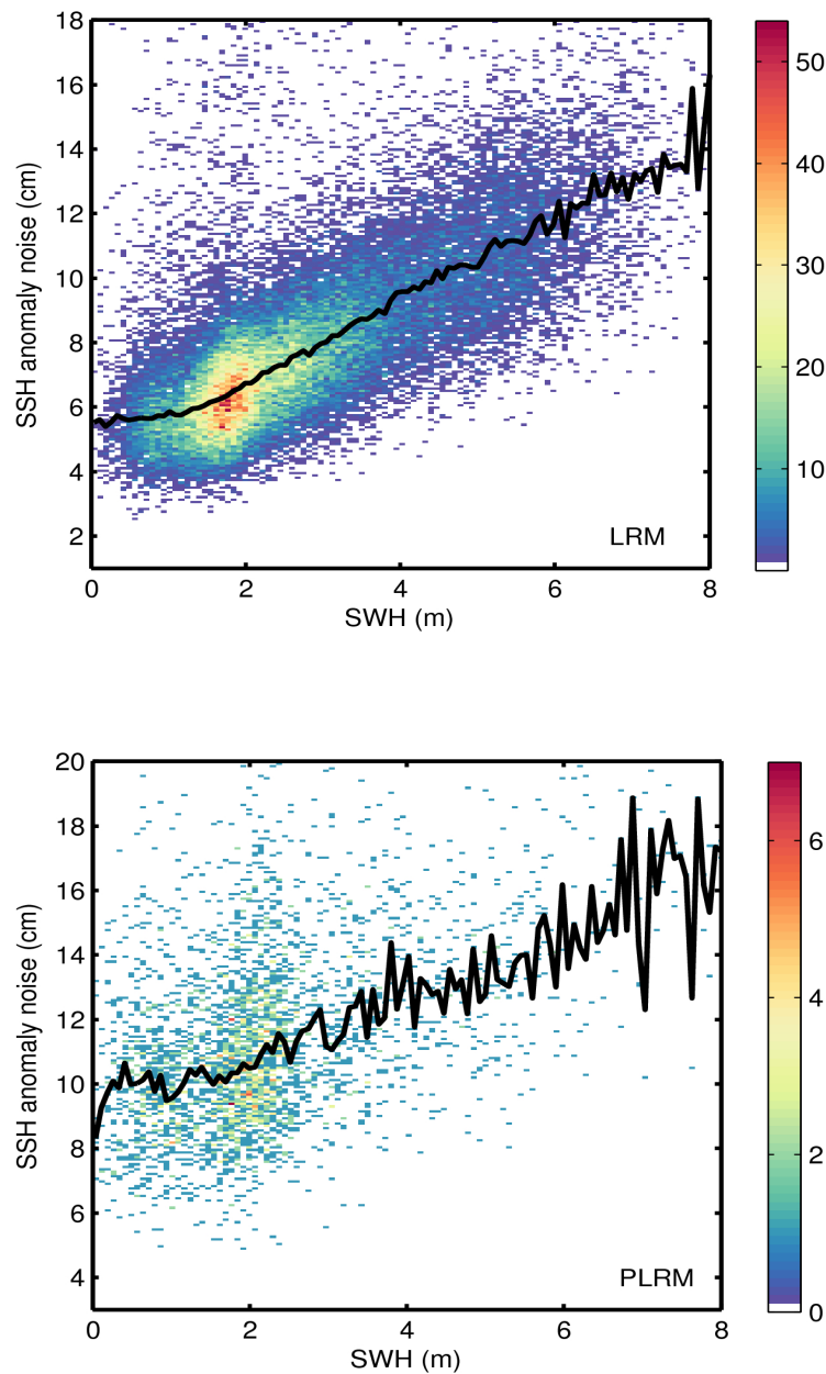
Figure 9. 2D histogram showing flag-valid SSH anomaly noise as a function of SWH for LRM (top) and PLRM (bottom) for 25/06/2017. The black line denotes the median SSH anomaly noise as a function of SWH.
