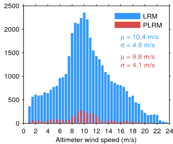
Figure 33. Histogram of flag-valid wind over oceans and lakes for LRM (blue) and PLRM (red) for 25/06/2017. The mean ( \mu ) and standard deviation ( \sigma ) are also shown. Note that values larger than 24 m/s are excluded from the histogram for the sake of readability but not from the computation of \mu and \sigma .
