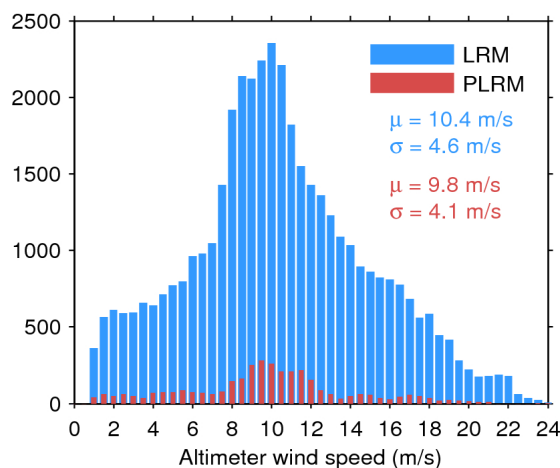
Figure 35. Histogram of science-valid wind over oceans and lakes for LRM (blue) and PLRM (red) for 25/06/2017. The mean ( \mu ) and standard deviation ( \sigma ) are also shown. Note that values larger than 24 m/s are excluded from the histogram for the sake of readability but not from the computation of \mu and \sigma .
