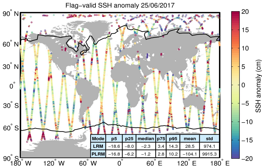
Figure 5. Geographical distribution of flag-valid 1-Hz SSH anomaly data over oceans and lakes for 25/06/2017. The statistical values shown in the table refer to the SSH anomaly in cm and are calculated separately for LRM and PLRM regions. Measurements taken over polar polygons have been excluded from the computation of the statistical values. The black lines mark the outer limit of the Arctic and Antarctic polar polygons.
