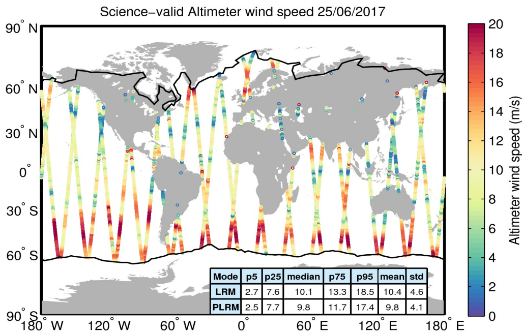
Figure 34. Geographical distribution of science-valid wind data over oceans and lakes for 25/06/2017. The statistical values shown in the table refer to the wind in m/s and are calculated separately for LRM and PLRM regions. The black lines mark the outer limit of the Arctic and Antarctic polar polygons. Gray circles denote records that have been rejected based on the editing criteria described in Table 5.
