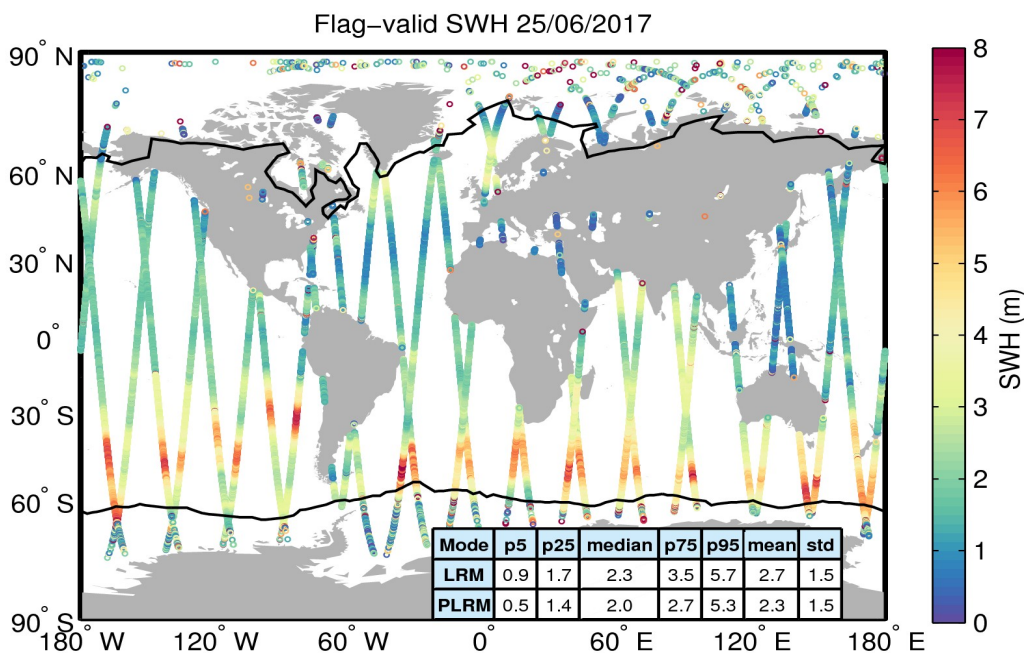
Figure 15. Geographical distribution of flag-valid SWH data over oceans and lakes for 25/06/2017. The statistical values shown in the table refer to the SWH in m and are calculated separately for LRM and PLRM regions. Measurements taken over polar polygons have been excluded from the computation of the statistical values. The black lines mark the outer limit of the Arctic and Antarctic polar polygons.
