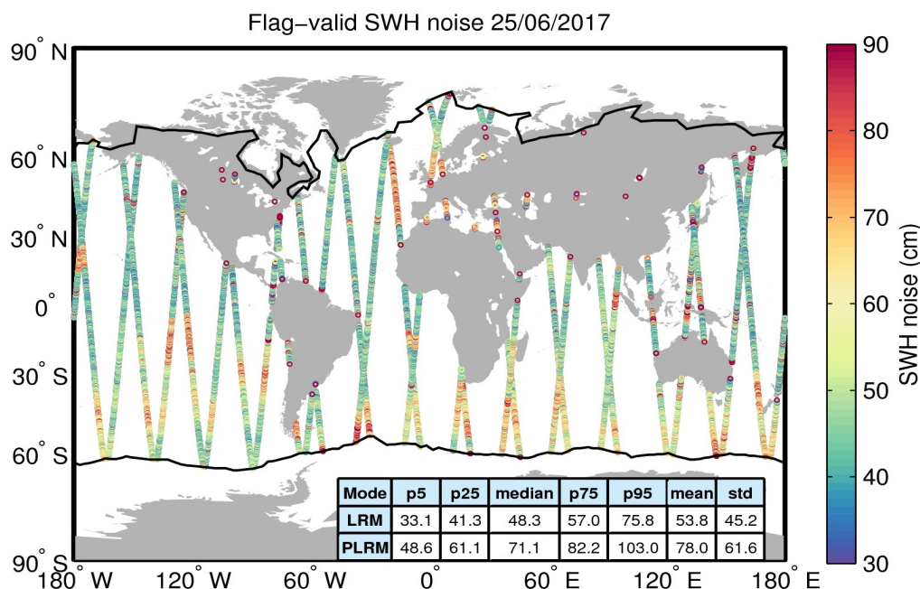
Figure 18. Geographical distribution of flag-valid 20-Hz SWH measurement noise over oceans and lakes for 25/06/2017. The statistical values shown in the table refer to the SWH noise and are calculated separately for LRM and PLRM regions. Measurements taken over polar polygons have been excluded from the computation of the statistical values. The black lines mark the outer limit of the Arctic and Antarctic polar polygons.
