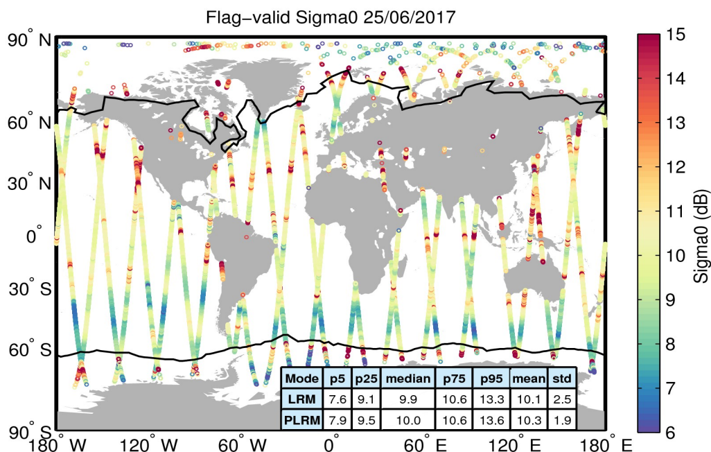
Figure 23. Geographical distribution of flag-valid sigma0 data over oceans and lakes for 25/06/2017. The statistical values shown in the table refer to the sigma0 in dB and are calculated separately for LRM and PLRM regions. Measurements taken over polar polygons have been excluded from the computation of the statistical values. The black lines mark the outer limit of the Arctic and Antarctic polar polygons.
