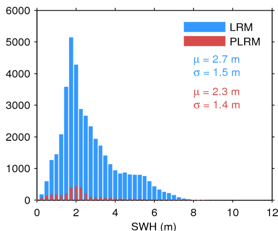
Figure 20. Histogram of science-valid SWH over oceans and lakes for LRM (blue) and PLRM (red) for 25/06/2017. The mean ( \mu ) and standard deviation ( \sigma ) are also shown. Note that values larger than 12 m are excluded from the histogram for the sake of readability but not from the computation of \mu and \sigma .
