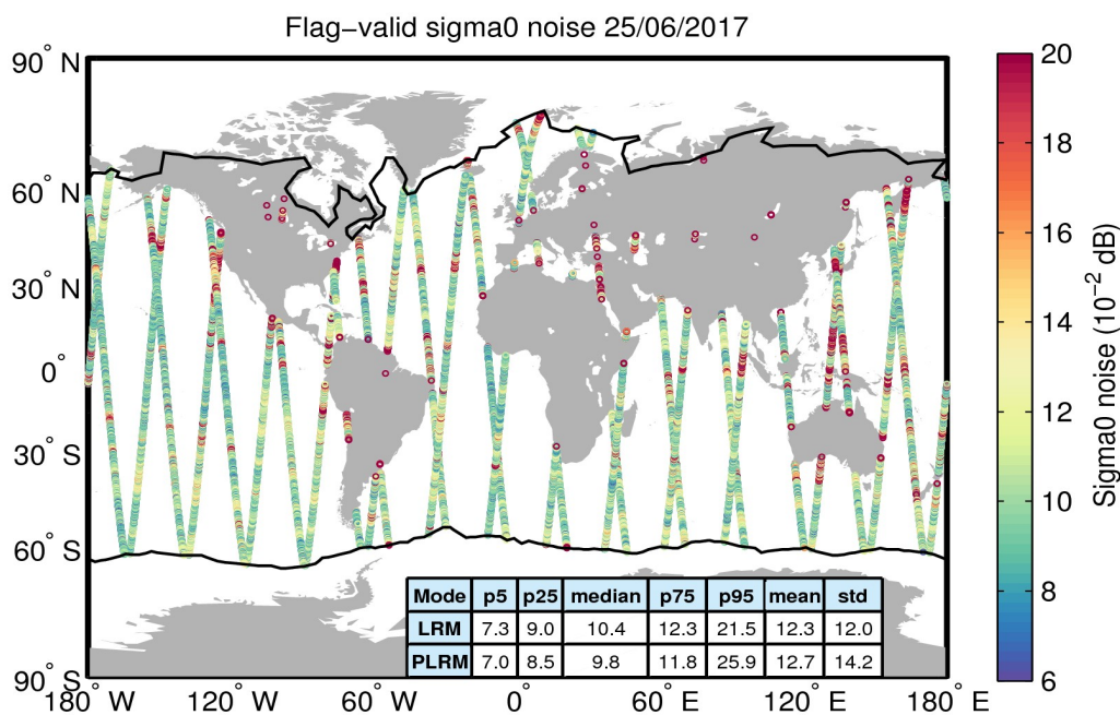
Figure 26. Geographical distribution of flag-valid 20-Hz sigma0 measurement noise over oceans and lakes for 25/06/2017. The statistical values shown in the table refer to the sigma0 noise and are calculated separately for LRM and PLRM regions. Measurements taken over polar polygons have been excluded from the computation of the statistical values. The black lines mark the outer limit of the Arctic and Antarctic polar polygons.
