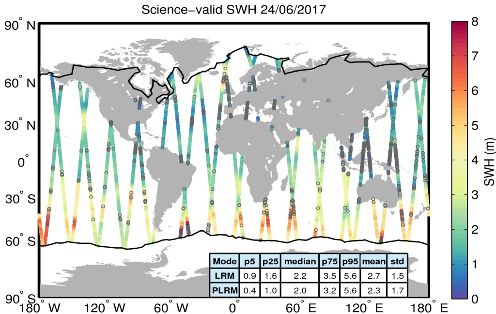
Figure 19. Geographical distribution of science-valid SWH data over oceans and lakes for 24/06/2017. The statistical values shown in the table refer to the SWH in m and are calculated separately for LRM and PLRM regions. The black lines mark the outer limit of the Arctic and Antarctic polar polygons. Gray circles denote records that have been rejected based on the editing criteria described in Table 3.
