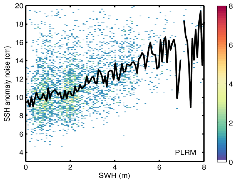
Figure 9. 2D histogram showing flag-valid SSH anomaly noise as a function of SWH for LRM (top) and PLRM (bottom) for 24/06/2017. The black line denotes the median SSH anomaly noise as a function of SWH.
