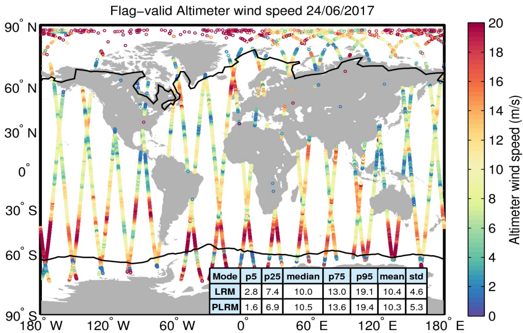
Figure 31. Geographical distribution of flag-valid wind data over oceans and lakes for 24/06/2017. The statistical values shown in the table refer to the wind in m/s and are calculated separately for LRM and PLRM regions. Measurements taken over polar polygons have been excluded from the computation of the statistical values. The black lines mark the outer limit of the Arctic and Antarctic polar polygons.
