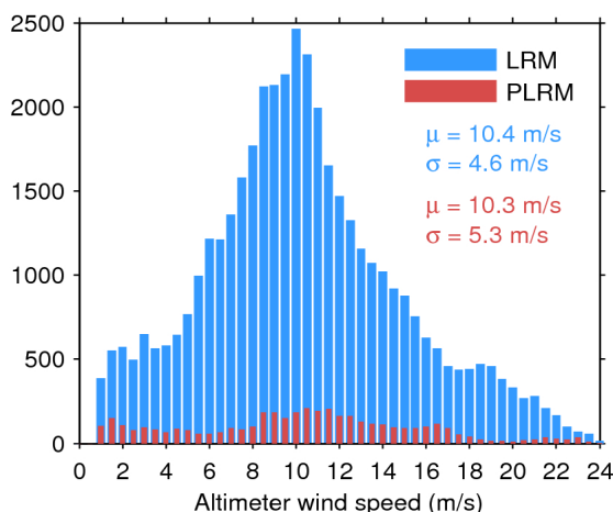
Figure 33. Histogram of flag-valid wind over oceans and lakes for LRM (blue) and PLRM (red) for 24/06/2017. The mean ( \mu ) and standard deviation ( \sigma ) are also shown. Note that values larger than 24 m/s are excluded from the histogram for the sake of readability but not from the computation of \mu and \sigma .
