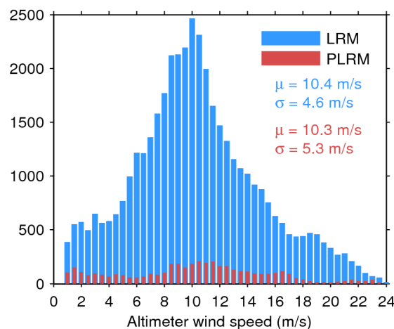
Figure 35. Histogram of science-valid wind over oceans and lakes for LRM (blue) and PLRM (red) for 24/06/2017. The mean ( \mu ) and standard deviation ( \sigma ) are also shown. Note that values larger than 24 m/s are excluded from the histogram for the sake of readability but not from the computation of \mu and \sigma .
