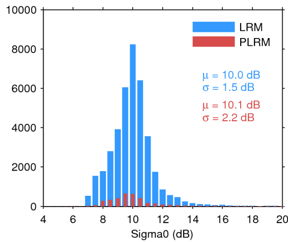
Figure 28. Histogram of science-valid sigma0 over oceans and lakes for LRM (blue) and PLRM (red) for 24/06/2017. The mean ( \mu ) and standard deviation ( \sigma ) are also shown. Note that values outside [4 20] dB are excluded from the histogram for the sake of readability but not from the computation of \mu and \sigma .
