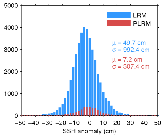
Figure 7. Histogram of flag-valid SSH anomaly over oceans and lakes for LRM (blue) and PLRM (red) for 24/06/2017. The mean ( \mu ) and standard deviation ( \sigma ) are also shown. Note that values outside [-50 50] cm are excluded from the histogram for the sake of readability but not from the computation of \mu and \sigma .
