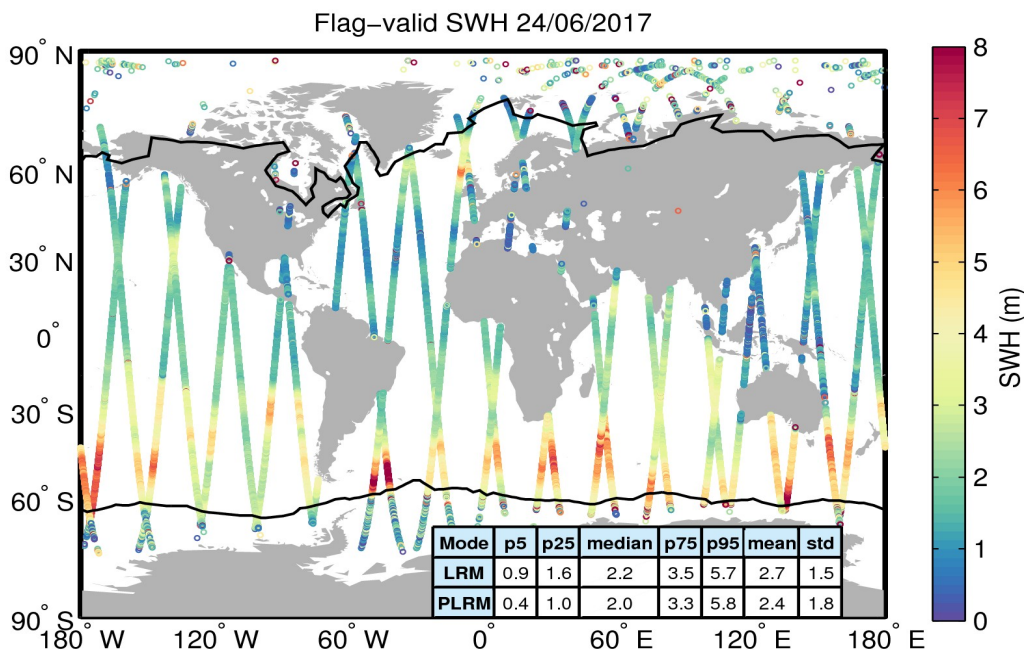
Figure 15. Geographical distribution of flag-valid SWH data over oceans and lakes for 24/06/2017. The statistical values shown in the table refer to the SWH in m and are calculated separately for LRM and PLRM regions. Measurements taken over polar polygons have been excluded from the computation of the statistical values. The black lines mark the outer limit of the Arctic and Antarctic polar polygons.
