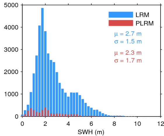
Figure 20. Histogram of science-valid SWH over oceans and lakes for LRM (blue) and PLRM (red) for 24/06/2017. The mean ( \mu ) and standard deviation ( \sigma ) are also shown. Note that values larger than 12 m are excluded from the histogram for the sake of readability but not from the computation of \mu and \sigma .
