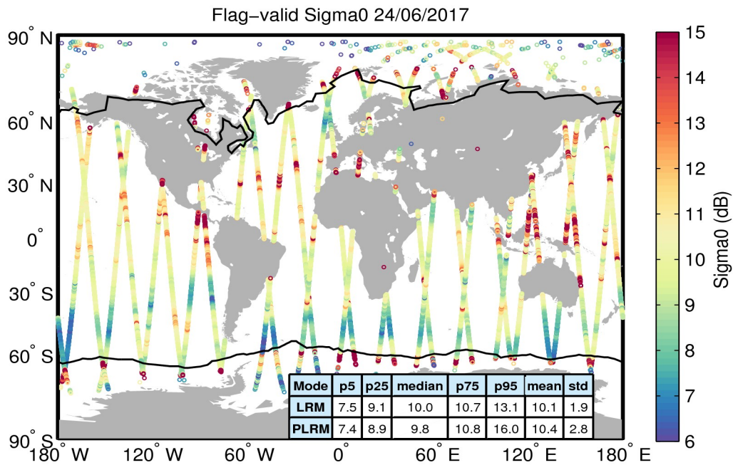
Figure 23. Geographical distribution of flag-valid sigma0 data over oceans and lakes for 24/06/2017. The statistical values shown in the table refer to the sigma0 in dB and are calculated separately for LRM and PLRM regions. Measurements taken over polar polygons have been excluded from the computation of the statistical values. The black lines mark the outer limit of the Arctic and Antarctic polar polygons.
