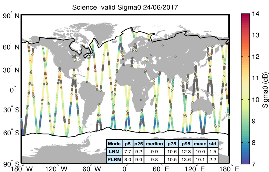
Figure 27. Geographical distribution of science-valid sigma0 data over oceans and lakes for 24/06/2017. The statistical values shown in the table refer to the sigma0 in dB and are calculated separately for LRM and PLRM regions. The black lines mark the outer limit of the Arctic and Antarctic polar polygons. Gray circles denote records that have been rejected based on the editing criteria described in Table 4.
