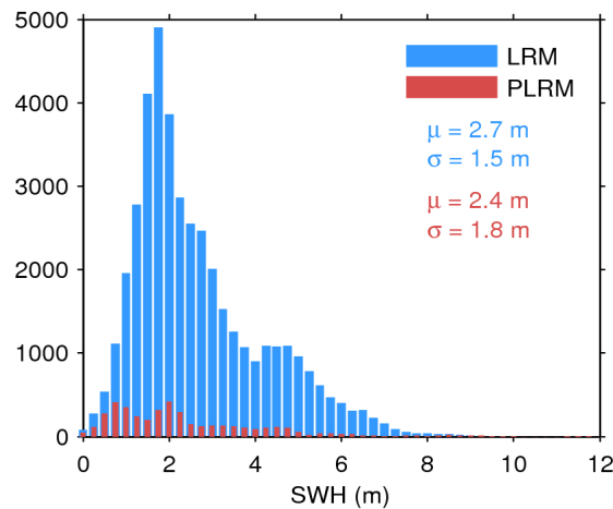
Figure 17. Histogram of flag-valid SWH over oceans and lakes for LRM (blue) and PLRM (red) for 24/06/2017. The mean ( \mu ) and standard deviation ( \sigma ) are also shown. Note that values larger than 12 m are excluded from the histogram for the sake of readability but not from the computation of \mu and \sigma .
