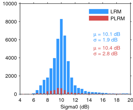
Figure 25. Histogram of flag-valid sigma0 over oceans and lakes for LRM (blue) and PLRM (red) for 24/06/2017. The mean ( \mu ) and standard deviation ( \sigma ) are also shown. Note that values outside [4 20] dB are excluded from the histogram for the sake of readability but not from the computation of \mu and \sigma .
