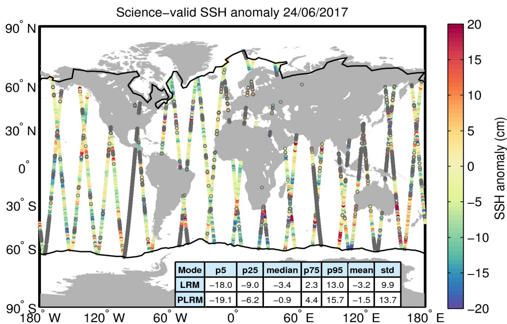
Figure 10. Geographical distribution of science-valid SSH anomaly data over oceans and lakes for 24/06/2017. The statistical values shown in the table refer to the SSH anomaly in cm and are calculated separately for LRM and PLRM regions. The black lines mark the outer limit of the Arctic and Antarctic polar polygons. Gray circles denote records that have been rejected based on the editing criteria described in Table 2.
