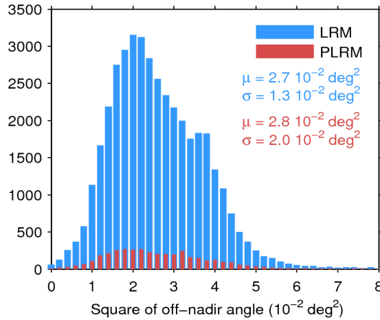
Figure 39. Histogram of flag-valid mispointing over oceans and lakes for LRM (blue) and PLRM (red) for 24/06/2017. Only positive values have been considered. The mean ( \mu ) and standard deviation ( \sigma ) are also shown. Note that values larger than 8 \cdot 10^{-2} \text{ deg}^2 are excluded from the histogram for the sake of readability but not from the computation of \mu and \sigma .
