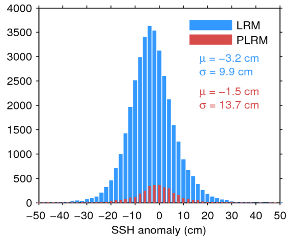
Figure 11. Histogram of science-valid SSH anomaly over oceans and lakes for LRM (blue) and PLRM (red) for 24/06/2017. The mean ( \mu ) and standard deviation ( \sigma ) are also shown. Note that values outside [-50\ 50] cm are excluded from the histogram for the sake of readability but not from the computation of \mu and \sigma .
