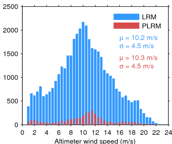
Figure 33. Histogram of flag-valid wind over oceans and lakes for LRM (blue) and PLRM (red) for 23/06/2017. The mean ( \mu ) and standard deviation ( \sigma ) are also shown. Note that values larger than 24 m/s are excluded from the histogram for the sake of readability but not from the computation of \mu and \sigma .
