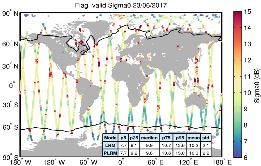
Figure 23. Geographical distribution of flag-valid sigma0 data over oceans and lakes for 23/06/2017. The statistical values shown in the table refer to the sigma0 in dB and are calculated separately for LRM and PLRM regions. Measurements taken over polar polygons have been excluded from the computation of the statistical values. The black lines mark the outer limit of the Arctic and Antarctic polar polygons.
