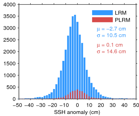
Figure 11. Histogram of science-valid SSH anomaly over oceans and lakes for LRM (blue) and PLRM (red) for 23/06/2017. The mean ( \mu ) and standard deviation ( \sigma ) are also shown. Note that values outside [-50\ 50] cm are excluded from the histogram for the sake of readability but not from the computation of \mu and \sigma .
