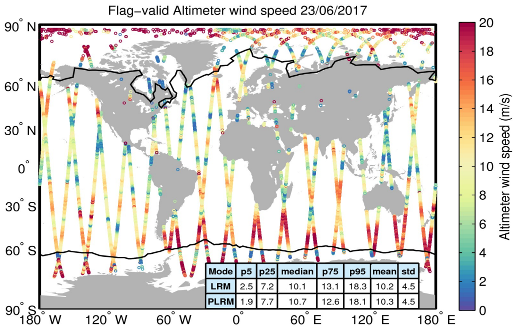
Figure 31. Geographical distribution of flag-valid wind data over oceans and lakes for 23/06/2017. The statistical values shown in the table refer to the wind in m/s and are calculated separately for LRM and PLRM regions. Measurements taken over polar polygons have been excluded from the computation of the statistical values. The black lines mark the outer limit of the Arctic and Antarctic polar polygons.
