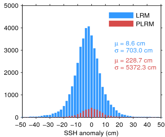
Figure 7. Histogram of flag-valid SSH anomaly over oceans and lakes for LRM (blue) and PLRM (red) for 23/06/2017. The mean ( \mu ) and standard deviation ( \sigma ) are also shown. Note that values outside [-50\ 50] cm are excluded from the histogram for the sake of readability but not from the computation of \mu and \sigma .
