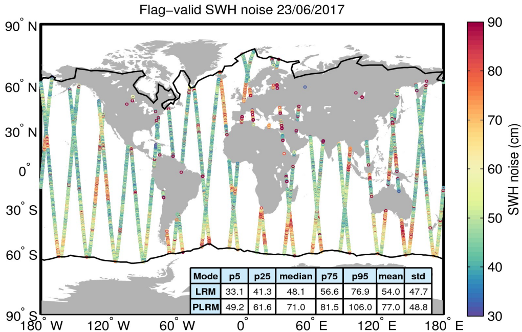
Figure 18. Geographical distribution of flag-valid 20-Hz SWH measurement noise over oceans and lakes for 23/06/2017. The statistical values shown in the table refer to the SWH noise and are calculated separately for LRM and PLRM regions. Measurements taken over polar polygons have been excluded from the computation of the statistical values. The black lines mark the outer limit of the Arctic and Antarctic polar polygons.
