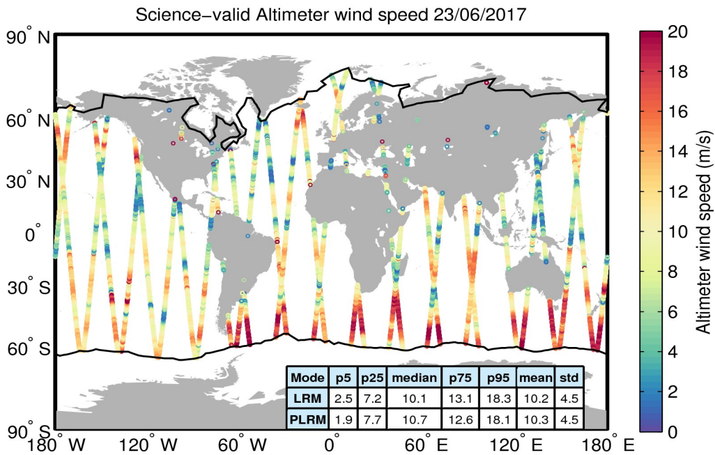
Figure 34. Geographical distribution of science-valid wind data over oceans and lakes for 23/06/2017. The statistical values shown in the table refer to the wind in m/s and are calculated separately for LRM and PLRM regions. The black lines mark the outer limit of the Arctic and Antarctic polar polygons. Gray circles denote records that have been rejected based on the editing criteria described in Table 5.
