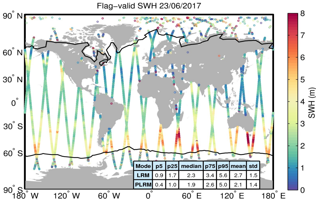
Figure 15. Geographical distribution of flag-valid SWH data over oceans and lakes for 23/06/2017. The statistical values shown in the table refer to the SWH in m and are calculated separately for LRM and PLRM regions. Measurements taken over polar polygons have been excluded from the computation of the statistical values. The black lines mark the outer limit of the Arctic and Antarctic polar polygons.
