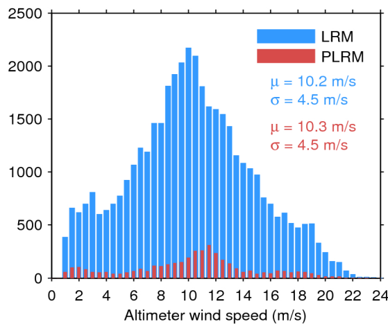
Figure 35. Histogram of science-valid wind over oceans and lakes for LRM (blue) and PLRM (red) for 23/06/2017. The mean ( \mu ) and standard deviation ( \sigma ) are also shown. Note that values larger than 24 m/s are excluded from the histogram for the sake of readability but not from the computation of \mu and \sigma .
