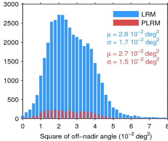
Figure 39. Histogram of flag-valid mispointing over oceans and lakes for LRM (blue) and PLRM (red) for 23/06/2017. Only positive values have been considered. The mean ( \mu ) and standard deviation ( \sigma ) are also shown. Note that values larger than 8 \cdot 10^{-2} \text{ deg}^2 are excluded from the histogram for the sake of readability but not from the computation of \mu and \sigma .
