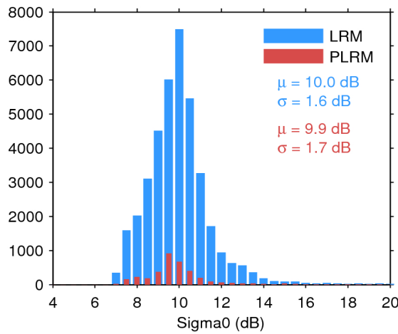
Figure 28. Histogram of science-valid sigma0 over oceans and lakes for LRM (blue) and PLRM (red) for 23/06/2017. The mean ( \mu ) and standard deviation ( \sigma ) are also shown. Note that values outside [4 20] dB are excluded from the histogram for the sake of readability but not from the computation of \mu and \sigma .
