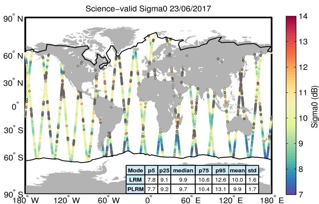
Figure 27. Geographical distribution of science-valid sigma0 data over oceans and lakes for 23/06/2017. The statistical values shown in the table refer to the sigma0 in dB and are calculated separately for LRM and PLRM regions. The black lines mark the outer limit of the Arctic and Antarctic polar polygons. Gray circles denote records that have been rejected based on the editing criteria described in Table 4.
