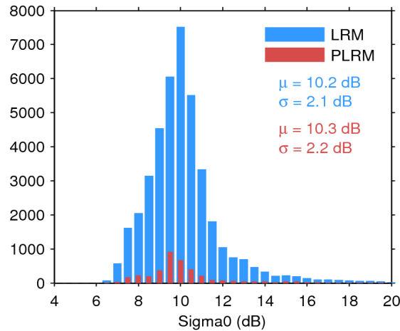
Figure 25. Histogram of flag-valid sigma0 over oceans and lakes for LRM (blue) and PLRM (red) for 23/06/2017. The mean ( \mu ) and standard deviation ( \sigma ) are also shown. Note that values outside [4 20] dB are excluded from the histogram for the sake of readability but not from the computation of \mu and \sigma .
