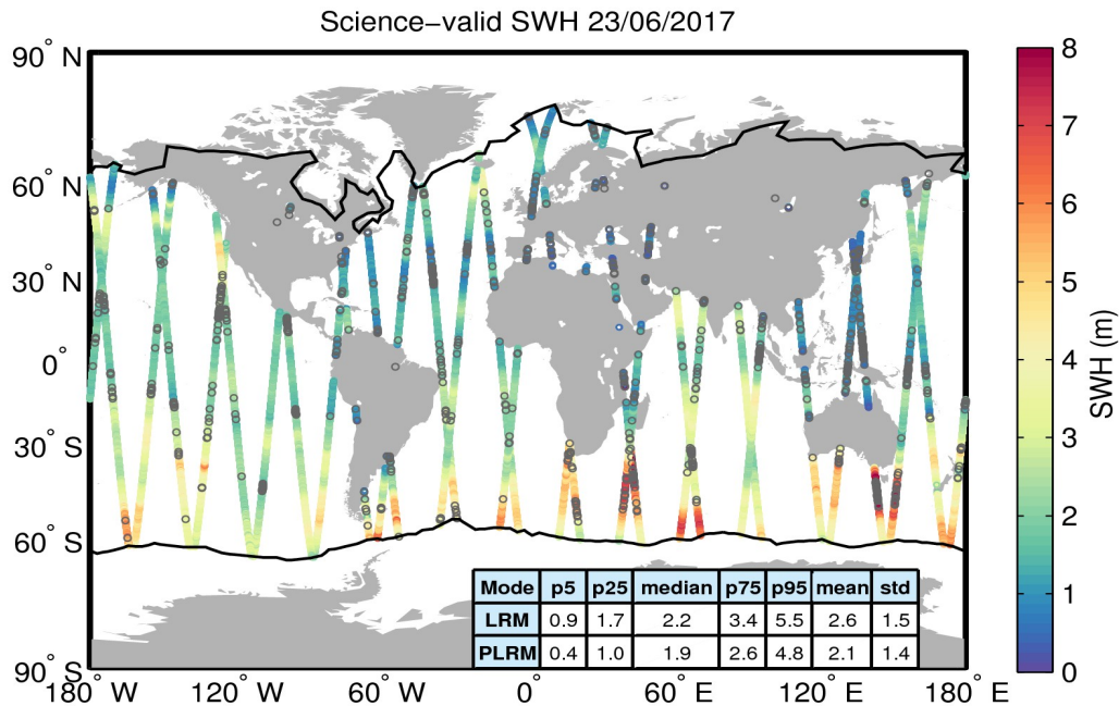
Figure 19. Geographical distribution of science-valid SWH data over oceans and lakes for 23/06/2017. The statistical values shown in the table refer to the SWH in m and are calculated separately for LRM and PLRM regions. The black lines mark the outer limit of the Arctic and Antarctic polar polygons. Gray circles denote records that have been rejected based on the editing criteria described in Table 3.
