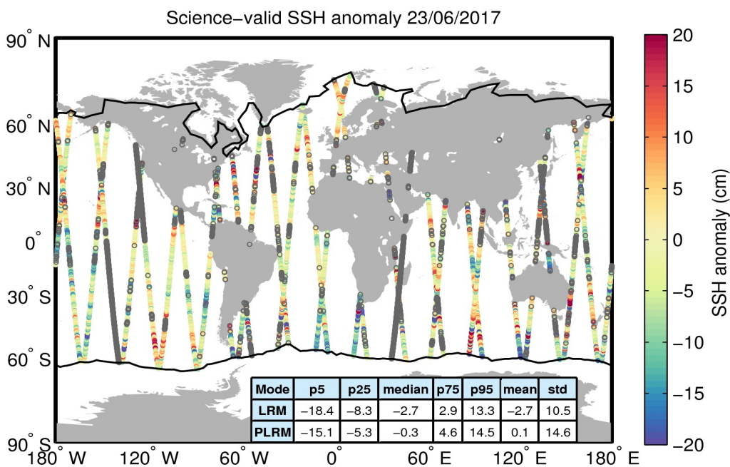
Figure 10. Geographical distribution of science-valid SSH anomaly data over oceans and lakes for 23/06/2017. The statistical values shown in the table refer to the SSH anomaly in cm and are calculated separately for LRM and PLRM regions. The black lines mark the outer limit of the Arctic and Antarctic polar polygons. Gray circles denote records that have been rejected based on the editing criteria described in Table 2.
