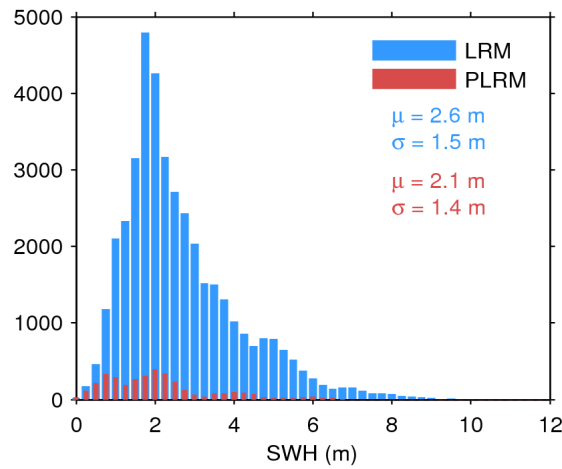
Figure 20. Histogram of science-valid SWH over oceans and lakes for LRM (blue) and PLRM (red) for 23/06/2017. The mean ( \mu ) and standard deviation ( \sigma ) are also shown. Note that values larger than 12 m are excluded from the histogram for the sake of readability but not from the computation of \mu and \sigma .
