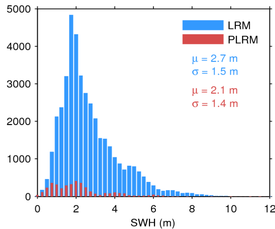
Figure 17. Histogram of flag-valid SWH over oceans and lakes for LRM (blue) and PLRM (red) for 23/06/2017. The mean ( \mu ) and standard deviation ( \sigma ) are also shown. Note that values larger than 12 m are excluded from the histogram for the sake of readability but not from the computation of \mu and \sigma .
