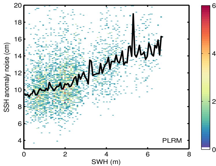
Figure 9. 2D histogram showing flag-valid SSH anomaly noise as a function of SWH for LRM (top) and PLRM (bottom) for 23/06/2017. The black line denotes the median SSH anomaly noise as a function of SWH.
