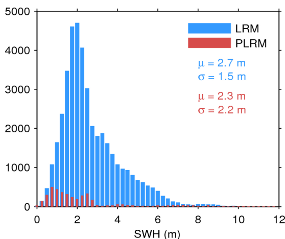
Figure 17. Histogram of flag-valid SWH over oceans and lakes for LRM (blue) and PLRM (red) for 22/06/2017. The mean ( \mu ) and standard deviation ( \sigma ) are also shown. Note that values larger than 12 m are excluded from the histogram for the sake of readability but not from the computation of \mu and \sigma .
