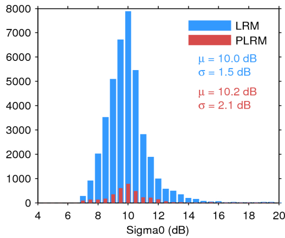
Figure 28. Histogram of science-valid sigma0 over oceans and lakes for LRM (blue) and PLRM (red) for 22/06/2017. The mean ( \mu ) and standard deviation ( \sigma ) are also shown. Note that values outside [4 20] dB are excluded from the histogram for the sake of readability but not from the computation of \mu and \sigma .
