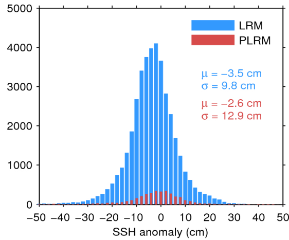
Figure 11. Histogram of science-valid SSH anomaly over oceans and lakes for LRM (blue) and PLRM (red) for 22/06/2017. The mean ( \mu ) and standard deviation ( \sigma ) are also shown. Note that values outside [-50 50] cm are excluded from the histogram for the sake of readability but not from the computation of \mu and \sigma .
