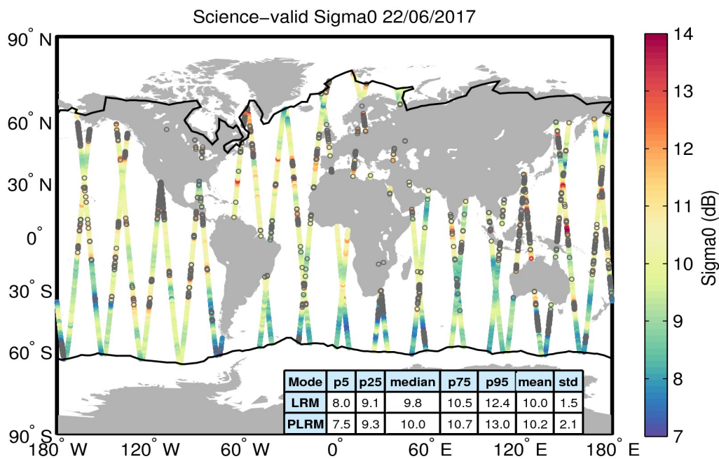
Figure 27. Geographical distribution of science-valid sigma0 data over oceans and lakes for 22/06/2017. The statistical values shown in the table refer to the sigma0 in dB and are calculated separately for LRM and PLRM regions. The black lines mark the outer limit of the Arctic and Antarctic polar polygons. Gray circles denote records that have been rejected based on the editing criteria described in Table 4.
