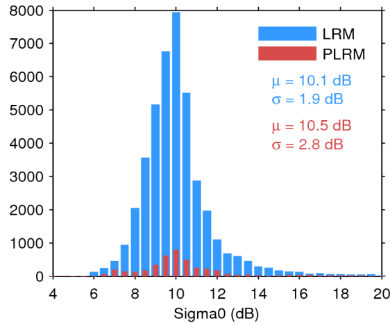
Figure 25. Histogram of flag-valid sigma0 over oceans and lakes for LRM (blue) and PLRM (red) for 22/06/2017. The mean ( \mu ) and standard deviation ( \sigma ) are also shown. Note that values outside [4 20] dB are excluded from the histogram for the sake of readability but not from the computation of \mu and \sigma .
