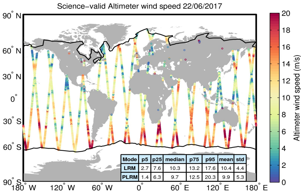
Figure 34. Geographical distribution of science-valid wind data over oceans and lakes for 22/06/2017. The statistical values shown in the table refer to the wind in m/s and are calculated separately for LRM and PLRM regions. The black lines mark the outer limit of the Arctic and Antarctic polar polygons. Gray circles denote records that have been rejected based on the editing criteria described in Table 5.
