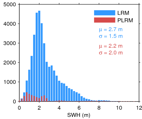
Figure 20. Histogram of science-valid SWH over oceans and lakes for LRM (blue) and PLRM (red) for 22/06/2017. The mean ( \mu ) and standard deviation ( \sigma ) are also shown. Note that values larger than 12 m are excluded from the histogram for the sake of readability but not from the computation of \mu and \sigma .
