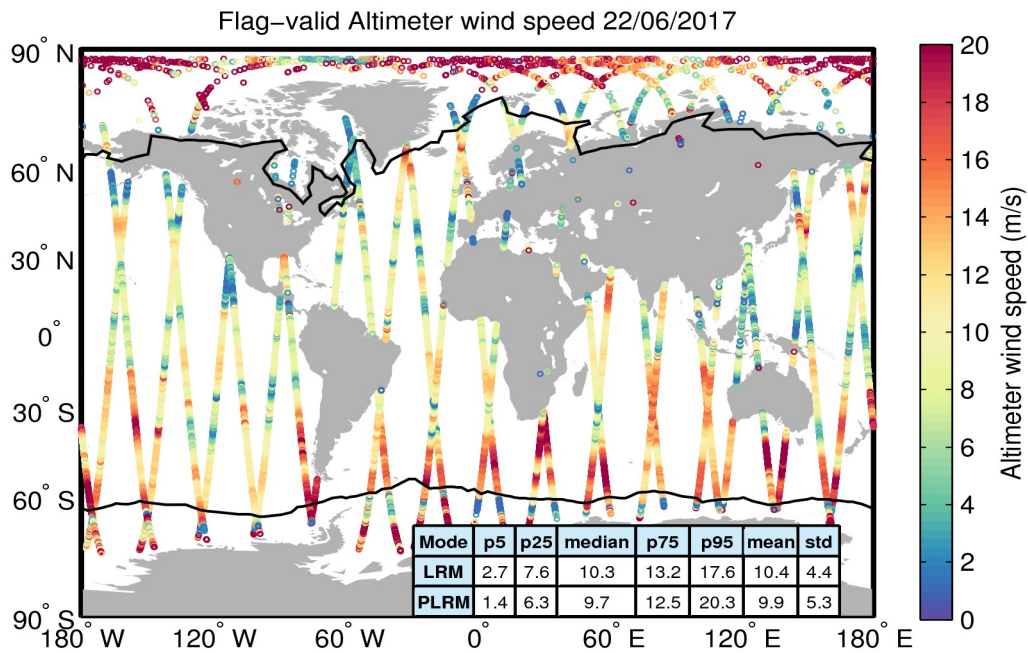
Figure 31. Geographical distribution of flag-valid wind data over oceans and lakes for 22/06/2017. The statistical values shown in the table refer to the wind in m/s and are calculated separately for LRM and PLRM regions. Measurements taken over polar polygons have been excluded from the computation of the statistical values. The black lines mark the outer limit of the Arctic and Antarctic polar polygons.
