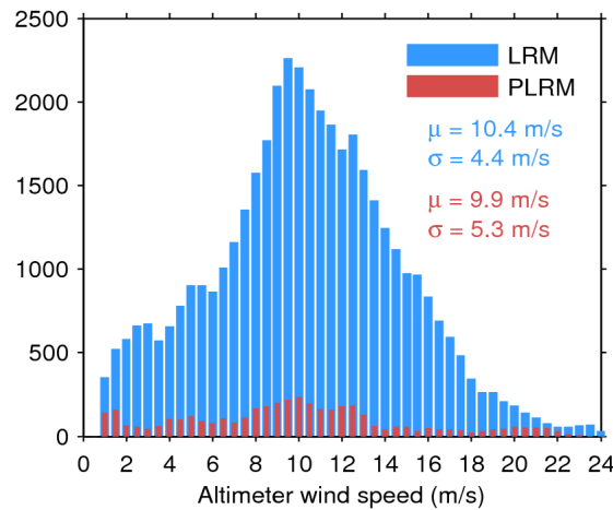
Figure 33. Histogram of flag-valid wind over oceans and lakes for LRM (blue) and PLRM (red) for 22/06/2017. The mean ( \mu ) and standard deviation ( \sigma ) are also shown. Note that values larger than 24 m/s are excluded from the histogram for the sake of readability but not from the computation of \mu and \sigma .
