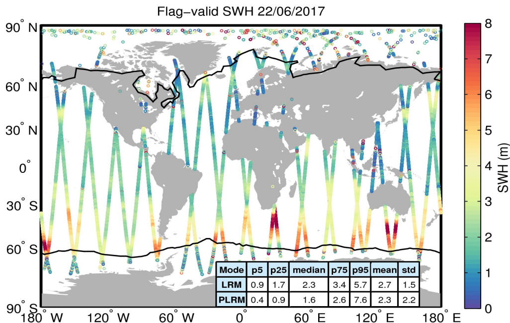
Figure 15. Geographical distribution of flag-valid SWH data over oceans and lakes for 22/06/2017. The statistical values shown in the table refer to the SWH in m and are calculated separately for LRM and PLRM regions. Measurements taken over polar polygons have been excluded from the computation of the statistical values. The black lines mark the outer limit of the Arctic and Antarctic polar polygons.
