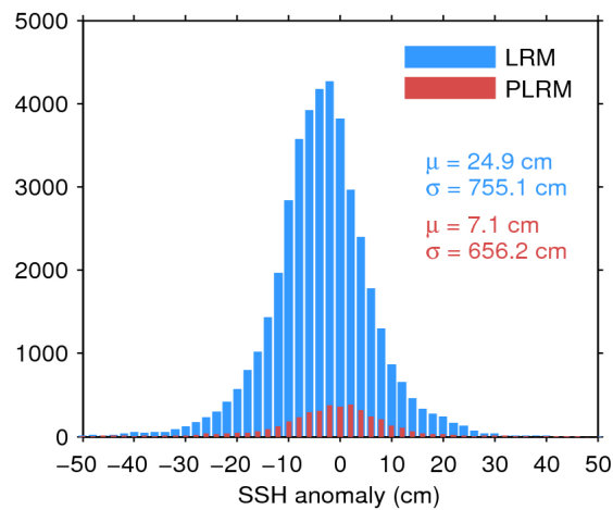
Figure 7. Histogram of flag-valid SSH anomaly over oceans and lakes for LRM (blue) and PLRM (red) for 22/06/2017. The mean ( \mu ) and standard deviation ( \sigma ) are also shown. Note that values outside [-50 50] cm are excluded from the histogram for the sake of readability but not from the computation of \mu and \sigma .
