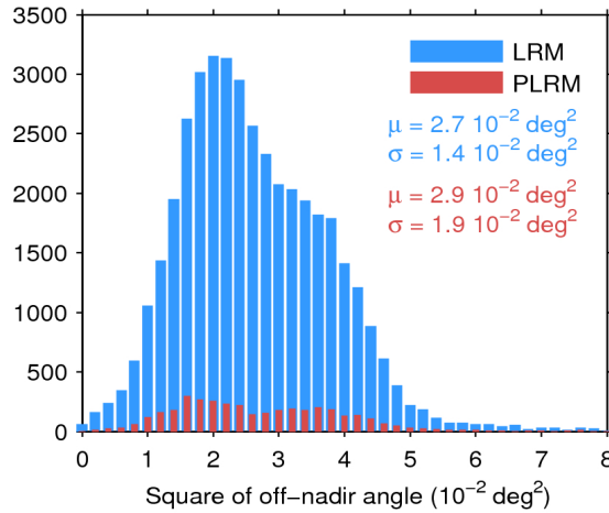
Figure 39. Histogram of flag-valid mispointing over oceans and lakes for LRM (blue) and PLRM (red) for 22/06/2017. Only positive values have been considered. The mean ( \mu ) and standard deviation ( \sigma ) are also shown. Note that values larger than 8 \cdot 10^{-2} \text{ deg}^2 are excluded from the histogram for the sake of readability but not from the computation of \mu and \sigma .
