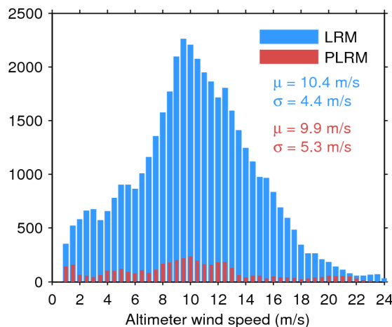
Figure 35. Histogram of science-valid wind over oceans and lakes for LRM (blue) and PLRM (red) for 22/06/2017. The mean ( \mu ) and standard deviation ( \sigma ) are also shown. Note that values larger than 24 m/s are excluded from the histogram for the sake of readability but not from the computation of \mu and \sigma .
