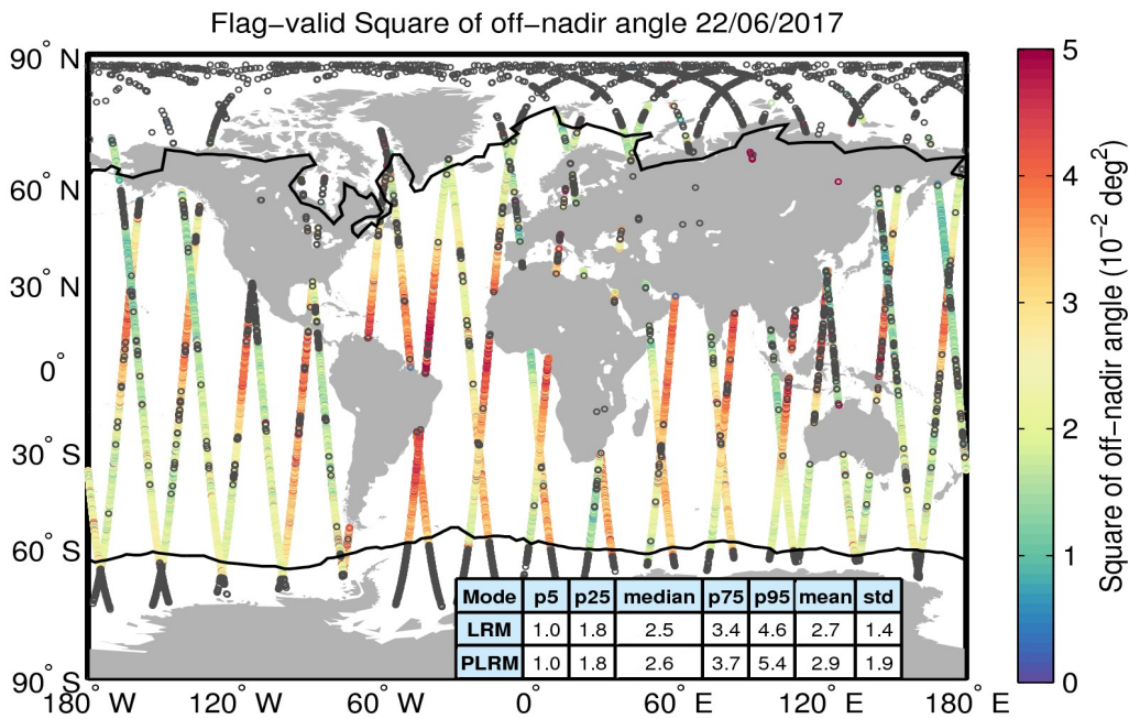
Figure 37. Geographical distribution of flag-valid mispointing data over oceans and lakes for 22/06/2017. The statistical values shown in the table refer to the mispointing in 10^{-2} \text{ deg}^2 and are calculated separately for LRM and PLRM regions. Measurements taken over polar polygons have been excluded from the computation of the statistical values. The black lines mark the outer limit of the Arctic and Antarctic polar polygons. Gray circles denote negative values.
