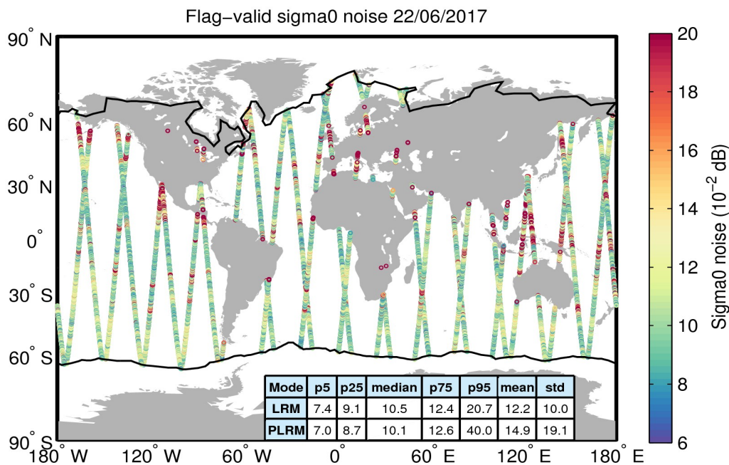
Figure 26. Geographical distribution of flag-valid 20-Hz sigma0 measurement noise over oceans and lakes for 22/06/2017. The statistical values shown in the table refer to the sigma0 noise and are calculated separately for LRM and PLRM regions. Measurements taken over polar polygons have been excluded from the computation of the statistical values. The black lines mark the outer limit of the Arctic and Antarctic polar polygons.
