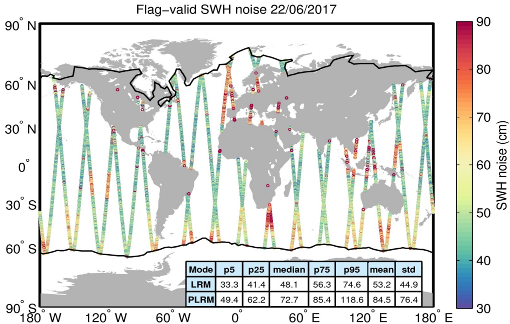
Figure 18. Geographical distribution of flag-valid 20-Hz SWH measurement noise over oceans and lakes for 22/06/2017. The statistical values shown in the table refer to the SWH noise and are calculated separately for LRM and PLRM regions. Measurements taken over polar polygons have been excluded from the computation of the statistical values. The black lines mark the outer limit of the Arctic and Antarctic polar polygons.
