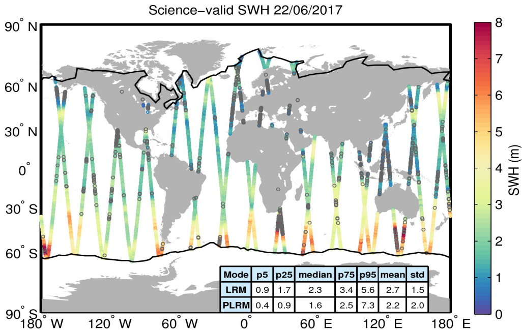
Figure 19. Geographical distribution of science-valid SWH data over oceans and lakes for 22/06/2017. The statistical values shown in the table refer to the SWH in m and are calculated separately for LRM and PLRM regions. The black lines mark the outer limit of the Arctic and Antarctic polar polygons. Gray circles denote records that have been rejected based on the editing criteria described in Table 3.
