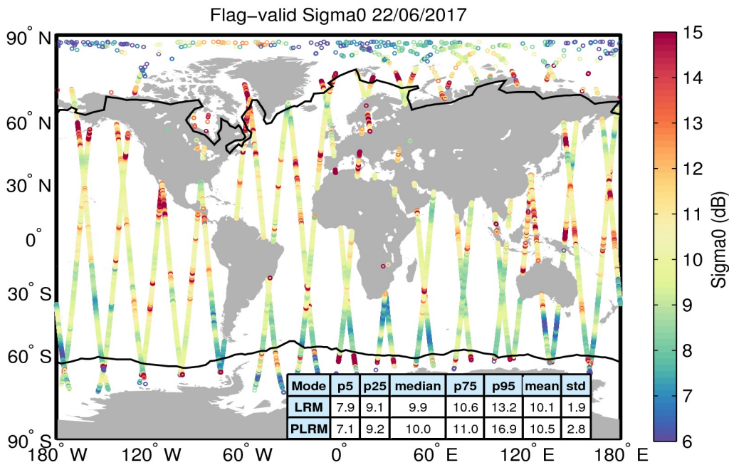
Figure 23. Geographical distribution of flag-valid sigma0 data over oceans and lakes for 22/06/2017. The statistical values shown in the table refer to the sigma0 in dB and are calculated separately for LRM and PLRM regions. Measurements taken over polar polygons have been excluded from the computation of the statistical values. The black lines mark the outer limit of the Arctic and Antarctic polar polygons.
