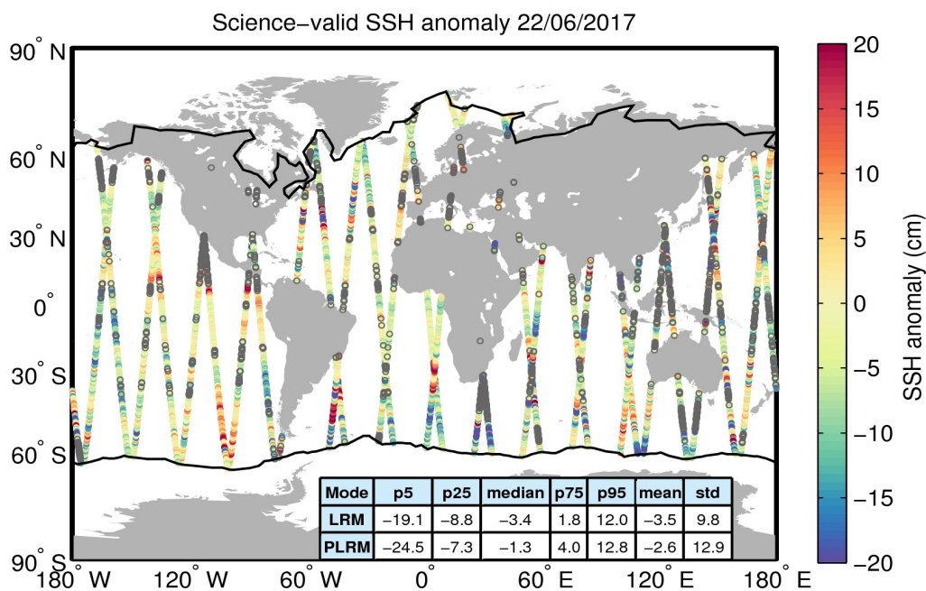
Figure 10. Geographical distribution of science-valid SSH anomaly data over oceans and lakes for 22/06/2017. The statistical values shown in the table refer to the SSH anomaly in cm and are calculated separately for LRM and PLRM regions. The black lines mark the outer limit of the Arctic and Antarctic polar polygons. Gray circles denote records that have been rejected based on the editing criteria described in Table 2.
