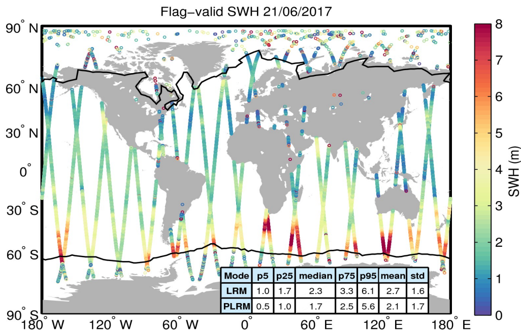
Figure 15. Geographical distribution of flag-valid SWH data over oceans and lakes for 21/06/2017. The statistical values shown in the table refer to the SWH in m and are calculated separately for LRM and PLRM regions. Measurements taken over polar polygons have been excluded from the computation of the statistical values. The black lines mark the outer limit of the Arctic and Antarctic polar polygons.
