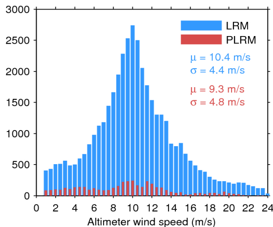
Figure 35. Histogram of science-valid wind over oceans and lakes for LRM (blue) and PLRM (red) for 21/06/2017. The mean ( \mu ) and standard deviation ( \sigma ) are also shown. Note that values larger than 24 m/s are excluded from the histogram for the sake of readability but not from the computation of \mu and \sigma .
