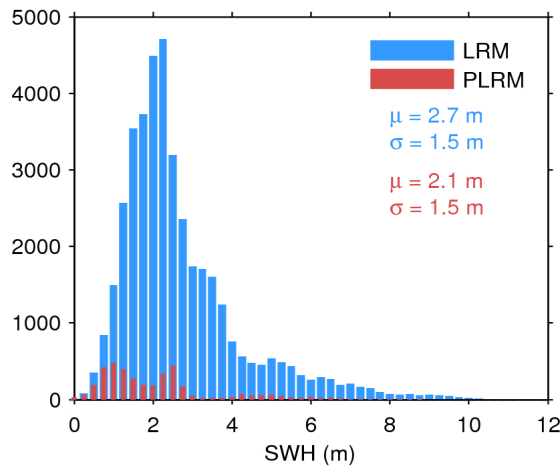
Figure 20. Histogram of science-valid SWH over oceans and lakes for LRM (blue) and PLRM (red) for 21/06/2017. The mean ( \mu ) and standard deviation ( \sigma ) are also shown. Note that values larger than 12 m are excluded from the histogram for the sake of readability but not from the computation of \mu and \sigma .
