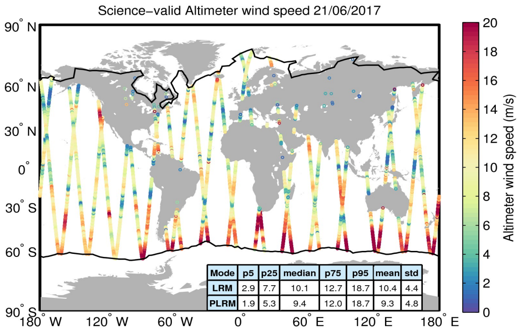
Figure 34. Geographical distribution of science-valid wind data over oceans and lakes for 21/06/2017. The statistical values shown in the table refer to the wind in m/s and are calculated separately for LRM and PLRM regions. The black lines mark the outer limit of the Arctic and Antarctic polar polygons. Gray circles denote records that have been rejected based on the editing criteria described in Table 5.
