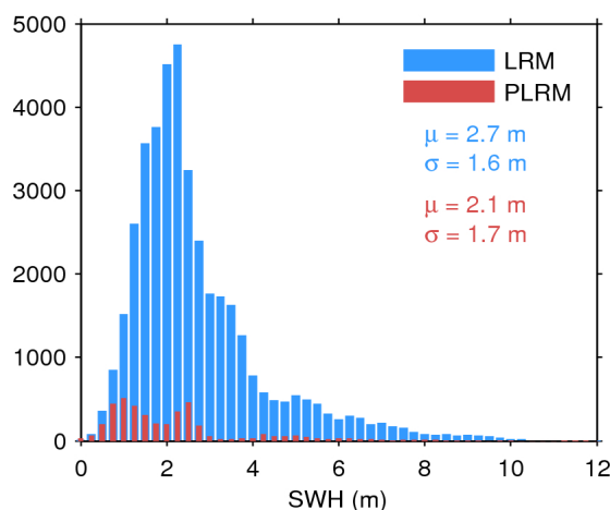
Figure 17. Histogram of flag-valid SWH over oceans and lakes for LRM (blue) and PLRM (red) for 21/06/2017. The mean ( \mu ) and standard deviation ( \sigma ) are also shown. Note that values larger than 12 m are excluded from the histogram for the sake of readability but not from the computation of \mu and \sigma .
