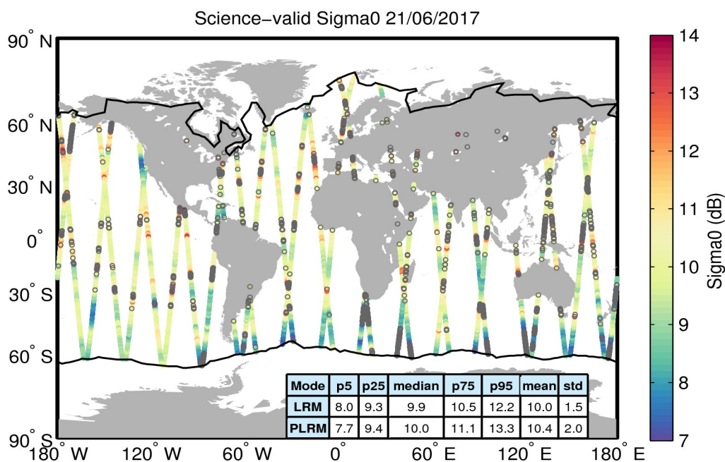
Figure 27. Geographical distribution of science-valid sigma0 data over oceans and lakes for 21/06/2017. The statistical values shown in the table refer to the sigma0 in dB and are calculated separately for LRM and PLRM regions. The black lines mark the outer limit of the Arctic and Antarctic polar polygons. Gray circles denote records that have been rejected based on the editing criteria described in Table 4.
