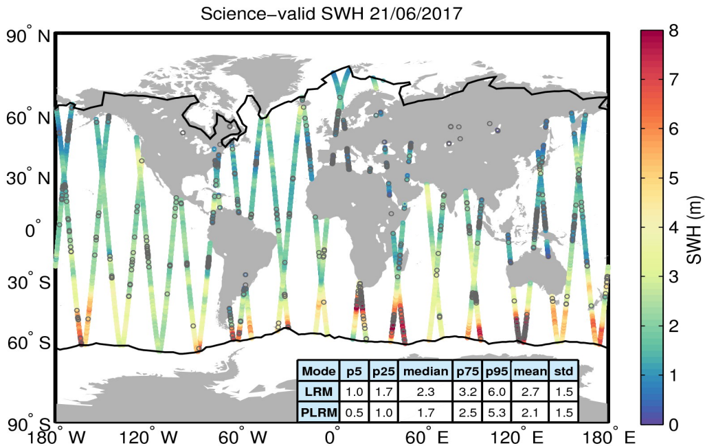
Figure 19. Geographical distribution of science-valid SWH data over oceans and lakes for 21/06/2017. The statistical values shown in the table refer to the SWH in m and are calculated separately for LRM and PLRM regions. The black lines mark the outer limit of the Arctic and Antarctic polar polygons. Gray circles denote records that have been rejected based on the editing criteria described in Table 3.
