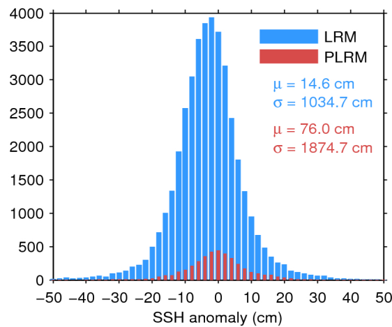
Figure 7. Histogram of flag-valid SSH anomaly over oceans and lakes for LRM (blue) and PLRM (red) for 21/06/2017. The mean ( \mu ) and standard deviation ( \sigma ) are also shown. Note that values outside [-50 50] cm are excluded from the histogram for the sake of readability but not from the computation of \mu and \sigma .
