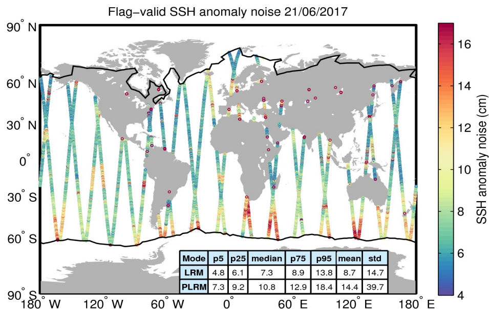
Figure 8. Geographical distribution of flag-valid 20-Hz SSH anomaly measurement noise over oceans and lakes for 21/06/2017. The statistical values shown in the table refer to the SSH anomaly noise and are calculated separately for LRM and PLRM regions. Measurements taken over polar polygons have been excluded from the computation of the statistical values. The black lines mark the outer limit of the Arctic and Antarctic polar polygons.
