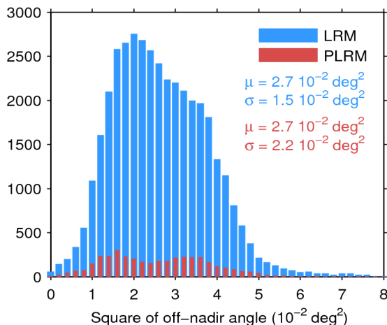
Figure 39. Histogram of flag-valid mispointing over oceans and lakes for LRM (blue) and PLRM (red) for 21/06/2017. Only positive values have been considered. The mean ( \mu ) and standard deviation ( \sigma ) are also shown. Note that values larger than 8 \cdot 10^{-2} \text{ deg}^2 are excluded from the histogram for the sake of readability but not from the computation of \mu and \sigma .
