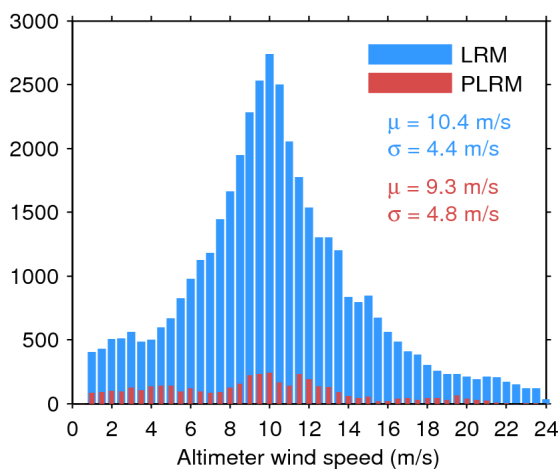
Figure 33. Histogram of flag-valid wind over oceans and lakes for LRM (blue) and PLRM (red) for 21/06/2017. The mean ( \mu ) and standard deviation ( \sigma ) are also shown. Note that values larger than 24 m/s are excluded from the histogram for the sake of readability but not from the computation of \mu and \sigma .
