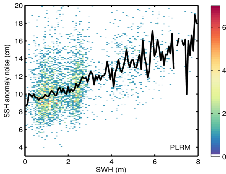
Figure 9. 2D histogram showing flag-valid SSH anomaly noise as a function of SWH for LRM (top) and PLRM (bottom) for 21/06/2017. The black line denotes the median SSH anomaly noise as a function of SWH.
