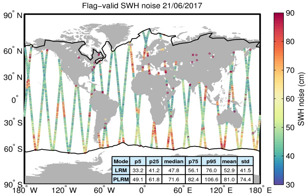
Figure 18. Geographical distribution of flag-valid 20-Hz SWH measurement noise over oceans and lakes for 21/06/2017. The statistical values shown in the table refer to the SWH noise and are calculated separately for LRM and PLRM regions. Measurements taken over polar polygons have been excluded from the computation of the statistical values. The black lines mark the outer limit of the Arctic and Antarctic polar polygons.
