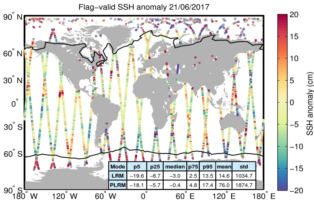
Figure 5. Geographical distribution of flag-valid 1-Hz SSH anomaly data over oceans and lakes for 21/06/2017. The statistical values shown in the table refer to the SSH anomaly in cm and are calculated separately for LRM and PLRM regions. Measurements taken over polar polygons have been excluded from the computation of the statistical values. The black lines mark the outer limit of the Arctic and Antarctic polar polygons.
