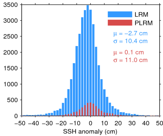
Figure 11. Histogram of science-valid SSH anomaly over oceans and lakes for LRM (blue) and PLRM (red) for 21/06/2017. The mean ( \mu ) and standard deviation ( \sigma ) are also shown. Note that values outside [-50\ 50] cm are excluded from the histogram for the sake of readability but not from the computation of \mu and \sigma .
