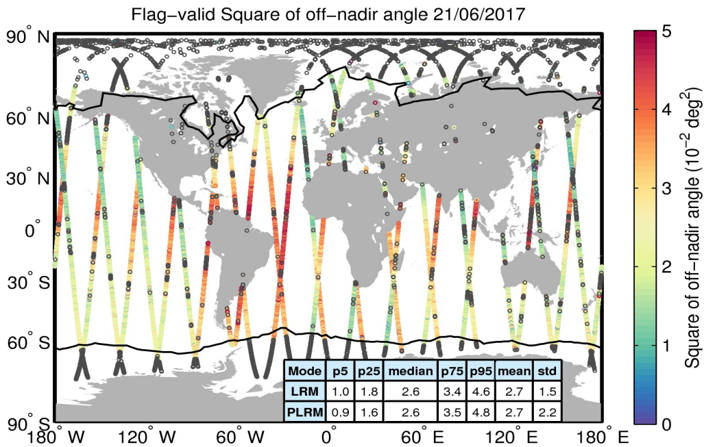
Figure 37. Geographical distribution of flag-valid mispointing data over oceans and lakes for 21/06/2017. The statistical values shown in the table refer to the mispointing in 10^{-2} deg 2 and are calculated separately for LRM and PLRM regions. Measurements taken over polar polygons have been excluded from the computation of the statistical values. The black lines mark the outer limit of the Arctic and Antarctic polar polygons. Gray circles denote negative values.
