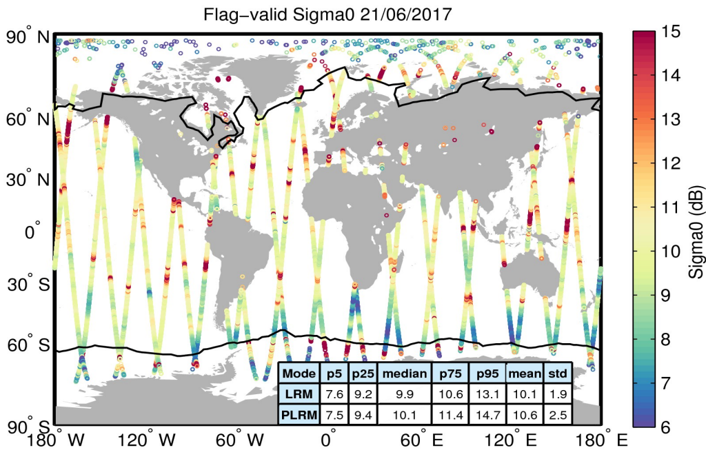
Figure 23. Geographical distribution of flag-valid sigma0 data over oceans and lakes for 21/06/2017. The statistical values shown in the table refer to the sigma0 in dB and are calculated separately for LRM and PLRM regions. Measurements taken over polar polygons have been excluded from the computation of the statistical values. The black lines mark the outer limit of the Arctic and Antarctic polar polygons.
