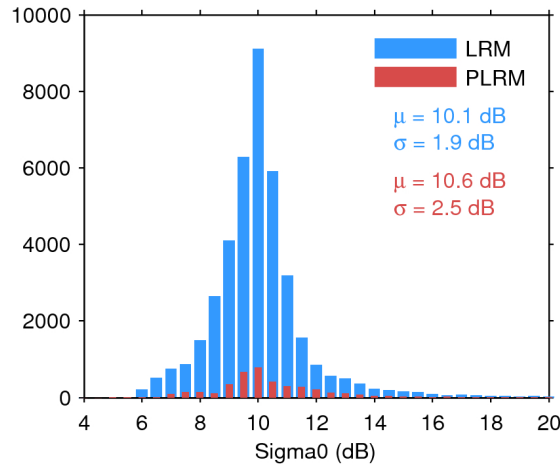
Figure 25. Histogram of flag-valid sigma0 over oceans and lakes for LRM (blue) and PLRM (red) for 21/06/2017. The mean ( \mu ) and standard deviation ( \sigma ) are also shown. Note that values outside [4 20] dB are excluded from the histogram for the sake of readability but not from the computation of \mu and \sigma .
