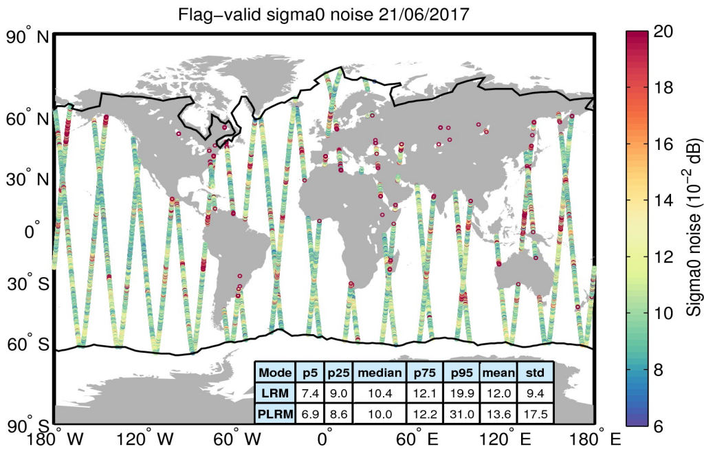
Figure 26. Geographical distribution of flag-valid 20-Hz sigma0 measurement noise over oceans and lakes for 21/06/2017. The statistical values shown in the table refer to the sigma0 noise and are calculated separately for LRM and PLRM regions. Measurements taken over polar polygons have been excluded from the computation of the statistical values. The black lines mark the outer limit of the Arctic and Antarctic polar polygons.
