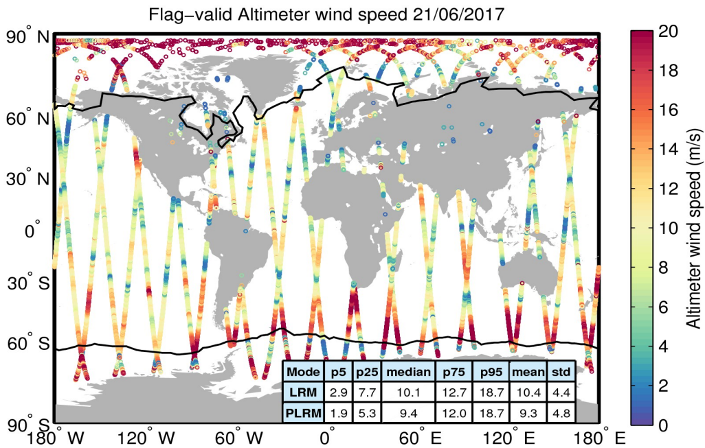
Figure 31. Geographical distribution of flag-valid wind data over oceans and lakes for 21/06/2017. The statistical values shown in the table refer to the wind in m/s and are calculated separately for LRM and PLRM regions. Measurements taken over polar polygons have been excluded from the computation of the statistical values. The black lines mark the outer limit of the Arctic and Antarctic polar polygons.
