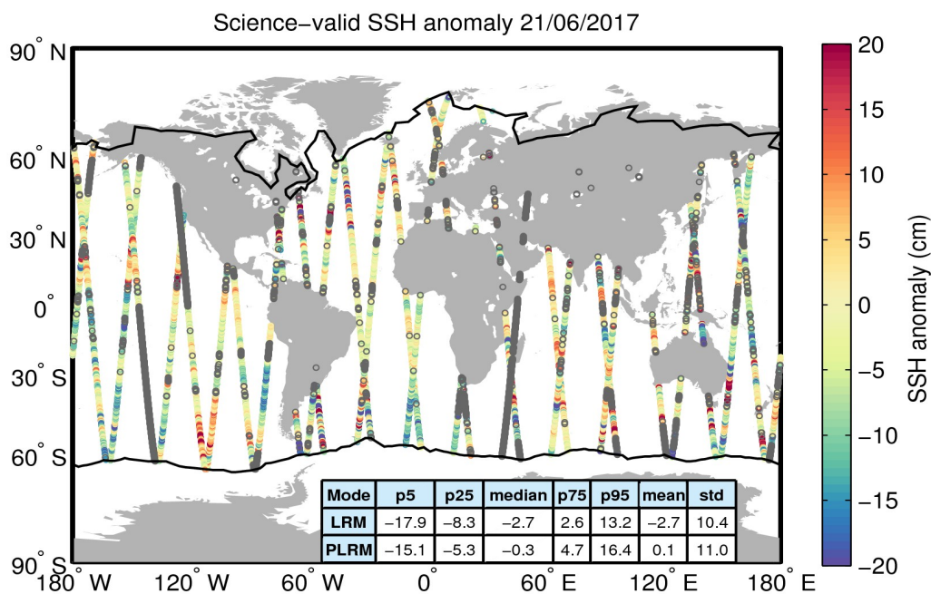
Figure 10. Geographical distribution of science-valid SSH anomaly data over oceans and lakes for 21/06/2017. The statistical values shown in the table refer to the SSH anomaly in cm and are calculated separately for LRM and PLRM regions. The black lines mark the outer limit of the Arctic and Antarctic polar polygons. Gray circles denote records that have been rejected based on the editing criteria described in Table 2.
