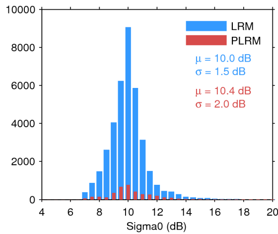
Figure 28. Histogram of science-valid sigma0 over oceans and lakes for LRM (blue) and PLRM (red) for 21/06/2017. The mean ( \mu ) and standard deviation ( \sigma ) are also shown. Note that values outside [4 20] dB are excluded from the histogram for the sake of readability but not from the computation of \mu and \sigma .
