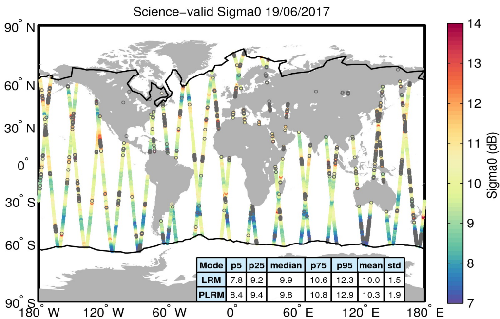
Figure 27. Geographical distribution of science-valid sigma0 data over oceans and lakes for 19/06/2017. The statistical values shown in the table refer to the sigma0 in dB and are calculated separately for LRM and PLRM regions. The black lines mark the outer limit of the Arctic and Antarctic polar polygons. Gray circles denote records that have been rejected based on the editing criteria described in Table 4.
