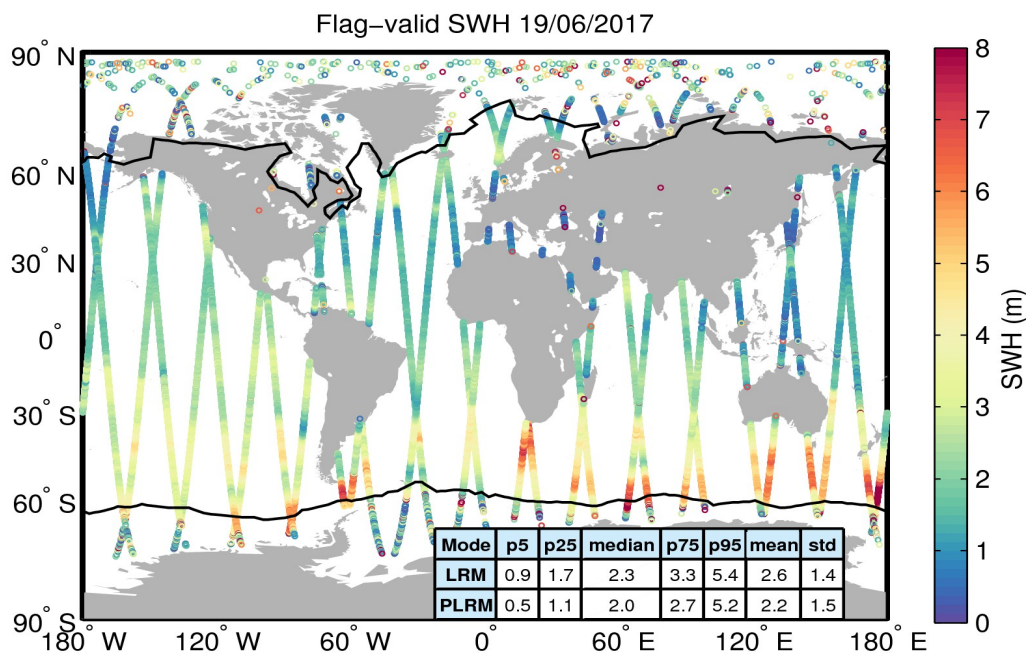
Figure 15. Geographical distribution of flag-valid SWH data over oceans and lakes for 19/06/2017. The statistical values shown in the table refer to the SWH in m and are calculated separately for LRM and PLRM regions. Measurements taken over polar polygons have been excluded from the computation of the statistical values. The black lines mark the outer limit of the Arctic and Antarctic polar polygons.
