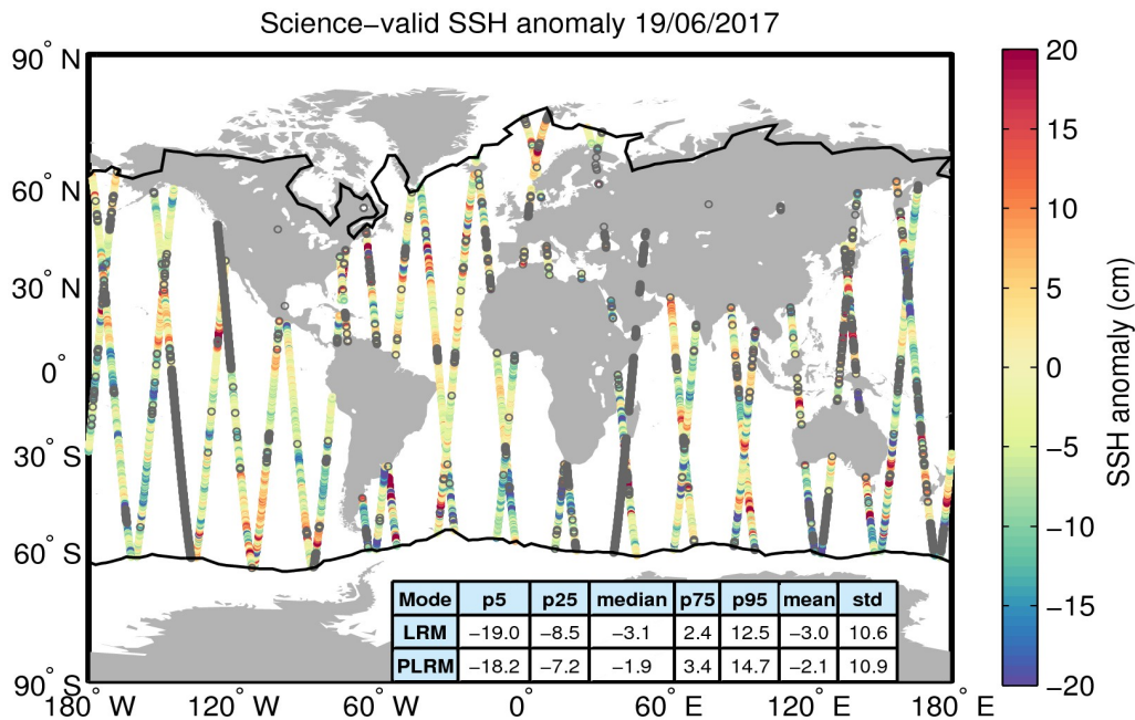
Figure 10. Geographical distribution of science-valid SSH anomaly data over oceans and lakes for 19/06/2017. The statistical values shown in the table refer to the SSH anomaly in cm and are calculated separately for LRM and PLRM regions. The black lines mark the outer limit of the Arctic and Antarctic polar polygons. Gray circles denote records that have been rejected based on the editing criteria described in Table 2.
