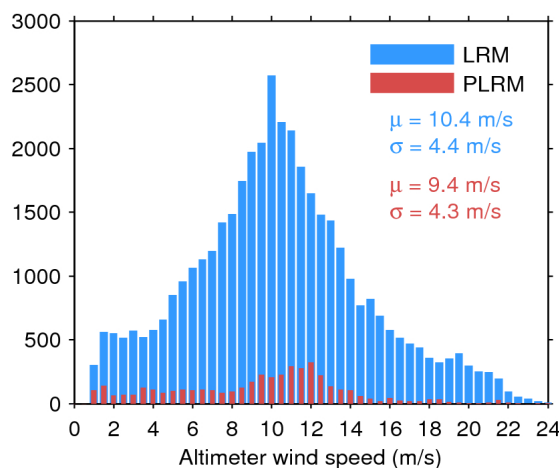
Figure 35. Histogram of science-valid wind over oceans and lakes for LRM (blue) and PLRM (red) for 19/06/2017. The mean ( \mu ) and standard deviation ( \sigma ) are also shown. Note that values larger than 24 m/s are excluded from the histogram for the sake of readability but not from the computation of \mu and \sigma .
