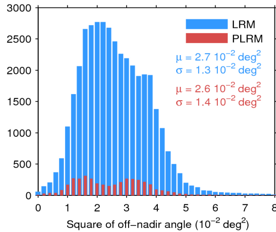
Figure 39. Histogram of flag-valid mispointing over oceans and lakes for LRM (blue) and PLRM (red) for 19/06/2017. Only positive values have been considered. The mean ( \mu ) and standard deviation ( \sigma ) are also shown. Note that values larger than 8 \cdot 10^{-2} \text{ deg}^2 are excluded from the histogram for the sake of readability but not from the computation of \mu and \sigma .
