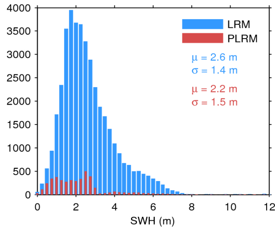
Figure 17. Histogram of flag-valid SWH over oceans and lakes for LRM (blue) and PLRM (red) for 19/06/2017. The mean ( \mu ) and standard deviation ( \sigma ) are also shown. Note that values larger than 12 m are excluded from the histogram for the sake of readability but not from the computation of \mu and \sigma .
