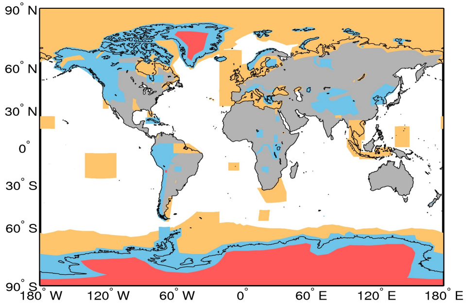
Figure A1. Extent of the regions defining the geographical mode mask for 19/06/2017. The regions where SAR, and SARIn are operated are denoted by the orange and blue polygons, respectively. LRM is operated over areas of the continental ice sheets (red polygons) and over oceans and land not covered by other modes.
