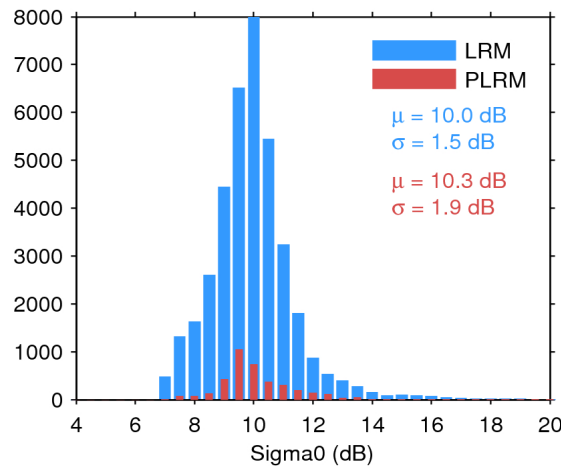
Figure 28. Histogram of science-valid sigma0 over oceans and lakes for LRM (blue) and PLRM (red) for 19/06/2017. The mean ( \mu ) and standard deviation ( \sigma ) are also shown. Note that values outside [4 20] dB are excluded from the histogram for the sake of readability but not from the computation of \mu and \sigma .
