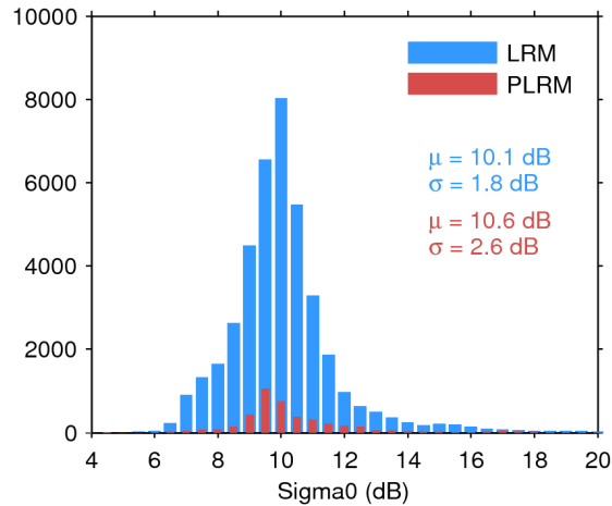
Figure 25. Histogram of flag-valid sigma0 over oceans and lakes for LRM (blue) and PLRM (red) for 19/06/2017. The mean ( \mu ) and standard deviation ( \sigma ) are also shown. Note that values outside [4 20] dB are excluded from the histogram for the sake of readability but not from the computation of \mu and \sigma .
