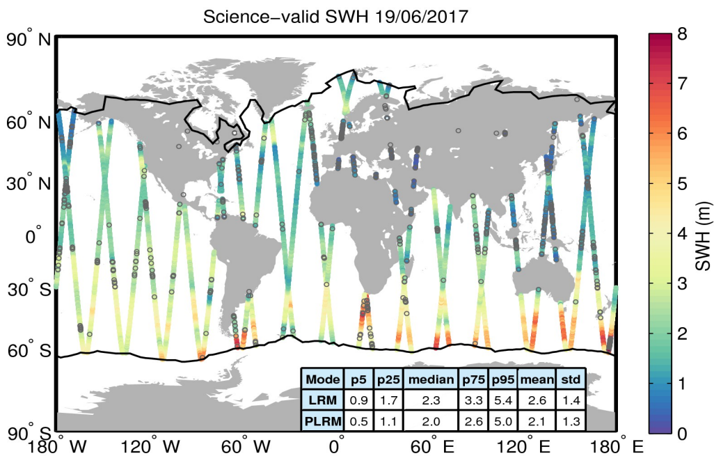
Figure 19. Geographical distribution of science-valid SWH data over oceans and lakes for 19/06/2017. The statistical values shown in the table refer to the SWH in m and are calculated separately for LRM and PLRM regions. The black lines mark the outer limit of the Arctic and Antarctic polar polygons. Gray circles denote records that have been rejected based on the editing criteria described in Table 3.
