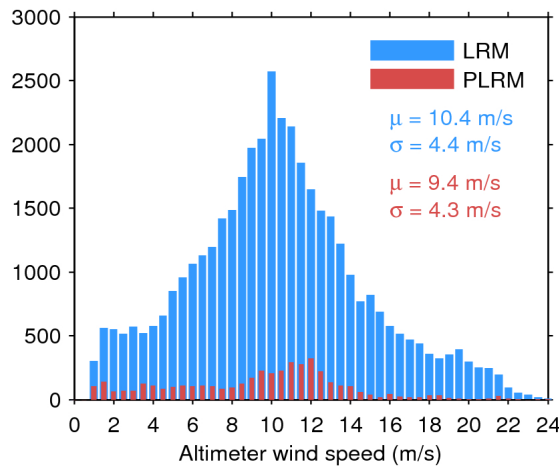
Figure 33. Histogram of flag-valid wind over oceans and lakes for LRM (blue) and PLRM (red) for 19/06/2017. The mean ( \mu ) and standard deviation ( \sigma ) are also shown. Note that values larger than 24 m/s are excluded from the histogram for the sake of readability but not from the computation of \mu and \sigma .
