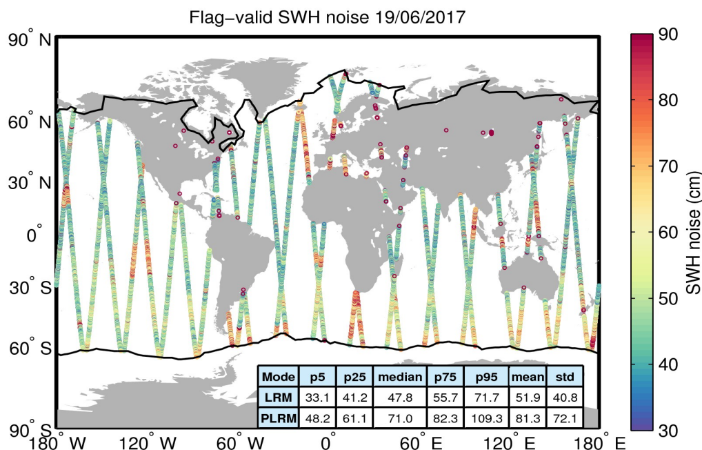
Figure 18. Geographical distribution of flag-valid 20-Hz SWH measurement noise over oceans and lakes for 19/06/2017. The statistical values shown in the table refer to the SWH noise and are calculated separately for LRM and PLRM regions. Measurements taken over polar polygons have been excluded from the computation of the statistical values. The black lines mark the outer limit of the Arctic and Antarctic polar polygons.
