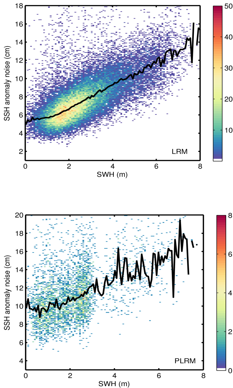
Figure 9. 2D histogram showing flag-valid SSH anomaly noise as a function of SWH for LRM (top) and PLRM (bottom) for 19/06/2017. The black line denotes the median SSH anomaly noise as a function of SWH.
