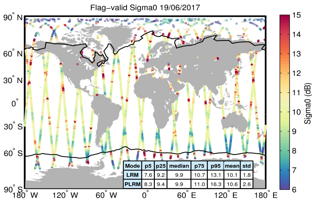
Figure 23. Geographical distribution of flag-valid sigma0 data over oceans and lakes for 19/06/2017. The statistical values shown in the table refer to the sigma0 in dB and are calculated separately for LRM and PLRM regions. Measurements taken over polar polygons have been excluded from the computation of the statistical values. The black lines mark the outer limit of the Arctic and Antarctic polar polygons.
