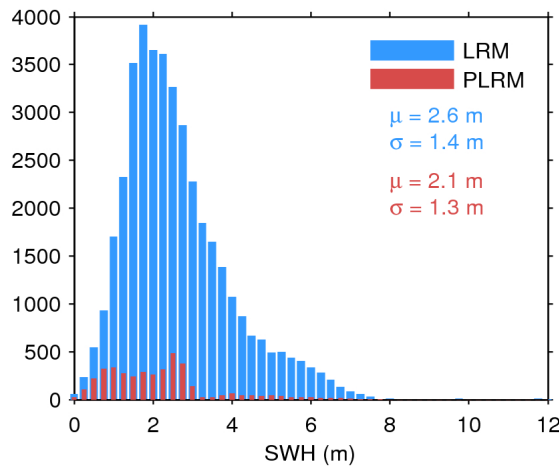
Figure 20. Histogram of science-valid SWH over oceans and lakes for LRM (blue) and PLRM (red) for 19/06/2017. The mean ( \mu ) and standard deviation ( \sigma ) are also shown. Note that values larger than 12 m are excluded from the histogram for the sake of readability but not from the computation of \mu and \sigma .
