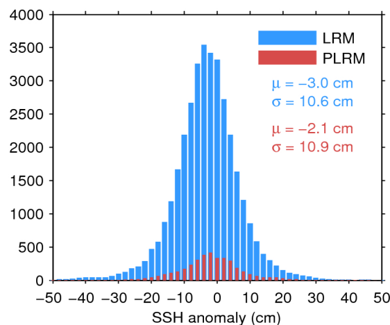
Figure 11. Histogram of science-valid SSH anomaly over oceans and lakes for LRM (blue) and PLRM (red) for 19/06/2017. The mean ( \mu ) and standard deviation ( \sigma ) are also shown. Note that values outside [-50 50] cm are excluded from the histogram for the sake of readability but not from the computation of \mu and \sigma .
