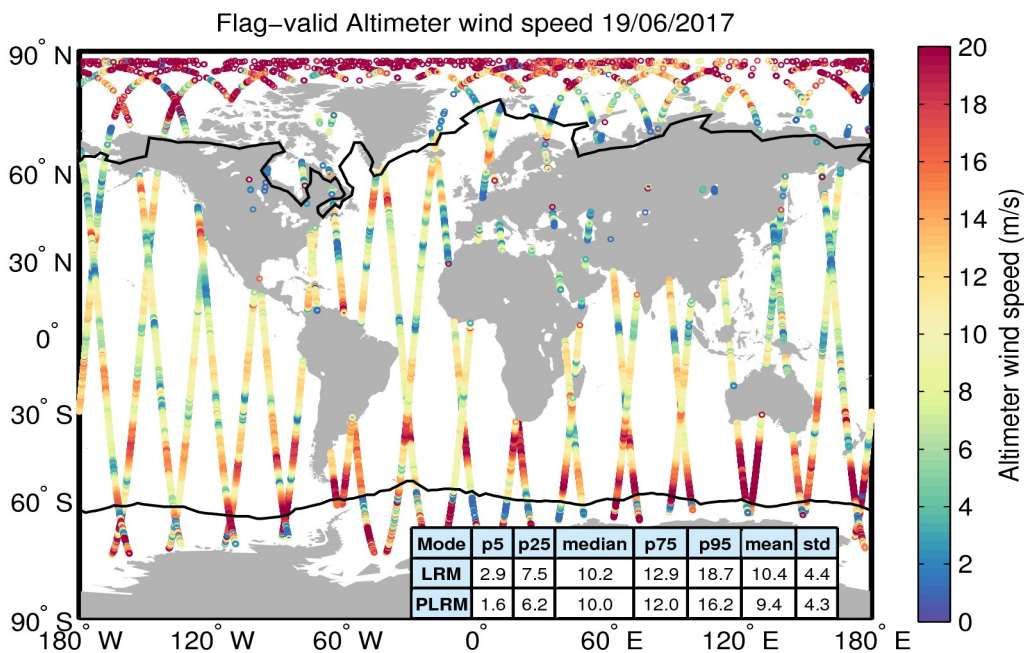
Figure 31. Geographical distribution of flag-valid wind data over oceans and lakes for 19/06/2017. The statistical values shown in the table refer to the wind in m/s and are calculated separately for LRM and PLRM regions. Measurements taken over polar polygons have been excluded from the computation of the statistical values. The black lines mark the outer limit of the Arctic and Antarctic polar polygons.
