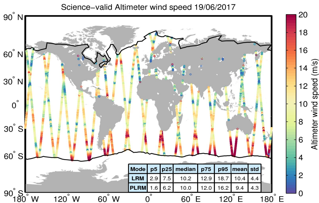
Figure 34. Geographical distribution of science-valid wind data over oceans and lakes for 19/06/2017. The statistical values shown in the table refer to the wind in m/s and are calculated separately for LRM and PLRM regions. The black lines mark the outer limit of the Arctic and Antarctic polar polygons. Gray circles denote records that have been rejected based on the editing criteria described in Table 5.
