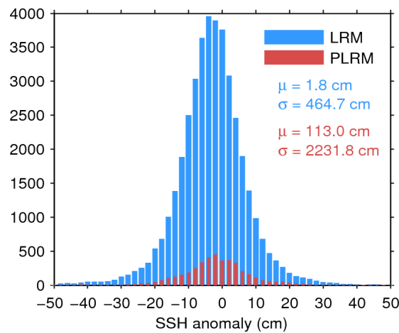
Figure 7. Histogram of flag-valid SSH anomaly over oceans and lakes for LRM (blue) and PLRM (red) for 19/06/2017. The mean ( \mu ) and standard deviation ( \sigma ) are also shown. Note that values outside [-50 \ 50] cm are excluded from the histogram for the sake of readability but not from the computation of \mu and \sigma .
