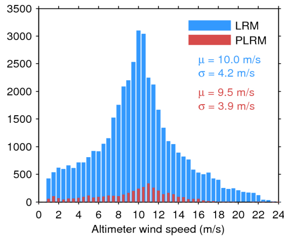
Figure 33. Histogram of flag-valid wind over oceans and lakes for LRM (blue) and PLRM (red) for 18/06/2017. The mean ( \mu ) and standard deviation ( \sigma ) are also shown. Note that values larger than 24 m/s are excluded from the histogram for the sake of readability but not from the computation of \mu and \sigma .
