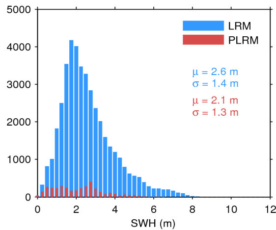
Figure 20. Histogram of science-valid SWH over oceans and lakes for LRM (blue) and PLRM (red) for 18/06/2017. The mean ( \mu ) and standard deviation ( \sigma ) are also shown. Note that values larger than 12 m are excluded from the histogram for the sake of readability but not from the computation of \mu and \sigma .
