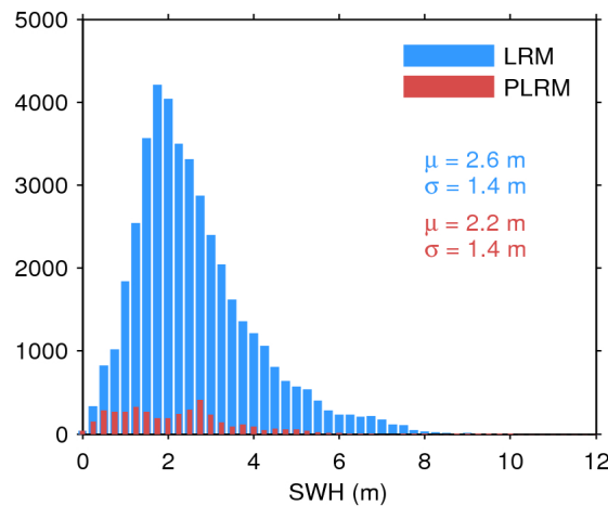
Figure 17. Histogram of flag-valid SWH over oceans and lakes for LRM (blue) and PLRM (red) for 18/06/2017. The mean ( \mu ) and standard deviation ( \sigma ) are also shown. Note that values larger than 12 m are excluded from the histogram for the sake of readability but not from the computation of \mu and \sigma .
