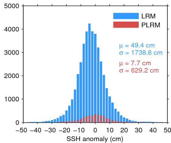
Figure 7. Histogram of flag-valid SSH anomaly over oceans and lakes for LRM (blue) and PLRM (red) for 18/06/2017. The mean ( \mu ) and standard deviation ( \sigma ) are also shown. Note that values outside [-50 50] cm are excluded from the histogram for the sake of readability but not from the computation of \mu and \sigma .
