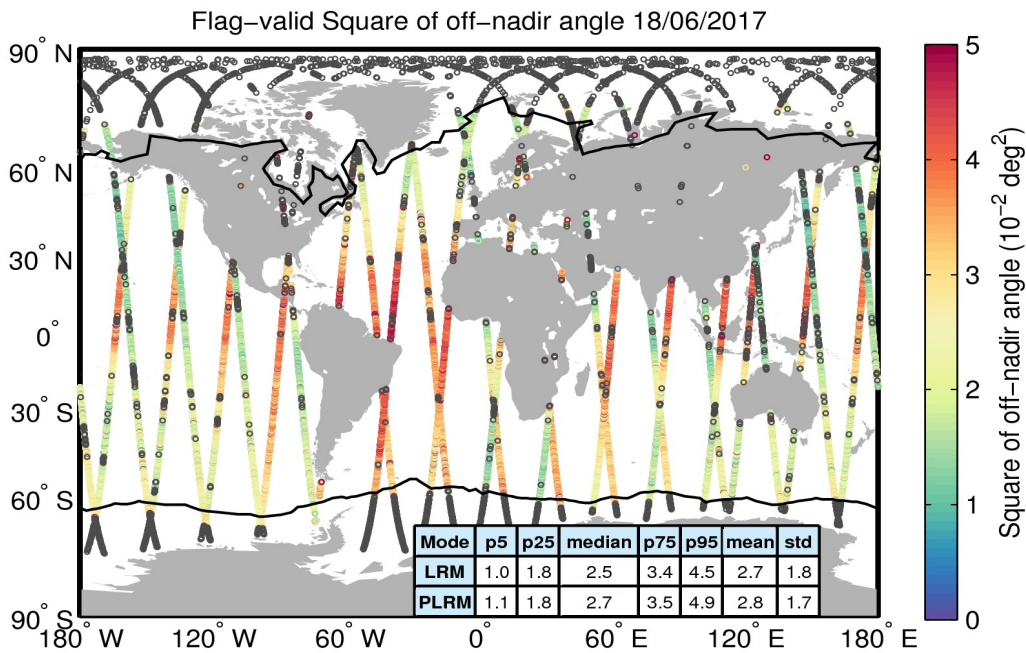
Figure 37. Geographical distribution of flag-valid mispointing data over oceans and lakes for 18/06/2017. The statistical values shown in the table refer to the mispointing in 10^{-2} \text{ deg}^2 and are calculated separately for LRM and PLRM regions. Measurements taken over polar polygons have been excluded from the computation of the statistical values. The black lines mark the outer limit of the Arctic and Antarctic polar polygons. Gray circles denote negative values.
