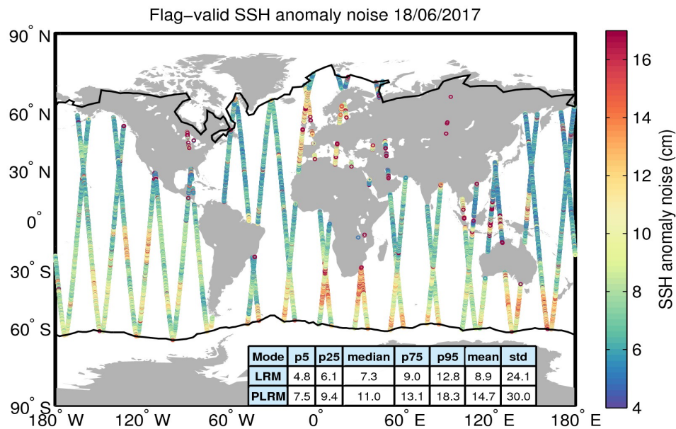
Figure 8. Geographical distribution of flag-valid 20-Hz SSH anomaly measurement noise over oceans and lakes for 18/06/2017. The statistical values shown in the table refer to the SSH anomaly noise and are calculated separately for LRM and PLRM regions. Measurements taken over polar polygons have been excluded from the computation of the statistical values. The black lines mark the outer limit of the Arctic and Antarctic polar polygons.
