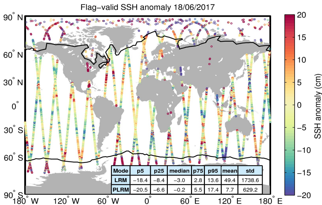
Figure 5. Geographical distribution of flag-valid 1-Hz SSH anomaly data over oceans and lakes for 18/06/2017. The statistical values shown in the table refer to the SSH anomaly in cm and are calculated separately for LRM and PLRM regions. Measurements taken over polar polygons have been excluded from the computation of the statistical values. The black lines mark the outer limit of the Arctic and Antarctic polar polygons.
