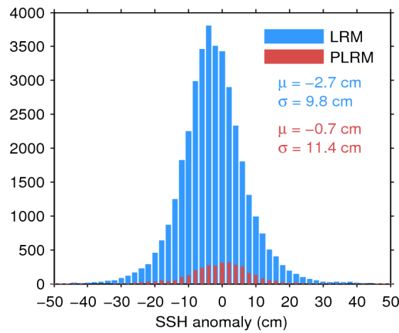
Figure 11. Histogram of science-valid SSH anomaly over oceans and lakes for LRM (blue) and PLRM (red) for 18/06/2017. The mean ( \mu ) and standard deviation ( \sigma ) are also shown. Note that values outside [-50 50] cm are excluded from the histogram for the sake of readability but not from the computation of \mu and \sigma .
