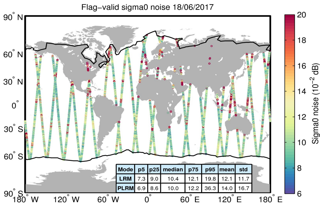
Figure 26. Geographical distribution of flag-valid 20-Hz sigma0 measurement noise over oceans and lakes for 18/06/2017. The statistical values shown in the table refer to the sigma0 noise and are calculated separately for LRM and PLRM regions. Measurements taken over polar polygons have been excluded from the computation of the statistical values. The black lines mark the outer limit of the Arctic and Antarctic polar polygons.
