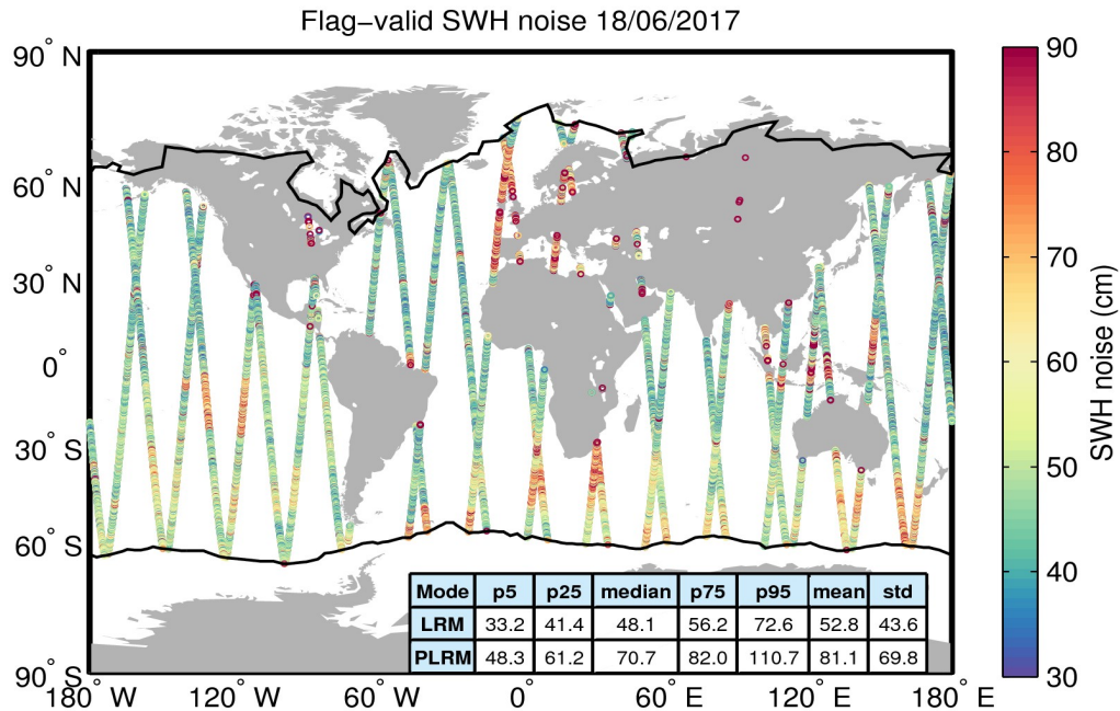
Figure 18. Geographical distribution of flag-valid 20-Hz SWH measurement noise over oceans and lakes for 18/06/2017. The statistical values shown in the table refer to the SWH noise and are calculated separately for LRM and PLRM regions. Measurements taken over polar polygons have been excluded from the computation of the statistical values. The black lines mark the outer limit of the Arctic and Antarctic polar polygons.
