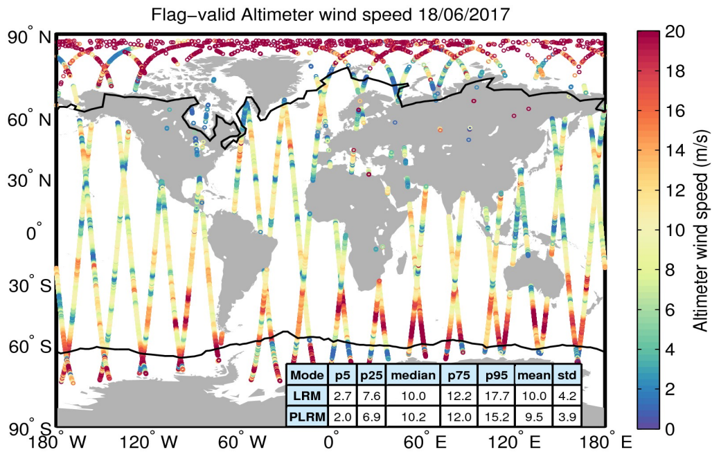
Figure 31. Geographical distribution of flag-valid wind data over oceans and lakes for 18/06/2017. The statistical values shown in the table refer to the wind in m/s and are calculated separately for LRM and PLRM regions. Measurements taken over polar polygons have been excluded from the computation of the statistical values. The black lines mark the outer limit of the Arctic and Antarctic polar polygons.
