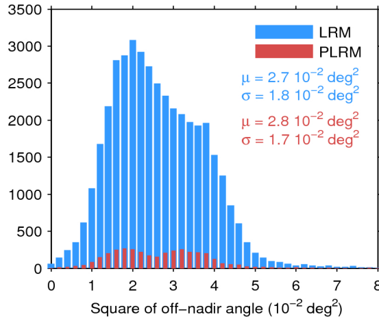
Figure 39. Histogram of flag-valid mispointing over oceans and lakes for LRM (blue) and PLRM (red) for 18/06/2017. Only positive values have been considered. The mean ( \mu ) and standard deviation ( \sigma ) are also shown. Note that values larger than 8 \cdot 10^{-2} \text{ deg}^2 are excluded from the histogram for the sake of readability but not from the computation of \mu and \sigma .
