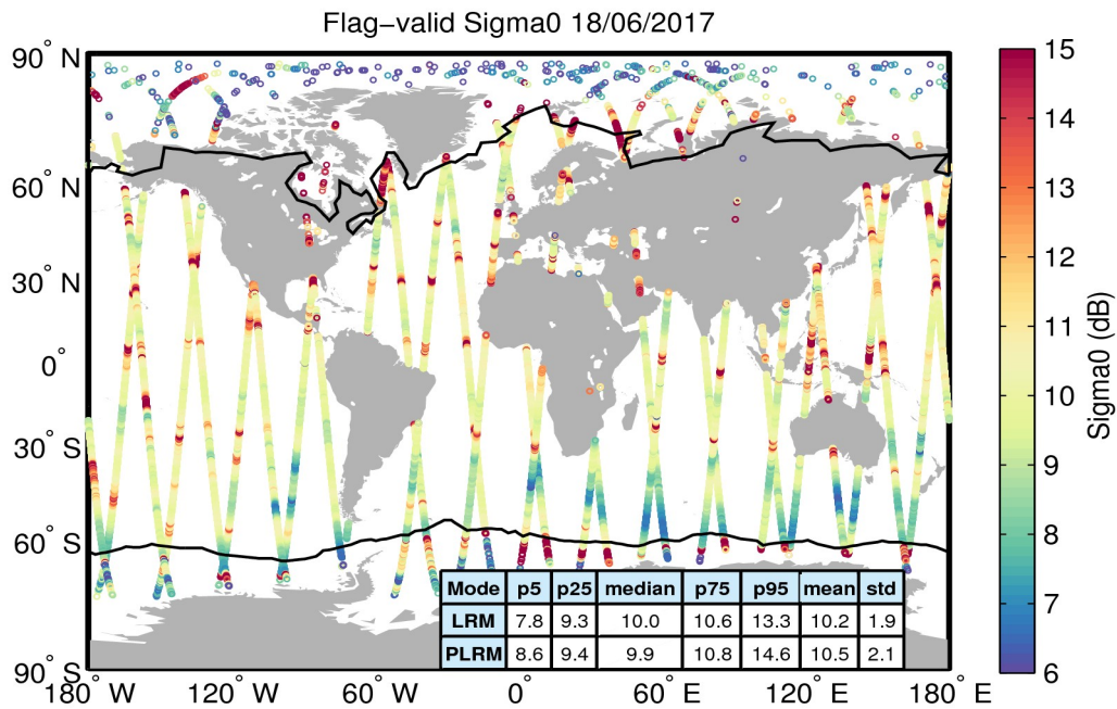
Figure 23. Geographical distribution of flag-valid sigma0 data over oceans and lakes for 18/06/2017. The statistical values shown in the table refer to the sigma0 in dB and are calculated separately for LRM and PLRM regions. Measurements taken over polar polygons have been excluded from the computation of the statistical values. The black lines mark the outer limit of the Arctic and Antarctic polar polygons.
