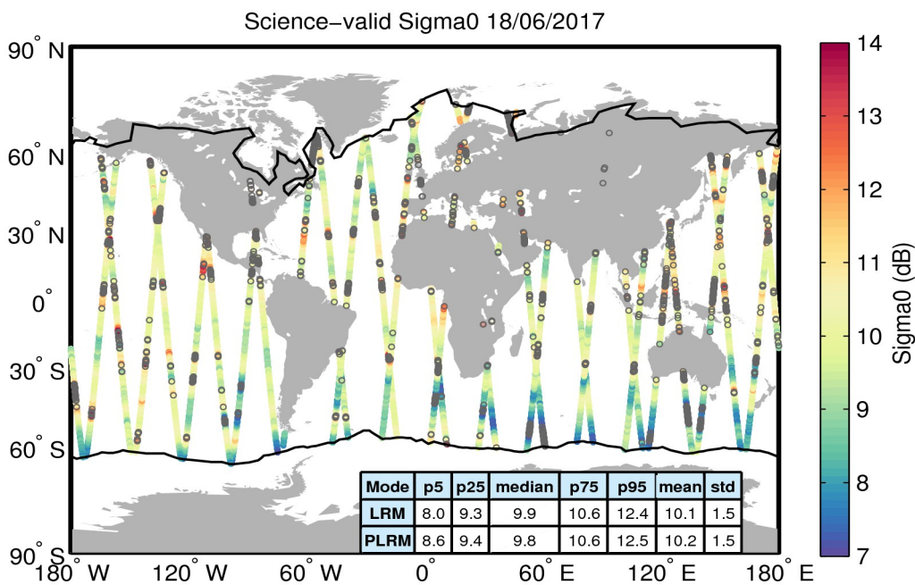
Figure 27. Geographical distribution of science-valid sigma0 data over oceans and lakes for 18/06/2017. The statistical values shown in the table refer to the sigma0 in dB and are calculated separately for LRM and PLRM regions. The black lines mark the outer limit of the Arctic and Antarctic polar polygons. Gray circles denote records that have been rejected based on the editing criteria described in Table 4.
