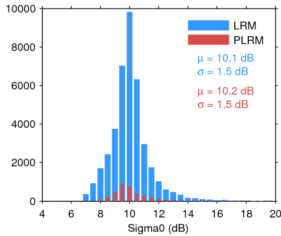
Figure 28. Histogram of science-valid sigma0 over oceans and lakes for LRM (blue) and PLRM (red) for 18/06/2017. The mean ( \mu ) and standard deviation ( \sigma ) are also shown. Note that values outside [4 20] dB are excluded from the histogram for the sake of readability but not from the computation of \mu and \sigma .
