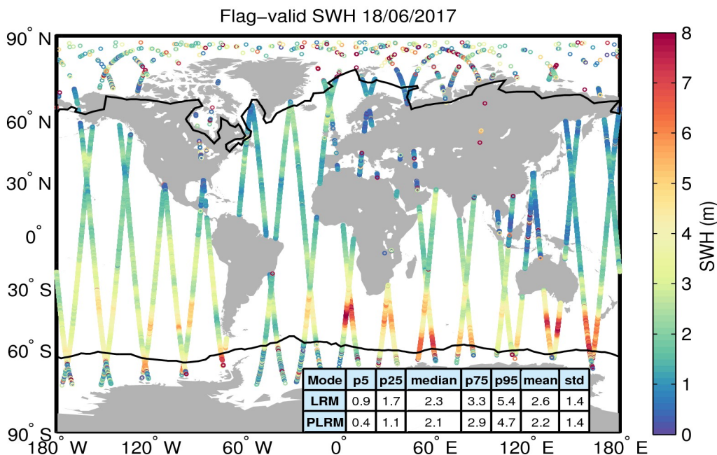
Figure 15. Geographical distribution of flag-valid SWH data over oceans and lakes for 18/06/2017. The statistical values shown in the table refer to the SWH in m and are calculated separately for LRM and PLRM regions. Measurements taken over polar polygons have been excluded from the computation of the statistical values. The black lines mark the outer limit of the Arctic and Antarctic polar polygons.
