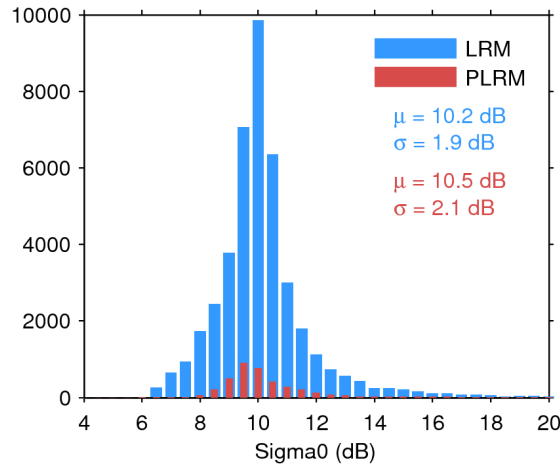
Figure 25. Histogram of flag-valid sigma0 over oceans and lakes for LRM (blue) and PLRM (red) for 18/06/2017. The mean ( \mu ) and standard deviation ( \sigma ) are also shown. Note that values outside [4 20] dB are excluded from the histogram for the sake of readability but not from the computation of \mu and \sigma .
