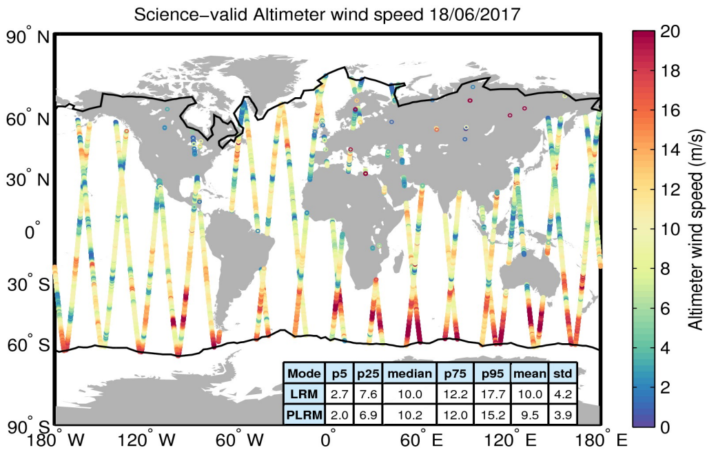
Figure 34. Geographical distribution of science-valid wind data over oceans and lakes for 18/06/2017. The statistical values shown in the table refer to the wind in m/s and are calculated separately for LRM and PLRM regions. The black lines mark the outer limit of the Arctic and Antarctic polar polygons. Gray circles denote records that have been rejected based on the editing criteria described in Table 5.
