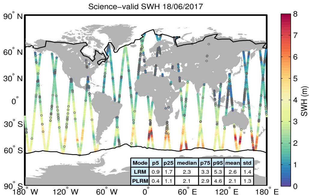
Figure 19. Geographical distribution of science-valid SWH data over oceans and lakes for 18/06/2017. The statistical values shown in the table refer to the SWH in m and are calculated separately for LRM and PLRM regions. The black lines mark the outer limit of the Arctic and Antarctic polar polygons. Gray circles denote records that have been rejected based on the editing criteria described in Table 3.
