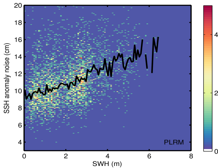
Figure 9. 2D histogram showing flag-valid SSH anomaly noise as a function of SWH for LRM (top) and PLRM (bottom) for 18/06/2017. The black line denotes the median SSH anomaly noise as a function of SWH.
