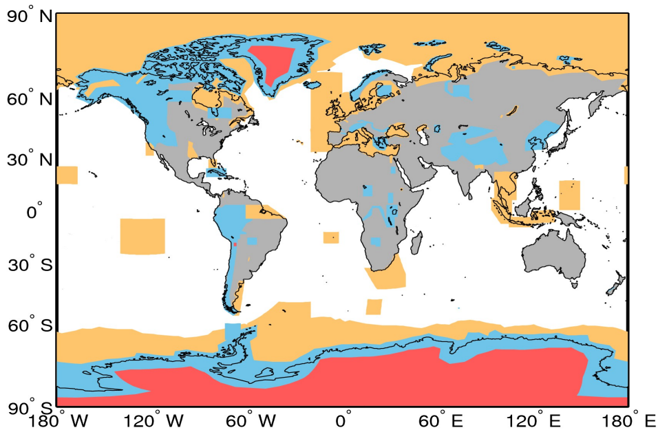
Figure A1. Extent of the regions defining the geographical mode mask for 18/06/2017. The regions where SAR, and SARIn are operated are denoted by the orange and blue polygons, respectively. LRM is operated over areas of the continental ice sheets (red polygons) and over oceans and land not covered by other modes.
