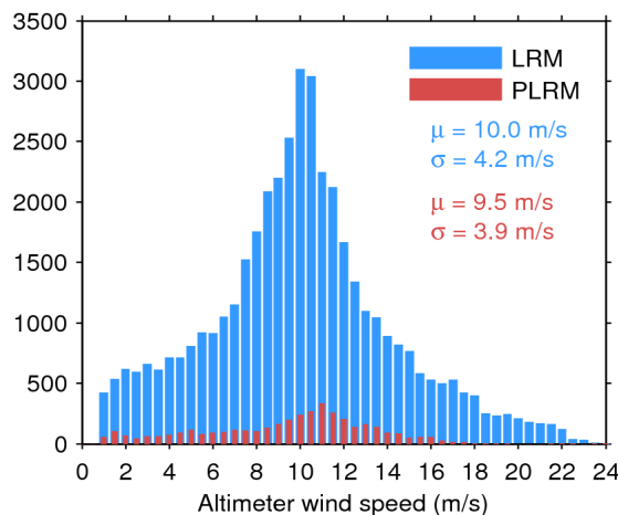
Figure 35. Histogram of science-valid wind over oceans and lakes for LRM (blue) and PLRM (red) for 18/06/2017. The mean ( \mu ) and standard deviation ( \sigma ) are also shown. Note that values larger than 24 m/s are excluded from the histogram for the sake of readability but not from the computation of \mu and \sigma .
