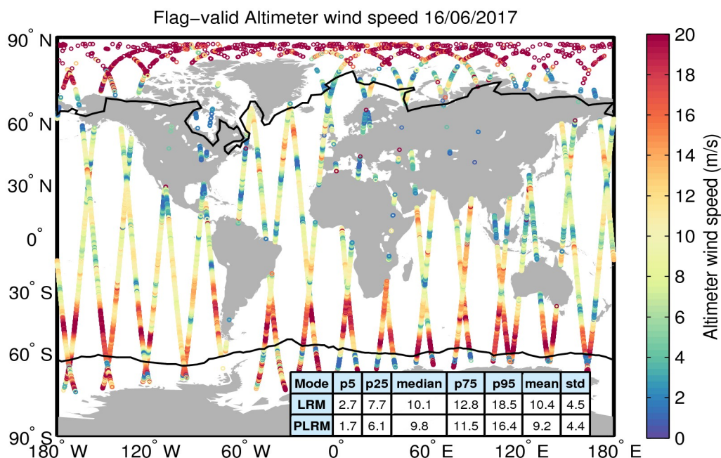
Figure 31. Geographical distribution of flag-valid wind data over oceans and lakes for 16/06/2017. The statistical values shown in the table refer to the wind in m/s and are calculated separately for LRM and PLRM regions. Measurements taken over polar polygons have been excluded from the computation of the statistical values. The black lines mark the outer limit of the Arctic and Antarctic polar polygons.
