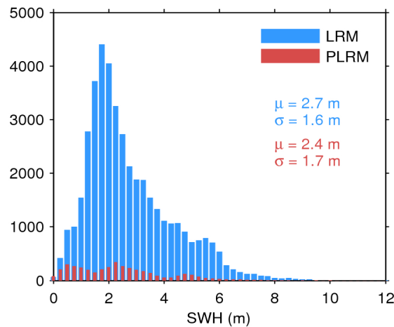
Figure 17. Histogram of flag-valid SWH over oceans and lakes for LRM (blue) and PLRM (red) for 16/06/2017. The mean ( \mu ) and standard deviation ( \sigma ) are also shown. Note that values larger than 12 m are excluded from the histogram for the sake of readability but not from the computation of \mu and \sigma .
