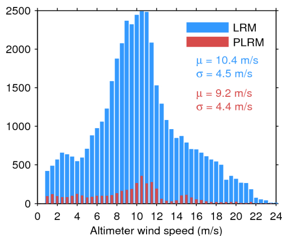
Figure 35. Histogram of science-valid wind over oceans and lakes for LRM (blue) and PLRM (red) for 16/06/2017. The mean ( \mu ) and standard deviation ( \sigma ) are also shown. Note that values larger than 24 m/s are excluded from the histogram for the sake of readability but not from the computation of \mu and \sigma .
