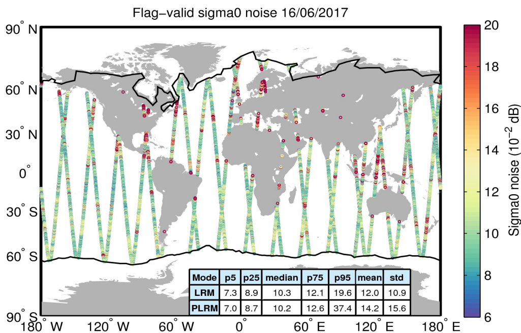
Figure 26. Geographical distribution of flag-valid 20-Hz sigma0 measurement noise over oceans and lakes for 16/06/2017. The statistical values shown in the table refer to the sigma0 noise and are calculated separately for LRM and PLRM regions. Measurements taken over polar polygons have been excluded from the computation of the statistical values. The black lines mark the outer limit of the Arctic and Antarctic polar polygons.
