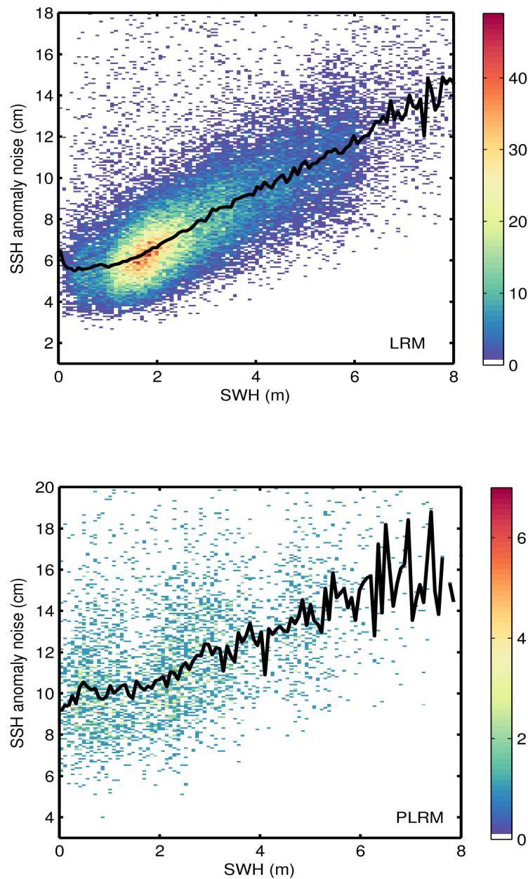
Figure 9. 2D histogram showing flag-valid SSH anomaly noise as a function of SWH for LRM (top) and PLRM (bottom) for 16/06/2017. The black line denotes the median SSH anomaly noise as a function of SWH.
