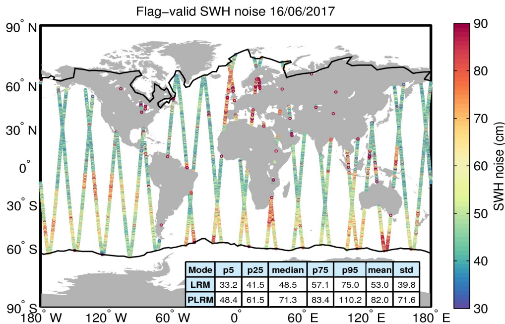
Figure 18. Geographical distribution of flag-valid 20-Hz SWH measurement noise over oceans and lakes for 16/06/2017. The statistical values shown in the table refer to the SWH noise and are calculated separately for LRM and PLRM regions. Measurements taken over polar polygons have been excluded from the computation of the statistical values. The black lines mark the outer limit of the Arctic and Antarctic polar polygons.
