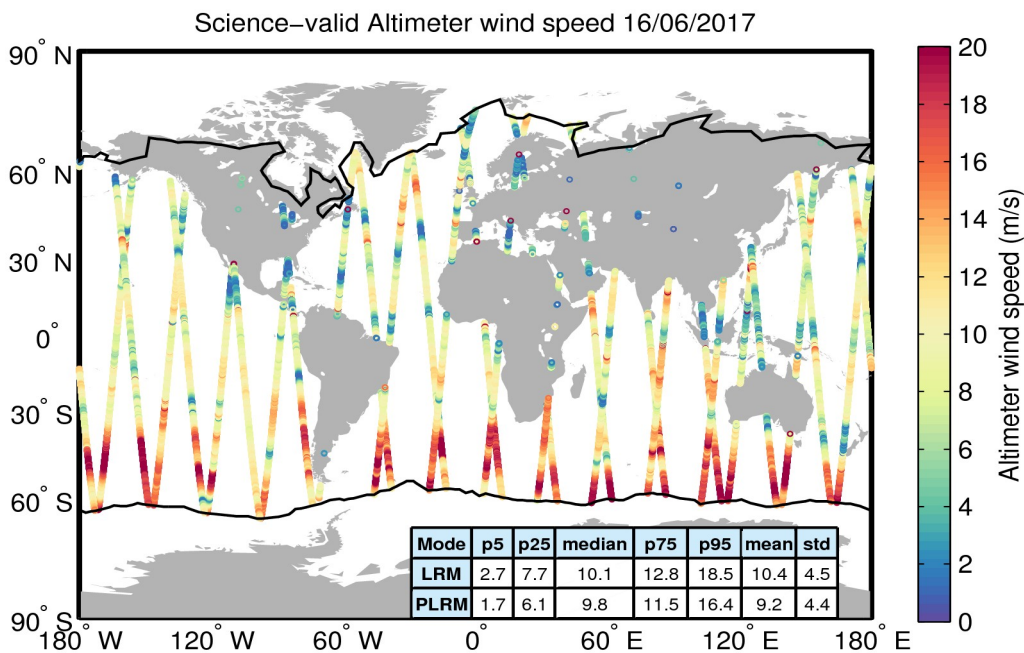
Figure 34. Geographical distribution of science-valid wind data over oceans and lakes for 16/06/2017. The statistical values shown in the table refer to the wind in m/s and are calculated separately for LRM and PLRM regions. The black lines mark the outer limit of the Arctic and Antarctic polar polygons. Gray circles denote records that have been rejected based on the editing criteria described in Table 5.
