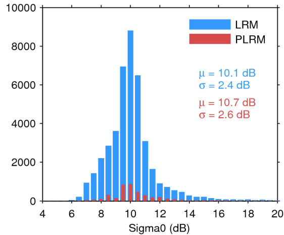
Figure 25. Histogram of flag-valid sigma0 over oceans and lakes for LRM (blue) and PLRM (red) for 16/06/2017. The mean ( \mu ) and standard deviation ( \sigma ) are also shown. Note that values outside [4 20] dB are excluded from the histogram for the sake of readability but not from the computation of \mu and \sigma .
