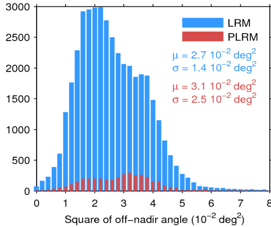
Figure 39. Histogram of flag-valid mispointing over oceans and lakes for LRM (blue) and PLRM (red) for 16/06/2017. Only positive values have been considered. The mean ( \mu ) and standard deviation ( \sigma ) are also shown. Note that values larger than 8 \cdot 10^{-2} \text{ deg}^2 are excluded from the histogram for the sake of readability but not from the computation of \mu and \sigma .
