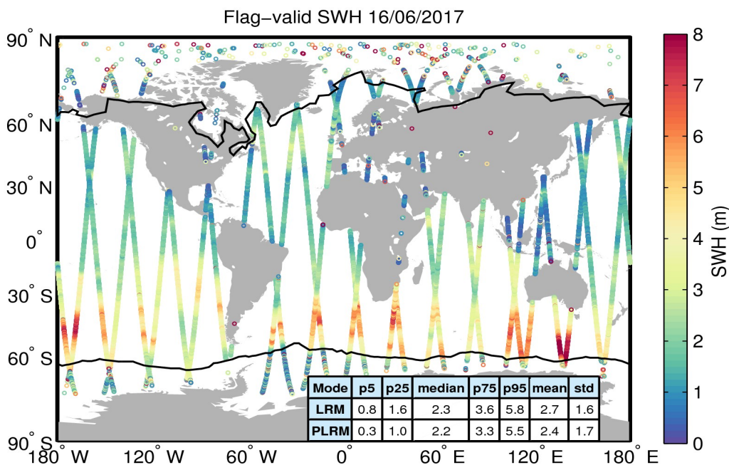
Figure 15. Geographical distribution of flag-valid SWH data over oceans and lakes for 16/06/2017. The statistical values shown in the table refer to the SWH in m and are calculated separately for LRM and PLRM regions. Measurements taken over polar polygons have been excluded from the computation of the statistical values. The black lines mark the outer limit of the Arctic and Antarctic polar polygons.
