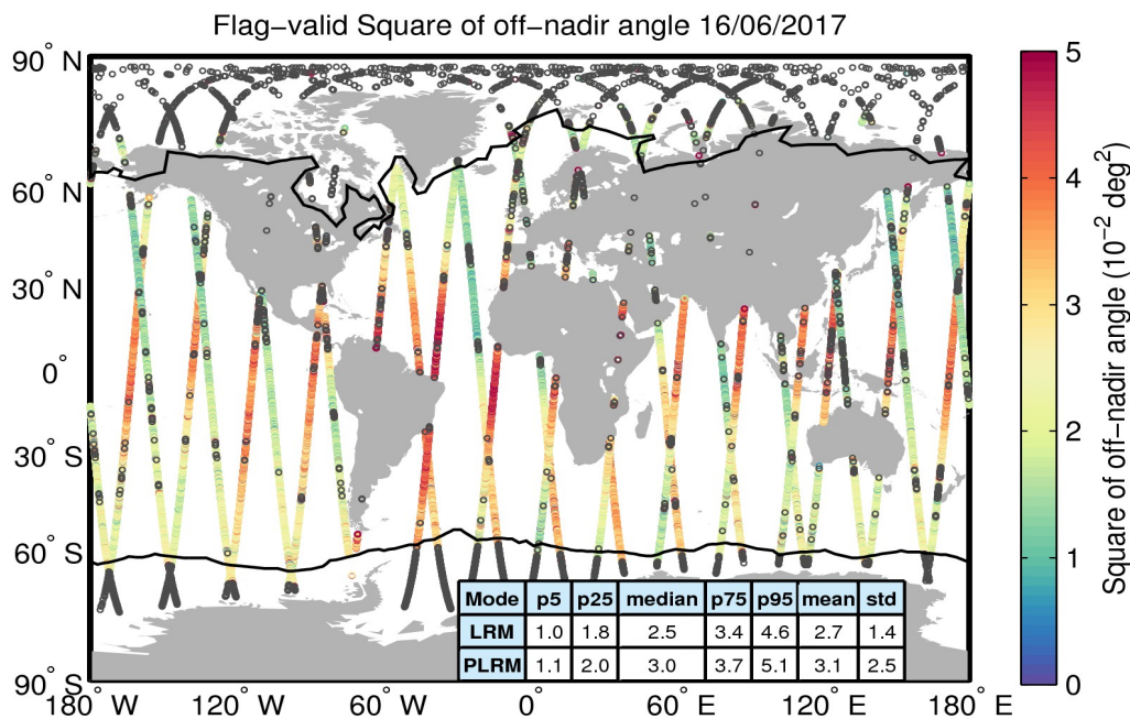
Figure 37. Geographical distribution of flag-valid mispointing data over oceans and lakes for 16/06/2017. The statistical values shown in the table refer to the mispointing in 10^{-2} deg 2 and are calculated separately for LRM and PLRM regions. Measurements taken over polar polygons have been excluded from the computation of the statistical values. The black lines mark the outer limit of the Arctic and Antarctic polar polygons. Gray circles denote negative values.
