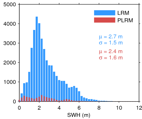
Figure 20. Histogram of science-valid SWH over oceans and lakes for LRM (blue) and PLRM (red) for 16/06/2017. The mean ( \mu ) and standard deviation ( \sigma ) are also shown. Note that values larger than 12 m are excluded from the histogram for the sake of readability but not from the computation of \mu and \sigma .
