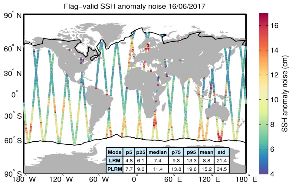
Figure 8. Geographical distribution of flag-valid 20-Hz SSH anomaly measurement noise over oceans and lakes for 16/06/2017. The statistical values shown in the table refer to the SSH anomaly noise and are calculated separately for LRM and PLRM regions. Measurements taken over polar polygons have been excluded from the computation of the statistical values. The black lines mark the outer limit of the Arctic and Antarctic polar polygons.
