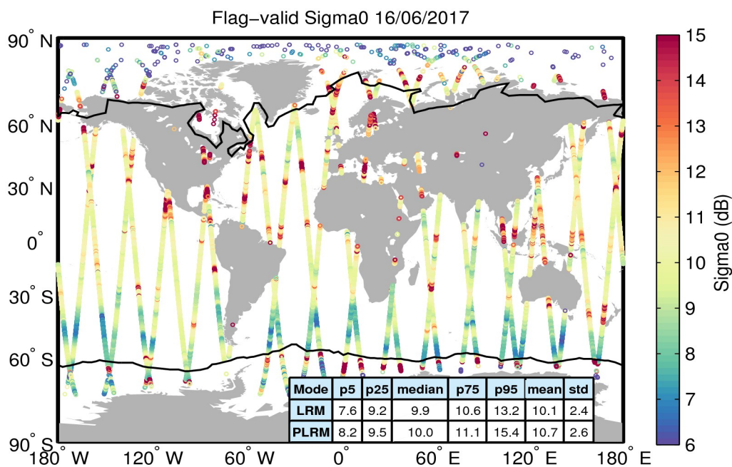
Figure 23. Geographical distribution of flag-valid sigma0 data over oceans and lakes for 16/06/2017. The statistical values shown in the table refer to the sigma0 in dB and are calculated separately for LRM and PLRM regions. Measurements taken over polar polygons have been excluded from the computation of the statistical values. The black lines mark the outer limit of the Arctic and Antarctic polar polygons.
