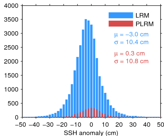
Figure 11. Histogram of science-valid SSH anomaly over oceans and lakes for LRM (blue) and PLRM (red) for 16/06/2017. The mean ( \mu ) and standard deviation ( \sigma ) are also shown. Note that values outside [-50 50] cm are excluded from the histogram for the sake of readability but not from the computation of \mu and \sigma .
