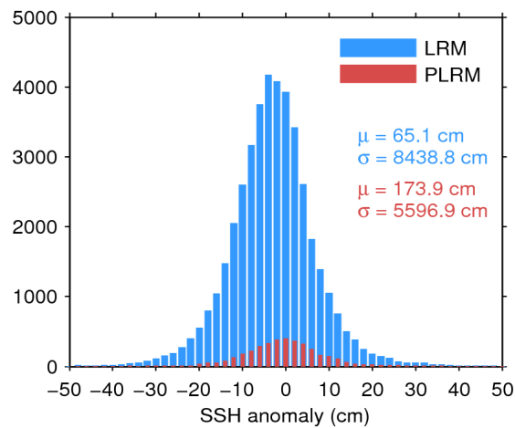
Figure 7. Histogram of flag-valid SSH anomaly over oceans and lakes for LRM (blue) and PLRM (red) for 16/06/2017. The mean ( \mu ) and standard deviation ( \sigma ) are also shown. Note that values outside [-50\ 50] cm are excluded from the histogram for the sake of readability but not from the computation of \mu and \sigma .
