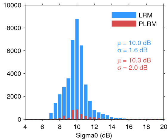
Figure 28. Histogram of science-valid sigma0 over oceans and lakes for LRM (blue) and PLRM (red) for 16/06/2017. The mean ( \mu ) and standard deviation ( \sigma ) are also shown. Note that values outside [4 20] dB are excluded from the histogram for the sake of readability but not from the computation of \mu and \sigma .
