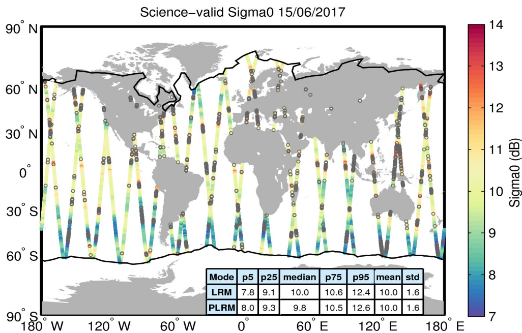
Figure 27. Geographical distribution of science-valid sigma0 data over oceans and lakes for 15/06/2017. The statistical values shown in the table refer to the sigma0 in dB and are calculated separately for LRM and PLRM regions. The black lines mark the outer limit of the Arctic and Antarctic polar polygons. Gray circles denote records that have been rejected based on the editing criteria described in Table 4.
