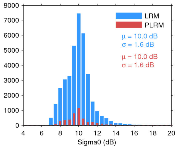
Figure 28. Histogram of science-valid sigma0 over oceans and lakes for LRM (blue) and PLRM (red) for 15/06/2017. The mean ( \mu ) and standard deviation ( \sigma ) are also shown. Note that values outside [4 20] dB are excluded from the histogram for the sake of readability but not from the computation of \mu and \sigma .
