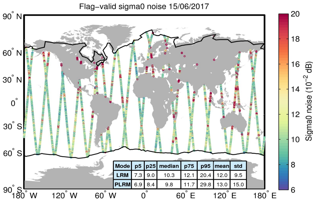
Figure 26. Geographical distribution of flag-valid 20-Hz sigma0 measurement noise over oceans and lakes for 15/06/2017. The statistical values shown in the table refer to the sigma0 noise and are calculated separately for LRM and PLRM regions. Measurements taken over polar polygons have been excluded from the computation of the statistical values. The black lines mark the outer limit of the Arctic and Antarctic polar polygons.
