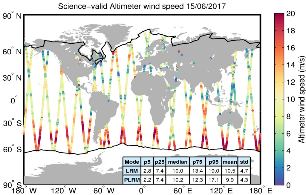
Figure 34. Geographical distribution of science-valid wind data over oceans and lakes for 15/06/2017. The statistical values shown in the table refer to the wind in m/s and are calculated separately for LRM and PLRM regions. The black lines mark the outer limit of the Arctic and Antarctic polar polygons. Gray circles denote records that have been rejected based on the editing criteria described in Table 5.
