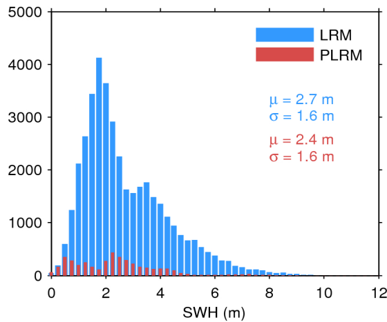
Figure 20. Histogram of science-valid SWH over oceans and lakes for LRM (blue) and PLRM (red) for 15/06/2017. The mean ( \mu ) and standard deviation ( \sigma ) are also shown. Note that values larger than 12 m are excluded from the histogram for the sake of readability but not from the computation of \mu and \sigma .
