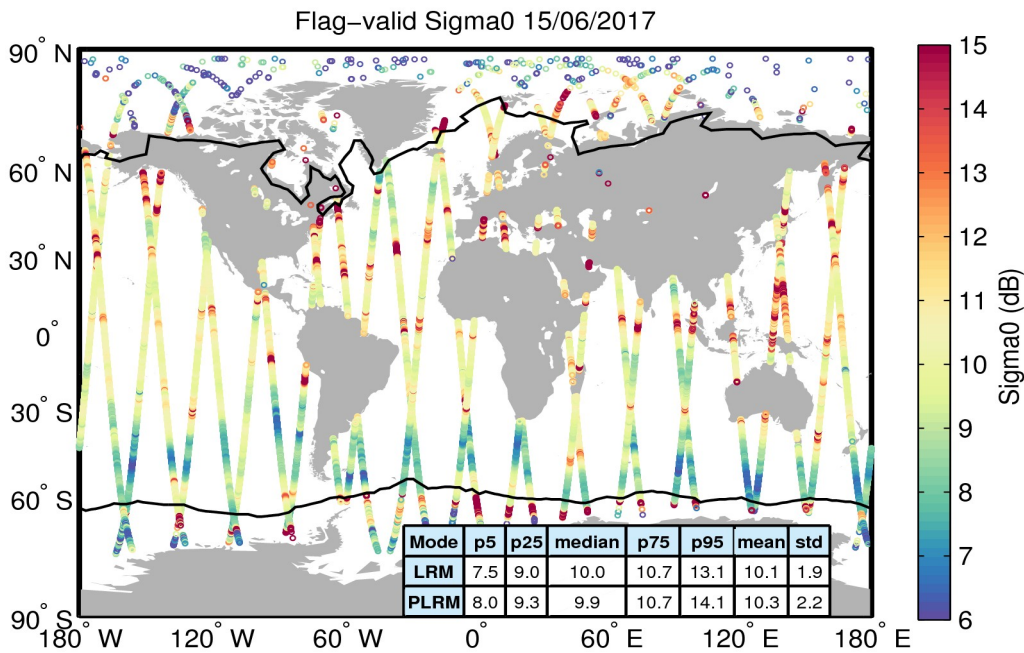
Figure 23. Geographical distribution of flag-valid sigma0 data over oceans and lakes for 15/06/2017. The statistical values shown in the table refer to the sigma0 in dB and are calculated separately for LRM and PLRM regions. Measurements taken over polar polygons have been excluded from the computation of the statistical values. The black lines mark the outer limit of the Arctic and Antarctic polar polygons.
