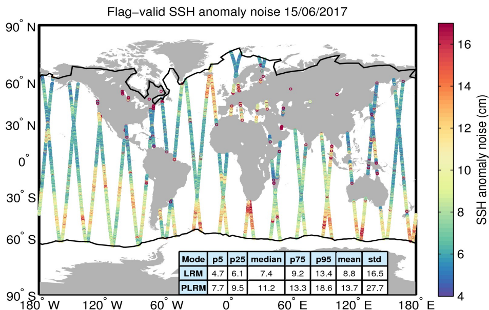
Figure 8. Geographical distribution of flag-valid 20-Hz SSH anomaly measurement noise over oceans and lakes for 15/06/2017. The statistical values shown in the table refer to the SSH anomaly noise and are calculated separately for LRM and PLRM regions. Measurements taken over polar polygons have been excluded from the computation of the statistical values. The black lines mark the outer limit of the Arctic and Antarctic polar polygons.
