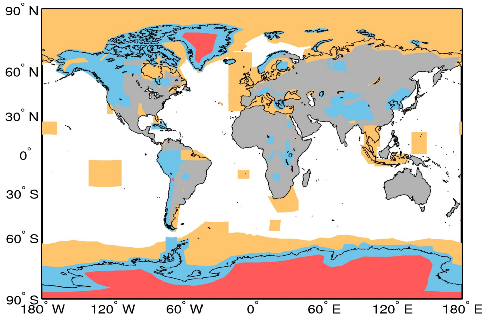
Figure A1. Extent of the regions defining the geographical mode mask for 15/06/2017. The regions where SAR, and SARIn are operated are denoted by the orange and blue polygons, respectively. LRM is operated over areas of the continental ice sheets (red polygons) and over oceans and land not covered by other modes.
