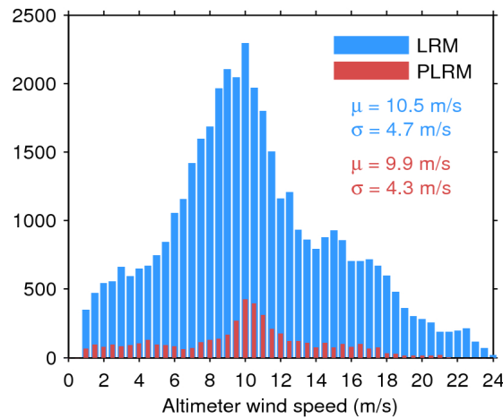
Figure 33. Histogram of flag-valid wind over oceans and lakes for LRM (blue) and PLRM (red) for 15/06/2017. The mean ( \mu ) and standard deviation ( \sigma ) are also shown. Note that values larger than 24 m/s are excluded from the histogram for the sake of readability but not from the computation of \mu and \sigma .
