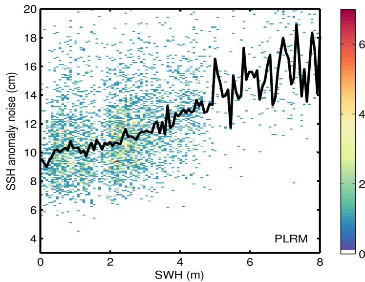
Figure 9. 2D histogram showing flag-valid SSH anomaly noise as a function of SWH for LRM (top) and PLRM (bottom) for 15/06/2017. The black line denotes the median SSH anomaly noise as a function of SWH.
