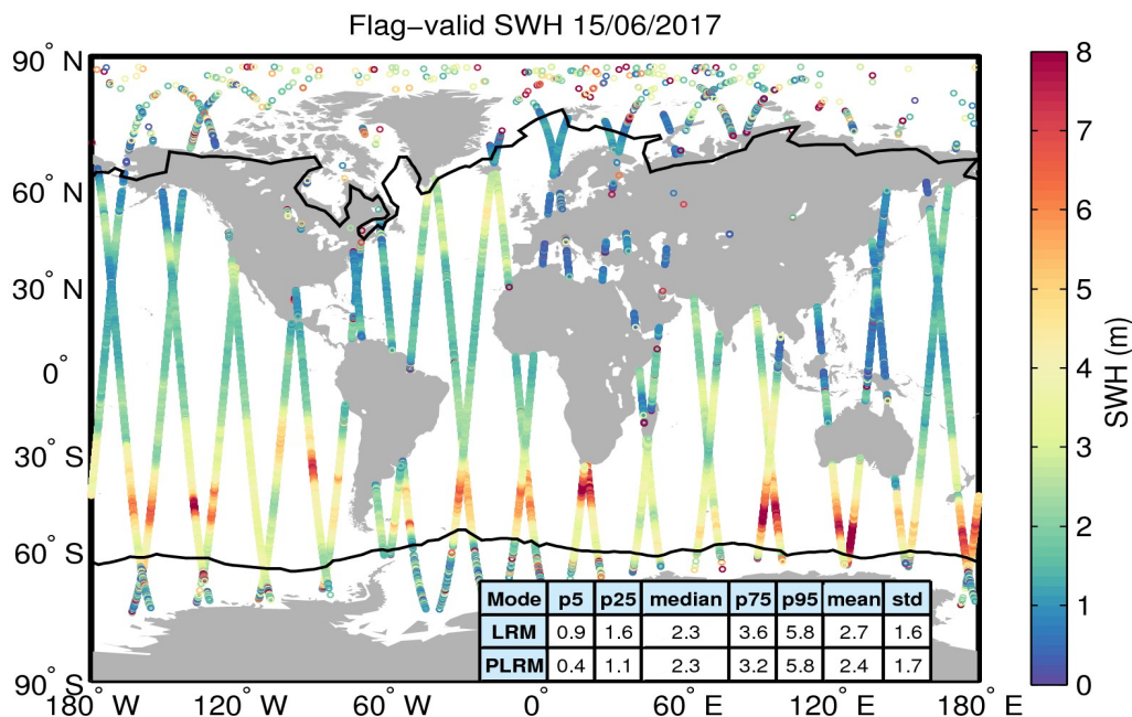
Figure 15. Geographical distribution of flag-valid SWH data over oceans and lakes for 15/06/2017. The statistical values shown in the table refer to the SWH in m and are calculated separately for LRM and PLRM regions. Measurements taken over polar polygons have been excluded from the computation of the statistical values. The black lines mark the outer limit of the Arctic and Antarctic polar polygons.
