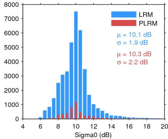
Figure 25. Histogram of flag-valid sigma0 over oceans and lakes for LRM (blue) and PLRM (red) for 15/06/2017. The mean ( \mu ) and standard deviation ( \sigma ) are also shown. Note that values outside [4 20] dB are excluded from the histogram for the sake of readability but not from the computation of \mu and \sigma .
