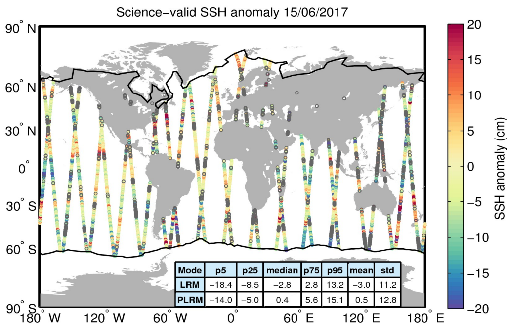
Figure 10. Geographical distribution of science-valid SSH anomaly data over oceans and lakes for 15/06/2017. The statistical values shown in the table refer to the SSH anomaly in cm and are calculated separately for LRM and PLRM regions. The black lines mark the outer limit of the Arctic and Antarctic polar polygons. Gray circles denote records that have been rejected based on the editing criteria described in Table 2.
