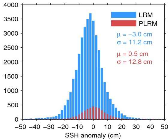
Figure 11. Histogram of science-valid SSH anomaly over oceans and lakes for LRM (blue) and PLRM (red) for 15/06/2017. The mean ( \mu ) and standard deviation ( \sigma ) are also shown. Note that values outside [-50\ 50] cm are excluded from the histogram for the sake of readability but not from the computation of \mu and \sigma .
