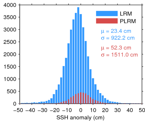
Figure 7. Histogram of flag-valid SSH anomaly over oceans and lakes for LRM (blue) and PLRM (red) for 15/06/2017. The mean ( \mu ) and standard deviation ( \sigma ) are also shown. Note that values outside [-50\ 50] cm are excluded from the histogram for the sake of readability but not from the computation of \mu and \sigma .
