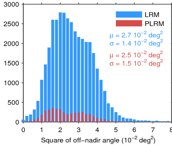
Figure 39. Histogram of flag-valid mispointing over oceans and lakes for LRM (blue) and PLRM (red) for 15/06/2017. Only positive values have been considered. The mean ( \mu ) and standard deviation ( \sigma ) are also shown. Note that values larger than 8 \cdot 10^{-2} \text{ deg}^2 are excluded from the histogram for the sake of readability but not from the computation of \mu and \sigma .
