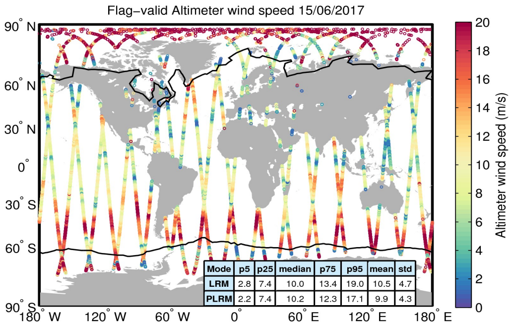
Figure 31. Geographical distribution of flag-valid wind data over oceans and lakes for 15/06/2017. The statistical values shown in the table refer to the wind in m/s and are calculated separately for LRM and PLRM regions. Measurements taken over polar polygons have been excluded from the computation of the statistical values. The black lines mark the outer limit of the Arctic and Antarctic polar polygons.
