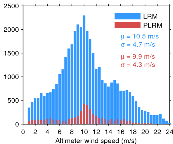
Figure 35. Histogram of science-valid wind over oceans and lakes for LRM (blue) and PLRM (red) for 15/06/2017. The mean ( \mu ) and standard deviation ( \sigma ) are also shown. Note that values larger than 24 m/s are excluded from the histogram for the sake of readability but not from the computation of \mu and \sigma .
