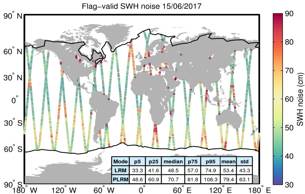
Figure 18. Geographical distribution of flag-valid 20-Hz SWH measurement noise over oceans and lakes for 15/06/2017. The statistical values shown in the table refer to the SWH noise and are calculated separately for LRM and PLRM regions. Measurements taken over polar polygons have been excluded from the computation of the statistical values. The black lines mark the outer limit of the Arctic and Antarctic polar polygons.
