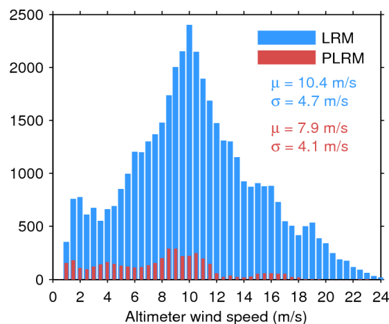
Figure 35. Histogram of science-valid wind over oceans and lakes for LRM (blue) and PLRM (red) for 14/06/2017. The mean ( \mu ) and standard deviation ( \sigma ) are also shown. Note that values larger than 24 m/s are excluded from the histogram for the sake of readability but not from the computation of \mu and \sigma .
