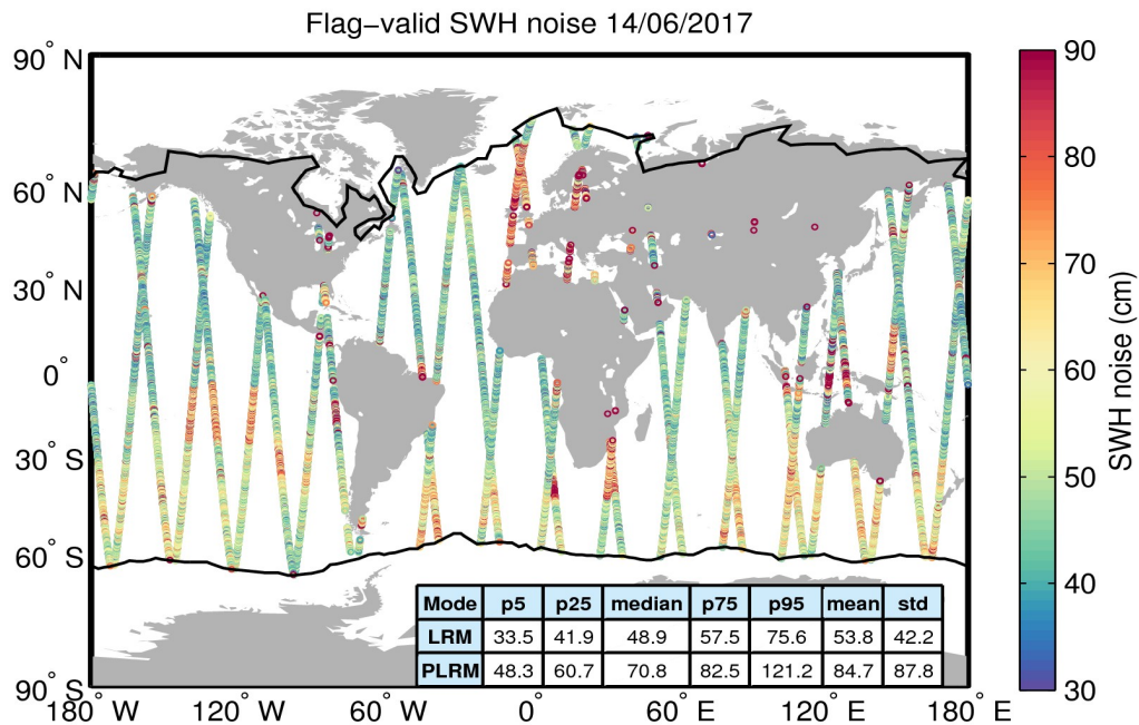
Figure 18. Geographical distribution of flag-valid 20-Hz SWH measurement noise over oceans and lakes for 14/06/2017. The statistical values shown in the table refer to the SWH noise and are calculated separately for LRM and PLRM regions. Measurements taken over polar polygons have been excluded from the computation of the statistical values. The black lines mark the outer limit of the Arctic and Antarctic polar polygons.
