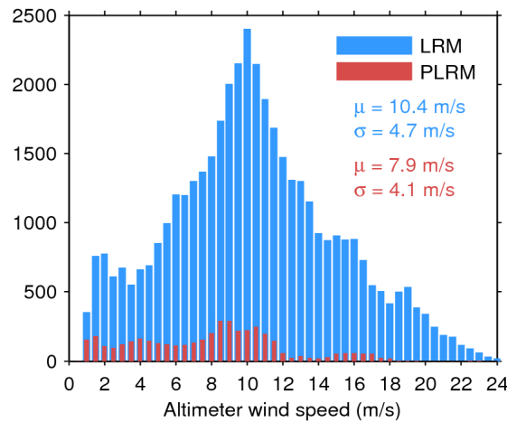
Figure 33. Histogram of flag-valid wind over oceans and lakes for LRM (blue) and PLRM (red) for 14/06/2017. The mean ( \mu ) and standard deviation ( \sigma ) are also shown. Note that values larger than 24 m/s are excluded from the histogram for the sake of readability but not from the computation of \mu and \sigma .
