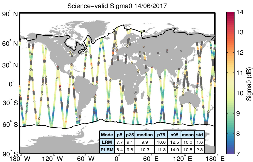
Figure 27. Geographical distribution of science-valid sigma0 data over oceans and lakes for 14/06/2017. The statistical values shown in the table refer to the sigma0 in dB and are calculated separately for LRM and PLRM regions. The black lines mark the outer limit of the Arctic and Antarctic polar polygons. Gray circles denote records that have been rejected based on the editing criteria described in Table 4.
