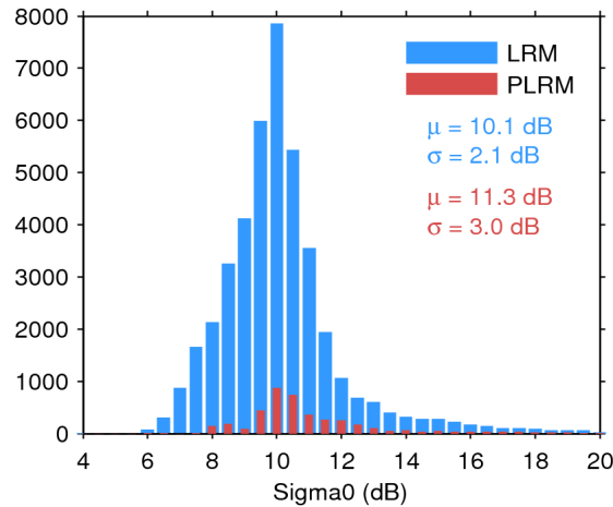
Figure 25. Histogram of flag-valid sigma0 over oceans and lakes for LRM (blue) and PLRM (red) for 14/06/2017. The mean ( \mu ) and standard deviation ( \sigma ) are also shown. Note that values outside [4 20] dB are excluded from the histogram for the sake of readability but not from the computation of \mu and \sigma .
