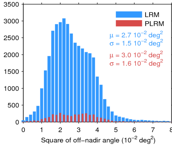
Figure 39. Histogram of flag-valid mispointing over oceans and lakes for LRM (blue) and PLRM (red) for 14/06/2017. Only positive values have been considered. The mean ( \mu ) and standard deviation ( \sigma ) are also shown. Note that values larger than 8 \cdot 10^{-2} \text{ deg}^2 are excluded from the histogram for the sake of readability but not from the computation of \mu and \sigma .
