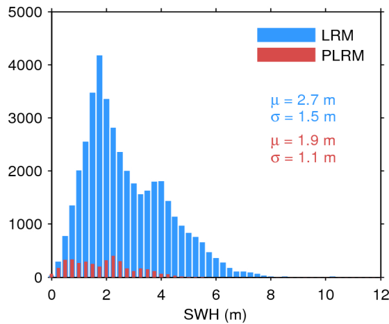
Figure 20. Histogram of science-valid SWH over oceans and lakes for LRM (blue) and PLRM (red) for 14/06/2017. The mean ( \mu ) and standard deviation ( \sigma ) are also shown. Note that values larger than 12 m are excluded from the histogram for the sake of readability but not from the computation of \mu and \sigma .
