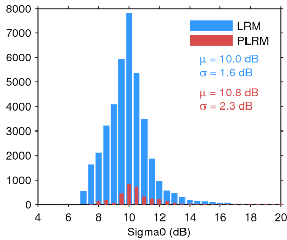
Figure 28. Histogram of science-valid sigma0 over oceans and lakes for LRM (blue) and PLRM (red) for 14/06/2017. The mean ( \mu ) and standard deviation ( \sigma ) are also shown. Note that values outside [4 20] dB are excluded from the histogram for the sake of readability but not from the computation of \mu and \sigma .
