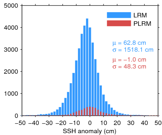
Figure 7. Histogram of flag-valid SSH anomaly over oceans and lakes for LRM (blue) and PLRM (red) for 14/06/2017. The mean ( \mu ) and standard deviation ( \sigma ) are also shown. Note that values outside [-50\ 50] cm are excluded from the histogram for the sake of readability but not from the computation of \mu and \sigma .
