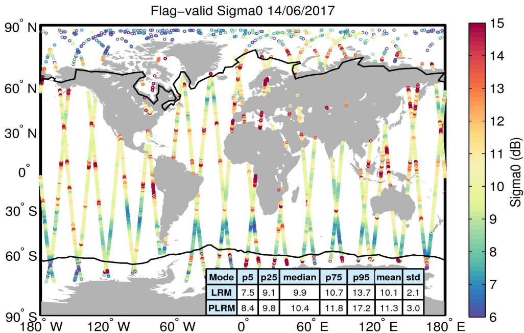
Figure 23. Geographical distribution of flag-valid sigma0 data over oceans and lakes for 14/06/2017. The statistical values shown in the table refer to the sigma0 in dB and are calculated separately for LRM and PLRM regions. Measurements taken over polar polygons have been excluded from the computation of the statistical values. The black lines mark the outer limit of the Arctic and Antarctic polar polygons.
