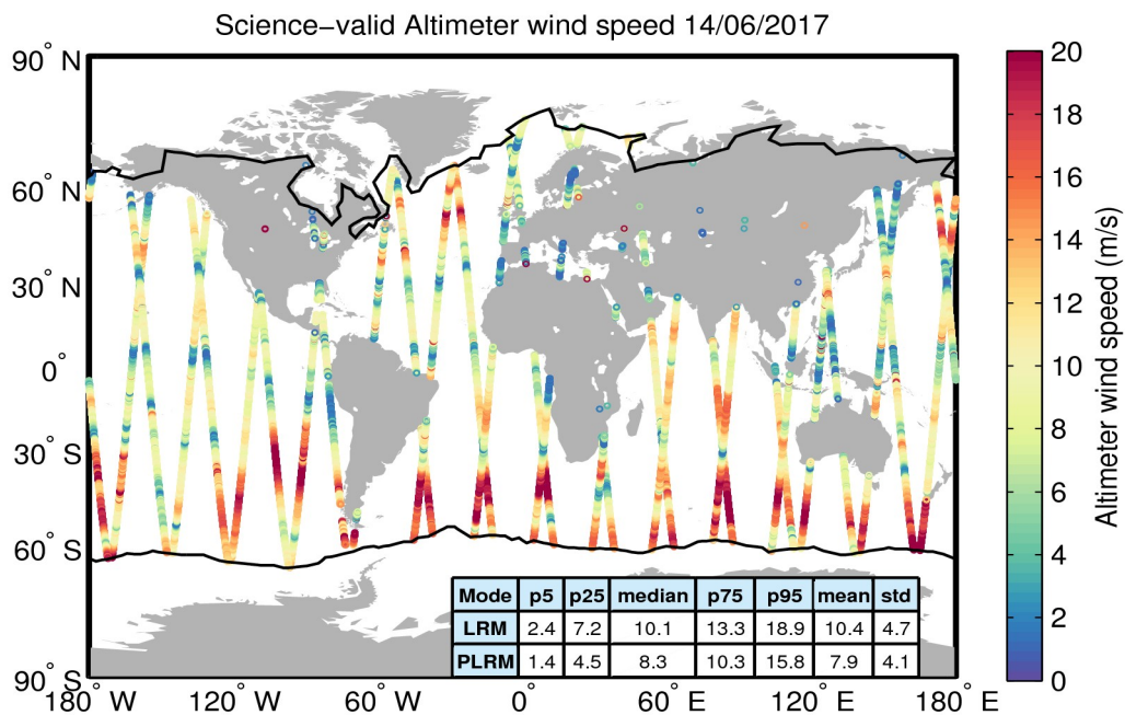
Figure 34. Geographical distribution of science-valid wind data over oceans and lakes for 14/06/2017. The statistical values shown in the table refer to the wind in m/s and are calculated separately for LRM and PLRM regions. The black lines mark the outer limit of the Arctic and Antarctic polar polygons. Gray circles denote records that have been rejected based on the editing criteria described in Table 5.
