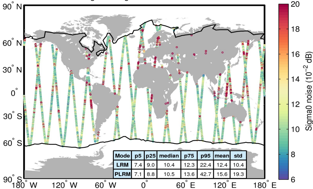
Flag-valid sigma0 noise 14/06/2017
