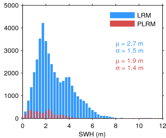
Figure 17. Histogram of flag-valid SWH over oceans and lakes for LRM (blue) and PLRM (red) for 14/06/2017. The mean ( \mu ) and standard deviation ( \sigma ) are also shown. Note that values larger than 12 m are excluded from the histogram for the sake of readability but not from the computation of \mu and \sigma .
