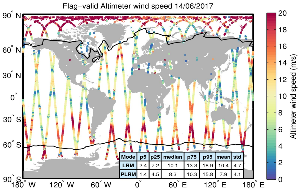
Figure 31. Geographical distribution of flag-valid wind data over oceans and lakes for 14/06/2017. The statistical values shown in the table refer to the wind in m/s and are calculated separately for LRM and PLRM regions. Measurements taken over polar polygons have been excluded from the computation of the statistical values. The black lines mark the outer limit of the Arctic and Antarctic polar polygons.
