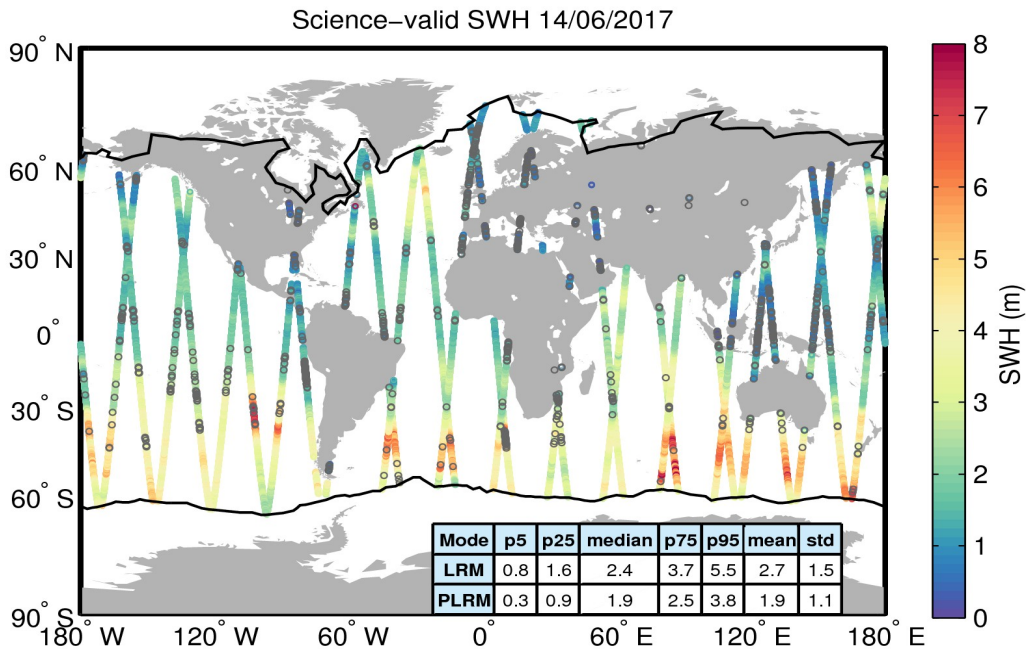
Figure 19. Geographical distribution of science-valid SWH data over oceans and lakes for 14/06/2017. The statistical values shown in the table refer to the SWH in m and are calculated separately for LRM and PLRM regions. The black lines mark the outer limit of the Arctic and Antarctic polar polygons. Gray circles denote records that have been rejected based on the editing criteria described in Table 3.
