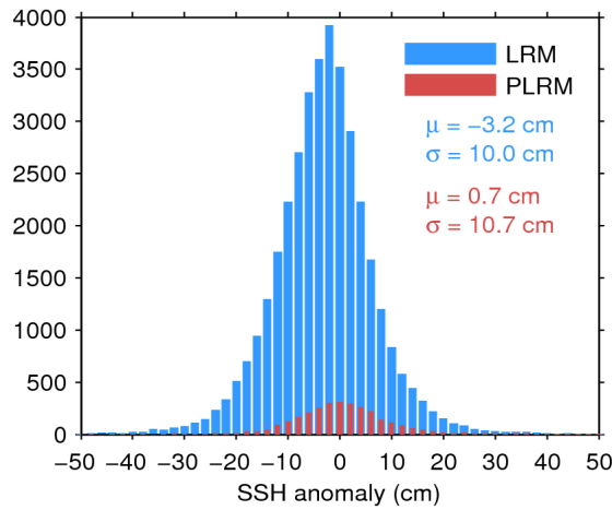
Figure 11. Histogram of science-valid SSH anomaly over oceans and lakes for LRM (blue) and PLRM (red) for 14/06/2017. The mean ( \mu ) and standard deviation ( \sigma ) are also shown. Note that values outside [-50 50] cm are excluded from the histogram for the sake of readability but not from the computation of \mu and \sigma .
