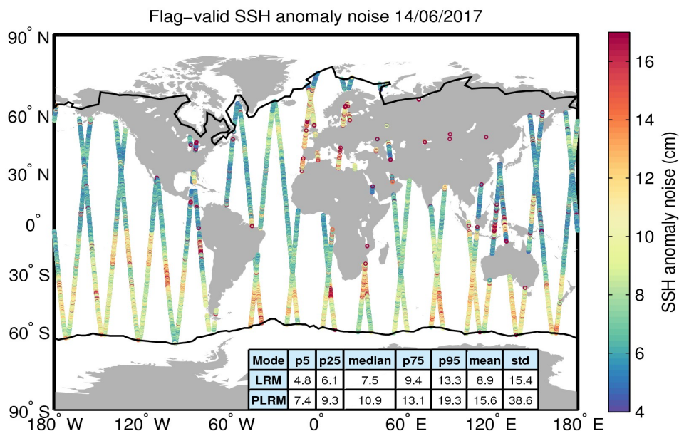
Figure 8. Geographical distribution of flag-valid 20-Hz SSH anomaly measurement noise over oceans and lakes for 14/06/2017. The statistical values shown in the table refer to the SSH anomaly noise and are calculated separately for LRM and PLRM regions. Measurements taken over polar polygons have been excluded from the computation of the statistical values. The black lines mark the outer limit of the Arctic and Antarctic polar polygons.
