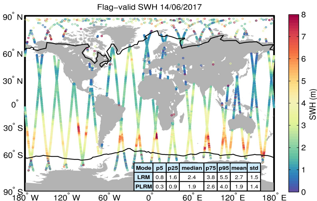
Figure 15. Geographical distribution of flag-valid SWH data over oceans and lakes for 14/06/2017. The statistical values shown in the table refer to the SWH in m and are calculated separately for LRM and PLRM regions. Measurements taken over polar polygons have been excluded from the computation of the statistical values. The black lines mark the outer limit of the Arctic and Antarctic polar polygons.
