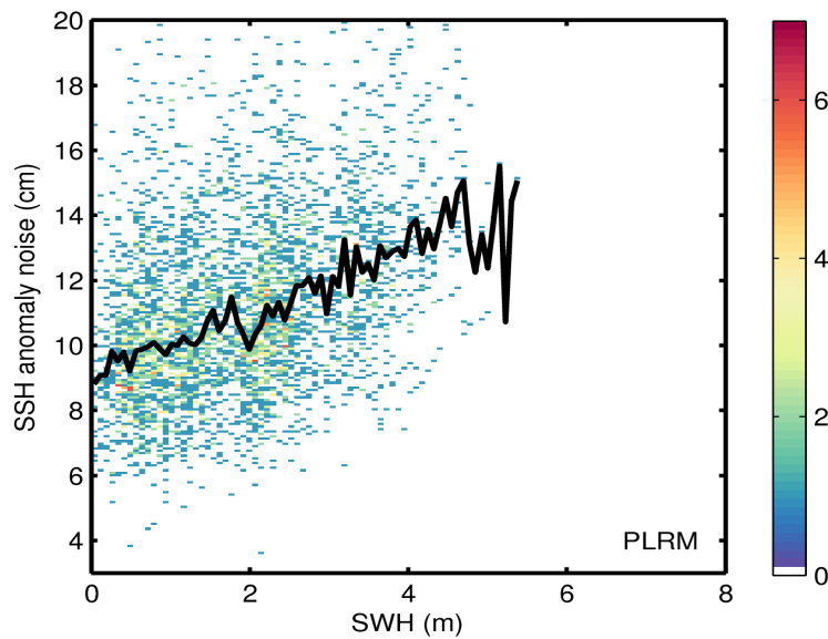
Figure 9. 2D histogram showing flag-valid SSH anomaly noise as a function of SWH for LRM (top) and PLRM (bottom) for 14/06/2017. The black line denotes the median SSH anomaly noise as a function of SWH.
