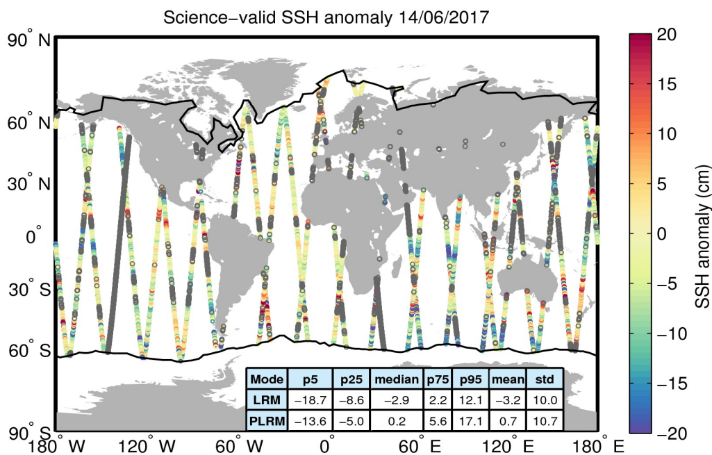
Figure 10. Geographical distribution of science-valid SSH anomaly data over oceans and lakes for 14/06/2017. The statistical values shown in the table refer to the SSH anomaly in cm and are calculated separately for LRM and PLRM regions. The black lines mark the outer limit of the Arctic and Antarctic polar polygons. Gray circles denote records that have been rejected based on the editing criteria described in Table 2.
