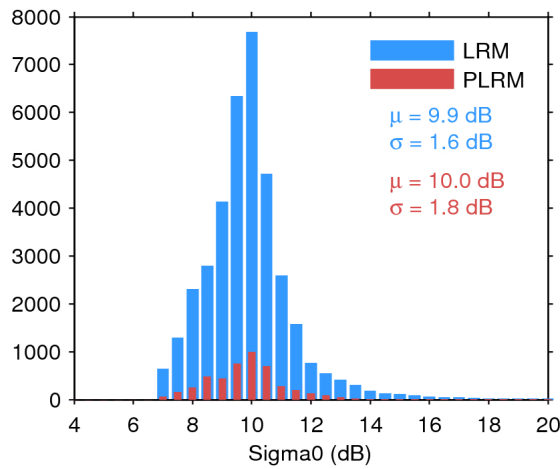
Figure 28. Histogram of science-valid sigma0 over oceans and lakes for LRM (blue) and PLRM (red) for 11/06/2017. The mean ( \mu ) and standard deviation ( \sigma ) are also shown. Note that values outside [4 20] dB are excluded from the histogram for the sake of readability but not from the computation of \mu and \sigma .
