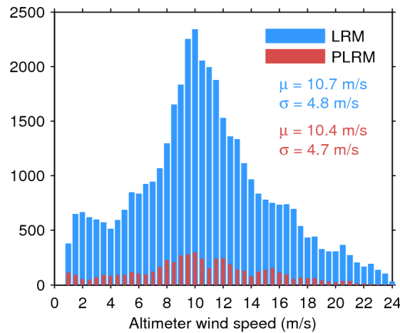
Figure 33. Histogram of flag-valid wind over oceans and lakes for LRM (blue) and PLRM (red) for 11/06/2017. The mean ( \mu ) and standard deviation ( \sigma ) are also shown. Note that values larger than 24 m/s are excluded from the histogram for the sake of readability but not from the computation of \mu and \sigma .
