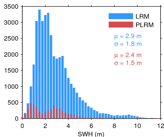
Figure 17. Histogram of flag-valid SWH over oceans and lakes for LRM (blue) and PLRM (red) for 11/06/2017. The mean ( \mu ) and standard deviation ( \sigma ) are also shown. Note that values larger than 12 m are excluded from the histogram for the sake of readability but not from the computation of \mu and \sigma .
