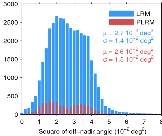
Figure 39. Histogram of flag-valid mispointing over oceans and lakes for LRM (blue) and PLRM (red) for 11/06/2017. Only positive values have been considered. The mean ( \mu ) and standard deviation ( \sigma ) are also shown. Note that values larger than 8 \cdot 10^{-2} \text{ deg}^2 are excluded from the histogram for the sake of readability but not from the computation of \mu and \sigma .
