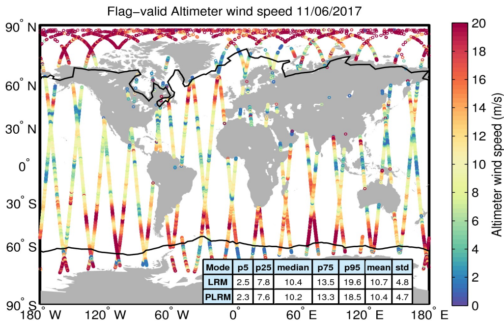
Figure 31. Geographical distribution of flag-valid wind data over oceans and lakes for 11/06/2017. The statistical values shown in the table refer to the wind in m/s and are calculated separately for LRM and PLRM regions. Measurements taken over polar polygons have been excluded from the computation of the statistical values. The black lines mark the outer limit of the Arctic and Antarctic polar polygons.
