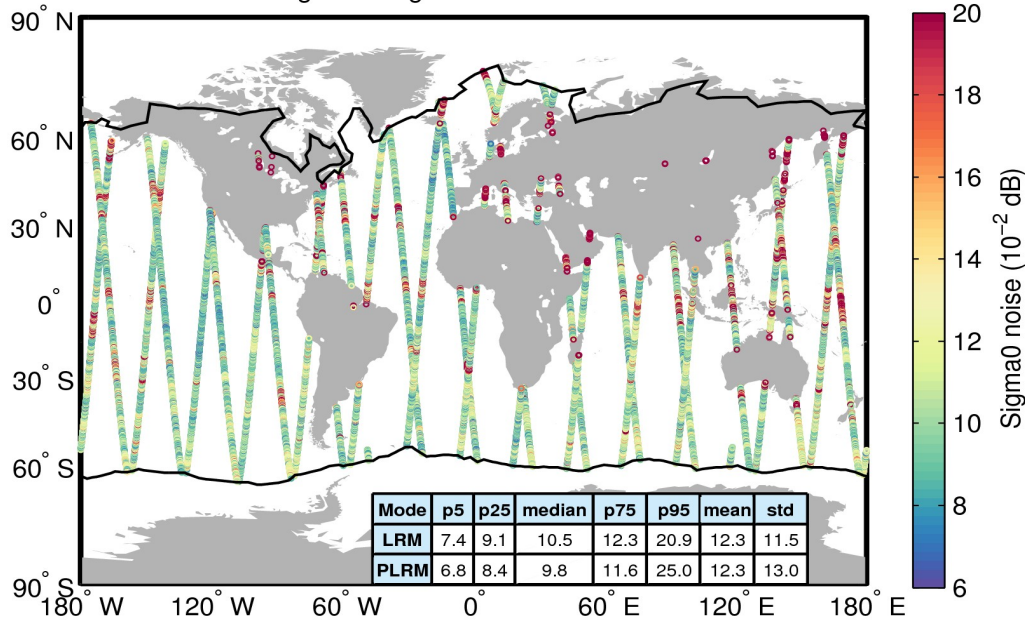
Flag-valid sigma0 noise 11/06/2017
