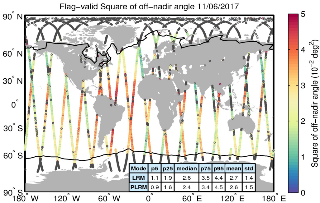
Figure 37. Geographical distribution of flag-valid mispointing data over oceans and lakes for 11/06/2017. The statistical values shown in the table refer to the mispointing in 10^{-2} deg 2 and are calculated separately for LRM and PLRM regions. Measurements taken over polar polygons have been excluded from the computation of the statistical values. The black lines mark the outer limit of the Arctic and Antarctic polar polygons. Gray circles denote negative values.
