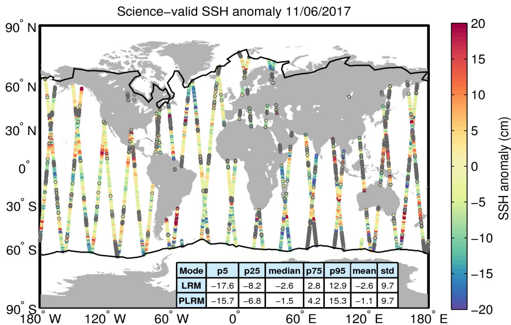
Figure 10. Geographical distribution of science-valid SSH anomaly data over oceans and lakes for 11/06/2017. The statistical values shown in the table refer to the SSH anomaly in cm and are calculated separately for LRM and PLRM regions. The black lines mark the outer limit of the Arctic and Antarctic polar polygons. Gray circles denote records that have been rejected based on the editing criteria described in Table 2.
