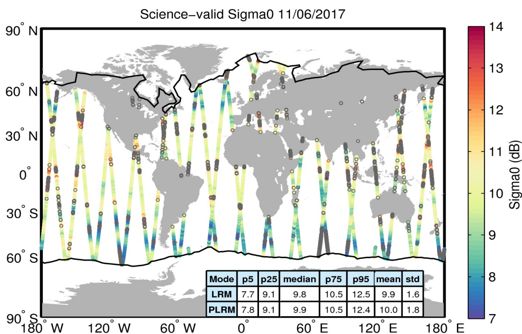
Figure 27. Geographical distribution of science-valid sigma0 data over oceans and lakes for 11/06/2017. The statistical values shown in the table refer to the sigma0 in dB and are calculated separately for LRM and PLRM regions. The black lines mark the outer limit of the Arctic and Antarctic polar polygons. Gray circles denote records that have been rejected based on the editing criteria described in Table 4.
