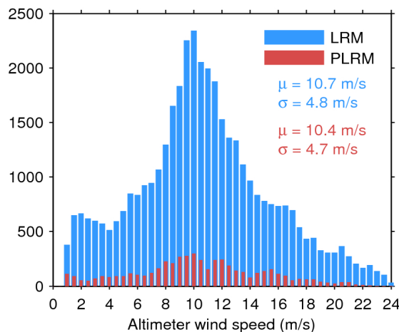
Figure 35. Histogram of science-valid wind over oceans and lakes for LRM (blue) and PLRM (red) for 11/06/2017. The mean ( \mu ) and standard deviation ( \sigma ) are also shown. Note that values larger than 24 m/s are excluded from the histogram for the sake of readability but not from the computation of \mu and \sigma .
