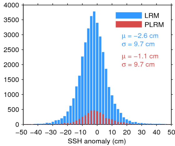
Figure 11. Histogram of science-valid SSH anomaly over oceans and lakes for LRM (blue) and PLRM (red) for 11/06/2017. The mean ( \mu ) and standard deviation ( \sigma ) are also shown. Note that values outside [-50 50] cm are excluded from the histogram for the sake of readability but not from the computation of \mu and \sigma .
