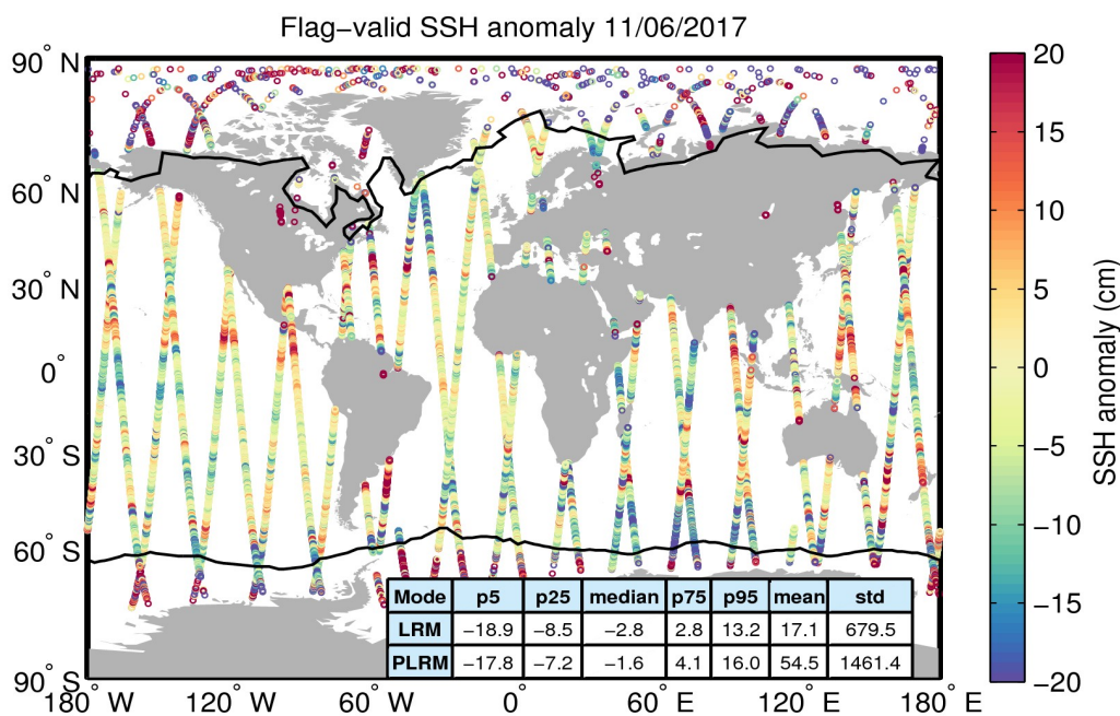
Figure 5. Geographical distribution of flag-valid 1-Hz SSH anomaly data over oceans and lakes for 11/06/2017. The statistical values shown in the table refer to the SSH anomaly in cm and are calculated separately for LRM and PLRM regions. Measurements taken over polar polygons have been excluded from the computation of the statistical values. The black lines mark the outer limit of the Arctic and Antarctic polar polygons.
