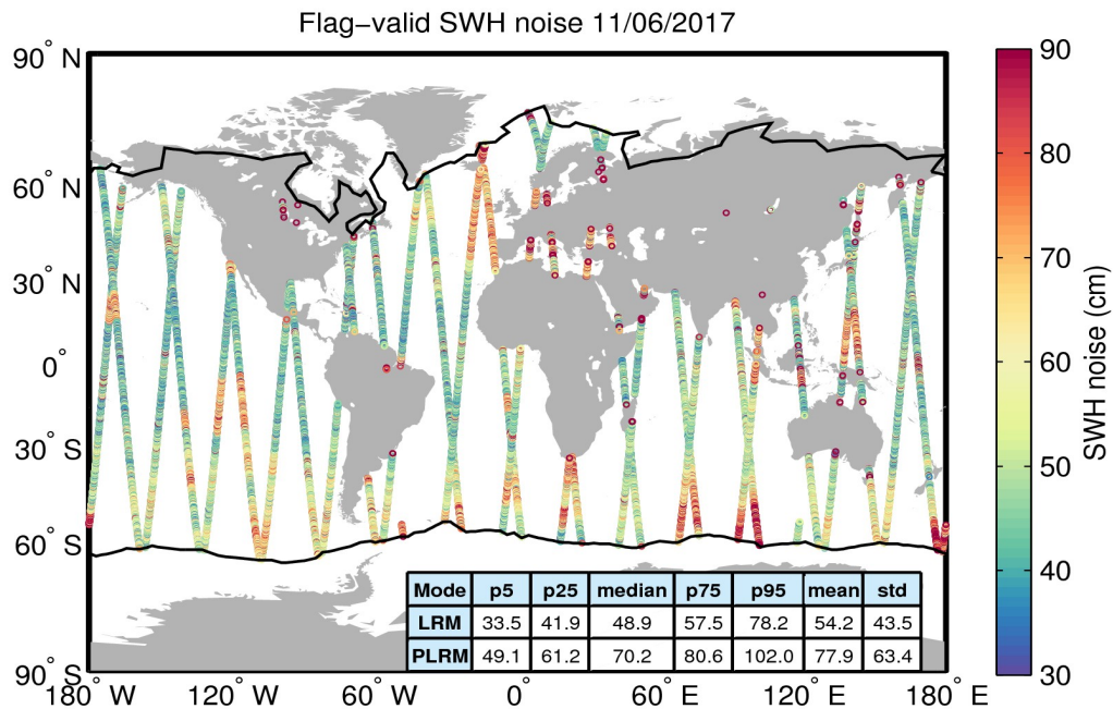
Figure 18. Geographical distribution of flag-valid 20-Hz SWH measurement noise over oceans and lakes for 11/06/2017. The statistical values shown in the table refer to the SWH noise and are calculated separately for LRM and PLRM regions. Measurements taken over polar polygons have been excluded from the computation of the statistical values. The black lines mark the outer limit of the Arctic and Antarctic polar polygons.
