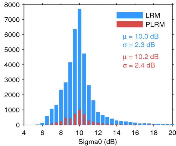
Figure 25. Histogram of flag-valid sigma0 over oceans and lakes for LRM (blue) and PLRM (red) for 11/06/2017. The mean ( \mu ) and standard deviation ( \sigma ) are also shown. Note that values outside [4 20] dB are excluded from the histogram for the sake of readability but not from the computation of \mu and \sigma .
