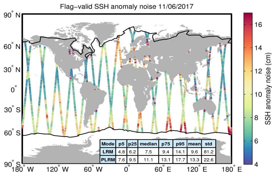
Figure 8. Geographical distribution of flag-valid 20-Hz SSH anomaly measurement noise over oceans and lakes for 11/06/2017. The statistical values shown in the table refer to the SSH anomaly noise and are calculated separately for LRM and PLRM regions. Measurements taken over polar polygons have been excluded from the computation of the statistical values. The black lines mark the outer limit of the Arctic and Antarctic polar polygons.
