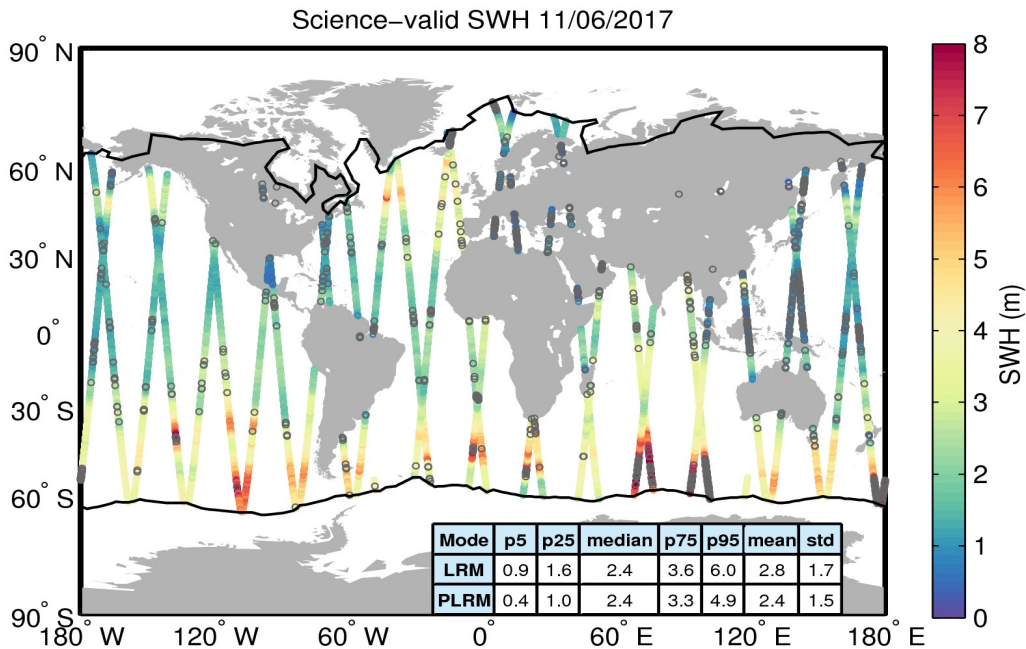
Figure 19. Geographical distribution of science-valid SWH data over oceans and lakes for 11/06/2017. The statistical values shown in the table refer to the SWH in m and are calculated separately for LRM and PLRM regions. The black lines mark the outer limit of the Arctic and Antarctic polar polygons. Gray circles denote records that have been rejected based on the editing criteria described in Table 3.
