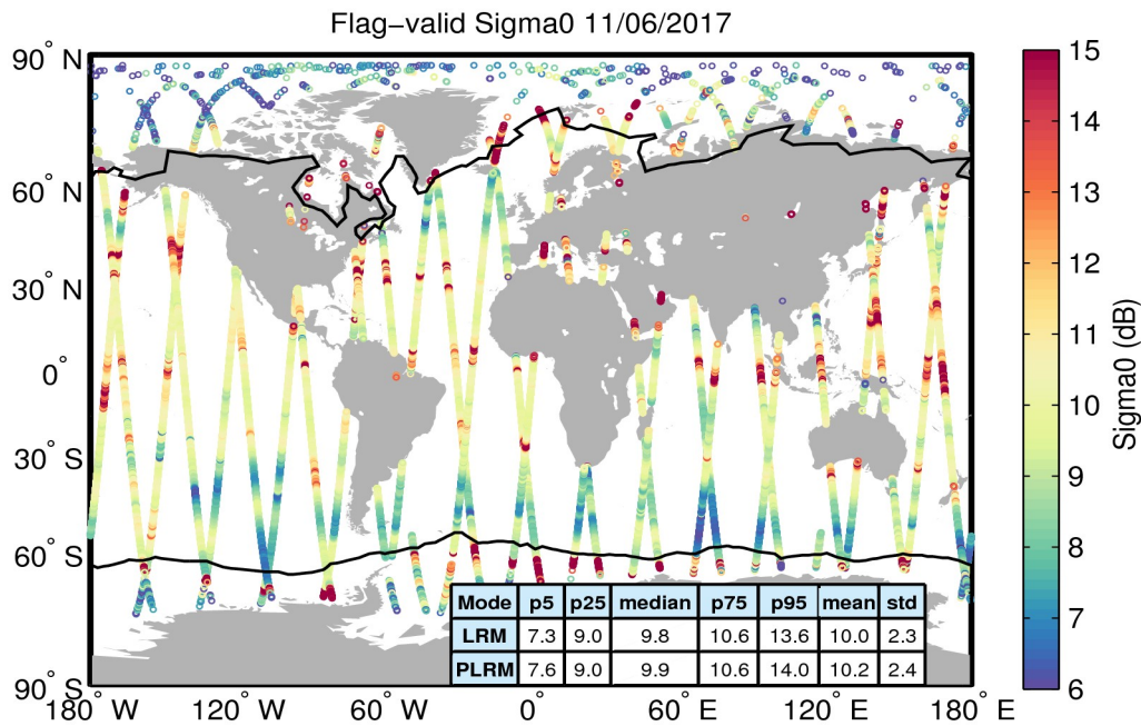
Figure 23. Geographical distribution of flag-valid sigma0 data over oceans and lakes for 11/06/2017. The statistical values shown in the table refer to the sigma0 in dB and are calculated separately for LRM and PLRM regions. Measurements taken over polar polygons have been excluded from the computation of the statistical values. The black lines mark the outer limit of the Arctic and Antarctic polar polygons.
