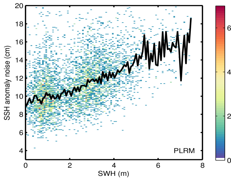
Figure 9. 2D histogram showing flag-valid SSH anomaly noise as a function of SWH for LRM (top) and PLRM (bottom) for 11/06/2017. The black line denotes the median SSH anomaly noise as a function of SWH.
