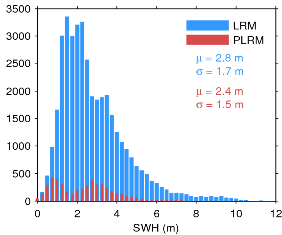
Figure 20. Histogram of science-valid SWH over oceans and lakes for LRM (blue) and PLRM (red) for 11/06/2017. The mean ( \mu ) and standard deviation ( \sigma ) are also shown. Note that values larger than 12 m are excluded from the histogram for the sake of readability but not from the computation of \mu and \sigma .
