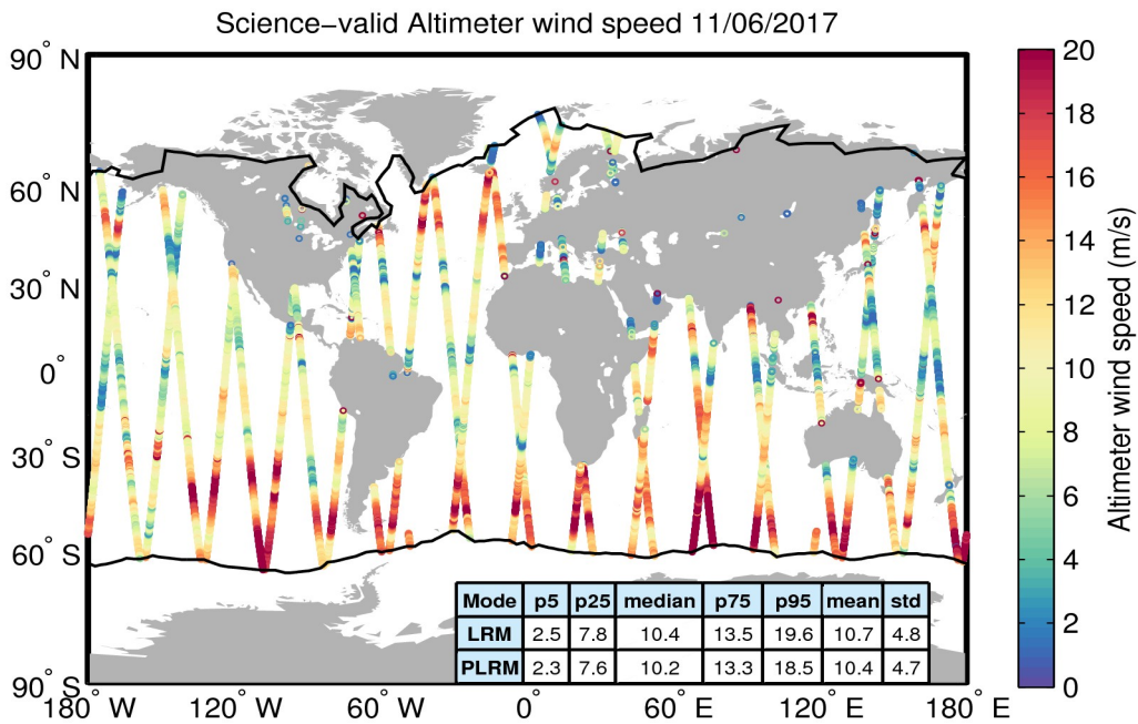
Figure 34. Geographical distribution of science-valid wind data over oceans and lakes for 11/06/2017. The statistical values shown in the table refer to the wind in m/s and are calculated separately for LRM and PLRM regions. The black lines mark the outer limit of the Arctic and Antarctic polar polygons. Gray circles denote records that have been rejected based on the editing criteria described in Table 5.
