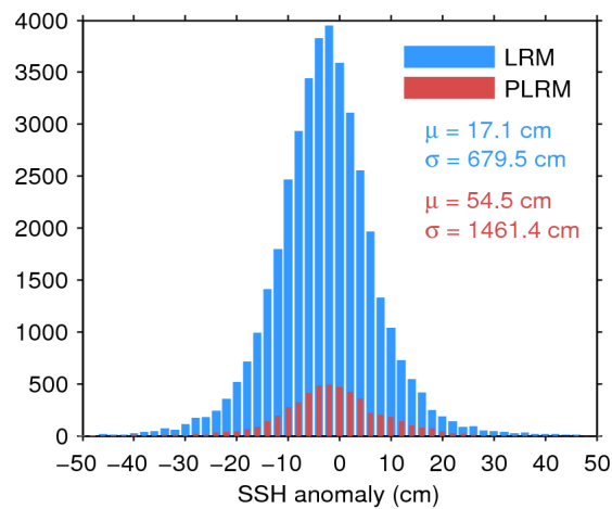
Figure 7. Histogram of flag-valid SSH anomaly over oceans and lakes for LRM (blue) and PLRM (red) for 11/06/2017. The mean ( \mu ) and standard deviation ( \sigma ) are also shown. Note that values outside [-50 50] cm are excluded from the histogram for the sake of readability but not from the computation of \mu and \sigma .
