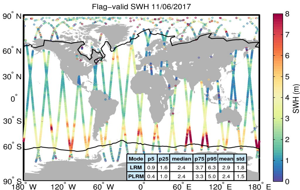
Figure 15. Geographical distribution of flag-valid SWH data over oceans and lakes for 11/06/2017. The statistical values shown in the table refer to the SWH in m and are calculated separately for LRM and PLRM regions. Measurements taken over polar polygons have been excluded from the computation of the statistical values. The black lines mark the outer limit of the Arctic and Antarctic polar polygons.
