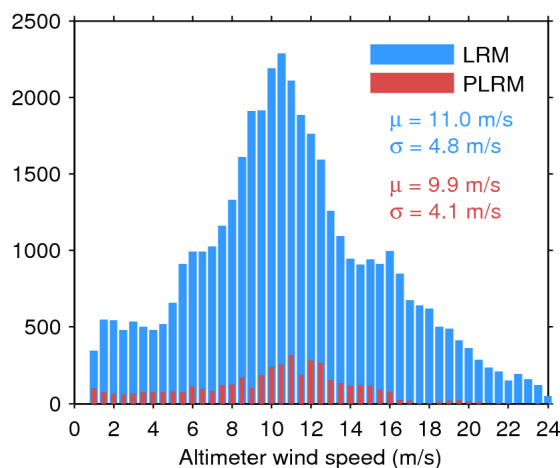
Figure 35. Histogram of science-valid wind over oceans and lakes for LRM (blue) and PLRM (red) for 10/06/2017. The mean ( \mu ) and standard deviation ( \sigma ) are also shown. Note that values larger than 24 m/s are excluded from the histogram for the sake of readability but not from the computation of \mu and \sigma .
