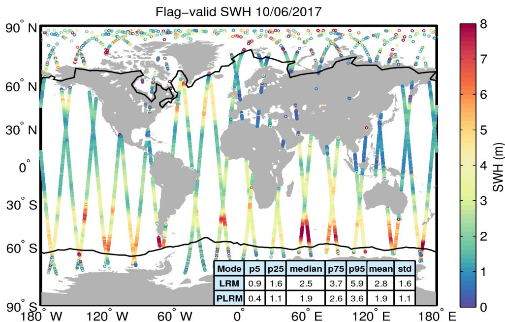
Figure 15. Geographical distribution of flag-valid SWH data over oceans and lakes for 10/06/2017. The statistical values shown in the table refer to the SWH in m and are calculated separately for LRM and PLRM regions. Measurements taken over polar polygons have been excluded from the computation of the statistical values. The black lines mark the outer limit of the Arctic and Antarctic polar polygons.
