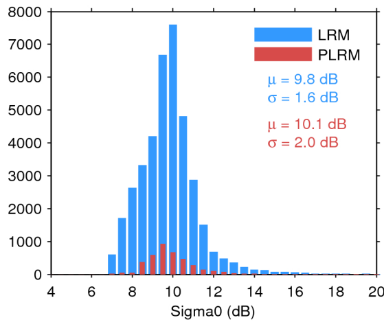
Figure 28. Histogram of science-valid sigma0 over oceans and lakes for LRM (blue) and PLRM (red) for 10/06/2017. The mean ( \mu ) and standard deviation ( \sigma ) are also shown. Note that values outside [4 20] dB are excluded from the histogram for the sake of readability but not from the computation of \mu and \sigma .
