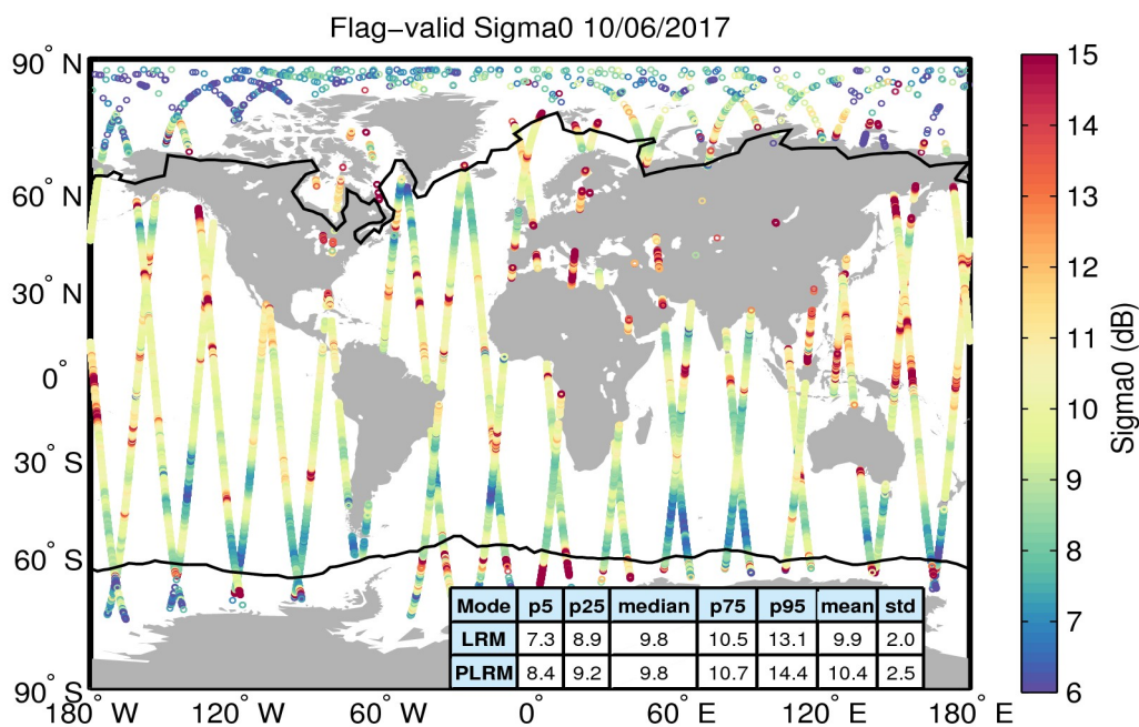
Figure 23. Geographical distribution of flag-valid sigma0 data over oceans and lakes for 10/06/2017. The statistical values shown in the table refer to the sigma0 in dB and are calculated separately for LRM and PLRM regions. Measurements taken over polar polygons have been excluded from the computation of the statistical values. The black lines mark the outer limit of the Arctic and Antarctic polar polygons.
