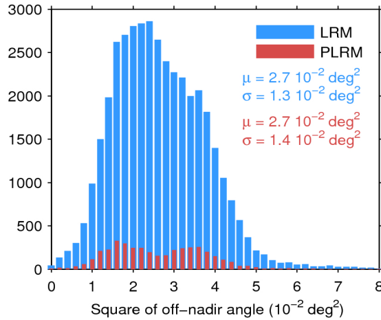
Figure 39. Histogram of flag-valid mispointing over oceans and lakes for LRM (blue) and PLRM (red) for 10/06/2017. Only positive values have been considered. The mean ( \mu ) and standard deviation ( \sigma ) are also shown. Note that values larger than 8 \cdot 10^{-2} \text{ deg}^2 are excluded from the histogram for the sake of readability but not from the computation of \mu and \sigma .
