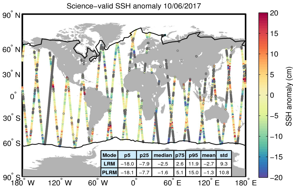
Figure 10. Geographical distribution of science-valid SSH anomaly data over oceans and lakes for 10/06/2017. The statistical values shown in the table refer to the SSH anomaly in cm and are calculated separately for LRM and PLRM regions. The black lines mark the outer limit of the Arctic and Antarctic polar polygons. Gray circles denote records that have been rejected based on the editing criteria described in Table 2.
