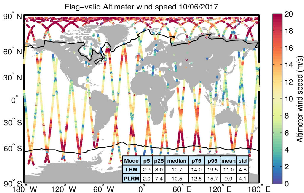
Figure 31. Geographical distribution of flag-valid wind data over oceans and lakes for 10/06/2017. The statistical values shown in the table refer to the wind in m/s and are calculated separately for LRM and PLRM regions. Measurements taken over polar polygons have been excluded from the computation of the statistical values. The black lines mark the outer limit of the Arctic and Antarctic polar polygons.
