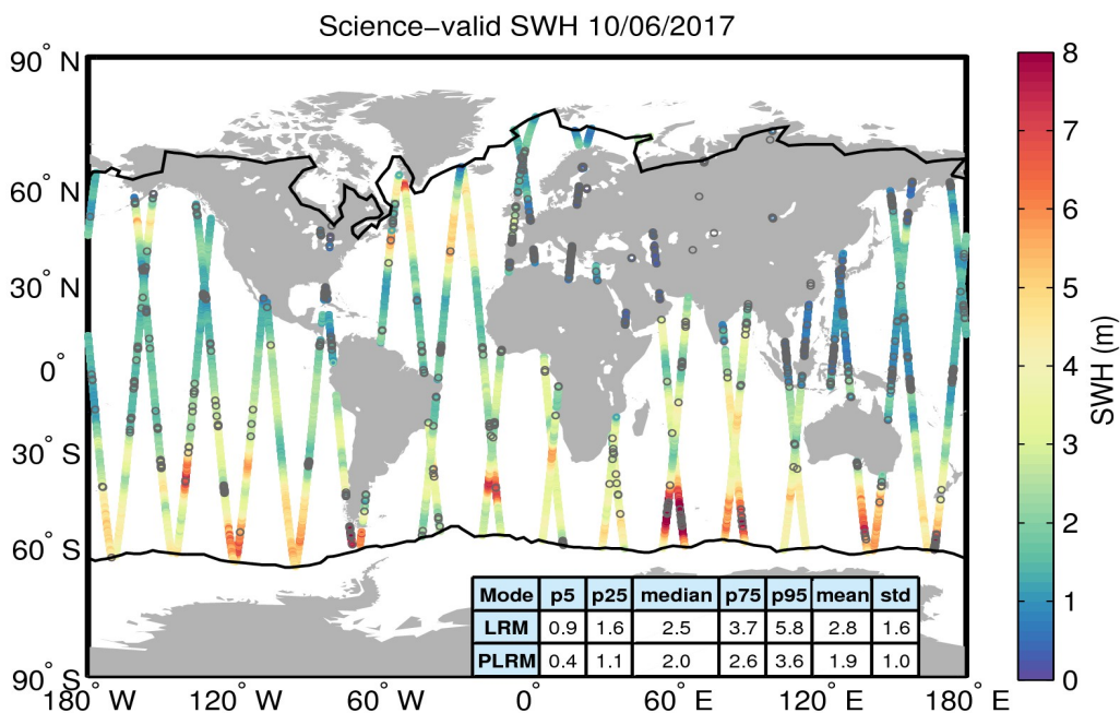
Figure 19. Geographical distribution of science-valid SWH data over oceans and lakes for 10/06/2017. The statistical values shown in the table refer to the SWH in m and are calculated separately for LRM and PLRM regions. The black lines mark the outer limit of the Arctic and Antarctic polar polygons. Gray circles denote records that have been rejected based on the editing criteria described in Table 3.
