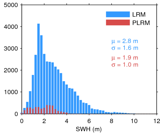
Figure 20. Histogram of science-valid SWH over oceans and lakes for LRM (blue) and PLRM (red) for 10/06/2017. The mean ( \mu ) and standard deviation ( \sigma ) are also shown. Note that values larger than 12 m are excluded from the histogram for the sake of readability but not from the computation of \mu and \sigma .
