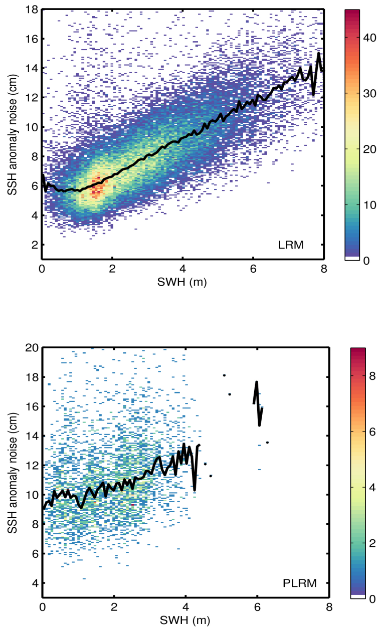
Figure 9. 2D histogram showing flag-valid SSH anomaly noise as a function of SWH for LRM (top) and PLRM (bottom) for 10/06/2017. The black line denotes the median SSH anomaly noise as a function of SWH.
