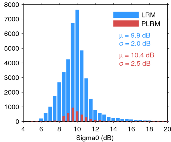
Figure 25. Histogram of flag-valid sigma0 over oceans and lakes for LRM (blue) and PLRM (red) for 10/06/2017. The mean ( \mu ) and standard deviation ( \sigma ) are also shown. Note that values outside [4 20] dB are excluded from the histogram for the sake of readability but not from the computation of \mu and \sigma .
