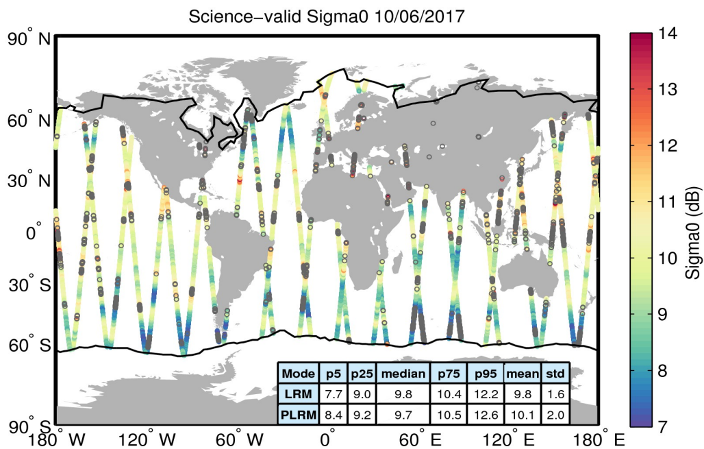
Figure 27. Geographical distribution of science-valid sigma0 data over oceans and lakes for 10/06/2017. The statistical values shown in the table refer to the sigma0 in dB and are calculated separately for LRM and PLRM regions. The black lines mark the outer limit of the Arctic and Antarctic polar polygons. Gray circles denote records that have been rejected based on the editing criteria described in Table 4.
