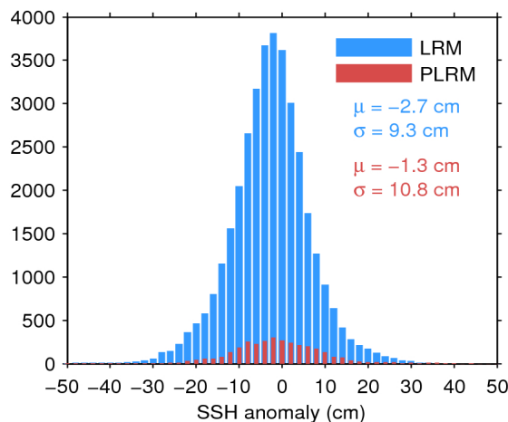
Figure 11. Histogram of science-valid SSH anomaly over oceans and lakes for LRM (blue) and PLRM (red) for 10/06/2017. The mean ( \mu ) and standard deviation ( \sigma ) are also shown. Note that values outside [-50 50] cm are excluded from the histogram for the sake of readability but not from the computation of \mu and \sigma .
