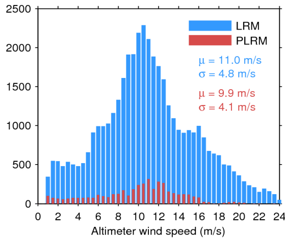
Figure 33. Histogram of flag-valid wind over oceans and lakes for LRM (blue) and PLRM (red) for 10/06/2017. The mean ( \mu ) and standard deviation ( \sigma ) are also shown. Note that values larger than 24 m/s are excluded from the histogram for the sake of readability but not from the computation of \mu and \sigma .
