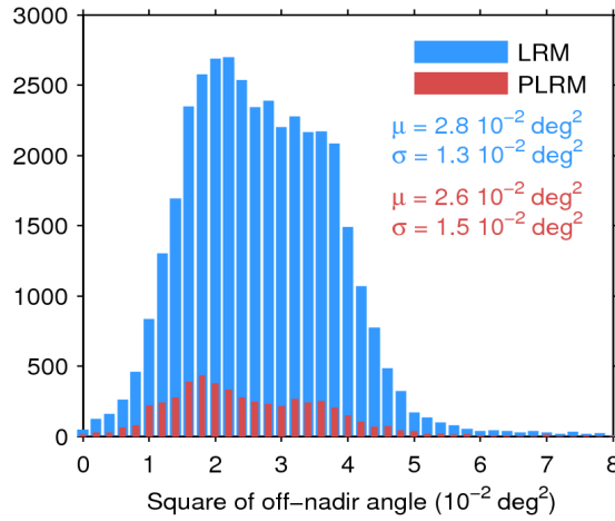
Figure 39. Histogram of flag-valid mispointing over oceans and lakes for LRM (blue) and PLRM (red) for 09/06/2017. Only positive values have been considered. The mean ( \mu ) and standard deviation ( \sigma ) are also shown. Note that values larger than 8 \cdot 10^{-2} \text{ deg}^2 are excluded from the histogram for the sake of readability but not from the computation of \mu and \sigma .
