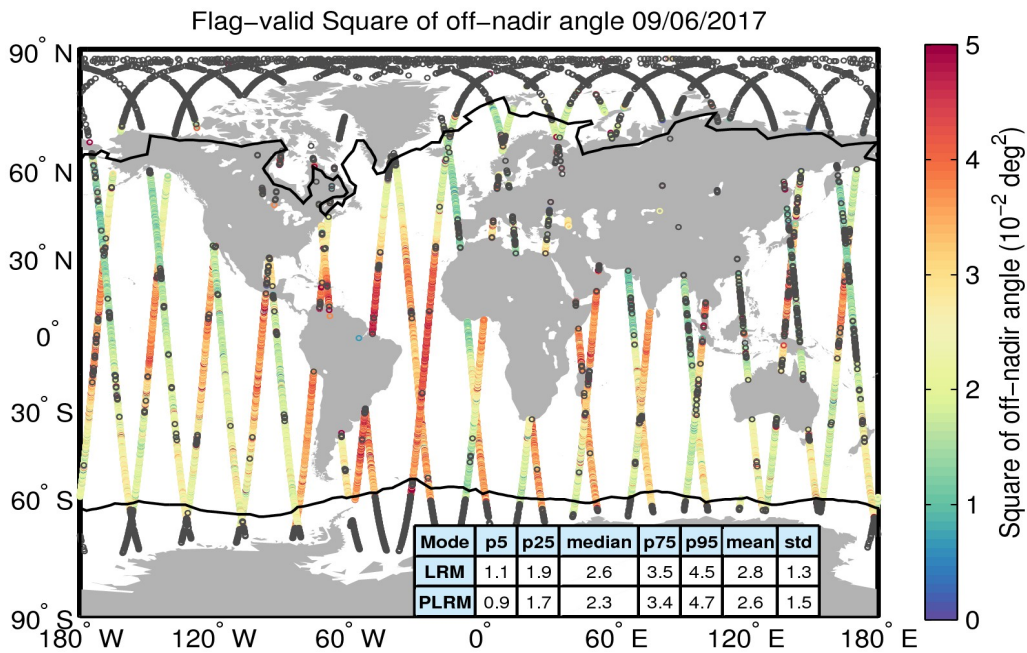
Figure 37. Geographical distribution of flag-valid mispointing data over oceans and lakes for 09/06/2017. The statistical values shown in the table refer to the mispointing in 10^{-2} deg 2 and are calculated separately for LRM and PLRM regions. Measurements taken over polar polygons have been excluded from the computation of the statistical values. The black lines mark the outer limit of the Arctic and Antarctic polar polygons. Gray circles denote negative values.
