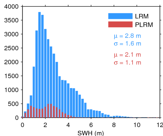
Figure 17. Histogram of flag-valid SWH over oceans and lakes for LRM (blue) and PLRM (red) for 09/06/2017. The mean ( \mu ) and standard deviation ( \sigma ) are also shown. Note that values larger than 12 m are excluded from the histogram for the sake of readability but not from the computation of \mu and \sigma .
