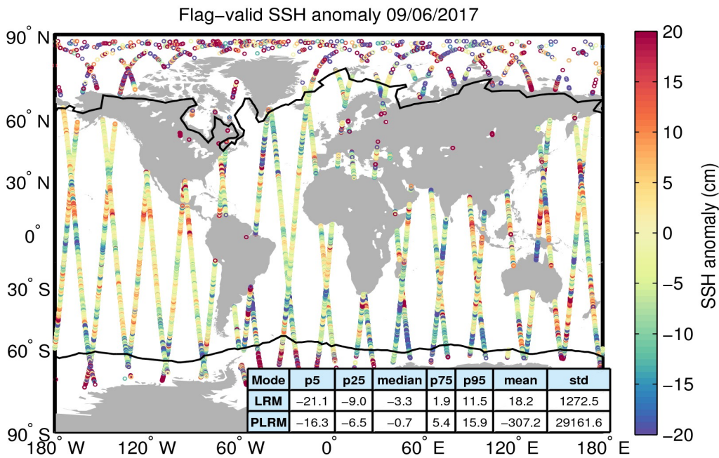
Figure 5. Geographical distribution of flag-valid 1-Hz SSH anomaly data over oceans and lakes for 09/06/2017. The statistical values shown in the table refer to the SSH anomaly in cm and are calculated separately for LRM and PLRM regions. Measurements taken over polar polygons have been excluded from the computation of the statistical values. The black lines mark the outer limit of the Arctic and Antarctic polar polygons.
