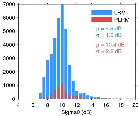
Figure 28. Histogram of science-valid sigma0 over oceans and lakes for LRM (blue) and PLRM (red) for 09/06/2017. The mean ( \mu ) and standard deviation ( \sigma ) are also shown. Note that values outside [4 20] dB are excluded from the histogram for the sake of readability but not from the computation of \mu and \sigma .
