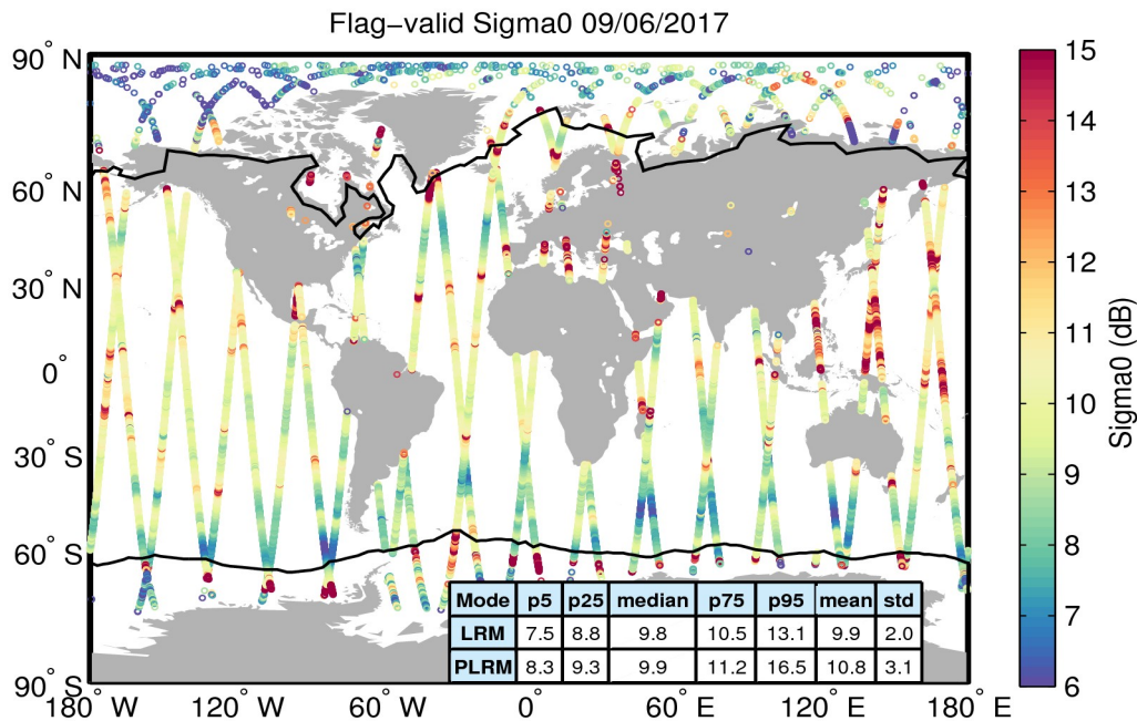
Figure 23. Geographical distribution of flag-valid sigma0 data over oceans and lakes for 09/06/2017. The statistical values shown in the table refer to the sigma0 in dB and are calculated separately for LRM and PLRM regions. Measurements taken over polar polygons have been excluded from the computation of the statistical values. The black lines mark the outer limit of the Arctic and Antarctic polar polygons.
