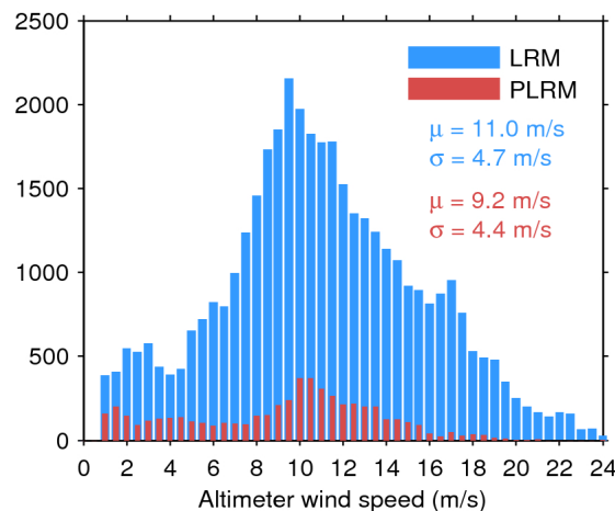
Figure 35. Histogram of science-valid wind over oceans and lakes for LRM (blue) and PLRM (red) for 09/06/2017. The mean ( \mu ) and standard deviation ( \sigma ) are also shown. Note that values larger than 24 m/s are excluded from the histogram for the sake of readability but not from the computation of \mu and \sigma .
