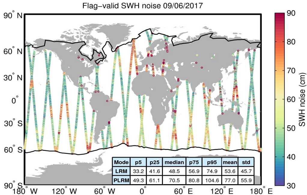
Figure 18. Geographical distribution of flag-valid 20-Hz SWH measurement noise over oceans and lakes for 09/06/2017. The statistical values shown in the table refer to the SWH noise and are calculated separately for LRM and PLRM regions. Measurements taken over polar polygons have been excluded from the computation of the statistical values. The black lines mark the outer limit of the Arctic and Antarctic polar polygons.
