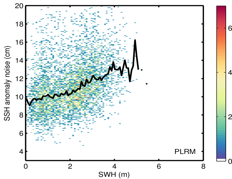
Figure 9. 2D histogram showing flag-valid SSH anomaly noise as a function of SWH for LRM (top) and PLRM (bottom) for 09/06/2017. The black line denotes the median SSH anomaly noise as a function of SWH.
