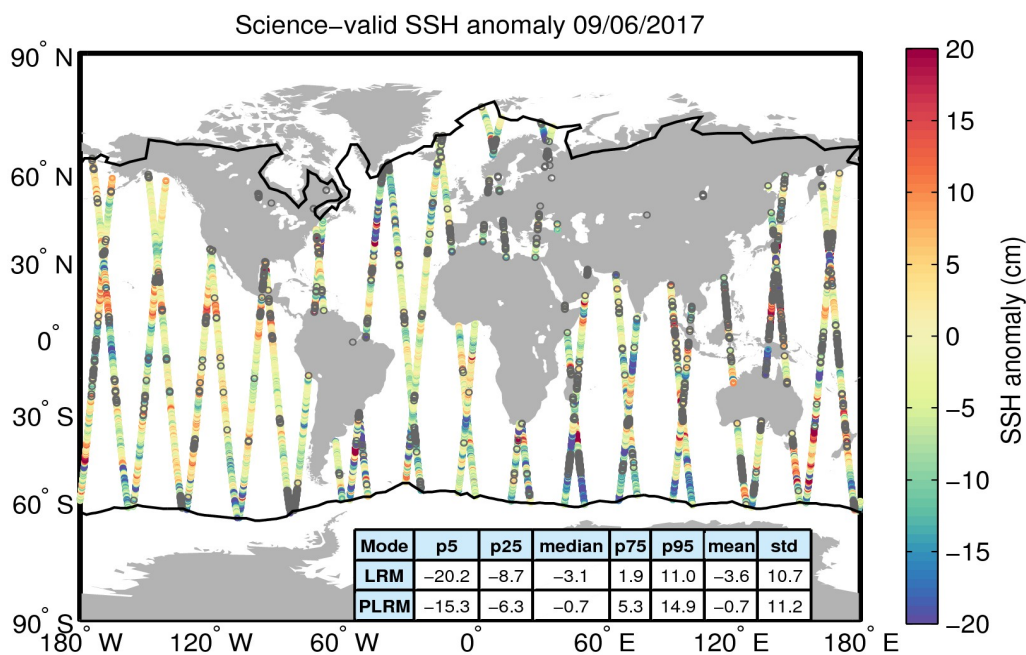
Figure 10. Geographical distribution of science-valid SSH anomaly data over oceans and lakes for 09/06/2017. The statistical values shown in the table refer to the SSH anomaly in cm and are calculated separately for LRM and PLRM regions. The black lines mark the outer limit of the Arctic and Antarctic polar polygons. Gray circles denote records that have been rejected based on the editing criteria described in Table 2.
