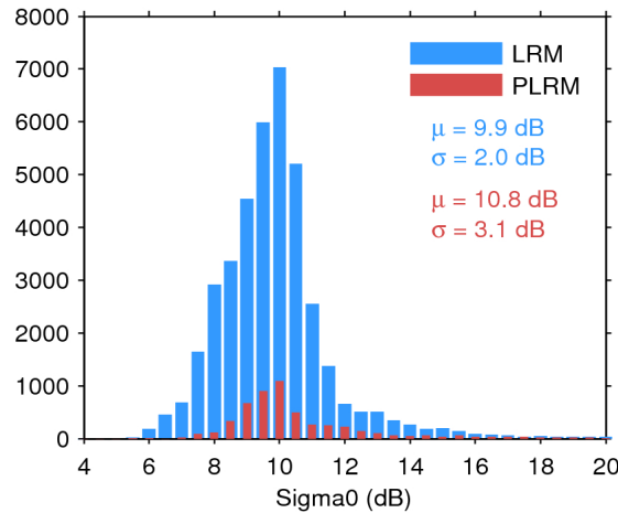
Figure 25. Histogram of flag-valid sigma0 over oceans and lakes for LRM (blue) and PLRM (red) for 09/06/2017. The mean ( \mu ) and standard deviation ( \sigma ) are also shown. Note that values outside [4 20] dB are excluded from the histogram for the sake of readability but not from the computation of \mu and \sigma .
