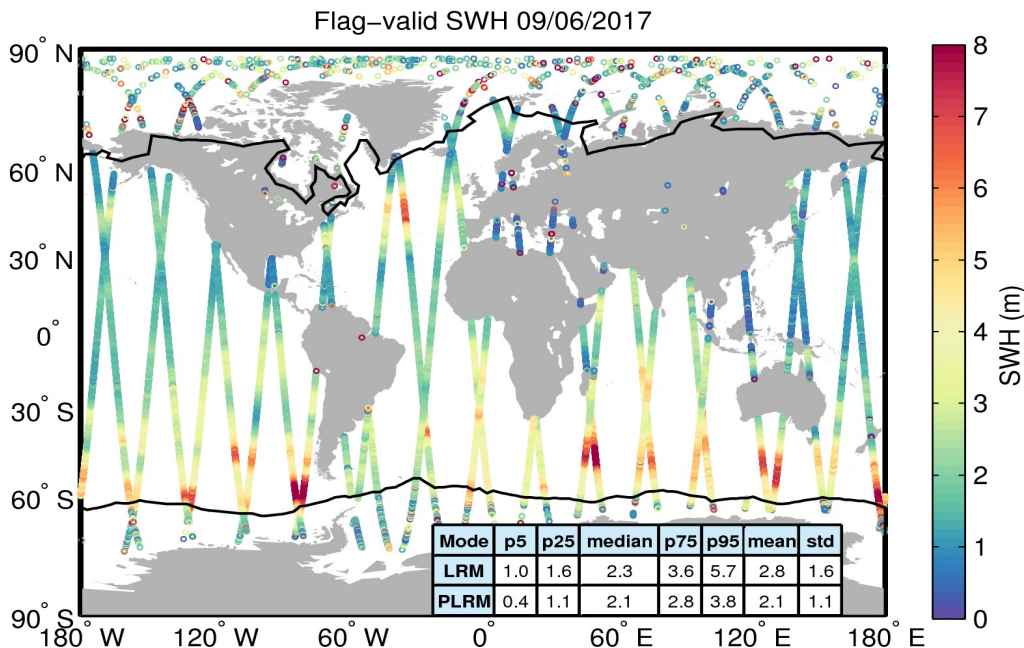
Figure 15. Geographical distribution of flag-valid SWH data over oceans and lakes for 09/06/2017. The statistical values shown in the table refer to the SWH in m and are calculated separately for LRM and PLRM regions. Measurements taken over polar polygons have been excluded from the computation of the statistical values. The black lines mark the outer limit of the Arctic and Antarctic polar polygons.
