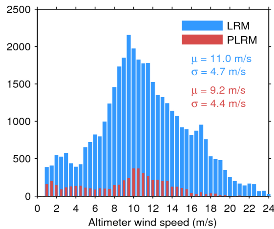
Figure 33. Histogram of flag-valid wind over oceans and lakes for LRM (blue) and PLRM (red) for 09/06/2017. The mean ( \mu ) and standard deviation ( \sigma ) are also shown. Note that values larger than 24 m/s are excluded from the histogram for the sake of readability but not from the computation of \mu and \sigma .
