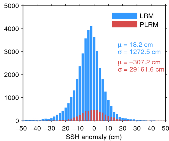
Figure 7. Histogram of flag-valid SSH anomaly over oceans and lakes for LRM (blue) and PLRM (red) for 09/06/2017. The mean ( \mu ) and standard deviation ( \sigma ) are also shown. Note that values outside [-50\ 50] cm are excluded from the histogram for the sake of readability but not from the computation of \mu and \sigma .
