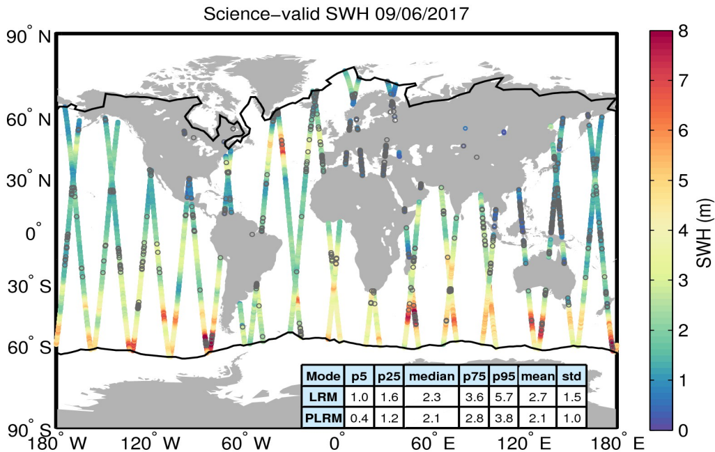
Figure 19. Geographical distribution of science-valid SWH data over oceans and lakes for 09/06/2017. The statistical values shown in the table refer to the SWH in m and are calculated separately for LRM and PLRM regions. The black lines mark the outer limit of the Arctic and Antarctic polar polygons. Gray circles denote records that have been rejected based on the editing criteria described in Table 3.
