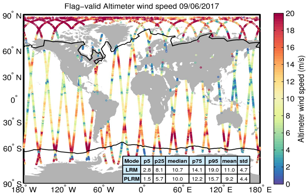
Figure 31. Geographical distribution of flag-valid wind data over oceans and lakes for 09/06/2017. The statistical values shown in the table refer to the wind in m/s and are calculated separately for LRM and PLRM regions. Measurements taken over polar polygons have been excluded from the computation of the statistical values. The black lines mark the outer limit of the Arctic and Antarctic polar polygons.
