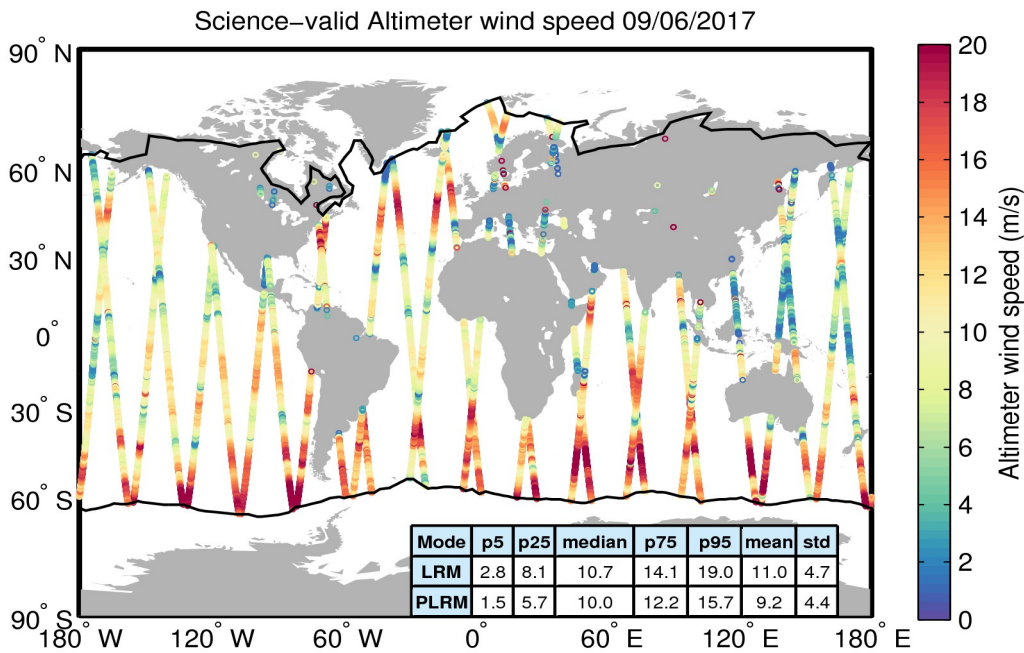
Figure 34. Geographical distribution of science-valid wind data over oceans and lakes for 09/06/2017. The statistical values shown in the table refer to the wind in m/s and are calculated separately for LRM and PLRM regions. The black lines mark the outer limit of the Arctic and Antarctic polar polygons. Gray circles denote records that have been rejected based on the editing criteria described in Table 5.
