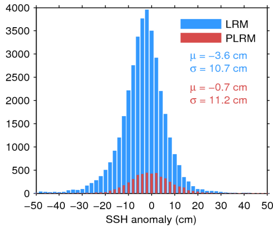
Figure 11. Histogram of science-valid SSH anomaly over oceans and lakes for LRM (blue) and PLRM (red) for 09/06/2017. The mean ( \mu ) and standard deviation ( \sigma ) are also shown. Note that values outside [-50\ 50] cm are excluded from the histogram for the sake of readability but not from the computation of \mu and \sigma .
