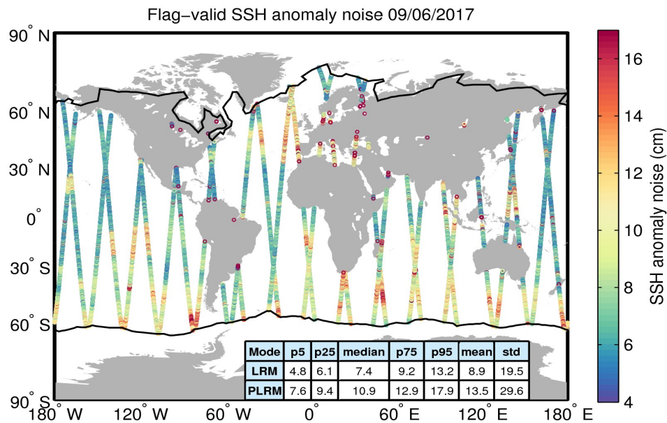
Figure 8. Geographical distribution of flag-valid 20-Hz SSH anomaly measurement noise over oceans and lakes for 09/06/2017. The statistical values shown in the table refer to the SSH anomaly noise and are calculated separately for LRM and PLRM regions. Measurements taken over polar polygons have been excluded from the computation of the statistical values. The black lines mark the outer limit of the Arctic and Antarctic polar polygons.
