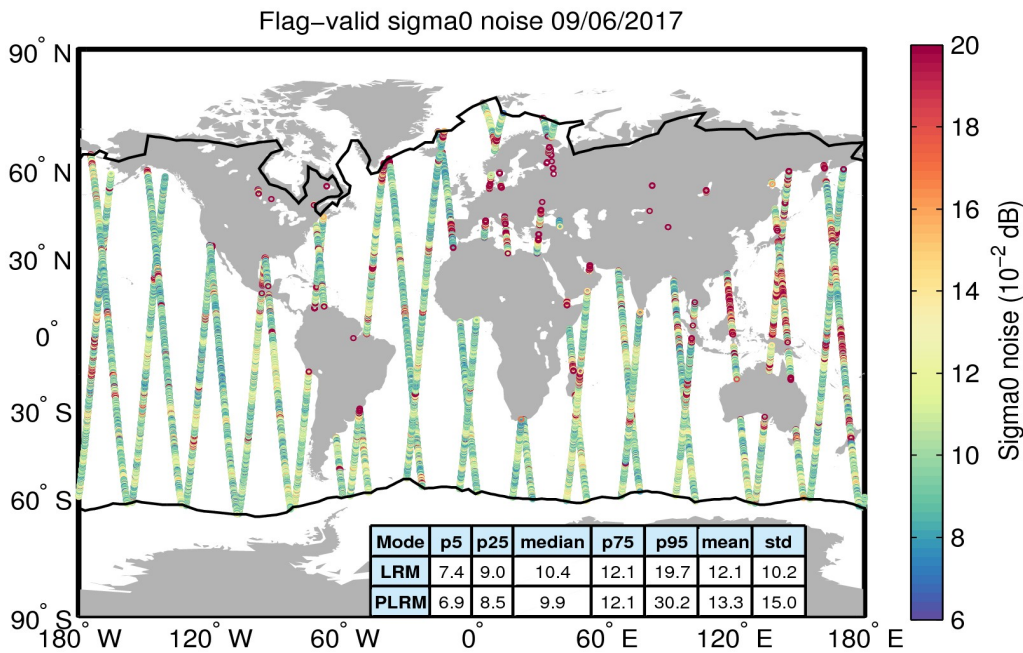
Figure 26. Geographical distribution of flag-valid 20-Hz sigma0 measurement noise over oceans and lakes for 09/06/2017. The statistical values shown in the table refer to the sigma0 noise and are calculated separately for LRM and PLRM regions. Measurements taken over polar polygons have been excluded from the computation of the statistical values. The black lines mark the outer limit of the Arctic and Antarctic polar polygons.
