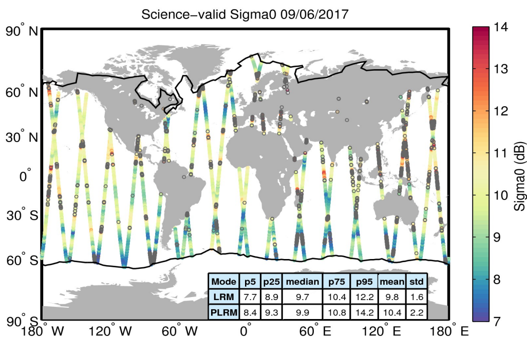
Figure 27. Geographical distribution of science-valid sigma0 data over oceans and lakes for 09/06/2017. The statistical values shown in the table refer to the sigma0 in dB and are calculated separately for LRM and PLRM regions. The black lines mark the outer limit of the Arctic and Antarctic polar polygons. Gray circles denote records that have been rejected based on the editing criteria described in Table 4.
