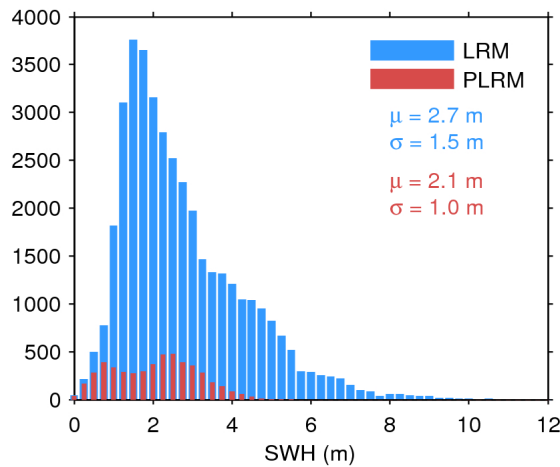
Figure 20. Histogram of science-valid SWH over oceans and lakes for LRM (blue) and PLRM (red) for 09/06/2017. The mean ( \mu ) and standard deviation ( \sigma ) are also shown. Note that values larger than 12 m are excluded from the histogram for the sake of readability but not from the computation of \mu and \sigma .
