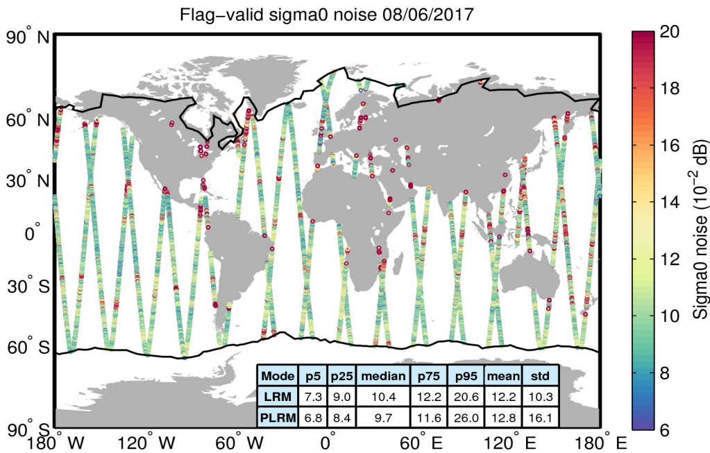
Figure 26. Geographical distribution of flag-valid 20-Hz sigma0 measurement noise over oceans and lakes for 08/06/2017. The statistical values shown in the table refer to the sigma0 noise and are calculated separately for LRM and PLRM regions. Measurements taken over polar polygons have been excluded from the computation of the statistical values. The black lines mark the outer limit of the Arctic and Antarctic polar polygons.
