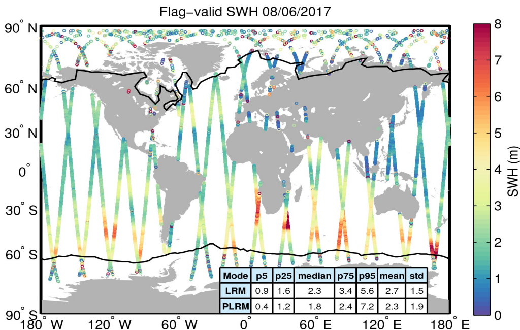
Figure 15. Geographical distribution of flag-valid SWH data over oceans and lakes for 08/06/2017. The statistical values shown in the table refer to the SWH in m and are calculated separately for LRM and PLRM regions. Measurements taken over polar polygons have been excluded from the computation of the statistical values. The black lines mark the outer limit of the Arctic and Antarctic polar polygons.
