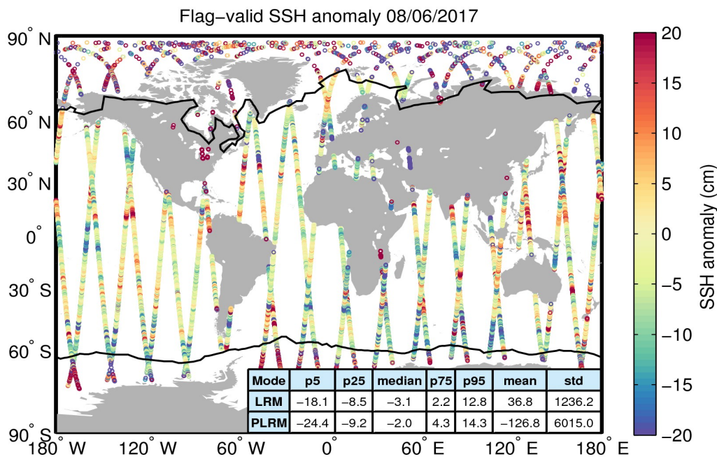
Figure 5. Geographical distribution of flag-valid 1-Hz SSH anomaly data over oceans and lakes for 08/06/2017. The statistical values shown in the table refer to the SSH anomaly in cm and are calculated separately for LRM and PLRM regions. Measurements taken over polar polygons have been excluded from the computation of the statistical values. The black lines mark the outer limit of the Arctic and Antarctic polar polygons.
