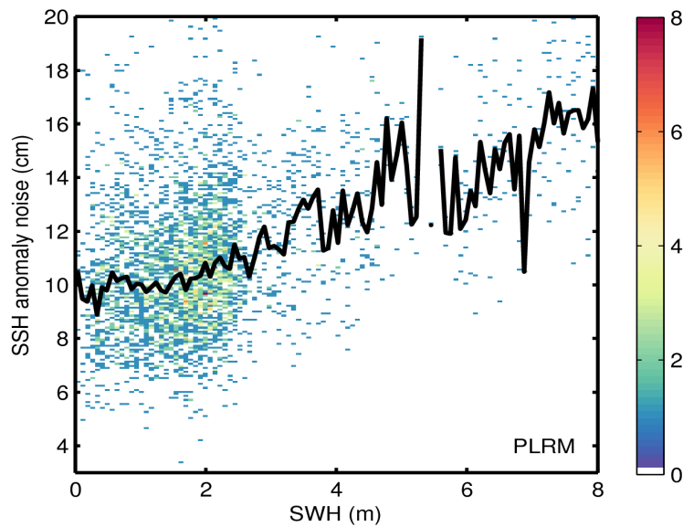
Figure 9. 2D histogram showing flag-valid SSH anomaly noise as a function of SWH for LRM (top) and PLRM (bottom) for 08/06/2017. The black line denotes the median SSH anomaly noise as a function of SWH.
