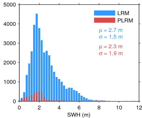
Figure 17. Histogram of flag-valid SWH over oceans and lakes for LRM (blue) and PLRM (red) for 08/06/2017. The mean ( \mu ) and standard deviation ( \sigma ) are also shown. Note that values larger than 12 m are excluded from the histogram for the sake of readability but not from the computation of \mu and \sigma .
