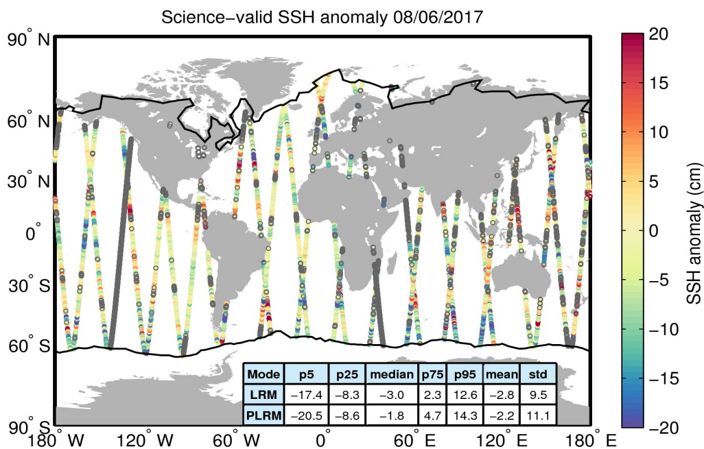
Figure 10. Geographical distribution of science-valid SSH anomaly data over oceans and lakes for 08/06/2017. The statistical values shown in the table refer to the SSH anomaly in cm and are calculated separately for LRM and PLRM regions. The black lines mark the outer limit of the Arctic and Antarctic polar polygons. Gray circles denote records that have been rejected based on the editing criteria described in Table 2.
