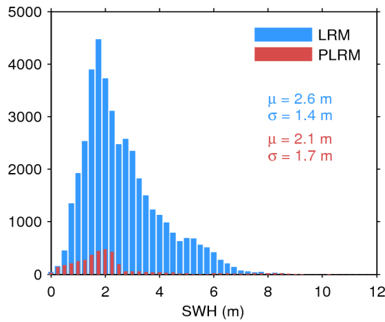
Figure 20. Histogram of science-valid SWH over oceans and lakes for LRM (blue) and PLRM (red) for 08/06/2017. The mean ( \mu ) and standard deviation ( \sigma ) are also shown. Note that values larger than 12 m are excluded from the histogram for the sake of readability but not from the computation of \mu and \sigma .
