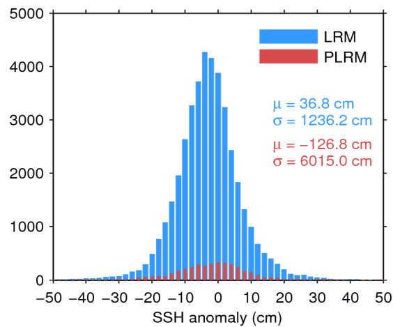
Figure 7. Histogram of flag-valid SSH anomaly over oceans and lakes for LRM (blue) and PLRM (red) for 08/06/2017. The mean ( \mu ) and standard deviation ( \sigma ) are also shown. Note that values outside [-50\ 50] cm are excluded from the histogram for the sake of readability but not from the computation of \mu and \sigma .
