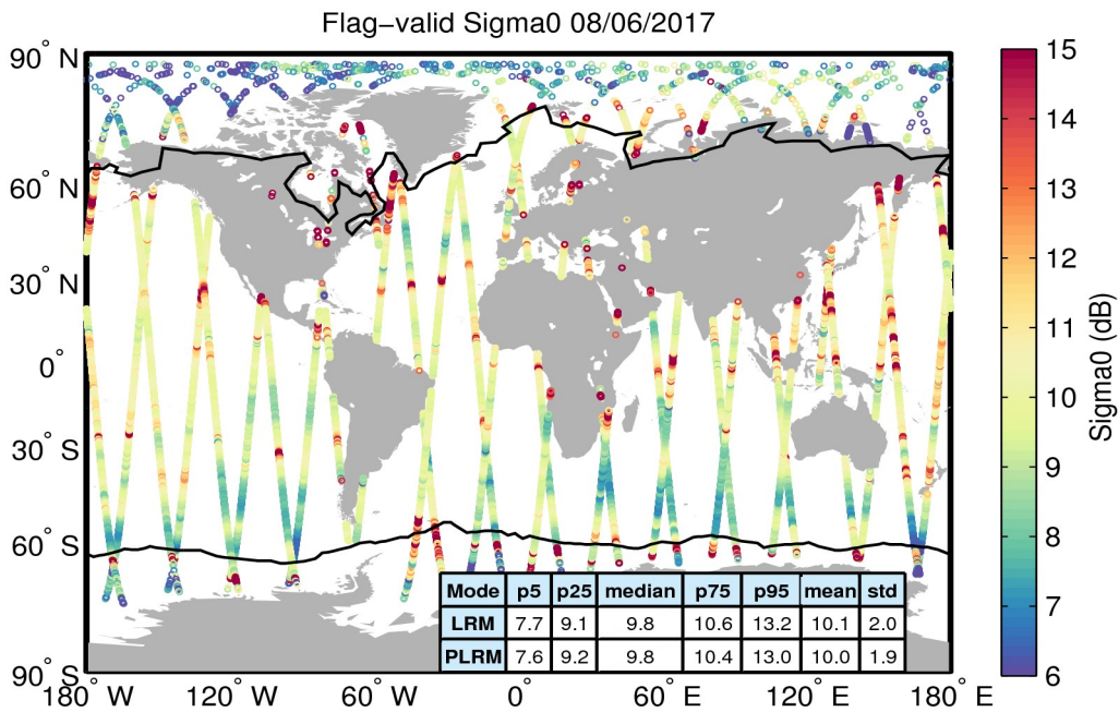
Figure 23. Geographical distribution of flag-valid sigma0 data over oceans and lakes for 08/06/2017. The statistical values shown in the table refer to the sigma0 in dB and are calculated separately for LRM and PLRM regions. Measurements taken over polar polygons have been excluded from the computation of the statistical values. The black lines mark the outer limit of the Arctic and Antarctic polar polygons.
