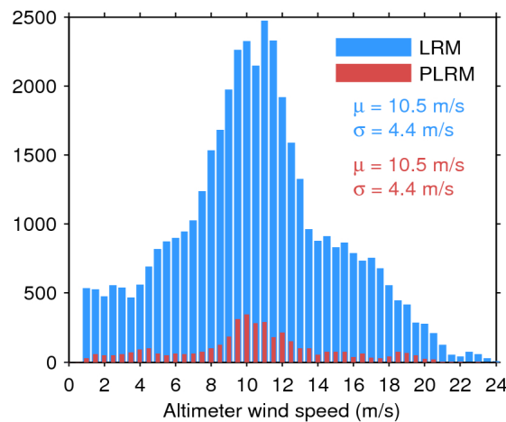
Figure 35. Histogram of science-valid wind over oceans and lakes for LRM (blue) and PLRM (red) for 08/06/2017. The mean ( \mu ) and standard deviation ( \sigma ) are also shown. Note that values larger than 24 m/s are excluded from the histogram for the sake of readability but not from the computation of \mu and \sigma .
