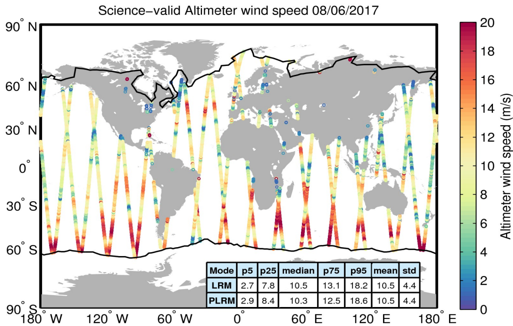
Figure 34. Geographical distribution of science-valid wind data over oceans and lakes for 08/06/2017. The statistical values shown in the table refer to the wind in m/s and are calculated separately for LRM and PLRM regions. The black lines mark the outer limit of the Arctic and Antarctic polar polygons. Gray circles denote records that have been rejected based on the editing criteria described in Table 5.
