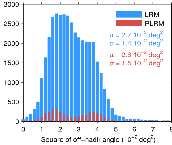
Figure 39. Histogram of flag-valid mispointing over oceans and lakes for LRM (blue) and PLRM (red) for 08/06/2017. Only positive values have been considered. The mean ( \mu ) and standard deviation ( \sigma ) are also shown. Note that values larger than 8 \cdot 10^{-2} \text{ deg}^2 are excluded from the histogram for the sake of readability but not from the computation of \mu and \sigma .
