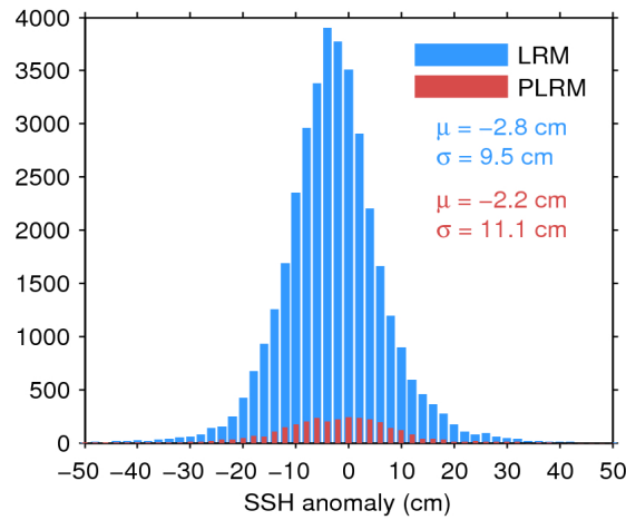
Figure 11. Histogram of science-valid SSH anomaly over oceans and lakes for LRM (blue) and PLRM (red) for 08/06/2017. The mean ( \mu ) and standard deviation ( \sigma ) are also shown. Note that values outside [-50 50] cm are excluded from the histogram for the sake of readability but not from the computation of \mu and \sigma .
