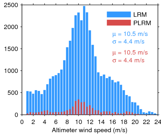
Figure 33. Histogram of flag-valid wind over oceans and lakes for LRM (blue) and PLRM (red) for 08/06/2017. The mean ( \mu ) and standard deviation ( \sigma ) are also shown. Note that values larger than 24 m/s are excluded from the histogram for the sake of readability but not from the computation of \mu and \sigma .
