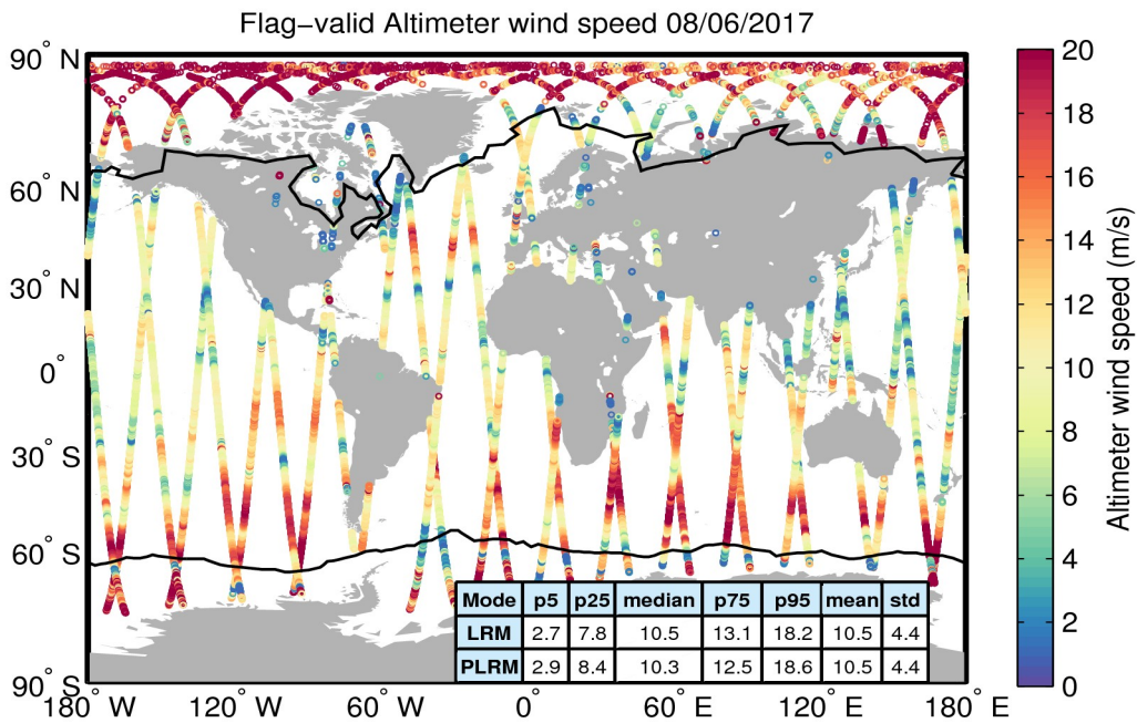
Figure 31. Geographical distribution of flag-valid wind data over oceans and lakes for 08/06/2017. The statistical values shown in the table refer to the wind in m/s and are calculated separately for LRM and PLRM regions. Measurements taken over polar polygons have been excluded from the computation of the statistical values. The black lines mark the outer limit of the Arctic and Antarctic polar polygons.
