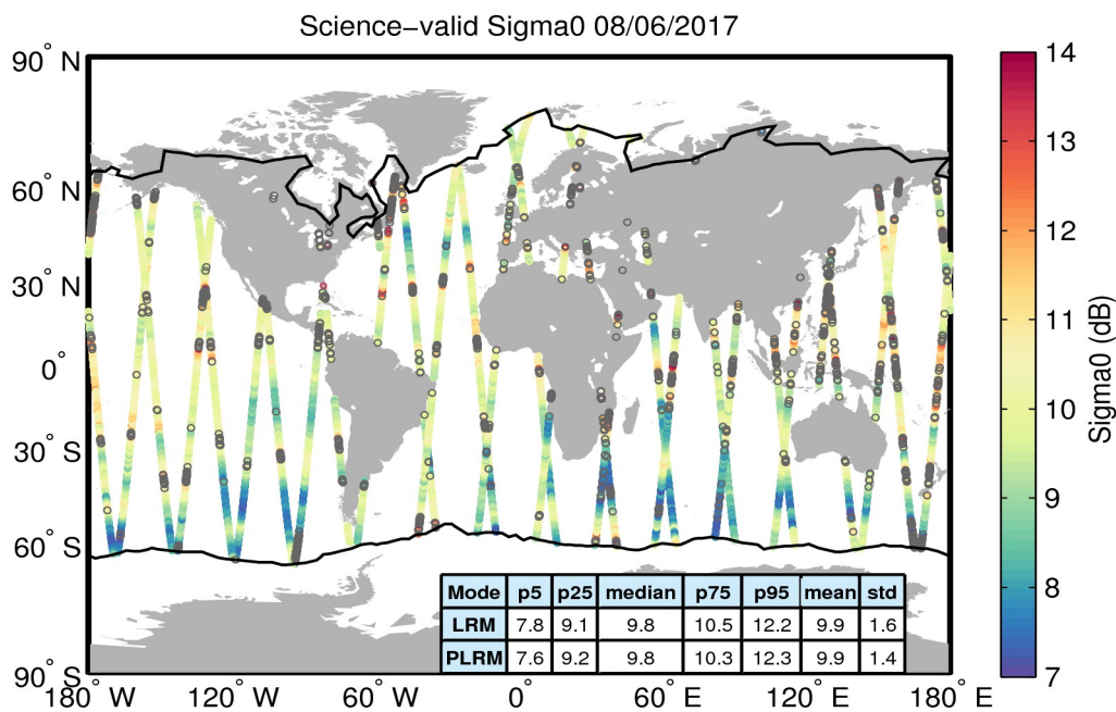
Figure 27. Geographical distribution of science-valid sigma0 data over oceans and lakes for 08/06/2017. The statistical values shown in the table refer to the sigma0 in dB and are calculated separately for LRM and PLRM regions. The black lines mark the outer limit of the Arctic and Antarctic polar polygons. Gray circles denote records that have been rejected based on the editing criteria described in Table 4.
