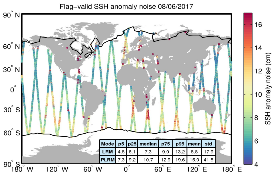
Figure 8. Geographical distribution of flag-valid 20-Hz SSH anomaly measurement noise over oceans and lakes for 08/06/2017. The statistical values shown in the table refer to the SSH anomaly noise and are calculated separately for LRM and PLRM regions. Measurements taken over polar polygons have been excluded from the computation of the statistical values. The black lines mark the outer limit of the Arctic and Antarctic polar polygons.
