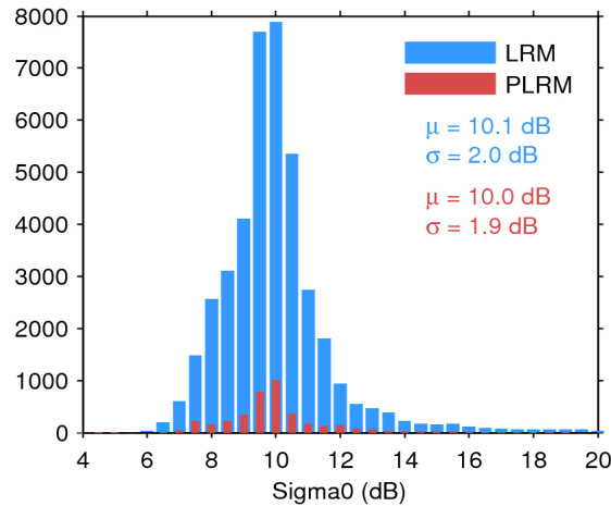
Figure 25. Histogram of flag-valid sigma0 over oceans and lakes for LRM (blue) and PLRM (red) for 08/06/2017. The mean ( \mu ) and standard deviation ( \sigma ) are also shown. Note that values outside [4 20] dB are excluded from the histogram for the sake of readability but not from the computation of \mu and \sigma .
