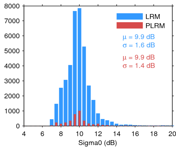
Figure 28. Histogram of science-valid sigma0 over oceans and lakes for LRM (blue) and PLRM (red) for 08/06/2017. The mean ( \mu ) and standard deviation ( \sigma ) are also shown. Note that values outside [4 20] dB are excluded from the histogram for the sake of readability but not from the computation of \mu and \sigma .
