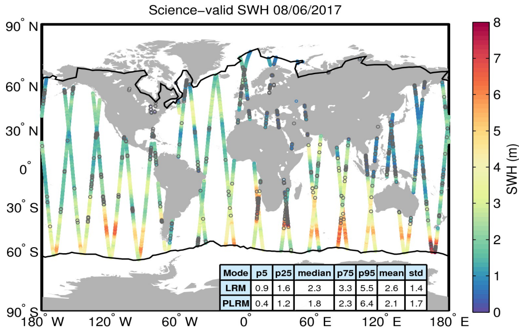
Figure 19. Geographical distribution of science-valid SWH data over oceans and lakes for 08/06/2017. The statistical values shown in the table refer to the SWH in m and are calculated separately for LRM and PLRM regions. The black lines mark the outer limit of the Arctic and Antarctic polar polygons. Gray circles denote records that have been rejected based on the editing criteria described in Table 3.
