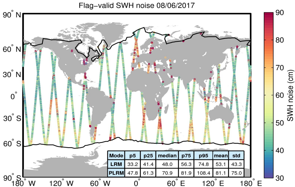
Figure 18. Geographical distribution of flag-valid 20-Hz SWH measurement noise over oceans and lakes for 08/06/2017. The statistical values shown in the table refer to the SWH noise and are calculated separately for LRM and PLRM regions. Measurements taken over polar polygons have been excluded from the computation of the statistical values. The black lines mark the outer limit of the Arctic and Antarctic polar polygons.
