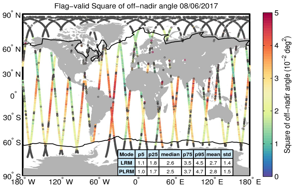
Figure 37. Geographical distribution of flag-valid mispointing data over oceans and lakes for 08/06/2017. The statistical values shown in the table refer to the mispointing in 10^{-2} deg 2 and are calculated separately for LRM and PLRM regions. Measurements taken over polar polygons have been excluded from the computation of the statistical values. The black lines mark the outer limit of the Arctic and Antarctic polar polygons. Gray circles denote negative values.
