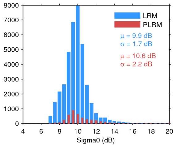
Figure 28. Histogram of science-valid sigma0 over oceans and lakes for LRM (blue) and PLRM (red) for 07/06/2017. The mean ( \mu ) and standard deviation ( \sigma ) are also shown. Note that values outside [4 20] dB are excluded from the histogram for the sake of readability but not from the computation of \mu and \sigma .
