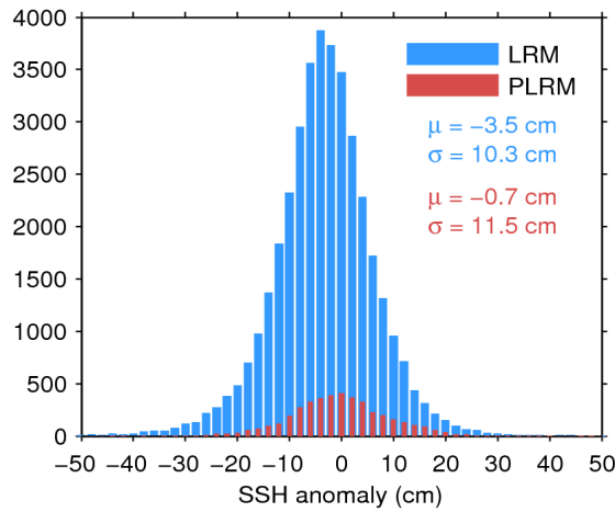
Figure 11. Histogram of science-valid SSH anomaly over oceans and lakes for LRM (blue) and PLRM (red) for 07/06/2017. The mean ( \mu ) and standard deviation ( \sigma ) are also shown. Note that values outside [-50 50] cm are excluded from the histogram for the sake of readability but not from the computation of \mu and \sigma .
