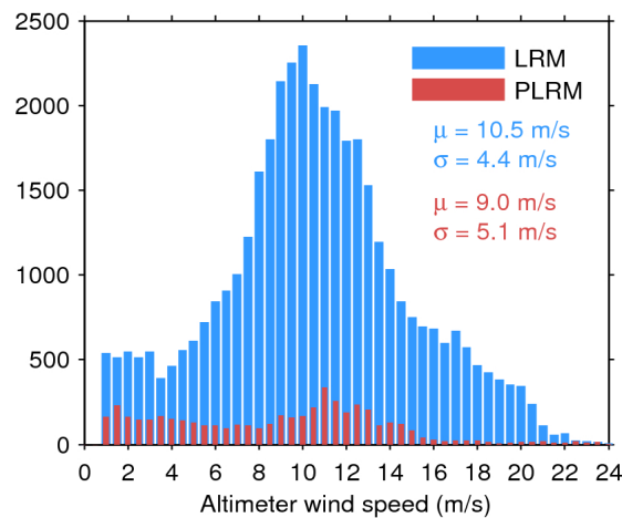
Figure 35. Histogram of science-valid wind over oceans and lakes for LRM (blue) and PLRM (red) for 07/06/2017. The mean ( \mu ) and standard deviation ( \sigma ) are also shown. Note that values larger than 24 m/s are excluded from the histogram for the sake of readability but not from the computation of \mu and \sigma .
