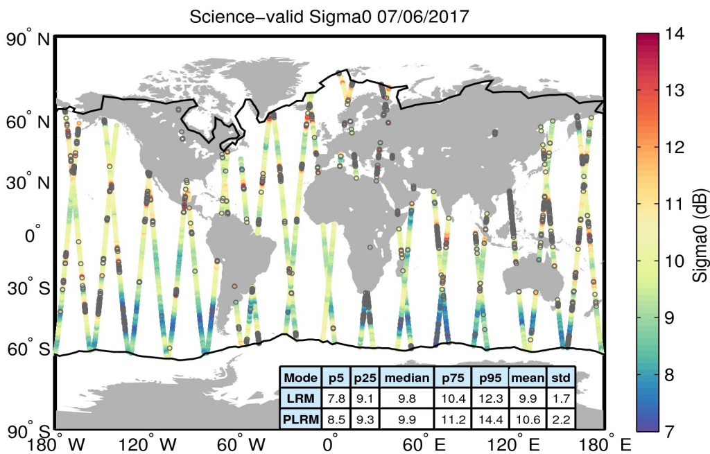
Figure 27. Geographical distribution of science-valid sigma0 data over oceans and lakes for 07/06/2017. The statistical values shown in the table refer to the sigma0 in dB and are calculated separately for LRM and PLRM regions. The black lines mark the outer limit of the Arctic and Antarctic polar polygons. Gray circles denote records that have been rejected based on the editing criteria described in Table 4.
