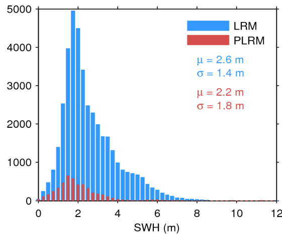
Figure 17. Histogram of flag-valid SWH over oceans and lakes for LRM (blue) and PLRM (red) for 07/06/2017. The mean ( \mu ) and standard deviation ( \sigma ) are also shown. Note that values larger than 12 m are excluded from the histogram for the sake of readability but not from the computation of \mu and \sigma .
