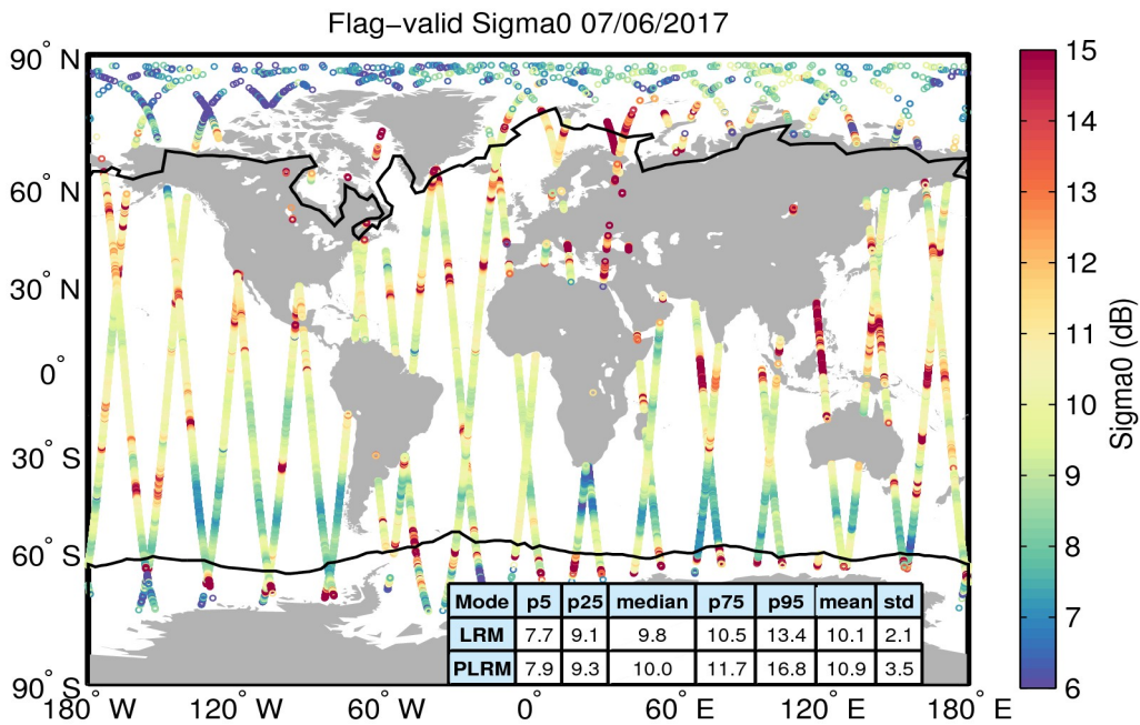
Figure 23. Geographical distribution of flag-valid sigma0 data over oceans and lakes for 07/06/2017. The statistical values shown in the table refer to the sigma0 in dB and are calculated separately for LRM and PLRM regions. Measurements taken over polar polygons have been excluded from the computation of the statistical values. The black lines mark the outer limit of the Arctic and Antarctic polar polygons.
