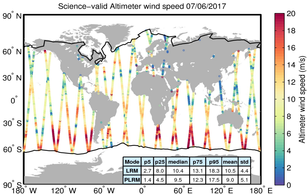
Figure 34. Geographical distribution of science-valid wind data over oceans and lakes for 07/06/2017. The statistical values shown in the table refer to the wind in m/s and are calculated separately for LRM and PLRM regions. The black lines mark the outer limit of the Arctic and Antarctic polar polygons. Gray circles denote records that have been rejected based on the editing criteria described in Table 5.
