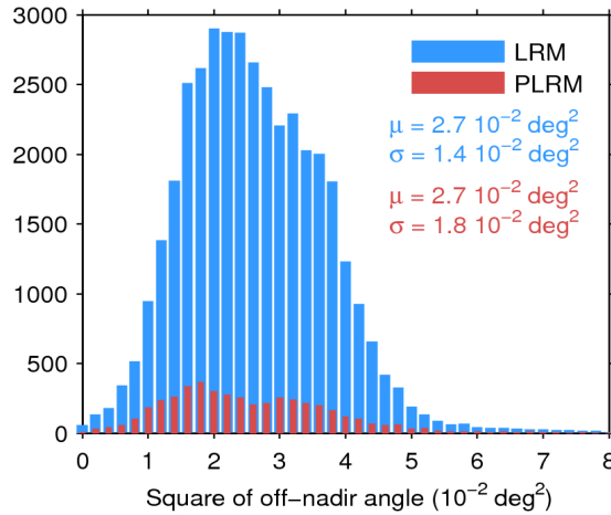
Figure 39. Histogram of flag-valid mispointing over oceans and lakes for LRM (blue) and PLRM (red) for 07/06/2017. Only positive values have been considered. The mean ( \mu ) and standard deviation ( \sigma ) are also shown. Note that values larger than 8 \cdot 10^{-2} \text{ deg}^2 are excluded from the histogram for the sake of readability but not from the computation of \mu and \sigma .
