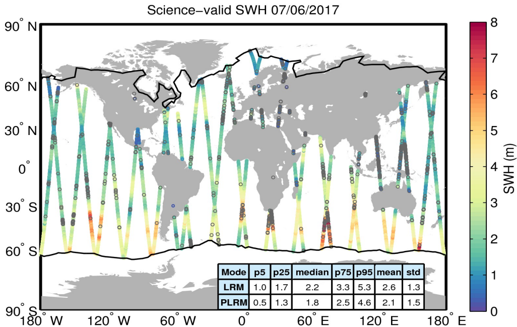
Figure 19. Geographical distribution of science-valid SWH data over oceans and lakes for 07/06/2017. The statistical values shown in the table refer to the SWH in m and are calculated separately for LRM and PLRM regions. The black lines mark the outer limit of the Arctic and Antarctic polar polygons. Gray circles denote records that have been rejected based on the editing criteria described in Table 3.
