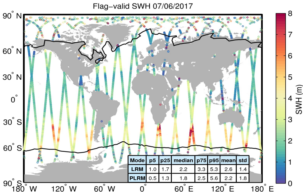
Figure 15. Geographical distribution of flag-valid SWH data over oceans and lakes for 07/06/2017. The statistical values shown in the table refer to the SWH in m and are calculated separately for LRM and PLRM regions. Measurements taken over polar polygons have been excluded from the computation of the statistical values. The black lines mark the outer limit of the Arctic and Antarctic polar polygons.
