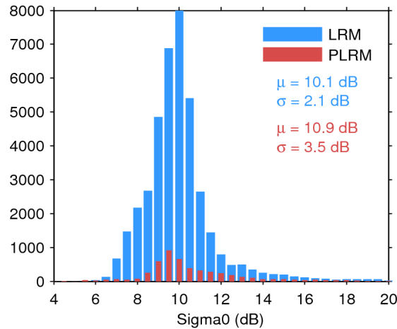
Figure 25. Histogram of flag-valid sigma0 over oceans and lakes for LRM (blue) and PLRM (red) for 07/06/2017. The mean ( \mu ) and standard deviation ( \sigma ) are also shown. Note that values outside [4 20] dB are excluded from the histogram for the sake of readability but not from the computation of \mu and \sigma .
