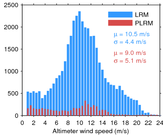
Figure 33. Histogram of flag-valid wind over oceans and lakes for LRM (blue) and PLRM (red) for 07/06/2017. The mean ( \mu ) and standard deviation ( \sigma ) are also shown. Note that values larger than 24 m/s are excluded from the histogram for the sake of readability but not from the computation of \mu and \sigma .
