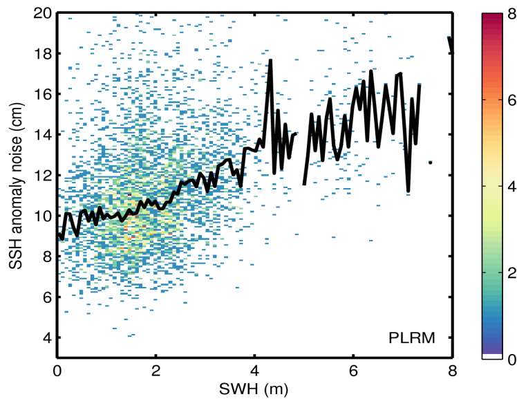
Figure 9. 2D histogram showing flag-valid SSH anomaly noise as a function of SWH for LRM (top) and PLRM (bottom) for 07/06/2017. The black line denotes the median SSH anomaly noise as a function of SWH.
