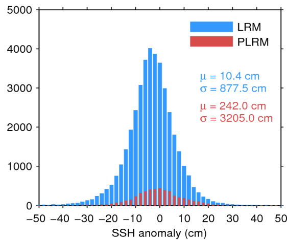
Figure 7. Histogram of flag-valid SSH anomaly over oceans and lakes for LRM (blue) and PLRM (red) for 07/06/2017. The mean ( \mu ) and standard deviation ( \sigma ) are also shown. Note that values outside [-50 50] cm are excluded from the histogram for the sake of readability but not from the computation of \mu and \sigma .
