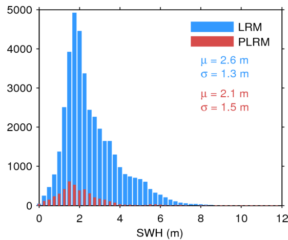
Figure 20. Histogram of science-valid SWH over oceans and lakes for LRM (blue) and PLRM (red) for 07/06/2017. The mean ( \mu ) and standard deviation ( \sigma ) are also shown. Note that values larger than 12 m are excluded from the histogram for the sake of readability but not from the computation of \mu and \sigma .
