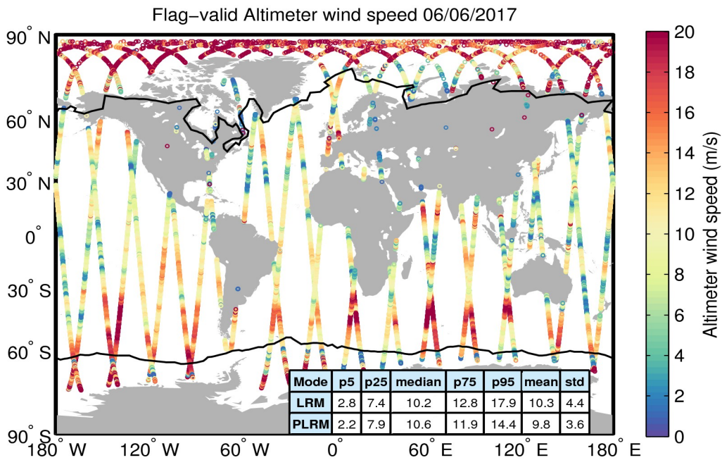
Figure 31. Geographical distribution of flag-valid wind data over oceans and lakes for 06/06/2017. The statistical values shown in the table refer to the wind in m/s and are calculated separately for LRM and PLRM regions. Measurements taken over polar polygons have been excluded from the computation of the statistical values. The black lines mark the outer limit of the Arctic and Antarctic polar polygons.
