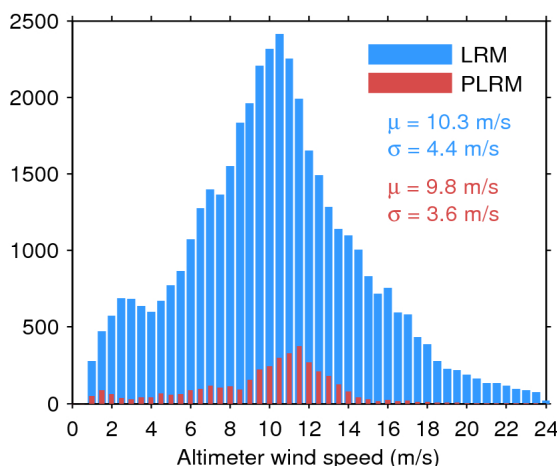
Figure 33. Histogram of flag-valid wind over oceans and lakes for LRM (blue) and PLRM (red) for 06/06/2017. The mean ( \mu ) and standard deviation ( \sigma ) are also shown. Note that values larger than 24 m/s are excluded from the histogram for the sake of readability but not from the computation of \mu and \sigma .
