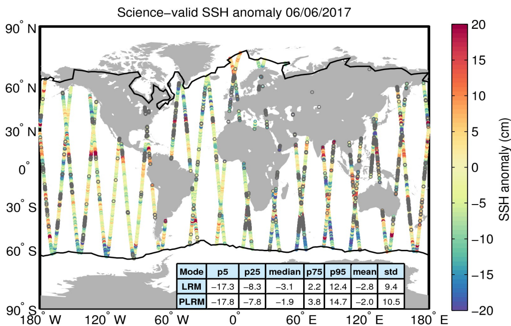
Figure 10. Geographical distribution of science-valid SSH anomaly data over oceans and lakes for 06/06/2017. The statistical values shown in the table refer to the SSH anomaly in cm and are calculated separately for LRM and PLRM regions. The black lines mark the outer limit of the Arctic and Antarctic polar polygons. Gray circles denote records that have been rejected based on the editing criteria described in Table 2.
