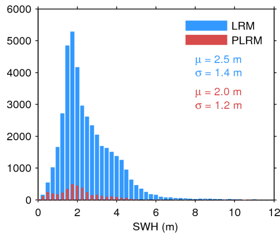
Figure 17. Histogram of flag-valid SWH over oceans and lakes for LRM (blue) and PLRM (red) for 06/06/2017. The mean ( \mu ) and standard deviation ( \sigma ) are also shown. Note that values larger than 12 m are excluded from the histogram for the sake of readability but not from the computation of \mu and \sigma .
