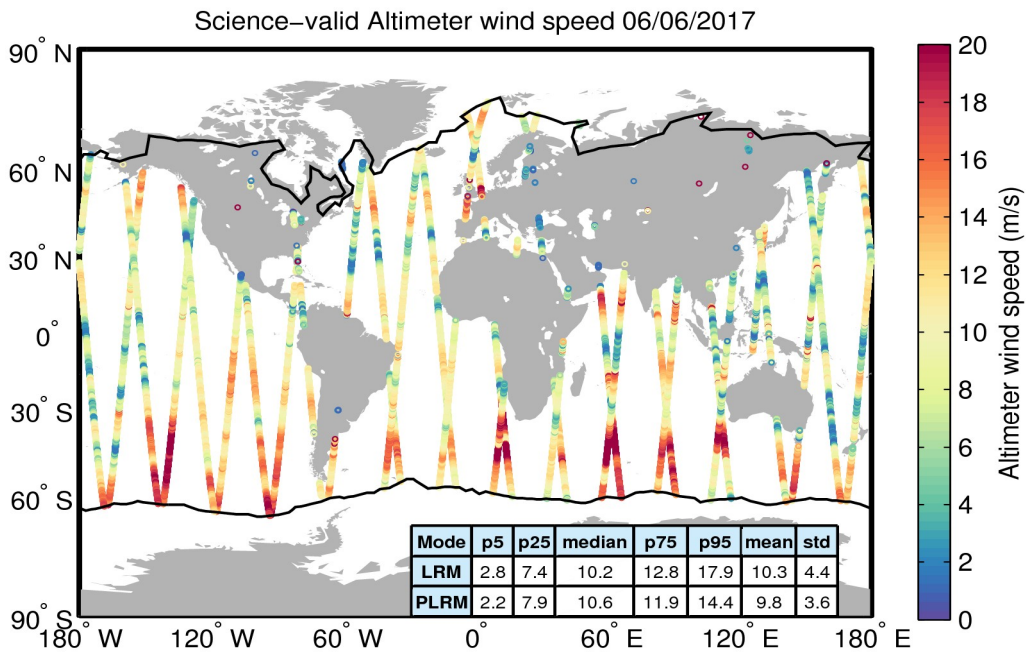
Figure 34. Geographical distribution of science-valid wind data over oceans and lakes for 06/06/2017. The statistical values shown in the table refer to the wind in m/s and are calculated separately for LRM and PLRM regions. The black lines mark the outer limit of the Arctic and Antarctic polar polygons. Gray circles denote records that have been rejected based on the editing criteria described in Table 5.
