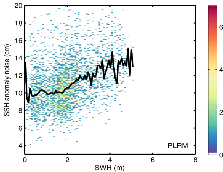
Figure 9. 2D histogram showing flag-valid SSH anomaly noise as a function of SWH for LRM (top) and PLRM (bottom) for 06/06/2017. The black line denotes the median SSH anomaly noise as a function of SWH.
