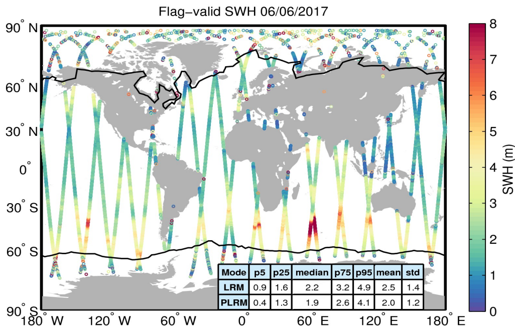
Figure 15. Geographical distribution of flag-valid SWH data over oceans and lakes for 06/06/2017. The statistical values shown in the table refer to the SWH in m and are calculated separately for LRM and PLRM regions. Measurements taken over polar polygons have been excluded from the computation of the statistical values. The black lines mark the outer limit of the Arctic and Antarctic polar polygons.
