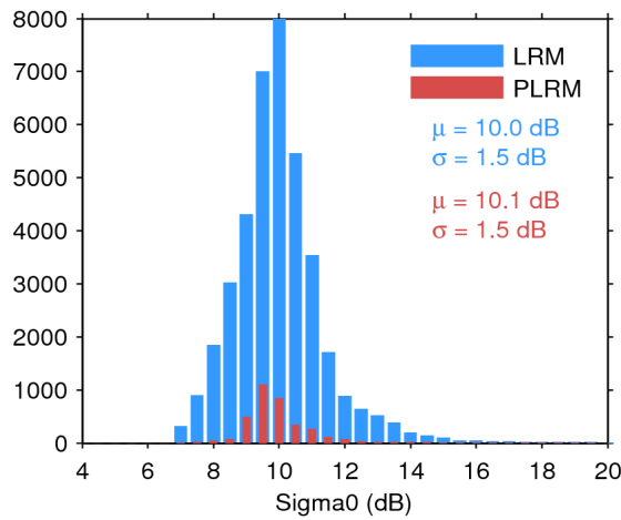
Figure 28. Histogram of science-valid sigma0 over oceans and lakes for LRM (blue) and PLRM (red) for 06/06/2017. The mean ( \mu ) and standard deviation ( \sigma ) are also shown. Note that values outside [4 20] dB are excluded from the histogram for the sake of readability but not from the computation of \mu and \sigma .
