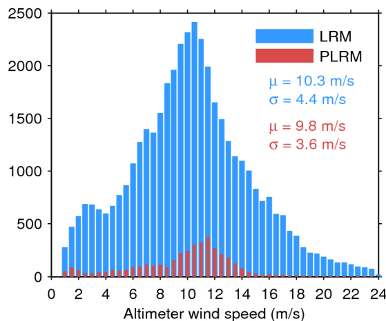
Figure 35. Histogram of science-valid wind over oceans and lakes for LRM (blue) and PLRM (red) for 06/06/2017. The mean ( \mu ) and standard deviation ( \sigma ) are also shown. Note that values larger than 24 m/s are excluded from the histogram for the sake of readability but not from the computation of \mu and \sigma .
