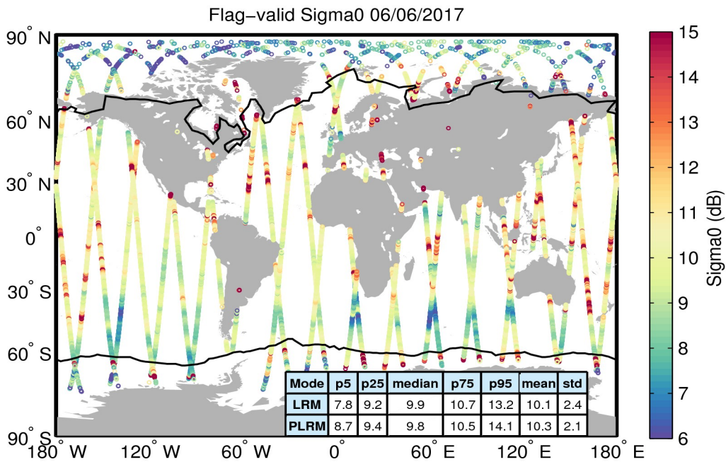
Figure 23. Geographical distribution of flag-valid sigma0 data over oceans and lakes for 06/06/2017. The statistical values shown in the table refer to the sigma0 in dB and are calculated separately for LRM and PLRM regions. Measurements taken over polar polygons have been excluded from the computation of the statistical values. The black lines mark the outer limit of the Arctic and Antarctic polar polygons.
