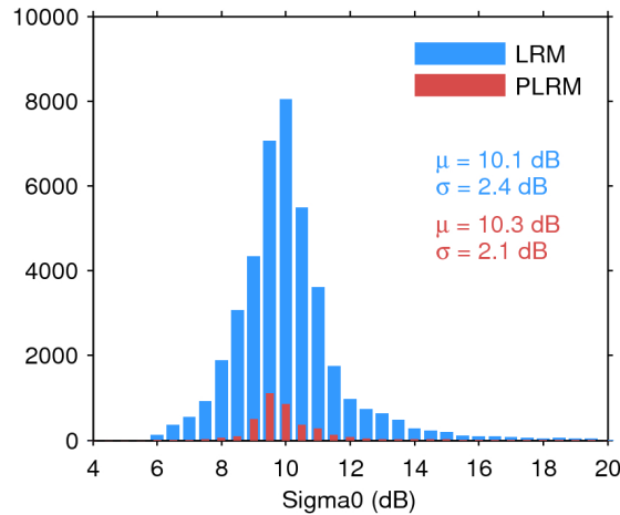
Figure 25. Histogram of flag-valid sigma0 over oceans and lakes for LRM (blue) and PLRM (red) for 06/06/2017. The mean ( \mu ) and standard deviation ( \sigma ) are also shown. Note that values outside [4 20] dB are excluded from the histogram for the sake of readability but not from the computation of \mu and \sigma .
