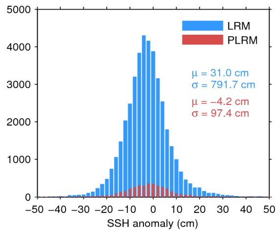
Figure 7. Histogram of flag-valid SSH anomaly over oceans and lakes for LRM (blue) and PLRM (red) for 06/06/2017. The mean ( \mu ) and standard deviation ( \sigma ) are also shown. Note that values outside [-50 \ 50] cm are excluded from the histogram for the sake of readability but not from the computation of \mu and \sigma .
