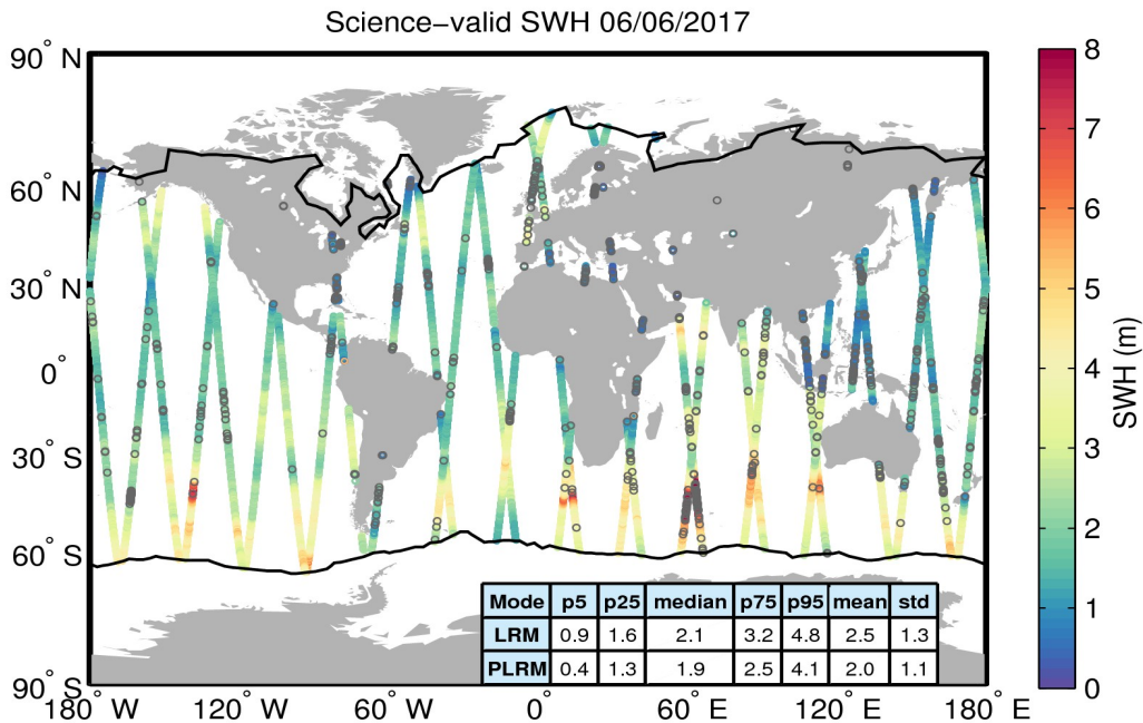
Figure 19. Geographical distribution of science-valid SWH data over oceans and lakes for 06/06/2017. The statistical values shown in the table refer to the SWH in m and are calculated separately for LRM and PLRM regions. The black lines mark the outer limit of the Arctic and Antarctic polar polygons. Gray circles denote records that have been rejected based on the editing criteria described in Table 3.
