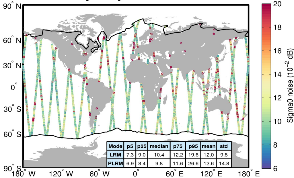
Flag-valid sigma0 noise 06/06/2017
