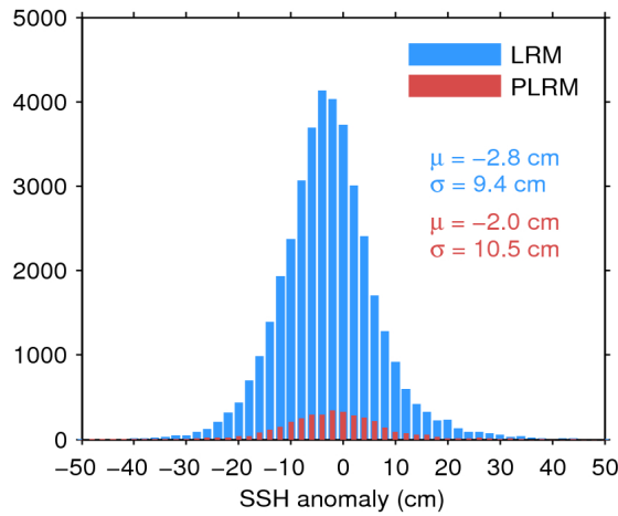
Figure 11. Histogram of science-valid SSH anomaly over oceans and lakes for LRM (blue) and PLRM (red) for 06/06/2017. The mean ( \mu ) and standard deviation ( \sigma ) are also shown. Note that values outside [-50\ 50] cm are excluded from the histogram for the sake of readability but not from the computation of \mu and \sigma .
