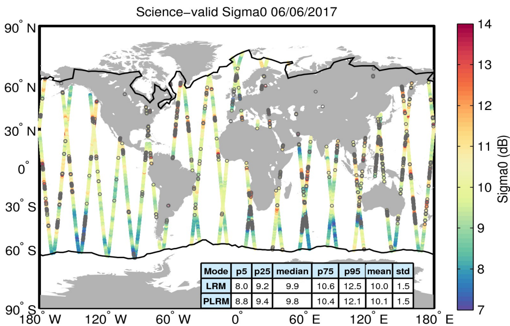
Figure 27. Geographical distribution of science-valid sigma0 data over oceans and lakes for 06/06/2017. The statistical values shown in the table refer to the sigma0 in dB and are calculated separately for LRM and PLRM regions. The black lines mark the outer limit of the Arctic and Antarctic polar polygons. Gray circles denote records that have been rejected based on the editing criteria described in Table 4.
