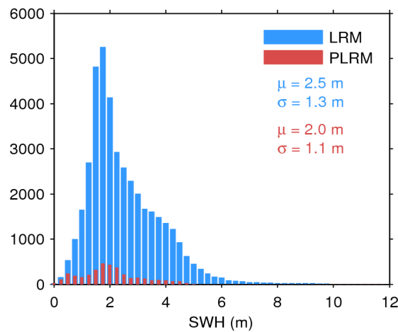
Figure 20. Histogram of science-valid SWH over oceans and lakes for LRM (blue) and PLRM (red) for 06/06/2017. The mean ( \mu ) and standard deviation ( \sigma ) are also shown. Note that values larger than 12 m are excluded from the histogram for the sake of readability but not from the computation of \mu and \sigma .
