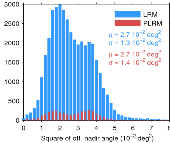
Figure 39. Histogram of flag-valid mispointing over oceans and lakes for LRM (blue) and PLRM (red) for 06/06/2017. Only positive values have been considered. The mean ( \mu ) and standard deviation ( \sigma ) are also shown. Note that values larger than 8 \cdot 10^{-2} \text{ deg}^2 are excluded from the histogram for the sake of readability but not from the computation of \mu and \sigma .
