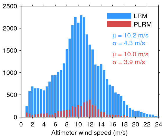
Figure 33. Histogram of flag-valid wind over oceans and lakes for LRM (blue) and PLRM (red) for 05/06/2017. The mean ( \mu ) and standard deviation ( \sigma ) are also shown. Note that values larger than 24 m/s are excluded from the histogram for the sake of readability but not from the computation of \mu and \sigma .
