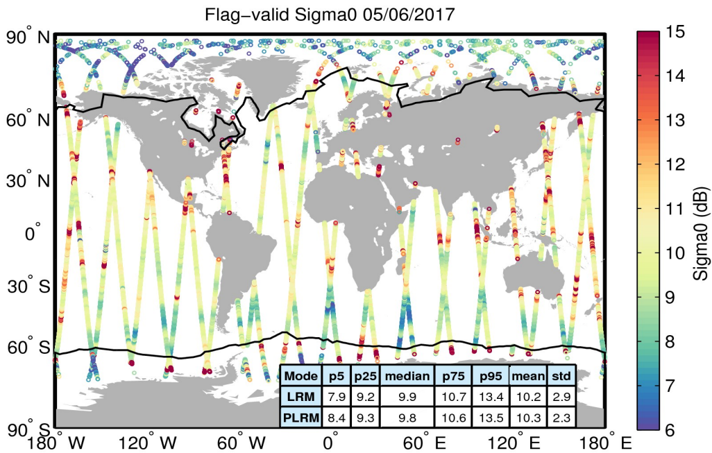
Figure 23. Geographical distribution of flag-valid sigma0 data over oceans and lakes for 05/06/2017. The statistical values shown in the table refer to the sigma0 in dB and are calculated separately for LRM and PLRM regions. Measurements taken over polar polygons have been excluded from the computation of the statistical values. The black lines mark the outer limit of the Arctic and Antarctic polar polygons.
