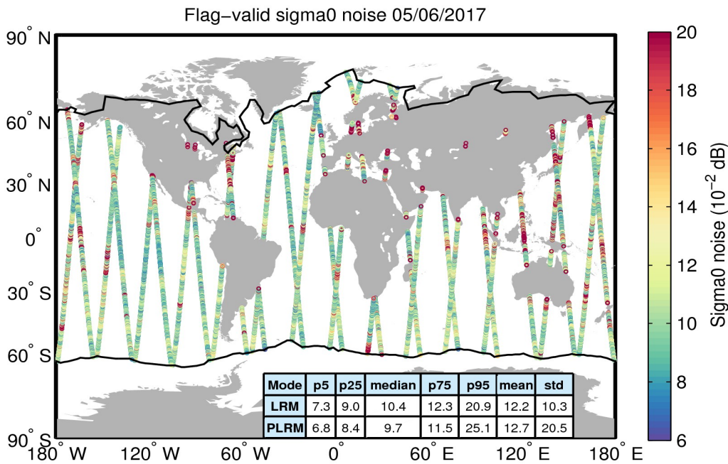
Figure 26. Geographical distribution of flag-valid 20-Hz sigma0 measurement noise over oceans and lakes for 05/06/2017. The statistical values shown in the table refer to the sigma0 noise and are calculated separately for LRM and PLRM regions. Measurements taken over polar polygons have been excluded from the computation of the statistical values. The black lines mark the outer limit of the Arctic and Antarctic polar polygons.
