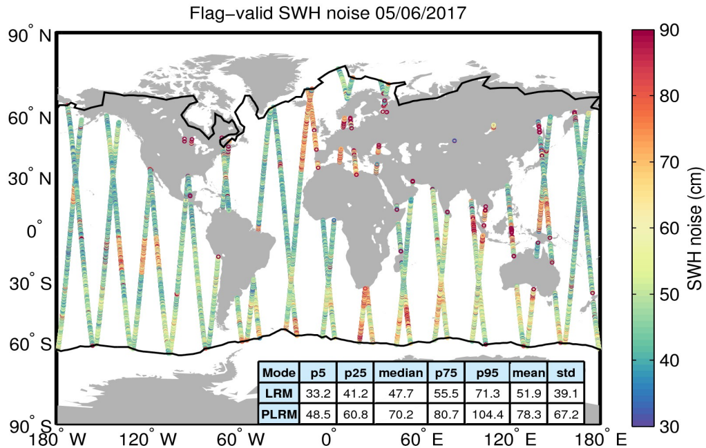
Figure 18. Geographical distribution of flag-valid 20-Hz SWH measurement noise over oceans and lakes for 05/06/2017. The statistical values shown in the table refer to the SWH noise and are calculated separately for LRM and PLRM regions. Measurements taken over polar polygons have been excluded from the computation of the statistical values. The black lines mark the outer limit of the Arctic and Antarctic polar polygons.
