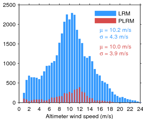
Figure 35. Histogram of science-valid wind over oceans and lakes for LRM (blue) and PLRM (red) for 05/06/2017. The mean ( \mu ) and standard deviation ( \sigma ) are also shown. Note that values larger than 24 m/s are excluded from the histogram for the sake of readability but not from the computation of \mu and \sigma .
