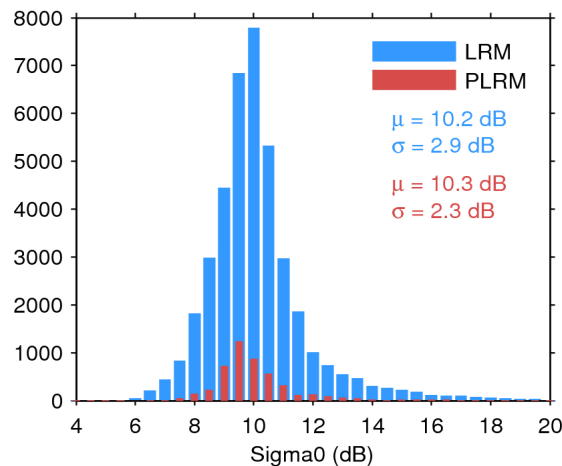
Figure 25. Histogram of flag-valid sigma0 over oceans and lakes for LRM (blue) and PLRM (red) for 05/06/2017. The mean ( \mu ) and standard deviation ( \sigma ) are also shown. Note that values outside [4 20] dB are excluded from the histogram for the sake of readability but not from the computation of \mu and \sigma .
