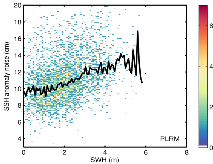
Figure 9. 2D histogram showing flag-valid SSH anomaly noise as a function of SWH for LRM (top) and PLRM (bottom) for 05/06/2017. The black line denotes the median SSH anomaly noise as a function of SWH.
