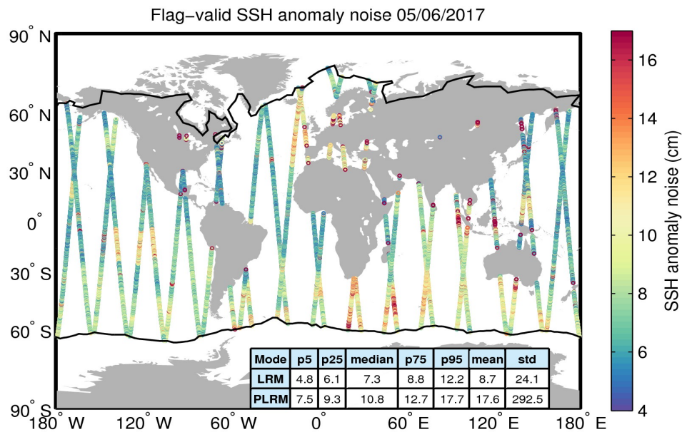
Figure 8. Geographical distribution of flag-valid 20-Hz SSH anomaly measurement noise over oceans and lakes for 05/06/2017. The statistical values shown in the table refer to the SSH anomaly noise and are calculated separately for LRM and PLRM regions. Measurements taken over polar polygons have been excluded from the computation of the statistical values. The black lines mark the outer limit of the Arctic and Antarctic polar polygons.
