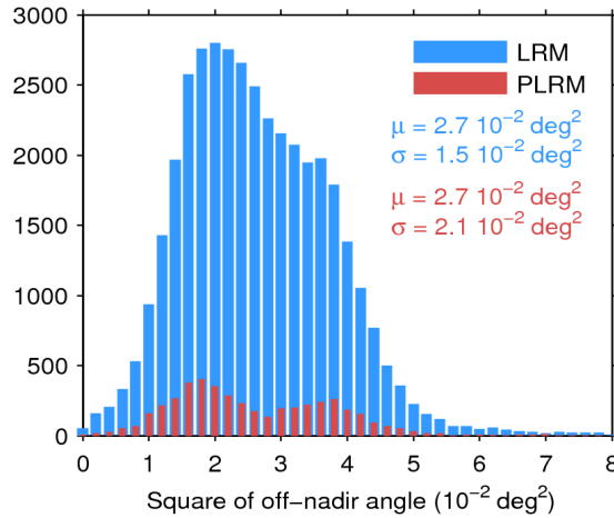
Figure 39. Histogram of flag-valid mispointing over oceans and lakes for LRM (blue) and PLRM (red) for 05/06/2017. Only positive values have been considered. The mean ( \mu ) and standard deviation ( \sigma ) are also shown. Note that values larger than 8 \cdot 10^{-2} \text{ deg}^2 are excluded from the histogram for the sake of readability but not from the computation of \mu and \sigma .
