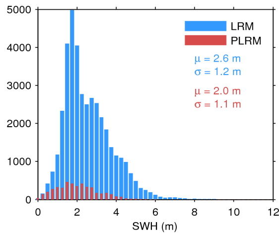
Figure 20. Histogram of science-valid SWH over oceans and lakes for LRM (blue) and PLRM (red) for 05/06/2017. The mean ( \mu ) and standard deviation ( \sigma ) are also shown. Note that values larger than 12 m are excluded from the histogram for the sake of readability but not from the computation of \mu and \sigma .
