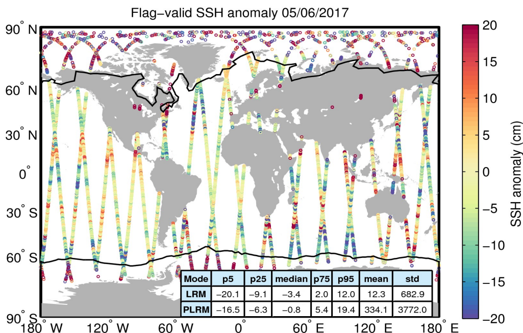
Figure 5. Geographical distribution of flag-valid 1-Hz SSH anomaly data over oceans and lakes for 05/06/2017. The statistical values shown in the table refer to the SSH anomaly in cm and are calculated separately for LRM and PLRM regions. Measurements taken over polar polygons have been excluded from the computation of the statistical values. The black lines mark the outer limit of the Arctic and Antarctic polar polygons.
