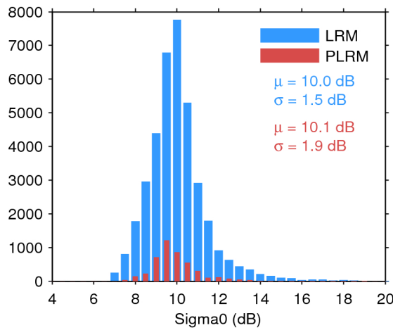
Figure 28. Histogram of science-valid sigma0 over oceans and lakes for LRM (blue) and PLRM (red) for 05/06/2017. The mean ( \mu ) and standard deviation ( \sigma ) are also shown. Note that values outside [4 20] dB are excluded from the histogram for the sake of readability but not from the computation of \mu and \sigma .
