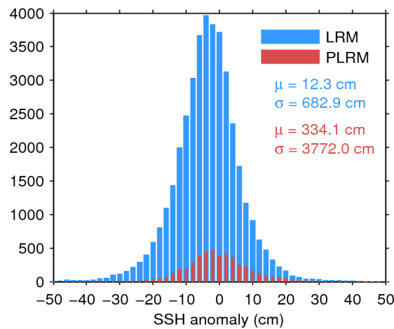
Figure 7. Histogram of flag-valid SSH anomaly over oceans and lakes for LRM (blue) and PLRM (red) for 05/06/2017. The mean ( \mu ) and standard deviation ( \sigma ) are also shown. Note that values outside [-50\ 50] cm are excluded from the histogram for the sake of readability but not from the computation of \mu and \sigma .
