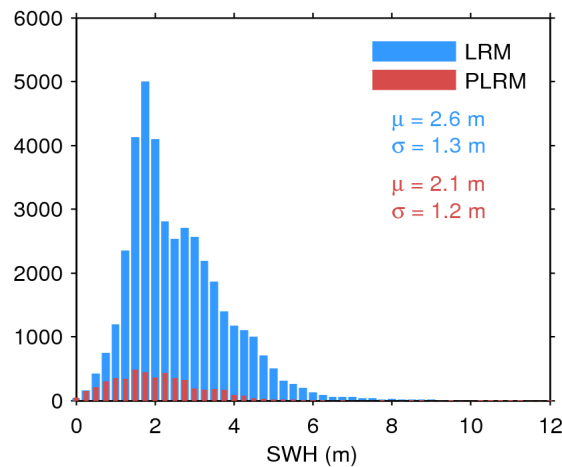
Figure 17. Histogram of flag-valid SWH over oceans and lakes for LRM (blue) and PLRM (red) for 05/06/2017. The mean ( \mu ) and standard deviation ( \sigma ) are also shown. Note that values larger than 12 m are excluded from the histogram for the sake of readability but not from the computation of \mu and \sigma .
