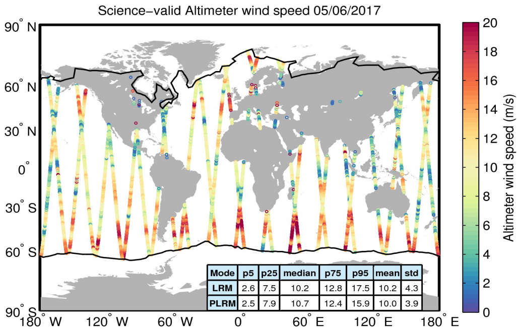
Figure 34. Geographical distribution of science-valid wind data over oceans and lakes for 05/06/2017. The statistical values shown in the table refer to the wind in m/s and are calculated separately for LRM and PLRM regions. The black lines mark the outer limit of the Arctic and Antarctic polar polygons. Gray circles denote records that have been rejected based on the editing criteria described in Table 5.
