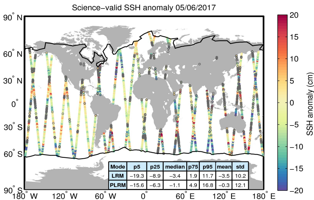
Figure 10. Geographical distribution of science-valid SSH anomaly data over oceans and lakes for 05/06/2017. The statistical values shown in the table refer to the SSH anomaly in cm and are calculated separately for LRM and PLRM regions. The black lines mark the outer limit of the Arctic and Antarctic polar polygons. Gray circles denote records that have been rejected based on the editing criteria described in Table 2.
