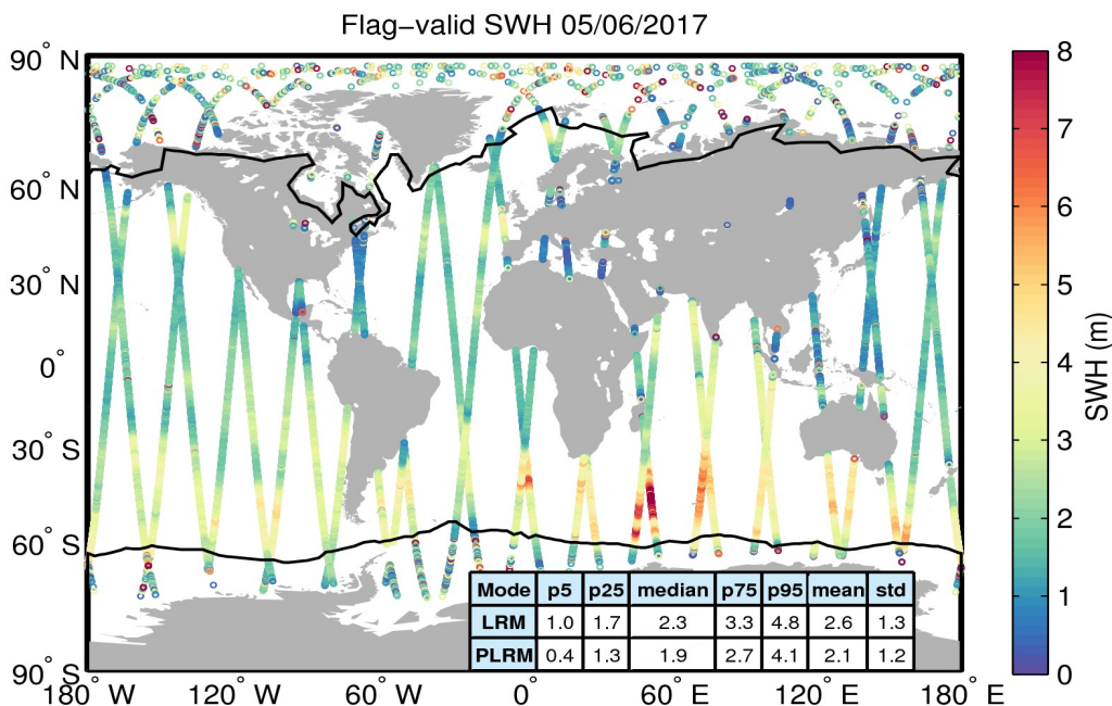
Figure 15. Geographical distribution of flag-valid SWH data over oceans and lakes for 05/06/2017. The statistical values shown in the table refer to the SWH in m and are calculated separately for LRM and PLRM regions. Measurements taken over polar polygons have been excluded from the computation of the statistical values. The black lines mark the outer limit of the Arctic and Antarctic polar polygons.
