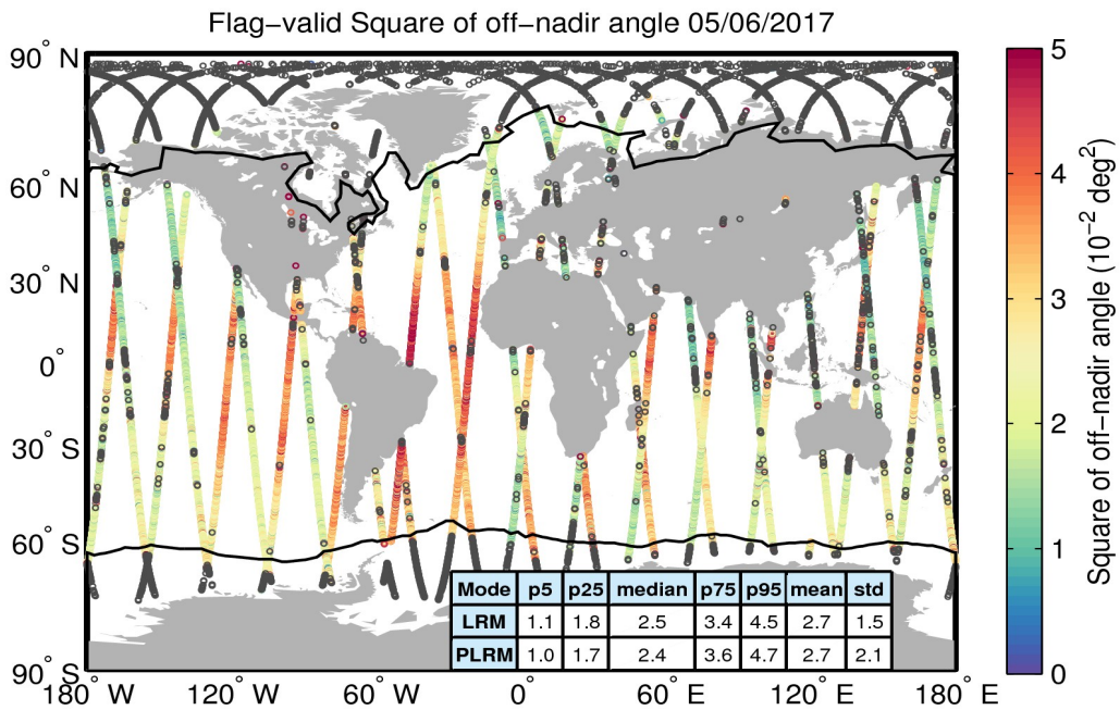
Figure 37. Geographical distribution of flag-valid mispointing data over oceans and lakes for 05/06/2017. The statistical values shown in the table refer to the mispointing in 10^{-2} deg 2 and are calculated separately for LRM and PLRM regions. Measurements taken over polar polygons have been excluded from the computation of the statistical values. The black lines mark the outer limit of the Arctic and Antarctic polar polygons. Gray circles denote negative values.
