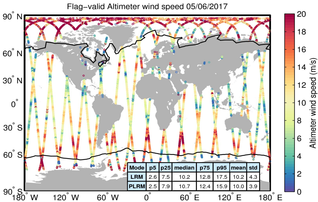
Figure 31. Geographical distribution of flag-valid wind data over oceans and lakes for 05/06/2017. The statistical values shown in the table refer to the wind in m/s and are calculated separately for LRM and PLRM regions. Measurements taken over polar polygons have been excluded from the computation of the statistical values. The black lines mark the outer limit of the Arctic and Antarctic polar polygons.
