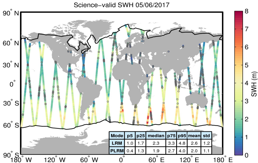
Figure 19. Geographical distribution of science-valid SWH data over oceans and lakes for 05/06/2017. The statistical values shown in the table refer to the SWH in m and are calculated separately for LRM and PLRM regions. The black lines mark the outer limit of the Arctic and Antarctic polar polygons. Gray circles denote records that have been rejected based on the editing criteria described in Table 3.
