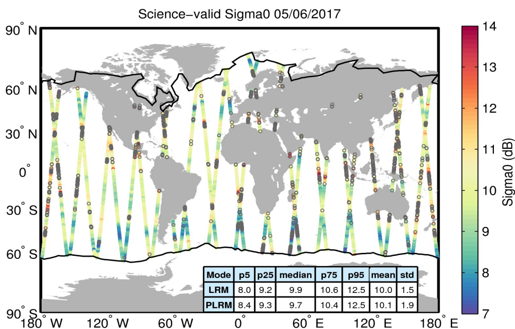
Figure 27. Geographical distribution of science-valid sigma0 data over oceans and lakes for 05/06/2017. The statistical values shown in the table refer to the sigma0 in dB and are calculated separately for LRM and PLRM regions. The black lines mark the outer limit of the Arctic and Antarctic polar polygons. Gray circles denote records that have been rejected based on the editing criteria described in Table 4.
