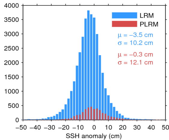
Figure 11. Histogram of science-valid SSH anomaly over oceans and lakes for LRM (blue) and PLRM (red) for 05/06/2017. The mean ( \mu ) and standard deviation ( \sigma ) are also shown. Note that values outside [-50\ 50] cm are excluded from the histogram for the sake of readability but not from the computation of \mu and \sigma .
