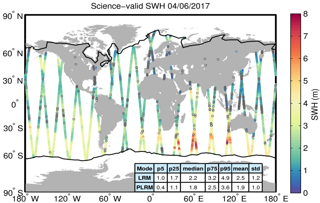
Figure 19. Geographical distribution of science-valid SWH data over oceans and lakes for 04/06/2017. The statistical values shown in the table refer to the SWH in m and are calculated separately for LRM and PLRM regions. The black lines mark the outer limit of the Arctic and Antarctic polar polygons. Gray circles denote records that have been rejected based on the editing criteria described in Table 3.
