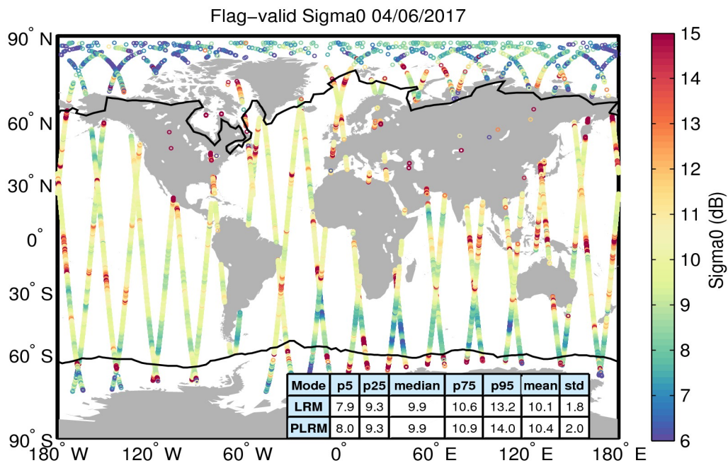
Figure 23. Geographical distribution of flag-valid sigma0 data over oceans and lakes for 04/06/2017. The statistical values shown in the table refer to the sigma0 in dB and are calculated separately for LRM and PLRM regions. Measurements taken over polar polygons have been excluded from the computation of the statistical values. The black lines mark the outer limit of the Arctic and Antarctic polar polygons.
