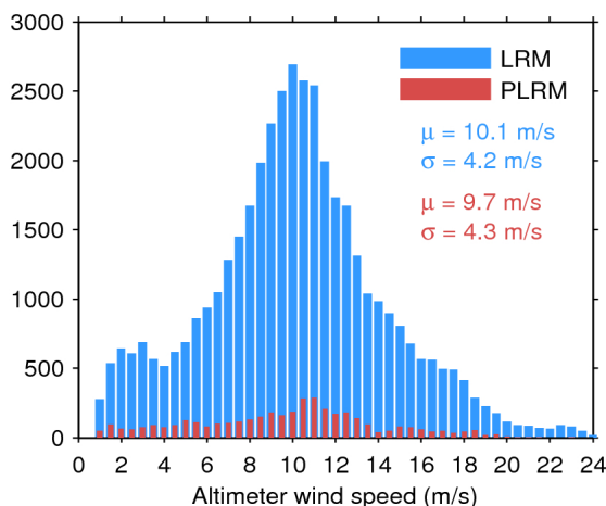
Figure 33. Histogram of flag-valid wind over oceans and lakes for LRM (blue) and PLRM (red) for 04/06/2017. The mean ( \mu ) and standard deviation ( \sigma ) are also shown. Note that values larger than 24 m/s are excluded from the histogram for the sake of readability but not from the computation of \mu and \sigma .
