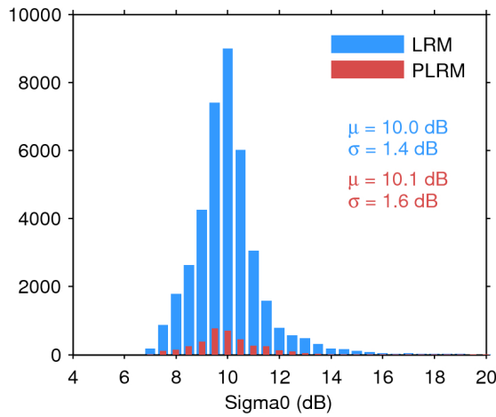
Figure 28. Histogram of science-valid sigma0 over oceans and lakes for LRM (blue) and PLRM (red) for 04/06/2017. The mean ( \mu ) and standard deviation ( \sigma ) are also shown. Note that values outside [4 20] dB are excluded from the histogram for the sake of readability but not from the computation of \mu and \sigma .
