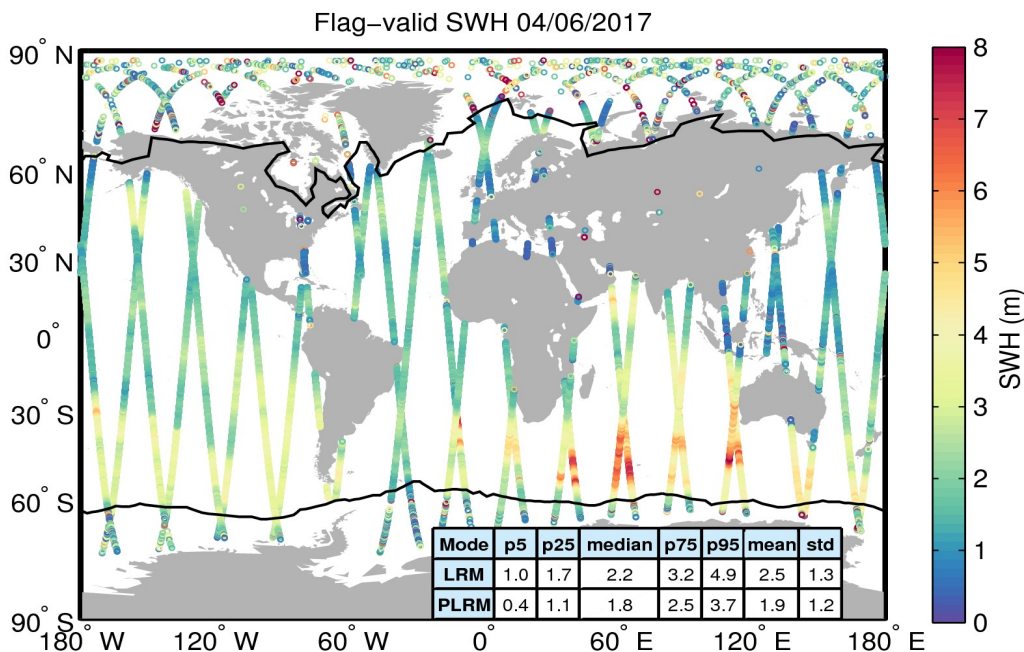
Figure 15. Geographical distribution of flag-valid SWH data over oceans and lakes for 04/06/2017. The statistical values shown in the table refer to the SWH in m and are calculated separately for LRM and PLRM regions. Measurements taken over polar polygons have been excluded from the computation of the statistical values. The black lines mark the outer limit of the Arctic and Antarctic polar polygons.
