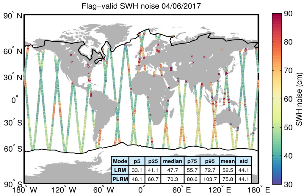
Figure 18. Geographical distribution of flag-valid 20-Hz SWH measurement noise over oceans and lakes for 04/06/2017. The statistical values shown in the table refer to the SWH noise and are calculated separately for LRM and PLRM regions. Measurements taken over polar polygons have been excluded from the computation of the statistical values. The black lines mark the outer limit of the Arctic and Antarctic polar polygons.
