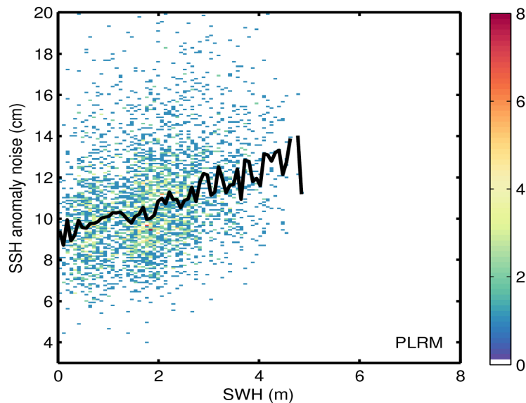
Figure 9. 2D histogram showing flag-valid SSH anomaly noise as a function of SWH for LRM (top) and PLRM (bottom) for 04/06/2017. The black line denotes the median SSH anomaly noise as a function of SWH.
