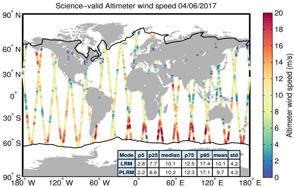
Figure 34. Geographical distribution of science-valid wind data over oceans and lakes for 04/06/2017. The statistical values shown in the table refer to the wind in m/s and are calculated separately for LRM and PLRM regions. The black lines mark the outer limit of the Arctic and Antarctic polar polygons. Gray circles denote records that have been rejected based on the editing criteria described in Table 5.
