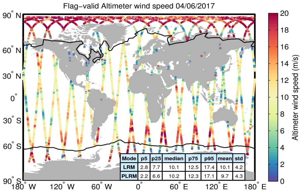
Figure 31. Geographical distribution of flag-valid wind data over oceans and lakes for 04/06/2017. The statistical values shown in the table refer to the wind in m/s and are calculated separately for LRM and PLRM regions. Measurements taken over polar polygons have been excluded from the computation of the statistical values. The black lines mark the outer limit of the Arctic and Antarctic polar polygons.
