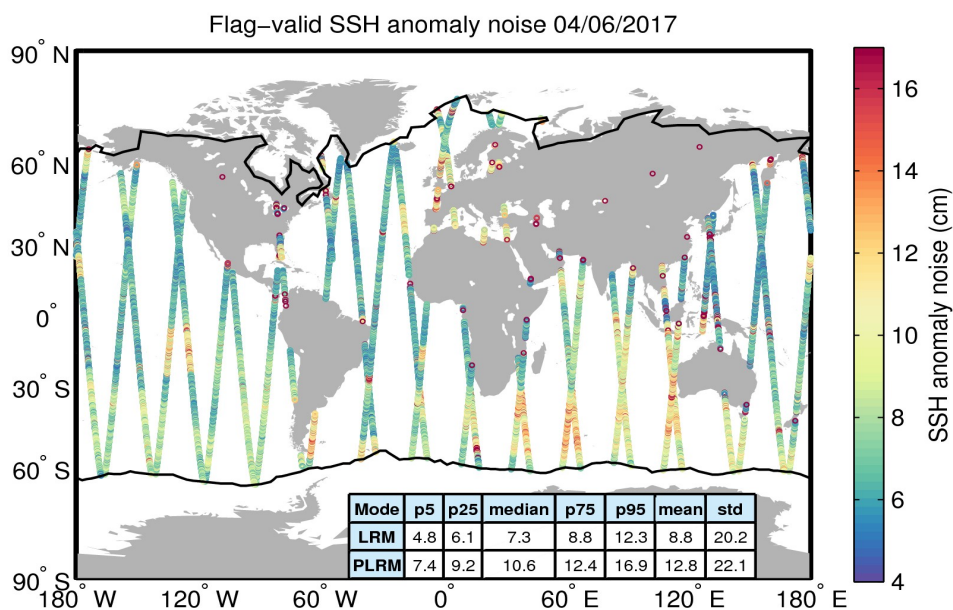
Figure 8. Geographical distribution of flag-valid 20-Hz SSH anomaly measurement noise over oceans and lakes for 04/06/2017. The statistical values shown in the table refer to the SSH anomaly noise and are calculated separately for LRM and PLRM regions. Measurements taken over polar polygons have been excluded from the computation of the statistical values. The black lines mark the outer limit of the Arctic and Antarctic polar polygons.
