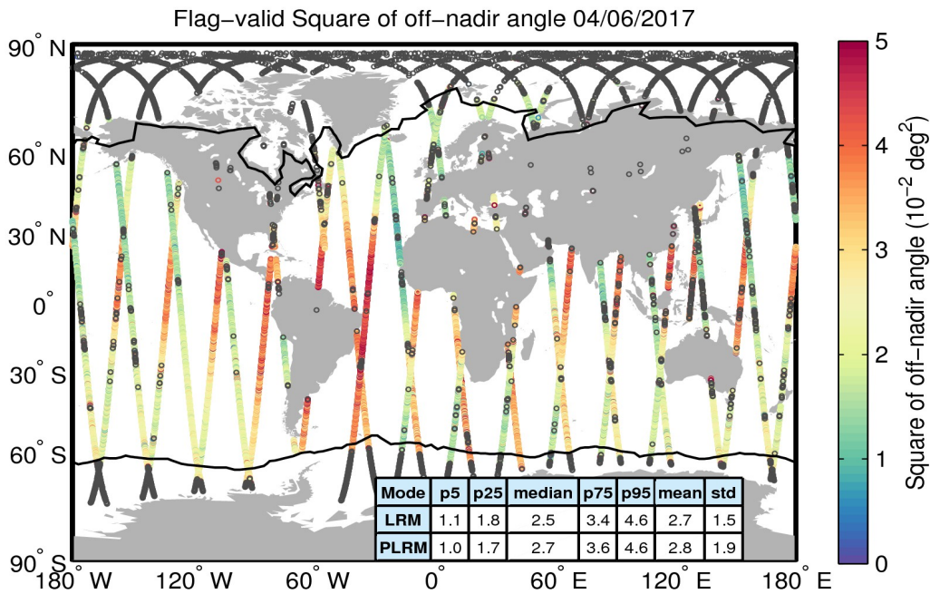
Figure 37. Geographical distribution of flag-valid mispointing data over oceans and lakes for 04/06/2017. The statistical values shown in the table refer to the mispointing in 10^{-2} deg 2 and are calculated separately for LRM and PLRM regions. Measurements taken over polar polygons have been excluded from the computation of the statistical values. The black lines mark the outer limit of the Arctic and Antarctic polar polygons. Gray circles denote negative values.
