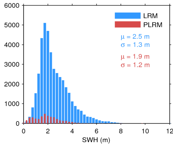
Figure 17. Histogram of flag-valid SWH over oceans and lakes for LRM (blue) and PLRM (red) for 04/06/2017. The mean ( \mu ) and standard deviation ( \sigma ) are also shown. Note that values larger than 12 m are excluded from the histogram for the sake of readability but not from the computation of \mu and \sigma .
