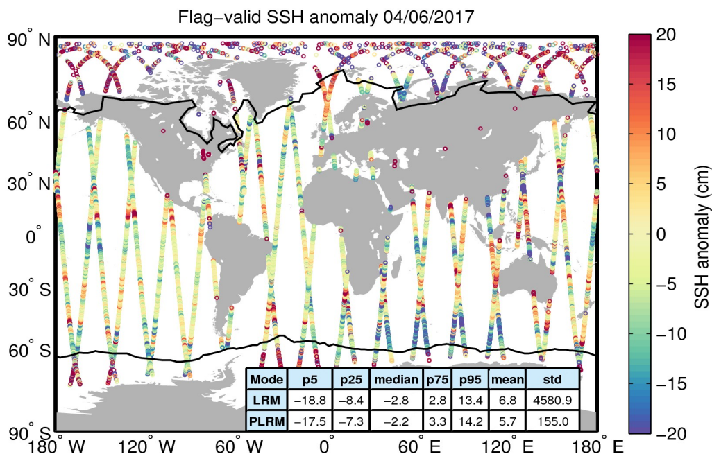
Figure 5. Geographical distribution of flag-valid 1-Hz SSH anomaly data over oceans and lakes for 04/06/2017. The statistical values shown in the table refer to the SSH anomaly in cm and are calculated separately for LRM and PLRM regions. Measurements taken over polar polygons have been excluded from the computation of the statistical values. The black lines mark the outer limit of the Arctic and Antarctic polar polygons.
