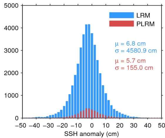
Figure 7. Histogram of flag-valid SSH anomaly over oceans and lakes for LRM (blue) and PLRM (red) for 04/06/2017. The mean ( \mu ) and standard deviation ( \sigma ) are also shown. Note that values outside [-50\ 50] cm are excluded from the histogram for the sake of readability but not from the computation of \mu and \sigma .
