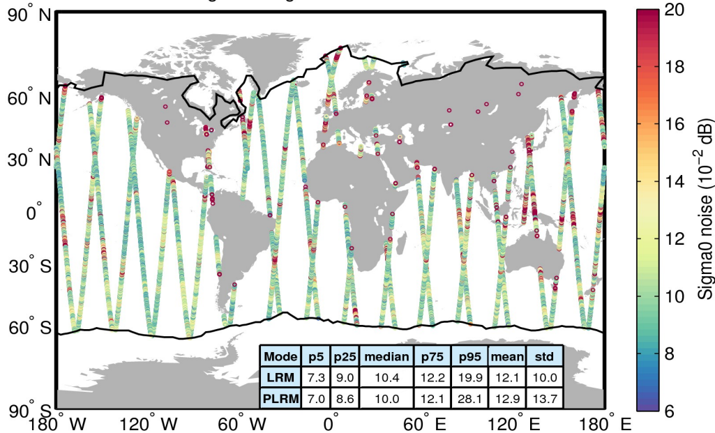
Flag-valid sigma0 noise 04/06/2017
