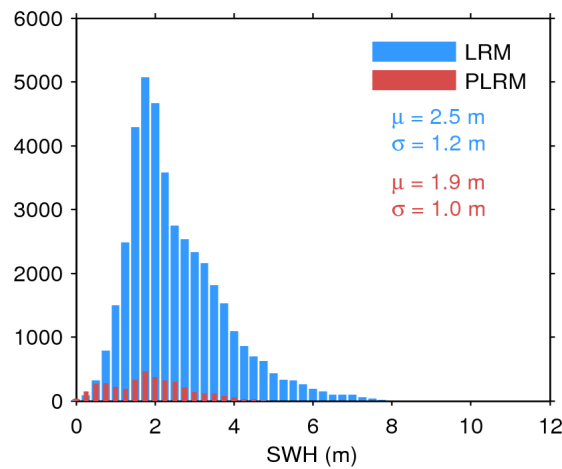
Figure 20. Histogram of science-valid SWH over oceans and lakes for LRM (blue) and PLRM (red) for 04/06/2017. The mean ( \mu ) and standard deviation ( \sigma ) are also shown. Note that values larger than 12 m are excluded from the histogram for the sake of readability but not from the computation of \mu and \sigma .
