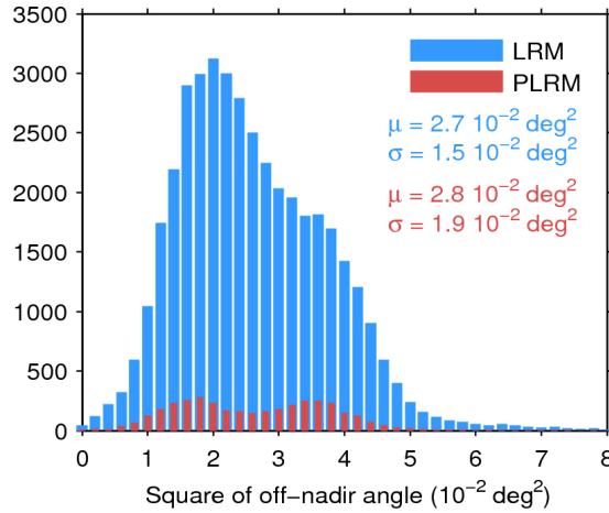
Figure 39. Histogram of flag-valid mispointing over oceans and lakes for LRM (blue) and PLRM (red) for 04/06/2017. Only positive values have been considered. The mean ( \mu ) and standard deviation ( \sigma ) are also shown. Note that values larger than 8 \cdot 10^{-2} \text{ deg}^2 are excluded from the histogram for the sake of readability but not from the computation of \mu and \sigma .
