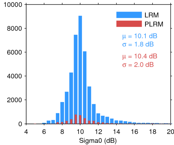
Figure 25. Histogram of flag-valid sigma0 over oceans and lakes for LRM (blue) and PLRM (red) for 04/06/2017. The mean ( \mu ) and standard deviation ( \sigma ) are also shown. Note that values outside [4 20] dB are excluded from the histogram for the sake of readability but not from the computation of \mu and \sigma .
