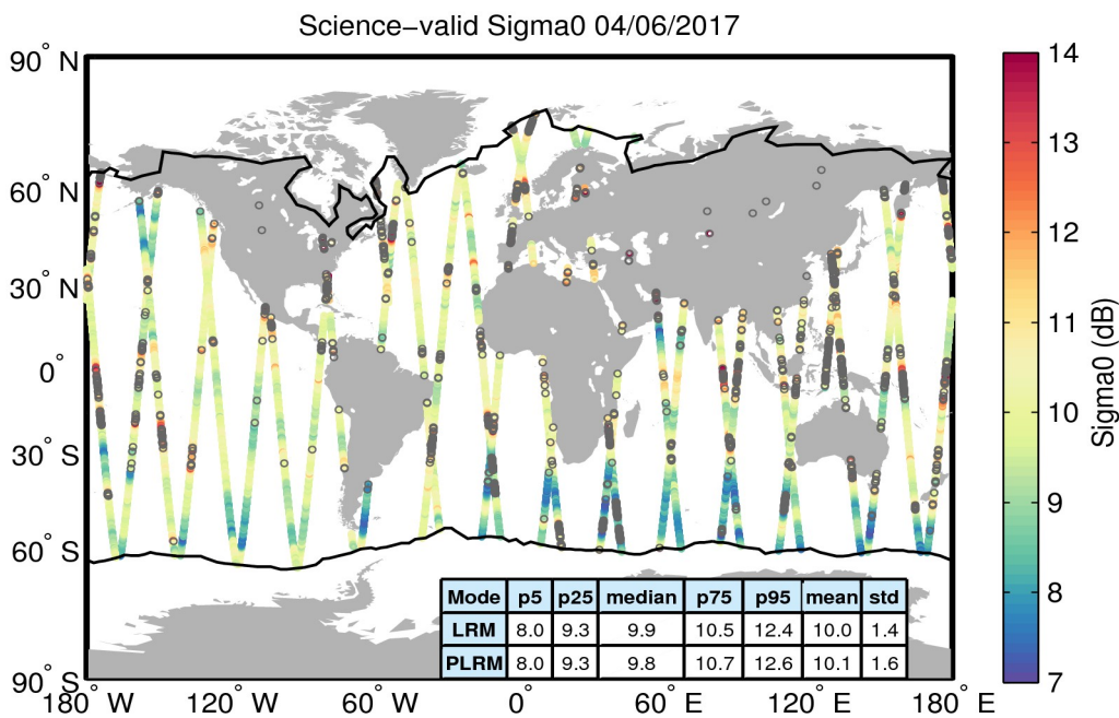
Figure 27. Geographical distribution of science-valid sigma0 data over oceans and lakes for 04/06/2017. The statistical values shown in the table refer to the sigma0 in dB and are calculated separately for LRM and PLRM regions. The black lines mark the outer limit of the Arctic and Antarctic polar polygons. Gray circles denote records that have been rejected based on the editing criteria described in Table 4.
