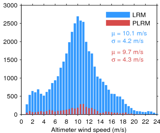
Figure 35. Histogram of science-valid wind over oceans and lakes for LRM (blue) and PLRM (red) for 04/06/2017. The mean ( \mu ) and standard deviation ( \sigma ) are also shown. Note that values larger than 24 m/s are excluded from the histogram for the sake of readability but not from the computation of \mu and \sigma .
