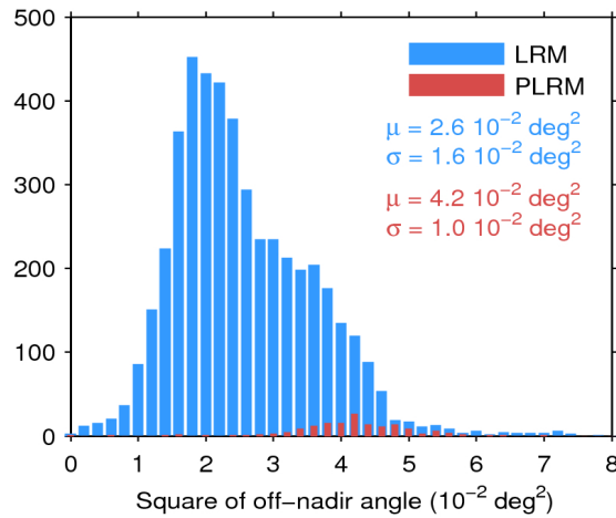
Figure 39. Histogram of flag-valid mispointing over oceans and lakes for LRM (blue) and PLRM (red) for 02/06/2017. Only positive values have been considered. The mean ( \mu ) and standard deviation ( \sigma ) are also shown. Note that values larger than 8 \cdot 10^{-2} \text{ deg}^2 are excluded from the histogram for the sake of readability but not from the computation of \mu and \sigma .
