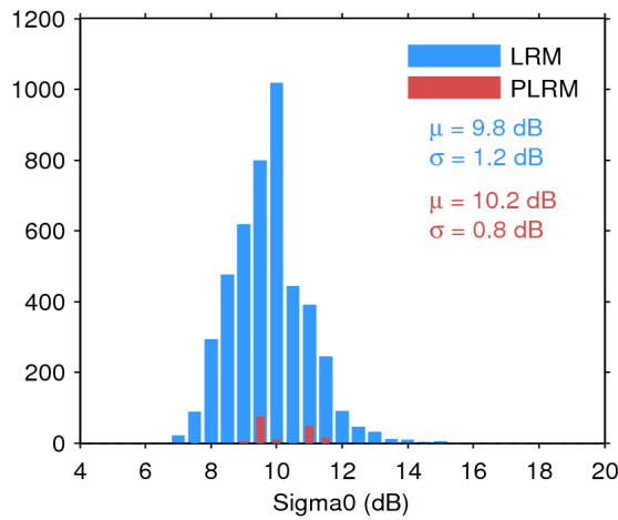
Figure 28. Histogram of science-valid sigma0 over oceans and lakes for LRM (blue) and PLRM (red) for 02/06/2017. The mean ( \mu ) and standard deviation ( \sigma ) are also shown. Note that values outside [4 20] dB are excluded from the histogram for the sake of readability but not from the computation of \mu and \sigma .
