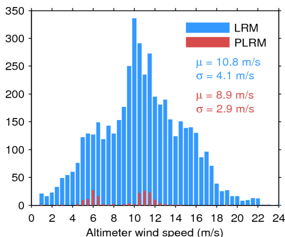
Figure 33. Histogram of flag-valid wind over oceans and lakes for LRM (blue) and PLRM (red) for 02/06/2017. The mean ( \mu ) and standard deviation ( \sigma ) are also shown. Note that values larger than 24 m/s are excluded from the histogram for the sake of readability but not from the computation of \mu and \sigma .
