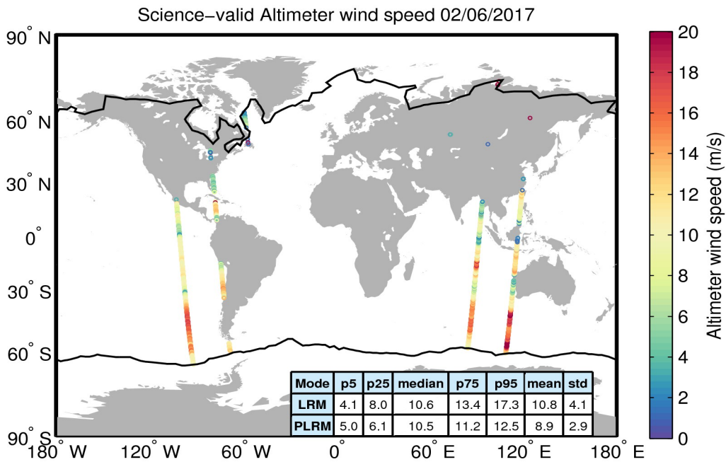
Figure 34. Geographical distribution of science-valid wind data over oceans and lakes for 02/06/2017. The statistical values shown in the table refer to the wind in m/s and are calculated separately for LRM and PLRM regions. The black lines mark the outer limit of the Arctic and Antarctic polar polygons. Gray circles denote records that have been rejected based on the editing criteria described in Table 5.
