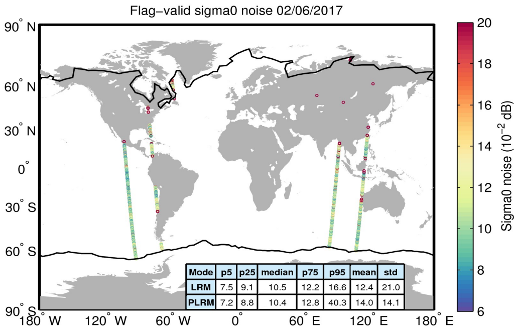
Figure 26. Geographical distribution of flag-valid 20-Hz sigma0 measurement noise over oceans and lakes for 02/06/2017. The statistical values shown in the table refer to the sigma0 noise and are calculated separately for LRM and PLRM regions. Measurements taken over polar polygons have been excluded from the computation of the statistical values. The black lines mark the outer limit of the Arctic and Antarctic polar polygons.
