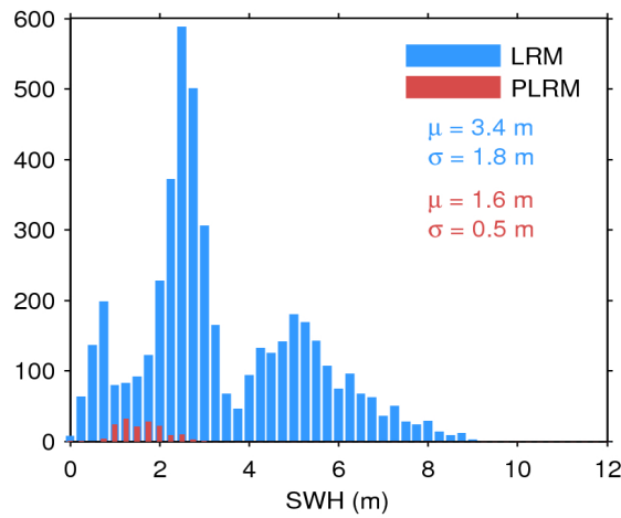
Figure 20. Histogram of science-valid SWH over oceans and lakes for LRM (blue) and PLRM (red) for 02/06/2017. The mean ( \mu ) and standard deviation ( \sigma ) are also shown. Note that values larger than 12 m are excluded from the histogram for the sake of readability but not from the computation of \mu and \sigma .
