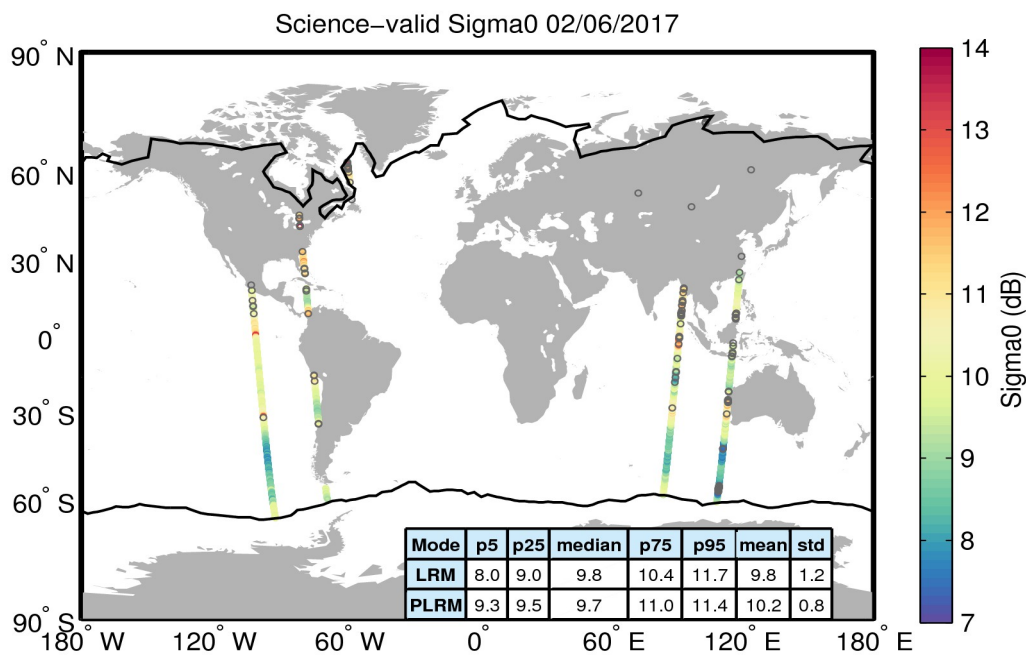
Figure 27. Geographical distribution of science-valid sigma0 data over oceans and lakes for 02/06/2017. The statistical values shown in the table refer to the sigma0 in dB and are calculated separately for LRM and PLRM regions. The black lines mark the outer limit of the Arctic and Antarctic polar polygons. Gray circles denote records that have been rejected based on the editing criteria described in Table 4.
