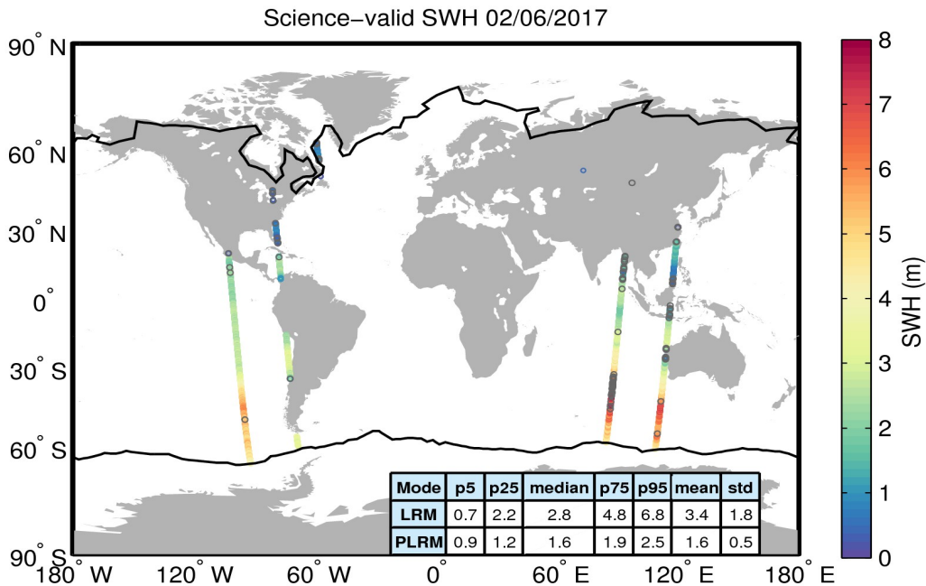
Figure 19. Geographical distribution of science-valid SWH data over oceans and lakes for 02/06/2017. The statistical values shown in the table refer to the SWH in m and are calculated separately for LRM and PLRM regions. The black lines mark the outer limit of the Arctic and Antarctic polar polygons. Gray circles denote records that have been rejected based on the editing criteria described in Table 3.
