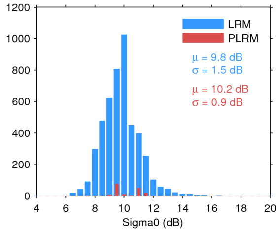
Figure 25. Histogram of flag-valid sigma0 over oceans and lakes for LRM (blue) and PLRM (red) for 02/06/2017. The mean ( \mu ) and standard deviation ( \sigma ) are also shown. Note that values outside [4 20] dB are excluded from the histogram for the sake of readability but not from the computation of \mu and \sigma .
