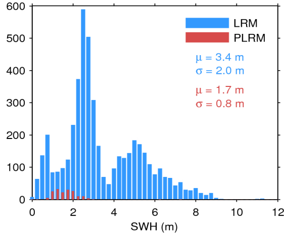
Figure 17. Histogram of flag-valid SWH over oceans and lakes for LRM (blue) and PLRM (red) for 02/06/2017. The mean ( \mu ) and standard deviation ( \sigma ) are also shown. Note that values larger than 12 m are excluded from the histogram for the sake of readability but not from the computation of \mu and \sigma .
