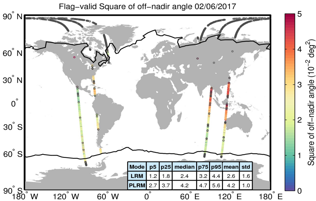
Figure 37. Geographical distribution of flag-valid mispointing data over oceans and lakes for 02/06/2017. The statistical values shown in the table refer to the mispointing in 10^{-2} deg 2 and are calculated separately for LRM and PLRM regions. Measurements taken over polar polygons have been excluded from the computation of the statistical values. The black lines mark the outer limit of the Arctic and Antarctic polar polygons. Gray circles denote negative values.
