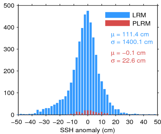
Figure 7. Histogram of flag-valid SSH anomaly over oceans and lakes for LRM (blue) and PLRM (red) for 02/06/2017. The mean ( \mu ) and standard deviation ( \sigma ) are also shown. Note that values outside [-50 \ 50] cm are excluded from the histogram for the sake of readability but not from the computation of \mu and \sigma .
