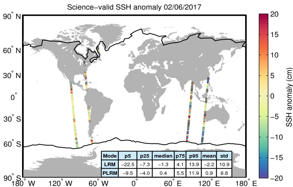
Figure 10. Geographical distribution of science-valid SSH anomaly data over oceans and lakes for 02/06/2017. The statistical values shown in the table refer to the SSH anomaly in cm and are calculated separately for LRM and PLRM regions. The black lines mark the outer limit of the Arctic and Antarctic polar polygons. Gray circles denote records that have been rejected based on the editing criteria described in Table 2.
