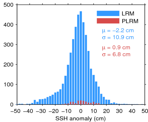
Figure 11. Histogram of science-valid SSH anomaly over oceans and lakes for LRM (blue) and PLRM (red) for 02/06/2017. The mean ( \mu ) and standard deviation ( \sigma ) are also shown. Note that values outside [-50\ 50] cm are excluded from the histogram for the sake of readability but not from the computation of \mu and \sigma .
