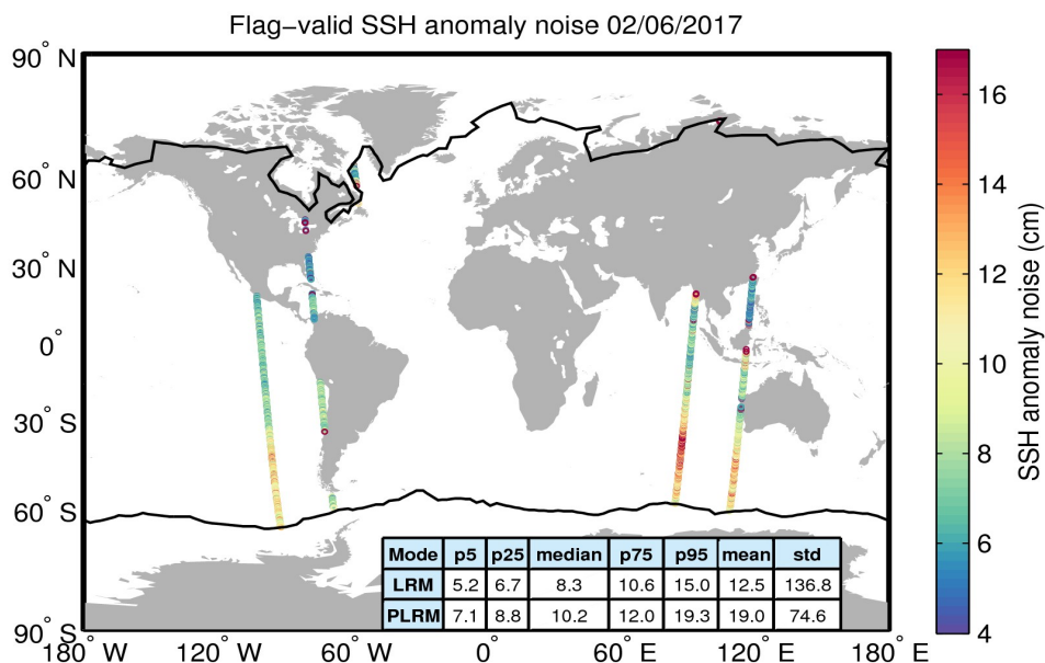
Figure 8. Geographical distribution of flag-valid 20-Hz SSH anomaly measurement noise over oceans and lakes for 02/06/2017. The statistical values shown in the table refer to the SSH anomaly noise and are calculated separately for LRM and PLRM regions. Measurements taken over polar polygons have been excluded from the computation of the statistical values. The black lines mark the outer limit of the Arctic and Antarctic polar polygons.
