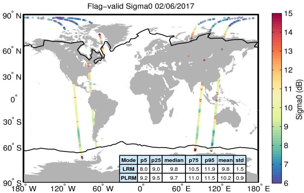
Figure 23. Geographical distribution of flag-valid sigma0 data over oceans and lakes for 02/06/2017. The statistical values shown in the table refer to the sigma0 in dB and are calculated separately for LRM and PLRM regions. Measurements taken over polar polygons have been excluded from the computation of the statistical values. The black lines mark the outer limit of the Arctic and Antarctic polar polygons.
