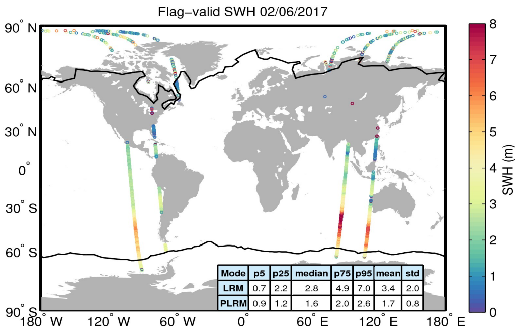
Figure 15. Geographical distribution of flag-valid SWH data over oceans and lakes for 02/06/2017. The statistical values shown in the table refer to the SWH in m and are calculated separately for LRM and PLRM regions. Measurements taken over polar polygons have been excluded from the computation of the statistical values. The black lines mark the outer limit of the Arctic and Antarctic polar polygons.
