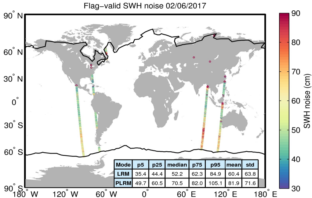
Figure 18. Geographical distribution of flag-valid 20-Hz SWH measurement noise over oceans and lakes for 02/06/2017. The statistical values shown in the table refer to the SWH noise and are calculated separately for LRM and PLRM regions. Measurements taken over polar polygons have been excluded from the computation of the statistical values. The black lines mark the outer limit of the Arctic and Antarctic polar polygons.
