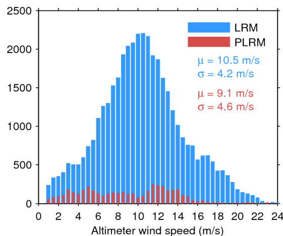
Figure 35. Histogram of science-valid wind over oceans and lakes for LRM (blue) and PLRM (red) for 01/06/2017. The mean ( \mu ) and standard deviation ( \sigma ) are also shown. Note that values larger than 24 m/s are excluded from the histogram for the sake of readability but not from the computation of \mu and \sigma .
