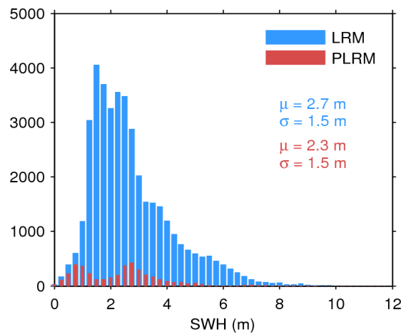
Figure 20. Histogram of science-valid SWH over oceans and lakes for LRM (blue) and PLRM (red) for 01/06/2017. The mean ( \mu ) and standard deviation ( \sigma ) are also shown. Note that values larger than 12 m are excluded from the histogram for the sake of readability but not from the computation of \mu and \sigma .
