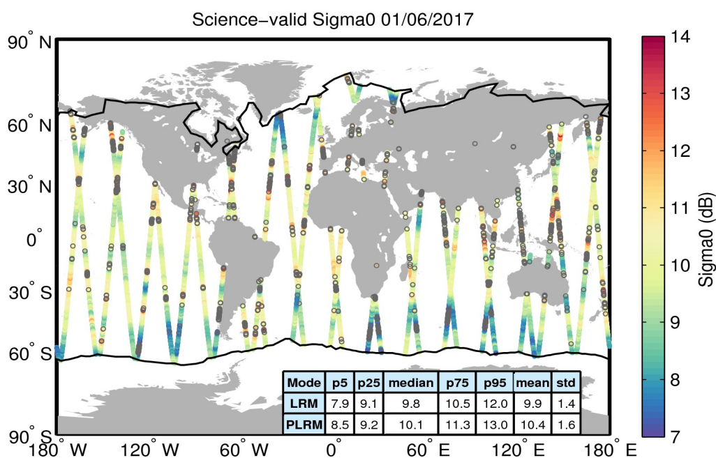
Figure 27. Geographical distribution of science-valid sigma0 data over oceans and lakes for 01/06/2017. The statistical values shown in the table refer to the sigma0 in dB and are calculated separately for LRM and PLRM regions. The black lines mark the outer limit of the Arctic and Antarctic polar polygons. Gray circles denote records that have been rejected based on the editing criteria described in Table 4.
