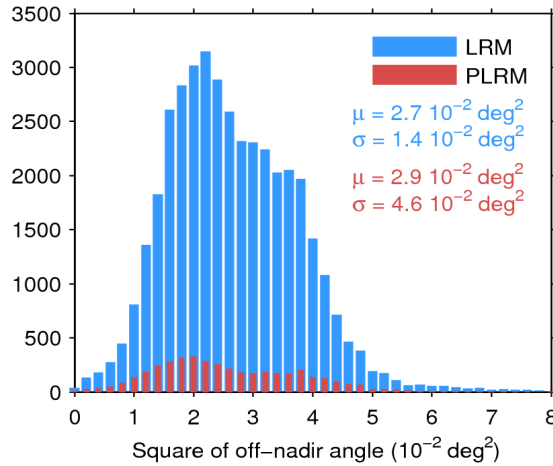
Figure 39. Histogram of flag-valid mispointing over oceans and lakes for LRM (blue) and PLRM (red) for 01/06/2017. Only positive values have been considered. The mean ( \mu ) and standard deviation ( \sigma ) are also shown. Note that values larger than 8 \cdot 10^{-2} \text{ deg}^2 are excluded from the histogram for the sake of readability but not from the computation of \mu and \sigma .
