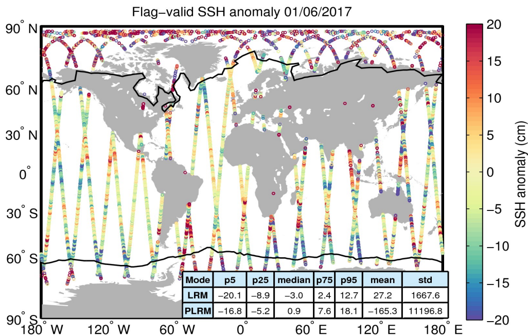
Figure 5. Geographical distribution of flag-valid 1-Hz SSH anomaly data over oceans and lakes for 01/06/2017. The statistical values shown in the table refer to the SSH anomaly in cm and are calculated separately for LRM and PLRM regions. Measurements taken over polar polygons have been excluded from the computation of the statistical values. The black lines mark the outer limit of the Arctic and Antarctic polar polygons.
