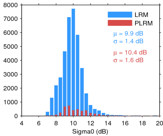
Figure 28. Histogram of science-valid sigma0 over oceans and lakes for LRM (blue) and PLRM (red) for 01/06/2017. The mean ( \mu ) and standard deviation ( \sigma ) are also shown. Note that values outside [4 20] dB are excluded from the histogram for the sake of readability but not from the computation of \mu and \sigma .
