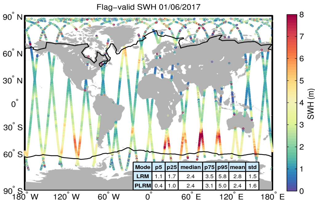
Figure 15. Geographical distribution of flag-valid SWH data over oceans and lakes for 01/06/2017. The statistical values shown in the table refer to the SWH in m and are calculated separately for LRM and PLRM regions. Measurements taken over polar polygons have been excluded from the computation of the statistical values. The black lines mark the outer limit of the Arctic and Antarctic polar polygons.
