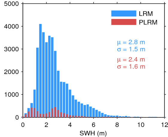
Figure 17. Histogram of flag-valid SWH over oceans and lakes for LRM (blue) and PLRM (red) for 01/06/2017. The mean ( \mu ) and standard deviation ( \sigma ) are also shown. Note that values larger than 12 m are excluded from the histogram for the sake of readability but not from the computation of \mu and \sigma .
