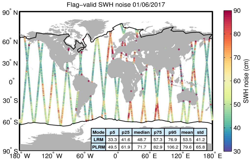
Figure 18. Geographical distribution of flag-valid 20-Hz SWH measurement noise over oceans and lakes for 01/06/2017. The statistical values shown in the table refer to the SWH noise and are calculated separately for LRM and PLRM regions. Measurements taken over polar polygons have been excluded from the computation of the statistical values. The black lines mark the outer limit of the Arctic and Antarctic polar polygons.
