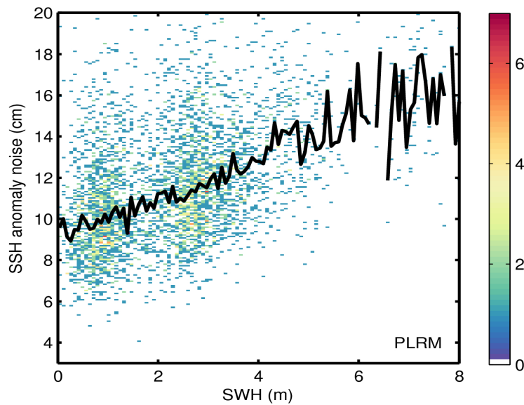
Figure 9. 2D histogram showing flag-valid SSH anomaly noise as a function of SWH for LRM (top) and PLRM (bottom) for 01/06/2017. The black line denotes the median SSH anomaly noise as a function of SWH.
