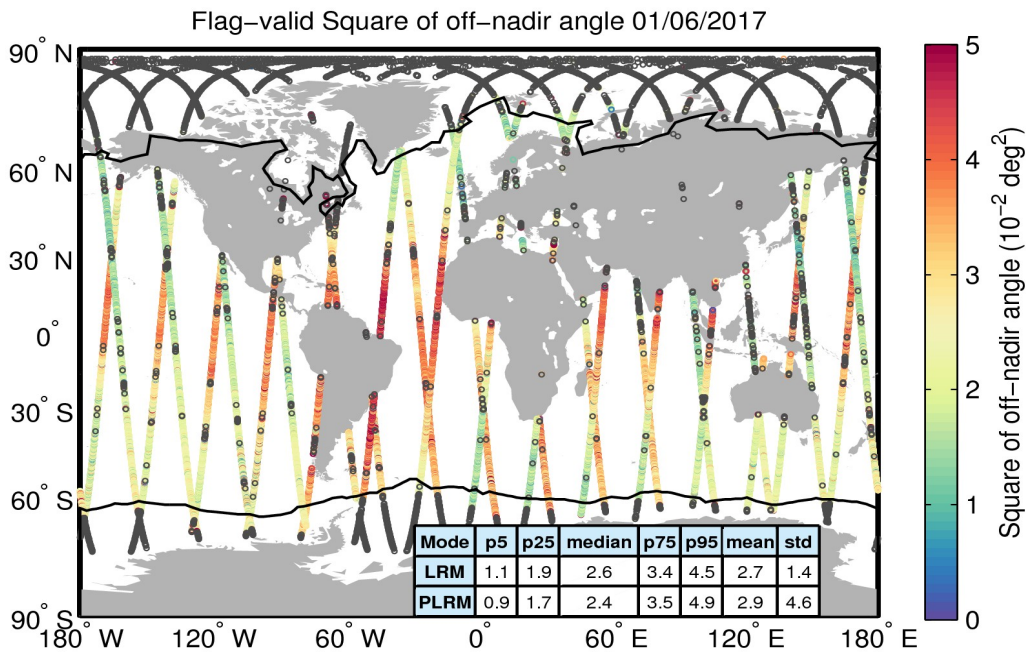
Figure 37. Geographical distribution of flag-valid mispointing data over oceans and lakes for 01/06/2017. The statistical values shown in the table refer to the mispointing in 10^{-2} deg 2 and are calculated separately for LRM and PLRM regions. Measurements taken over polar polygons have been excluded from the computation of the statistical values. The black lines mark the outer limit of the Arctic and Antarctic polar polygons. Gray circles denote negative values.
