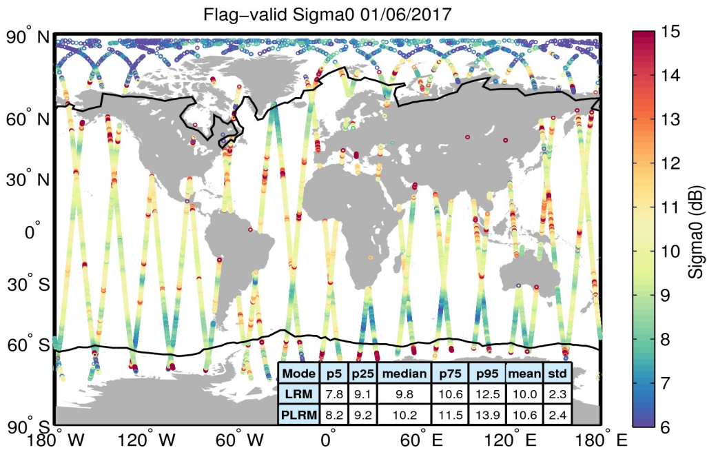
Figure 23. Geographical distribution of flag-valid sigma0 data over oceans and lakes for 01/06/2017. The statistical values shown in the table refer to the sigma0 in dB and are calculated separately for LRM and PLRM regions. Measurements taken over polar polygons have been excluded from the computation of the statistical values. The black lines mark the outer limit of the Arctic and Antarctic polar polygons.
