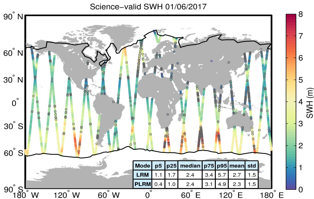
Figure 19. Geographical distribution of science-valid SWH data over oceans and lakes for 01/06/2017. The statistical values shown in the table refer to the SWH in m and are calculated separately for LRM and PLRM regions. The black lines mark the outer limit of the Arctic and Antarctic polar polygons. Gray circles denote records that have been rejected based on the editing criteria described in Table 3.
