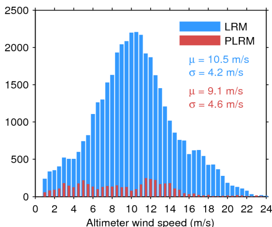
Figure 33. Histogram of flag-valid wind over oceans and lakes for LRM (blue) and PLRM (red) for 01/06/2017. The mean ( \mu ) and standard deviation ( \sigma ) are also shown. Note that values larger than 24 m/s are excluded from the histogram for the sake of readability but not from the computation of \mu and \sigma .
