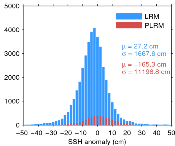
Figure 7. Histogram of flag-valid SSH anomaly over oceans and lakes for LRM (blue) and PLRM (red) for 01/06/2017. The mean ( \mu ) and standard deviation ( \sigma ) are also shown. Note that values outside [-50 50] cm are excluded from the histogram for the sake of readability but not from the computation of \mu and \sigma .
