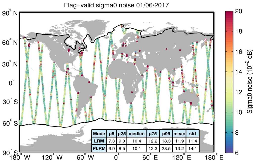
Figure 26. Geographical distribution of flag-valid 20-Hz sigma0 measurement noise over oceans and lakes for 01/06/2017. The statistical values shown in the table refer to the sigma0 noise and are calculated separately for LRM and PLRM regions. Measurements taken over polar polygons have been excluded from the computation of the statistical values. The black lines mark the outer limit of the Arctic and Antarctic polar polygons.
