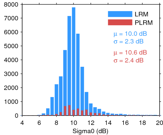
Figure 25. Histogram of flag-valid sigma0 over oceans and lakes for LRM (blue) and PLRM (red) for 01/06/2017. The mean ( \mu ) and standard deviation ( \sigma ) are also shown. Note that values outside [4 20] dB are excluded from the histogram for the sake of readability but not from the computation of \mu and \sigma .
