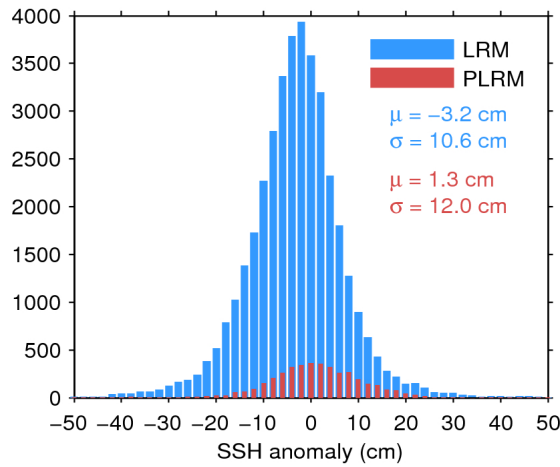
Figure 11. Histogram of science-valid SSH anomaly over oceans and lakes for LRM (blue) and PLRM (red) for 01/06/2017. The mean ( \mu ) and standard deviation ( \sigma ) are also shown. Note that values outside [-50\ 50] cm are excluded from the histogram for the sake of readability but not from the computation of \mu and \sigma .
