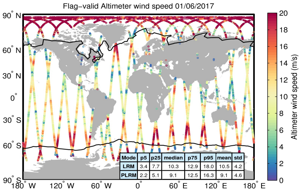
Figure 31. Geographical distribution of flag-valid wind data over oceans and lakes for 01/06/2017. The statistical values shown in the table refer to the wind in m/s and are calculated separately for LRM and PLRM regions. Measurements taken over polar polygons have been excluded from the computation of the statistical values. The black lines mark the outer limit of the Arctic and Antarctic polar polygons.
