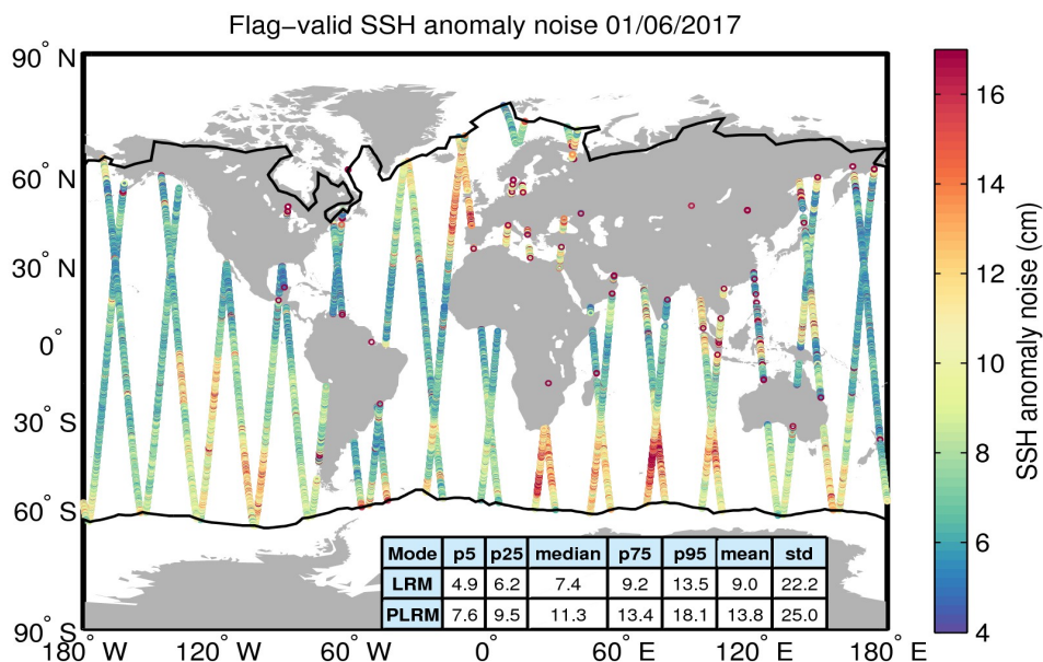
Figure 8. Geographical distribution of flag-valid 20-Hz SSH anomaly measurement noise over oceans and lakes for 01/06/2017. The statistical values shown in the table refer to the SSH anomaly noise and are calculated separately for LRM and PLRM regions. Measurements taken over polar polygons have been excluded from the computation of the statistical values. The black lines mark the outer limit of the Arctic and Antarctic polar polygons.
