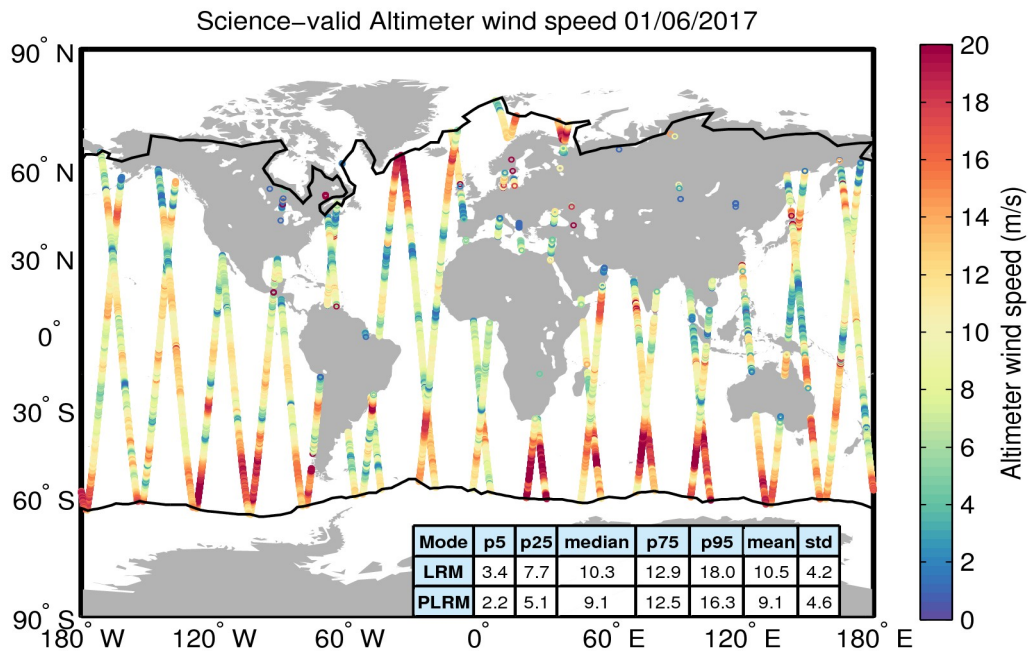
Figure 34. Geographical distribution of science-valid wind data over oceans and lakes for 01/06/2017. The statistical values shown in the table refer to the wind in m/s and are calculated separately for LRM and PLRM regions. The black lines mark the outer limit of the Arctic and Antarctic polar polygons. Gray circles denote records that have been rejected based on the editing criteria described in Table 5.
