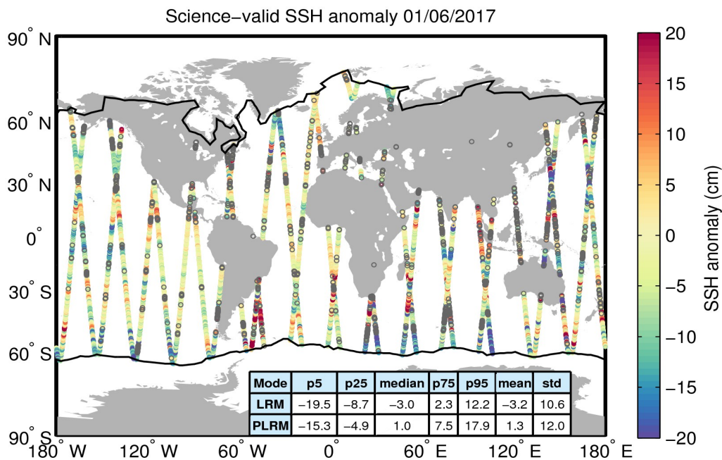
Figure 10. Geographical distribution of science-valid SSH anomaly data over oceans and lakes for 01/06/2017. The statistical values shown in the table refer to the SSH anomaly in cm and are calculated separately for LRM and PLRM regions. The black lines mark the outer limit of the Arctic and Antarctic polar polygons. Gray circles denote records that have been rejected based on the editing criteria described in Table 2.
