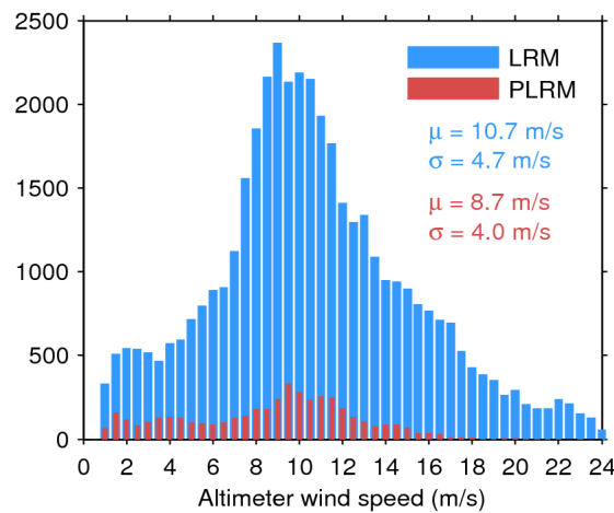
Figure 33. Histogram of flag-valid wind over oceans and lakes for LRM (blue) and PLRM (red) for 28/05/2017. The mean ( \mu ) and standard deviation ( \sigma ) are also shown. Note that values larger than 24 m/s are excluded from the histogram for the sake of readability but not from the computation of \mu and \sigma .
