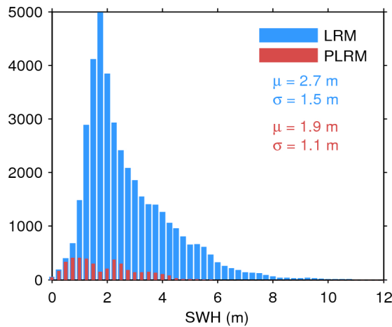
Figure 20. Histogram of science-valid SWH over oceans and lakes for LRM (blue) and PLRM (red) for 28/05/2017. The mean ( \mu ) and standard deviation ( \sigma ) are also shown. Note that values larger than 12 m are excluded from the histogram for the sake of readability but not from the computation of \mu and \sigma .
