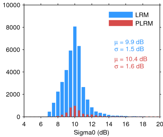
Figure 28. Histogram of science-valid sigma0 over oceans and lakes for LRM (blue) and PLRM (red) for 28/05/2017. The mean ( \mu ) and standard deviation ( \sigma ) are also shown. Note that values outside [4 20] dB are excluded from the histogram for the sake of readability but not from the computation of \mu and \sigma .
