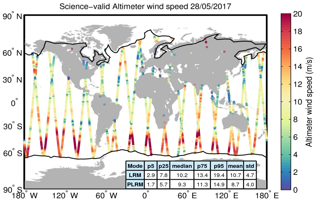
Figure 34. Geographical distribution of science-valid wind data over oceans and lakes for 28/05/2017. The statistical values shown in the table refer to the wind in m/s and are calculated separately for LRM and PLRM regions. The black lines mark the outer limit of the Arctic and Antarctic polar polygons. Gray circles denote records that have been rejected based on the editing criteria described in Table 5.
