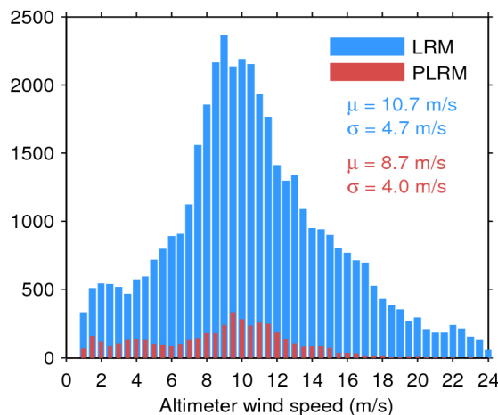
Figure 35. Histogram of science-valid wind over oceans and lakes for LRM (blue) and PLRM (red) for 28/05/2017. The mean ( \mu ) and standard deviation ( \sigma ) are also shown. Note that values larger than 24 m/s are excluded from the histogram for the sake of readability but not from the computation of \mu and \sigma .
