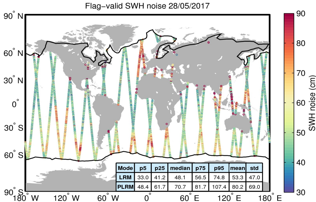
Figure 18. Geographical distribution of flag-valid 20-Hz SWH measurement noise over oceans and lakes for 28/05/2017. The statistical values shown in the table refer to the SWH noise and are calculated separately for LRM and PLRM regions. Measurements taken over polar polygons have been excluded from the computation of the statistical values. The black lines mark the outer limit of the Arctic and Antarctic polar polygons.
