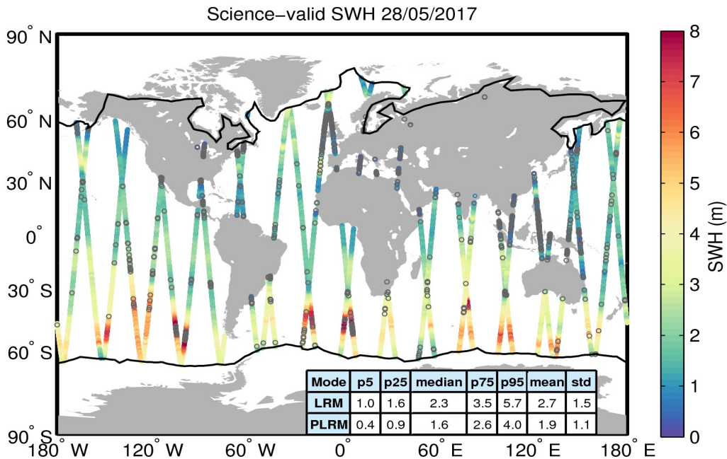
Figure 19. Geographical distribution of science-valid SWH data over oceans and lakes for 28/05/2017. The statistical values shown in the table refer to the SWH in m and are calculated separately for LRM and PLRM regions. The black lines mark the outer limit of the Arctic and Antarctic polar polygons. Gray circles denote records that have been rejected based on the editing criteria described in Table 3.
