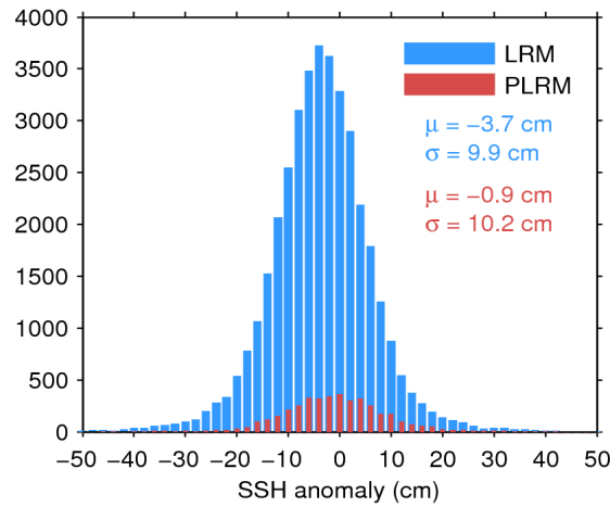
Figure 11. Histogram of science-valid SSH anomaly over oceans and lakes for LRM (blue) and PLRM (red) for 28/05/2017. The mean ( \mu ) and standard deviation ( \sigma ) are also shown. Note that values outside [-50 50] cm are excluded from the histogram for the sake of readability but not from the computation of \mu and \sigma .
