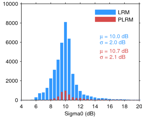
Figure 25. Histogram of flag-valid sigma0 over oceans and lakes for LRM (blue) and PLRM (red) for 28/05/2017. The mean ( \mu ) and standard deviation ( \sigma ) are also shown. Note that values outside [4 20] dB are excluded from the histogram for the sake of readability but not from the computation of \mu and \sigma .
