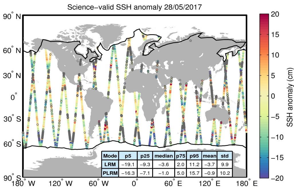
Figure 10. Geographical distribution of science-valid SSH anomaly data over oceans and lakes for 28/05/2017. The statistical values shown in the table refer to the SSH anomaly in cm and are calculated separately for LRM and PLRM regions. The black lines mark the outer limit of the Arctic and Antarctic polar polygons. Gray circles denote records that have been rejected based on the editing criteria described in Table 2.
