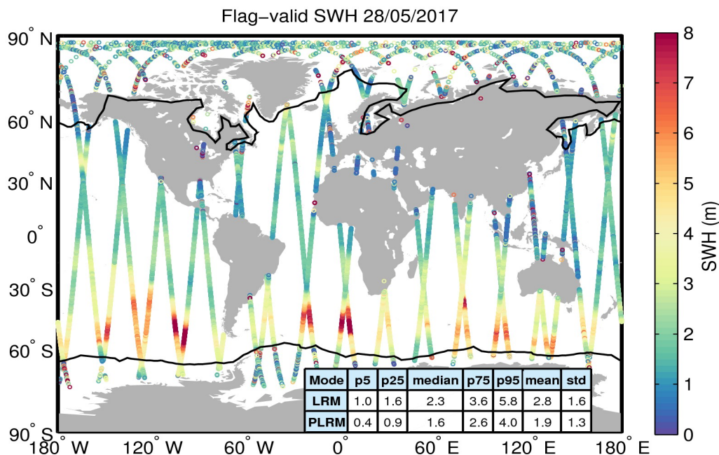
Figure 15. Geographical distribution of flag-valid SWH data over oceans and lakes for 28/05/2017. The statistical values shown in the table refer to the SWH in m and are calculated separately for LRM and PLRM regions. Measurements taken over polar polygons have been excluded from the computation of the statistical values. The black lines mark the outer limit of the Arctic and Antarctic polar polygons.
