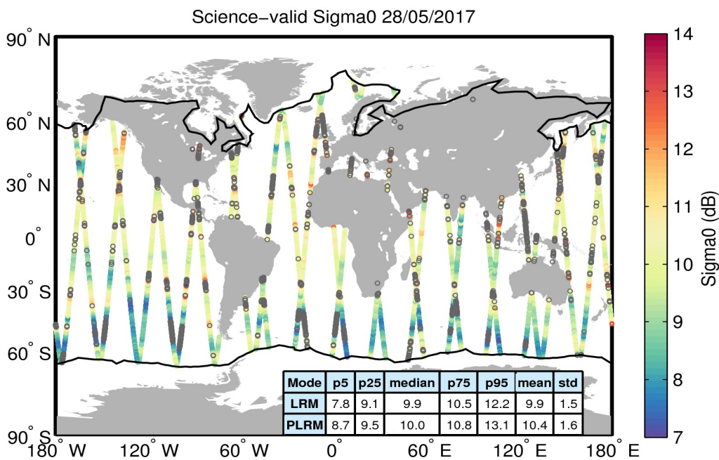
Figure 27. Geographical distribution of science-valid sigma0 data over oceans and lakes for 28/05/2017. The statistical values shown in the table refer to the sigma0 in dB and are calculated separately for LRM and PLRM regions. The black lines mark the outer limit of the Arctic and Antarctic polar polygons. Gray circles denote records that have been rejected based on the editing criteria described in Table 4.
