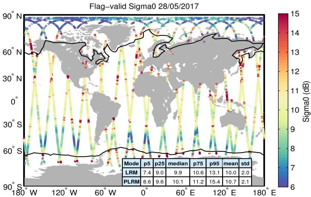
Figure 23. Geographical distribution of flag-valid sigma0 data over oceans and lakes for 28/05/2017. The statistical values shown in the table refer to the sigma0 in dB and are calculated separately for LRM and PLRM regions. Measurements taken over polar polygons have been excluded from the computation of the statistical values. The black lines mark the outer limit of the Arctic and Antarctic polar polygons.
