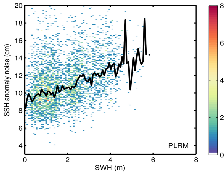
Figure 9. 2D histogram showing flag-valid SSH anomaly noise as a function of SWH for LRM (top) and PLRM (bottom) for 28/05/2017. The black line denotes the median SSH anomaly noise as a function of SWH.
