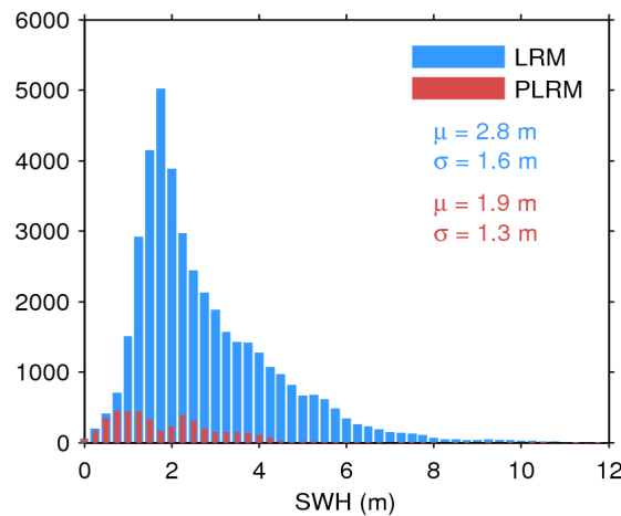
Figure 17. Histogram of flag-valid SWH over oceans and lakes for LRM (blue) and PLRM (red) for 28/05/2017. The mean ( \mu ) and standard deviation ( \sigma ) are also shown. Note that values larger than 12 m are excluded from the histogram for the sake of readability but not from the computation of \mu and \sigma .
