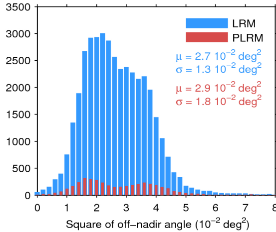
Figure 39. Histogram of flag-valid mispointing over oceans and lakes for LRM (blue) and PLRM (red) for 28/05/2017. Only positive values have been considered. The mean ( \mu ) and standard deviation ( \sigma ) are also shown. Note that values larger than 8 \cdot 10^{-2} \text{ deg}^2 are excluded from the histogram for the sake of readability but not from the computation of \mu and \sigma .
