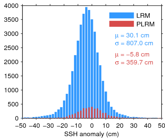
Figure 7. Histogram of flag-valid SSH anomaly over oceans and lakes for LRM (blue) and PLRM (red) for 28/05/2017. The mean ( \mu ) and standard deviation ( \sigma ) are also shown. Note that values outside [-50 50] cm are excluded from the histogram for the sake of readability but not from the computation of \mu and \sigma .
