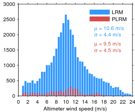
Figure 33. Histogram of flag-valid wind over oceans and lakes for LRM (blue) and PLRM (red) for 26/05/2017. The mean ( \mu ) and standard deviation ( \sigma ) are also shown. Note that values larger than 24 m/s are excluded from the histogram for the sake of readability but not from the computation of \mu and \sigma .
