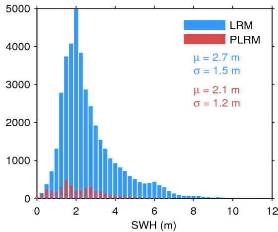
Figure 20. Histogram of science-valid SWH over oceans and lakes for LRM (blue) and PLRM (red) for 26/05/2017. The mean ( \mu ) and standard deviation ( \sigma ) are also shown. Note that values larger than 12 m are excluded from the histogram for the sake of readability but not from the computation of \mu and \sigma .
