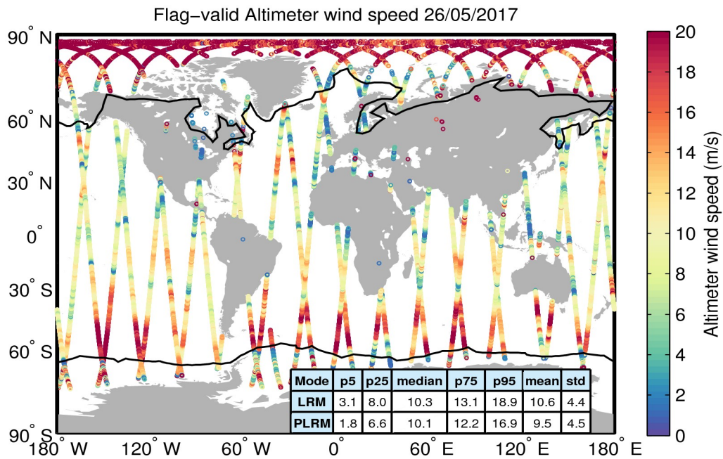
Figure 31. Geographical distribution of flag-valid wind data over oceans and lakes for 26/05/2017. The statistical values shown in the table refer to the wind in m/s and are calculated separately for LRM and PLRM regions. Measurements taken over polar polygons have been excluded from the computation of the statistical values. The black lines mark the outer limit of the Arctic and Antarctic polar polygons.
