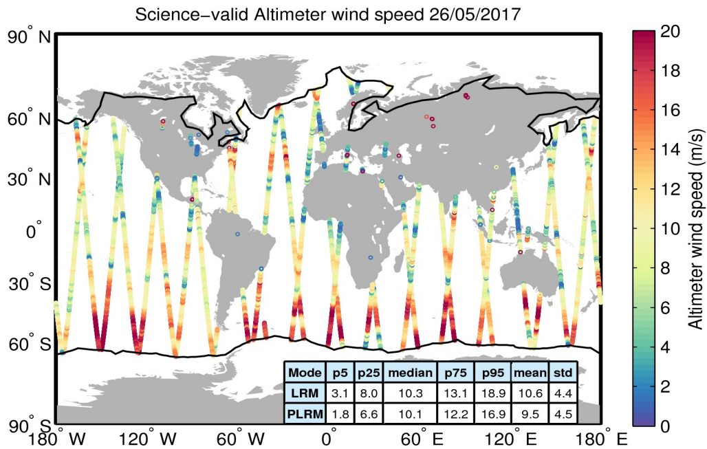
Figure 34. Geographical distribution of science-valid wind data over oceans and lakes for 26/05/2017. The statistical values shown in the table refer to the wind in m/s and are calculated separately for LRM and PLRM regions. The black lines mark the outer limit of the Arctic and Antarctic polar polygons. Gray circles denote records that have been rejected based on the editing criteria described in Table 5.
