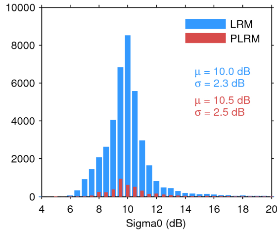
Figure 25. Histogram of flag-valid sigma0 over oceans and lakes for LRM (blue) and PLRM (red) for 26/05/2017. The mean ( \mu ) and standard deviation ( \sigma ) are also shown. Note that values outside [4 20] dB are excluded from the histogram for the sake of readability but not from the computation of \mu and \sigma .
