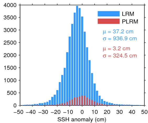
Figure 7. Histogram of flag-valid SSH anomaly over oceans and lakes for LRM (blue) and PLRM (red) for 26/05/2017. The mean ( \mu ) and standard deviation ( \sigma ) are also shown. Note that values outside [-50 \ 50] cm are excluded from the histogram for the sake of readability but not from the computation of \mu and \sigma .
