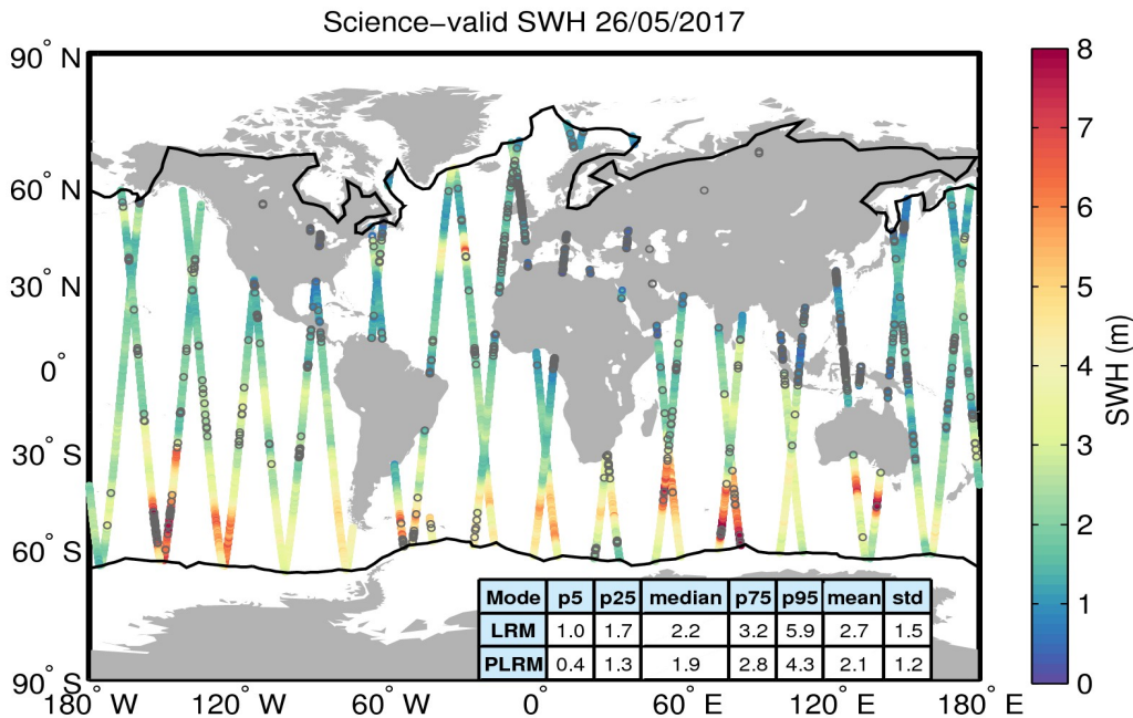
Figure 19. Geographical distribution of science-valid SWH data over oceans and lakes for 26/05/2017. The statistical values shown in the table refer to the SWH in m and are calculated separately for LRM and PLRM regions. The black lines mark the outer limit of the Arctic and Antarctic polar polygons. Gray circles denote records that have been rejected based on the editing criteria described in Table 3.
