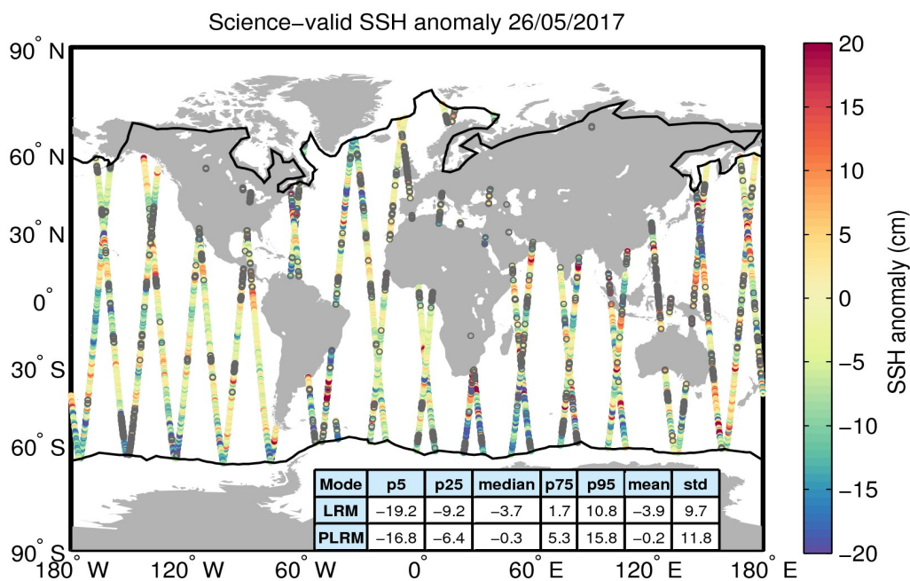
Figure 10. Geographical distribution of science-valid SSH anomaly data over oceans and lakes for 26/05/2017. The statistical values shown in the table refer to the SSH anomaly in cm and are calculated separately for LRM and PLRM regions. The black lines mark the outer limit of the Arctic and Antarctic polar polygons. Gray circles denote records that have been rejected based on the editing criteria described in Table 2.
