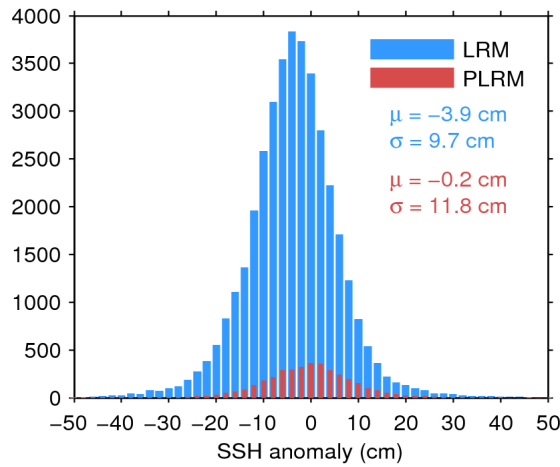
Figure 11. Histogram of science-valid SSH anomaly over oceans and lakes for LRM (blue) and PLRM (red) for 26/05/2017. The mean ( \mu ) and standard deviation ( \sigma ) are also shown. Note that values outside [-50 50] cm are excluded from the histogram for the sake of readability but not from the computation of \mu and \sigma .
