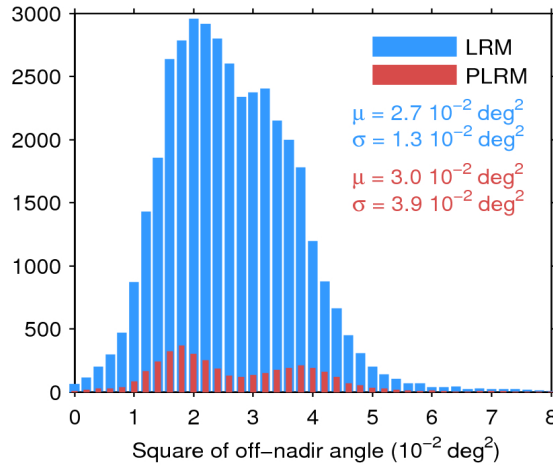
Figure 39. Histogram of flag-valid mispointing over oceans and lakes for LRM (blue) and PLRM (red) for 26/05/2017. Only positive values have been considered. The mean ( \mu ) and standard deviation ( \sigma ) are also shown. Note that values larger than 8 \cdot 10^{-2} \text{ deg}^2 are excluded from the histogram for the sake of readability but not from the computation of \mu and \sigma .
