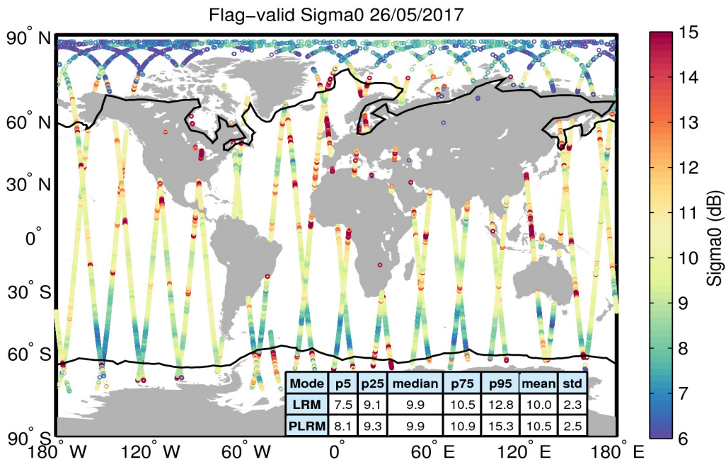
Figure 23. Geographical distribution of flag-valid sigma0 data over oceans and lakes for 26/05/2017. The statistical values shown in the table refer to the sigma0 in dB and are calculated separately for LRM and PLRM regions. Measurements taken over polar polygons have been excluded from the computation of the statistical values. The black lines mark the outer limit of the Arctic and Antarctic polar polygons.
