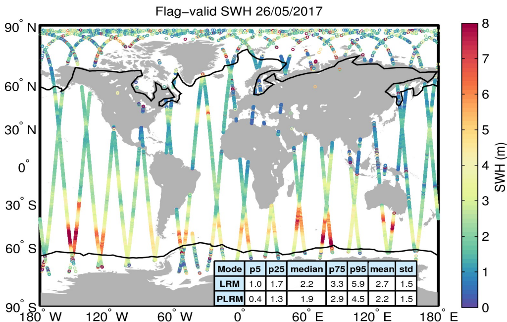
Figure 15. Geographical distribution of flag-valid SWH data over oceans and lakes for 26/05/2017. The statistical values shown in the table refer to the SWH in m and are calculated separately for LRM and PLRM regions. Measurements taken over polar polygons have been excluded from the computation of the statistical values. The black lines mark the outer limit of the Arctic and Antarctic polar polygons.
