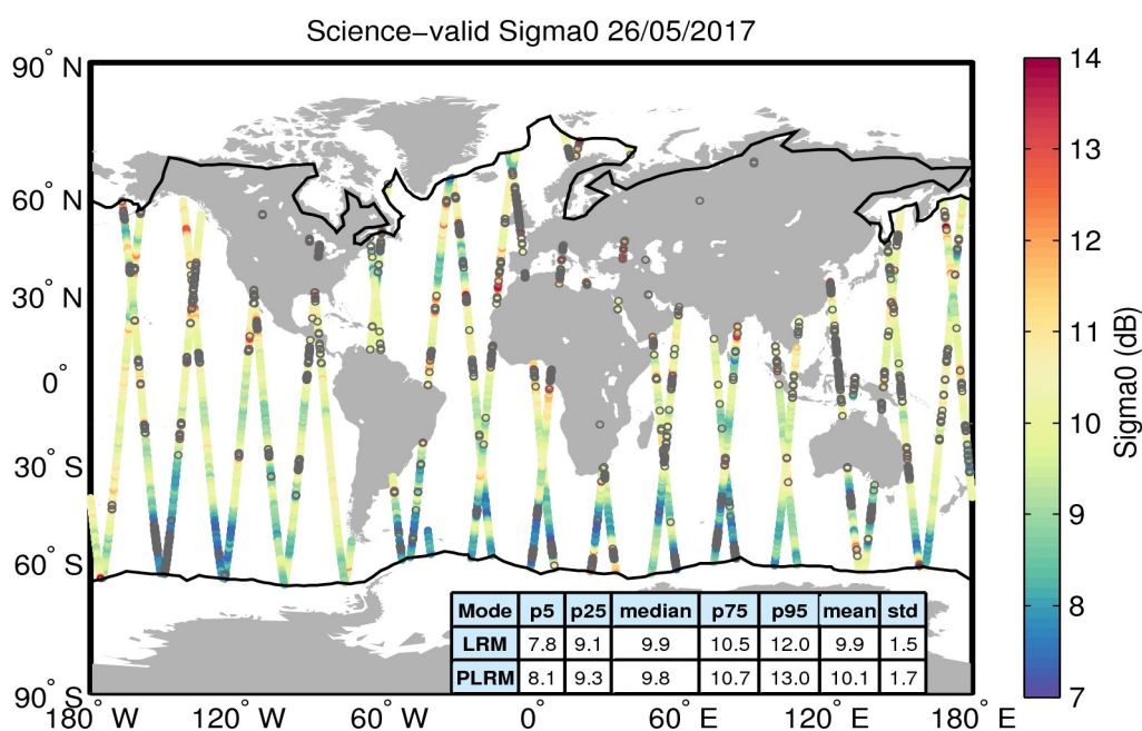
Figure 27. Geographical distribution of science-valid sigma0 data over oceans and lakes for 26/05/2017. The statistical values shown in the table refer to the sigma0 in dB and are calculated separately for LRM and PLRM regions. The black lines mark the outer limit of the Arctic and Antarctic polar polygons. Gray circles denote records that have been rejected based on the editing criteria described in Table 4.
