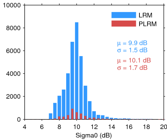
Figure 28. Histogram of science-valid sigma0 over oceans and lakes for LRM (blue) and PLRM (red) for 26/05/2017. The mean ( \mu ) and standard deviation ( \sigma ) are also shown. Note that values outside [4 20] dB are excluded from the histogram for the sake of readability but not from the computation of \mu and \sigma .
