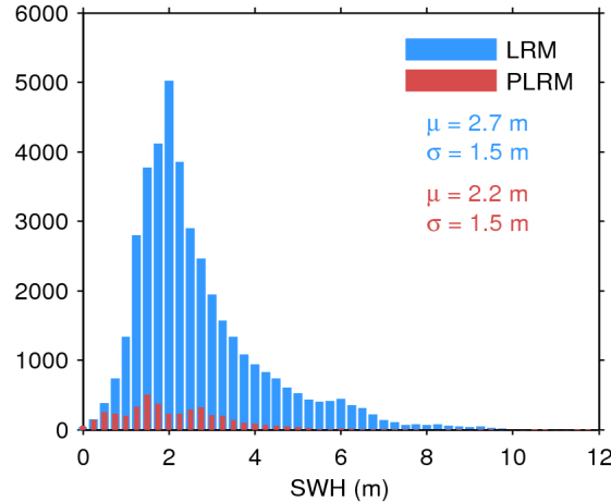
Figure 17. Histogram of flag-valid SWH over oceans and lakes for LRM (blue) and PLRM (red) for 26/05/2017. The mean ( \mu ) and standard deviation ( \sigma ) are also shown. Note that values larger than 12 m are excluded from the histogram for the sake of readability but not from the computation of \mu and \sigma .
