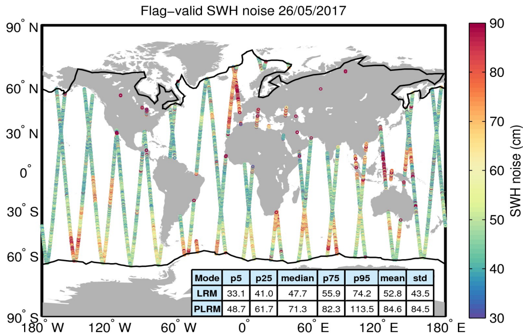
Figure 18. Geographical distribution of flag-valid 20-Hz SWH measurement noise over oceans and lakes for 26/05/2017. The statistical values shown in the table refer to the SWH noise and are calculated separately for LRM and PLRM regions. Measurements taken over polar polygons have been excluded from the computation of the statistical values. The black lines mark the outer limit of the Arctic and Antarctic polar polygons.
