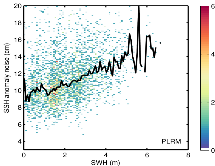
Figure 9. 2D histogram showing flag-valid SSH anomaly noise as a function of SWH for LRM (top) and PLRM (bottom) for 26/05/2017. The black line denotes the median SSH anomaly noise as a function of SWH.
