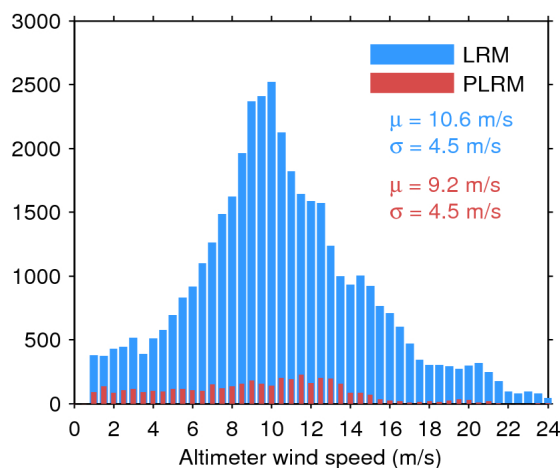
Figure 35. Histogram of science-valid wind over oceans and lakes for LRM (blue) and PLRM (red) for 25/05/2017. The mean ( \mu ) and standard deviation ( \sigma ) are also shown. Note that values larger than 24 m/s are excluded from the histogram for the sake of readability but not from the computation of \mu and \sigma .
