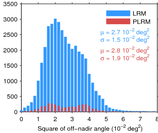
Figure 39. Histogram of flag-valid mispointing over oceans and lakes for LRM (blue) and PLRM (red) for 25/05/2017. Only positive values have been considered. The mean ( \mu ) and standard deviation ( \sigma ) are also shown. Note that values larger than 8 \cdot 10^{-2} \text{ deg}^2 are excluded from the histogram for the sake of readability but not from the computation of \mu and \sigma .
