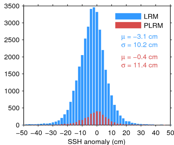
Figure 11. Histogram of science-valid SSH anomaly over oceans and lakes for LRM (blue) and PLRM (red) for 25/05/2017. The mean ( \mu ) and standard deviation ( \sigma ) are also shown. Note that values outside [-50 50] cm are excluded from the histogram for the sake of readability but not from the computation of \mu and \sigma .
