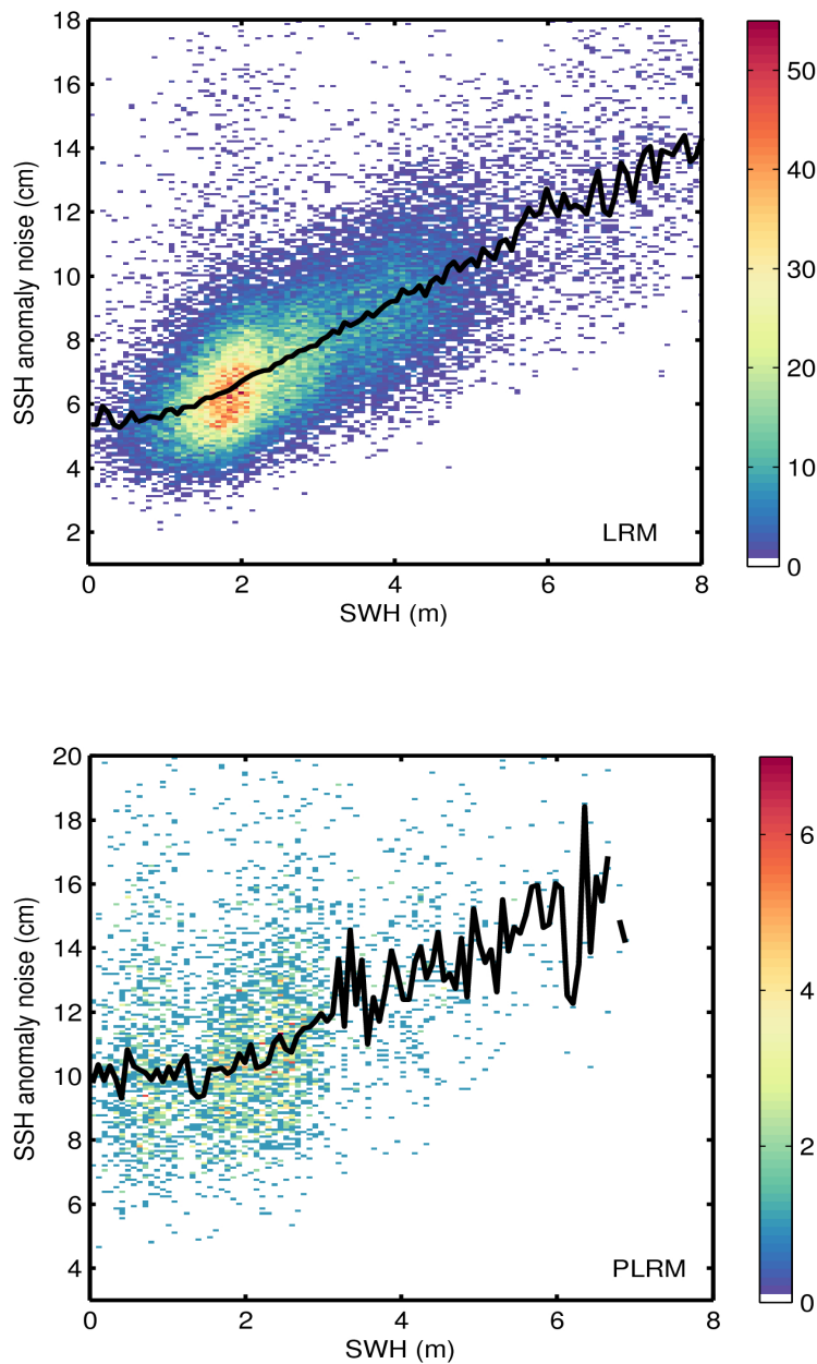
Figure 9. 2D histogram showing flag-valid SSH anomaly noise as a function of SWH for LRM (top) and PLRM (bottom) for 25/05/2017. The black line denotes the median SSH anomaly noise as a function of SWH.
