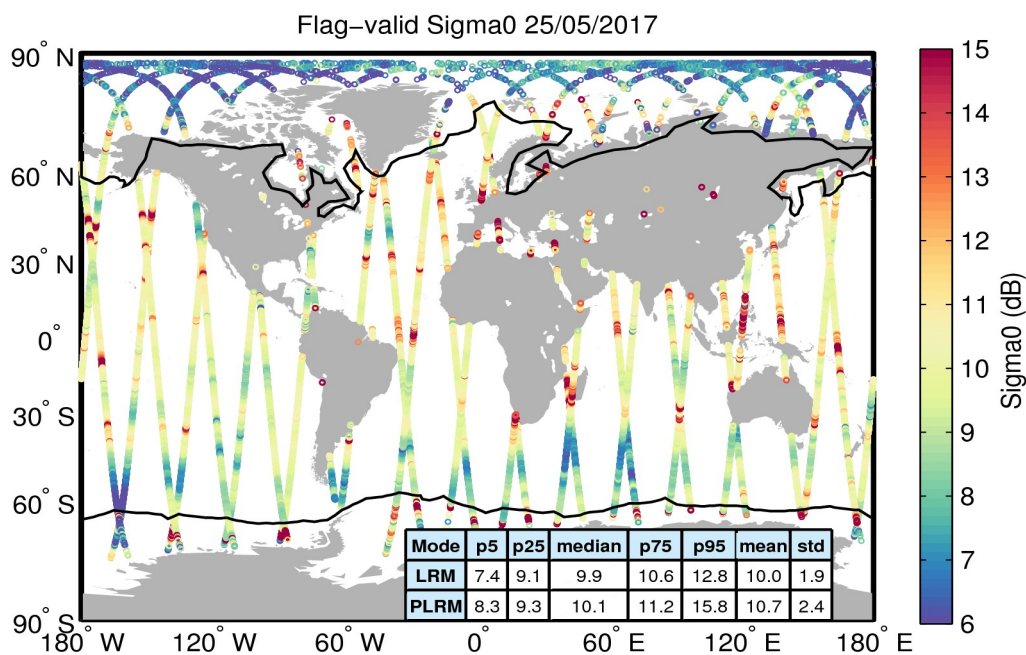
Figure 23. Geographical distribution of flag-valid sigma0 data over oceans and lakes for 25/05/2017. The statistical values shown in the table refer to the sigma0 in dB and are calculated separately for LRM and PLRM regions. Measurements taken over polar polygons have been excluded from the computation of the statistical values. The black lines mark the outer limit of the Arctic and Antarctic polar polygons.
