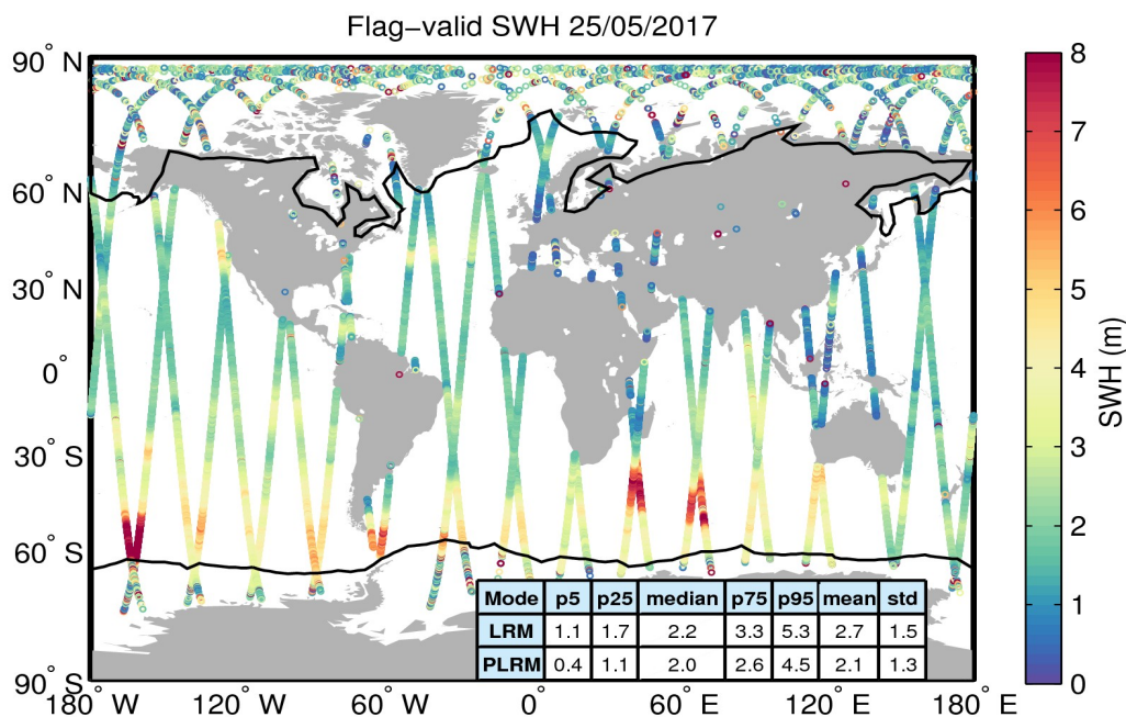
Figure 15. Geographical distribution of flag-valid SWH data over oceans and lakes for 25/05/2017. The statistical values shown in the table refer to the SWH in m and are calculated separately for LRM and PLRM regions. Measurements taken over polar polygons have been excluded from the computation of the statistical values. The black lines mark the outer limit of the Arctic and Antarctic polar polygons.
