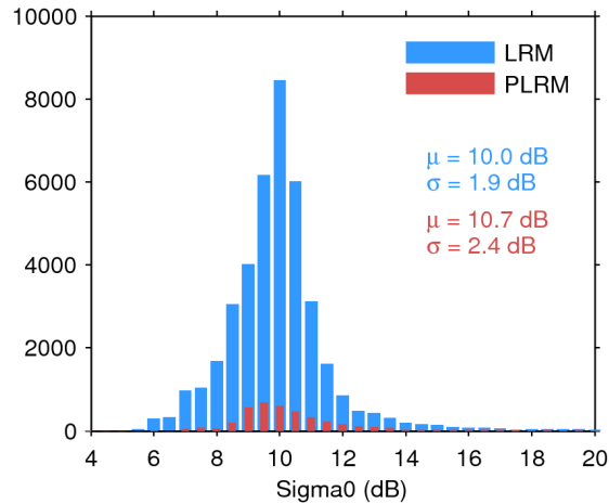
Figure 25. Histogram of flag-valid sigma0 over oceans and lakes for LRM (blue) and PLRM (red) for 25/05/2017. The mean ( \mu ) and standard deviation ( \sigma ) are also shown. Note that values outside [4 20] dB are excluded from the histogram for the sake of readability but not from the computation of \mu and \sigma .
