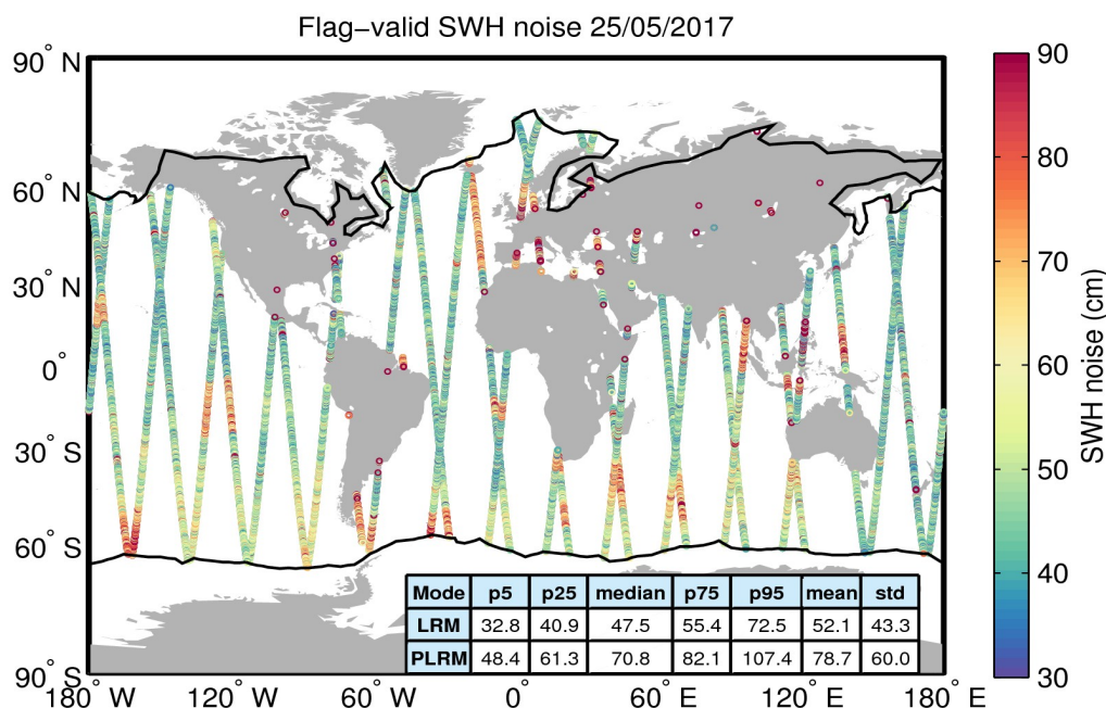
Figure 18. Geographical distribution of flag-valid 20-Hz SWH measurement noise over oceans and lakes for 25/05/2017. The statistical values shown in the table refer to the SWH noise and are calculated separately for LRM and PLRM regions. Measurements taken over polar polygons have been excluded from the computation of the statistical values. The black lines mark the outer limit of the Arctic and Antarctic polar polygons.
