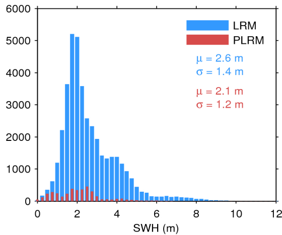
Figure 20. Histogram of science-valid SWH over oceans and lakes for LRM (blue) and PLRM (red) for 25/05/2017. The mean ( \mu ) and standard deviation ( \sigma ) are also shown. Note that values larger than 12 m are excluded from the histogram for the sake of readability but not from the computation of \mu and \sigma .
