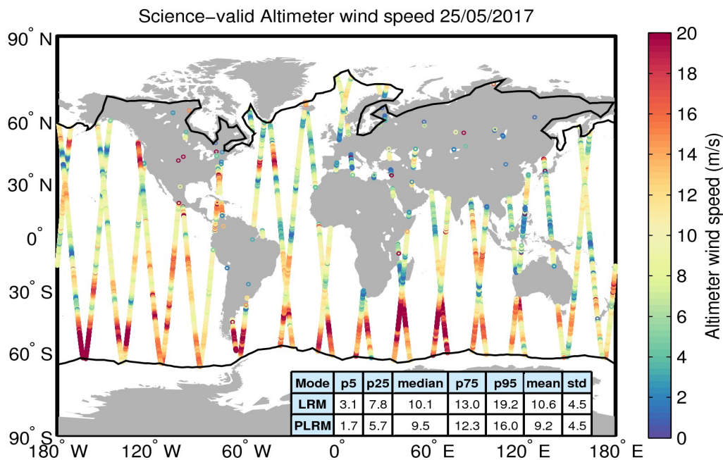
Figure 34. Geographical distribution of science-valid wind data over oceans and lakes for 25/05/2017. The statistical values shown in the table refer to the wind in m/s and are calculated separately for LRM and PLRM regions. The black lines mark the outer limit of the Arctic and Antarctic polar polygons. Gray circles denote records that have been rejected based on the editing criteria described in Table 5.
