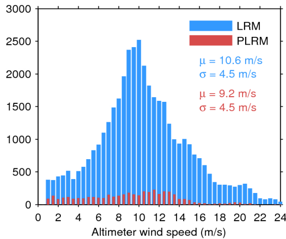
Figure 33. Histogram of flag-valid wind over oceans and lakes for LRM (blue) and PLRM (red) for 25/05/2017. The mean ( \mu ) and standard deviation ( \sigma ) are also shown. Note that values larger than 24 m/s are excluded from the histogram for the sake of readability but not from the computation of \mu and \sigma .
