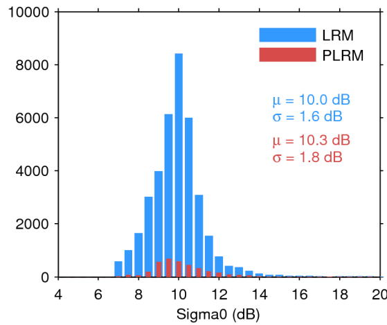
Figure 28. Histogram of science-valid sigma0 over oceans and lakes for LRM (blue) and PLRM (red) for 25/05/2017. The mean ( \mu ) and standard deviation ( \sigma ) are also shown. Note that values outside [4 20] dB are excluded from the histogram for the sake of readability but not from the computation of \mu and \sigma .
