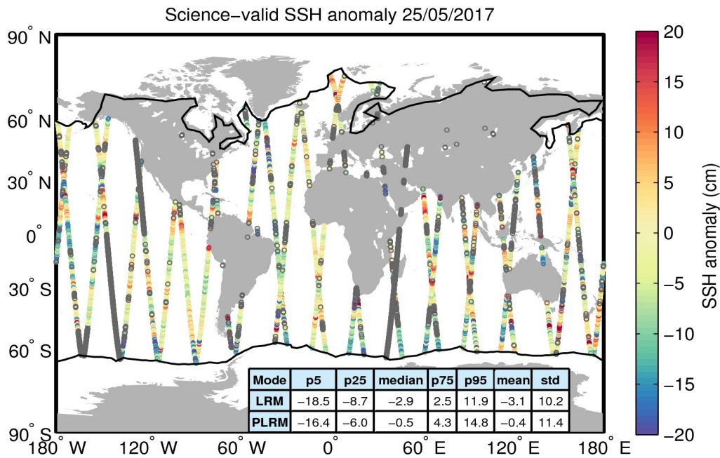
Figure 10. Geographical distribution of science-valid SSH anomaly data over oceans and lakes for 25/05/2017. The statistical values shown in the table refer to the SSH anomaly in cm and are calculated separately for LRM and PLRM regions. The black lines mark the outer limit of the Arctic and Antarctic polar polygons. Gray circles denote records that have been rejected based on the editing criteria described in Table 2.
