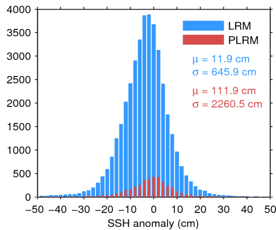
Figure 7. Histogram of flag-valid SSH anomaly over oceans and lakes for LRM (blue) and PLRM (red) for 25/05/2017. The mean ( \mu ) and standard deviation ( \sigma ) are also shown. Note that values outside [-50 50] cm are excluded from the histogram for the sake of readability but not from the computation of \mu and \sigma .
