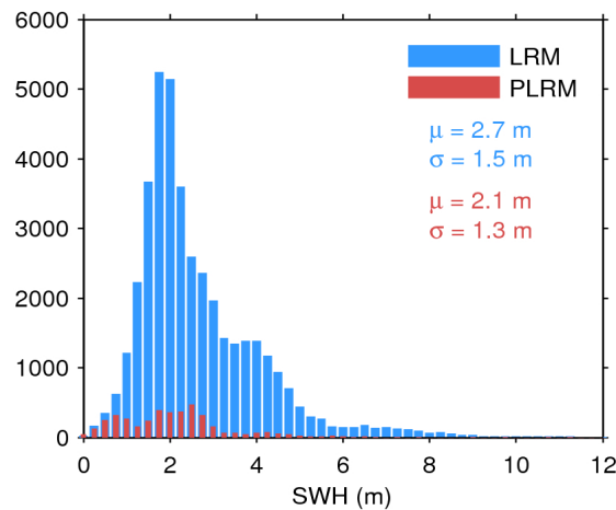
Figure 17. Histogram of flag-valid SWH over oceans and lakes for LRM (blue) and PLRM (red) for 25/05/2017. The mean ( \mu ) and standard deviation ( \sigma ) are also shown. Note that values larger than 12 m are excluded from the histogram for the sake of readability but not from the computation of \mu and \sigma .
