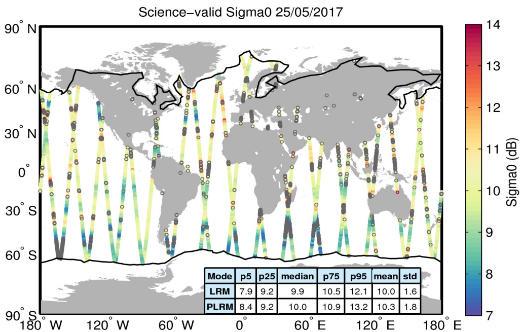
Figure 27. Geographical distribution of science-valid sigma0 data over oceans and lakes for 25/05/2017. The statistical values shown in the table refer to the sigma0 in dB and are calculated separately for LRM and PLRM regions. The black lines mark the outer limit of the Arctic and Antarctic polar polygons. Gray circles denote records that have been rejected based on the editing criteria described in Table 4.
