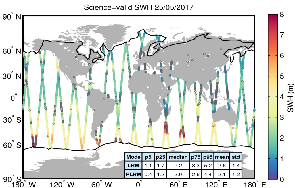
Figure 19. Geographical distribution of science-valid SWH data over oceans and lakes for 25/05/2017. The statistical values shown in the table refer to the SWH in m and are calculated separately for LRM and PLRM regions. The black lines mark the outer limit of the Arctic and Antarctic polar polygons. Gray circles denote records that have been rejected based on the editing criteria described in Table 3.
