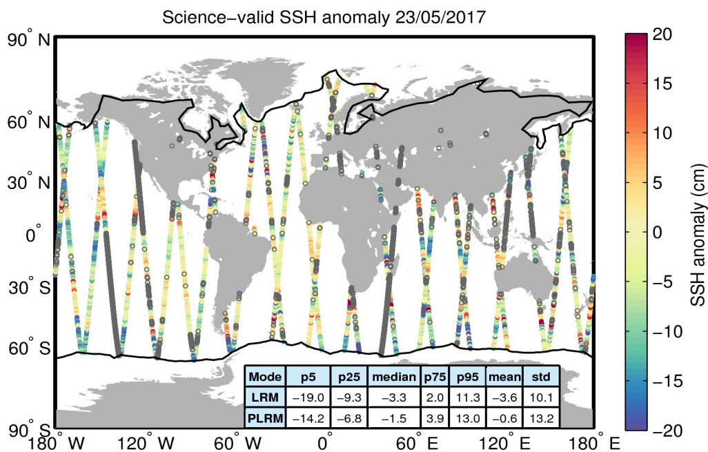
Figure 10. Geographical distribution of science-valid SSH anomaly data over oceans and lakes for 23/05/2017. The statistical values shown in the table refer to the SSH anomaly in cm and are calculated separately for LRM and PLRM regions. The black lines mark the outer limit of the Arctic and Antarctic polar polygons. Gray circles denote records that have been rejected based on the editing criteria described in Table 2.
