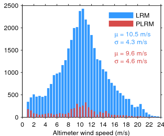
Figure 35. Histogram of science-valid wind over oceans and lakes for LRM (blue) and PLRM (red) for 23/05/2017. The mean ( \mu ) and standard deviation ( \sigma ) are also shown. Note that values larger than 24 m/s are excluded from the histogram for the sake of readability but not from the computation of \mu and \sigma .
