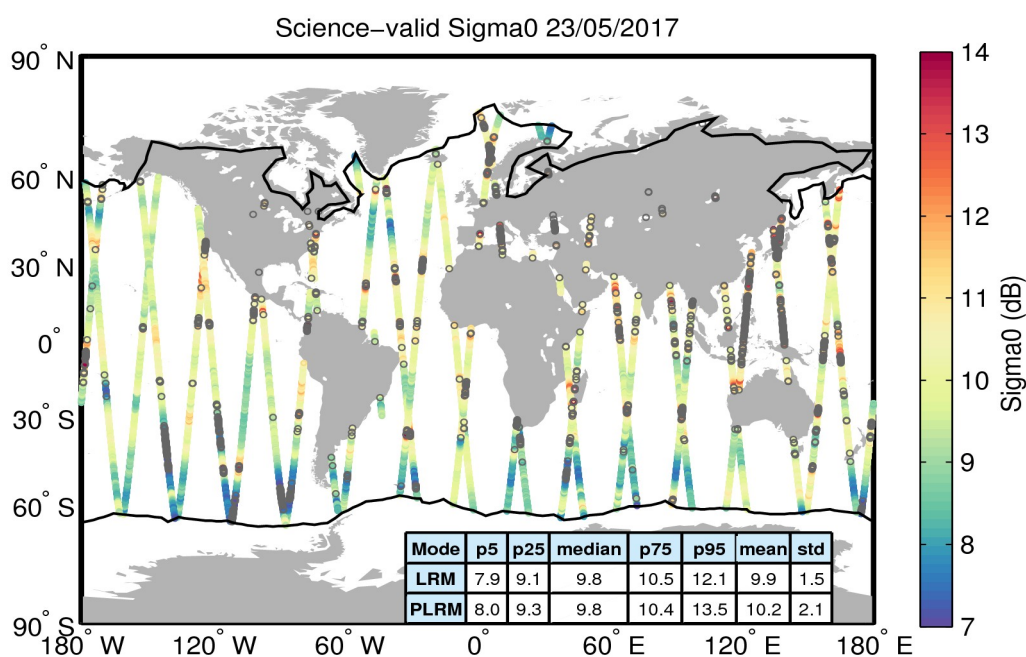
Figure 27. Geographical distribution of science-valid sigma0 data over oceans and lakes for 23/05/2017. The statistical values shown in the table refer to the sigma0 in dB and are calculated separately for LRM and PLRM regions. The black lines mark the outer limit of the Arctic and Antarctic polar polygons. Gray circles denote records that have been rejected based on the editing criteria described in Table 4.
