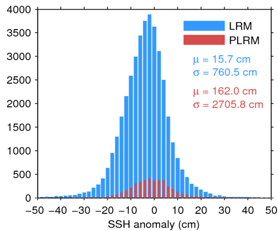
Figure 7. Histogram of flag-valid SSH anomaly over oceans and lakes for LRM (blue) and PLRM (red) for 23/05/2017. The mean ( \mu ) and standard deviation ( \sigma ) are also shown. Note that values outside [-50 50] cm are excluded from the histogram for the sake of readability but not from the computation of \mu and \sigma .
