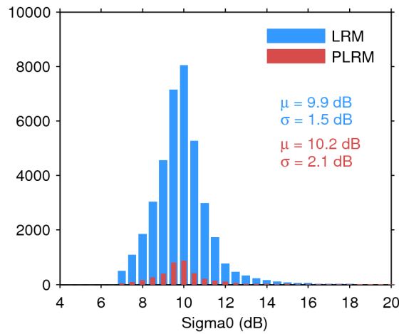
Figure 28. Histogram of science-valid sigma0 over oceans and lakes for LRM (blue) and PLRM (red) for 23/05/2017. The mean ( \mu ) and standard deviation ( \sigma ) are also shown. Note that values outside [4 20] dB are excluded from the histogram for the sake of readability but not from the computation of \mu and \sigma .
