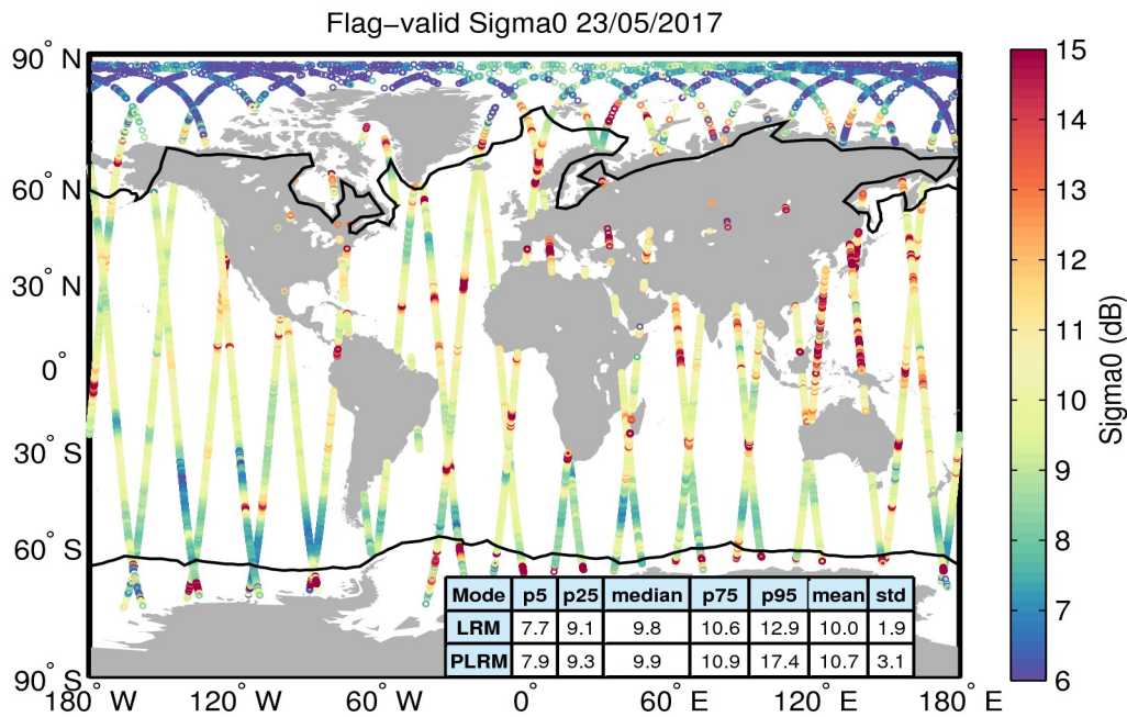
Figure 23. Geographical distribution of flag-valid sigma0 data over oceans and lakes for 23/05/2017. The statistical values shown in the table refer to the sigma0 in dB and are calculated separately for LRM and PLRM regions. Measurements taken over polar polygons have been excluded from the computation of the statistical values. The black lines mark the outer limit of the Arctic and Antarctic polar polygons.
