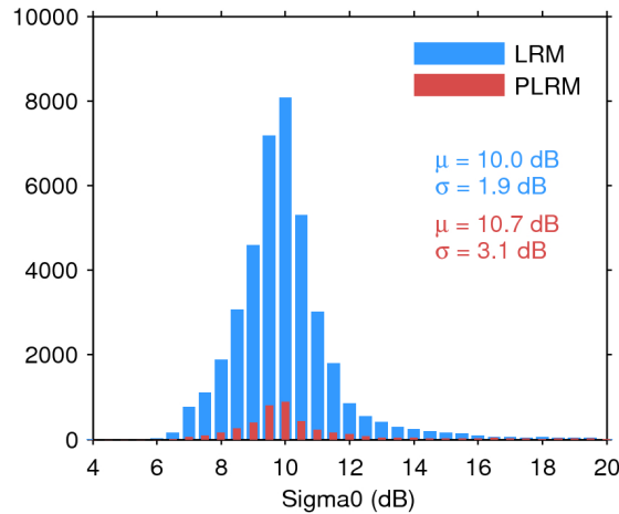
Figure 25. Histogram of flag-valid sigma0 over oceans and lakes for LRM (blue) and PLRM (red) for 23/05/2017. The mean ( \mu ) and standard deviation ( \sigma ) are also shown. Note that values outside [4 20] dB are excluded from the histogram for the sake of readability but not from the computation of \mu and \sigma .
