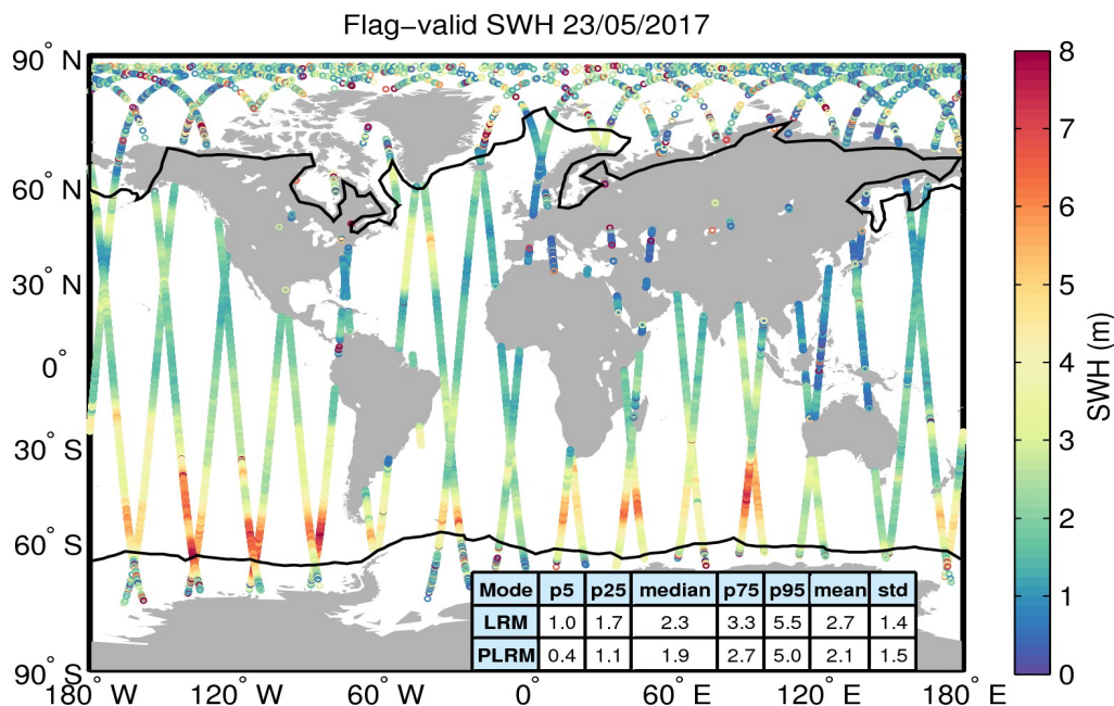
Figure 15. Geographical distribution of flag-valid SWH data over oceans and lakes for 23/05/2017. The statistical values shown in the table refer to the SWH in m and are calculated separately for LRM and PLRM regions. Measurements taken over polar polygons have been excluded from the computation of the statistical values. The black lines mark the outer limit of the Arctic and Antarctic polar polygons.
