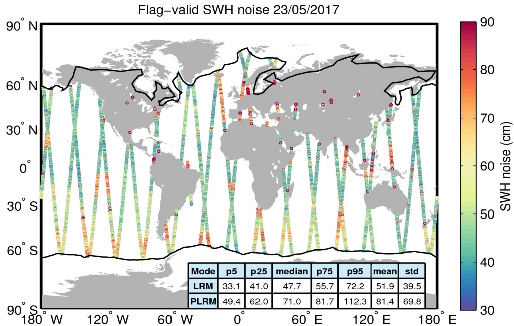
Figure 18. Geographical distribution of flag-valid 20-Hz SWH measurement noise over oceans and lakes for 23/05/2017. The statistical values shown in the table refer to the SWH noise and are calculated separately for LRM and PLRM regions. Measurements taken over polar polygons have been excluded from the computation of the statistical values. The black lines mark the outer limit of the Arctic and Antarctic polar polygons.
