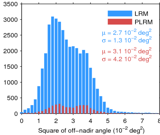
Figure 39. Histogram of flag-valid mispointing over oceans and lakes for LRM (blue) and PLRM (red) for 23/05/2017. Only positive values have been considered. The mean ( \mu ) and standard deviation ( \sigma ) are also shown. Note that values larger than 8 \cdot 10^{-2} \text{ deg}^2 are excluded from the histogram for the sake of readability but not from the computation of \mu and \sigma .
