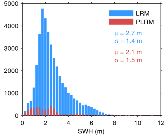
Figure 17. Histogram of flag-valid SWH over oceans and lakes for LRM (blue) and PLRM (red) for 23/05/2017. The mean ( \mu ) and standard deviation ( \sigma ) are also shown. Note that values larger than 12 m are excluded from the histogram for the sake of readability but not from the computation of \mu and \sigma .
