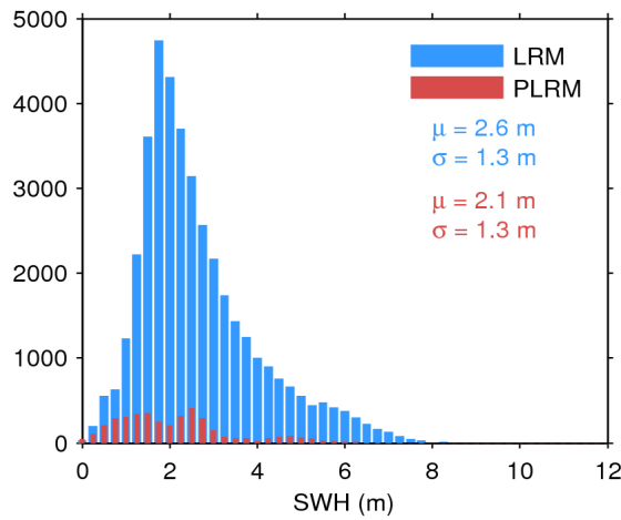
Figure 20. Histogram of science-valid SWH over oceans and lakes for LRM (blue) and PLRM (red) for 23/05/2017. The mean ( \mu ) and standard deviation ( \sigma ) are also shown. Note that values larger than 12 m are excluded from the histogram for the sake of readability but not from the computation of \mu and \sigma .
