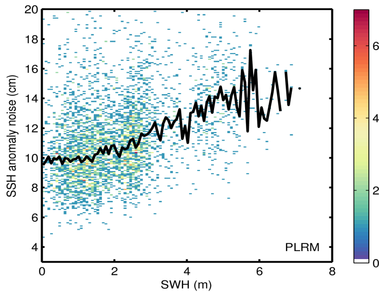
Figure 9. 2D histogram showing flag-valid SSH anomaly noise as a function of SWH for LRM (top) and PLRM (bottom) for 23/05/2017. The black line denotes the median SSH anomaly noise as a function of SWH.
