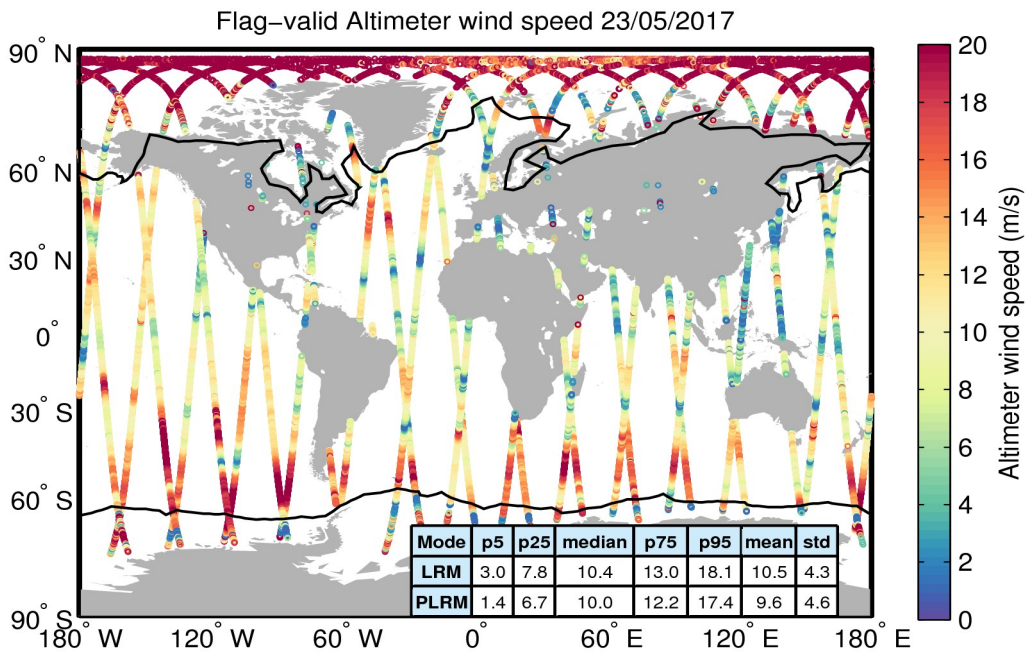
Figure 31. Geographical distribution of flag-valid wind data over oceans and lakes for 23/05/2017. The statistical values shown in the table refer to the wind in m/s and are calculated separately for LRM and PLRM regions. Measurements taken over polar polygons have been excluded from the computation of the statistical values. The black lines mark the outer limit of the Arctic and Antarctic polar polygons.
