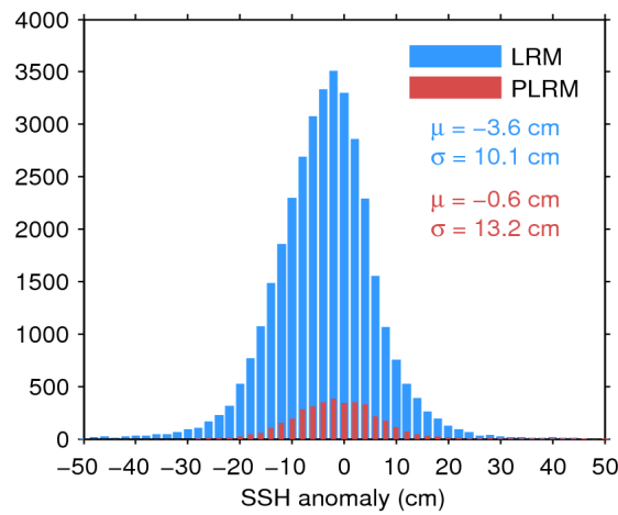
Figure 11. Histogram of science-valid SSH anomaly over oceans and lakes for LRM (blue) and PLRM (red) for 23/05/2017. The mean ( \mu ) and standard deviation ( \sigma ) are also shown. Note that values outside [-50\ 50] cm are excluded from the histogram for the sake of readability but not from the computation of \mu and \sigma .
