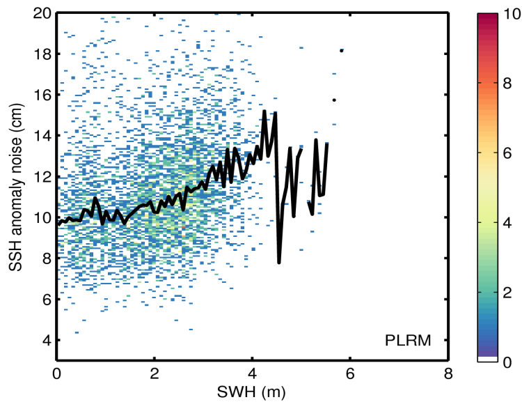
Figure 9. 2D histogram showing flag-valid SSH anomaly noise as a function of SWH for LRM (top) and PLRM (bottom) for 17/05/2017. The black line denotes the median SSH anomaly noise as a function of SWH.
