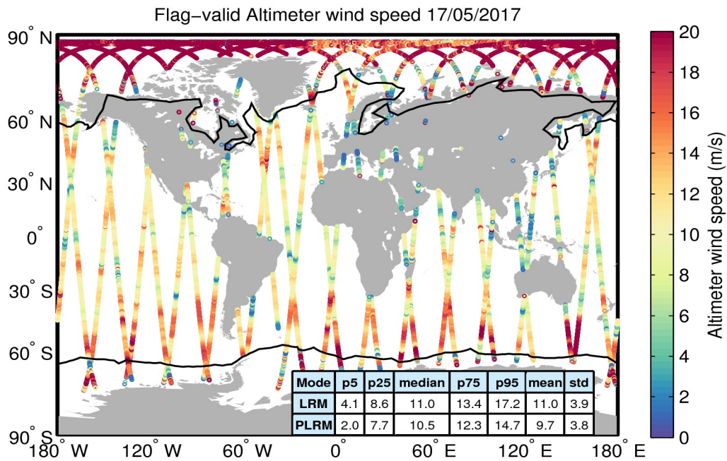
Figure 31. Geographical distribution of flag-valid wind data over oceans and lakes for 17/05/2017. The statistical values shown in the table refer to the wind in m/s and are calculated separately for LRM and PLRM regions. Measurements taken over polar polygons have been excluded from the computation of the statistical values. The black lines mark the outer limit of the Arctic and Antarctic polar polygons.
