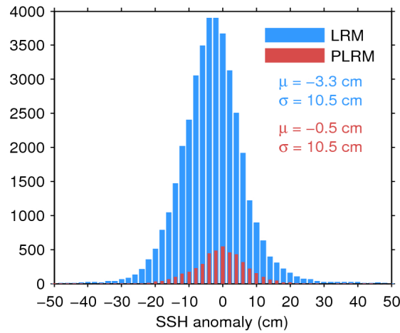
Figure 11. Histogram of science-valid SSH anomaly over oceans and lakes for LRM (blue) and PLRM (red) for 17/05/2017. The mean ( \mu ) and standard deviation ( \sigma ) are also shown. Note that values outside [-50\ 50] cm are excluded from the histogram for the sake of readability but not from the computation of \mu and \sigma .
