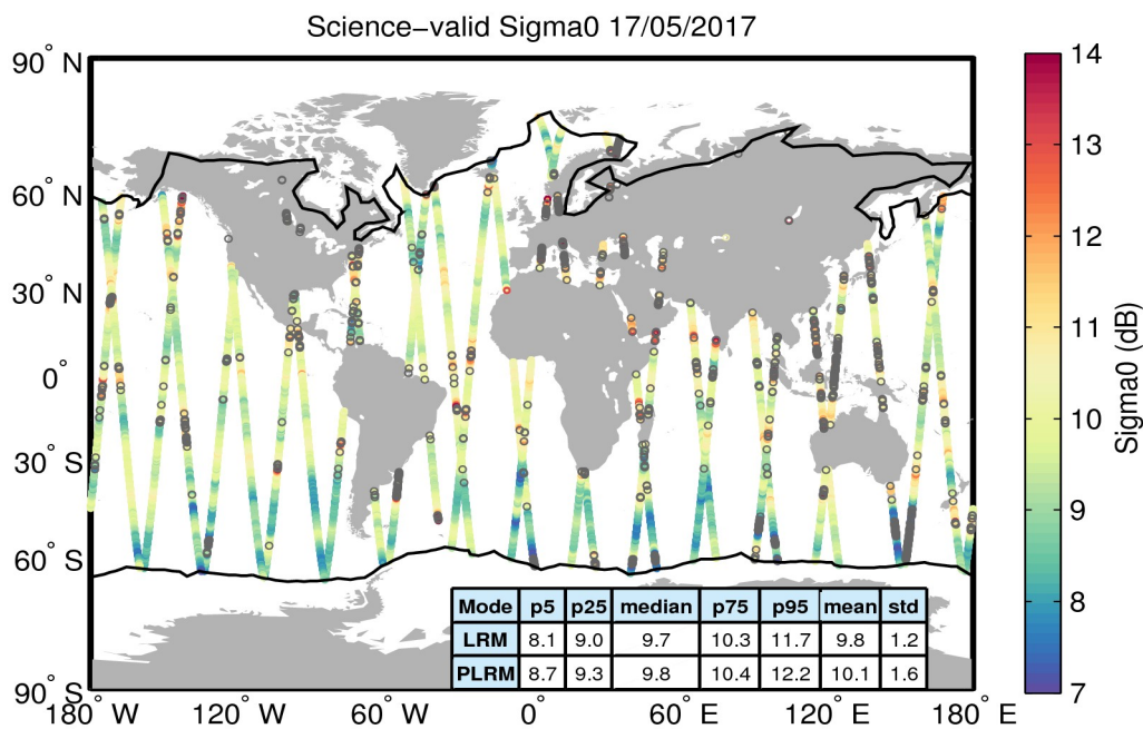
Figure 27. Geographical distribution of science-valid sigma0 data over oceans and lakes for 17/05/2017. The statistical values shown in the table refer to the sigma0 in dB and are calculated separately for LRM and PLRM regions. The black lines mark the outer limit of the Arctic and Antarctic polar polygons. Gray circles denote records that have been rejected based on the editing criteria described in Table 4.
