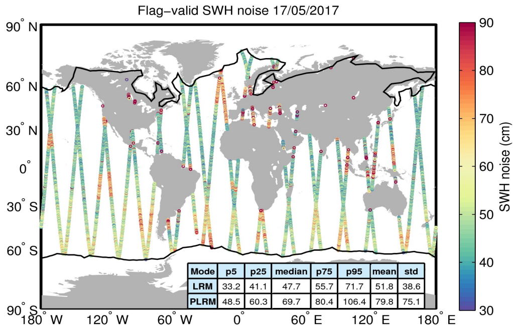
Figure 18. Geographical distribution of flag-valid 20-Hz SWH measurement noise over oceans and lakes for 17/05/2017. The statistical values shown in the table refer to the SWH noise and are calculated separately for LRM and PLRM regions. Measurements taken over polar polygons have been excluded from the computation of the statistical values. The black lines mark the outer limit of the Arctic and Antarctic polar polygons.
