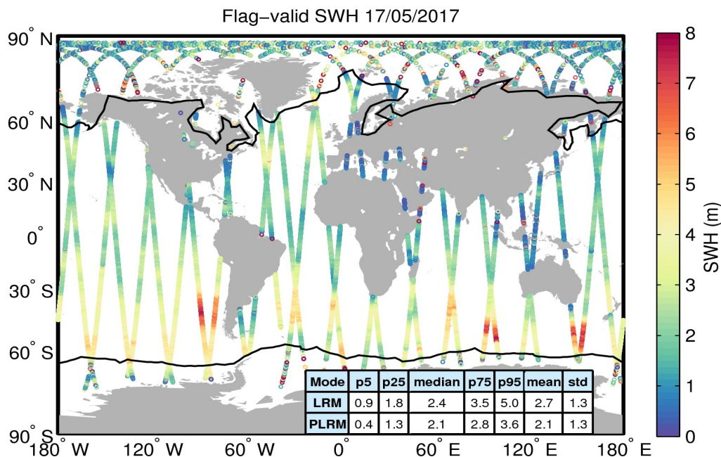
Figure 15. Geographical distribution of flag-valid SWH data over oceans and lakes for 17/05/2017. The statistical values shown in the table refer to the SWH in m and are calculated separately for LRM and PLRM regions. Measurements taken over polar polygons have been excluded from the computation of the statistical values. The black lines mark the outer limit of the Arctic and Antarctic polar polygons.
