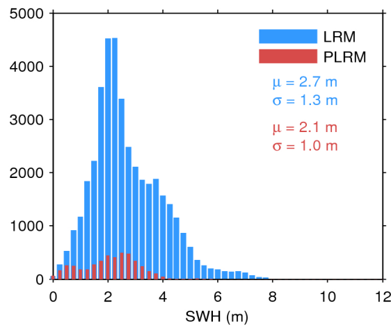
Figure 20. Histogram of science-valid SWH over oceans and lakes for LRM (blue) and PLRM (red) for 17/05/2017. The mean ( \mu ) and standard deviation ( \sigma ) are also shown. Note that values larger than 12 m are excluded from the histogram for the sake of readability but not from the computation of \mu and \sigma .
