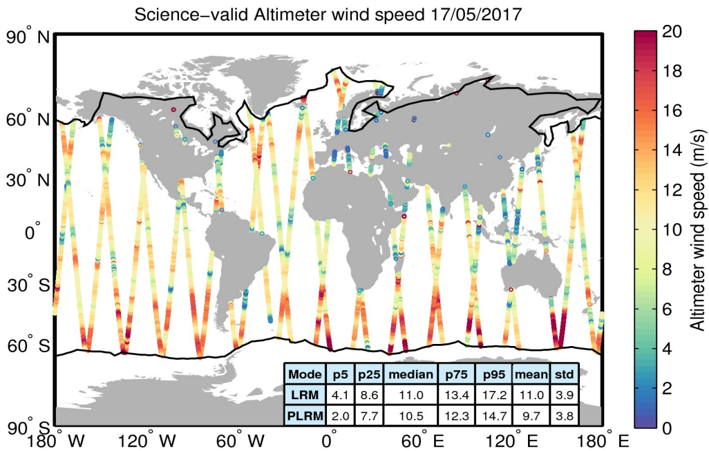
Figure 34. Geographical distribution of science-valid wind data over oceans and lakes for 17/05/2017. The statistical values shown in the table refer to the wind in m/s and are calculated separately for LRM and PLRM regions. The black lines mark the outer limit of the Arctic and Antarctic polar polygons. Gray circles denote records that have been rejected based on the editing criteria described in Table 5.
