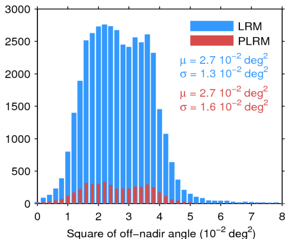
Figure 39. Histogram of flag-valid mispointing over oceans and lakes for LRM (blue) and PLRM (red) for 17/05/2017. Only positive values have been considered. The mean ( \mu ) and standard deviation ( \sigma ) are also shown. Note that values larger than 8 \cdot 10^{-2} \text{ deg}^2 are excluded from the histogram for the sake of readability but not from the computation of \mu and \sigma .
