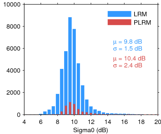
Figure 25. Histogram of flag-valid sigma0 over oceans and lakes for LRM (blue) and PLRM (red) for 17/05/2017. The mean ( \mu ) and standard deviation ( \sigma ) are also shown. Note that values outside [4 20] dB are excluded from the histogram for the sake of readability but not from the computation of \mu and \sigma .
