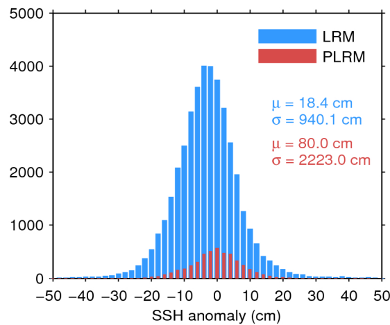
Figure 7. Histogram of flag-valid SSH anomaly over oceans and lakes for LRM (blue) and PLRM (red) for 17/05/2017. The mean ( \mu ) and standard deviation ( \sigma ) are also shown. Note that values outside [-50\ 50] cm are excluded from the histogram for the sake of readability but not from the computation of \mu and \sigma .
