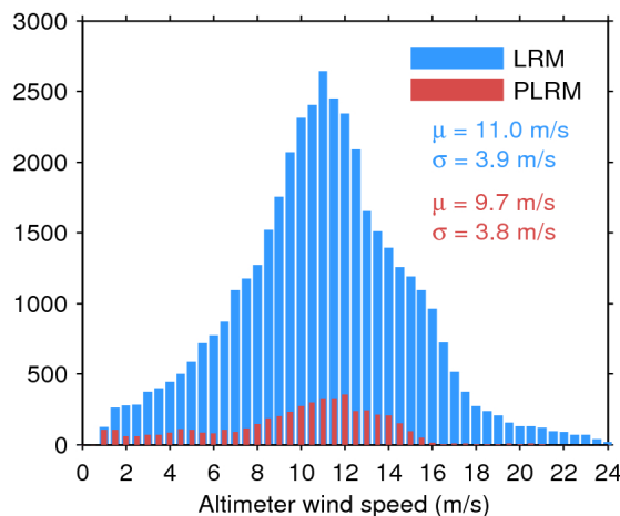
Figure 35. Histogram of science-valid wind over oceans and lakes for LRM (blue) and PLRM (red) for 17/05/2017. The mean ( \mu ) and standard deviation ( \sigma ) are also shown. Note that values larger than 24 m/s are excluded from the histogram for the sake of readability but not from the computation of \mu and \sigma .
