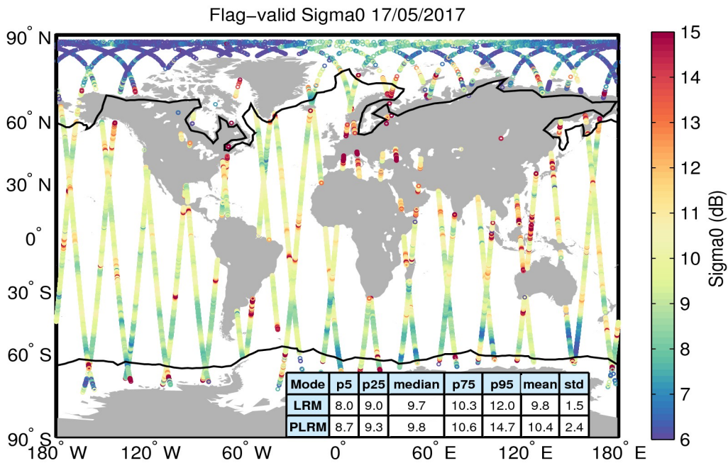
Figure 23. Geographical distribution of flag-valid sigma0 data over oceans and lakes for 17/05/2017. The statistical values shown in the table refer to the sigma0 in dB and are calculated separately for LRM and PLRM regions. Measurements taken over polar polygons have been excluded from the computation of the statistical values. The black lines mark the outer limit of the Arctic and Antarctic polar polygons.
