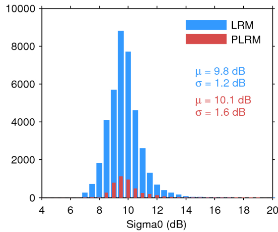
Figure 28. Histogram of science-valid sigma0 over oceans and lakes for LRM (blue) and PLRM (red) for 17/05/2017. The mean ( \mu ) and standard deviation ( \sigma ) are also shown. Note that values outside [4 20] dB are excluded from the histogram for the sake of readability but not from the computation of \mu and \sigma .
