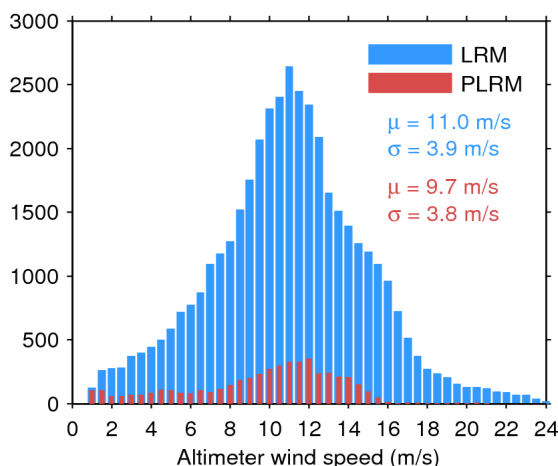
Figure 33. Histogram of flag-valid wind over oceans and lakes for LRM (blue) and PLRM (red) for 17/05/2017. The mean ( \mu ) and standard deviation ( \sigma ) are also shown. Note that values larger than 24 m/s are excluded from the histogram for the sake of readability but not from the computation of \mu and \sigma .
