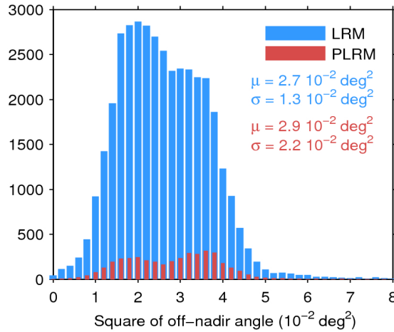
Figure 39. Histogram of flag-valid mispointing over oceans and lakes for LRM (blue) and PLRM (red) for 16/05/2017. Only positive values have been considered. The mean ( \mu ) and standard deviation ( \sigma ) are also shown. Note that values larger than 8 \cdot 10^{-2} \text{ deg}^2 are excluded from the histogram for the sake of readability but not from the computation of \mu and \sigma .
