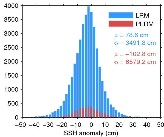
Figure 7. Histogram of flag-valid SSH anomaly over oceans and lakes for LRM (blue) and PLRM (red) for 16/05/2017. The mean ( \mu ) and standard deviation ( \sigma ) are also shown. Note that values outside [-50 50] cm are excluded from the histogram for the sake of readability but not from the computation of \mu and \sigma .
