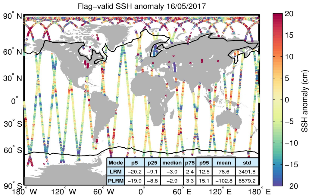
Figure 5. Geographical distribution of flag-valid 1-Hz SSH anomaly data over oceans and lakes for 16/05/2017. The statistical values shown in the table refer to the SSH anomaly in cm and are calculated separately for LRM and PLRM regions. Measurements taken over polar polygons have been excluded from the computation of the statistical values. The black lines mark the outer limit of the Arctic and Antarctic polar polygons.
