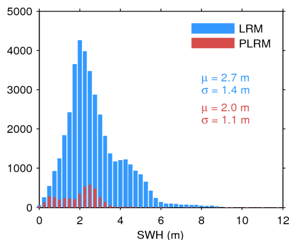
Figure 17. Histogram of flag-valid SWH over oceans and lakes for LRM (blue) and PLRM (red) for 16/05/2017. The mean ( \mu ) and standard deviation ( \sigma ) are also shown. Note that values larger than 12 m are excluded from the histogram for the sake of readability but not from the computation of \mu and \sigma .
