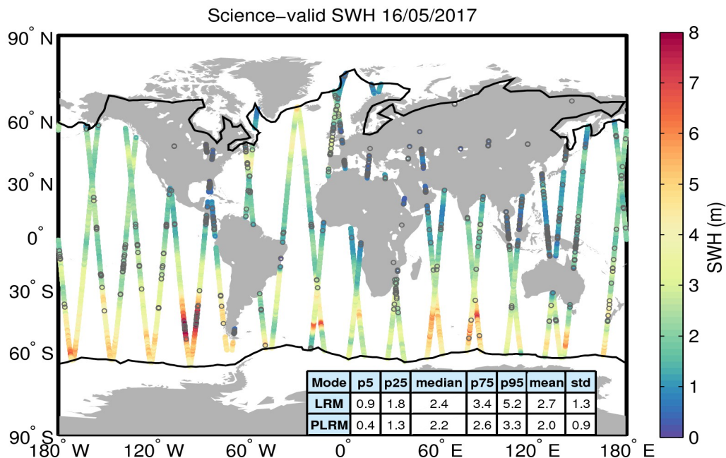
Figure 19. Geographical distribution of science-valid SWH data over oceans and lakes for 16/05/2017. The statistical values shown in the table refer to the SWH in m and are calculated separately for LRM and PLRM regions. The black lines mark the outer limit of the Arctic and Antarctic polar polygons. Gray circles denote records that have been rejected based on the editing criteria described in Table 3.
