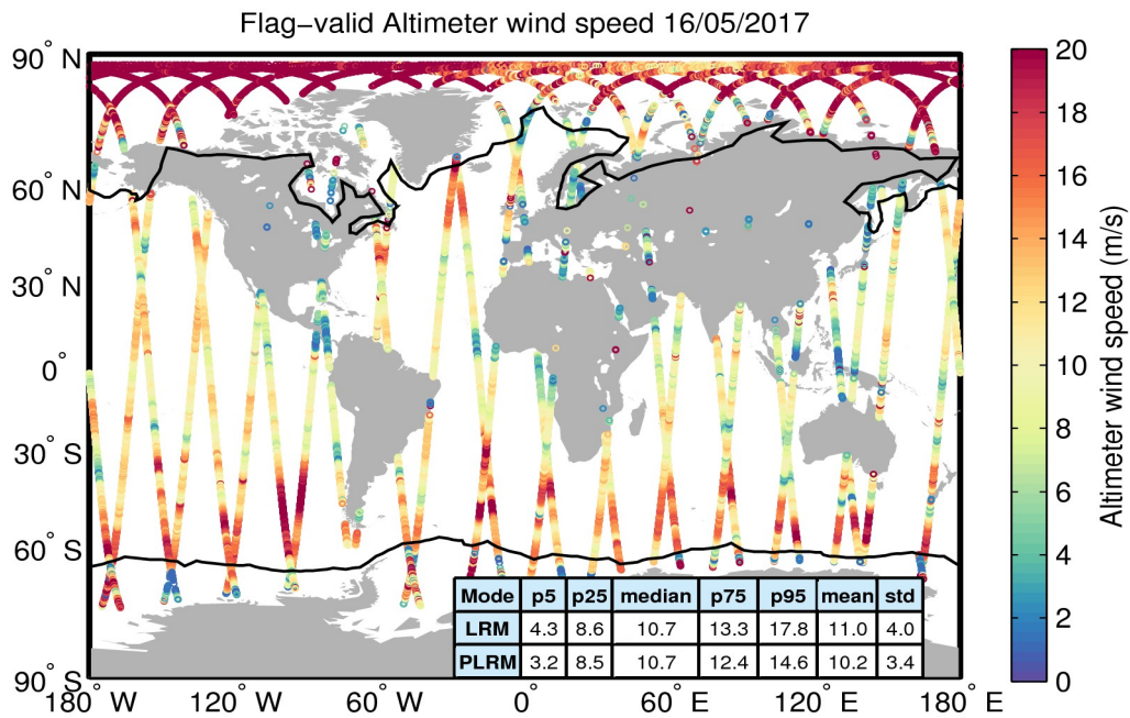
Figure 31. Geographical distribution of flag-valid wind data over oceans and lakes for 16/05/2017. The statistical values shown in the table refer to the wind in m/s and are calculated separately for LRM and PLRM regions. Measurements taken over polar polygons have been excluded from the computation of the statistical values. The black lines mark the outer limit of the Arctic and Antarctic polar polygons.
