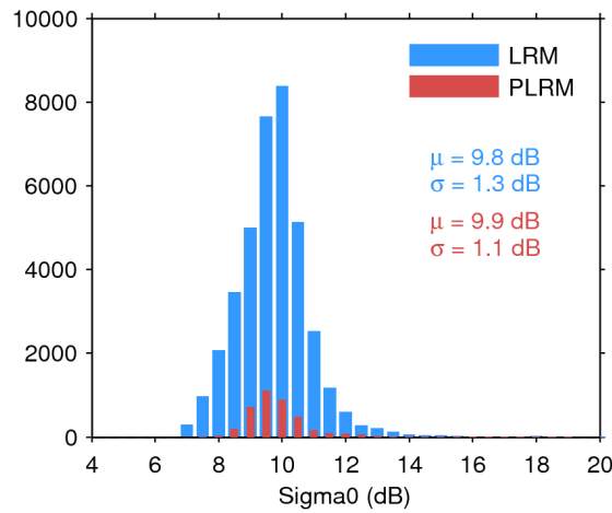
Figure 28. Histogram of science-valid sigma0 over oceans and lakes for LRM (blue) and PLRM (red) for 16/05/2017. The mean ( \mu ) and standard deviation ( \sigma ) are also shown. Note that values outside [4 20] dB are excluded from the histogram for the sake of readability but not from the computation of \mu and \sigma .
