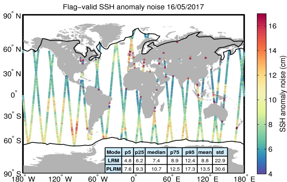
Figure 8. Geographical distribution of flag-valid 20-Hz SSH anomaly measurement noise over oceans and lakes for 16/05/2017. The statistical values shown in the table refer to the SSH anomaly noise and are calculated separately for LRM and PLRM regions. Measurements taken over polar polygons have been excluded from the computation of the statistical values. The black lines mark the outer limit of the Arctic and Antarctic polar polygons.
