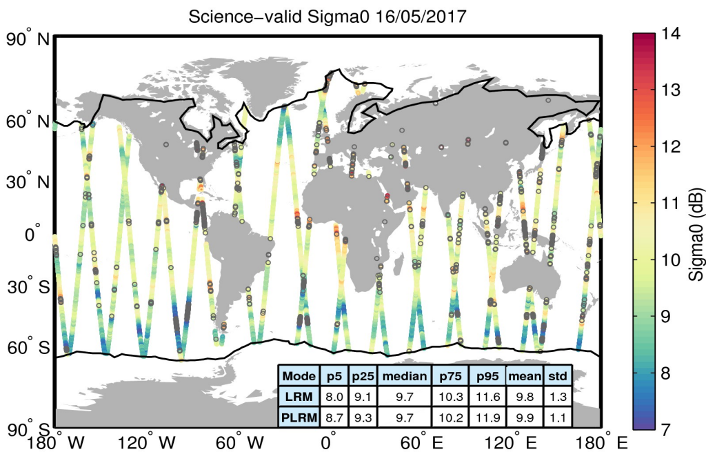
Figure 27. Geographical distribution of science-valid sigma0 data over oceans and lakes for 16/05/2017. The statistical values shown in the table refer to the sigma0 in dB and are calculated separately for LRM and PLRM regions. The black lines mark the outer limit of the Arctic and Antarctic polar polygons. Gray circles denote records that have been rejected based on the editing criteria described in Table 4.
