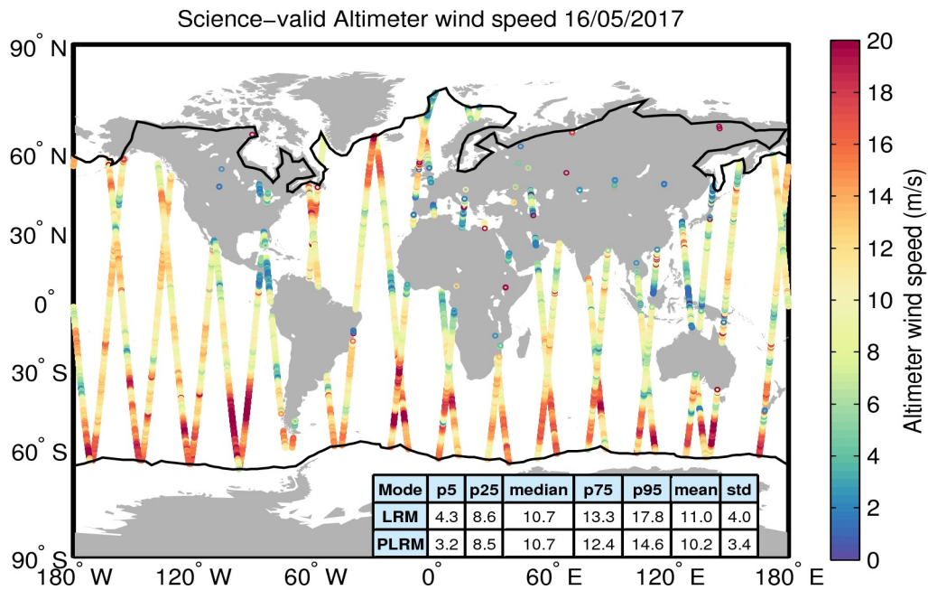
Figure 34. Geographical distribution of science-valid wind data over oceans and lakes for 16/05/2017. The statistical values shown in the table refer to the wind in m/s and are calculated separately for LRM and PLRM regions. The black lines mark the outer limit of the Arctic and Antarctic polar polygons. Gray circles denote records that have been rejected based on the editing criteria described in Table 5.
