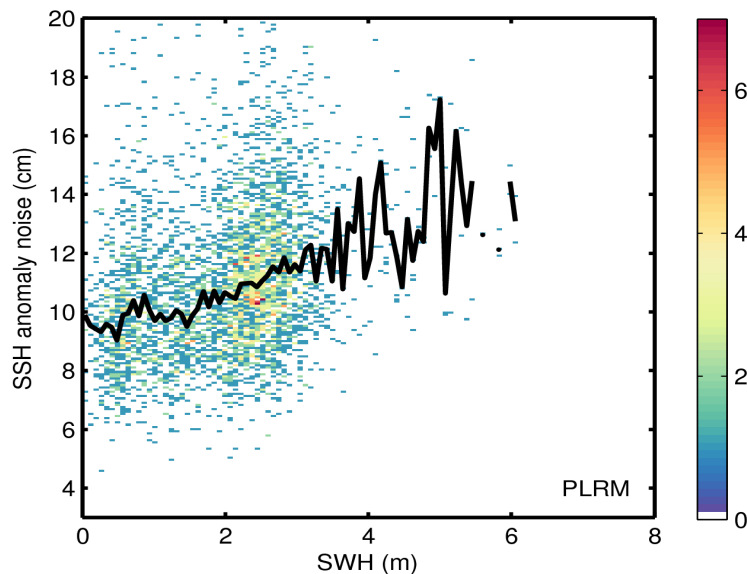
Figure 9. 2D histogram showing flag-valid SSH anomaly noise as a function of SWH for LRM (top) and PLRM (bottom) for 16/05/2017. The black line denotes the median SSH anomaly noise as a function of SWH.
