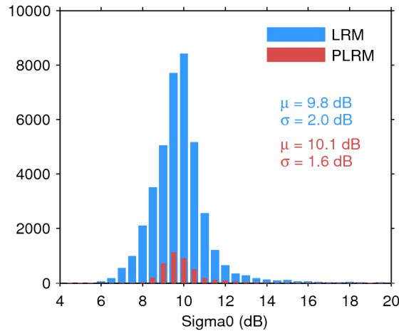
Figure 25. Histogram of flag-valid sigma0 over oceans and lakes for LRM (blue) and PLRM (red) for 16/05/2017. The mean ( \mu ) and standard deviation ( \sigma ) are also shown. Note that values outside [4 20] dB are excluded from the histogram for the sake of readability but not from the computation of \mu and \sigma .
