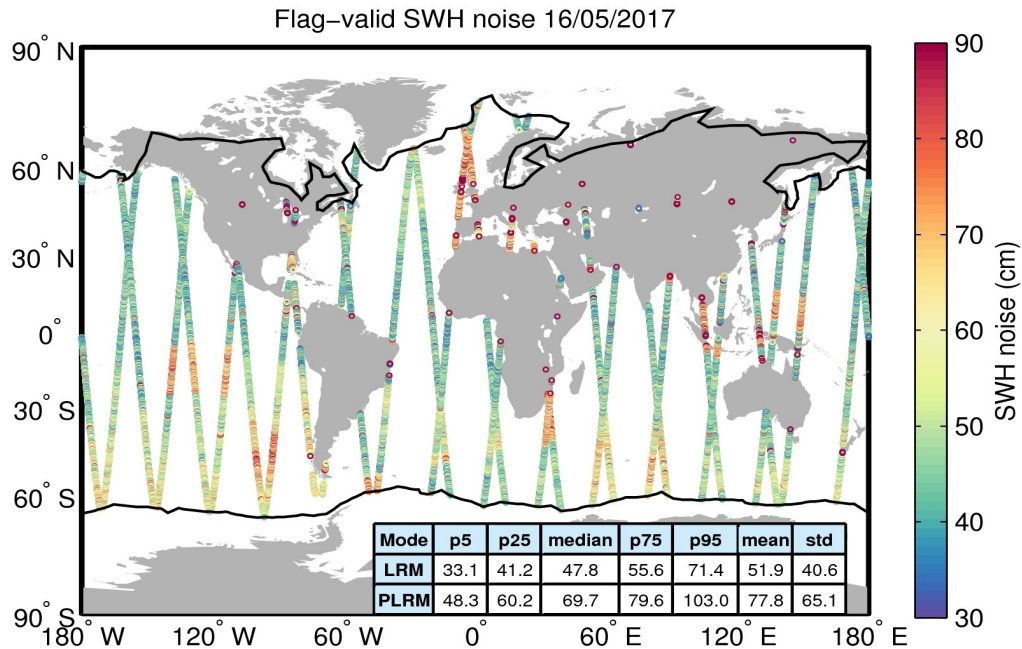
Figure 18. Geographical distribution of flag-valid 20-Hz SWH measurement noise over oceans and lakes for 16/05/2017. The statistical values shown in the table refer to the SWH noise and are calculated separately for LRM and PLRM regions. Measurements taken over polar polygons have been excluded from the computation of the statistical values. The black lines mark the outer limit of the Arctic and Antarctic polar polygons.
