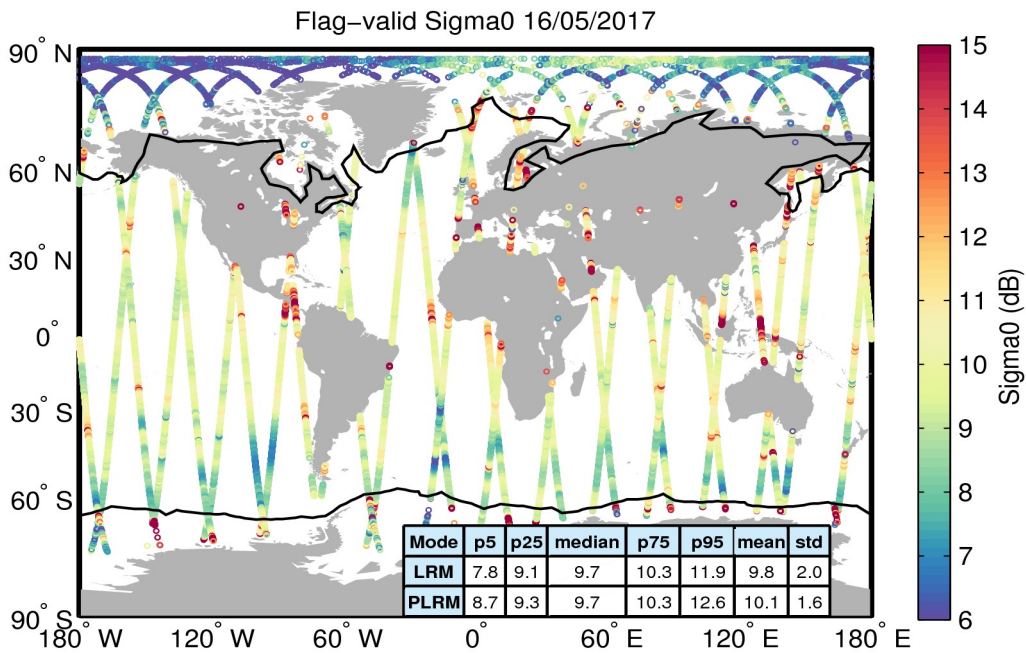
Figure 23. Geographical distribution of flag-valid sigma0 data over oceans and lakes for 16/05/2017. The statistical values shown in the table refer to the sigma0 in dB and are calculated separately for LRM and PLRM regions. Measurements taken over polar polygons have been excluded from the computation of the statistical values. The black lines mark the outer limit of the Arctic and Antarctic polar polygons.
