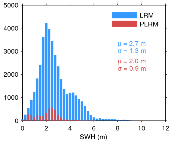
Figure 20. Histogram of science-valid SWH over oceans and lakes for LRM (blue) and PLRM (red) for 16/05/2017. The mean ( \mu ) and standard deviation ( \sigma ) are also shown. Note that values larger than 12 m are excluded from the histogram for the sake of readability but not from the computation of \mu and \sigma .
