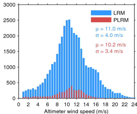
Figure 35. Histogram of science-valid wind over oceans and lakes for LRM (blue) and PLRM (red) for 16/05/2017. The mean ( \mu ) and standard deviation ( \sigma ) are also shown. Note that values larger than 24 m/s are excluded from the histogram for the sake of readability but not from the computation of \mu and \sigma .
