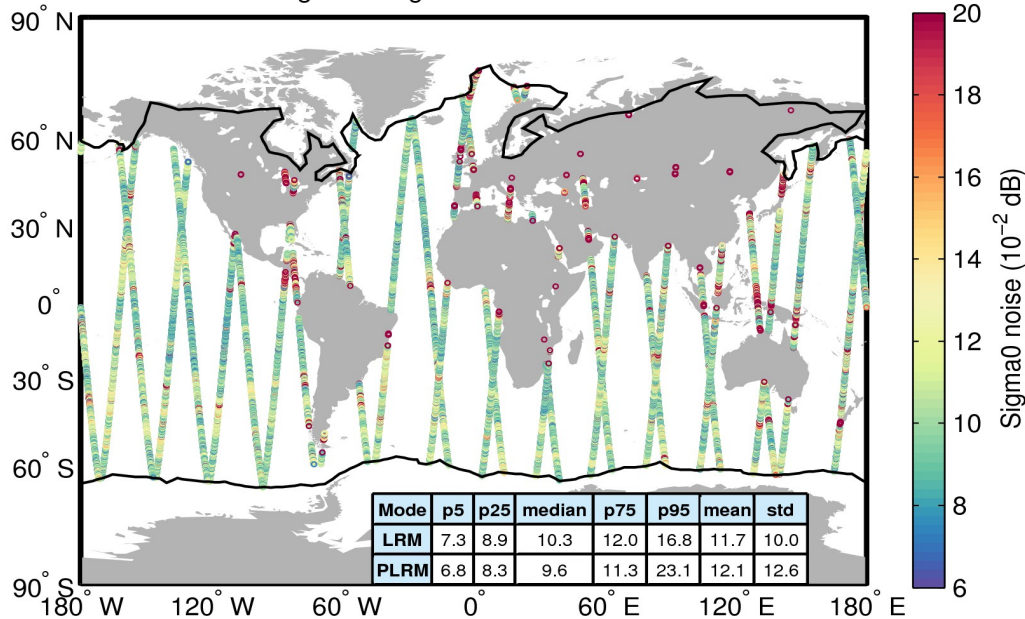
Flag-valid sigma0 noise 16/05/2017
