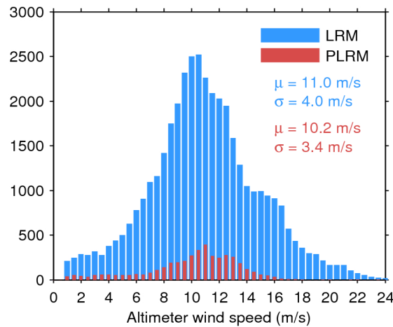
Figure 33. Histogram of flag-valid wind over oceans and lakes for LRM (blue) and PLRM (red) for 16/05/2017. The mean ( \mu ) and standard deviation ( \sigma ) are also shown. Note that values larger than 24 m/s are excluded from the histogram for the sake of readability but not from the computation of \mu and \sigma .
