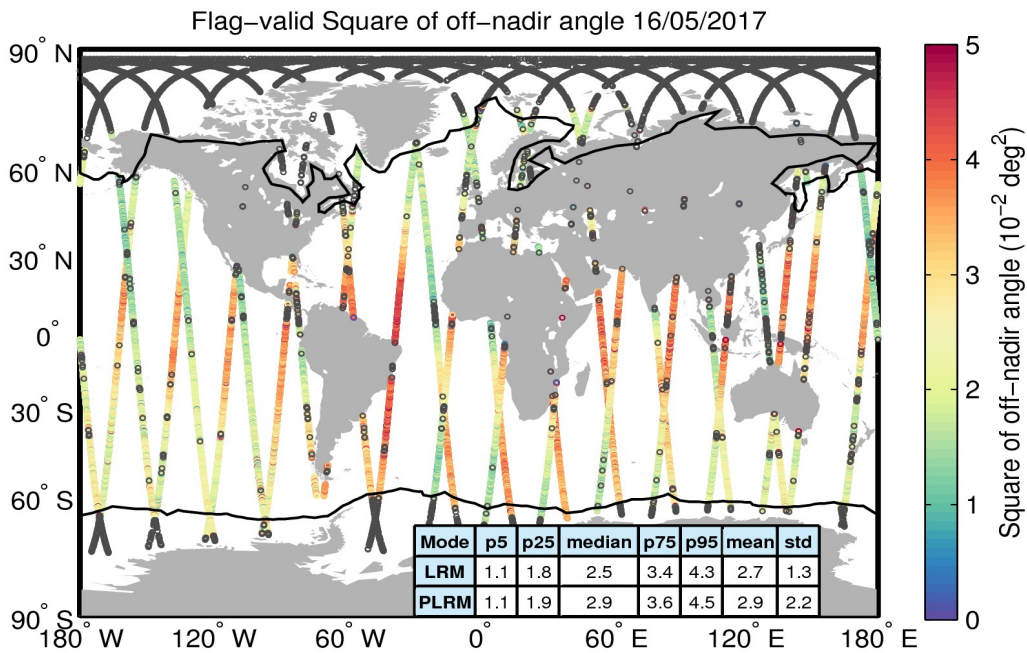
Figure 37. Geographical distribution of flag-valid mispointing data over oceans and lakes for 16/05/2017. The statistical values shown in the table refer to the mispointing in 10^{-2} deg 2 and are calculated separately for LRM and PLRM regions. Measurements taken over polar polygons have been excluded from the computation of the statistical values. The black lines mark the outer limit of the Arctic and Antarctic polar polygons. Gray circles denote negative values.
