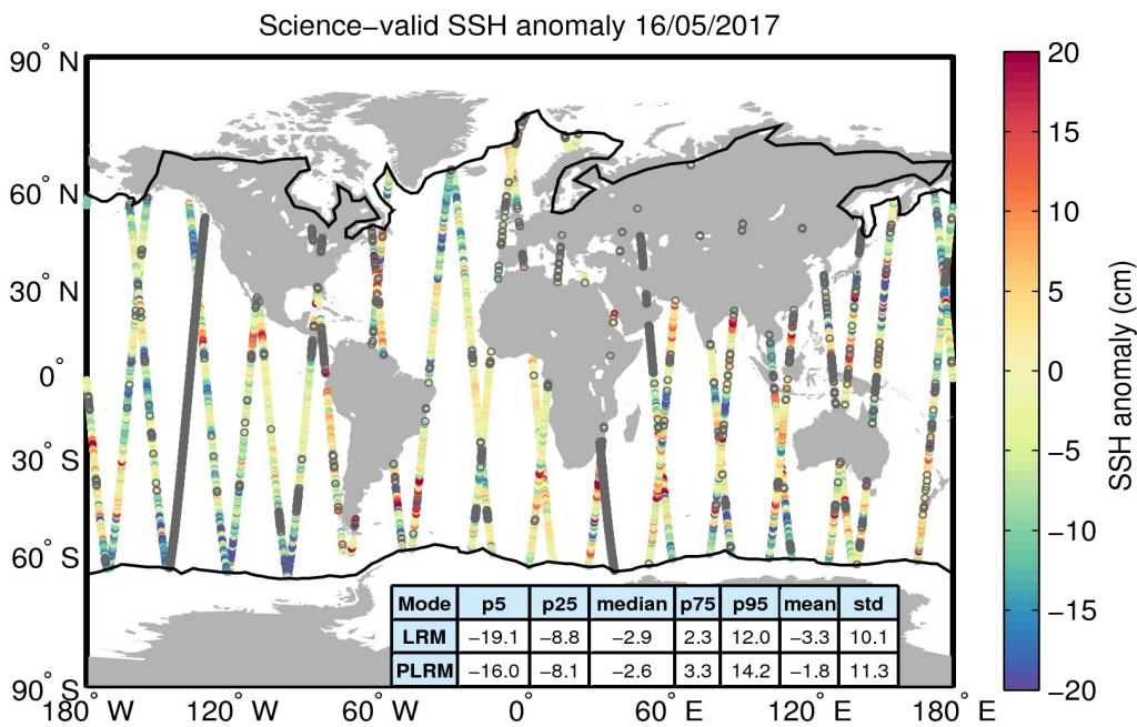
Figure 10. Geographical distribution of science-valid SSH anomaly data over oceans and lakes for 16/05/2017. The statistical values shown in the table refer to the SSH anomaly in cm and are calculated separately for LRM and PLRM regions. The black lines mark the outer limit of the Arctic and Antarctic polar polygons. Gray circles denote records that have been rejected based on the editing criteria described in Table 2.
