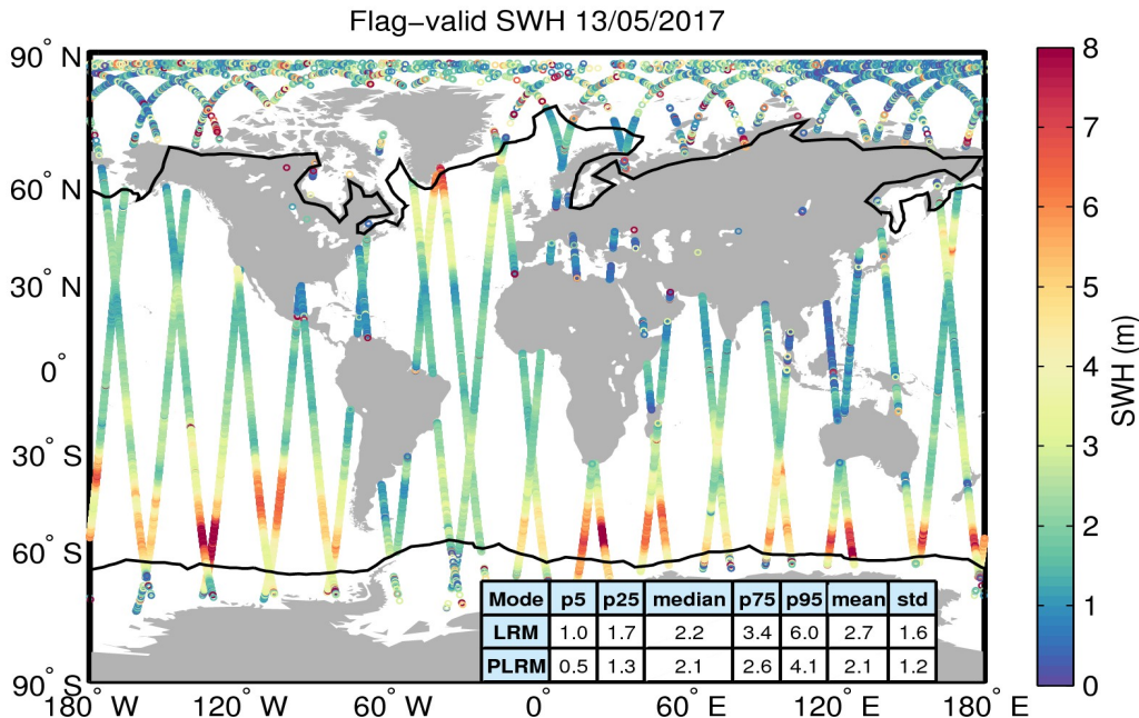
Figure 15. Geographical distribution of flag-valid SWH data over oceans and lakes for 13/05/2017. The statistical values shown in the table refer to the SWH in m and are calculated separately for LRM and PLRM regions. Measurements taken over polar polygons have been excluded from the computation of the statistical values. The black lines mark the outer limit of the Arctic and Antarctic polar polygons.
