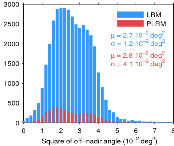
Figure 39. Histogram of flag-valid mispointing over oceans and lakes for LRM (blue) and PLRM (red) for 13/05/2017. Only positive values have been considered. The mean ( \mu ) and standard deviation ( \sigma ) are also shown. Note that values larger than 8 \cdot 10^{-2} \text{ deg}^2 are excluded from the histogram for the sake of readability but not from the computation of \mu and \sigma .
