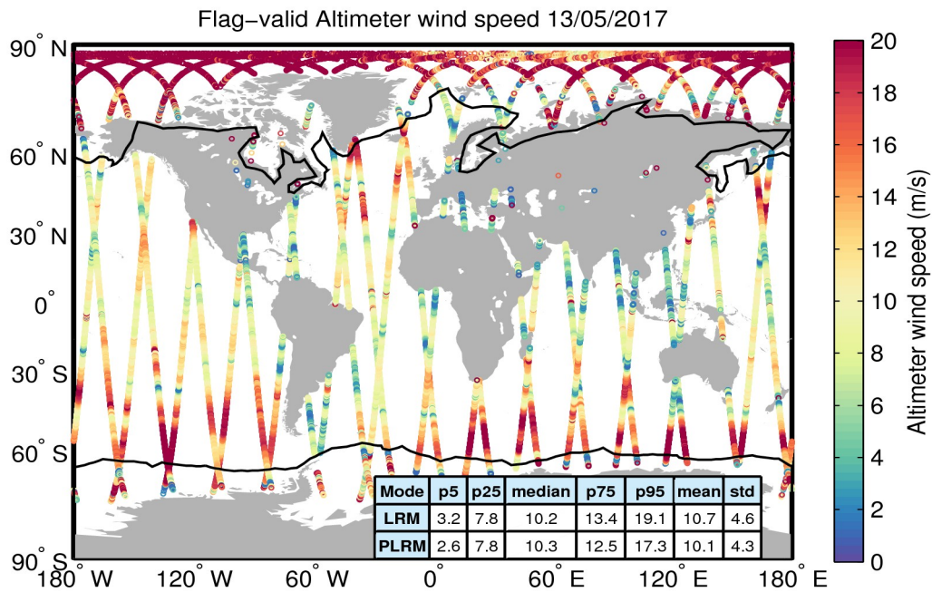
Figure 31. Geographical distribution of flag-valid wind data over oceans and lakes for 13/05/2017. The statistical values shown in the table refer to the wind in m/s and are calculated separately for LRM and PLRM regions. Measurements taken over polar polygons have been excluded from the computation of the statistical values. The black lines mark the outer limit of the Arctic and Antarctic polar polygons.
