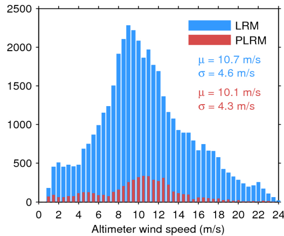
Figure 33. Histogram of flag-valid wind over oceans and lakes for LRM (blue) and PLRM (red) for 13/05/2017. The mean ( \mu ) and standard deviation ( \sigma ) are also shown. Note that values larger than 24 m/s are excluded from the histogram for the sake of readability but not from the computation of \mu and \sigma .
