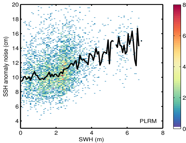
Figure 9. 2D histogram showing flag-valid SSH anomaly noise as a function of SWH for LRM (top) and PLRM (bottom) for 13/05/2017. The black line denotes the median SSH anomaly noise as a function of SWH.
