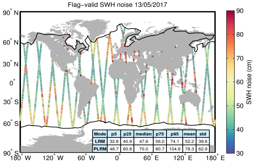
Figure 18. Geographical distribution of flag-valid 20-Hz SWH measurement noise over oceans and lakes for 13/05/2017. The statistical values shown in the table refer to the SWH noise and are calculated separately for LRM and PLRM regions. Measurements taken over polar polygons have been excluded from the computation of the statistical values. The black lines mark the outer limit of the Arctic and Antarctic polar polygons.
