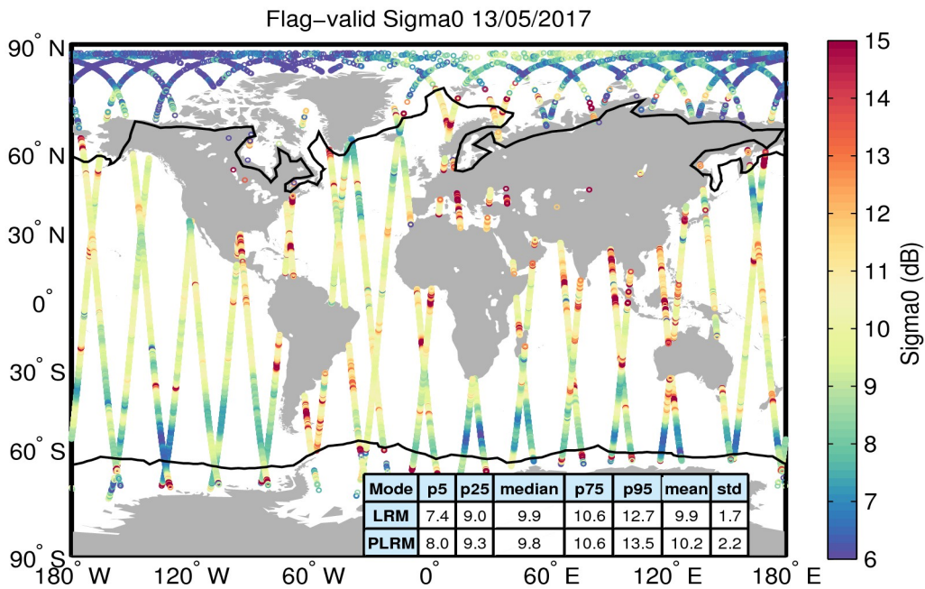
Figure 23. Geographical distribution of flag-valid sigma0 data over oceans and lakes for 13/05/2017. The statistical values shown in the table refer to the sigma0 in dB and are calculated separately for LRM and PLRM regions. Measurements taken over polar polygons have been excluded from the computation of the statistical values. The black lines mark the outer limit of the Arctic and Antarctic polar polygons.
