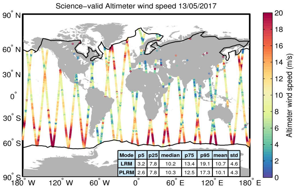
Figure 34. Geographical distribution of science-valid wind data over oceans and lakes for 13/05/2017. The statistical values shown in the table refer to the wind in m/s and are calculated separately for LRM and PLRM regions. The black lines mark the outer limit of the Arctic and Antarctic polar polygons. Gray circles denote records that have been rejected based on the editing criteria described in Table 5.
