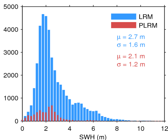
Figure 17. Histogram of flag-valid SWH over oceans and lakes for LRM (blue) and PLRM (red) for 13/05/2017. The mean ( \mu ) and standard deviation ( \sigma ) are also shown. Note that values larger than 12 m are excluded from the histogram for the sake of readability but not from the computation of \mu and \sigma .
