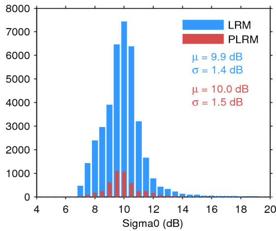
Figure 28. Histogram of science-valid sigma0 over oceans and lakes for LRM (blue) and PLRM (red) for 13/05/2017. The mean ( \mu ) and standard deviation ( \sigma ) are also shown. Note that values outside [4 20] dB are excluded from the histogram for the sake of readability but not from the computation of \mu and \sigma .
