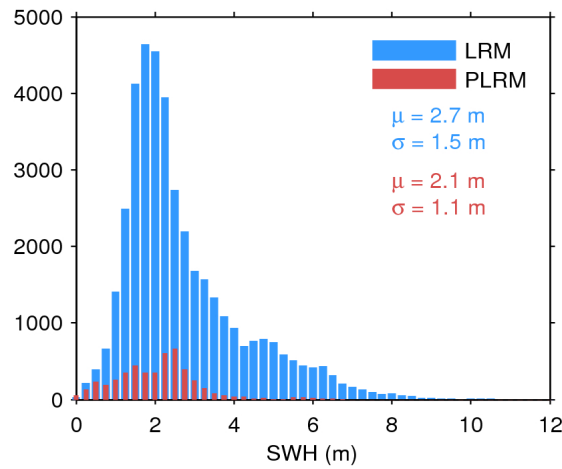
Figure 20. Histogram of science-valid SWH over oceans and lakes for LRM (blue) and PLRM (red) for 13/05/2017. The mean ( \mu ) and standard deviation ( \sigma ) are also shown. Note that values larger than 12 m are excluded from the histogram for the sake of readability but not from the computation of \mu and \sigma .
