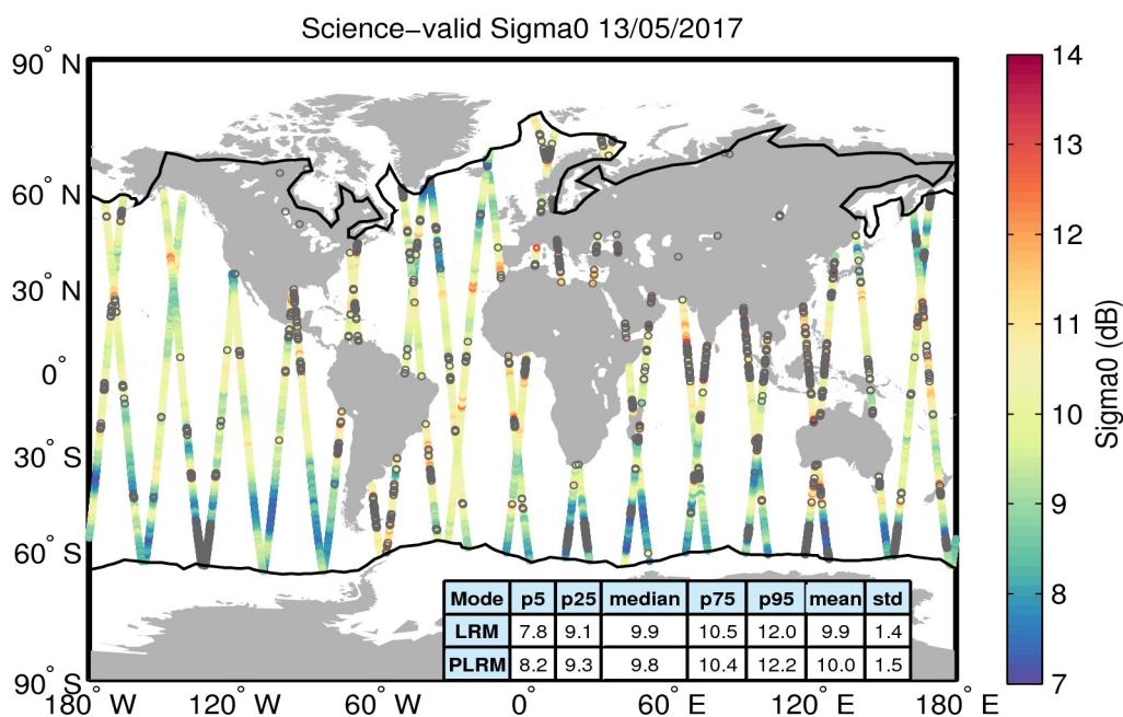
Figure 27. Geographical distribution of science-valid sigma0 data over oceans and lakes for 13/05/2017. The statistical values shown in the table refer to the sigma0 in dB and are calculated separately for LRM and PLRM regions. The black lines mark the outer limit of the Arctic and Antarctic polar polygons. Gray circles denote records that have been rejected based on the editing criteria described in Table 4.
