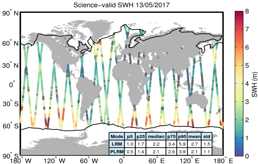
Figure 19. Geographical distribution of science-valid SWH data over oceans and lakes for 13/05/2017. The statistical values shown in the table refer to the SWH in m and are calculated separately for LRM and PLRM regions. The black lines mark the outer limit of the Arctic and Antarctic polar polygons. Gray circles denote records that have been rejected based on the editing criteria described in Table 3.
