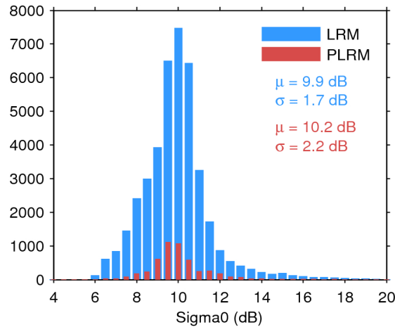
Figure 25. Histogram of flag-valid sigma0 over oceans and lakes for LRM (blue) and PLRM (red) for 13/05/2017. The mean ( \mu ) and standard deviation ( \sigma ) are also shown. Note that values outside [4 20] dB are excluded from the histogram for the sake of readability but not from the computation of \mu and \sigma .
