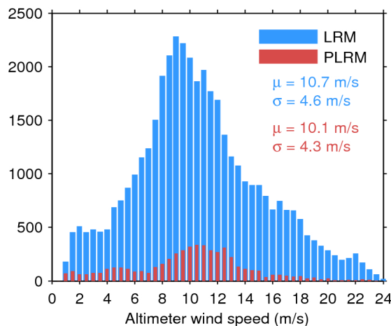
Figure 35. Histogram of science-valid wind over oceans and lakes for LRM (blue) and PLRM (red) for 13/05/2017. The mean ( \mu ) and standard deviation ( \sigma ) are also shown. Note that values larger than 24 m/s are excluded from the histogram for the sake of readability but not from the computation of \mu and \sigma .
