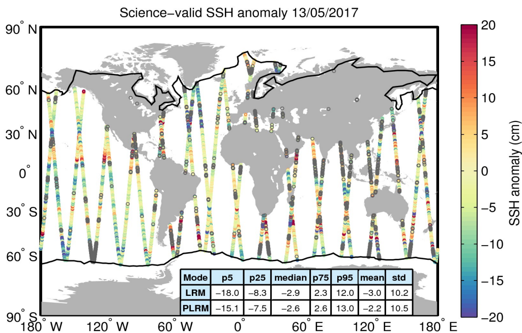
Figure 10. Geographical distribution of science-valid SSH anomaly data over oceans and lakes for 13/05/2017. The statistical values shown in the table refer to the SSH anomaly in cm and are calculated separately for LRM and PLRM regions. The black lines mark the outer limit of the Arctic and Antarctic polar polygons. Gray circles denote records that have been rejected based on the editing criteria described in Table 2.
