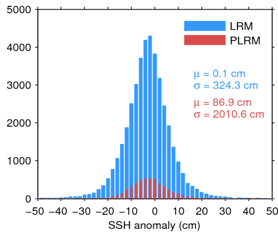
Figure 7. Histogram of flag-valid SSH anomaly over oceans and lakes for LRM (blue) and PLRM (red) for 13/05/2017. The mean ( \mu ) and standard deviation ( \sigma ) are also shown. Note that values outside [-50\ 50] cm are excluded from the histogram for the sake of readability but not from the computation of \mu and \sigma .
