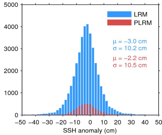
Figure 11. Histogram of science-valid SSH anomaly over oceans and lakes for LRM (blue) and PLRM (red) for 13/05/2017. The mean ( \mu ) and standard deviation ( \sigma ) are also shown. Note that values outside [-50\ 50] cm are excluded from the histogram for the sake of readability but not from the computation of \mu and \sigma .
