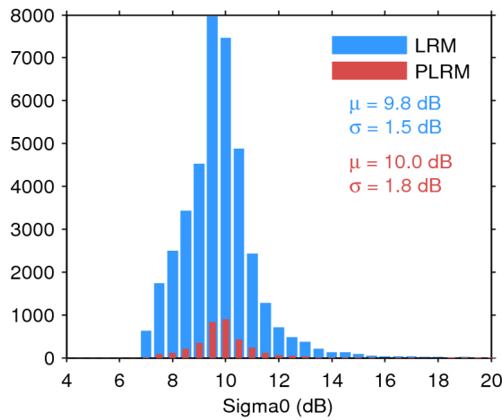
Figure 28. Histogram of science-valid sigma0 over oceans and lakes for LRM (blue) and PLRM (red) for 12/05/2017. The mean ( \mu ) and standard deviation ( \sigma ) are also shown. Note that values outside [4 20] dB are excluded from the histogram for the sake of readability but not from the computation of \mu and \sigma .
