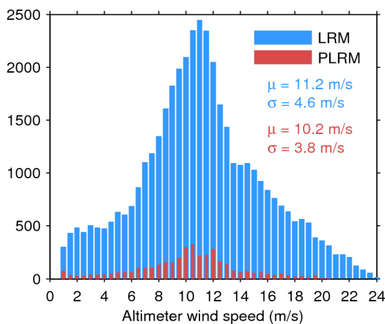
Figure 33. Histogram of flag-valid wind over oceans and lakes for LRM (blue) and PLRM (red) for 12/05/2017. The mean ( \mu ) and standard deviation ( \sigma ) are also shown. Note that values larger than 24 m/s are excluded from the histogram for the sake of readability but not from the computation of \mu and \sigma .
