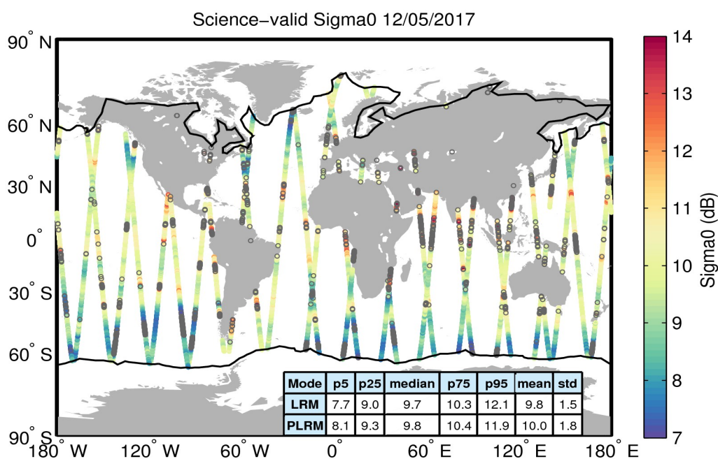
Figure 27. Geographical distribution of science-valid sigma0 data over oceans and lakes for 12/05/2017. The statistical values shown in the table refer to the sigma0 in dB and are calculated separately for LRM and PLRM regions. The black lines mark the outer limit of the Arctic and Antarctic polar polygons. Gray circles denote records that have been rejected based on the editing criteria described in Table 4.
