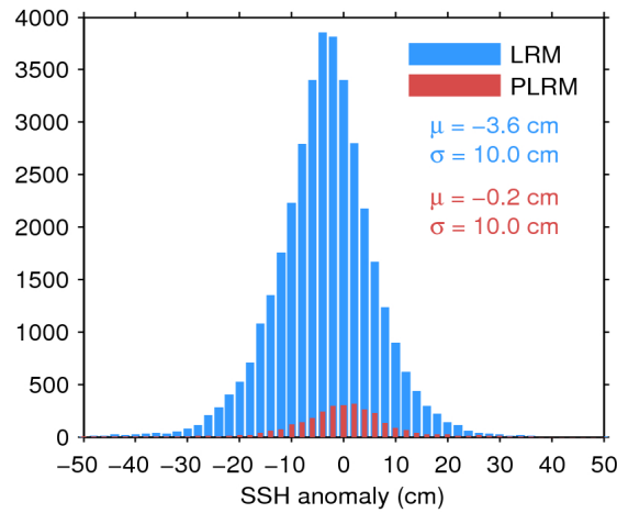
Figure 11. Histogram of science-valid SSH anomaly over oceans and lakes for LRM (blue) and PLRM (red) for 12/05/2017. The mean ( \mu ) and standard deviation ( \sigma ) are also shown. Note that values outside [-50 50] cm are excluded from the histogram for the sake of readability but not from the computation of \mu and \sigma .
