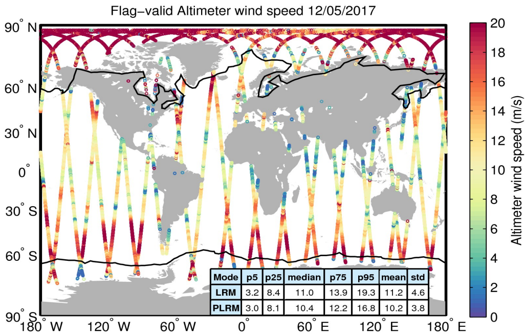
Figure 31. Geographical distribution of flag-valid wind data over oceans and lakes for 12/05/2017. The statistical values shown in the table refer to the wind in m/s and are calculated separately for LRM and PLRM regions. Measurements taken over polar polygons have been excluded from the computation of the statistical values. The black lines mark the outer limit of the Arctic and Antarctic polar polygons.
