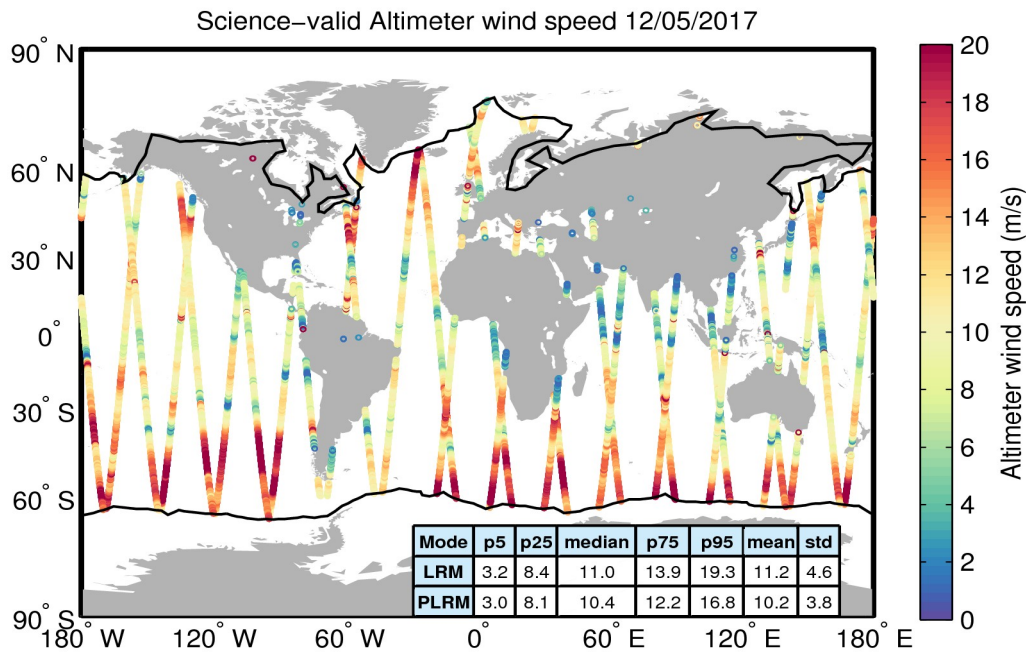
Figure 34. Geographical distribution of science-valid wind data over oceans and lakes for 12/05/2017. The statistical values shown in the table refer to the wind in m/s and are calculated separately for LRM and PLRM regions. The black lines mark the outer limit of the Arctic and Antarctic polar polygons. Gray circles denote records that have been rejected based on the editing criteria described in Table 5.
