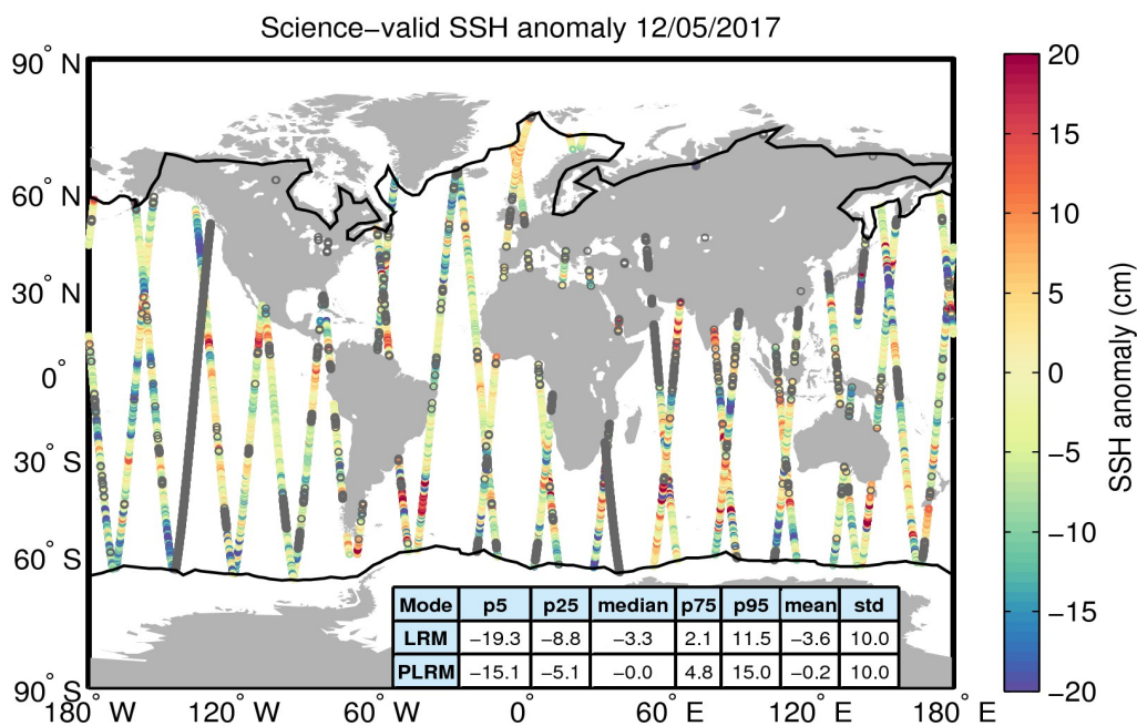
Figure 10. Geographical distribution of science-valid SSH anomaly data over oceans and lakes for 12/05/2017. The statistical values shown in the table refer to the SSH anomaly in cm and are calculated separately for LRM and PLRM regions. The black lines mark the outer limit of the Arctic and Antarctic polar polygons. Gray circles denote records that have been rejected based on the editing criteria described in Table 2.
