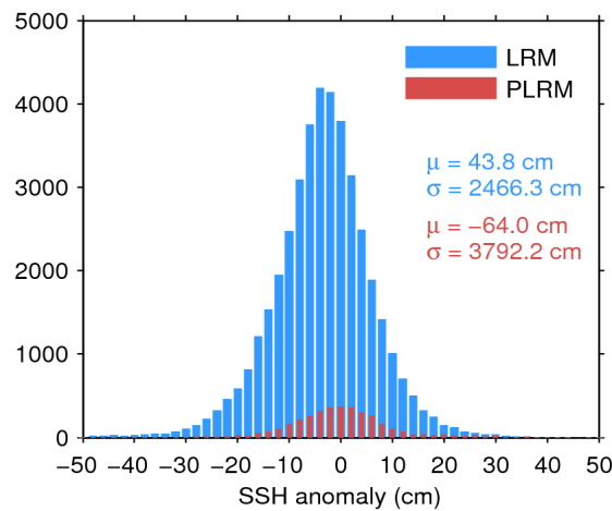
Figure 7. Histogram of flag-valid SSH anomaly over oceans and lakes for LRM (blue) and PLRM (red) for 12/05/2017. The mean ( \mu ) and standard deviation ( \sigma ) are also shown. Note that values outside [-50\ 50] cm are excluded from the histogram for the sake of readability but not from the computation of \mu and \sigma .
