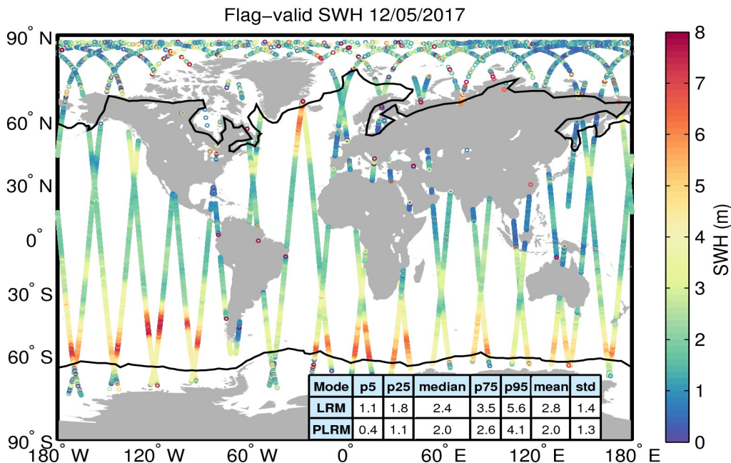
Figure 15. Geographical distribution of flag-valid SWH data over oceans and lakes for 12/05/2017. The statistical values shown in the table refer to the SWH in m and are calculated separately for LRM and PLRM regions. Measurements taken over polar polygons have been excluded from the computation of the statistical values. The black lines mark the outer limit of the Arctic and Antarctic polar polygons.
