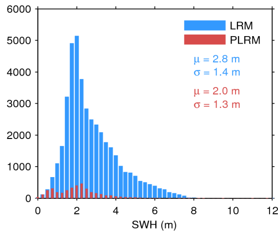
Figure 17. Histogram of flag-valid SWH over oceans and lakes for LRM (blue) and PLRM (red) for 12/05/2017. The mean ( \mu ) and standard deviation ( \sigma ) are also shown. Note that values larger than 12 m are excluded from the histogram for the sake of readability but not from the computation of \mu and \sigma .
