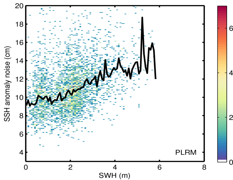
Figure 9. 2D histogram showing flag-valid SSH anomaly noise as a function of SWH for LRM (top) and PLRM (bottom) for 12/05/2017. The black line denotes the median SSH anomaly noise as a function of SWH.
