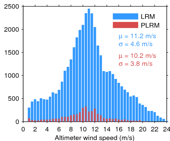
Figure 35. Histogram of science-valid wind over oceans and lakes for LRM (blue) and PLRM (red) for 12/05/2017. The mean ( \mu ) and standard deviation ( \sigma ) are also shown. Note that values larger than 24 m/s are excluded from the histogram for the sake of readability but not from the computation of \mu and \sigma .
