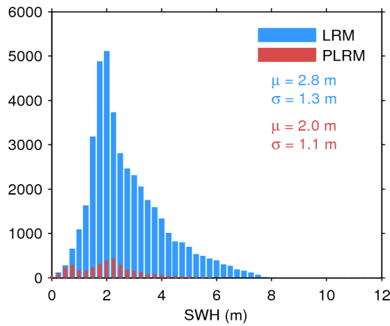
Figure 20. Histogram of science-valid SWH over oceans and lakes for LRM (blue) and PLRM (red) for 12/05/2017. The mean ( \mu ) and standard deviation ( \sigma ) are also shown. Note that values larger than 12 m are excluded from the histogram for the sake of readability but not from the computation of \mu and \sigma .
