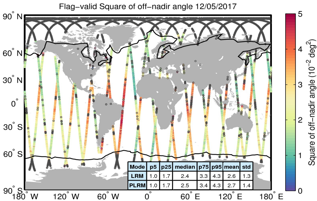
Figure 37. Geographical distribution of flag-valid mispointing data over oceans and lakes for 12/05/2017. The statistical values shown in the table refer to the mispointing in 10^{-2} \text{ deg}^2 and are calculated separately for LRM and PLRM regions. Measurements taken over polar polygons have been excluded from the computation of the statistical values. The black lines mark the outer limit of the Arctic and Antarctic polar polygons. Gray circles denote negative values.
