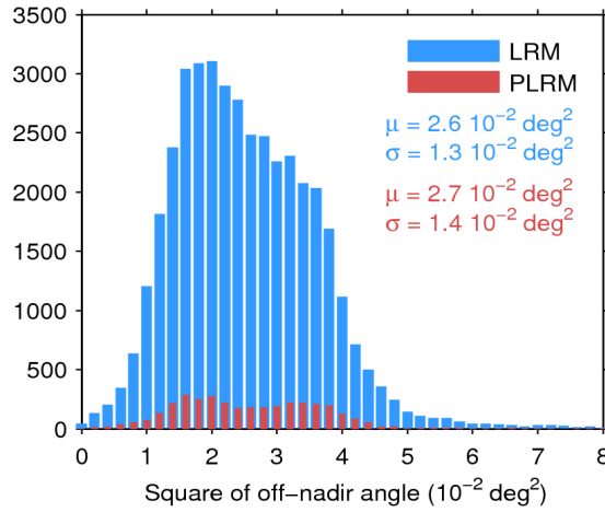
Figure 39. Histogram of flag-valid mispointing over oceans and lakes for LRM (blue) and PLRM (red) for 12/05/2017. Only positive values have been considered. The mean ( \mu ) and standard deviation ( \sigma ) are also shown. Note that values larger than 8 \cdot 10^{-2} \text{ deg}^2 are excluded from the histogram for the sake of readability but not from the computation of \mu and \sigma .
