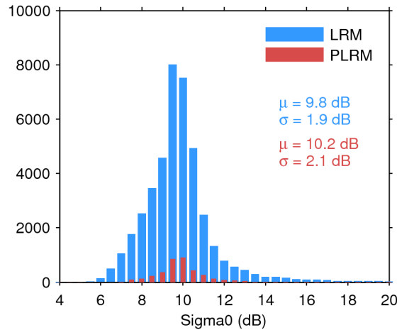
Figure 25. Histogram of flag-valid sigma0 over oceans and lakes for LRM (blue) and PLRM (red) for 12/05/2017. The mean ( \mu ) and standard deviation ( \sigma ) are also shown. Note that values outside [4 20] dB are excluded from the histogram for the sake of readability but not from the computation of \mu and \sigma .
