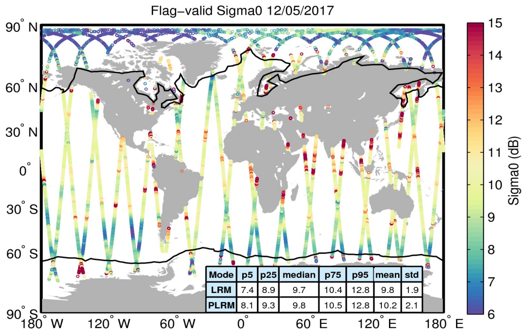
Figure 23. Geographical distribution of flag-valid sigma0 data over oceans and lakes for 12/05/2017. The statistical values shown in the table refer to the sigma0 in dB and are calculated separately for LRM and PLRM regions. Measurements taken over polar polygons have been excluded from the computation of the statistical values. The black lines mark the outer limit of the Arctic and Antarctic polar polygons.
