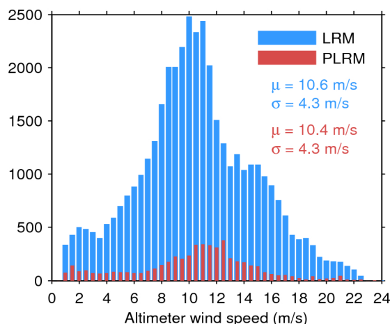
Figure 33. Histogram of flag-valid wind over oceans and lakes for LRM (blue) and PLRM (red) for 11/05/2017. The mean ( \mu ) and standard deviation ( \sigma ) are also shown. Note that values larger than 24 m/s are excluded from the histogram for the sake of readability but not from the computation of \mu and \sigma .
