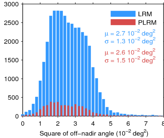
Figure 39. Histogram of flag-valid mispointing over oceans and lakes for LRM (blue) and PLRM (red) for 11/05/2017. Only positive values have been considered. The mean ( \mu ) and standard deviation ( \sigma ) are also shown. Note that values larger than 8 \cdot 10^{-2} \text{ deg}^2 are excluded from the histogram for the sake of readability but not from the computation of \mu and \sigma .
