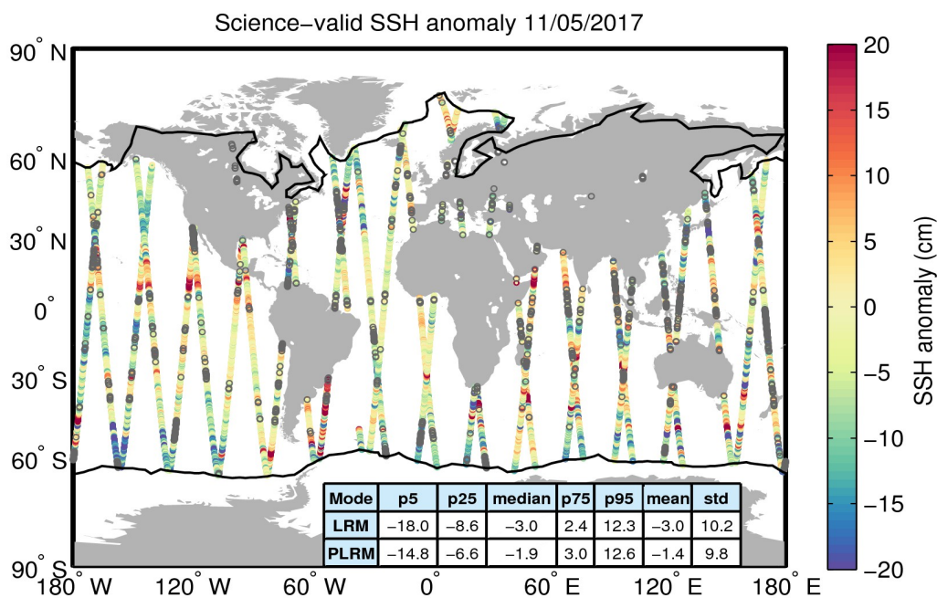
Figure 10. Geographical distribution of science-valid SSH anomaly data over oceans and lakes for 11/05/2017. The statistical values shown in the table refer to the SSH anomaly in cm and are calculated separately for LRM and PLRM regions. The black lines mark the outer limit of the Arctic and Antarctic polar polygons. Gray circles denote records that have been rejected based on the editing criteria described in Table 2.
