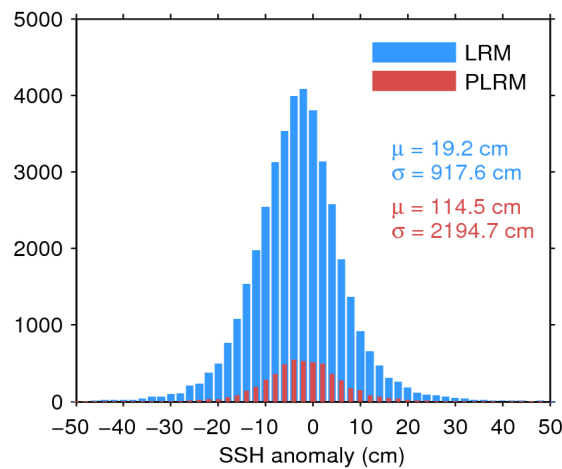
Figure 7. Histogram of flag-valid SSH anomaly over oceans and lakes for LRM (blue) and PLRM (red) for 11/05/2017. The mean ( \mu ) and standard deviation ( \sigma ) are also shown. Note that values outside [-50 50] cm are excluded from the histogram for the sake of readability but not from the computation of \mu and \sigma .
