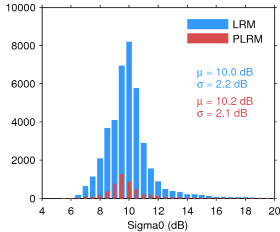
Figure 25. Histogram of flag-valid sigma0 over oceans and lakes for LRM (blue) and PLRM (red) for 11/05/2017. The mean ( \mu ) and standard deviation ( \sigma ) are also shown. Note that values outside [4 20] dB are excluded from the histogram for the sake of readability but not from the computation of \mu and \sigma .
