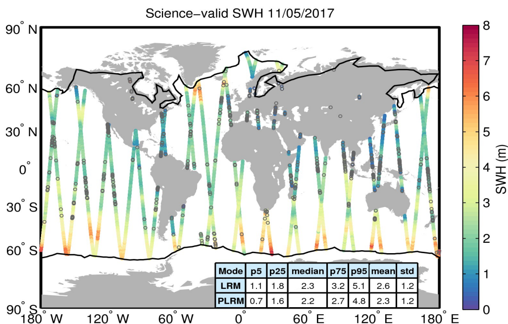
Figure 19. Geographical distribution of science-valid SWH data over oceans and lakes for 11/05/2017. The statistical values shown in the table refer to the SWH in m and are calculated separately for LRM and PLRM regions. The black lines mark the outer limit of the Arctic and Antarctic polar polygons. Gray circles denote records that have been rejected based on the editing criteria described in Table 3.
