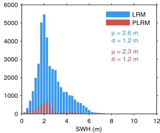
Figure 20. Histogram of science-valid SWH over oceans and lakes for LRM (blue) and PLRM (red) for 11/05/2017. The mean ( \mu ) and standard deviation ( \sigma ) are also shown. Note that values larger than 12 m are excluded from the histogram for the sake of readability but not from the computation of \mu and \sigma .
