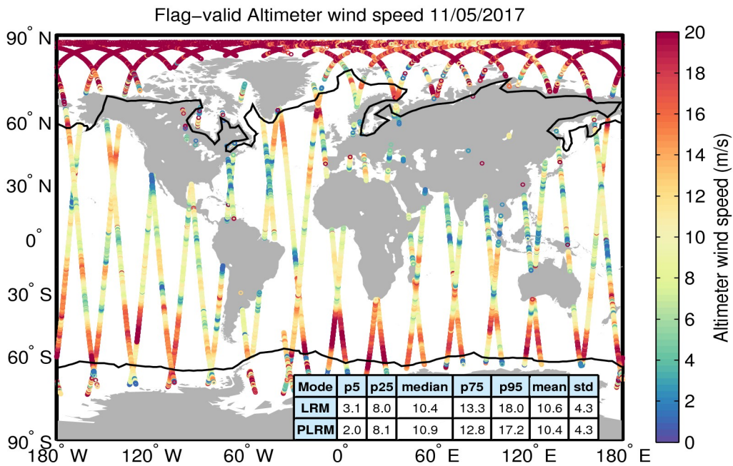
Figure 31. Geographical distribution of flag-valid wind data over oceans and lakes for 11/05/2017. The statistical values shown in the table refer to the wind in m/s and are calculated separately for LRM and PLRM regions. Measurements taken over polar polygons have been excluded from the computation of the statistical values. The black lines mark the outer limit of the Arctic and Antarctic polar polygons.
