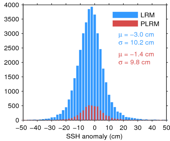
Figure 11. Histogram of science-valid SSH anomaly over oceans and lakes for LRM (blue) and PLRM (red) for 11/05/2017. The mean ( \mu ) and standard deviation ( \sigma ) are also shown. Note that values outside [-50 50] cm are excluded from the histogram for the sake of readability but not from the computation of \mu and \sigma .
