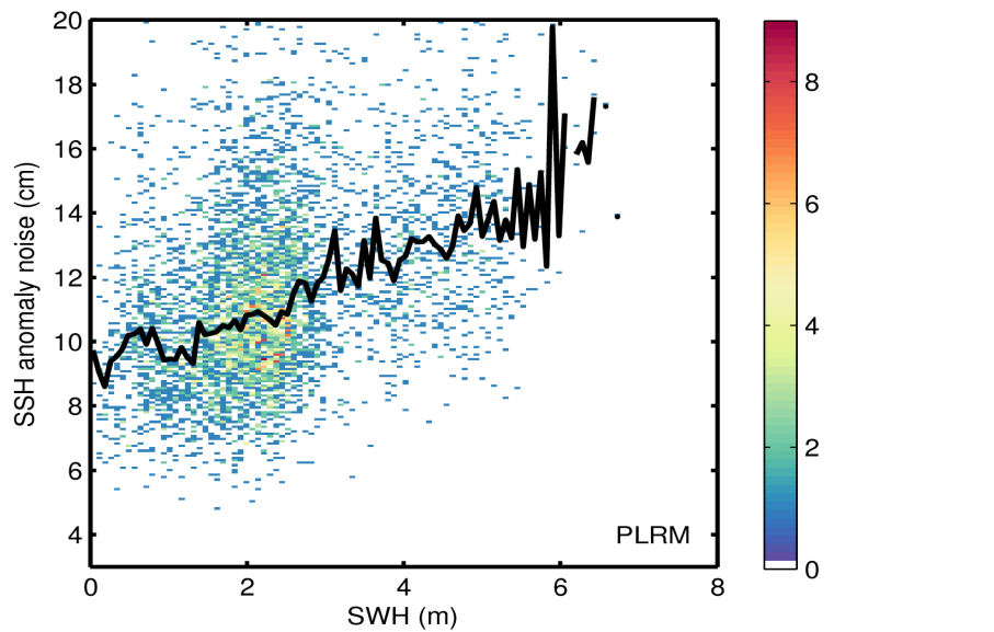
Figure 9. 2D histogram showing flag-valid SSH anomaly noise as a function of SWH for LRM (top) and PLRM (bottom) for 11/05/2017. The black line denotes the median SSH anomaly noise as a function of SWH.
