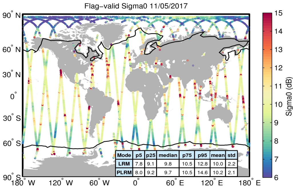
Figure 23. Geographical distribution of flag-valid sigma0 data over oceans and lakes for 11/05/2017. The statistical values shown in the table refer to the sigma0 in dB and are calculated separately for LRM and PLRM regions. Measurements taken over polar polygons have been excluded from the computation of the statistical values. The black lines mark the outer limit of the Arctic and Antarctic polar polygons.
