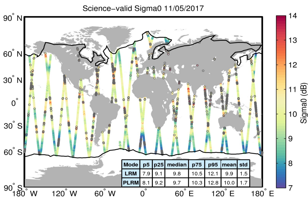
Figure 27. Geographical distribution of science-valid sigma0 data over oceans and lakes for 11/05/2017. The statistical values shown in the table refer to the sigma0 in dB and are calculated separately for LRM and PLRM regions. The black lines mark the outer limit of the Arctic and Antarctic polar polygons. Gray circles denote records that have been rejected based on the editing criteria described in Table 4.
