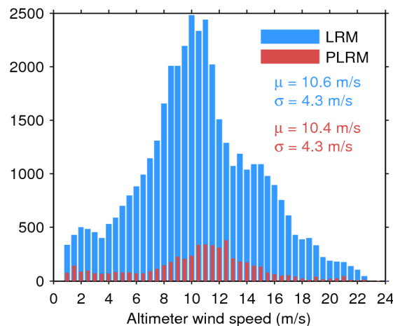
Figure 35. Histogram of science-valid wind over oceans and lakes for LRM (blue) and PLRM (red) for 11/05/2017. The mean ( \mu ) and standard deviation ( \sigma ) are also shown. Note that values larger than 24 m/s are excluded from the histogram for the sake of readability but not from the computation of \mu and \sigma .
