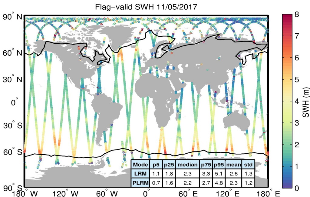
Figure 15. Geographical distribution of flag-valid SWH data over oceans and lakes for 11/05/2017. The statistical values shown in the table refer to the SWH in m and are calculated separately for LRM and PLRM regions. Measurements taken over polar polygons have been excluded from the computation of the statistical values. The black lines mark the outer limit of the Arctic and Antarctic polar polygons.
