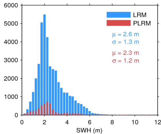
Figure 17. Histogram of flag-valid SWH over oceans and lakes for LRM (blue) and PLRM (red) for 11/05/2017. The mean ( \mu ) and standard deviation ( \sigma ) are also shown. Note that values larger than 12 m are excluded from the histogram for the sake of readability but not from the computation of \mu and \sigma .
