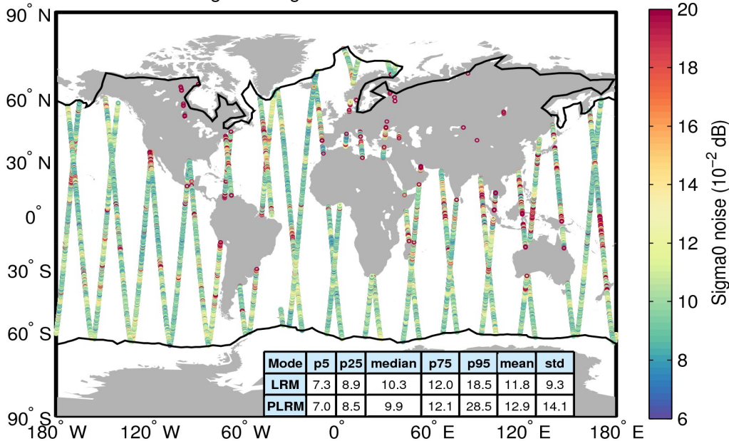
Flag-valid sigma0 noise 11/05/2017
