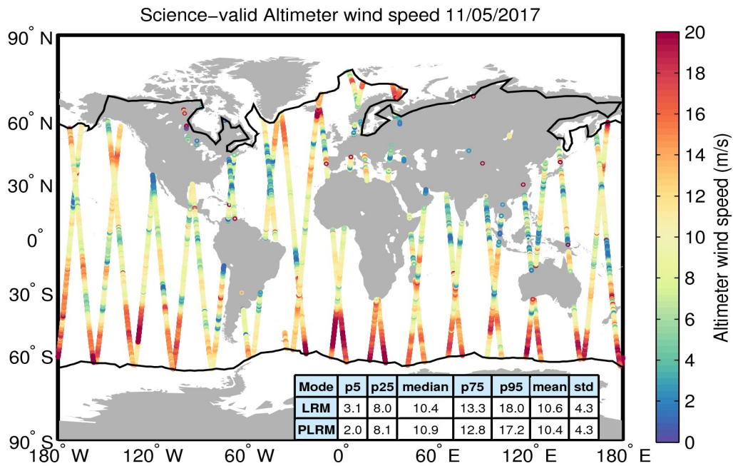
Figure 34. Geographical distribution of science-valid wind data over oceans and lakes for 11/05/2017. The statistical values shown in the table refer to the wind in m/s and are calculated separately for LRM and PLRM regions. The black lines mark the outer limit of the Arctic and Antarctic polar polygons. Gray circles denote records that have been rejected based on the editing criteria described in Table 5.
