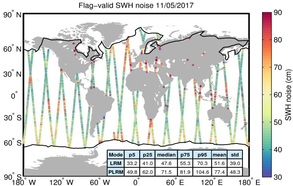
Figure 18. Geographical distribution of flag-valid 20-Hz SWH measurement noise over oceans and lakes for 11/05/2017. The statistical values shown in the table refer to the SWH noise and are calculated separately for LRM and PLRM regions. Measurements taken over polar polygons have been excluded from the computation of the statistical values. The black lines mark the outer limit of the Arctic and Antarctic polar polygons.
