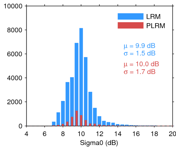
Figure 28. Histogram of science-valid sigma0 over oceans and lakes for LRM (blue) and PLRM (red) for 11/05/2017. The mean ( \mu ) and standard deviation ( \sigma ) are also shown. Note that values outside [4 20] dB are excluded from the histogram for the sake of readability but not from the computation of \mu and \sigma .
