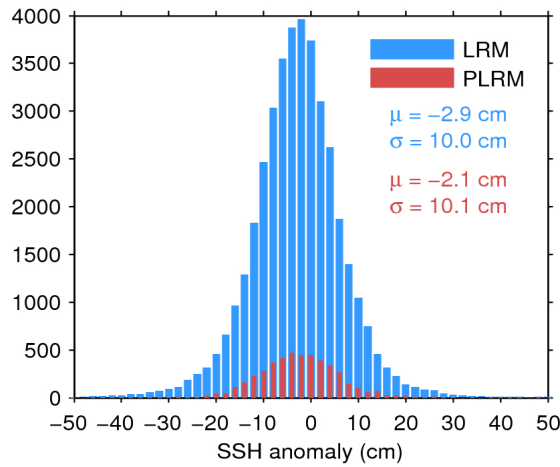
Figure 11. Histogram of science-valid SSH anomaly over oceans and lakes for LRM (blue) and PLRM (red) for 09/05/2017. The mean ( \mu ) and standard deviation ( \sigma ) are also shown. Note that values outside [-50\ 50] cm are excluded from the histogram for the sake of readability but not from the computation of \mu and \sigma .
