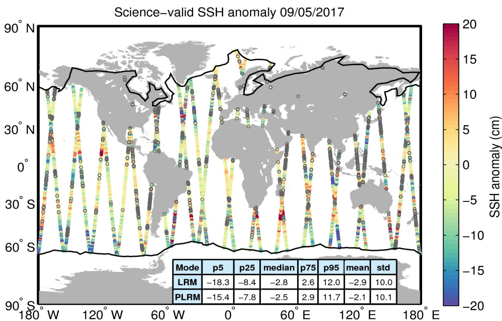
Figure 10. Geographical distribution of science-valid SSH anomaly data over oceans and lakes for 09/05/2017. The statistical values shown in the table refer to the SSH anomaly in cm and are calculated separately for LRM and PLRM regions. The black lines mark the outer limit of the Arctic and Antarctic polar polygons. Gray circles denote records that have been rejected based on the editing criteria described in Table 2.
