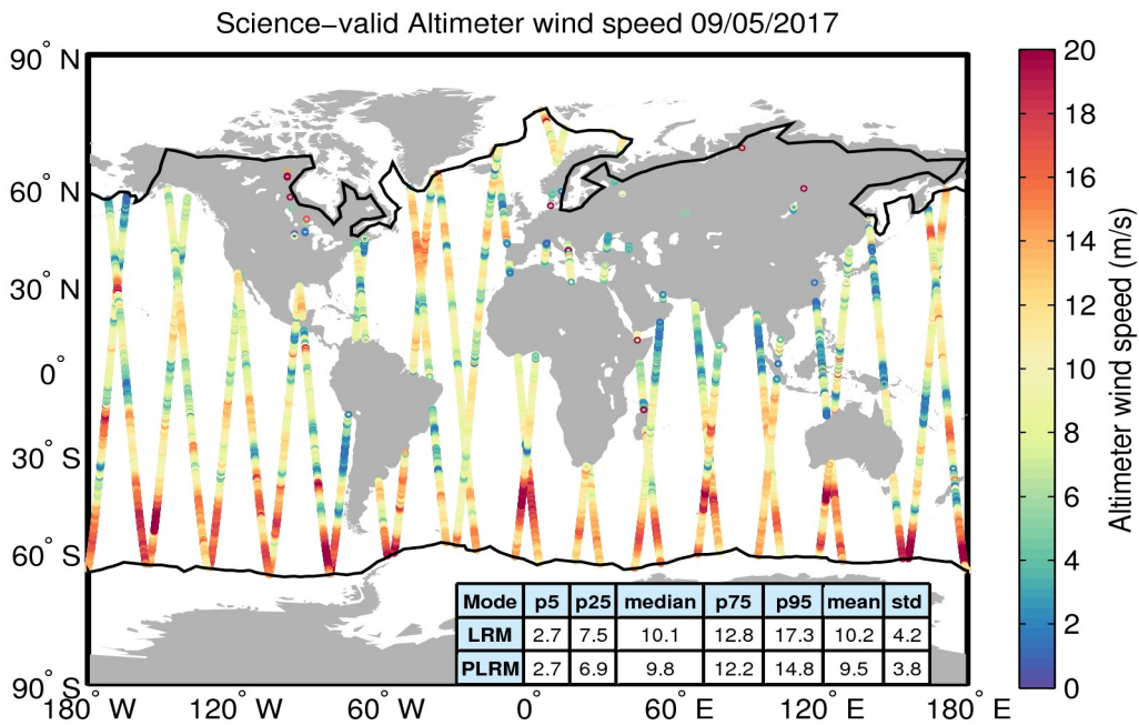
Figure 34. Geographical distribution of science-valid wind data over oceans and lakes for 09/05/2017. The statistical values shown in the table refer to the wind in m/s and are calculated separately for LRM and PLRM regions. The black lines mark the outer limit of the Arctic and Antarctic polar polygons. Gray circles denote records that have been rejected based on the editing criteria described in Table 5.
