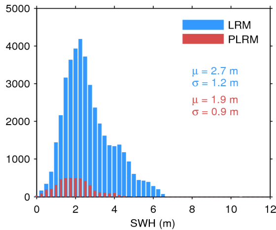
Figure 20. Histogram of science-valid SWH over oceans and lakes for LRM (blue) and PLRM (red) for 09/05/2017. The mean ( \mu ) and standard deviation ( \sigma ) are also shown. Note that values larger than 12 m are excluded from the histogram for the sake of readability but not from the computation of \mu and \sigma .
