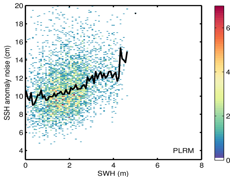
Figure 9. 2D histogram showing flag-valid SSH anomaly noise as a function of SWH for LRM (top) and PLRM (bottom) for 09/05/2017. The black line denotes the median SSH anomaly noise as a function of SWH.
