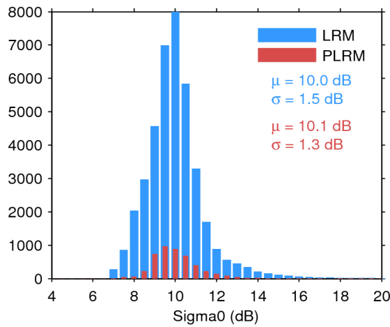
Figure 28. Histogram of science-valid sigma0 over oceans and lakes for LRM (blue) and PLRM (red) for 09/05/2017. The mean ( \mu ) and standard deviation ( \sigma ) are also shown. Note that values outside [4 20] dB are excluded from the histogram for the sake of readability but not from the computation of \mu and \sigma .
