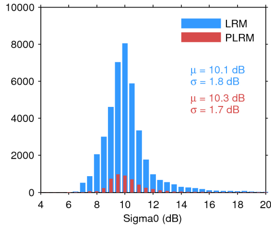
Figure 25. Histogram of flag-valid sigma0 over oceans and lakes for LRM (blue) and PLRM (red) for 09/05/2017. The mean ( \mu ) and standard deviation ( \sigma ) are also shown. Note that values outside [4 20] dB are excluded from the histogram for the sake of readability but not from the computation of \mu and \sigma .
