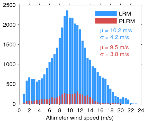
Figure 35. Histogram of science-valid wind over oceans and lakes for LRM (blue) and PLRM (red) for 09/05/2017. The mean ( \mu ) and standard deviation ( \sigma ) are also shown. Note that values larger than 24 m/s are excluded from the histogram for the sake of readability but not from the computation of \mu and \sigma .
