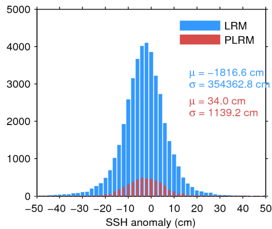
Figure 7. Histogram of flag-valid SSH anomaly over oceans and lakes for LRM (blue) and PLRM (red) for 09/05/2017. The mean ( \mu ) and standard deviation ( \sigma ) are also shown. Note that values outside [-50\ 50] cm are excluded from the histogram for the sake of readability but not from the computation of \mu and \sigma .
