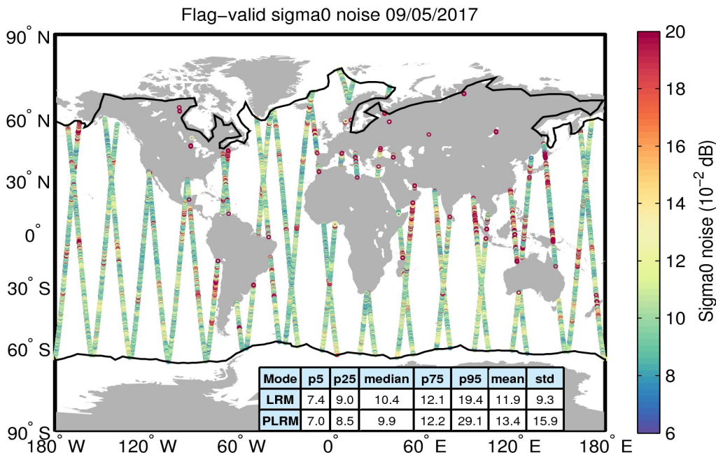
Figure 26. Geographical distribution of flag-valid 20-Hz sigma0 measurement noise over oceans and lakes for 09/05/2017. The statistical values shown in the table refer to the sigma0 noise and are calculated separately for LRM and PLRM regions. Measurements taken over polar polygons have been excluded from the computation of the statistical values. The black lines mark the outer limit of the Arctic and Antarctic polar polygons.
