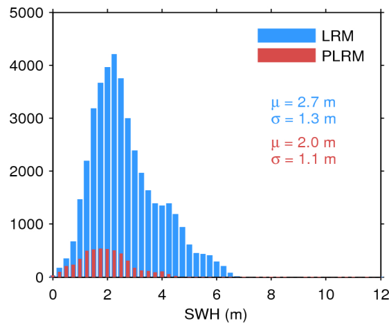
Figure 17. Histogram of flag-valid SWH over oceans and lakes for LRM (blue) and PLRM (red) for 09/05/2017. The mean ( \mu ) and standard deviation ( \sigma ) are also shown. Note that values larger than 12 m are excluded from the histogram for the sake of readability but not from the computation of \mu and \sigma .
