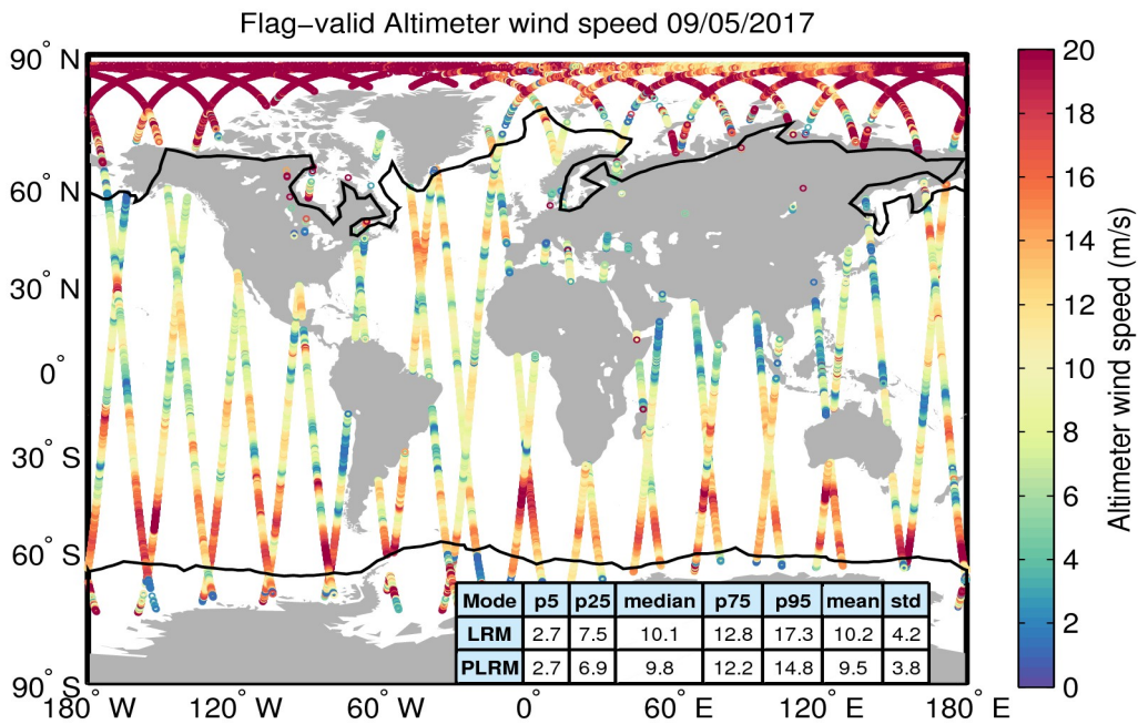
Figure 31. Geographical distribution of flag-valid wind data over oceans and lakes for 09/05/2017. The statistical values shown in the table refer to the wind in m/s and are calculated separately for LRM and PLRM regions. Measurements taken over polar polygons have been excluded from the computation of the statistical values. The black lines mark the outer limit of the Arctic and Antarctic polar polygons.
