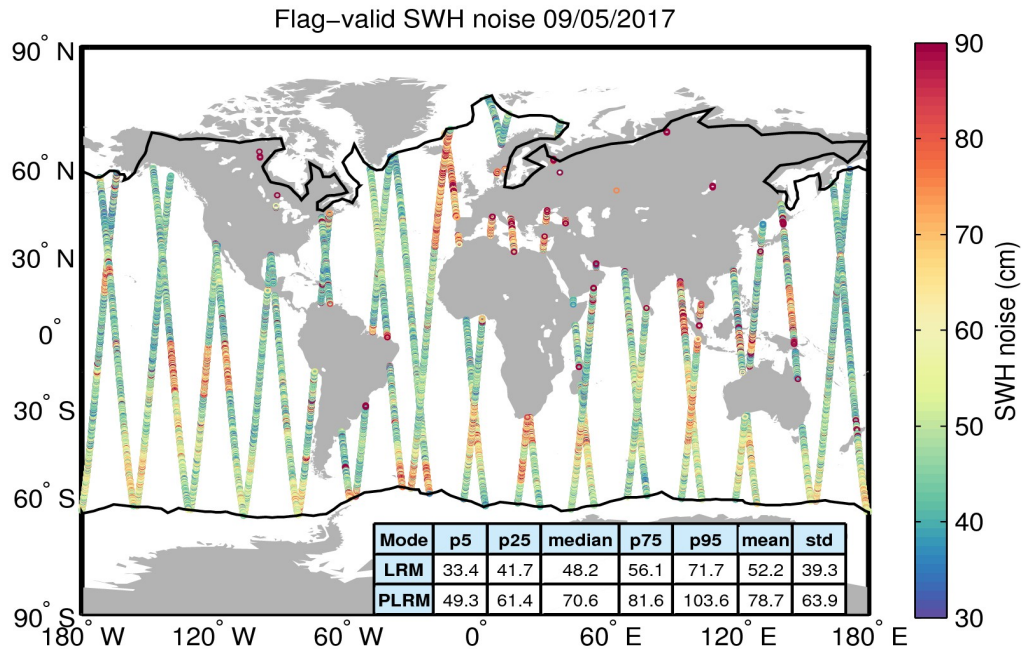
Figure 18. Geographical distribution of flag-valid 20-Hz SWH measurement noise over oceans and lakes for 09/05/2017. The statistical values shown in the table refer to the SWH noise and are calculated separately for LRM and PLRM regions. Measurements taken over polar polygons have been excluded from the computation of the statistical values. The black lines mark the outer limit of the Arctic and Antarctic polar polygons.
