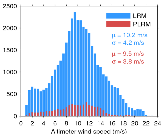
Figure 33. Histogram of flag-valid wind over oceans and lakes for LRM (blue) and PLRM (red) for 09/05/2017. The mean ( \mu ) and standard deviation ( \sigma ) are also shown. Note that values larger than 24 m/s are excluded from the histogram for the sake of readability but not from the computation of \mu and \sigma .
