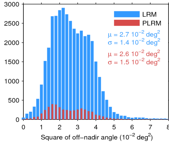
Figure 39. Histogram of flag-valid mispointing over oceans and lakes for LRM (blue) and PLRM (red) for 09/05/2017. Only positive values have been considered. The mean ( \mu ) and standard deviation ( \sigma ) are also shown. Note that values larger than 8 \cdot 10^{-2} \text{ deg}^2 are excluded from the histogram for the sake of readability but not from the computation of \mu and \sigma .
