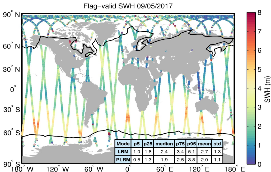
Figure 15. Geographical distribution of flag-valid SWH data over oceans and lakes for 09/05/2017. The statistical values shown in the table refer to the SWH in m and are calculated separately for LRM and PLRM regions. Measurements taken over polar polygons have been excluded from the computation of the statistical values. The black lines mark the outer limit of the Arctic and Antarctic polar polygons.
