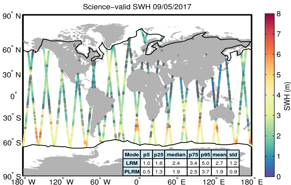
Figure 19. Geographical distribution of science-valid SWH data over oceans and lakes for 09/05/2017. The statistical values shown in the table refer to the SWH in m and are calculated separately for LRM and PLRM regions. The black lines mark the outer limit of the Arctic and Antarctic polar polygons. Gray circles denote records that have been rejected based on the editing criteria described in Table 3.
