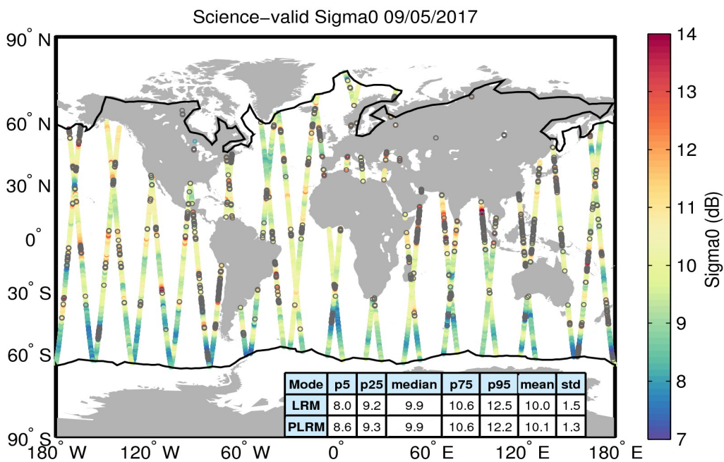
Figure 27. Geographical distribution of science-valid sigma0 data over oceans and lakes for 09/05/2017. The statistical values shown in the table refer to the sigma0 in dB and are calculated separately for LRM and PLRM regions. The black lines mark the outer limit of the Arctic and Antarctic polar polygons. Gray circles denote records that have been rejected based on the editing criteria described in Table 4.
