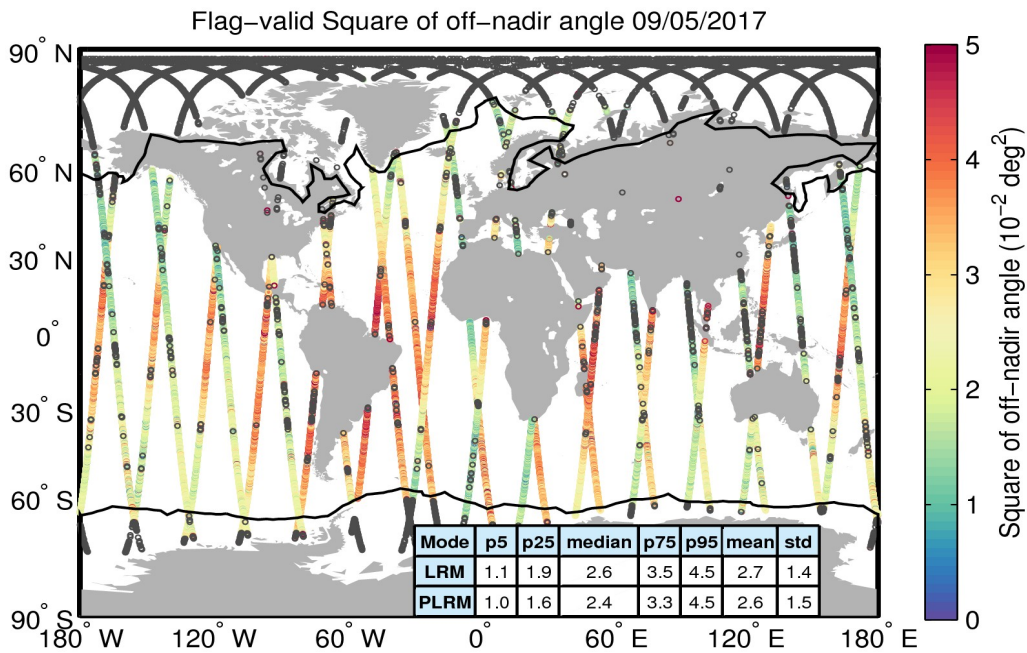
Figure 37. Geographical distribution of flag-valid mispointing data over oceans and lakes for 09/05/2017. The statistical values shown in the table refer to the mispointing in 10^{-2} deg 2 and are calculated separately for LRM and PLRM regions. Measurements taken over polar polygons have been excluded from the computation of the statistical values. The black lines mark the outer limit of the Arctic and Antarctic polar polygons. Gray circles denote negative values.
