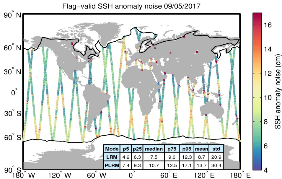
Figure 8. Geographical distribution of flag-valid 20-Hz SSH anomaly measurement noise over oceans and lakes for 09/05/2017. The statistical values shown in the table refer to the SSH anomaly noise and are calculated separately for LRM and PLRM regions. Measurements taken over polar polygons have been excluded from the computation of the statistical values. The black lines mark the outer limit of the Arctic and Antarctic polar polygons.
