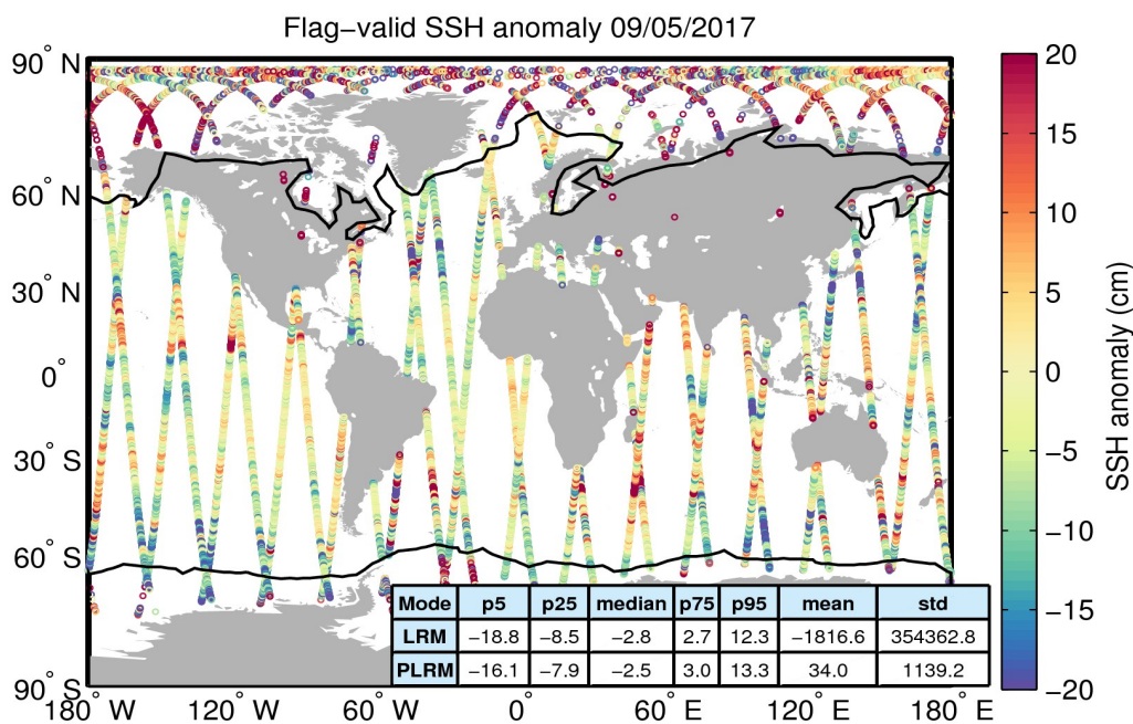
Figure 5. Geographical distribution of flag-valid 1-Hz SSH anomaly data over oceans and lakes for 09/05/2017. The statistical values shown in the table refer to the SSH anomaly in cm and are calculated separately for LRM and PLRM regions. Measurements taken over polar polygons have been excluded from the computation of the statistical values. The black lines mark the outer limit of the Arctic and Antarctic polar polygons.
