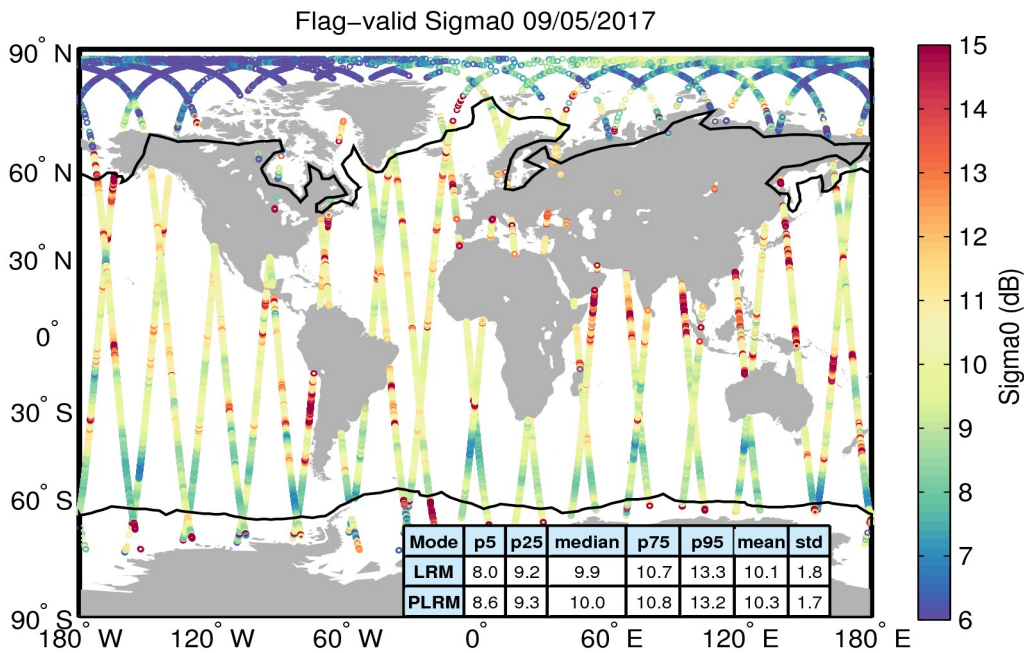
Figure 23. Geographical distribution of flag-valid sigma0 data over oceans and lakes for 09/05/2017. The statistical values shown in the table refer to the sigma0 in dB and are calculated separately for LRM and PLRM regions. Measurements taken over polar polygons have been excluded from the computation of the statistical values. The black lines mark the outer limit of the Arctic and Antarctic polar polygons.
