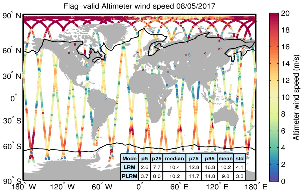
Figure 31. Geographical distribution of flag-valid wind data over oceans and lakes for 08/05/2017. The statistical values shown in the table refer to the wind in m/s and are calculated separately for LRM and PLRM regions. Measurements taken over polar polygons have been excluded from the computation of the statistical values. The black lines mark the outer limit of the Arctic and Antarctic polar polygons.
