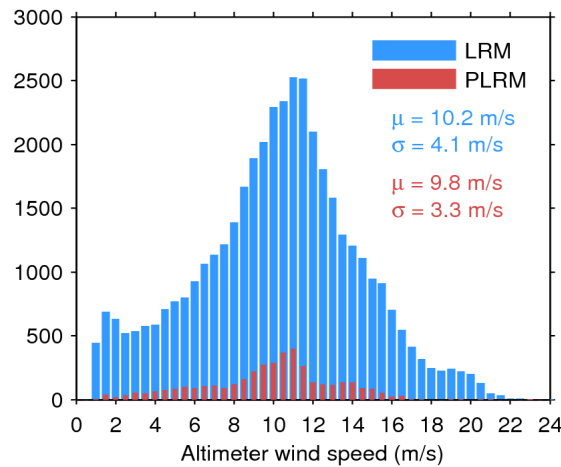
Figure 33. Histogram of flag-valid wind over oceans and lakes for LRM (blue) and PLRM (red) for 08/05/2017. The mean ( \mu ) and standard deviation ( \sigma ) are also shown. Note that values larger than 24 m/s are excluded from the histogram for the sake of readability but not from the computation of \mu and \sigma .
