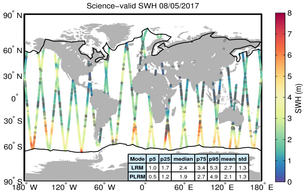
Figure 19. Geographical distribution of science-valid SWH data over oceans and lakes for 08/05/2017. The statistical values shown in the table refer to the SWH in m and are calculated separately for LRM and PLRM regions. The black lines mark the outer limit of the Arctic and Antarctic polar polygons. Gray circles denote records that have been rejected based on the editing criteria described in Table 3.
