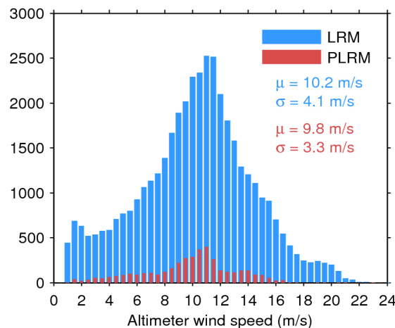
Figure 35. Histogram of science-valid wind over oceans and lakes for LRM (blue) and PLRM (red) for 08/05/2017. The mean ( \mu ) and standard deviation ( \sigma ) are also shown. Note that values larger than 24 m/s are excluded from the histogram for the sake of readability but not from the computation of \mu and \sigma .
