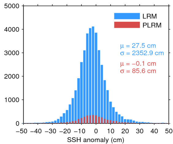
Figure 7. Histogram of flag-valid SSH anomaly over oceans and lakes for LRM (blue) and PLRM (red) for 08/05/2017. The mean ( \mu ) and standard deviation ( \sigma ) are also shown. Note that values outside [-50 50] cm are excluded from the histogram for the sake of readability but not from the computation of \mu and \sigma .
