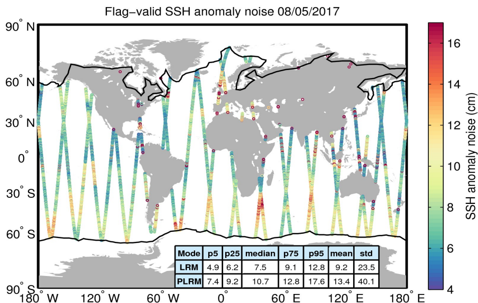
Figure 8. Geographical distribution of flag-valid 20-Hz SSH anomaly measurement noise over oceans and lakes for 08/05/2017. The statistical values shown in the table refer to the SSH anomaly noise and are calculated separately for LRM and PLRM regions. Measurements taken over polar polygons have been excluded from the computation of the statistical values. The black lines mark the outer limit of the Arctic and Antarctic polar polygons.
