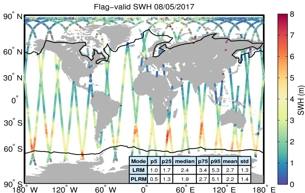
Figure 15. Geographical distribution of flag-valid SWH data over oceans and lakes for 08/05/2017. The statistical values shown in the table refer to the SWH in m and are calculated separately for LRM and PLRM regions. Measurements taken over polar polygons have been excluded from the computation of the statistical values. The black lines mark the outer limit of the Arctic and Antarctic polar polygons.
