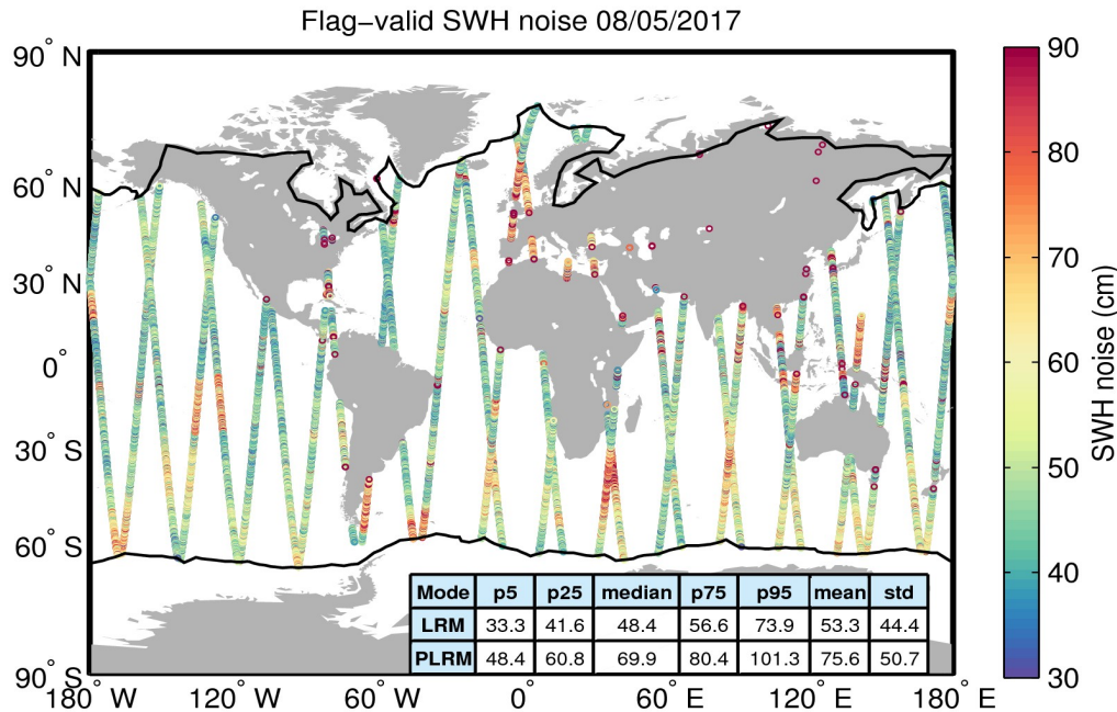
Figure 18. Geographical distribution of flag-valid 20-Hz SWH measurement noise over oceans and lakes for 08/05/2017. The statistical values shown in the table refer to the SWH noise and are calculated separately for LRM and PLRM regions. Measurements taken over polar polygons have been excluded from the computation of the statistical values. The black lines mark the outer limit of the Arctic and Antarctic polar polygons.
