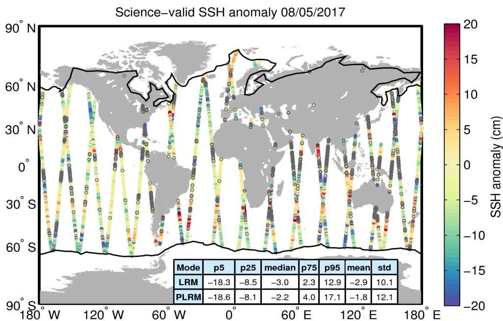
Figure 10. Geographical distribution of science-valid SSH anomaly data over oceans and lakes for 08/05/2017. The statistical values shown in the table refer to the SSH anomaly in cm and are calculated separately for LRM and PLRM regions. The black lines mark the outer limit of the Arctic and Antarctic polar polygons. Gray circles denote records that have been rejected based on the editing criteria described in Table 2.
