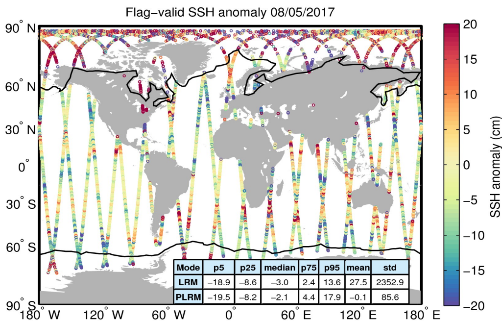
Figure 5. Geographical distribution of flag-valid 1-Hz SSH anomaly data over oceans and lakes for 08/05/2017. The statistical values shown in the table refer to the SSH anomaly in cm and are calculated separately for LRM and PLRM regions. Measurements taken over polar polygons have been excluded from the computation of the statistical values. The black lines mark the outer limit of the Arctic and Antarctic polar polygons.
