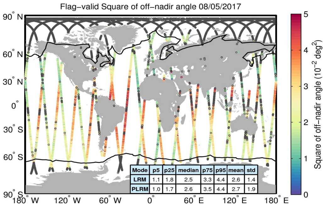
Figure 37. Geographical distribution of flag-valid mispointing data over oceans and lakes for 08/05/2017. The statistical values shown in the table refer to the mispointing in 10^{-2} deg 2 and are calculated separately for LRM and PLRM regions. Measurements taken over polar polygons have been excluded from the computation of the statistical values. The black lines mark the outer limit of the Arctic and Antarctic polar polygons. Gray circles denote negative values.
