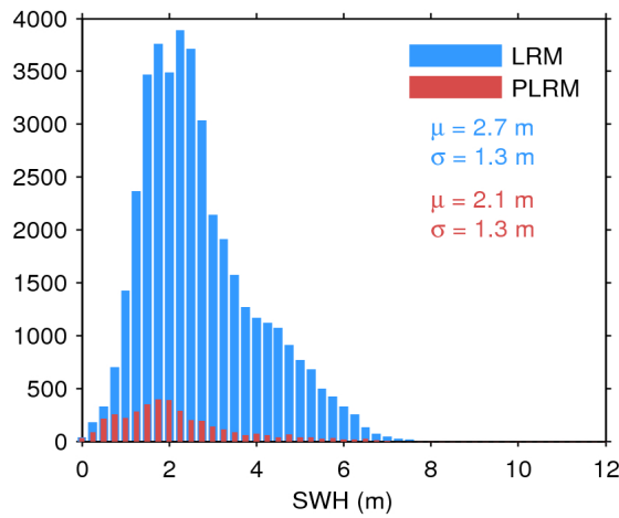
Figure 20. Histogram of science-valid SWH over oceans and lakes for LRM (blue) and PLRM (red) for 08/05/2017. The mean ( \mu ) and standard deviation ( \sigma ) are also shown. Note that values larger than 12 m are excluded from the histogram for the sake of readability but not from the computation of \mu and \sigma .
