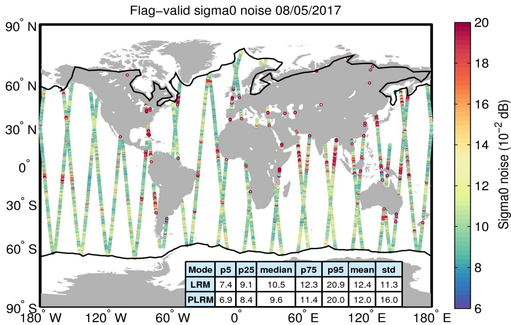
Figure 26. Geographical distribution of flag-valid 20-Hz sigma0 measurement noise over oceans and lakes for 08/05/2017. The statistical values shown in the table refer to the sigma0 noise and are calculated separately for LRM and PLRM regions. Measurements taken over polar polygons have been excluded from the computation of the statistical values. The black lines mark the outer limit of the Arctic and Antarctic polar polygons.
