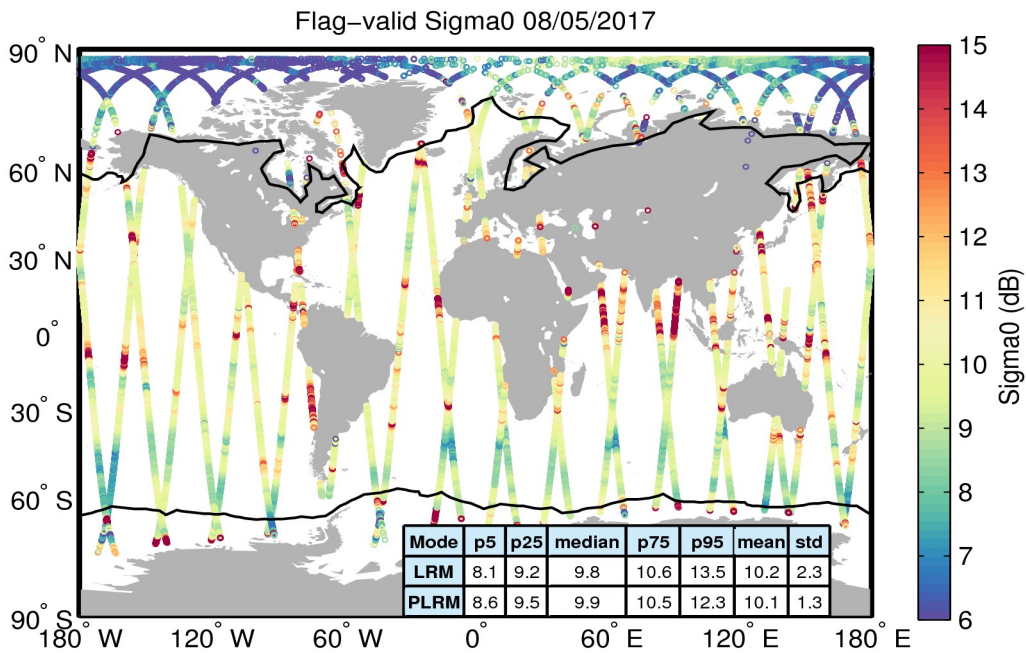
Figure 23. Geographical distribution of flag-valid sigma0 data over oceans and lakes for 08/05/2017. The statistical values shown in the table refer to the sigma0 in dB and are calculated separately for LRM and PLRM regions. Measurements taken over polar polygons have been excluded from the computation of the statistical values. The black lines mark the outer limit of the Arctic and Antarctic polar polygons.
