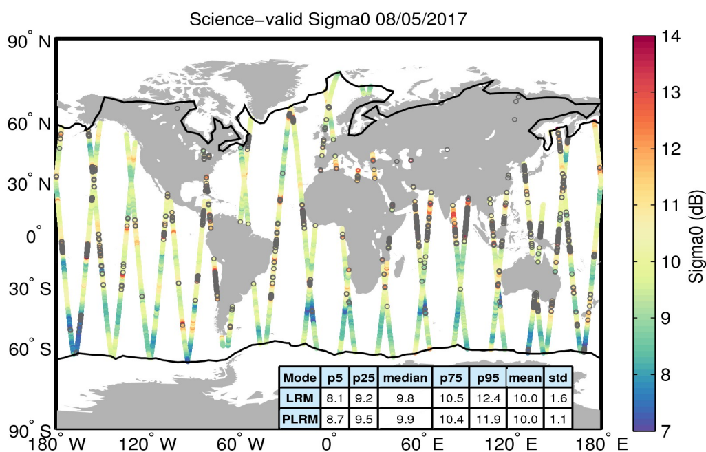
Figure 27. Geographical distribution of science-valid sigma0 data over oceans and lakes for 08/05/2017. The statistical values shown in the table refer to the sigma0 in dB and are calculated separately for LRM and PLRM regions. The black lines mark the outer limit of the Arctic and Antarctic polar polygons. Gray circles denote records that have been rejected based on the editing criteria described in Table 4.
