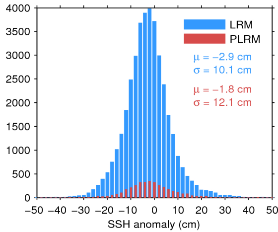
Figure 11. Histogram of science-valid SSH anomaly over oceans and lakes for LRM (blue) and PLRM (red) for 08/05/2017. The mean ( \mu ) and standard deviation ( \sigma ) are also shown. Note that values outside [-50\ 50] cm are excluded from the histogram for the sake of readability but not from the computation of \mu and \sigma .
