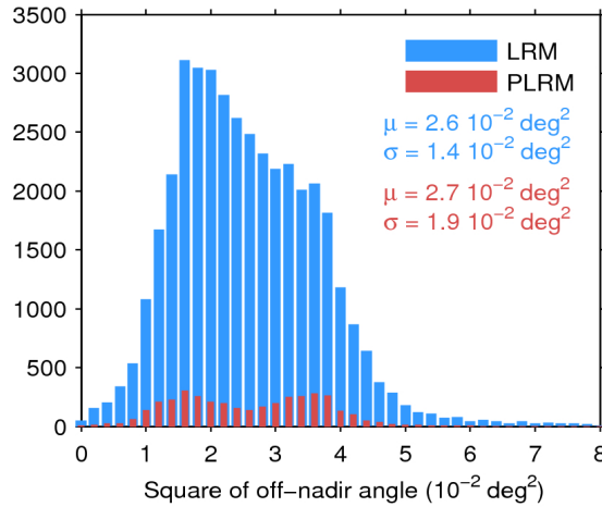
Figure 39. Histogram of flag-valid mispointing over oceans and lakes for LRM (blue) and PLRM (red) for 08/05/2017. Only positive values have been considered. The mean ( \mu ) and standard deviation ( \sigma ) are also shown. Note that values larger than 8 \cdot 10^{-2} \text{ deg}^2 are excluded from the histogram for the sake of readability but not from the computation of \mu and \sigma .
