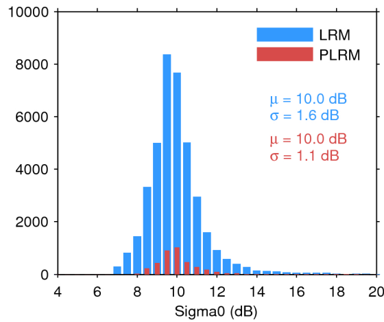
Figure 28. Histogram of science-valid sigma0 over oceans and lakes for LRM (blue) and PLRM (red) for 08/05/2017. The mean ( \mu ) and standard deviation ( \sigma ) are also shown. Note that values outside [4 20] dB are excluded from the histogram for the sake of readability but not from the computation of \mu and \sigma .
