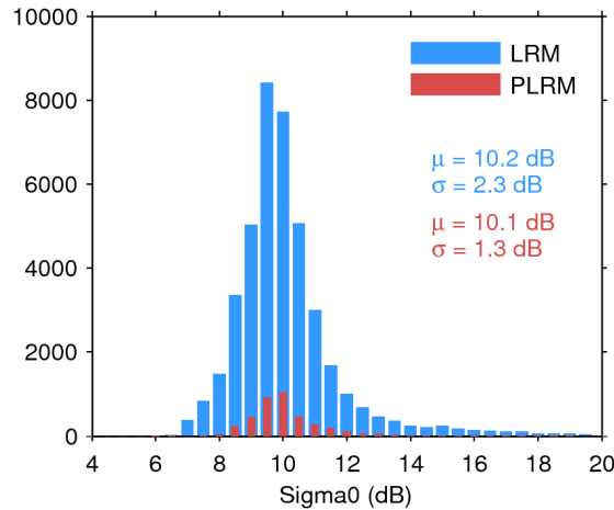
Figure 25. Histogram of flag-valid sigma0 over oceans and lakes for LRM (blue) and PLRM (red) for 08/05/2017. The mean ( \mu ) and standard deviation ( \sigma ) are also shown. Note that values outside [4 20] dB are excluded from the histogram for the sake of readability but not from the computation of \mu and \sigma .
