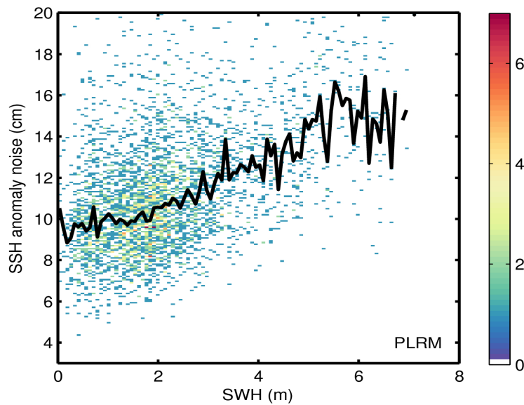
Figure 9. 2D histogram showing flag-valid SSH anomaly noise as a function of SWH for LRM (top) and PLRM (bottom) for 08/05/2017. The black line denotes the median SSH anomaly noise as a function of SWH.
