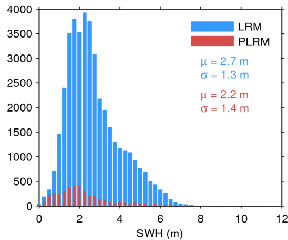
Figure 17. Histogram of flag-valid SWH over oceans and lakes for LRM (blue) and PLRM (red) for 08/05/2017. The mean ( \mu ) and standard deviation ( \sigma ) are also shown. Note that values larger than 12 m are excluded from the histogram for the sake of readability but not from the computation of \mu and \sigma .
