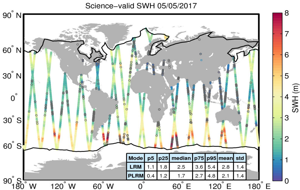
Figure 19. Geographical distribution of science-valid SWH data over oceans and lakes for 05/05/2017. The statistical values shown in the table refer to the SWH in m and are calculated separately for LRM and PLRM regions. The black lines mark the outer limit of the Arctic and Antarctic polar polygons. Gray circles denote records that have been rejected based on the editing criteria described in Table 3.
