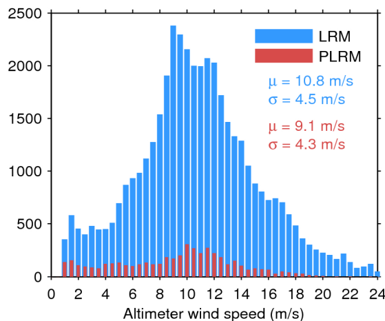
Figure 35. Histogram of science-valid wind over oceans and lakes for LRM (blue) and PLRM (red) for 05/05/2017. The mean ( \mu ) and standard deviation ( \sigma ) are also shown. Note that values larger than 24 m/s are excluded from the histogram for the sake of readability but not from the computation of \mu and \sigma .
