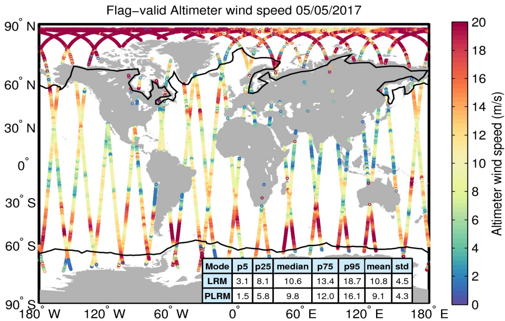
Figure 31. Geographical distribution of flag-valid wind data over oceans and lakes for 05/05/2017. The statistical values shown in the table refer to the wind in m/s and are calculated separately for LRM and PLRM regions. Measurements taken over polar polygons have been excluded from the computation of the statistical values. The black lines mark the outer limit of the Arctic and Antarctic polar polygons.
