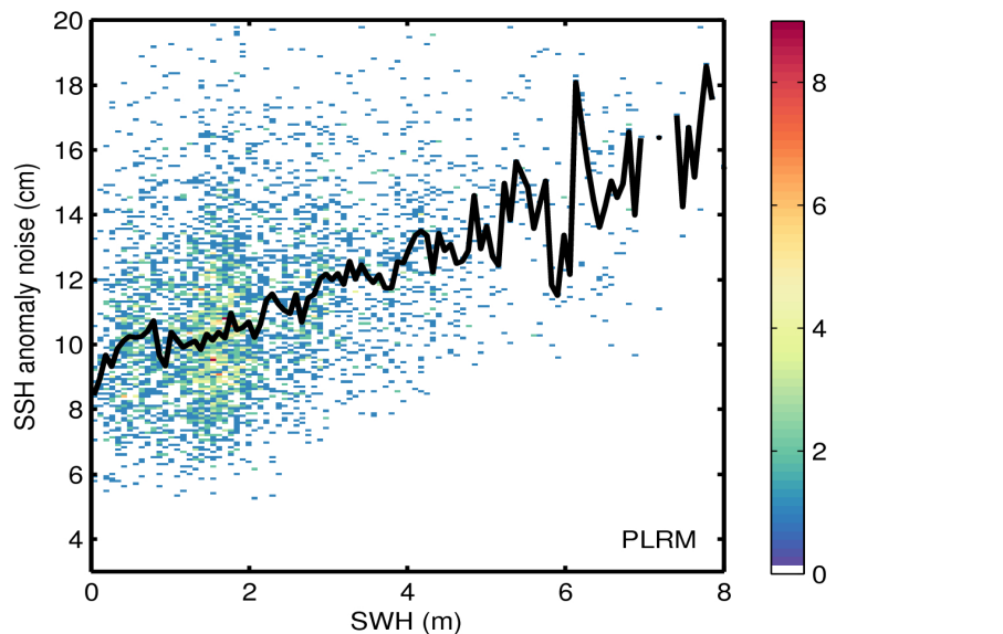
Figure 9. 2D histogram showing flag-valid SSH anomaly noise as a function of SWH for LRM (top) and PLRM (bottom) for 05/05/2017. The black line denotes the median SSH anomaly noise as a function of SWH.
