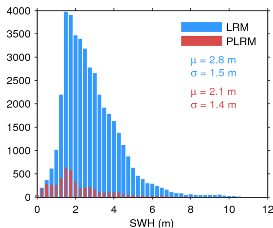
Figure 17. Histogram of flag-valid SWH over oceans and lakes for LRM (blue) and PLRM (red) for 05/05/2017. The mean ( \mu ) and standard deviation ( \sigma ) are also shown. Note that values larger than 12 m are excluded from the histogram for the sake of readability but not from the computation of \mu and \sigma .
