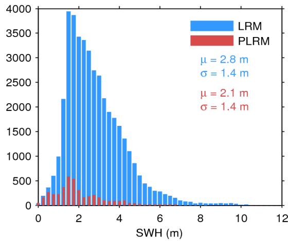
Figure 20. Histogram of science-valid SWH over oceans and lakes for LRM (blue) and PLRM (red) for 05/05/2017. The mean ( \mu ) and standard deviation ( \sigma ) are also shown. Note that values larger than 12 m are excluded from the histogram for the sake of readability but not from the computation of \mu and \sigma .
