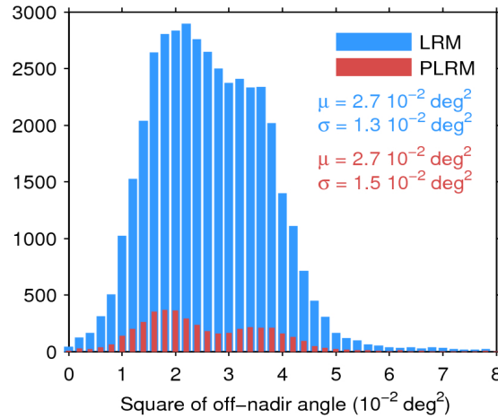
Figure 39. Histogram of flag-valid mispointing over oceans and lakes for LRM (blue) and PLRM (red) for 05/05/2017. Only positive values have been considered. The mean ( \mu ) and standard deviation ( \sigma ) are also shown. Note that values larger than 8 \cdot 10^{-2} \text{ deg}^2 are excluded from the histogram for the sake of readability but not from the computation of \mu and \sigma .
