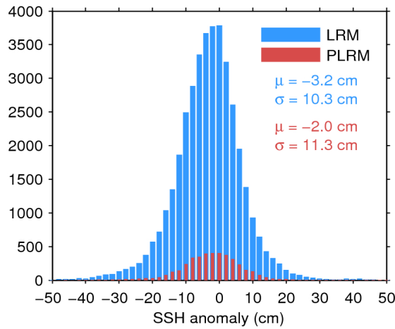
Figure 11. Histogram of science-valid SSH anomaly over oceans and lakes for LRM (blue) and PLRM (red) for 05/05/2017. The mean ( \mu ) and standard deviation ( \sigma ) are also shown. Note that values outside [-50\ 50] cm are excluded from the histogram for the sake of readability but not from the computation of \mu and \sigma .
