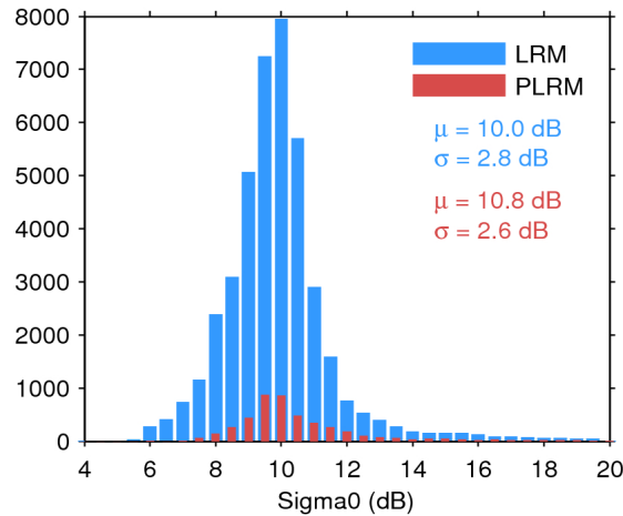
Figure 25. Histogram of flag-valid sigma0 over oceans and lakes for LRM (blue) and PLRM (red) for 05/05/2017. The mean ( \mu ) and standard deviation ( \sigma ) are also shown. Note that values outside [4 20] dB are excluded from the histogram for the sake of readability but not from the computation of \mu and \sigma .
