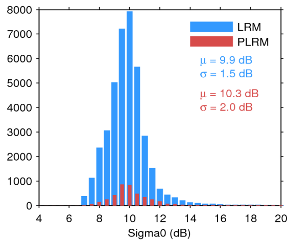
Figure 28. Histogram of science-valid sigma0 over oceans and lakes for LRM (blue) and PLRM (red) for 05/05/2017. The mean ( \mu ) and standard deviation ( \sigma ) are also shown. Note that values outside [4 20] dB are excluded from the histogram for the sake of readability but not from the computation of \mu and \sigma .
