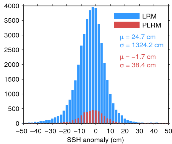
Figure 7. Histogram of flag-valid SSH anomaly over oceans and lakes for LRM (blue) and PLRM (red) for 05/05/2017. The mean ( \mu ) and standard deviation ( \sigma ) are also shown. Note that values outside [-50 \ 50] cm are excluded from the histogram for the sake of readability but not from the computation of \mu and \sigma .
