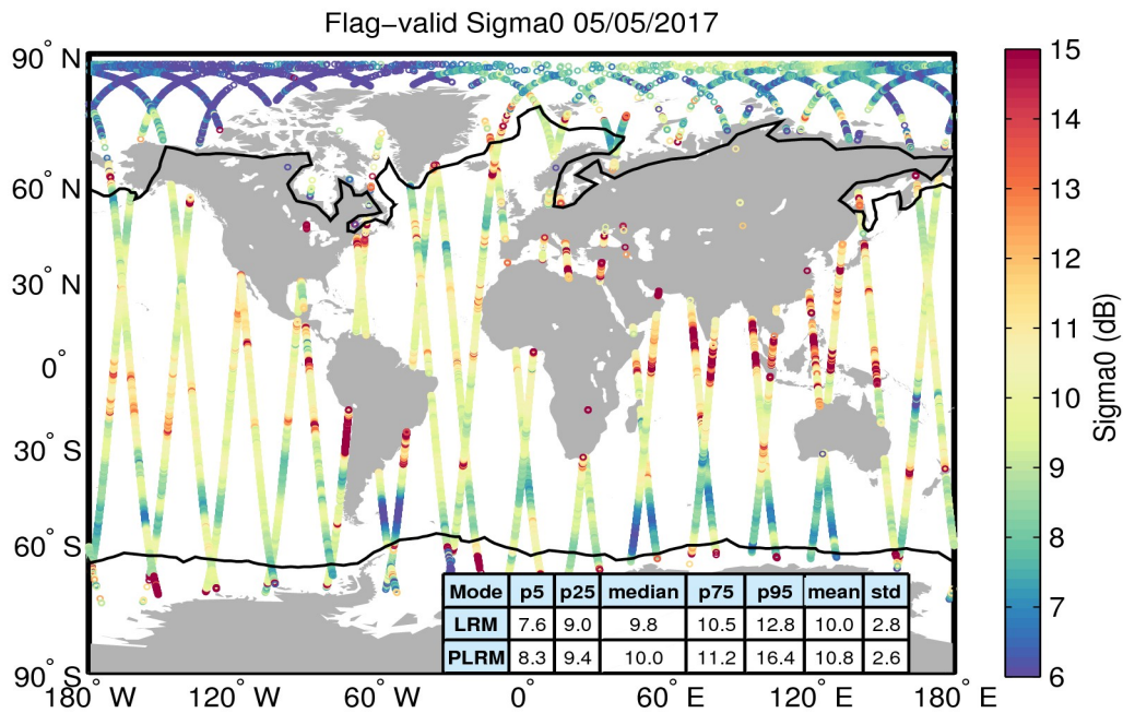
Figure 23. Geographical distribution of flag-valid sigma0 data over oceans and lakes for 05/05/2017. The statistical values shown in the table refer to the sigma0 in dB and are calculated separately for LRM and PLRM regions. Measurements taken over polar polygons have been excluded from the computation of the statistical values. The black lines mark the outer limit of the Arctic and Antarctic polar polygons.
