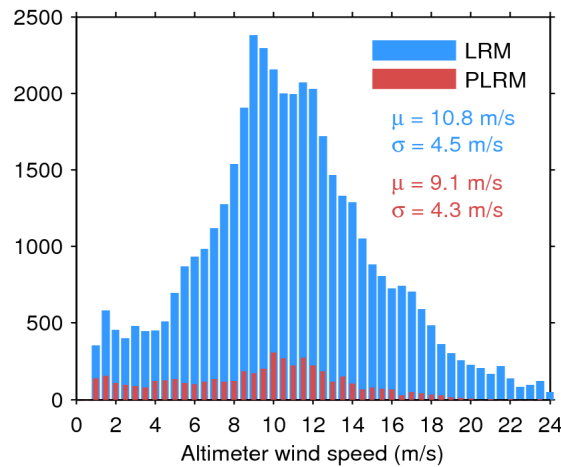
Figure 33. Histogram of flag-valid wind over oceans and lakes for LRM (blue) and PLRM (red) for 05/05/2017. The mean ( \mu ) and standard deviation ( \sigma ) are also shown. Note that values larger than 24 m/s are excluded from the histogram for the sake of readability but not from the computation of \mu and \sigma .
