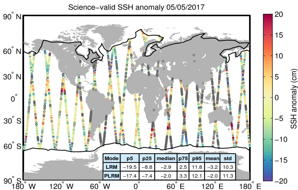
Figure 10. Geographical distribution of science-valid SSH anomaly data over oceans and lakes for 05/05/2017. The statistical values shown in the table refer to the SSH anomaly in cm and are calculated separately for LRM and PLRM regions. The black lines mark the outer limit of the Arctic and Antarctic polar polygons. Gray circles denote records that have been rejected based on the editing criteria described in Table 2.
