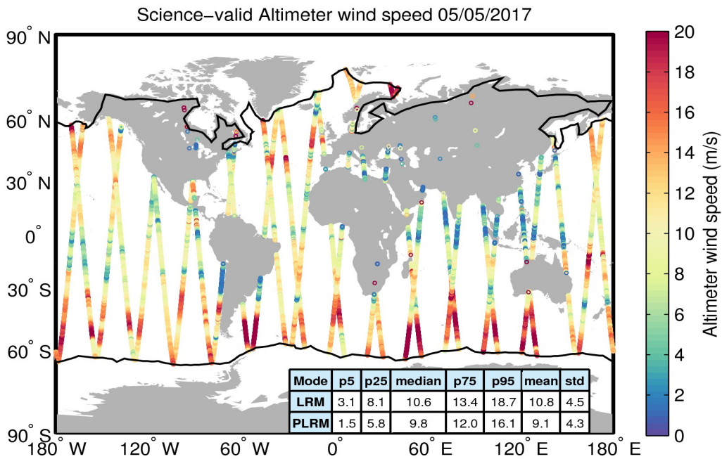
Figure 34. Geographical distribution of science-valid wind data over oceans and lakes for 05/05/2017. The statistical values shown in the table refer to the wind in m/s and are calculated separately for LRM and PLRM regions. The black lines mark the outer limit of the Arctic and Antarctic polar polygons. Gray circles denote records that have been rejected based on the editing criteria described in Table 5.
