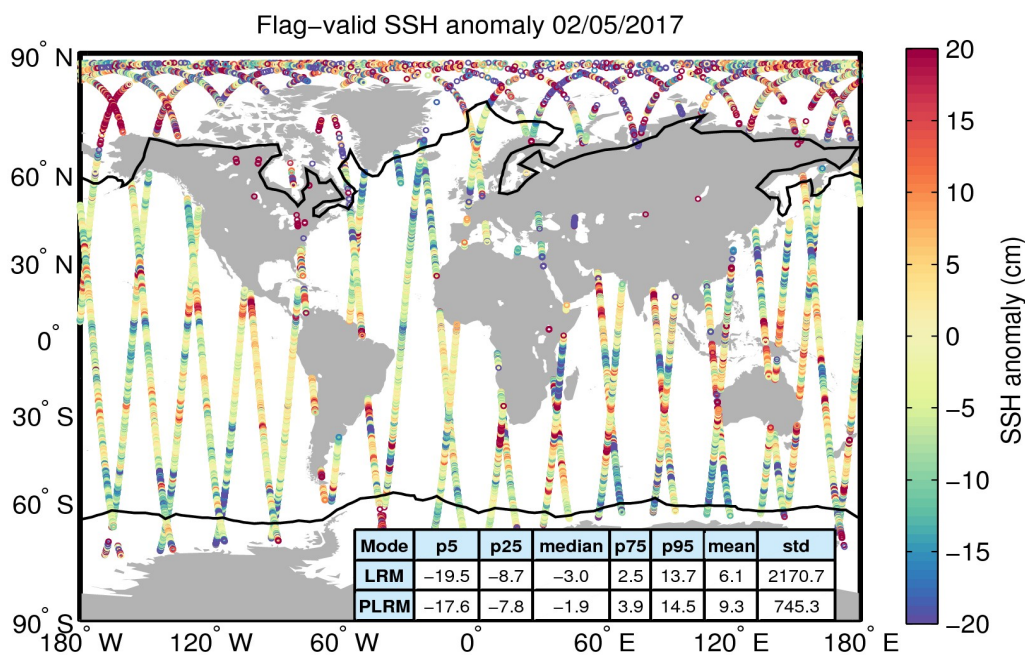
Figure 5. Geographical distribution of flag-valid 1-Hz SSH anomaly data over oceans and lakes for 02/05/2017. The statistical values shown in the table refer to the SSH anomaly in cm and are calculated separately for LRM and PLRM regions. Measurements taken over polar polygons have been excluded from the computation of the statistical values. The black lines mark the outer limit of the Arctic and Antarctic polar polygons.
