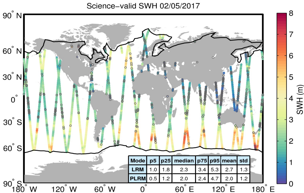
Figure 19. Geographical distribution of science-valid SWH data over oceans and lakes for 02/05/2017. The statistical values shown in the table refer to the SWH in m and are calculated separately for LRM and PLRM regions. The black lines mark the outer limit of the Arctic and Antarctic polar polygons. Gray circles denote records that have been rejected based on the editing criteria described in Table 3.
