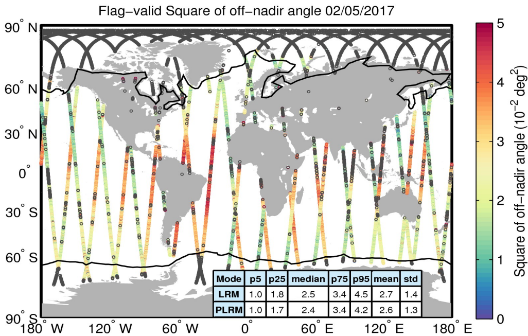
Figure 37. Geographical distribution of flag-valid mispointing data over oceans and lakes for 02/05/2017. The statistical values shown in the table refer to the mispointing in 10^{-2} deg 2 and are calculated separately for LRM and PLRM regions. Measurements taken over polar polygons have been excluded from the computation of the statistical values. The black lines mark the outer limit of the Arctic and Antarctic polar polygons. Gray circles denote negative values.
