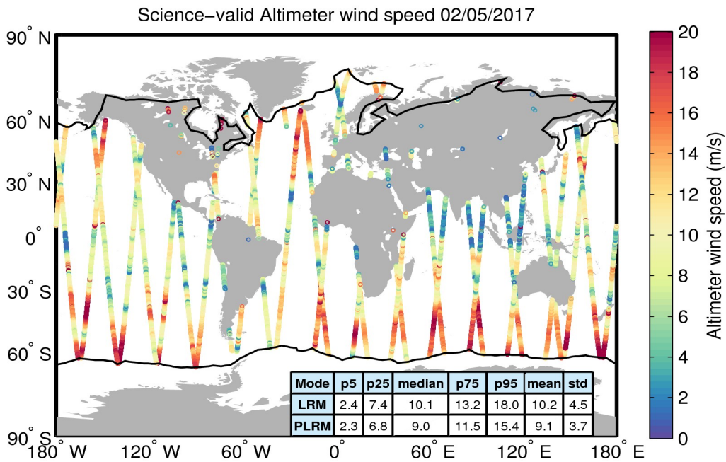
Figure 34. Geographical distribution of science-valid wind data over oceans and lakes for 02/05/2017. The statistical values shown in the table refer to the wind in m/s and are calculated separately for LRM and PLRM regions. The black lines mark the outer limit of the Arctic and Antarctic polar polygons. Gray circles denote records that have been rejected based on the editing criteria described in Table 5.
