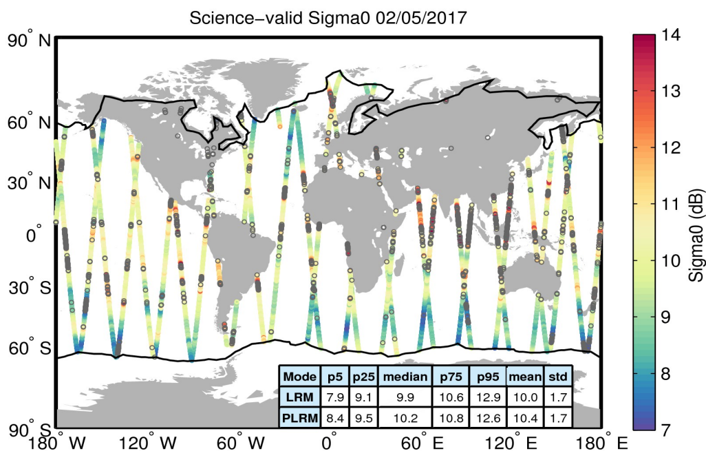
Figure 27. Geographical distribution of science-valid sigma0 data over oceans and lakes for 02/05/2017. The statistical values shown in the table refer to the sigma0 in dB and are calculated separately for LRM and PLRM regions. The black lines mark the outer limit of the Arctic and Antarctic polar polygons. Gray circles denote records that have been rejected based on the editing criteria described in Table 4.
