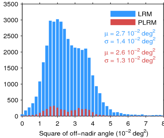
Figure 39. Histogram of flag-valid mispointing over oceans and lakes for LRM (blue) and PLRM (red) for 02/05/2017. Only positive values have been considered. The mean ( \mu ) and standard deviation ( \sigma ) are also shown. Note that values larger than 8 \cdot 10^{-2} \text{ deg}^2 are excluded from the histogram for the sake of readability but not from the computation of \mu and \sigma .
