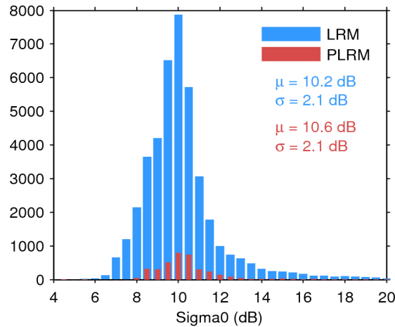
Figure 25. Histogram of flag-valid sigma0 over oceans and lakes for LRM (blue) and PLRM (red) for 02/05/2017. The mean ( \mu ) and standard deviation ( \sigma ) are also shown. Note that values outside [4 20] dB are excluded from the histogram for the sake of readability but not from the computation of \mu and \sigma .
