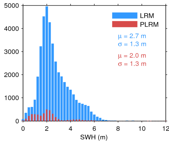
Figure 17. Histogram of flag-valid SWH over oceans and lakes for LRM (blue) and PLRM (red) for 02/05/2017. The mean ( \mu ) and standard deviation ( \sigma ) are also shown. Note that values larger than 12 m are excluded from the histogram for the sake of readability but not from the computation of \mu and \sigma .
