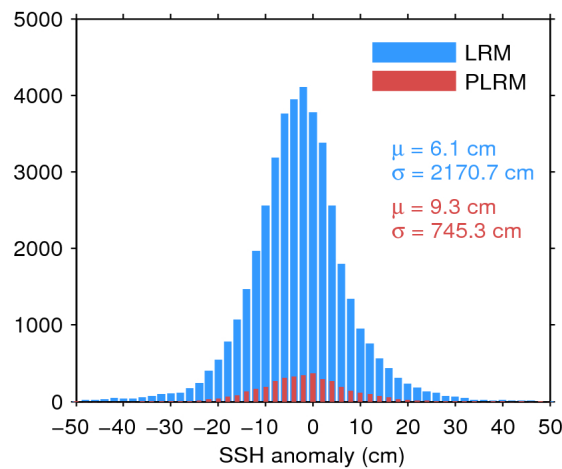
Figure 7. Histogram of flag-valid SSH anomaly over oceans and lakes for LRM (blue) and PLRM (red) for 02/05/2017. The mean ( \mu ) and standard deviation ( \sigma ) are also shown. Note that values outside [-50\ 50] cm are excluded from the histogram for the sake of readability but not from the computation of \mu and \sigma .
