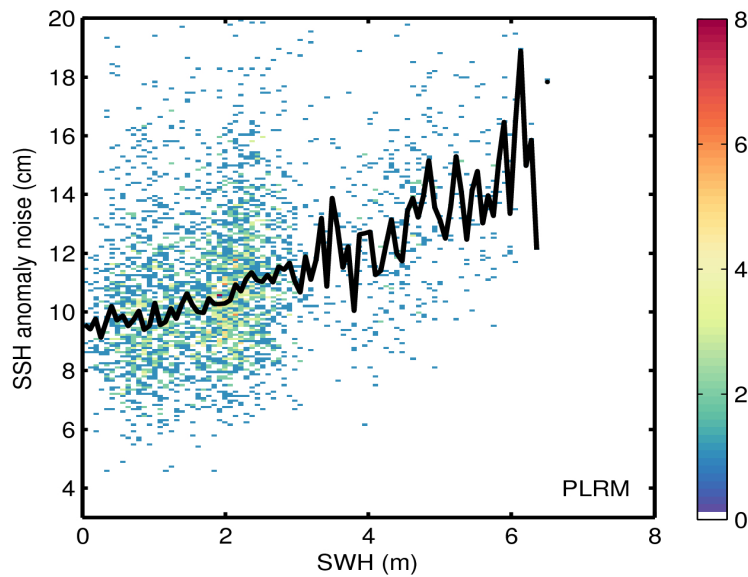
Figure 9. 2D histogram showing flag-valid SSH anomaly noise as a function of SWH for LRM (top) and PLRM (bottom) for 02/05/2017. The black line denotes the median SSH anomaly noise as a function of SWH.
