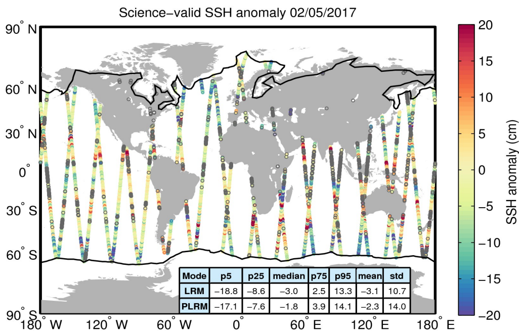
Figure 10. Geographical distribution of science-valid SSH anomaly data over oceans and lakes for 02/05/2017. The statistical values shown in the table refer to the SSH anomaly in cm and are calculated separately for LRM and PLRM regions. The black lines mark the outer limit of the Arctic and Antarctic polar polygons. Gray circles denote records that have been rejected based on the editing criteria described in Table 2.
