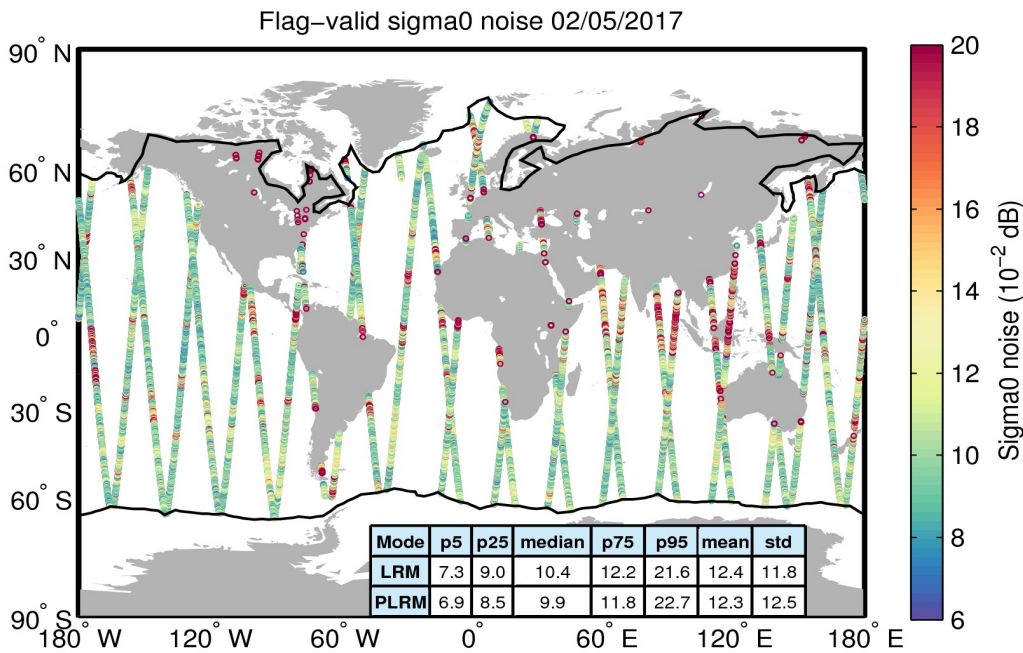
Figure 26. Geographical distribution of flag-valid 20-Hz sigma0 measurement noise over oceans and lakes for 02/05/2017. The statistical values shown in the table refer to the sigma0 noise and are calculated separately for LRM and PLRM regions. Measurements taken over polar polygons have been excluded from the computation of the statistical values. The black lines mark the outer limit of the Arctic and Antarctic polar polygons.
