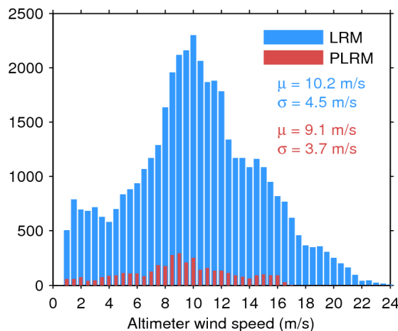
Figure 35. Histogram of science-valid wind over oceans and lakes for LRM (blue) and PLRM (red) for 02/05/2017. The mean ( \mu ) and standard deviation ( \sigma ) are also shown. Note that values larger than 24 m/s are excluded from the histogram for the sake of readability but not from the computation of \mu and \sigma .
