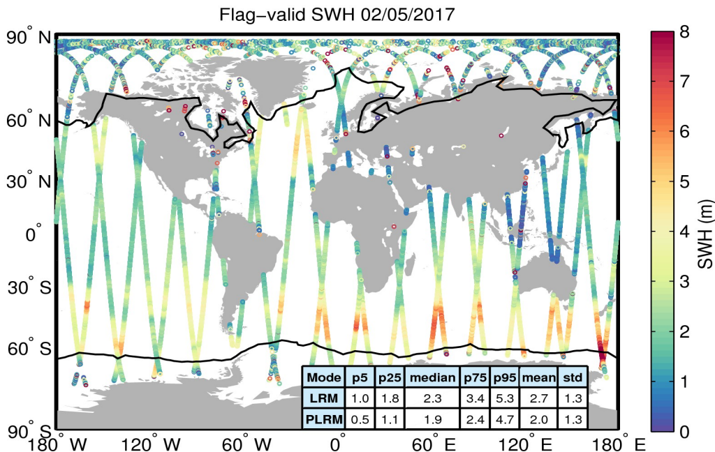
Figure 15. Geographical distribution of flag-valid SWH data over oceans and lakes for 02/05/2017. The statistical values shown in the table refer to the SWH in m and are calculated separately for LRM and PLRM regions. Measurements taken over polar polygons have been excluded from the computation of the statistical values. The black lines mark the outer limit of the Arctic and Antarctic polar polygons.
