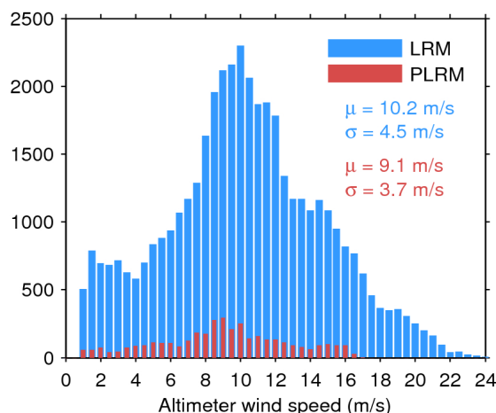
Figure 33. Histogram of flag-valid wind over oceans and lakes for LRM (blue) and PLRM (red) for 02/05/2017. The mean ( \mu ) and standard deviation ( \sigma ) are also shown. Note that values larger than 24 m/s are excluded from the histogram for the sake of readability but not from the computation of \mu and \sigma .
