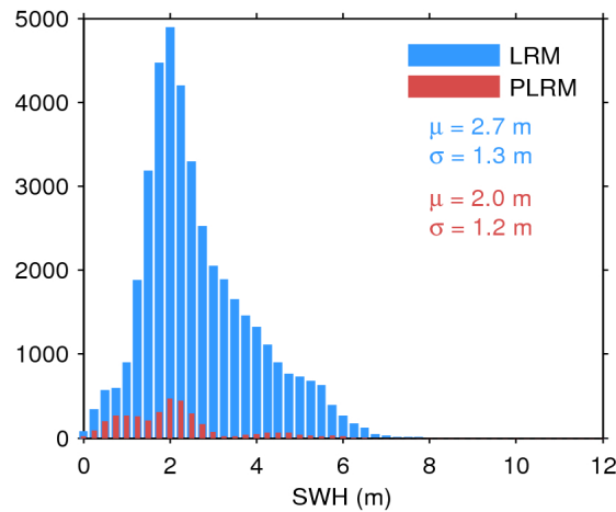
Figure 20. Histogram of science-valid SWH over oceans and lakes for LRM (blue) and PLRM (red) for 02/05/2017. The mean ( \mu ) and standard deviation ( \sigma ) are also shown. Note that values larger than 12 m are excluded from the histogram for the sake of readability but not from the computation of \mu and \sigma .
