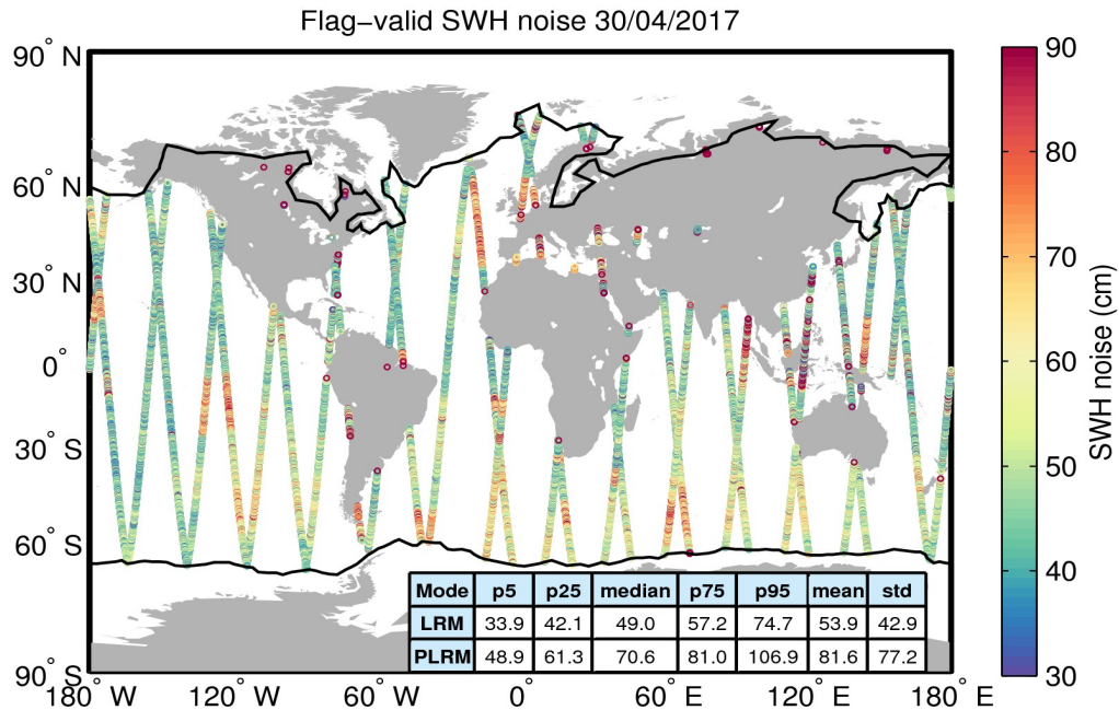
Figure 18. Geographical distribution of flag-valid 20-Hz SWH measurement noise over oceans and lakes for 30/04/2017. The statistical values shown in the table refer to the SWH noise and are calculated separately for LRM and PLRM regions. Measurements taken over polar polygons have been excluded from the computation of the statistical values. The black lines mark the outer limit of the Arctic and Antarctic polar polygons.
