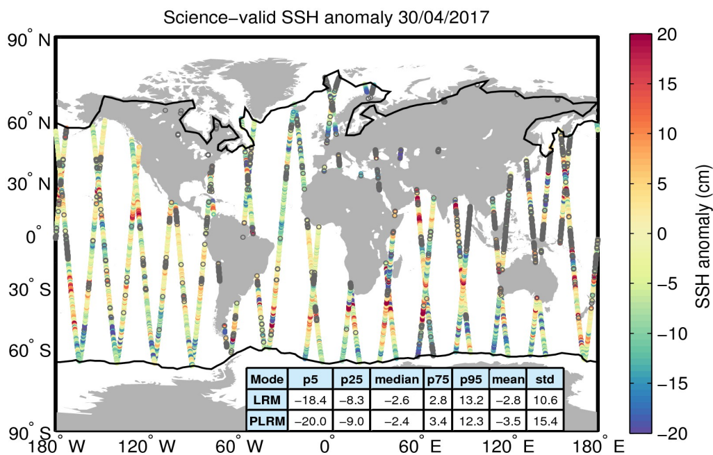
Figure 10. Geographical distribution of science-valid SSH anomaly data over oceans and lakes for 30/04/2017. The statistical values shown in the table refer to the SSH anomaly in cm and are calculated separately for LRM and PLRM regions. The black lines mark the outer limit of the Arctic and Antarctic polar polygons. Gray circles denote records that have been rejected based on the editing criteria described in Table 2.
