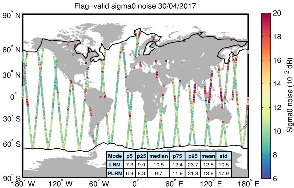
Figure 26. Geographical distribution of flag-valid 20-Hz sigma0 measurement noise over oceans and lakes for 30/04/2017. The statistical values shown in the table refer to the sigma0 noise and are calculated separately for LRM and PLRM regions. Measurements taken over polar polygons have been excluded from the computation of the statistical values. The black lines mark the outer limit of the Arctic and Antarctic polar polygons.
