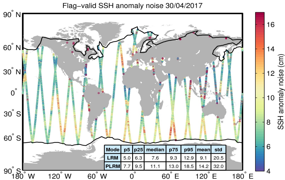
Figure 8. Geographical distribution of flag-valid 20-Hz SSH anomaly measurement noise over oceans and lakes for 30/04/2017. The statistical values shown in the table refer to the SSH anomaly noise and are calculated separately for LRM and PLRM regions. Measurements taken over polar polygons have been excluded from the computation of the statistical values. The black lines mark the outer limit of the Arctic and Antarctic polar polygons.
