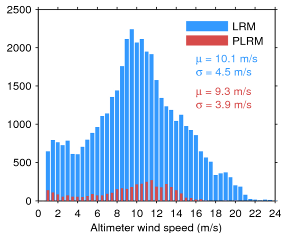
Figure 35. Histogram of science-valid wind over oceans and lakes for LRM (blue) and PLRM (red) for 30/04/2017. The mean ( \mu ) and standard deviation ( \sigma ) are also shown. Note that values larger than 24 m/s are excluded from the histogram for the sake of readability but not from the computation of \mu and \sigma .
