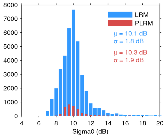
Figure 28. Histogram of science-valid sigma0 over oceans and lakes for LRM (blue) and PLRM (red) for 30/04/2017. The mean ( \mu ) and standard deviation ( \sigma ) are also shown. Note that values outside [4 20] dB are excluded from the histogram for the sake of readability but not from the computation of \mu and \sigma .
