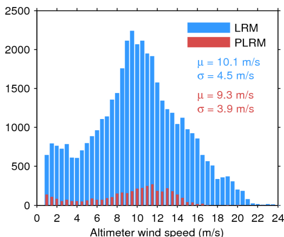
Figure 33. Histogram of flag-valid wind over oceans and lakes for LRM (blue) and PLRM (red) for 30/04/2017. The mean ( \mu ) and standard deviation ( \sigma ) are also shown. Note that values larger than 24 m/s are excluded from the histogram for the sake of readability but not from the computation of \mu and \sigma .
