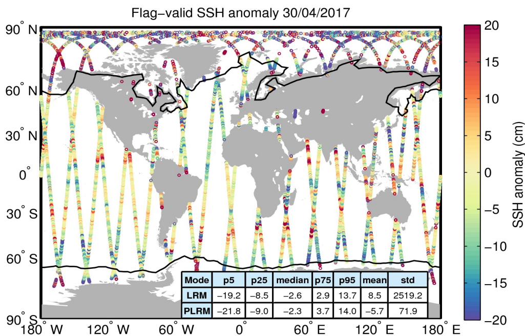
Figure 5. Geographical distribution of flag-valid 1-Hz SSH anomaly data over oceans and lakes for 30/04/2017. The statistical values shown in the table refer to the SSH anomaly in cm and are calculated separately for LRM and PLRM regions. Measurements taken over polar polygons have been excluded from the computation of the statistical values. The black lines mark the outer limit of the Arctic and Antarctic polar polygons.
