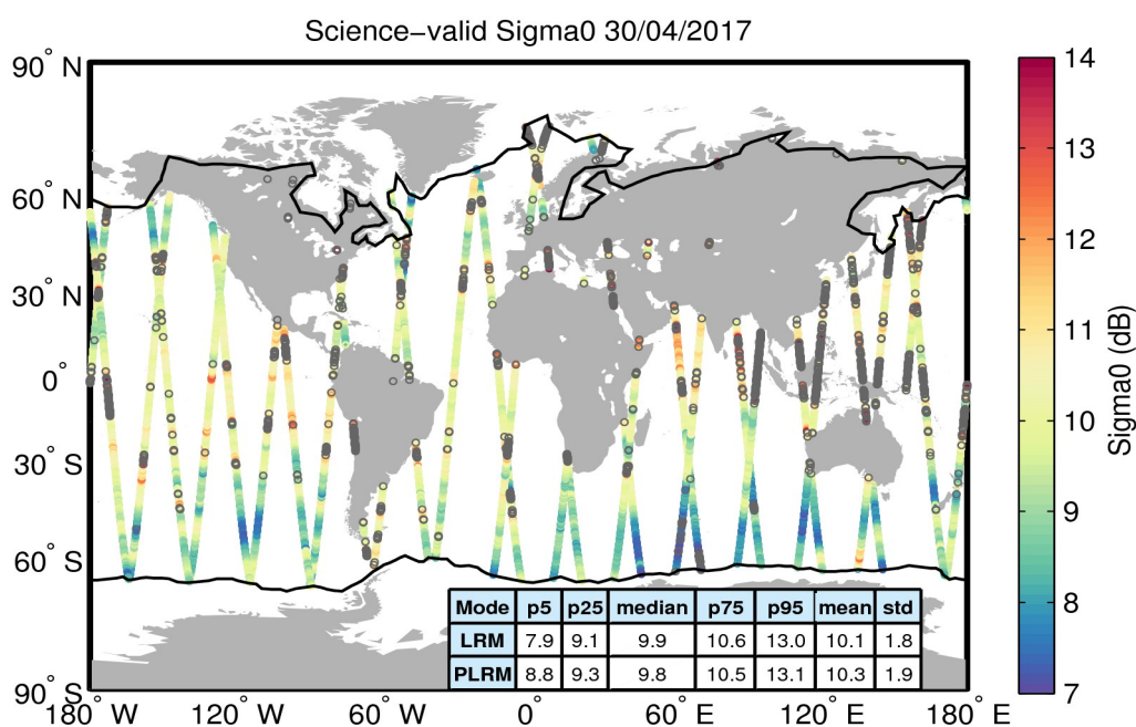
Figure 27. Geographical distribution of science-valid sigma0 data over oceans and lakes for 30/04/2017. The statistical values shown in the table refer to the sigma0 in dB and are calculated separately for LRM and PLRM regions. The black lines mark the outer limit of the Arctic and Antarctic polar polygons. Gray circles denote records that have been rejected based on the editing criteria described in Table 4.
