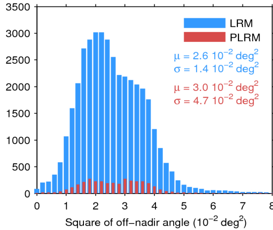
Figure 39. Histogram of flag-valid mispointing over oceans and lakes for LRM (blue) and PLRM (red) for 30/04/2017. Only positive values have been considered. The mean ( \mu ) and standard deviation ( \sigma ) are also shown. Note that values larger than 8 \cdot 10^{-2} \text{ deg}^2 are excluded from the histogram for the sake of readability but not from the computation of \mu and \sigma .
