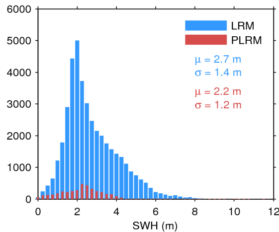
Figure 17. Histogram of flag-valid SWH over oceans and lakes for LRM (blue) and PLRM (red) for 30/04/2017. The mean ( \mu ) and standard deviation ( \sigma ) are also shown. Note that values larger than 12 m are excluded from the histogram for the sake of readability but not from the computation of \mu and \sigma .
