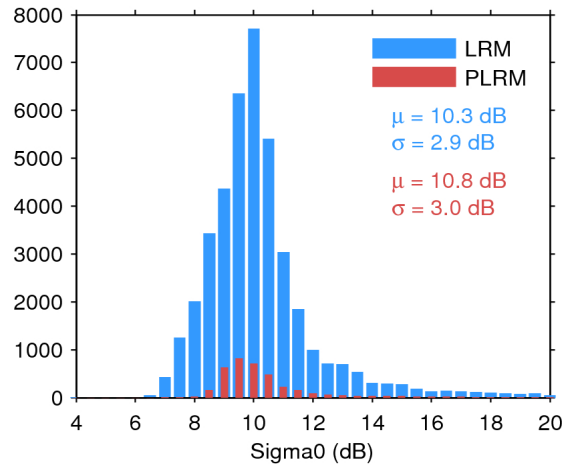
Figure 25. Histogram of flag-valid sigma0 over oceans and lakes for LRM (blue) and PLRM (red) for 30/04/2017. The mean ( \mu ) and standard deviation ( \sigma ) are also shown. Note that values outside [4 20] dB are excluded from the histogram for the sake of readability but not from the computation of \mu and \sigma .
