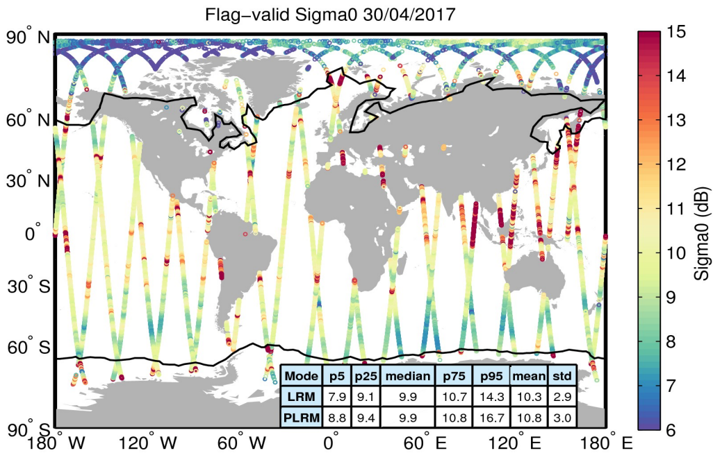
Figure 23. Geographical distribution of flag-valid sigma0 data over oceans and lakes for 30/04/2017. The statistical values shown in the table refer to the sigma0 in dB and are calculated separately for LRM and PLRM regions. Measurements taken over polar polygons have been excluded from the computation of the statistical values. The black lines mark the outer limit of the Arctic and Antarctic polar polygons.
