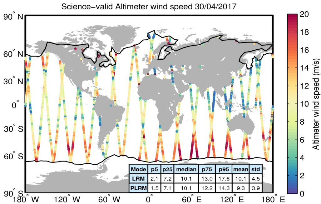
Figure 34. Geographical distribution of science-valid wind data over oceans and lakes for 30/04/2017. The statistical values shown in the table refer to the wind in m/s and are calculated separately for LRM and PLRM regions. The black lines mark the outer limit of the Arctic and Antarctic polar polygons. Gray circles denote records that have been rejected based on the editing criteria described in Table 5.
