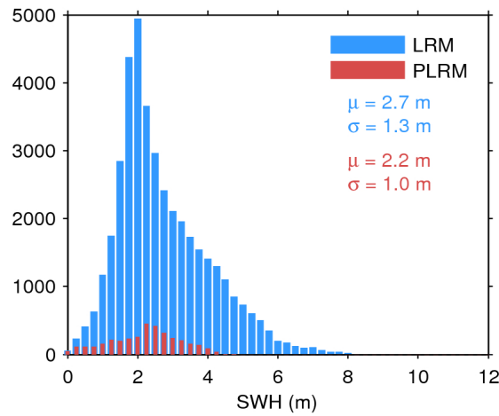
Figure 20. Histogram of science-valid SWH over oceans and lakes for LRM (blue) and PLRM (red) for 30/04/2017. The mean ( \mu ) and standard deviation ( \sigma ) are also shown. Note that values larger than 12 m are excluded from the histogram for the sake of readability but not from the computation of \mu and \sigma .
