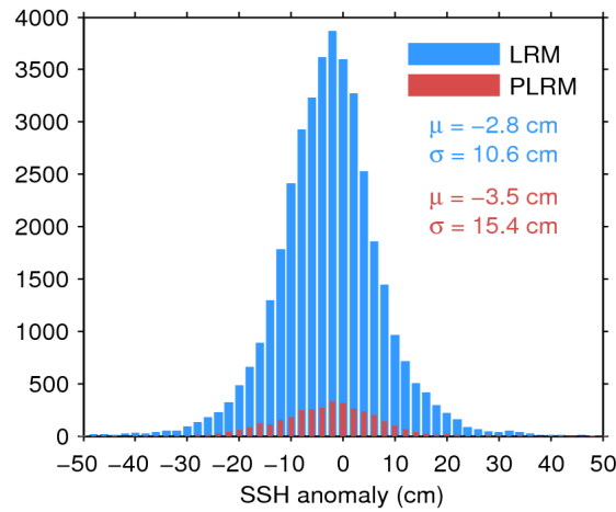
Figure 11. Histogram of science-valid SSH anomaly over oceans and lakes for LRM (blue) and PLRM (red) for 30/04/2017. The mean ( \mu ) and standard deviation ( \sigma ) are also shown. Note that values outside [-50 50] cm are excluded from the histogram for the sake of readability but not from the computation of \mu and \sigma .
