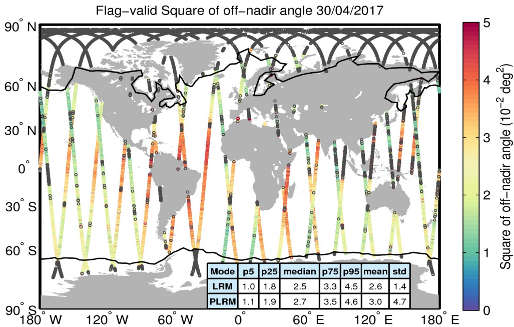
Figure 37. Geographical distribution of flag-valid mispointing data over oceans and lakes for 30/04/2017. The statistical values shown in the table refer to the mispointing in 10^{-2} deg 2 and are calculated separately for LRM and PLRM regions. Measurements taken over polar polygons have been excluded from the computation of the statistical values. The black lines mark the outer limit of the Arctic and Antarctic polar polygons. Gray circles denote negative values.
