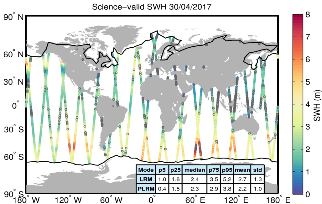
Figure 19. Geographical distribution of science-valid SWH data over oceans and lakes for 30/04/2017. The statistical values shown in the table refer to the SWH in m and are calculated separately for LRM and PLRM regions. The black lines mark the outer limit of the Arctic and Antarctic polar polygons. Gray circles denote records that have been rejected based on the editing criteria described in Table 3.
