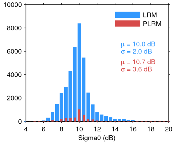
Figure 25. Histogram of flag-valid sigma0 over oceans and lakes for LRM (blue) and PLRM (red) for 28/04/2017. The mean ( \mu ) and standard deviation ( \sigma ) are also shown. Note that values outside [4 20] dB are excluded from the histogram for the sake of readability but not from the computation of \mu and \sigma .
