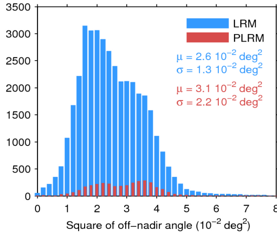
Figure 39. Histogram of flag-valid mispointing over oceans and lakes for LRM (blue) and PLRM (red) for 28/04/2017. Only positive values have been considered. The mean ( \mu ) and standard deviation ( \sigma ) are also shown. Note that values larger than 8 \cdot 10^{-2} \text{ deg}^2 are excluded from the histogram for the sake of readability but not from the computation of \mu and \sigma .
