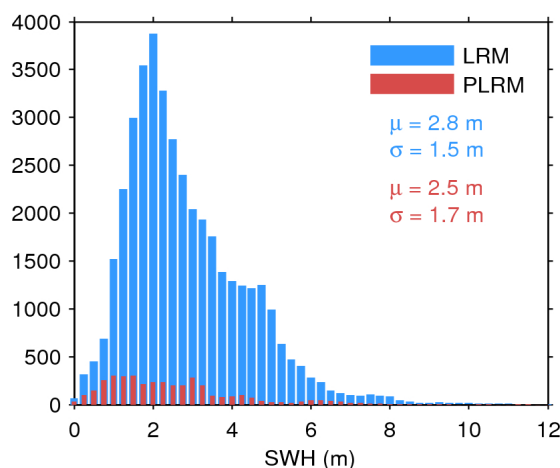
Figure 17. Histogram of flag-valid SWH over oceans and lakes for LRM (blue) and PLRM (red) for 28/04/2017. The mean ( \mu ) and standard deviation ( \sigma ) are also shown. Note that values larger than 12 m are excluded from the histogram for the sake of readability but not from the computation of \mu and \sigma .
