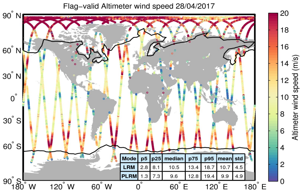
Figure 31. Geographical distribution of flag-valid wind data over oceans and lakes for 28/04/2017. The statistical values shown in the table refer to the wind in m/s and are calculated separately for LRM and PLRM regions. Measurements taken over polar polygons have been excluded from the computation of the statistical values. The black lines mark the outer limit of the Arctic and Antarctic polar polygons.
