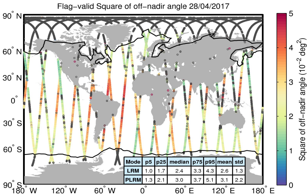
Figure 37. Geographical distribution of flag-valid mispointing data over oceans and lakes for 28/04/2017. The statistical values shown in the table refer to the mispointing in 10^{-2} deg 2 and are calculated separately for LRM and PLRM regions. Measurements taken over polar polygons have been excluded from the computation of the statistical values. The black lines mark the outer limit of the Arctic and Antarctic polar polygons. Gray circles denote negative values.
