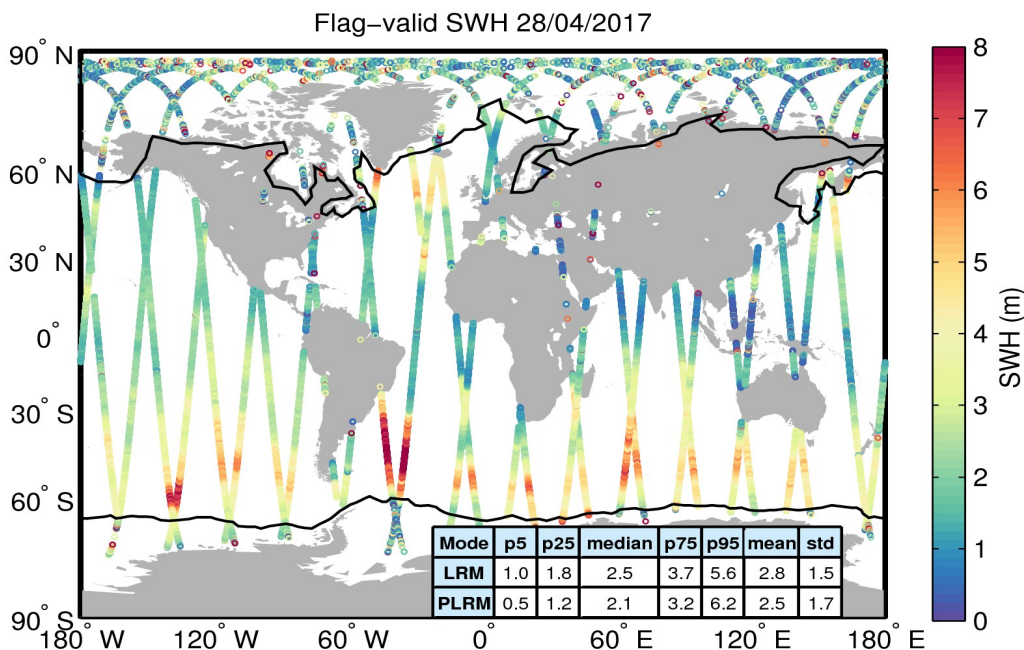
Figure 15. Geographical distribution of flag-valid SWH data over oceans and lakes for 28/04/2017. The statistical values shown in the table refer to the SWH in m and are calculated separately for LRM and PLRM regions. Measurements taken over polar polygons have been excluded from the computation of the statistical values. The black lines mark the outer limit of the Arctic and Antarctic polar polygons.
