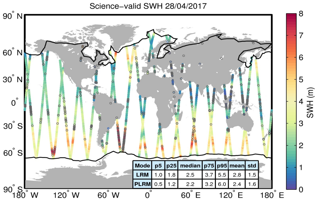
Figure 19. Geographical distribution of science-valid SWH data over oceans and lakes for 28/04/2017. The statistical values shown in the table refer to the SWH in m and are calculated separately for LRM and PLRM regions. The black lines mark the outer limit of the Arctic and Antarctic polar polygons. Gray circles denote records that have been rejected based on the editing criteria described in Table 3.
