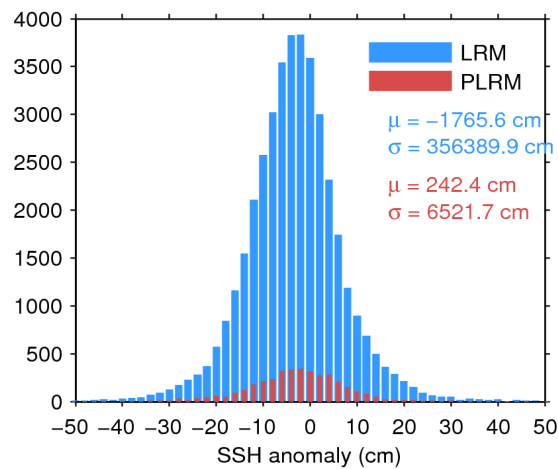
Figure 7. Histogram of flag-valid SSH anomaly over oceans and lakes for LRM (blue) and PLRM (red) for 28/04/2017. The mean ( \mu ) and standard deviation ( \sigma ) are also shown. Note that values outside [-50 \ 50] cm are excluded from the histogram for the sake of readability but not from the computation of \mu and \sigma .
