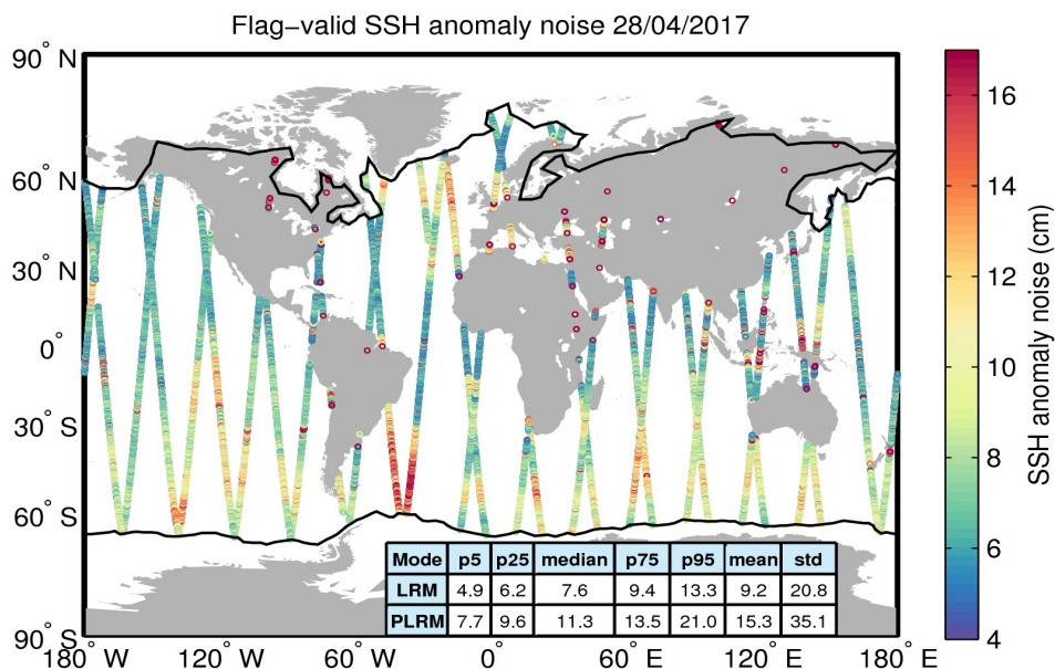
Figure 8. Geographical distribution of flag-valid 20-Hz SSH anomaly measurement noise over oceans and lakes for 28/04/2017. The statistical values shown in the table refer to the SSH anomaly noise and are calculated separately for LRM and PLRM regions. Measurements taken over polar polygons have been excluded from the computation of the statistical values. The black lines mark the outer limit of the Arctic and Antarctic polar polygons.
