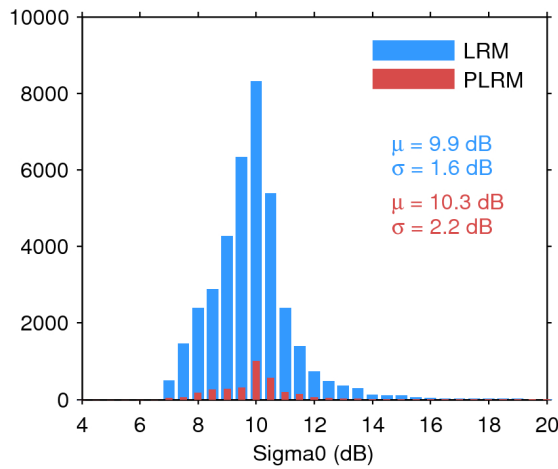
Figure 28. Histogram of science-valid sigma0 over oceans and lakes for LRM (blue) and PLRM (red) for 28/04/2017. The mean ( \mu ) and standard deviation ( \sigma ) are also shown. Note that values outside [4 20] dB are excluded from the histogram for the sake of readability but not from the computation of \mu and \sigma .
