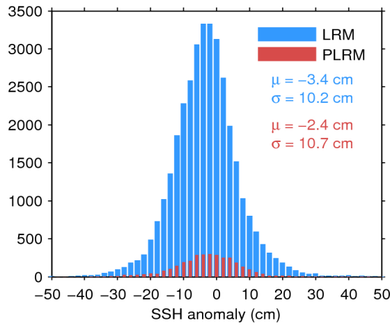
Figure 11. Histogram of science-valid SSH anomaly over oceans and lakes for LRM (blue) and PLRM (red) for 28/04/2017. The mean ( \mu ) and standard deviation ( \sigma ) are also shown. Note that values outside [-50\ 50] cm are excluded from the histogram for the sake of readability but not from the computation of \mu and \sigma .
