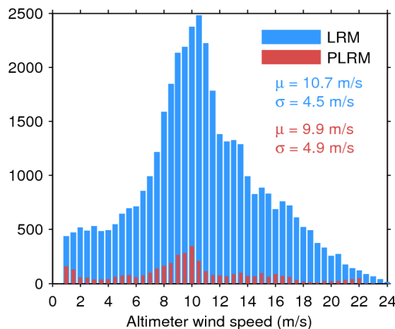
Figure 35. Histogram of science-valid wind over oceans and lakes for LRM (blue) and PLRM (red) for 28/04/2017. The mean ( \mu ) and standard deviation ( \sigma ) are also shown. Note that values larger than 24 m/s are excluded from the histogram for the sake of readability but not from the computation of \mu and \sigma .
