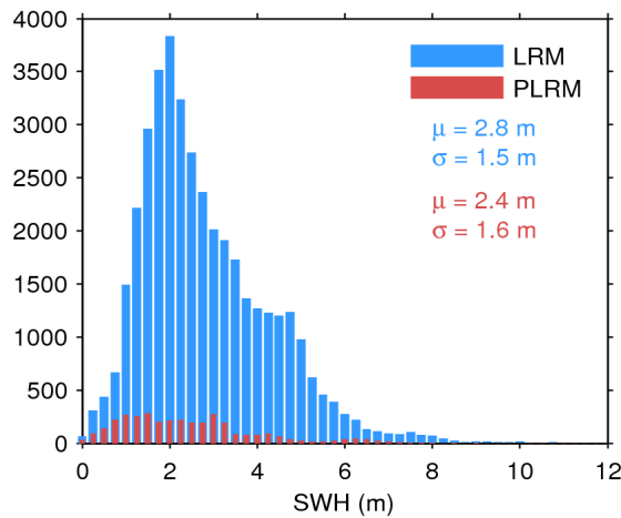
Figure 20. Histogram of science-valid SWH over oceans and lakes for LRM (blue) and PLRM (red) for 28/04/2017. The mean ( \mu ) and standard deviation ( \sigma ) are also shown. Note that values larger than 12 m are excluded from the histogram for the sake of readability but not from the computation of \mu and \sigma .
