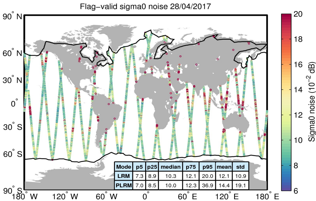
Figure 26. Geographical distribution of flag-valid 20-Hz sigma0 measurement noise over oceans and lakes for 28/04/2017. The statistical values shown in the table refer to the sigma0 noise and are calculated separately for LRM and PLRM regions. Measurements taken over polar polygons have been excluded from the computation of the statistical values. The black lines mark the outer limit of the Arctic and Antarctic polar polygons.
