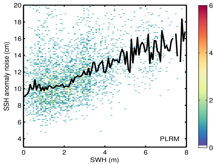
Figure 9. 2D histogram showing flag-valid SSH anomaly noise as a function of SWH for LRM (top) and PLRM (bottom) for 28/04/2017. The black line denotes the median SSH anomaly noise as a function of SWH.
