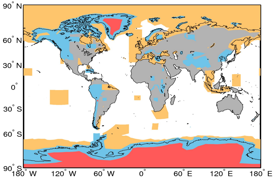
Figure A1. Extent of the regions defining the geographical mode mask for 28/04/2017. The regions where SAR, and SARIn are operated are denoted by the orange and blue polygons, respectively. LRM is operated over areas of the continental ice sheets (red polygons) and over oceans and land not covered by other modes.
