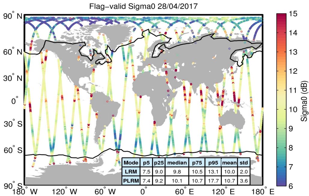
Figure 23. Geographical distribution of flag-valid sigma0 data over oceans and lakes for 28/04/2017. The statistical values shown in the table refer to the sigma0 in dB and are calculated separately for LRM and PLRM regions. Measurements taken over polar polygons have been excluded from the computation of the statistical values. The black lines mark the outer limit of the Arctic and Antarctic polar polygons.
