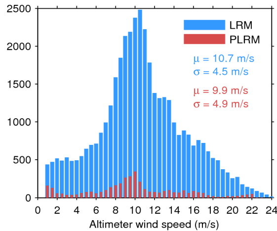
Figure 33. Histogram of flag-valid wind over oceans and lakes for LRM (blue) and PLRM (red) for 28/04/2017. The mean ( \mu ) and standard deviation ( \sigma ) are also shown. Note that values larger than 24 m/s are excluded from the histogram for the sake of readability but not from the computation of \mu and \sigma .
